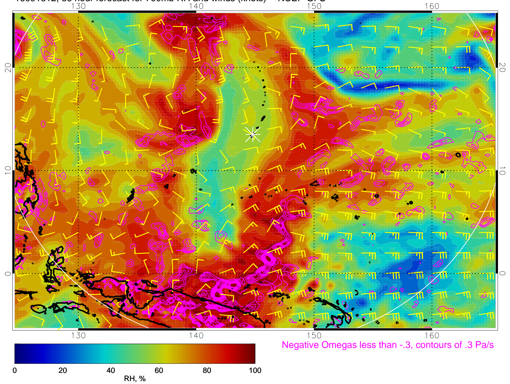
16091612, 36 hour forecast for 700mb RH and winds (knots) -- NCEP GFS
