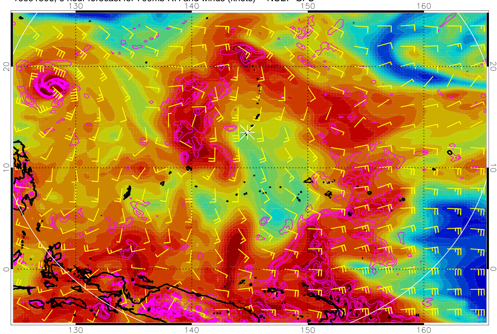
16091506, 6 hour forecast for 700mb RH and winds (knots) -- NCEP GFS
