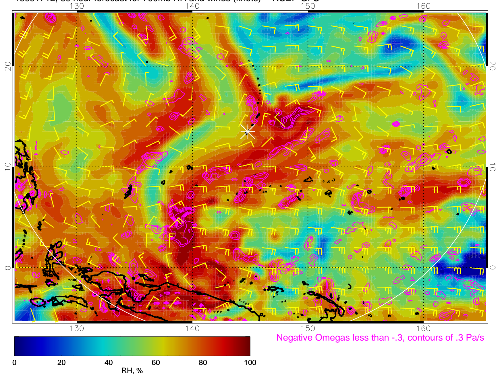
16091712, 60 hour forecast for 700mb RH and winds (knots) -- NCEP GFS
