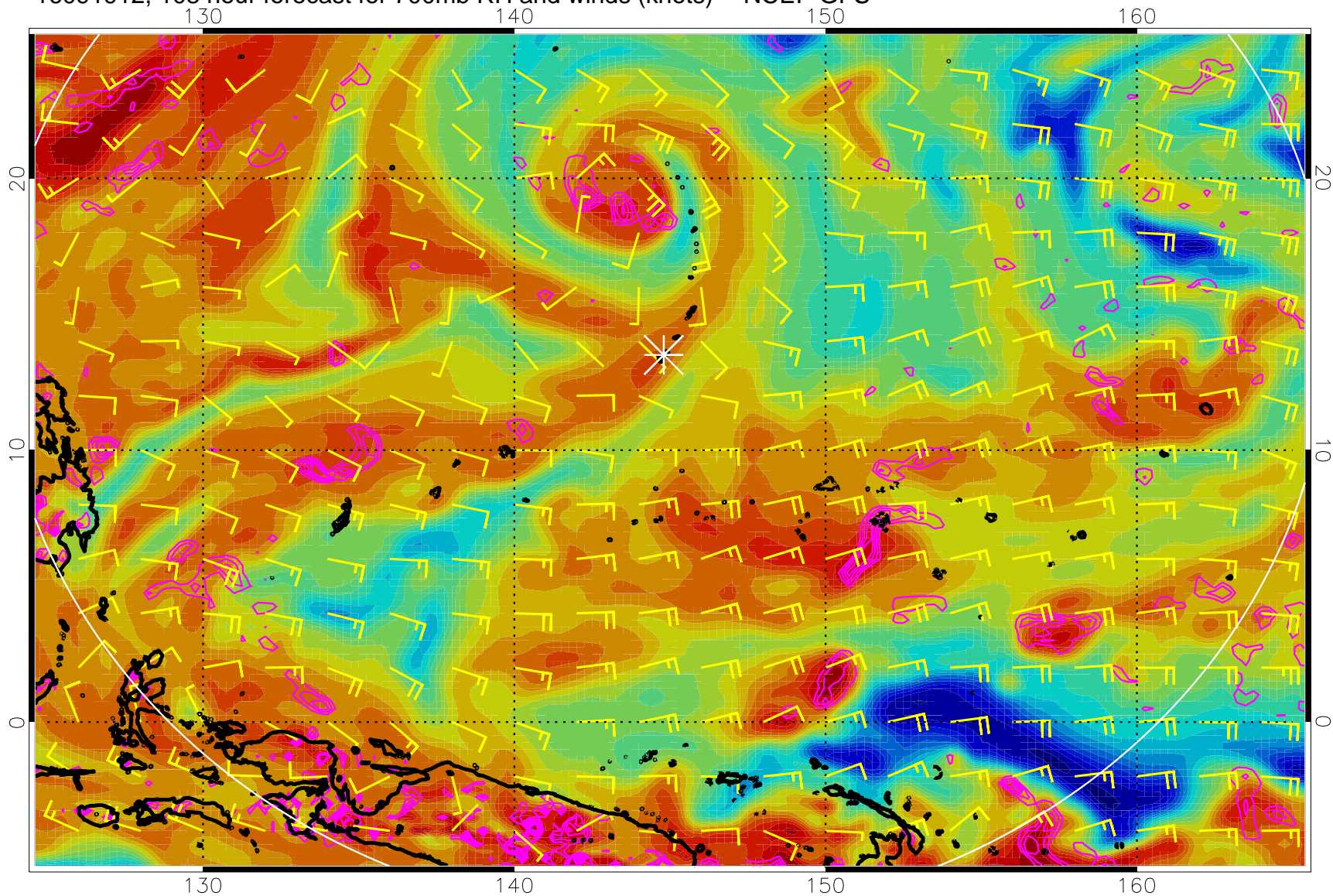
16091912, 108 hour forecast for 700mb RH and winds (knots) -- NCEP GFS
