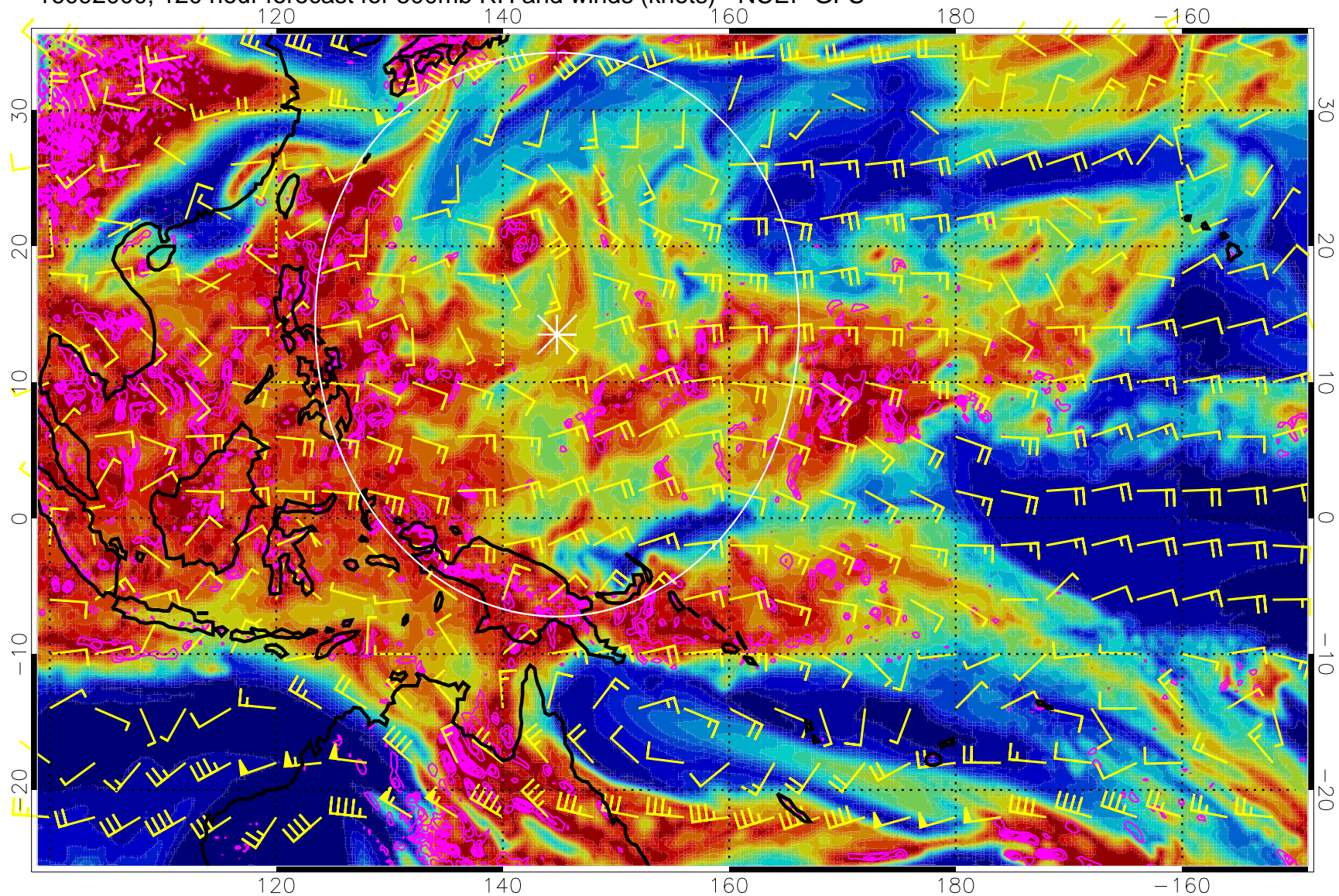
16092000, 120 hour forecast for 500mb RH and winds (knots) - NCEP GFS
