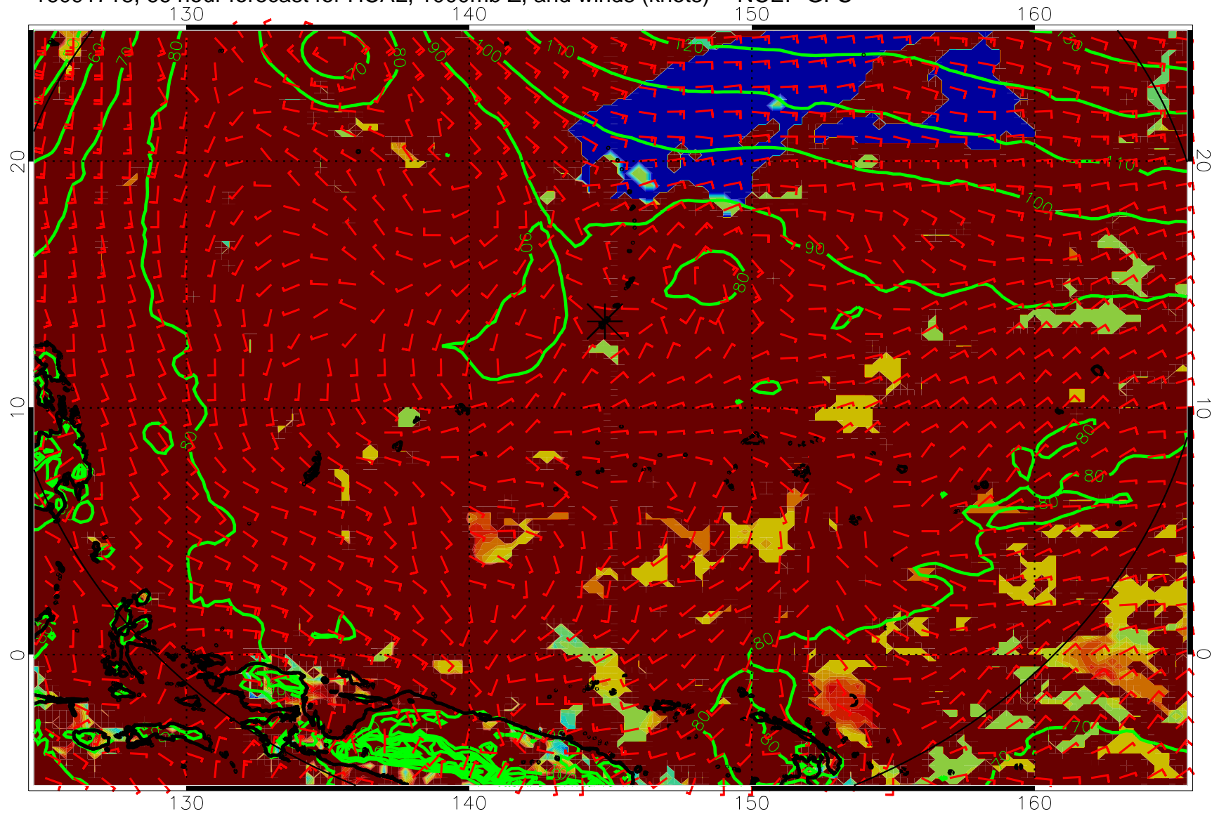
16091718, 66 hour forecast for HCAL, 1000mb Z, and winds (knots) -- NCEP GFS
