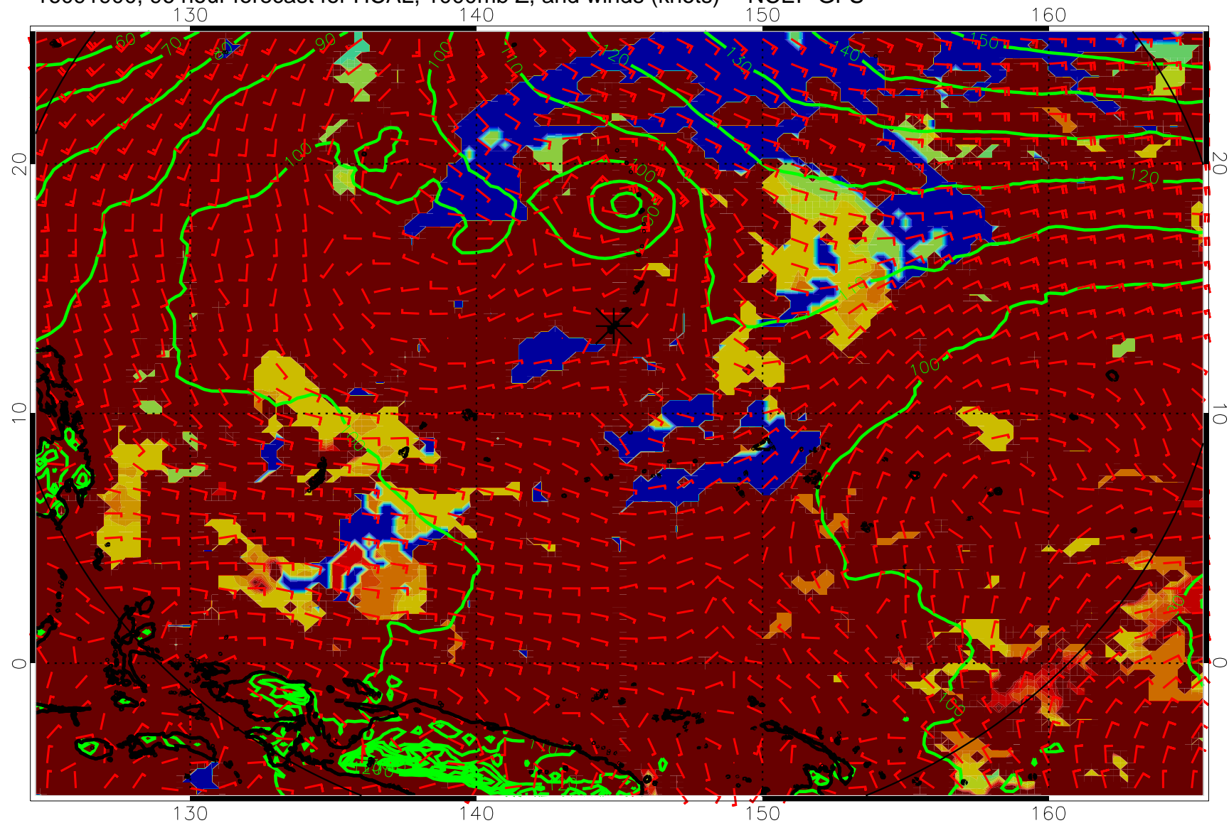
16091900, 96 hour forecast for HCAL, 1000mb Z, and winds (knots) -- NCEP GFS
