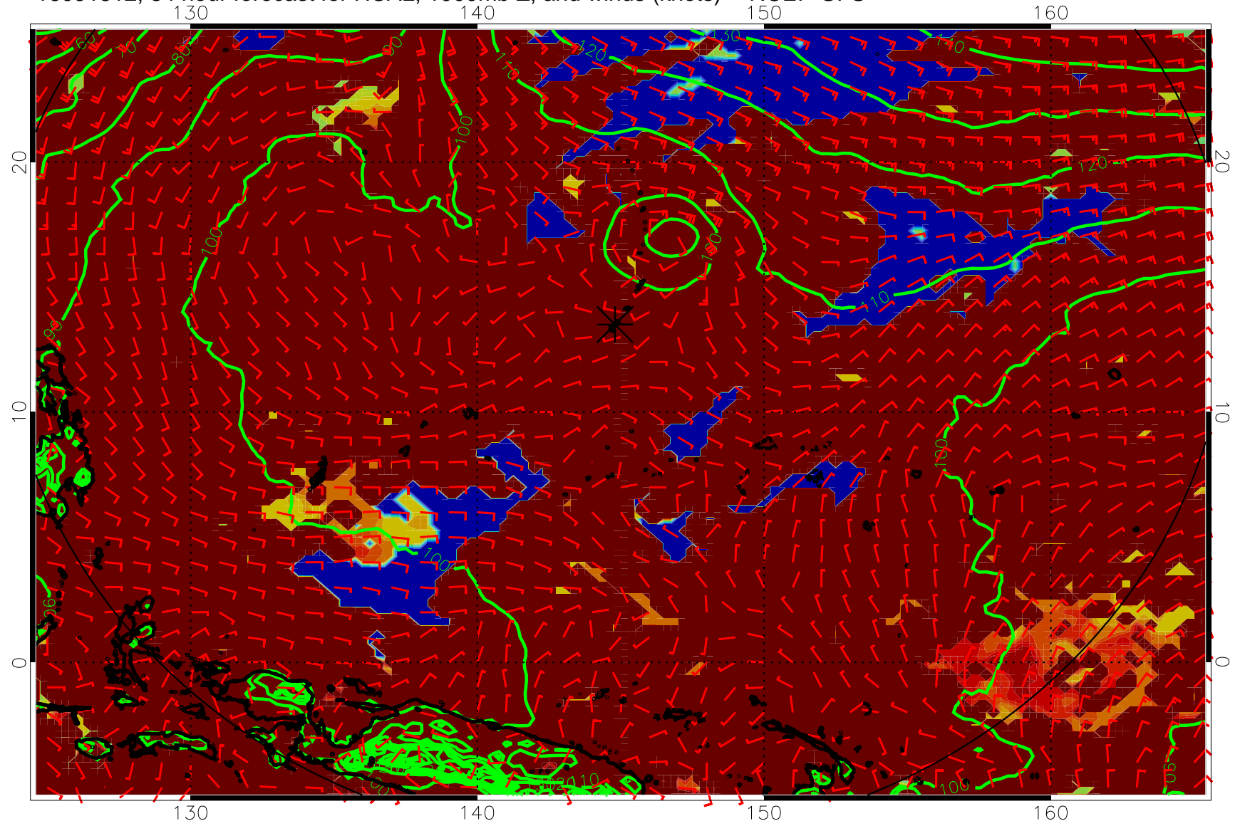
16091812, 84 hour forecast for HCAL, 1000mb Z, and winds (knots) -- NCEP GFS
