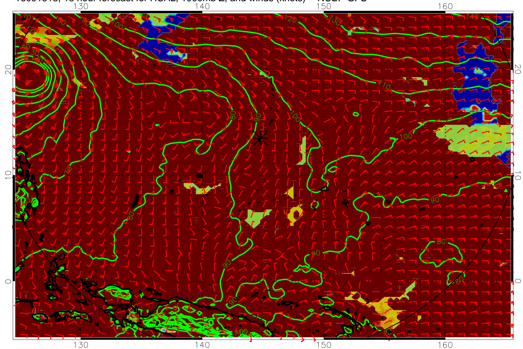
16091518, 18 hour forecast for HCAL, 1000mb Z, and winds (knots) -- NCEP GFS
