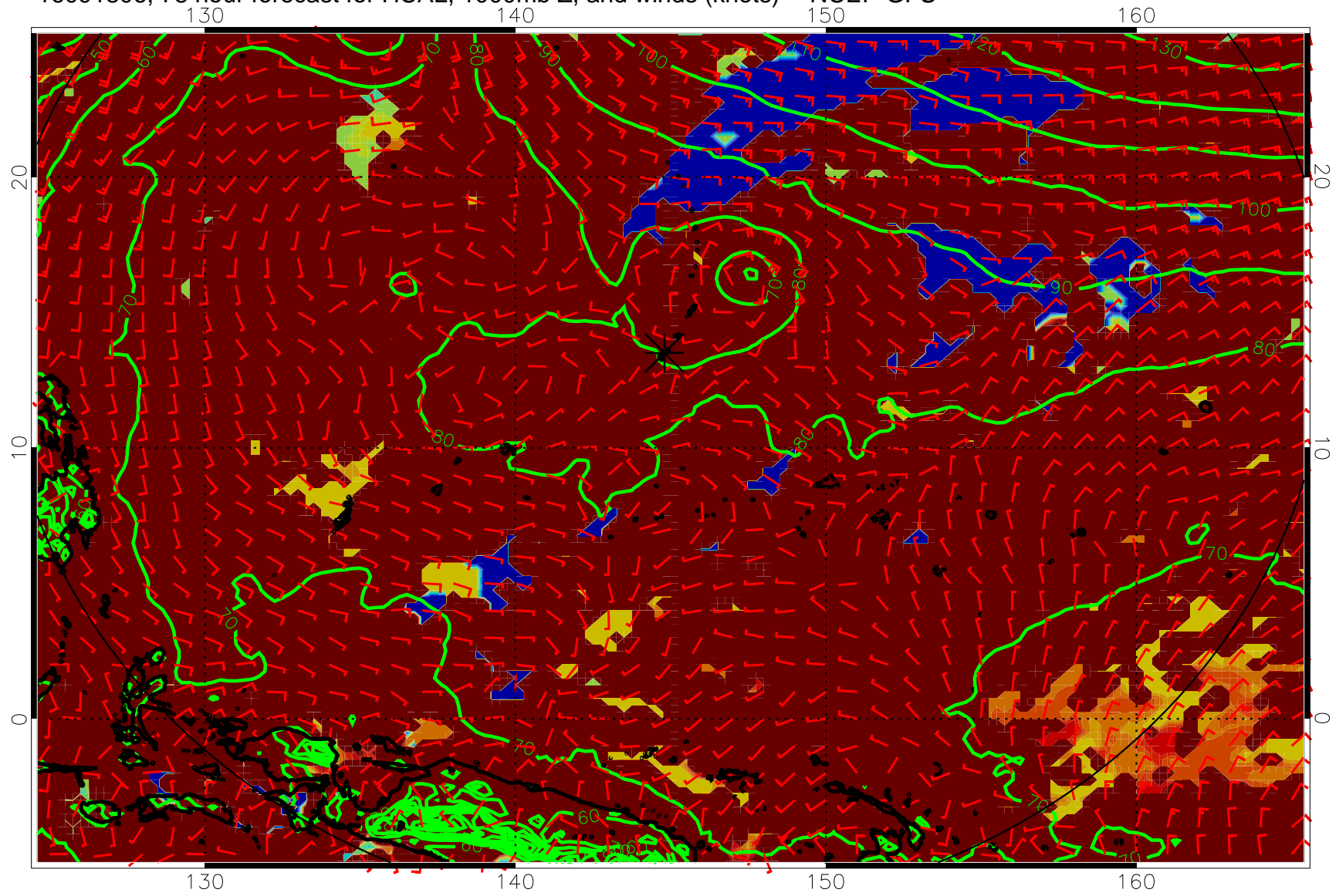
16091806, 78 hour forecast for HCAL, 1000mb Z, and winds (knots) -- NCEP GFS
