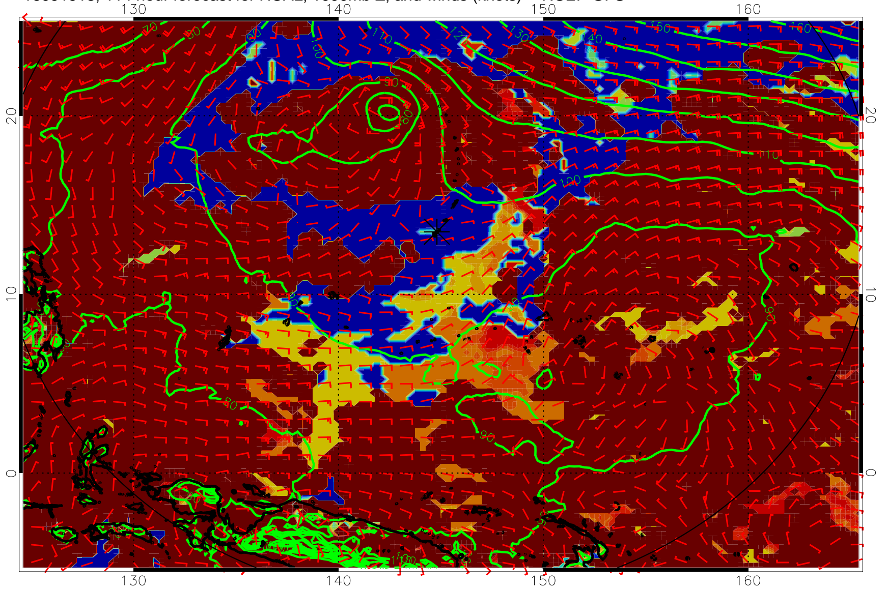
16091918, 114 hour forecast for HCAL, 1000mb Z, and winds (knots) -- NCEP GFS
