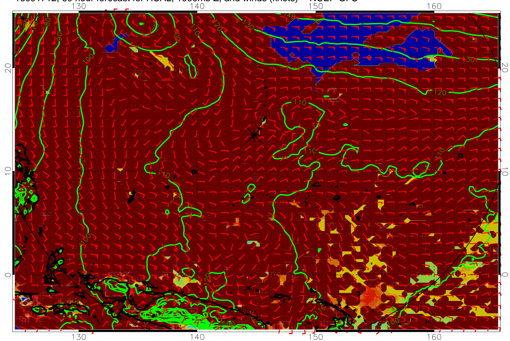
16091712, 60 hour forecast for HCAL, 1000mb Z, and winds (knots) -- NCEP GFS
