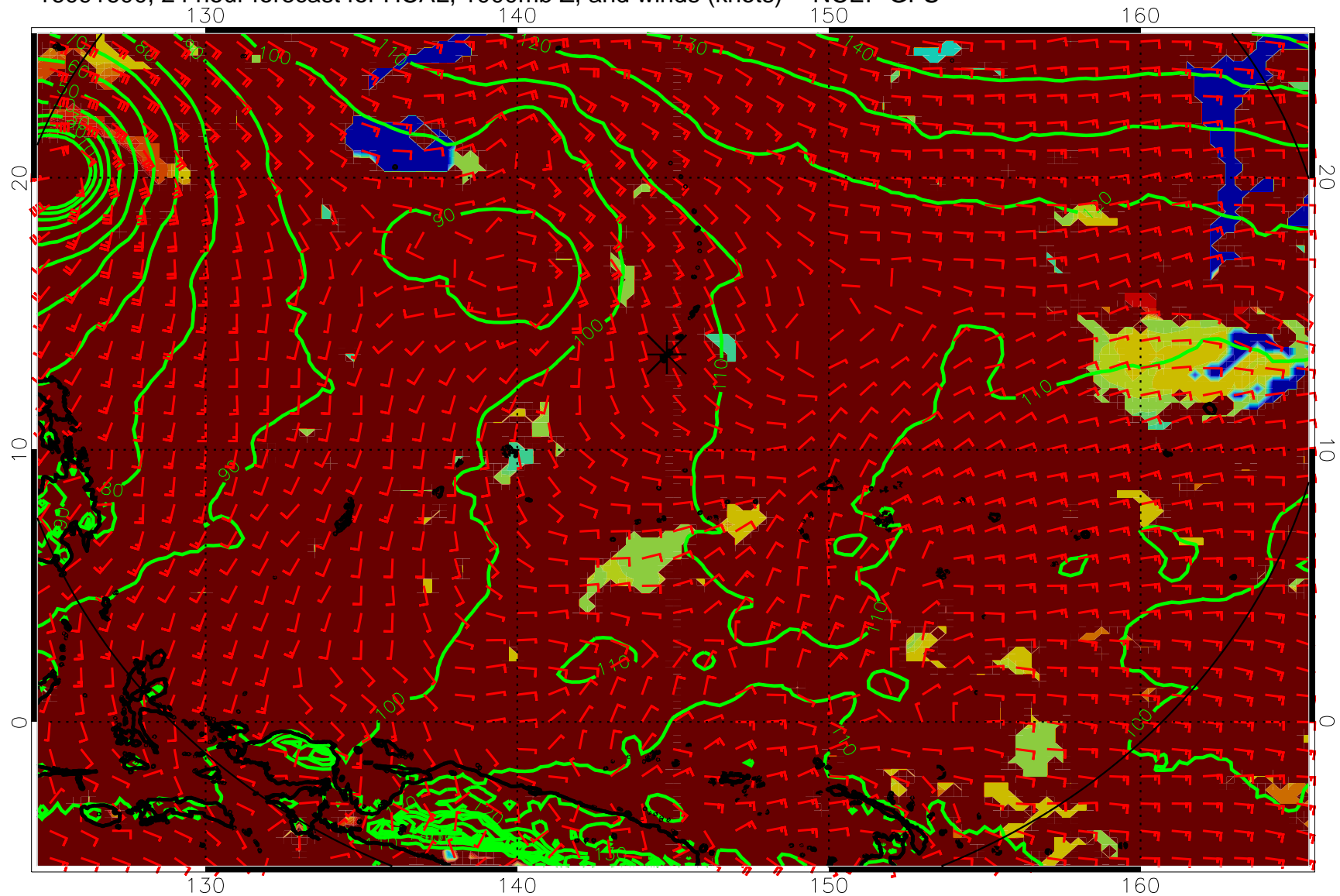
16091600, 24 hour forecast for HCAL, 1000mb Z, and winds (knots) -- NCEP GFS
