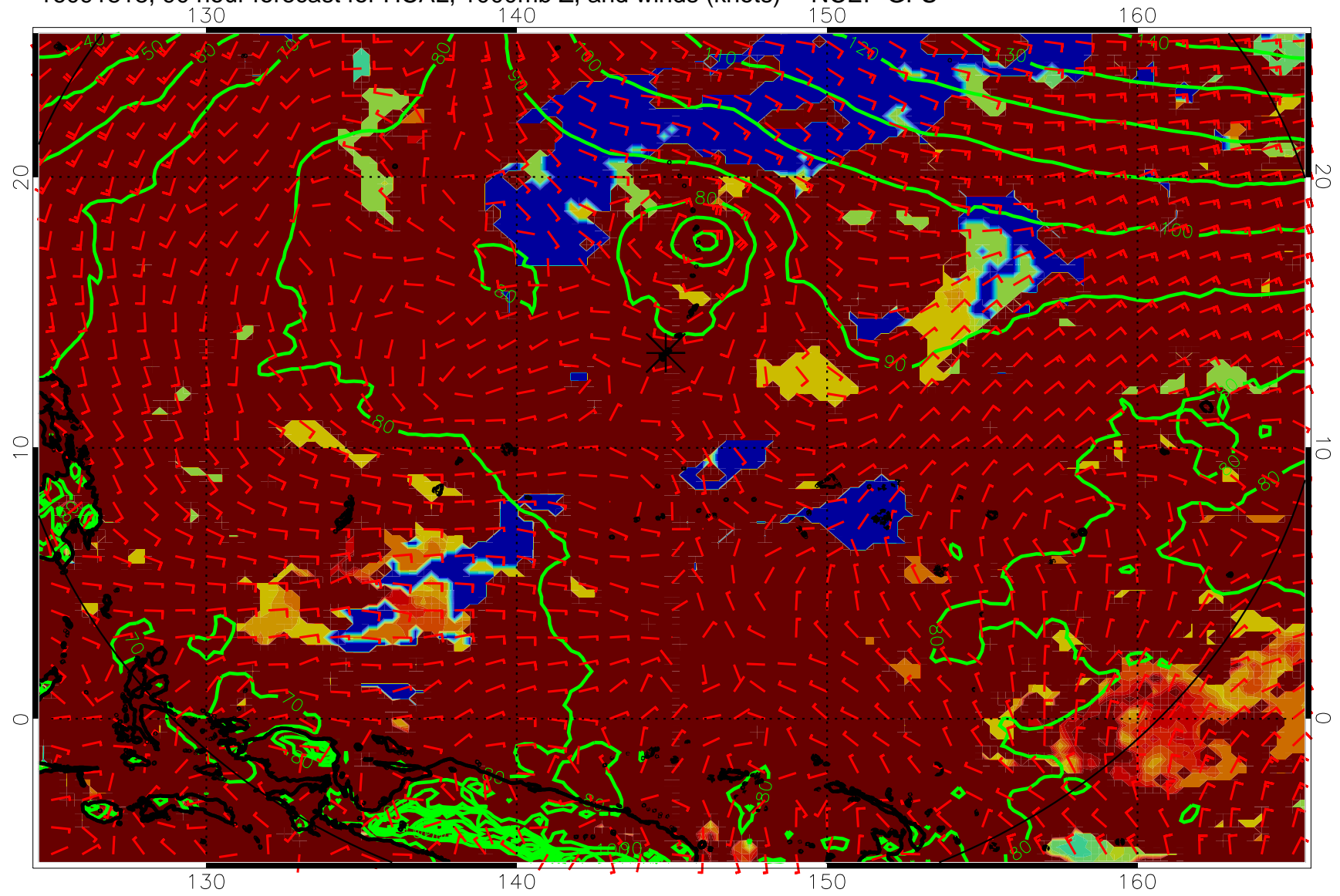
16091818, 90 hour forecast for HCAL, 1000mb Z, and winds (knots) -- NCEP GFS
