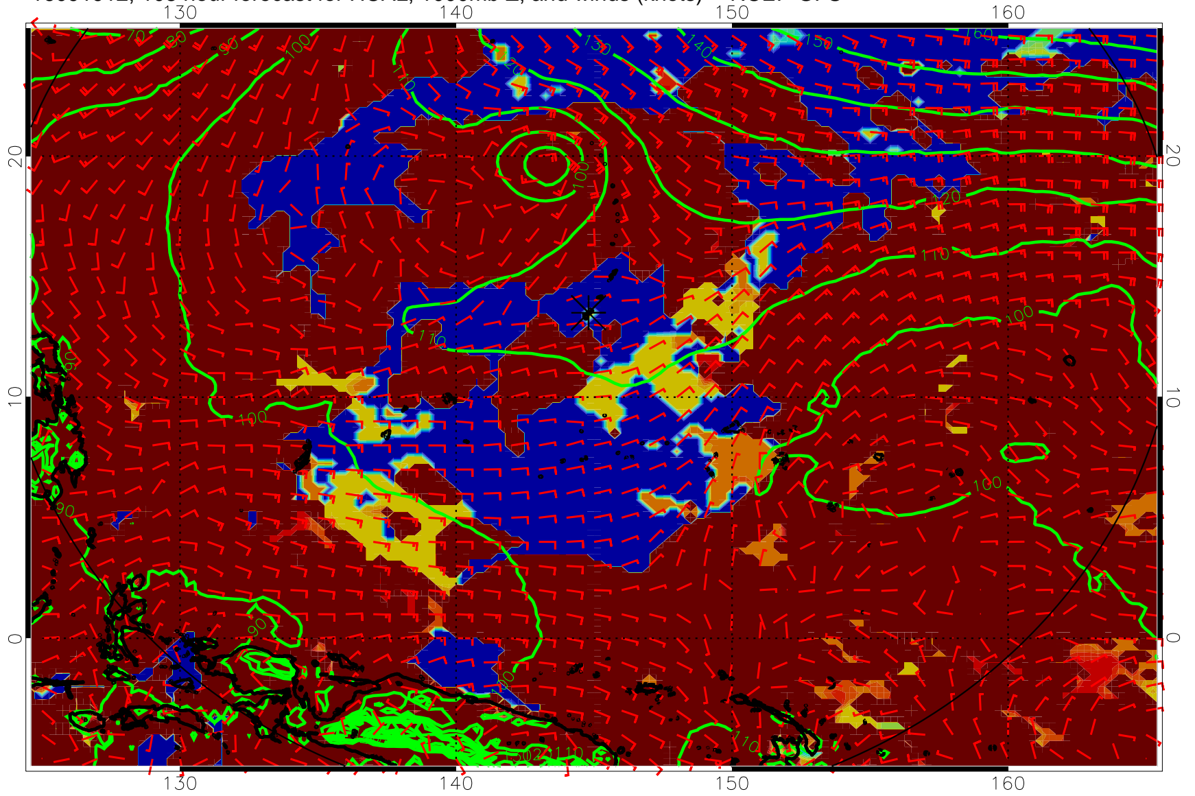
16091912, 108 hour forecast for HCAL, 1000mb Z, and winds (knots) -- NCEP GFS
