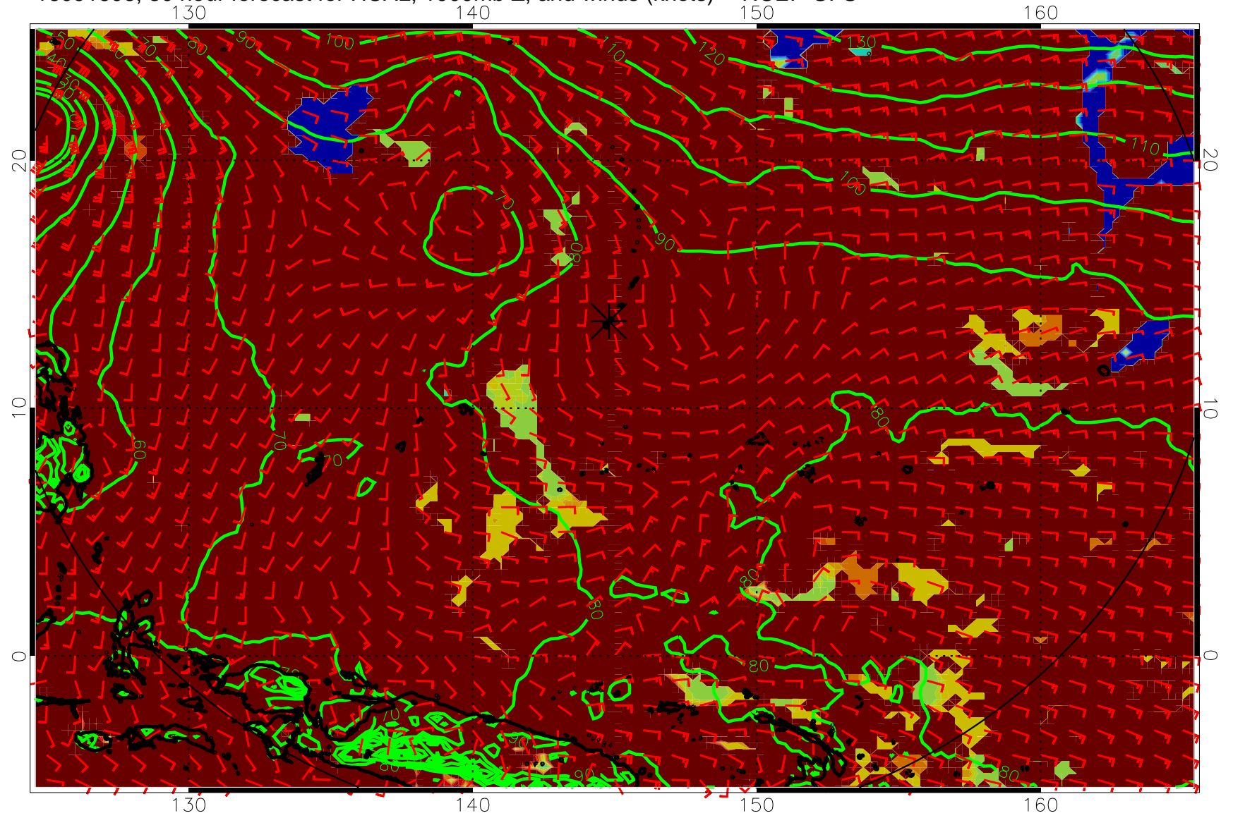
16091606, 30 hour forecast for HCAL, 1000mb Z, and winds (knots) -- NCEP GFS
