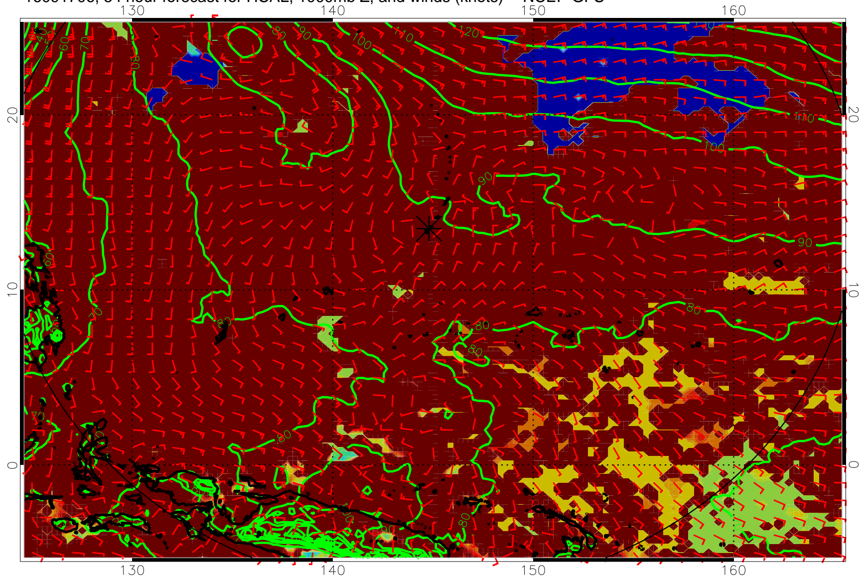
16091706, 54 hour forecast for HCAL, 1000mb Z, and winds (knots) -- NCEP GFS
