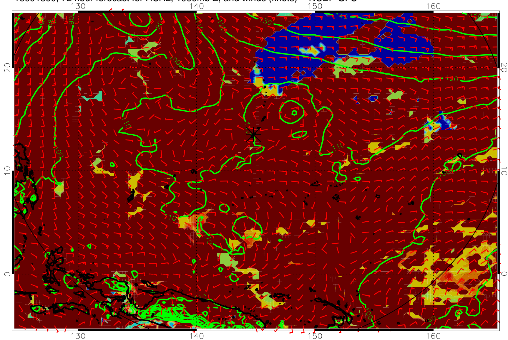
16091800, 72 hour forecast for HCAL, 1000mb Z, and winds (knots) -- NCEP GFS
