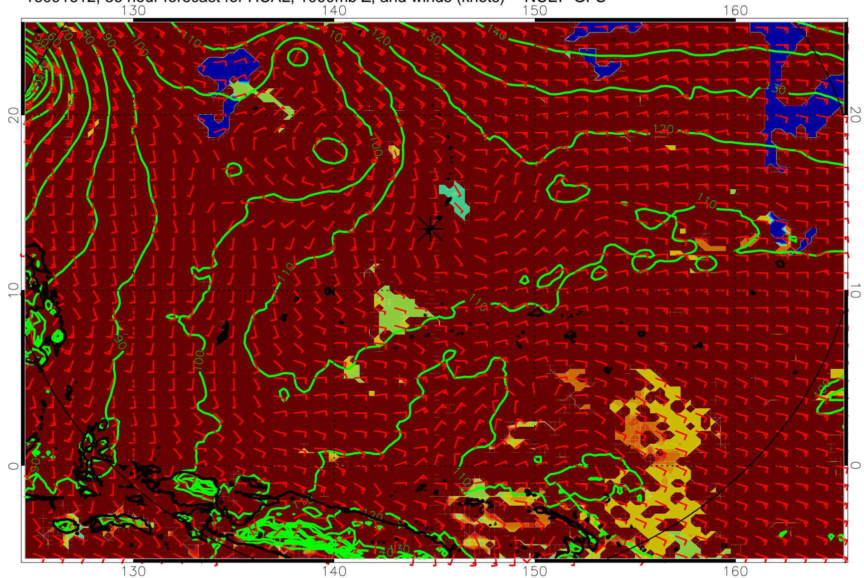
16091612, 36 hour forecast for HCAL, 1000mb Z, and winds (knots) -- NCEP GFS
