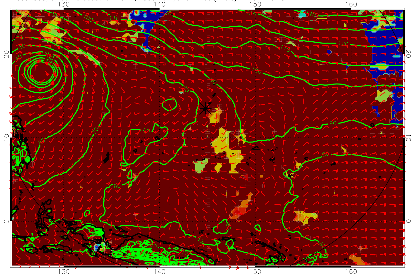
16091506, 6 hour forecast for HCAL, 1000mb Z, and winds (knots) -- NCEP GFS
