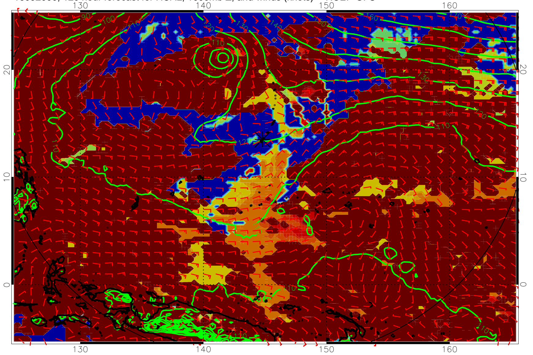
16092000, 120 hour forecast for HCAL, 1000mb Z, and winds (knots) -- NCEP GFS
