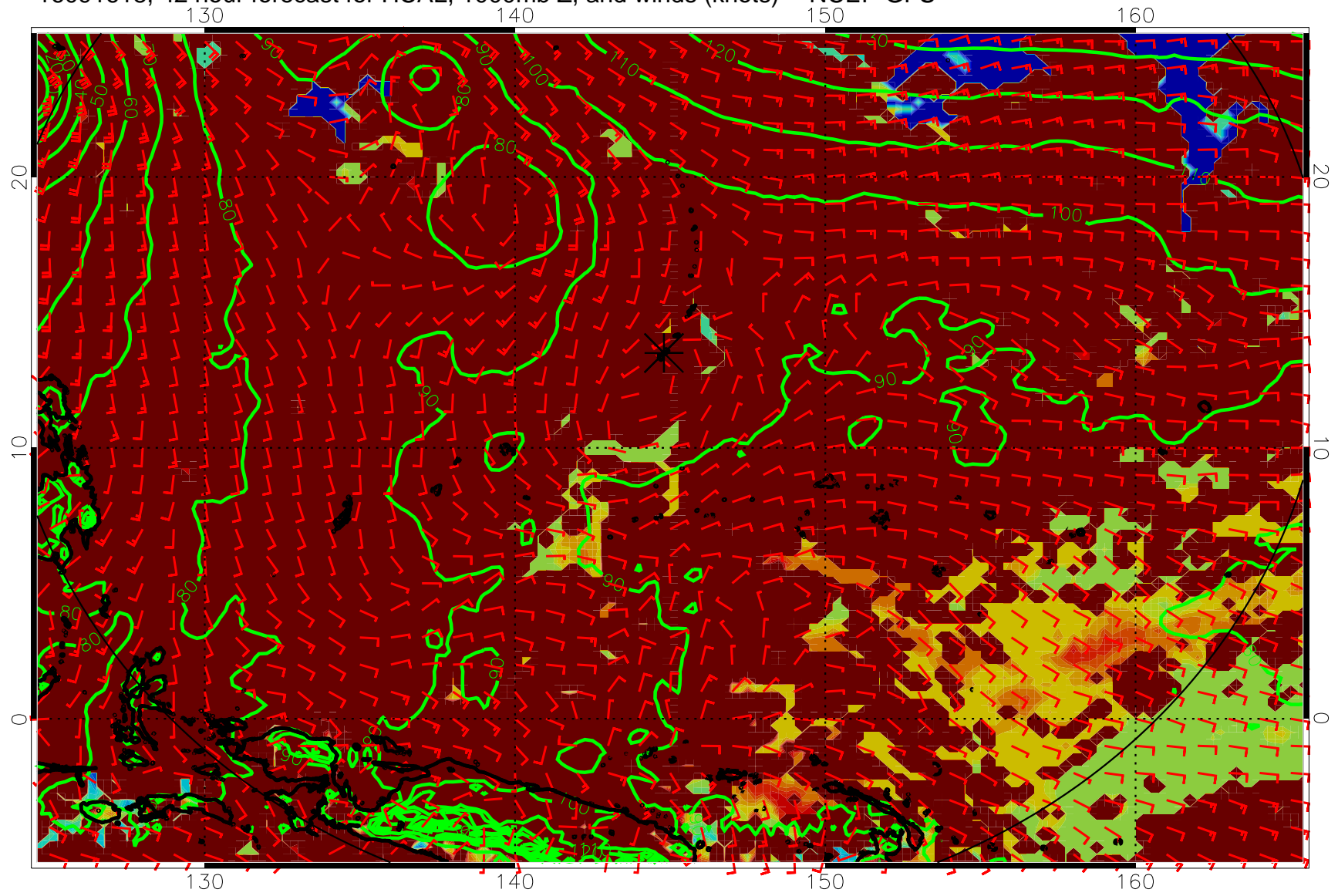
16091618, 42 hour forecast for HCAL, 1000mb Z, and winds (knots) -- NCEP GFS
