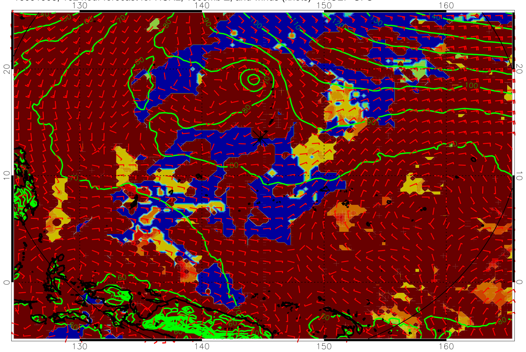
16091906, 102 hour forecast for HCAL, 1000mb Z, and winds (knots) -- NCEP GFS
