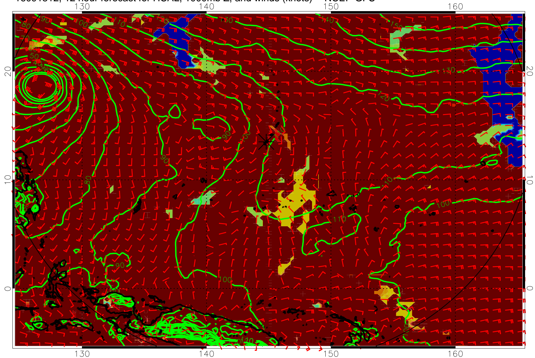
16091512, 12 hour forecast for HCAL, 1000mb Z, and winds (knots) -- NCEP GFS
