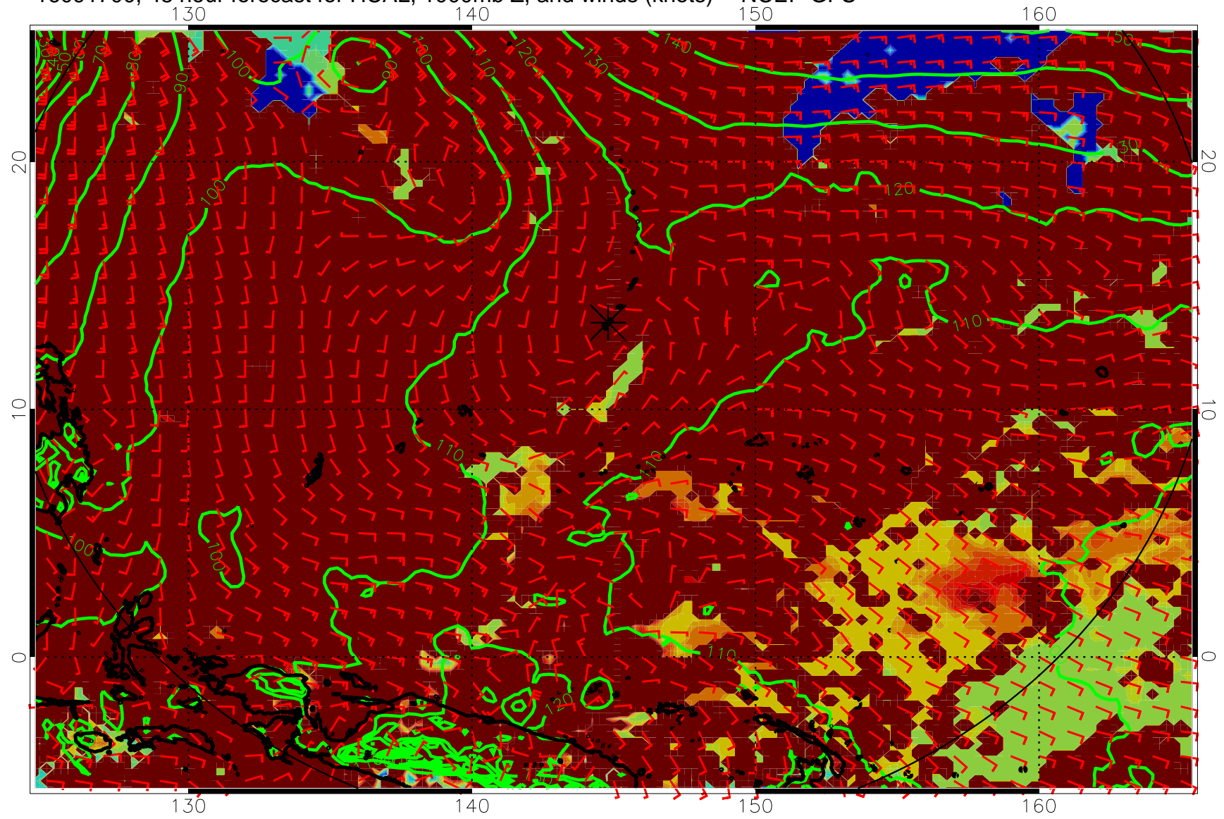
16091700, 48 hour forecast for HCAL, 1000mb Z, and winds (knots) -- NCEP GFS
