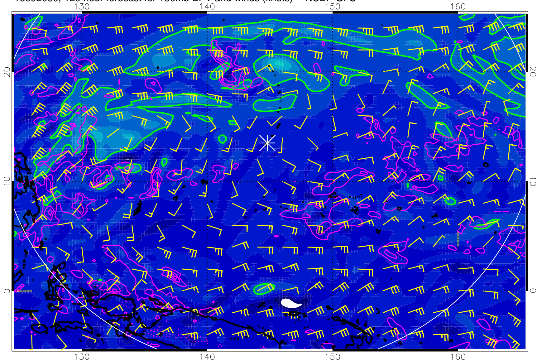
16092000, 120 hour forecast for 150mb EPV and winds (knots) -- NCEP GFS
