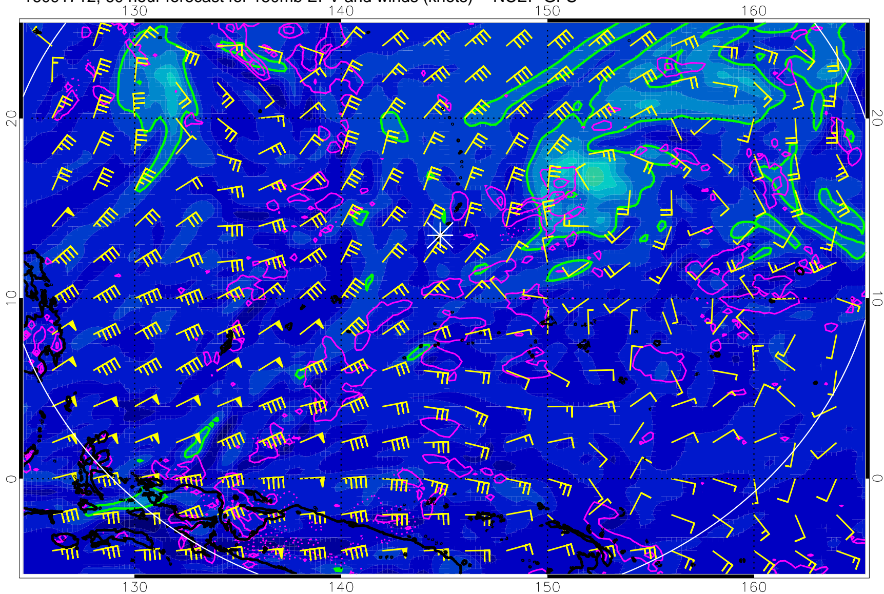
16091712, 60 hour forecast for 150mb EPV and winds (knots) -- NCEP GFS
