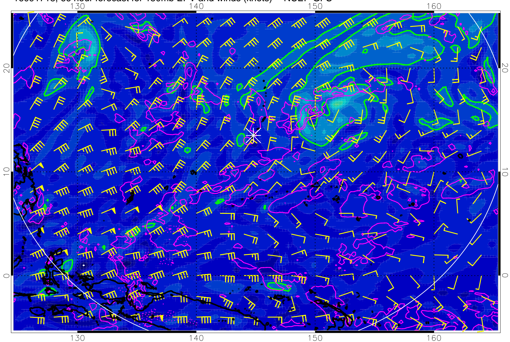
16091718, 66 hour forecast for 150mb EPV and winds (knots) -- NCEP GFS
