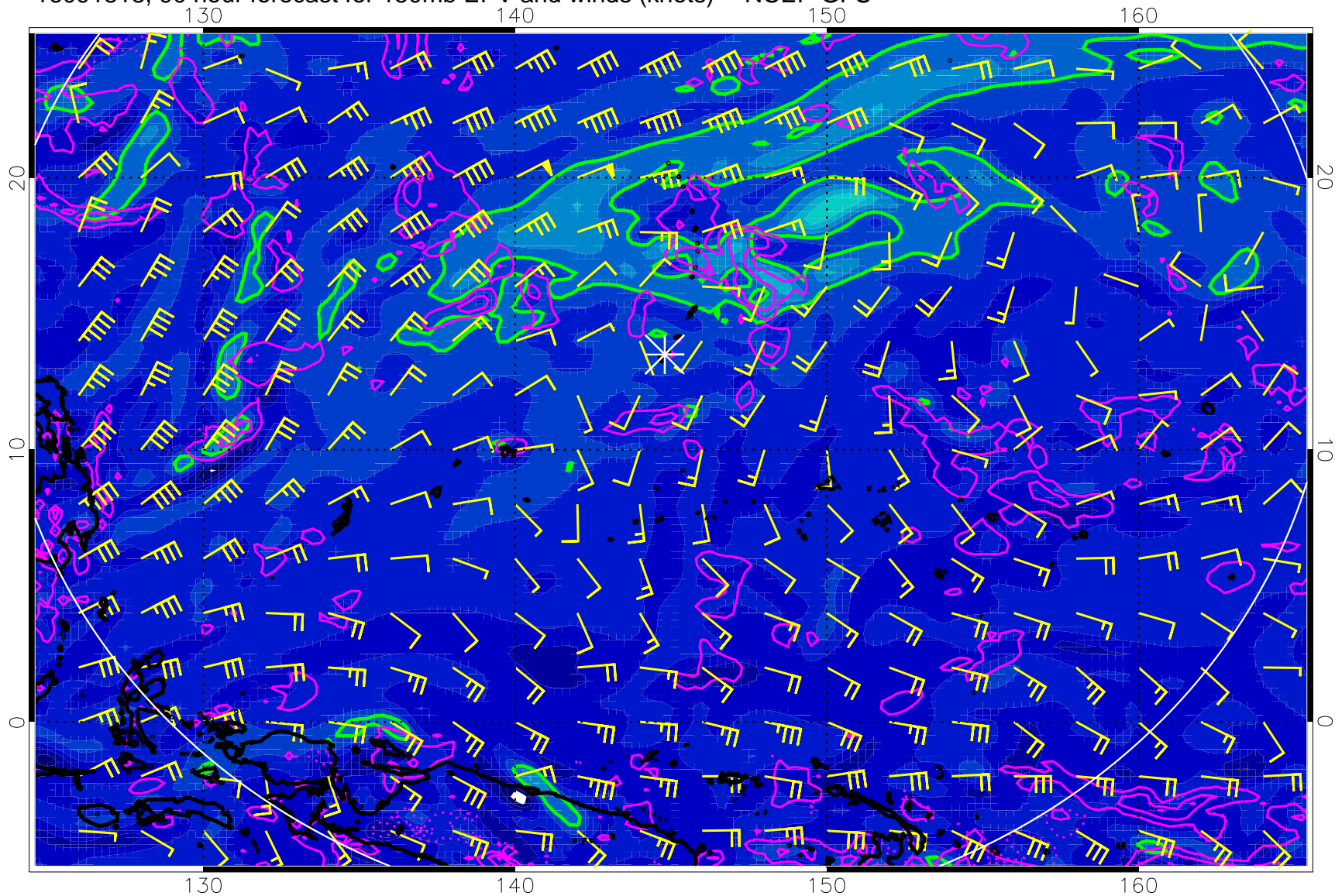
16091818, 90 hour forecast for 150mb EPV and winds (knots) -- NCEP GFS
