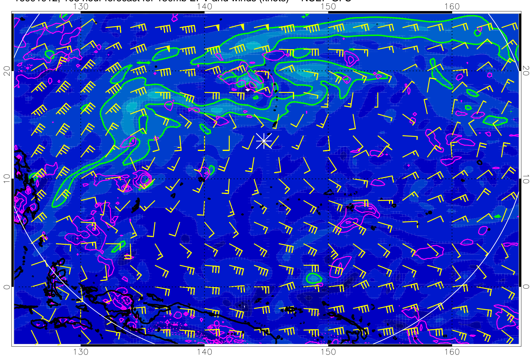
16091912, 108 hour forecast for 150mb EPV and winds (knots) -- NCEP GFS
