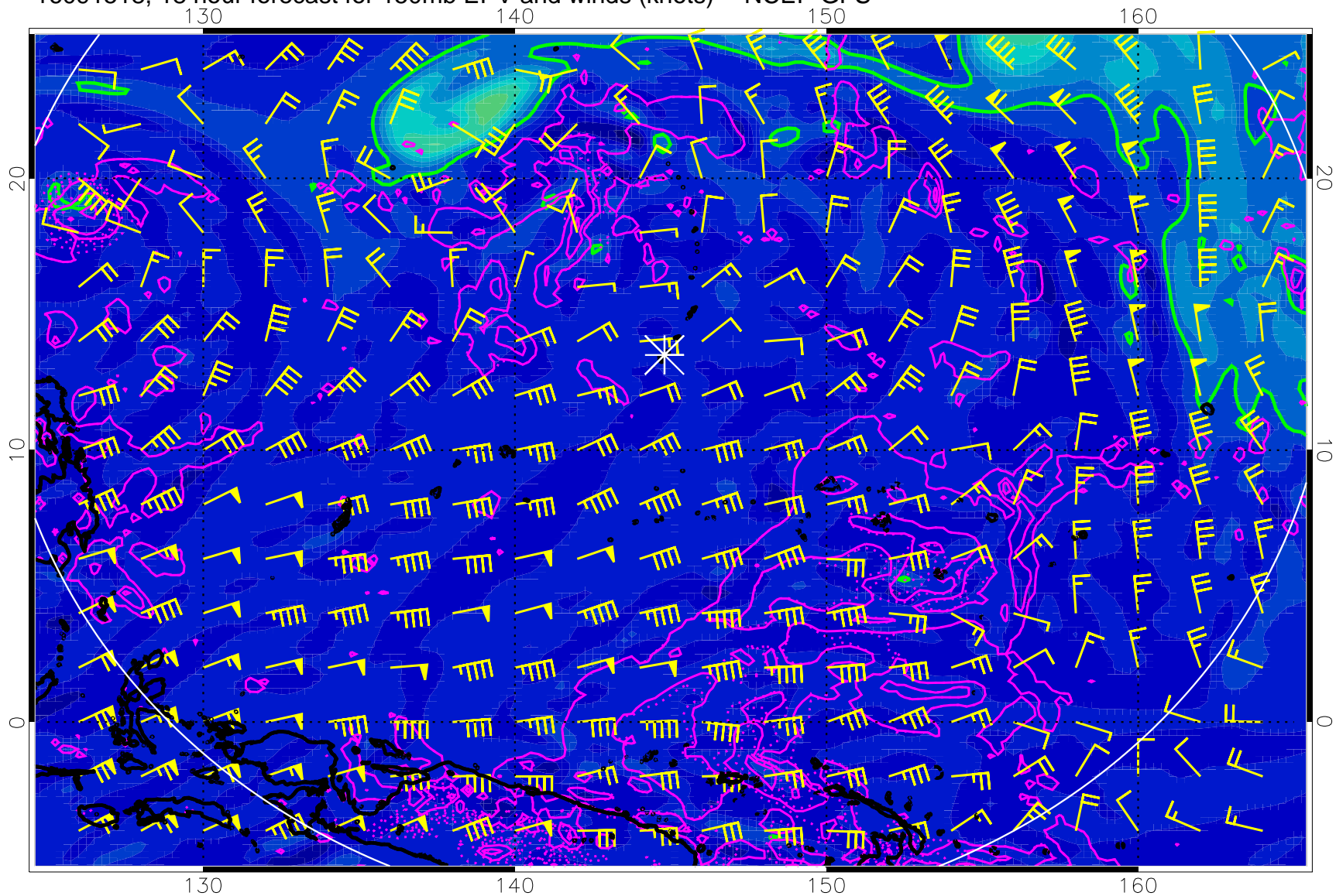
16091518, 18 hour forecast for 150mb EPV and winds (knots) -- NCEP GFS
