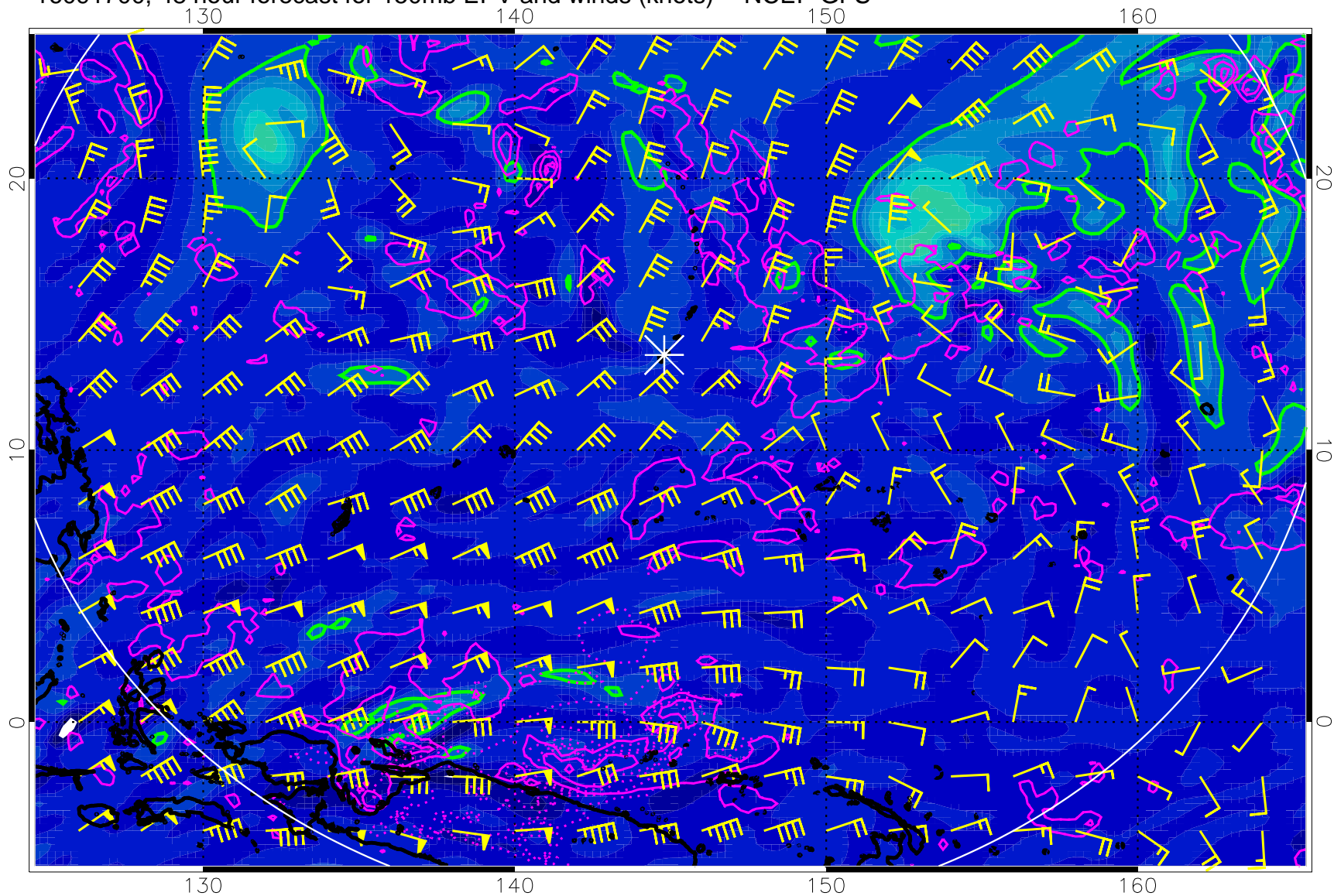
16091700, 48 hour forecast for 150mb EPV and winds (knots) -- NCEP GFS
