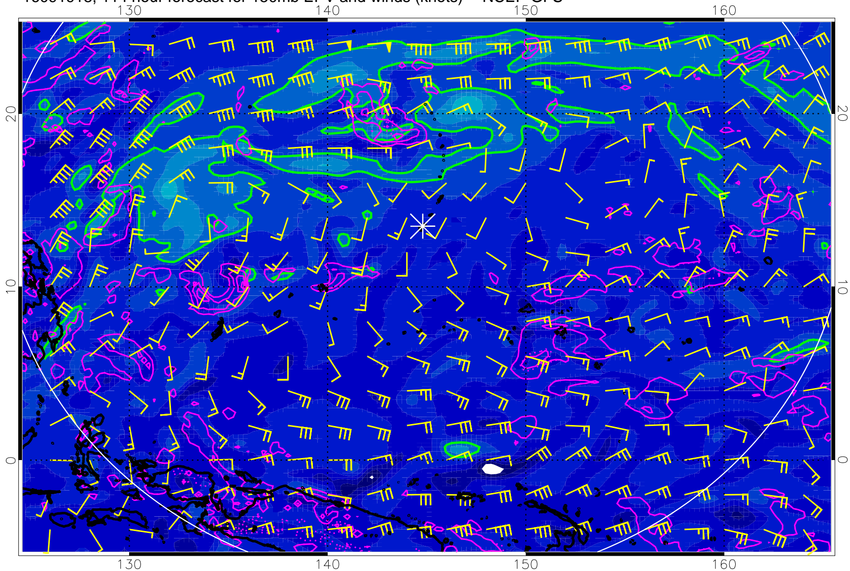
16091918, 114 hour forecast for 150mb EPV and winds (knots) -- NCEP GFS
