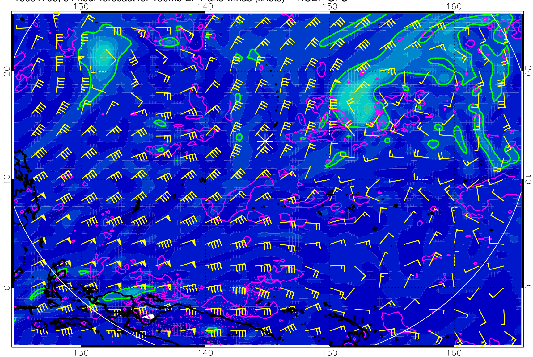
16091706, 54 hour forecast for 150mb EPV and winds (knots) -- NCEP GFS
