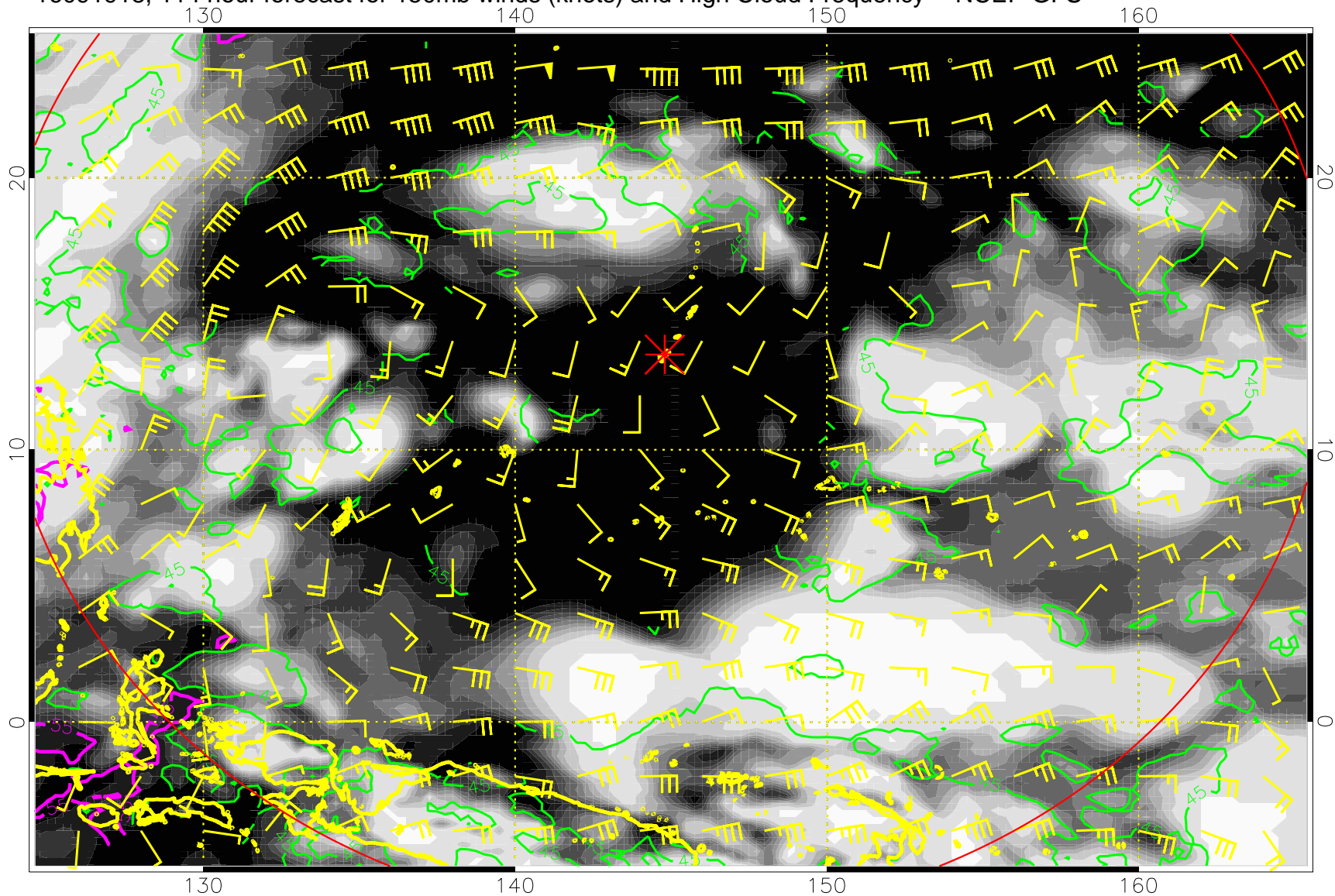
16091918, 114 hour forecast for 150mb winds (knots) and High Cloud Frequency -- NCEP GFS
