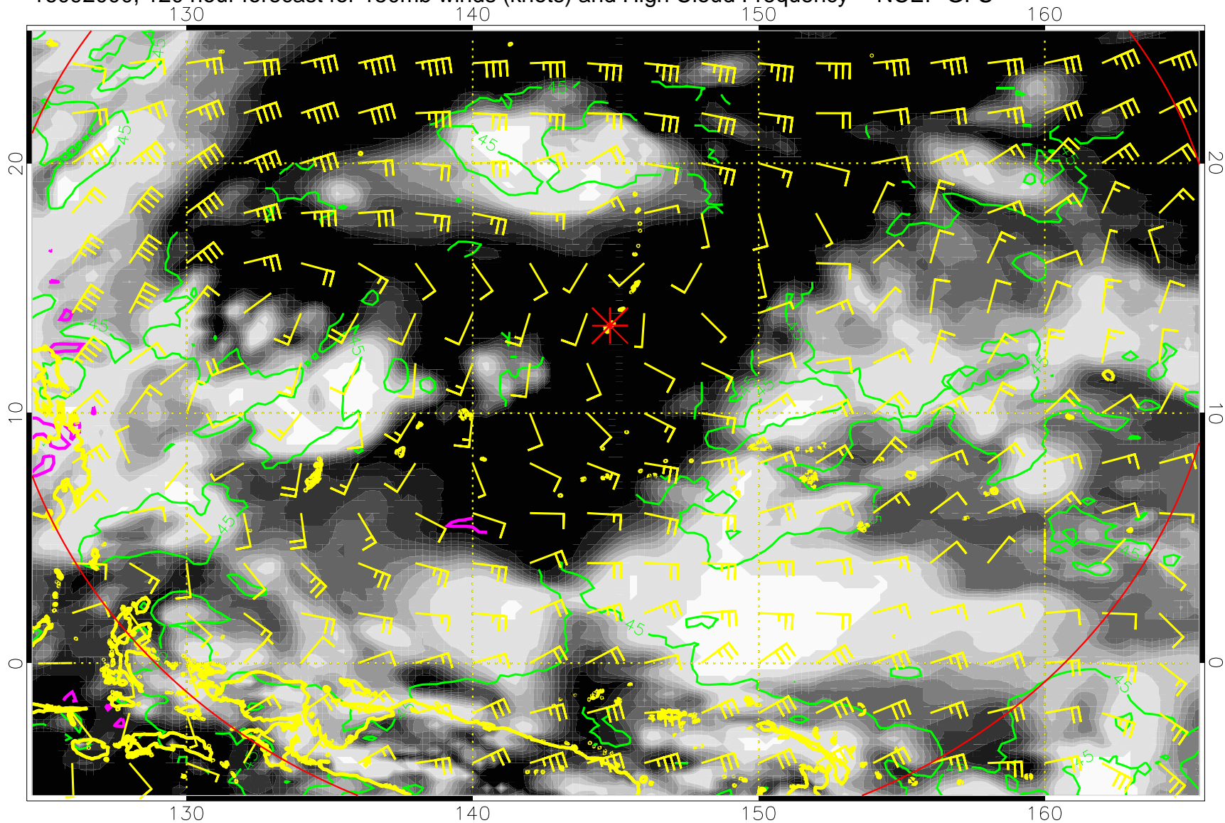
16092000, 120 hour forecast for 150mb winds (knots) and High Cloud Frequency -- NCEP GFS
