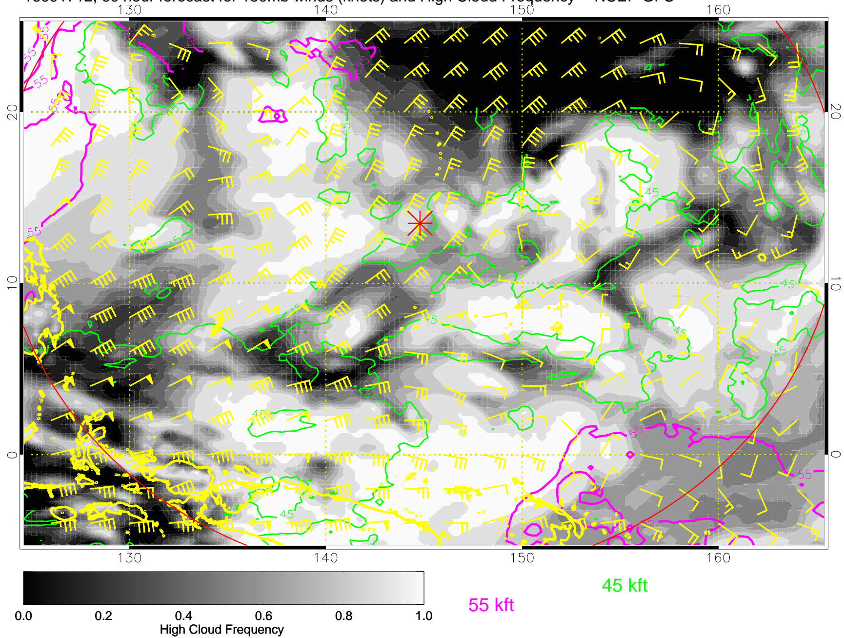
16091712, 60 hour forecast for 150mb winds (knots) and High Cloud Frequency -- NCEP GFS
