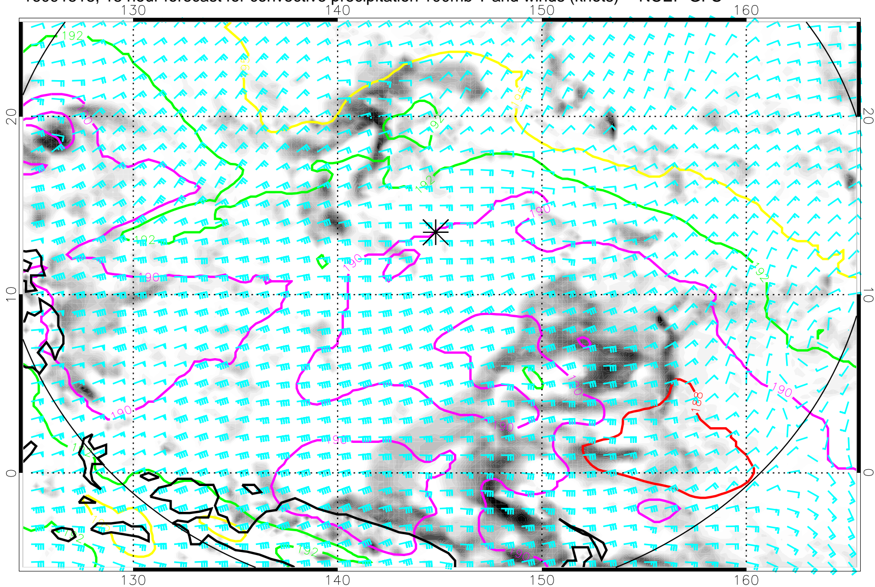
16091518, 18 hour forecast for convective precipitation 100mb T and winds (knots) -- NCEP GFS
