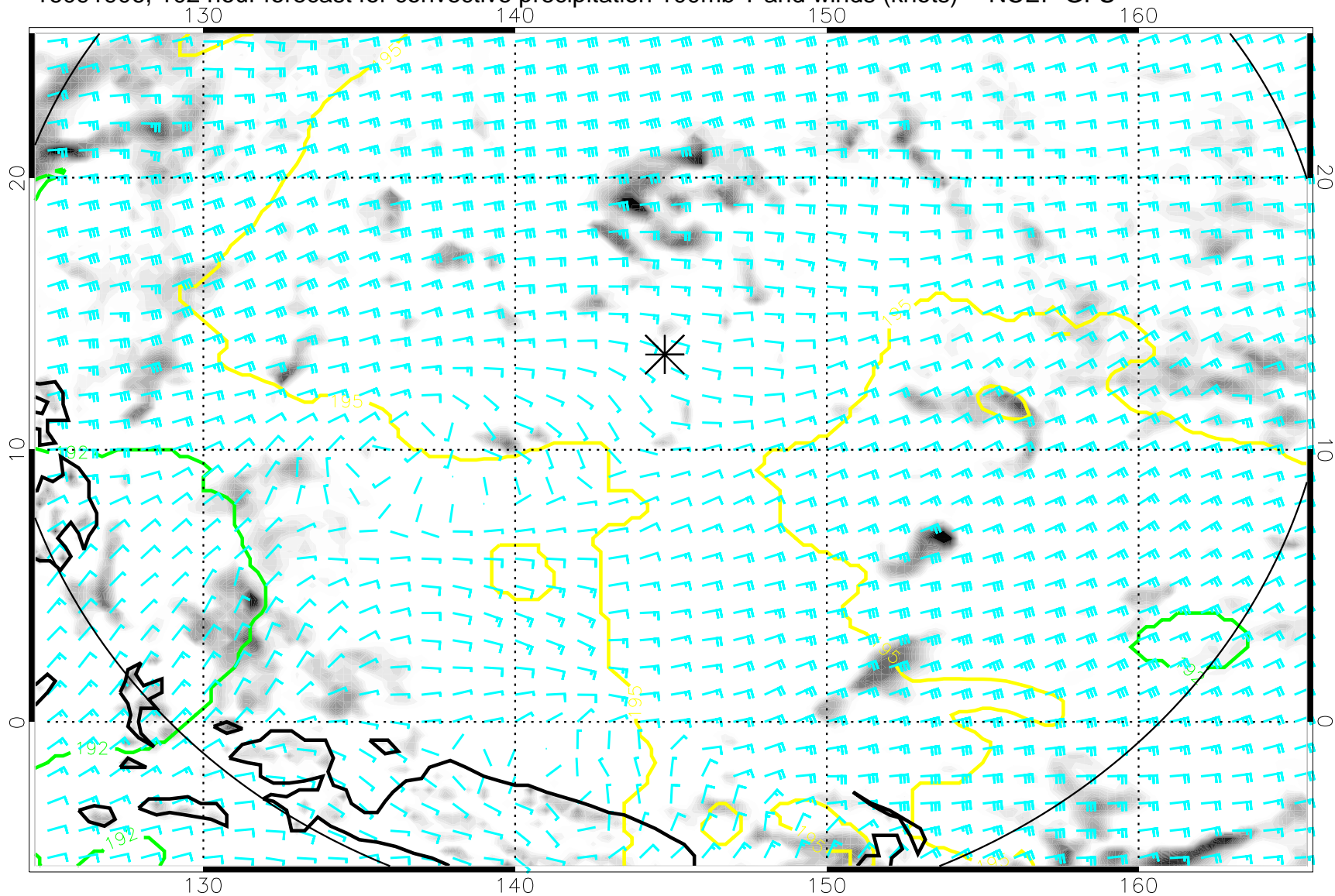
16091906, 102 hour forecast for convective precipitation 100mb T and winds (knots) -- NCEP GFS
