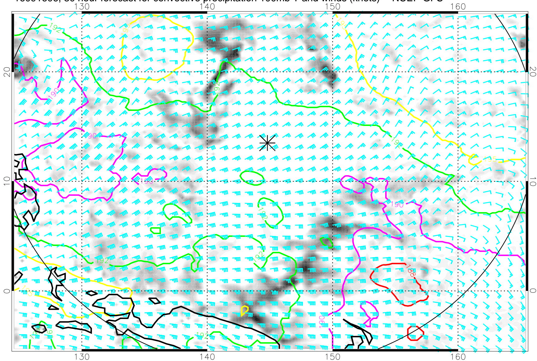
16091606, 30 hour forecast for convective precipitation 100mb T and winds (knots) -- NCEP GFS
