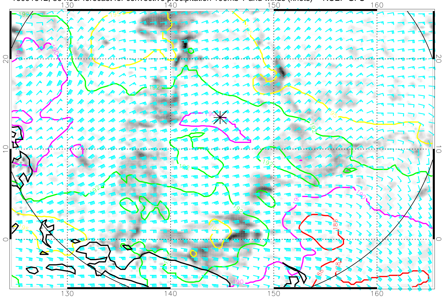
16091612, 36 hour forecast for convective precipitation 100mb T and winds (knots) -- NCEP GFS
