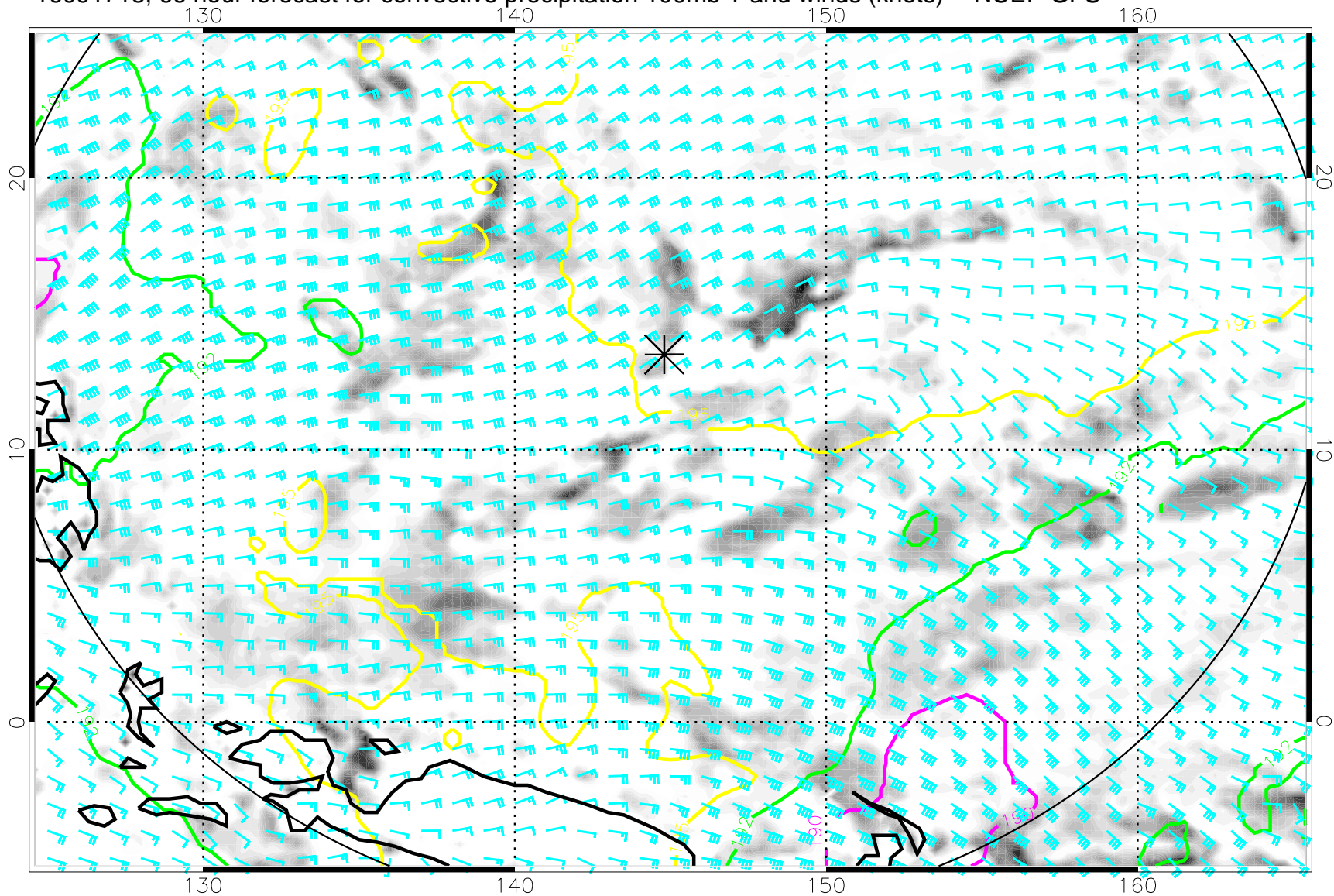
16091718, 66 hour forecast for convective precipitation 100mb T and winds (knots) -- NCEP GFS
