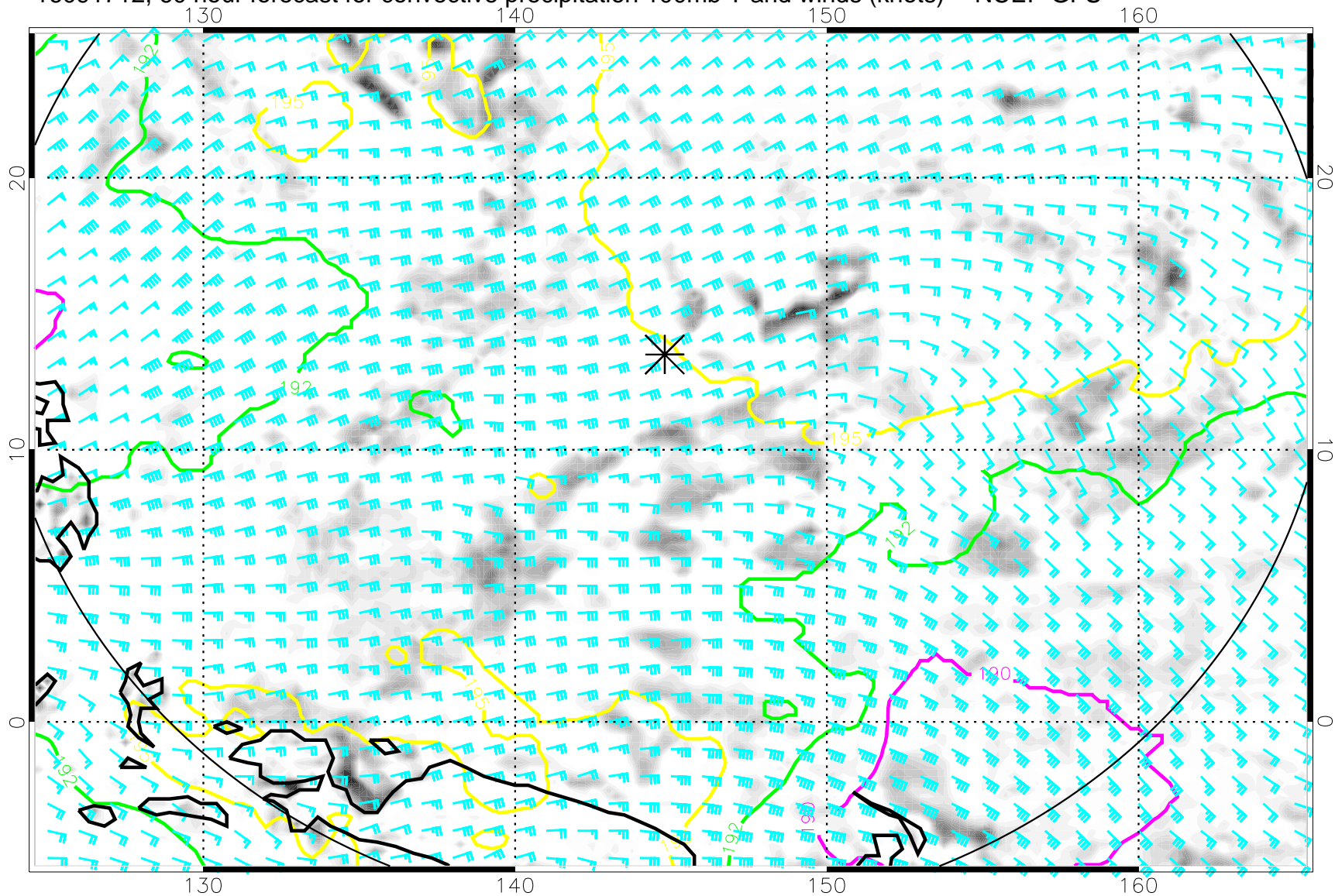
16091712, 60 hour forecast for convective precipitation 100mb T and winds (knots) -- NCEP GFS
