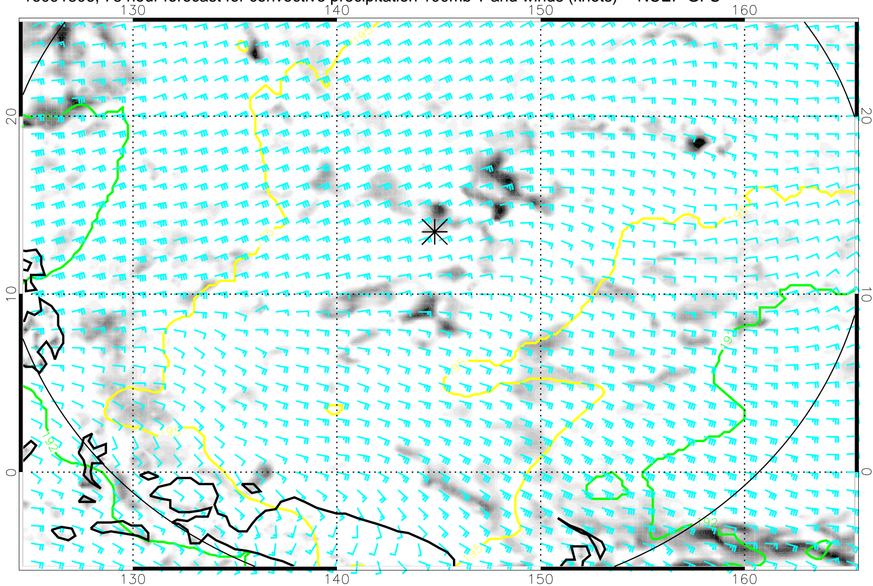
16091806, 78 hour forecast for convective precipitation 100mb T and winds (knots) -- NCEP GFS
