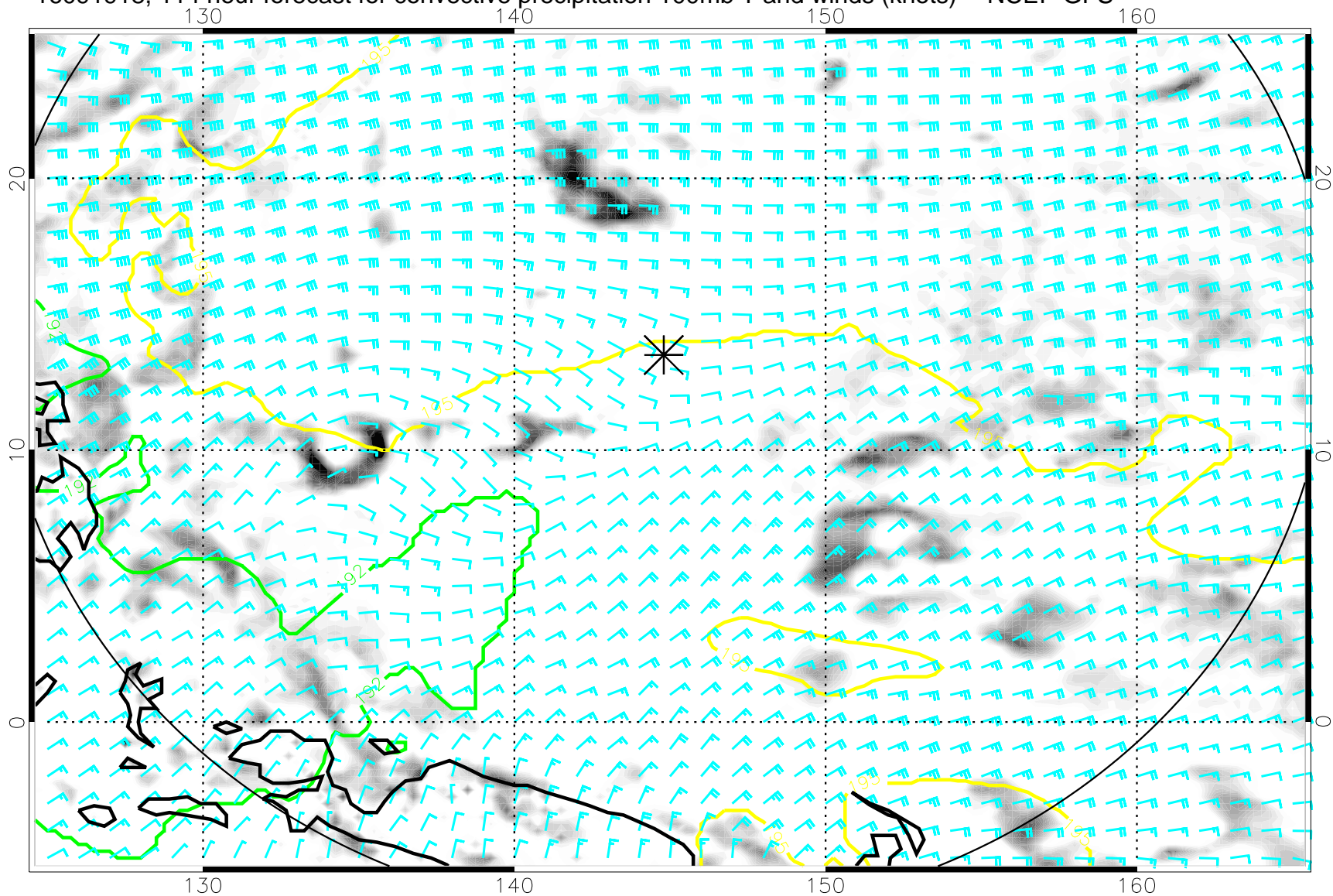
16091918, 114 hour forecast for convective precipitation 100mb T and winds (knots) -- NCEP GFS
