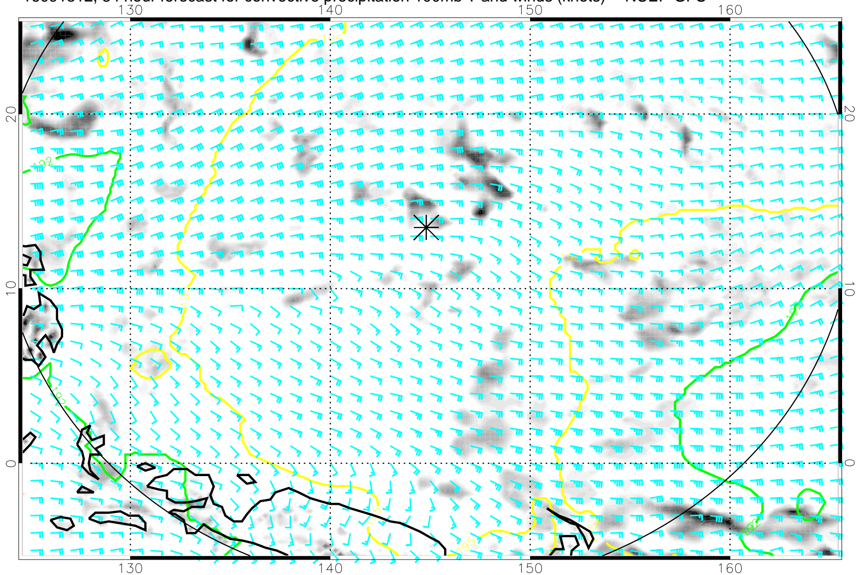
16091812, 84 hour forecast for convective precipitation 100mb T and winds (knots) -- NCEP GFS
