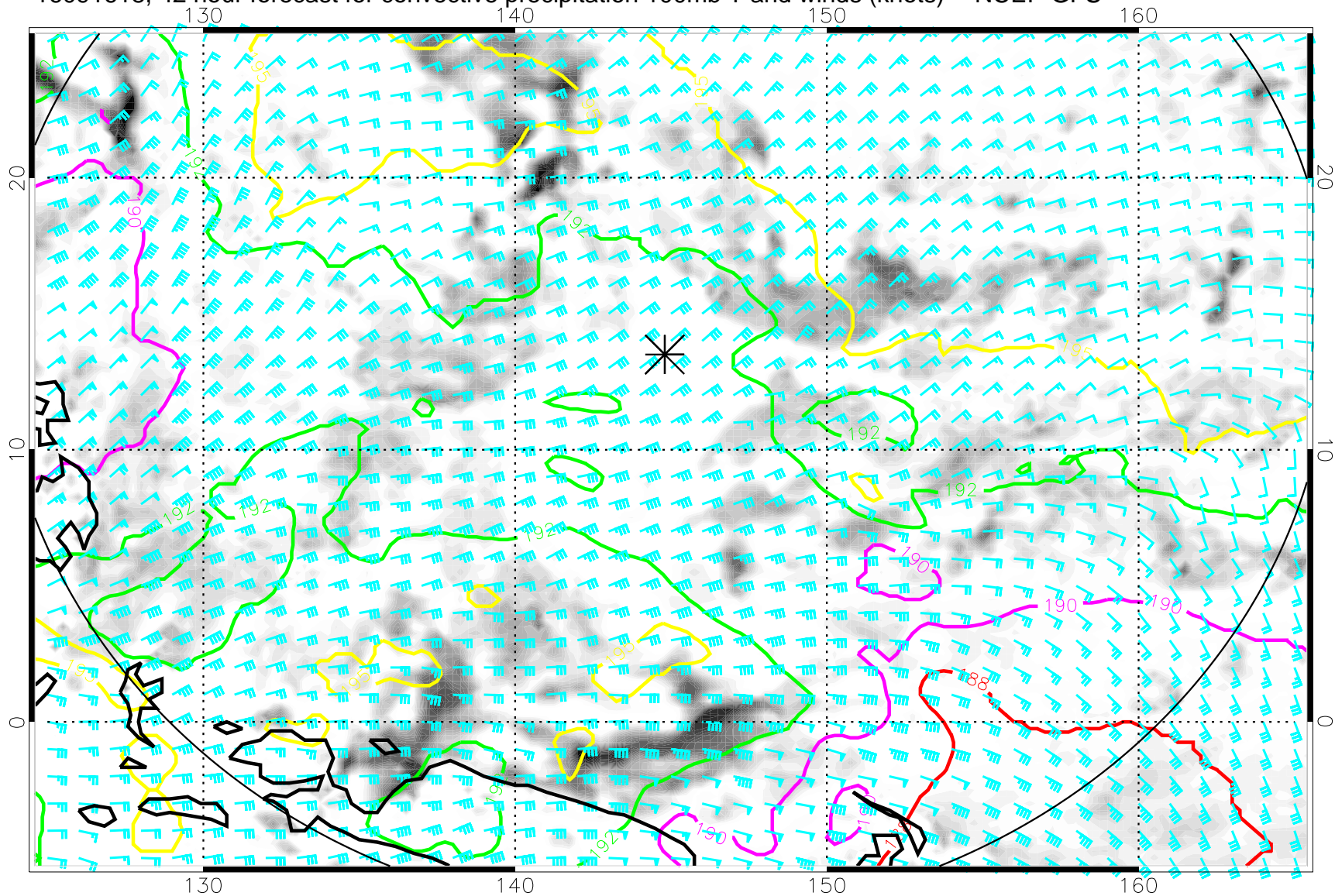
16091618, 42 hour forecast for convective precipitation 100mb T and winds (knots) -- NCEP GFS
