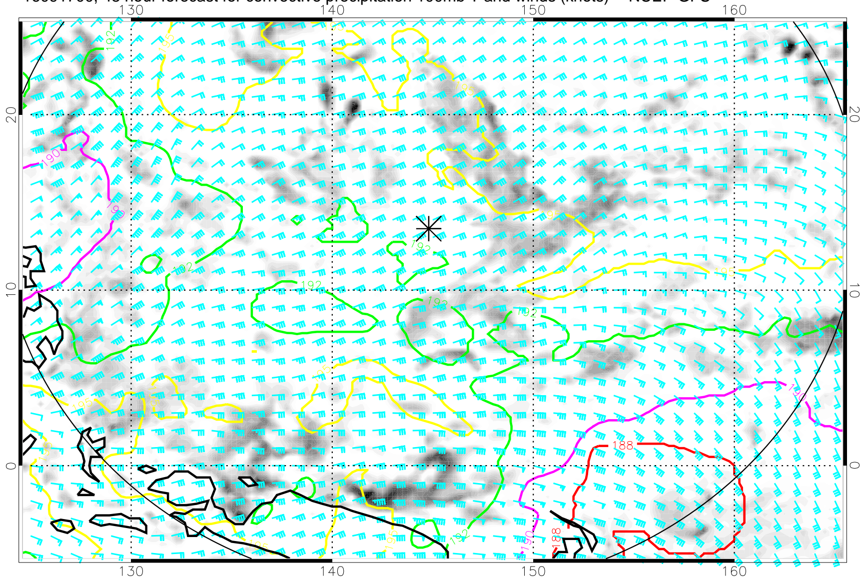
16091700, 48 hour forecast for convective precipitation 100mb T and winds (knots) -- NCEP GFS
