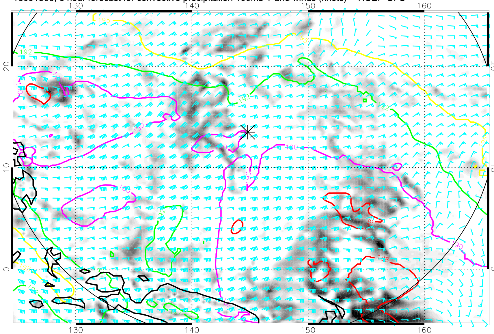
16091506, 6 hour forecast for convective precipitation 100mb T and winds (knots) -- NCEP GFS
