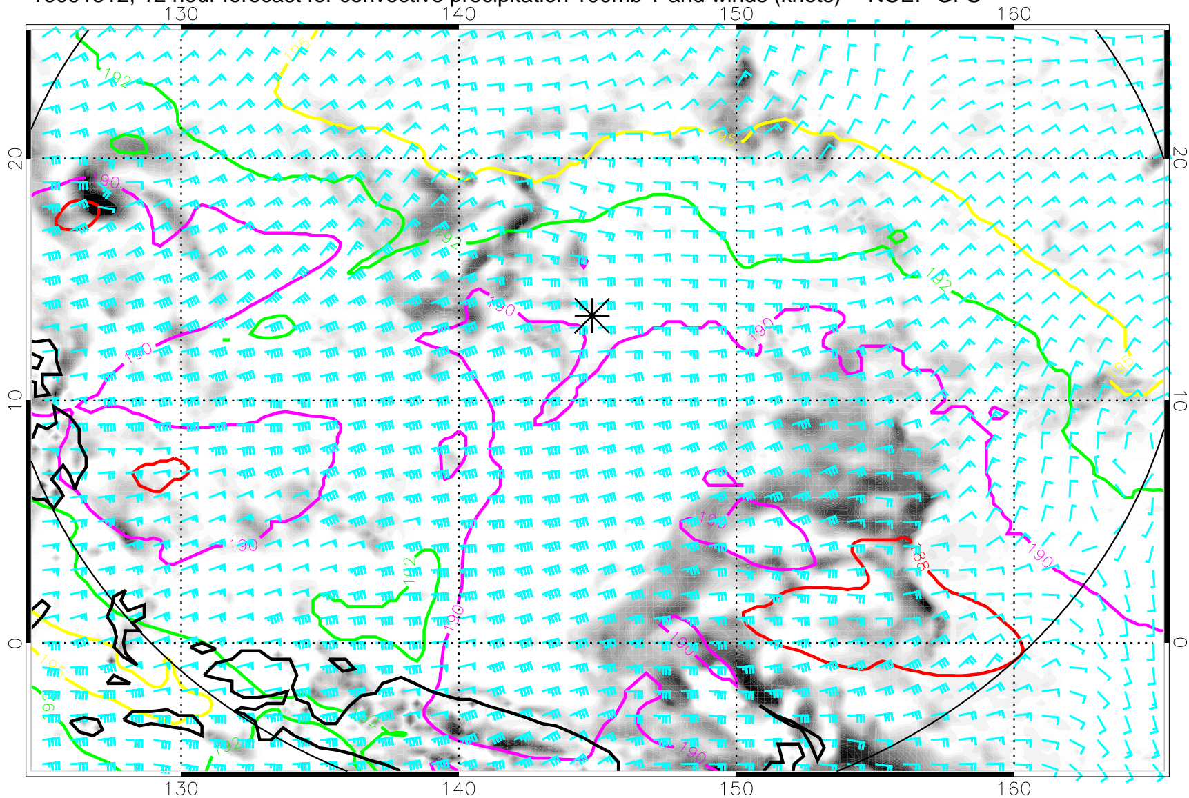
16091512, 12 hour forecast for convective precipitation 100mb T and winds (knots) -- NCEP GFS
