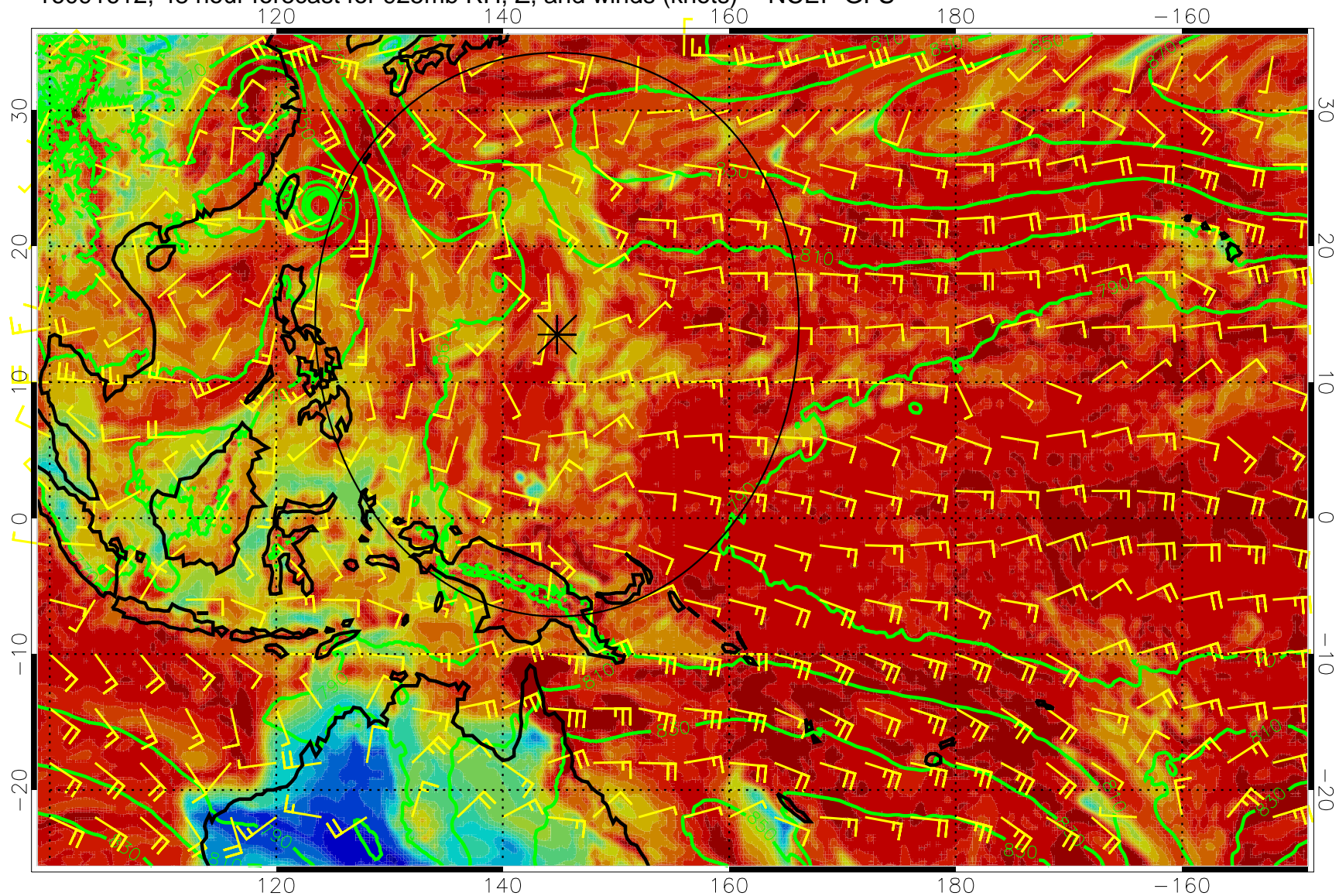
16091612, 48 hour forecast for 925mb RH, Z, and winds (knots) -- NCEP GFS
