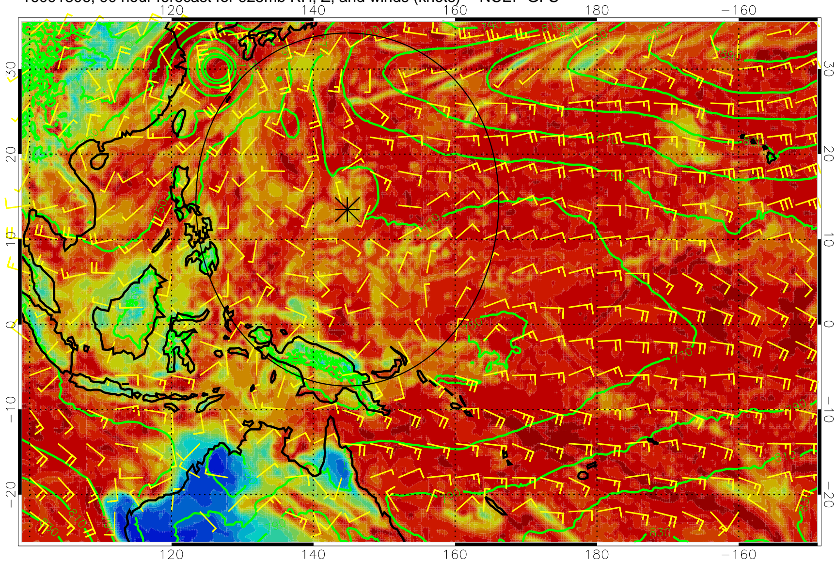
16091806, 90 hour forecast for 925mb RH, Z, and winds (knots) -- NCEP GFS
