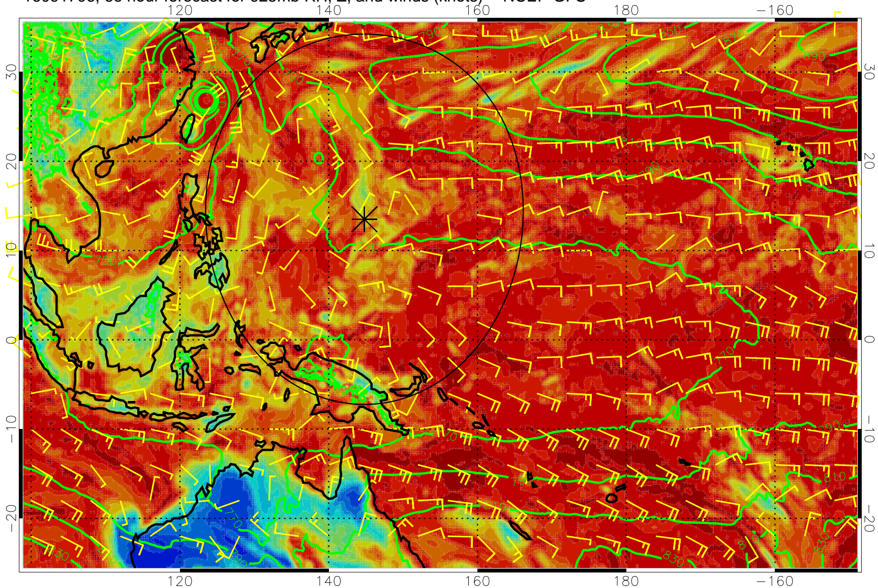
16091706, 66 hour forecast for 925mb RH, Z, and winds (knots) -- NCEP GFS
