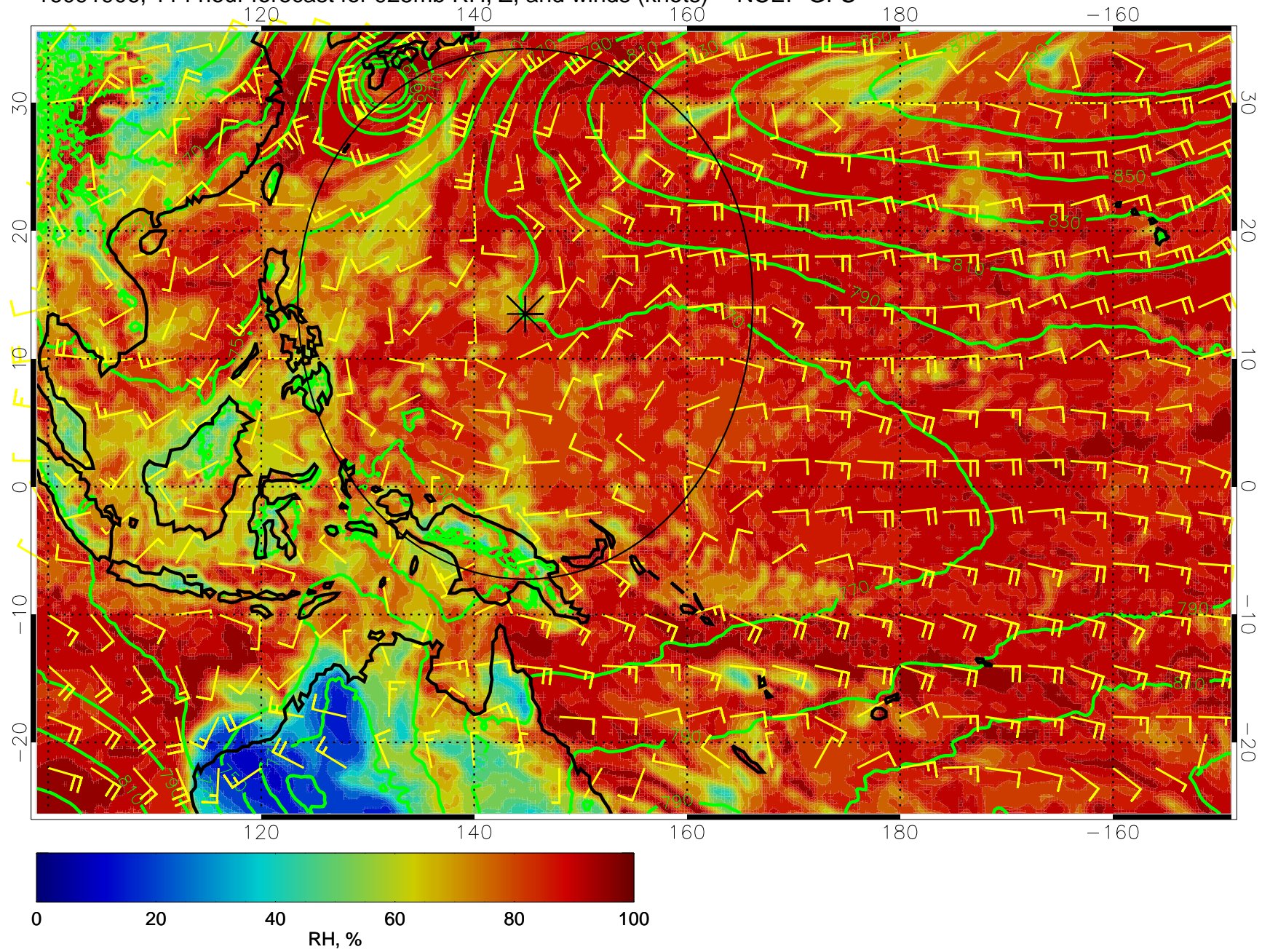
16091906, 114 hour forecast for 925mb RH, Z, and winds (knots) -- NCEP GFS
