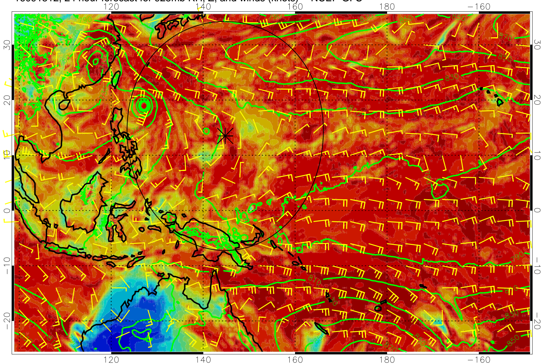
16091512, 24 hour forecast for 925mb RH, Z, and winds (knots) -- NCEP GFS
