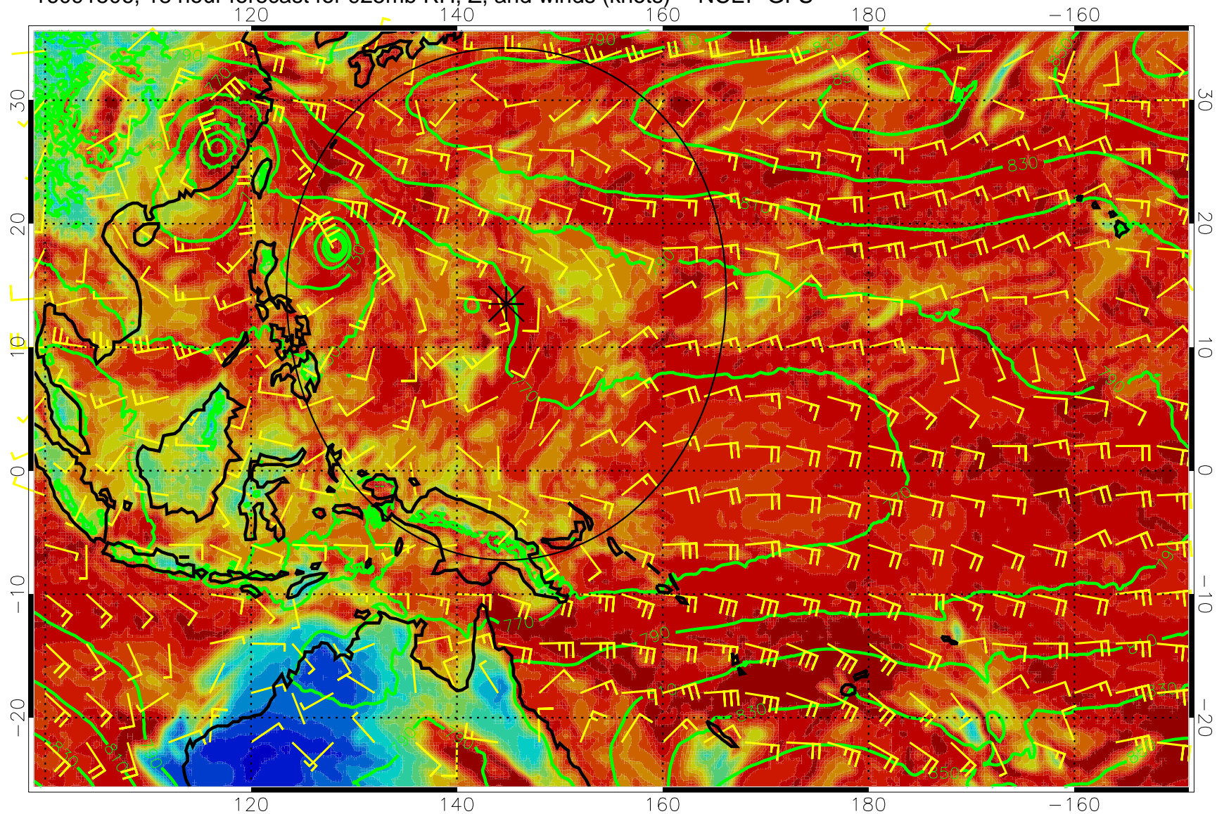
16091506, 18 hour forecast for 925mb RH, Z, and winds (knots) -- NCEP GFS
