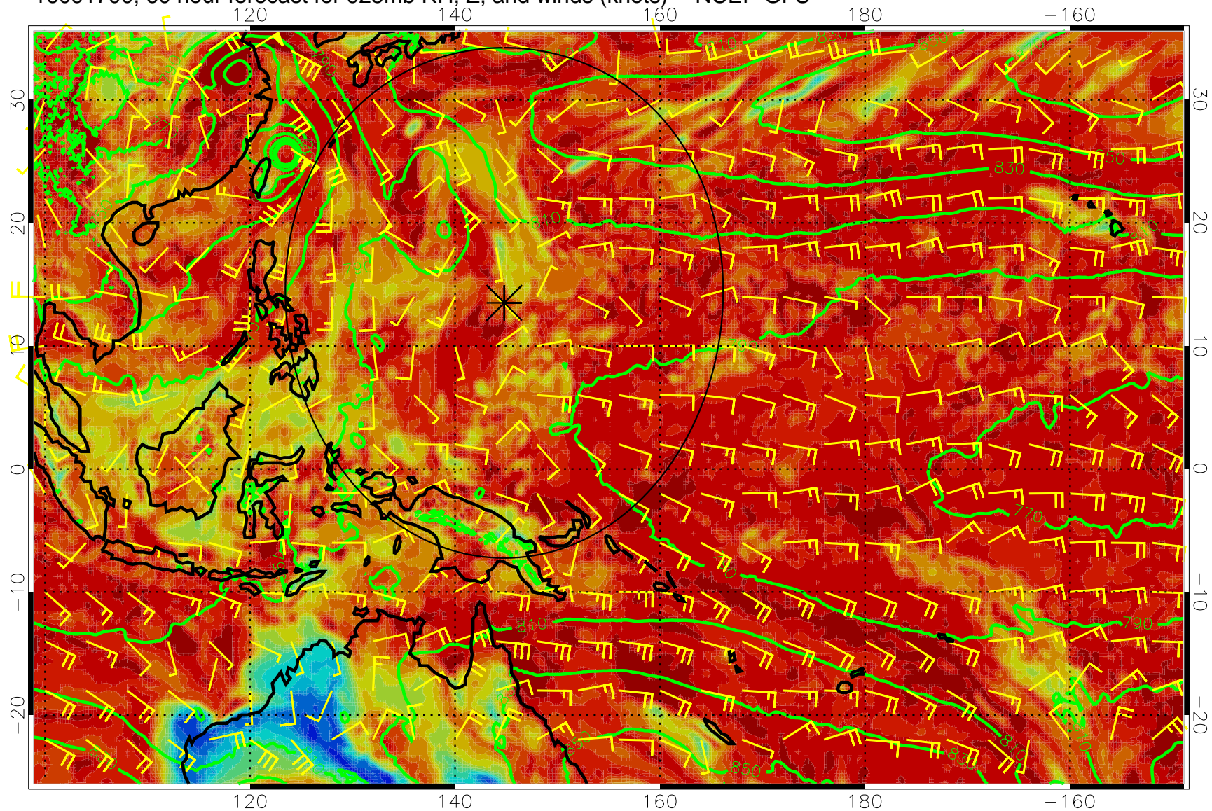
16091700, 60 hour forecast for 925mb RH, Z, and winds (knots) -- NCEP GFS
