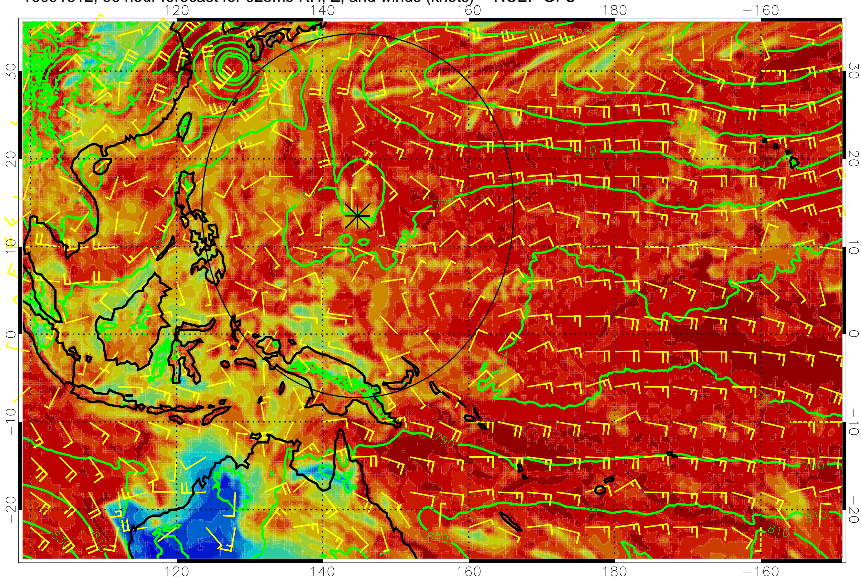
16091812, 96 hour forecast for 925mb RH, Z, and winds (knots) -- NCEP GFS
