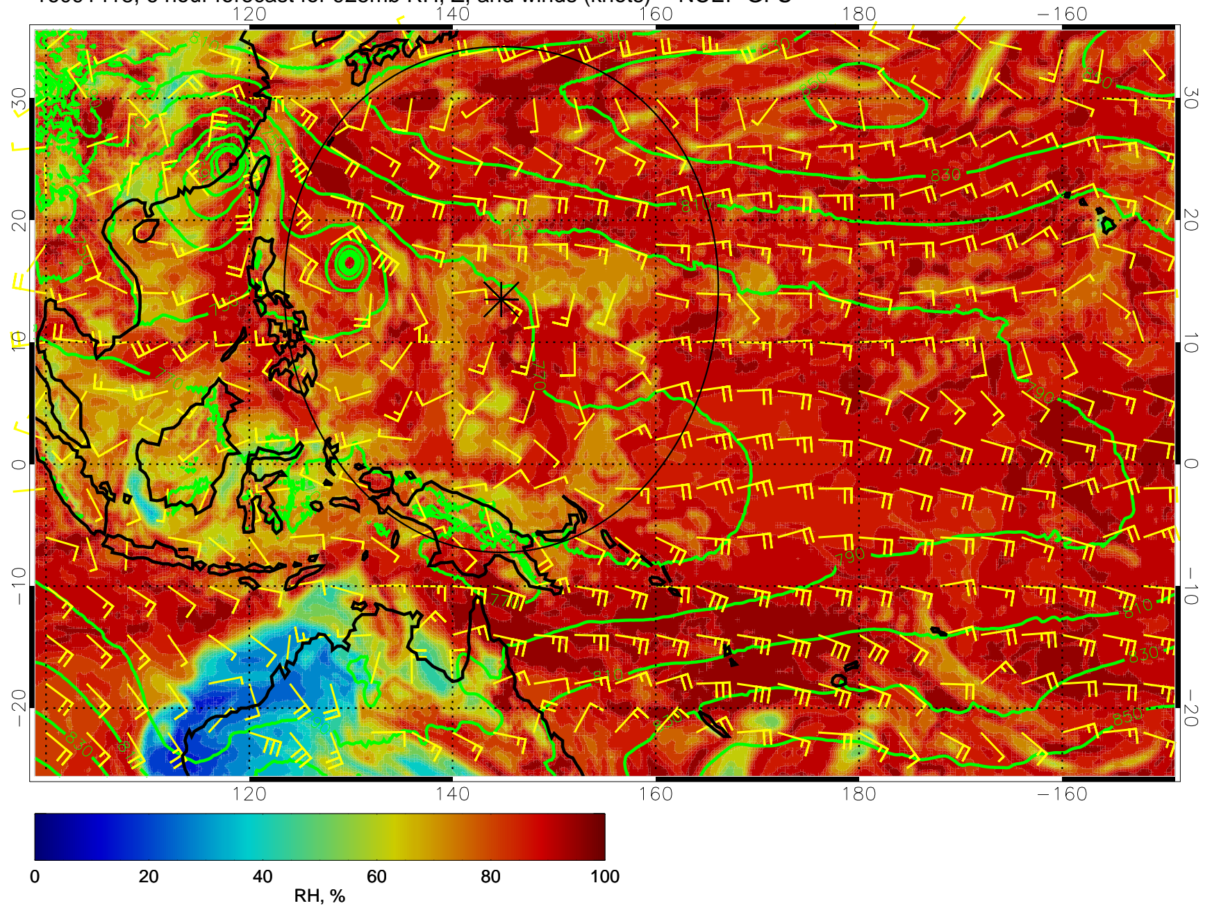
16091418, 6 hour forecast for 925mb RH, Z, and winds (knots) -- NCEP GFS
