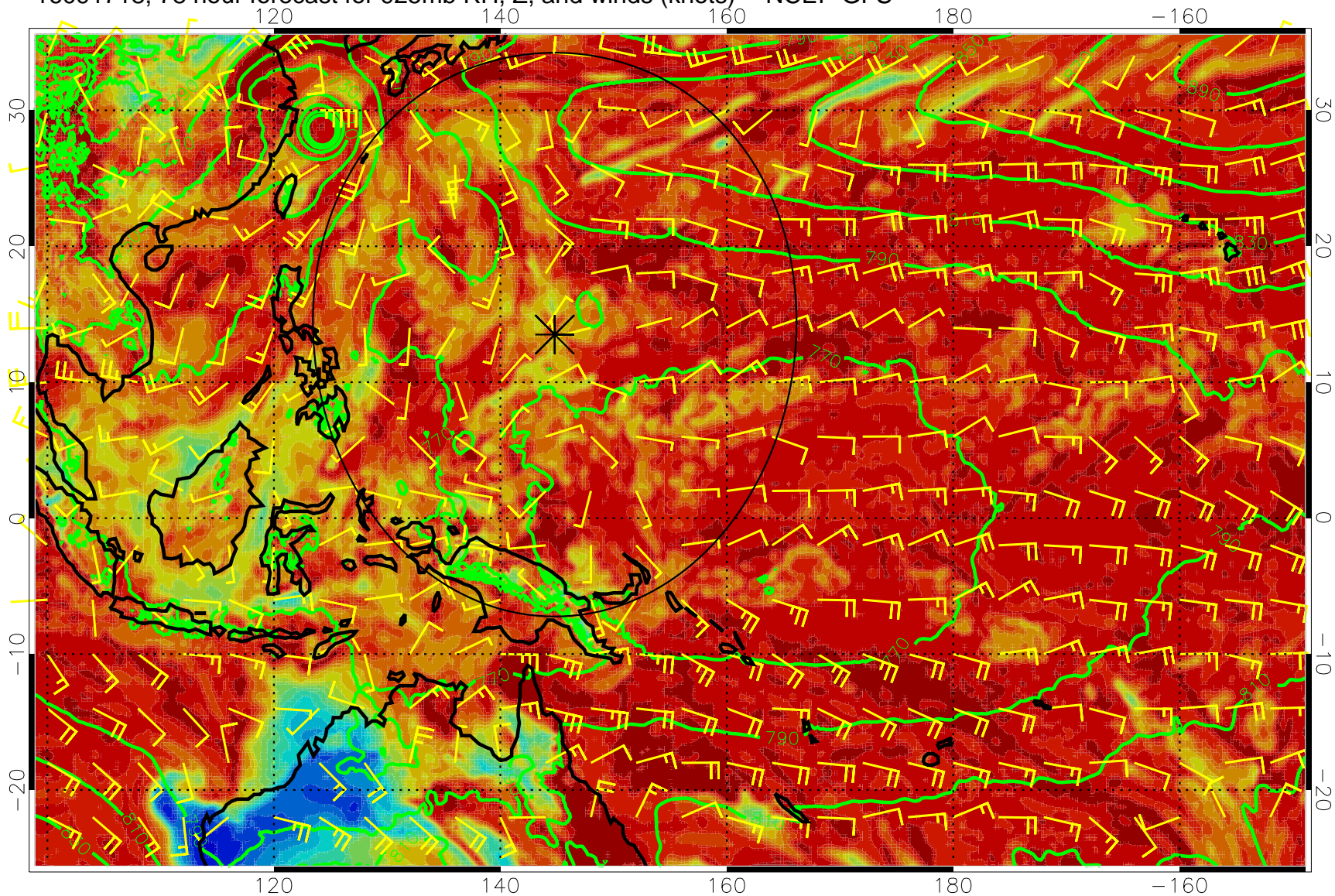
16091718, 78 hour forecast for 925mb RH, Z, and winds (knots) -- NCEP GFS
