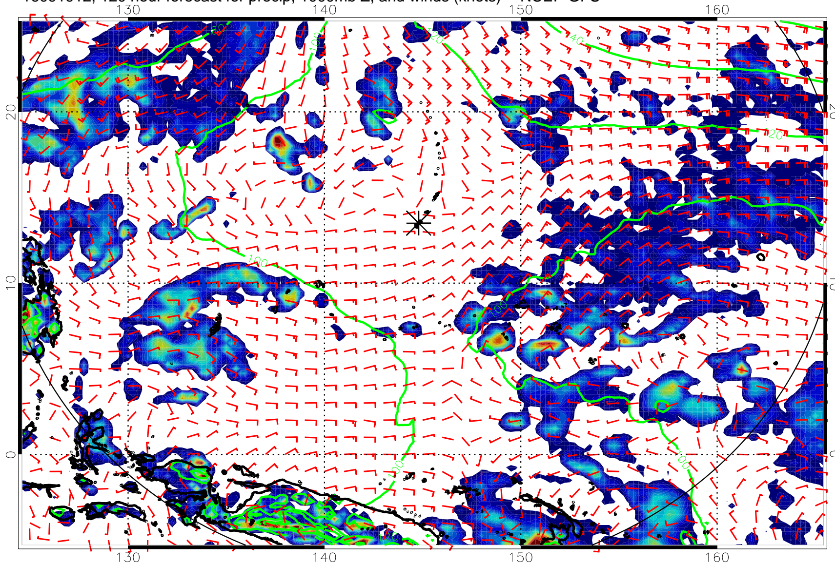
16091912, 120 hour forecast for precip, 1000mb Z, and winds (knots) -- NCEP GFS
