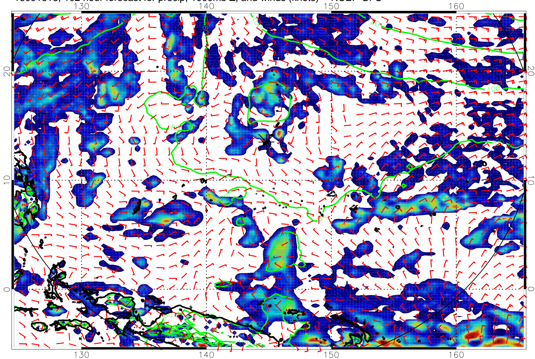
16091818, 102 hour forecast for precip, 1000mb Z, and winds (knots) -- NCEP GFS
