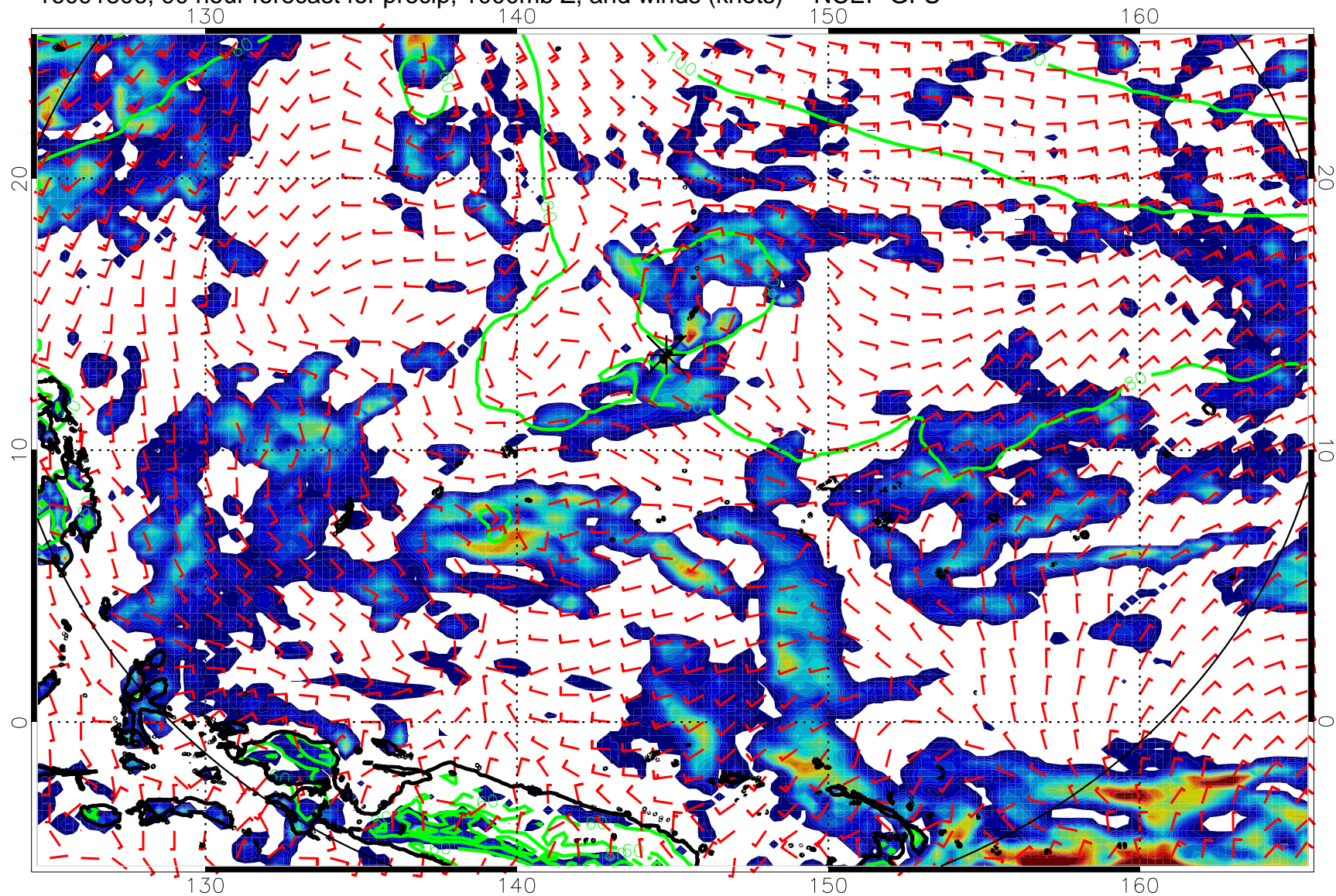
16091806, 90 hour forecast for precip, 1000mb Z, and winds (knots) -- NCEP GFS
