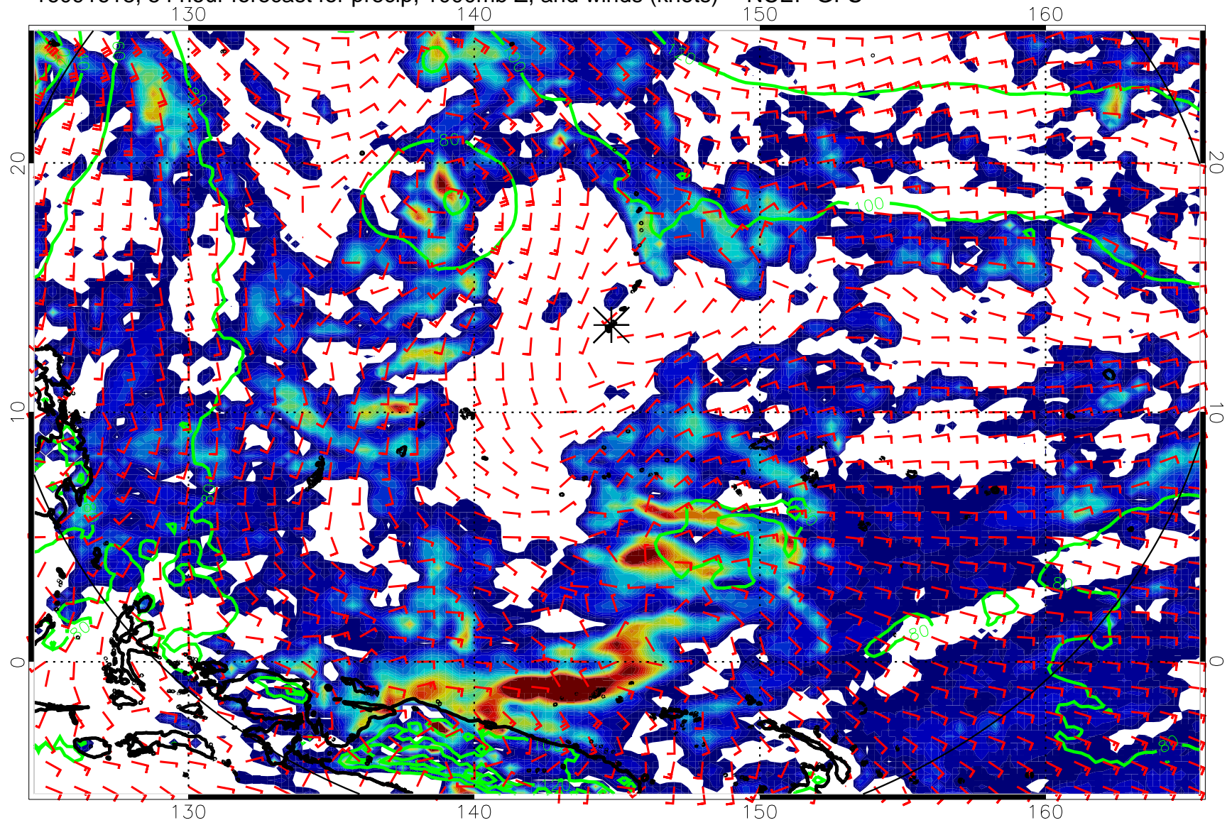
16091618, 54 hour forecast for precip, 1000mb Z, and winds (knots) -- NCEP GFS
