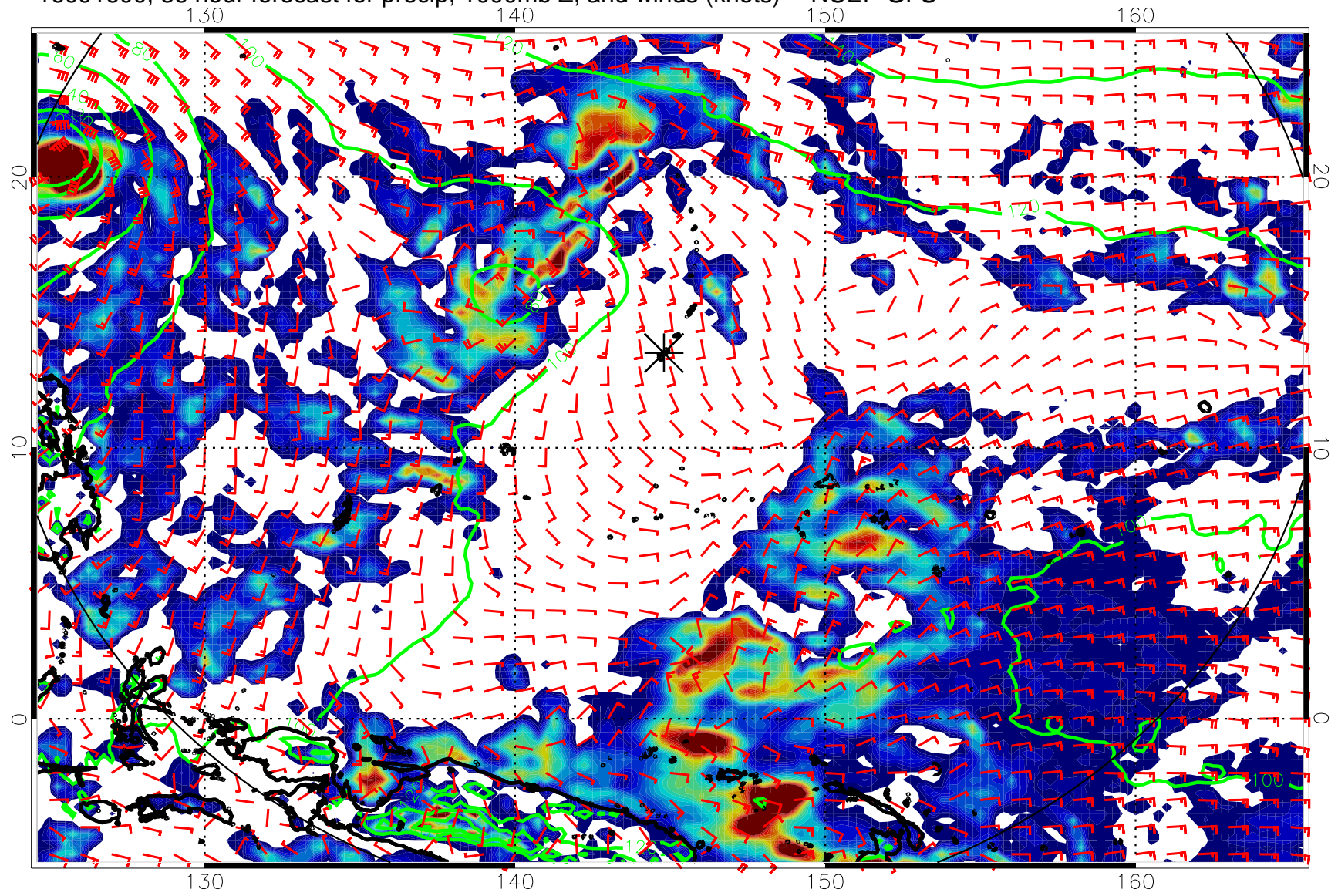
16091600, 36 hour forecast for precip, 1000mb Z, and winds (knots) -- NCEP GFS
