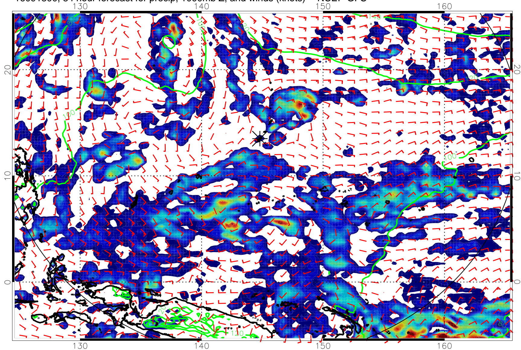
16091800, 84 hour forecast for precip, 1000mb Z, and winds (knots) -- NCEP GFS
