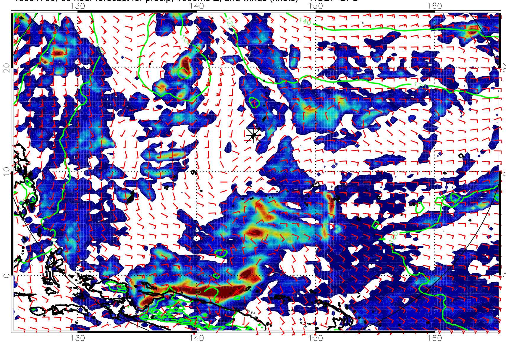
16091700, 60 hour forecast for precip, 1000mb Z, and winds (knots) -- NCEP GFS
