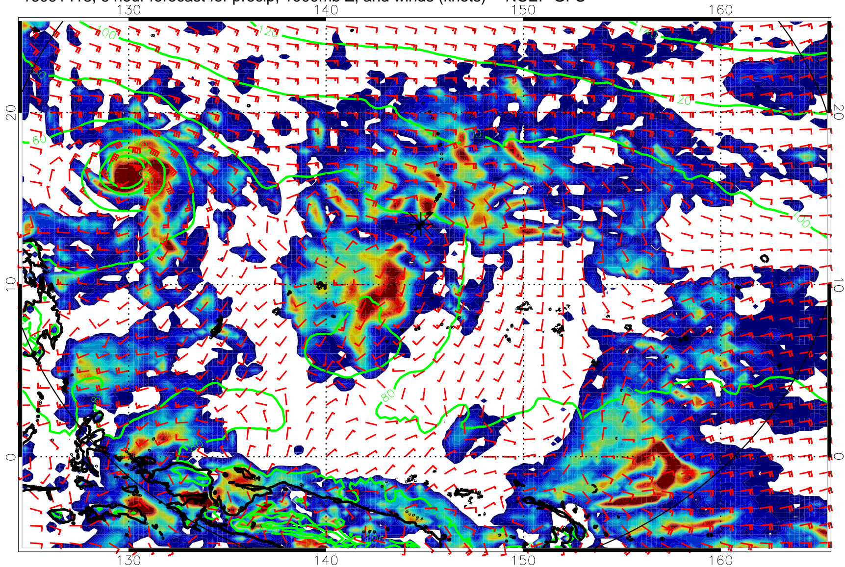
16091418, 6 hour forecast for precip, 1000mb Z, and winds (knots) -- NCEP GFS
