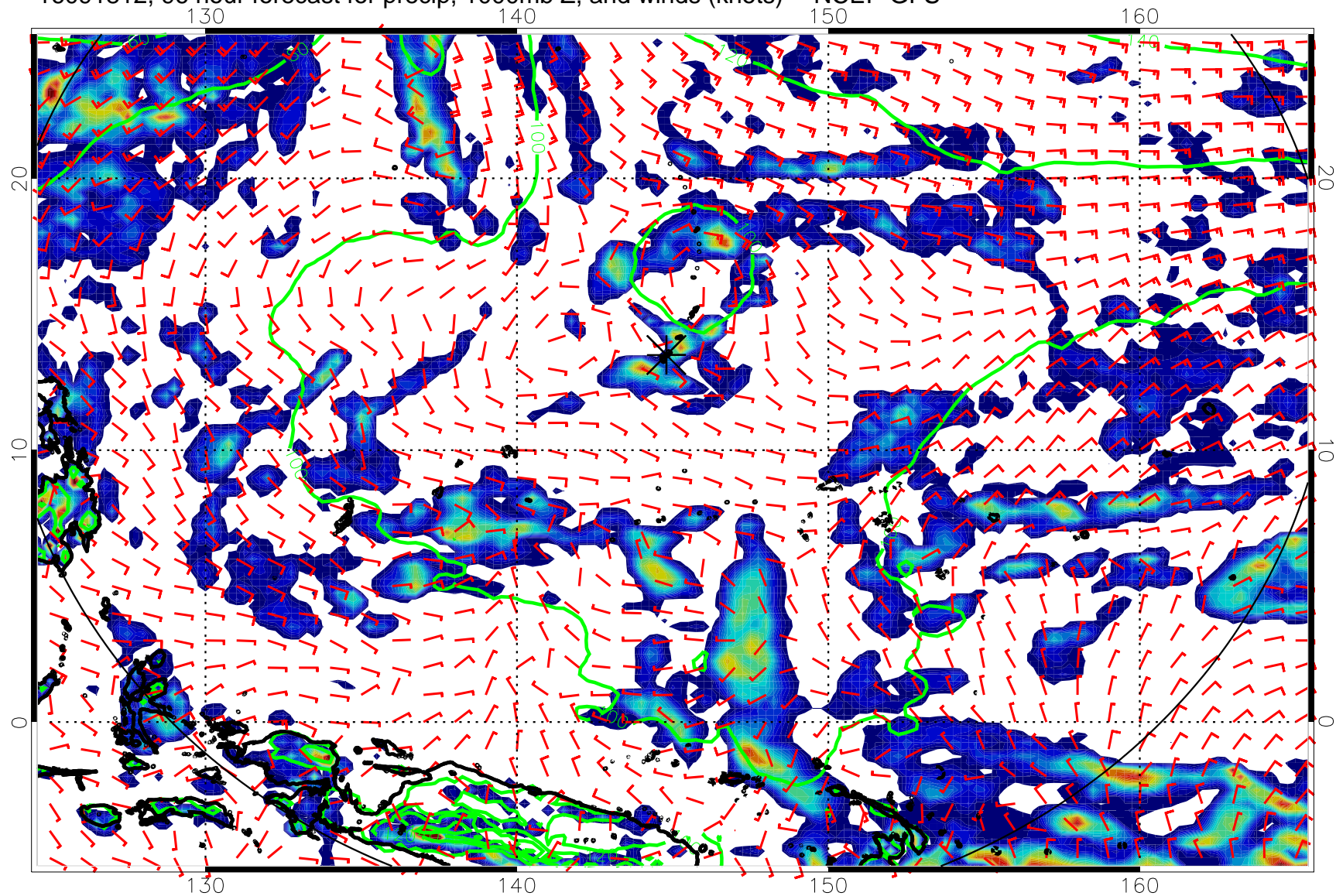
16091812, 96 hour forecast for precip, 1000mb Z, and winds (knots) -- NCEP GFS
