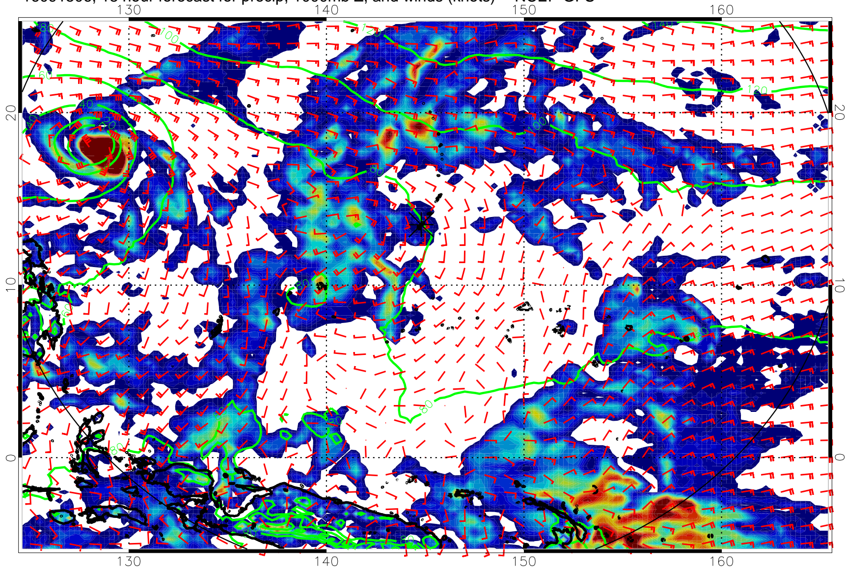
16091506, 18 hour forecast for precip, 1000mb Z, and winds (knots) -- NCEP GFS
