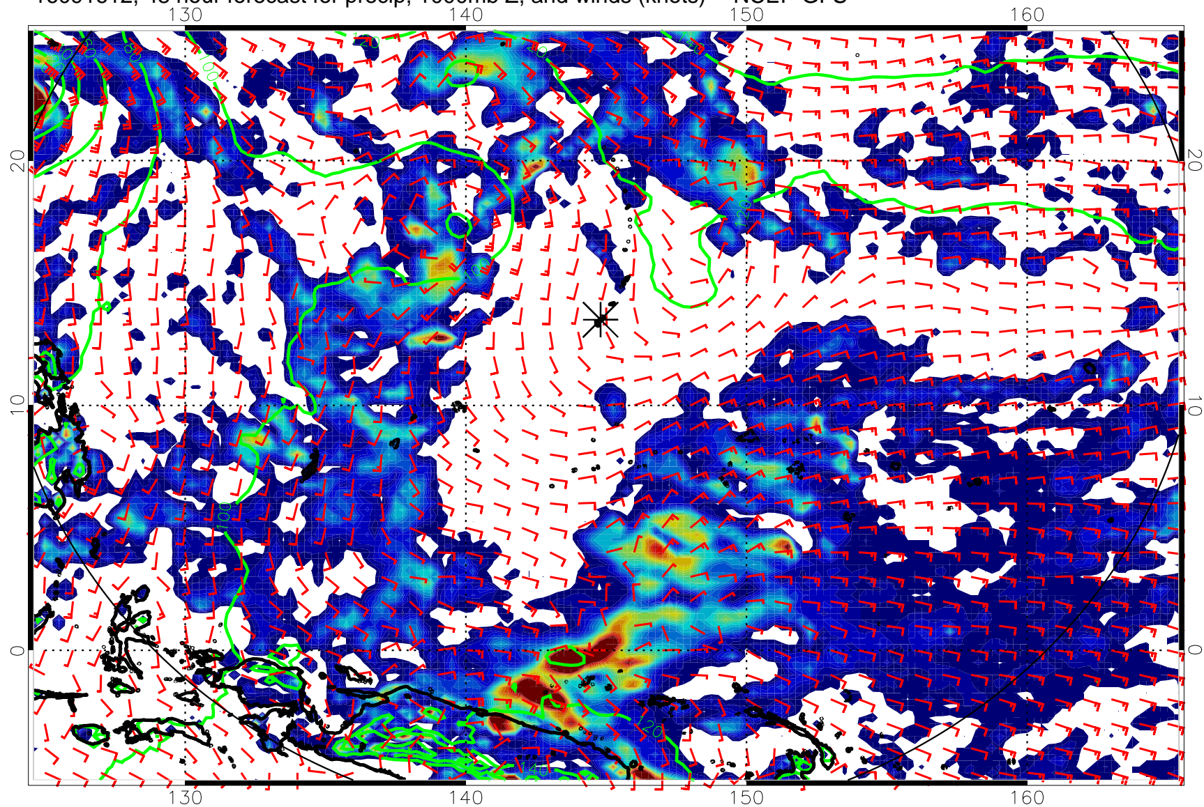
16091612, 48 hour forecast for precip, 1000mb Z, and winds (knots) -- NCEP GFS
