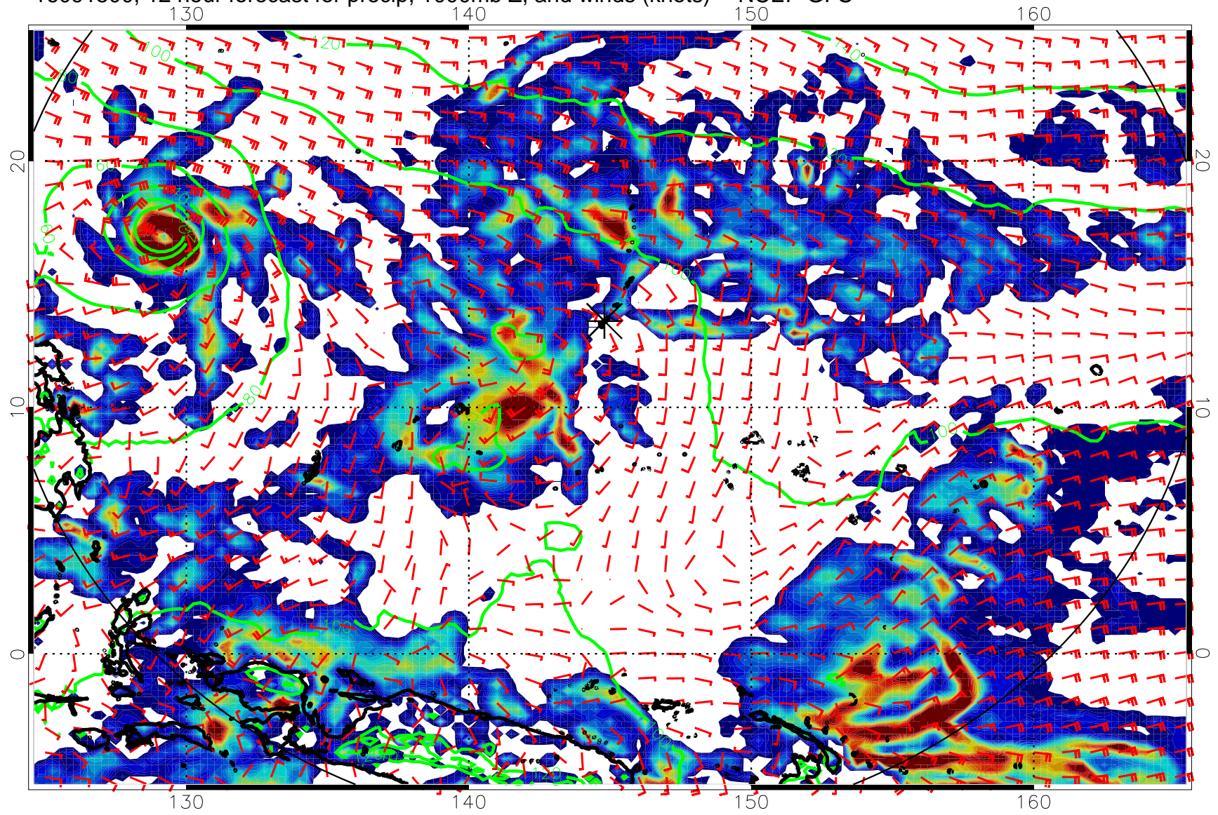
16091500, 12 hour forecast for precip, 1000mb Z, and winds (knots) -- NCEP GFS
