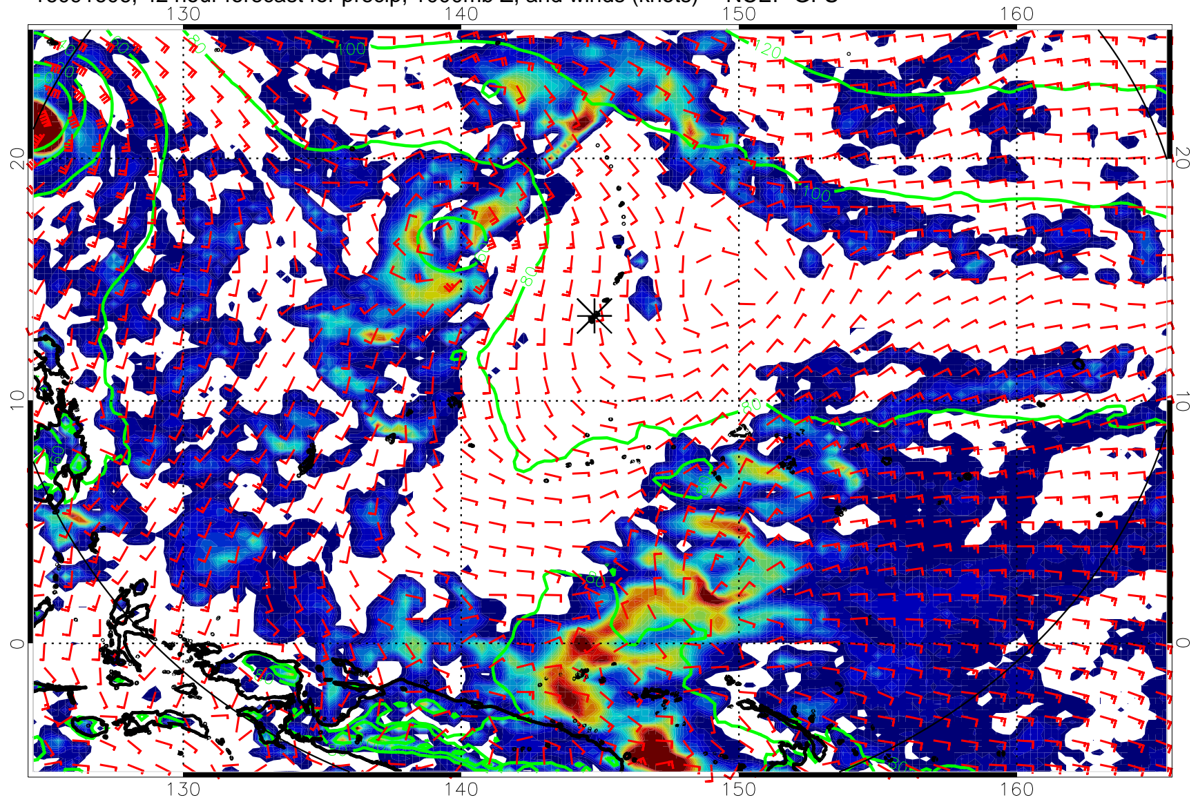
16091606, 42 hour forecast for precip, 1000mb Z, and winds (knots) -- NCEP GFS
