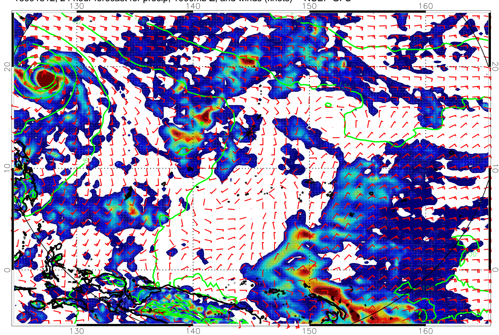
16091512, 24 hour forecast for precip, 1000mb Z, and winds (knots) -- NCEP GFS
