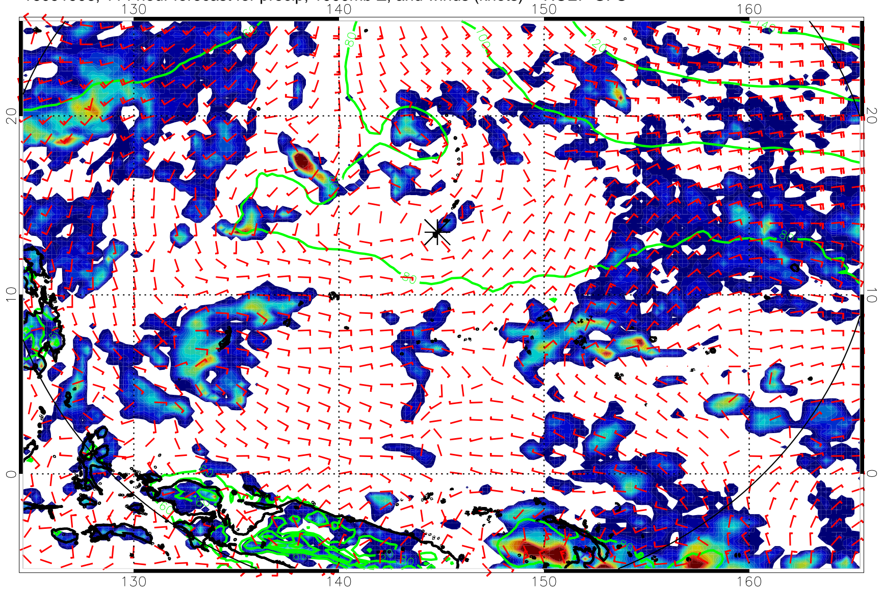
16091906, 114 hour forecast for precip, 1000mb Z, and winds (knots) -- NCEP GFS
