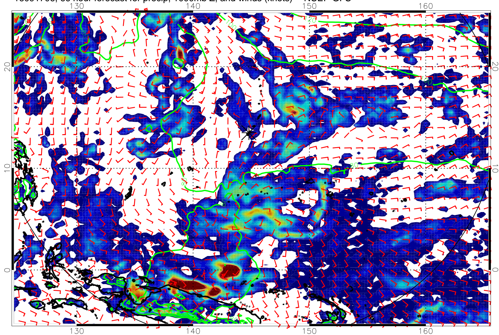
16091706, 66 hour forecast for precip, 1000mb Z, and winds (knots) -- NCEP GFS
