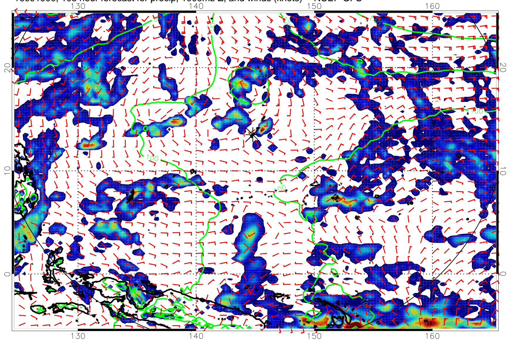
16091900, 108 hour forecast for precip, 1000mb Z, and winds (knots) -- NCEP GFS
