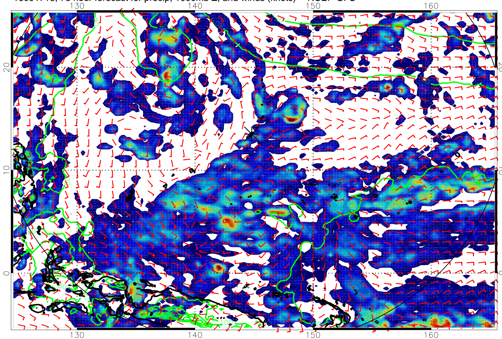
16091718, 78 hour forecast for precip, 1000mb Z, and winds (knots) -- NCEP GFS
