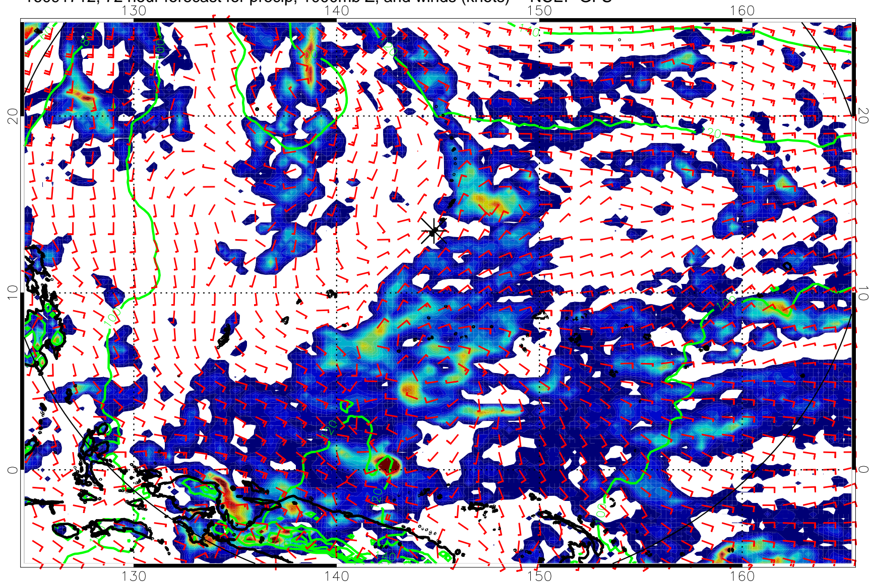
16091712, 72 hour forecast for precip, 1000mb Z, and winds (knots) -- NCEP GFS
