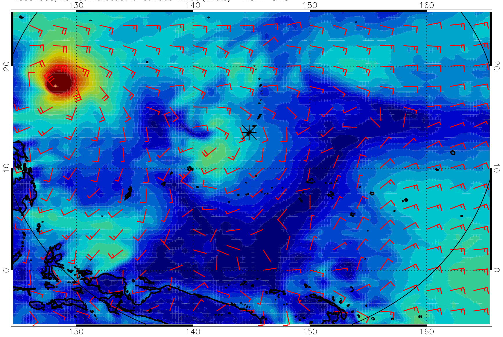
16091506, 18 hour forecast for surface winds (knots) -- NCEP GFS
