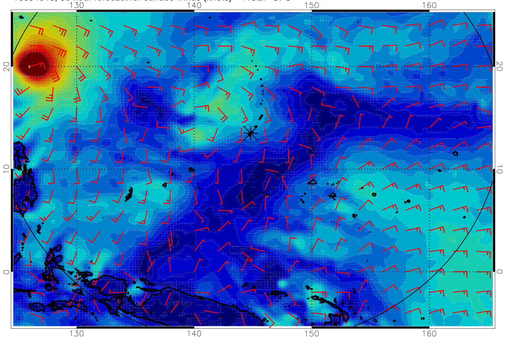
16091518, 30 hour forecast for surface winds (knots) -- NCEP GFS
