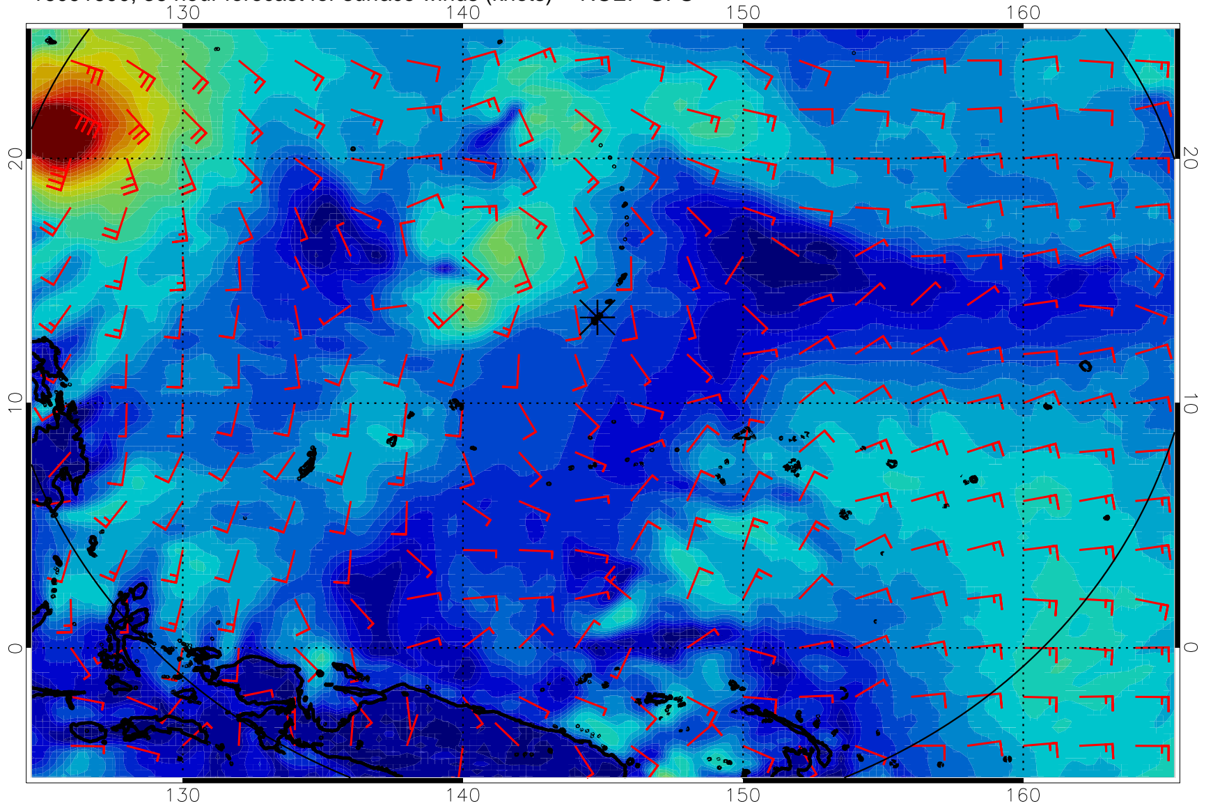
16091600, 36 hour forecast for surface winds (knots) -- NCEP GFS
