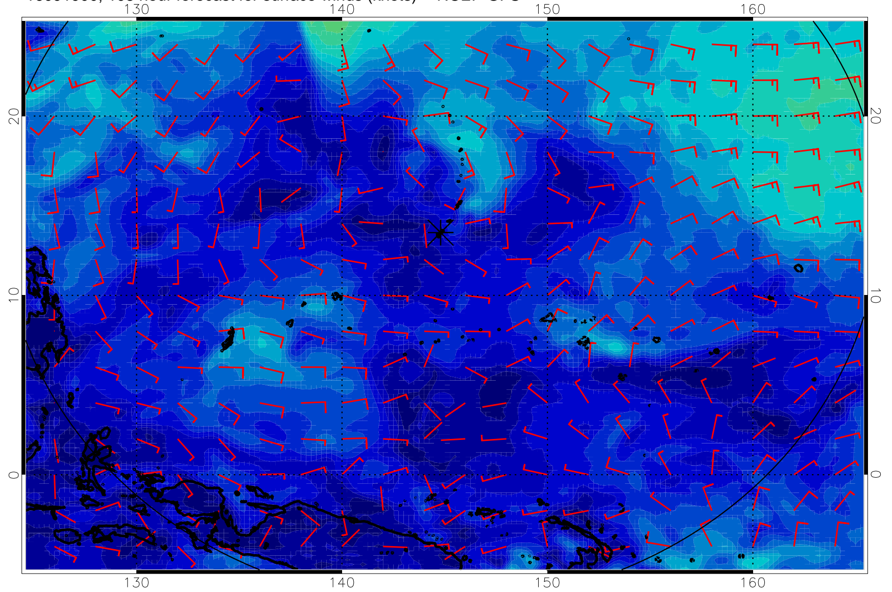
16091900, 108 hour forecast for surface winds (knots) -- NCEP GFS
