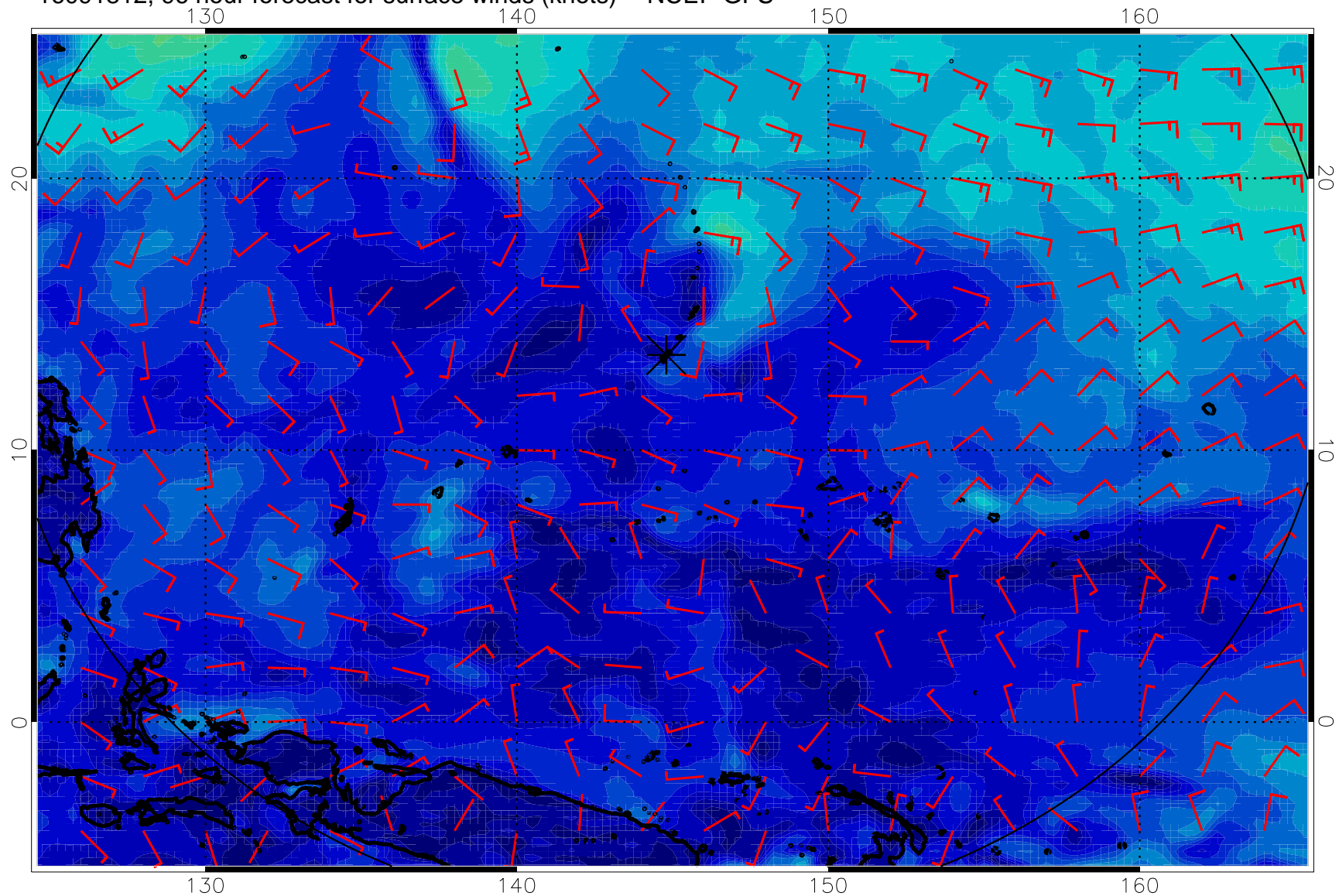
16091812, 96 hour forecast for surface winds (knots) -- NCEP GFS
