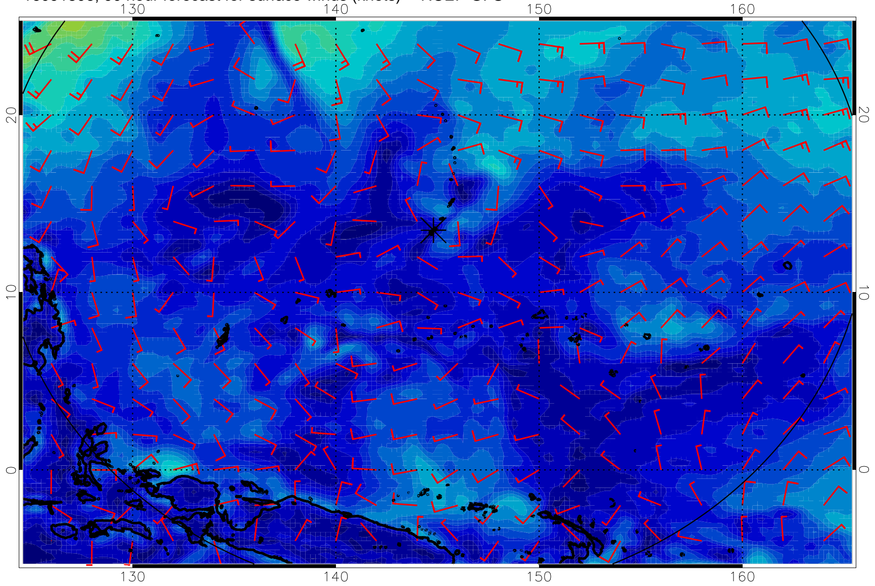
16091806, 90 hour forecast for surface winds (knots) -- NCEP GFS
