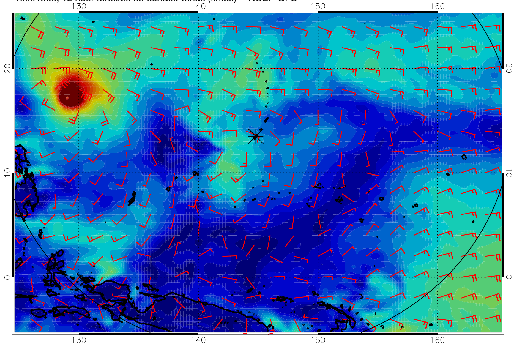
16091500, 12 hour forecast for surface winds (knots) -- NCEP GFS
