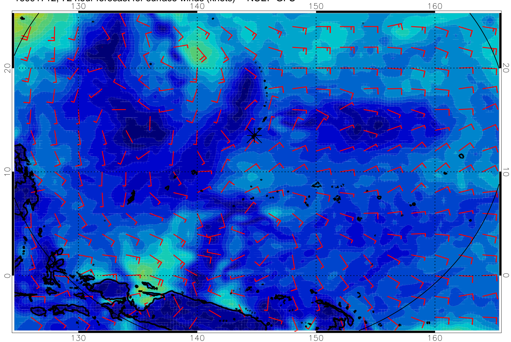
16091712, 72 hour forecast for surface winds (knots) -- NCEP GFS
