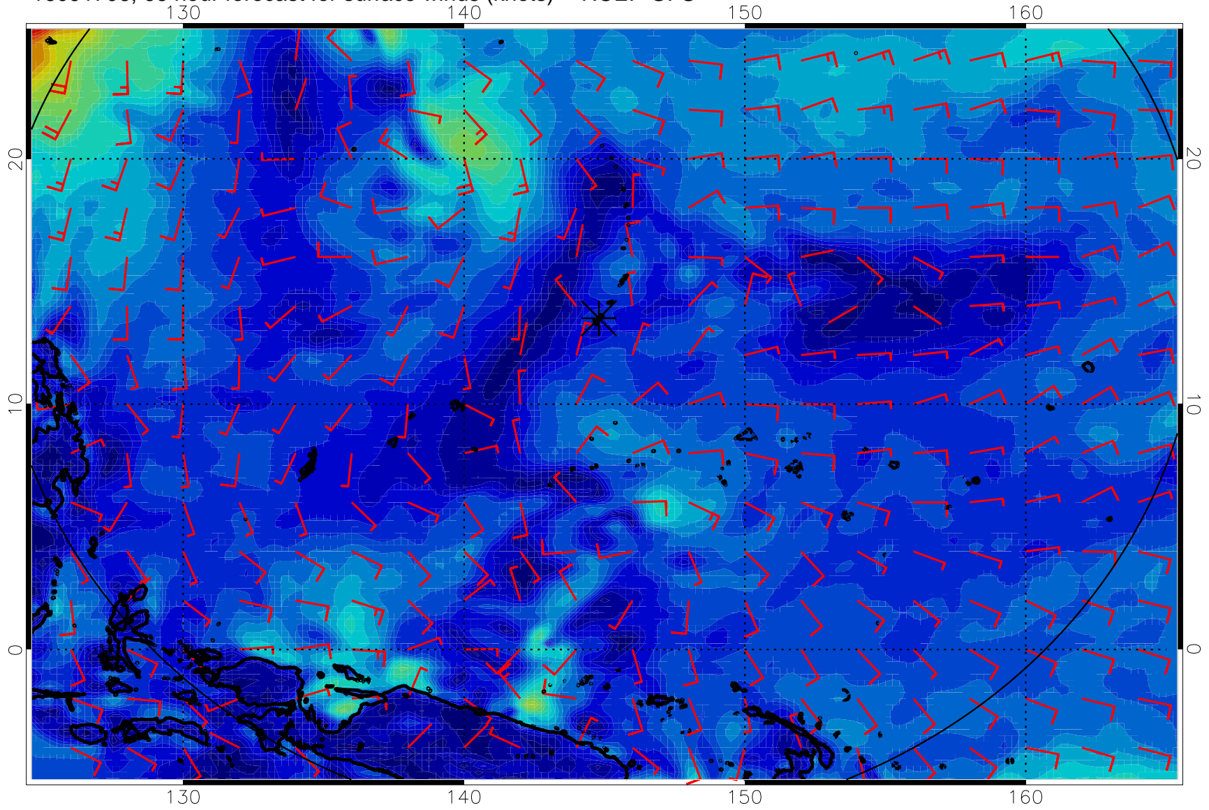
16091706, 66 hour forecast for surface winds (knots) -- NCEP GFS
