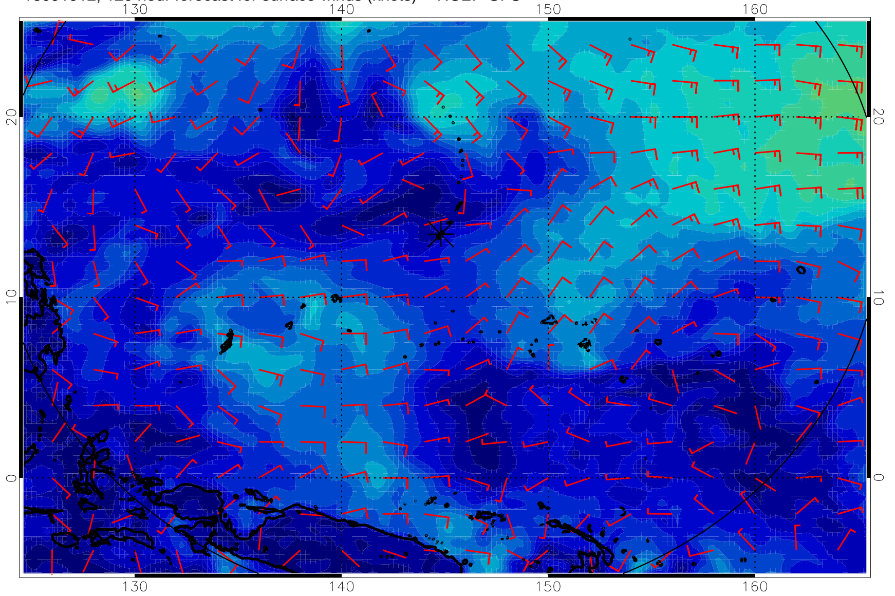
16091912, 120 hour forecast for surface winds (knots) -- NCEP GFS
