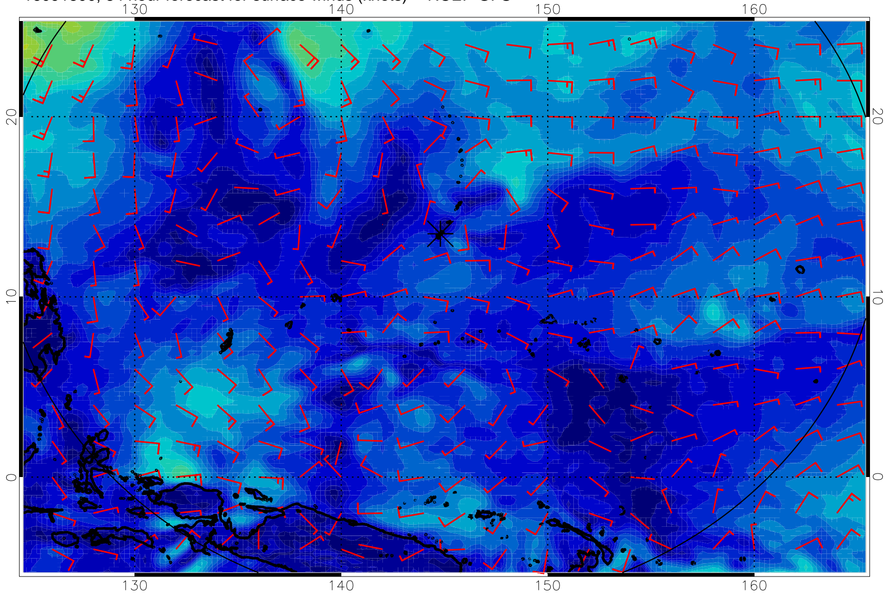
16091800, 84 hour forecast for surface winds (knots) -- NCEP GFS
