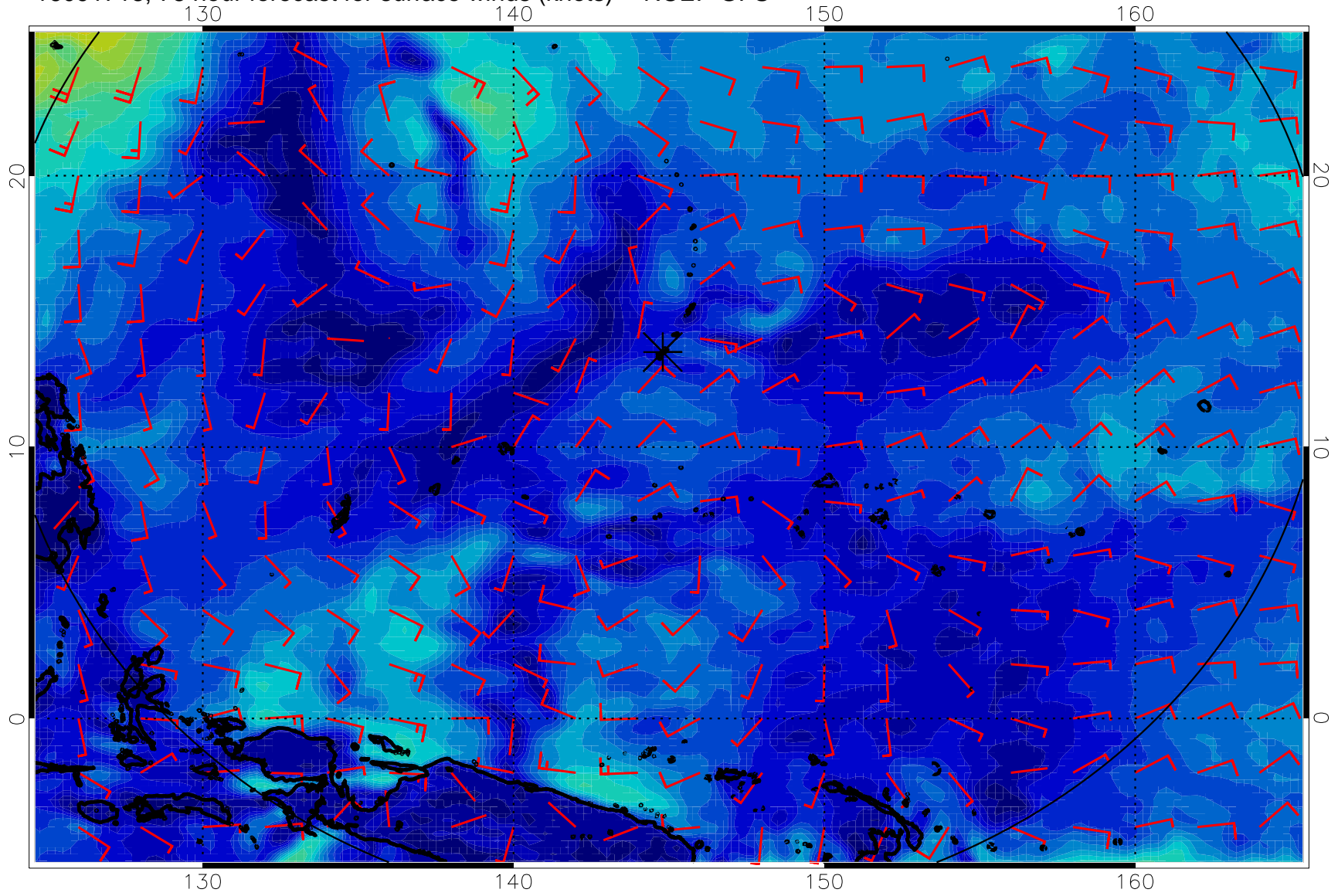
16091718, 78 hour forecast for surface winds (knots) -- NCEP GFS
