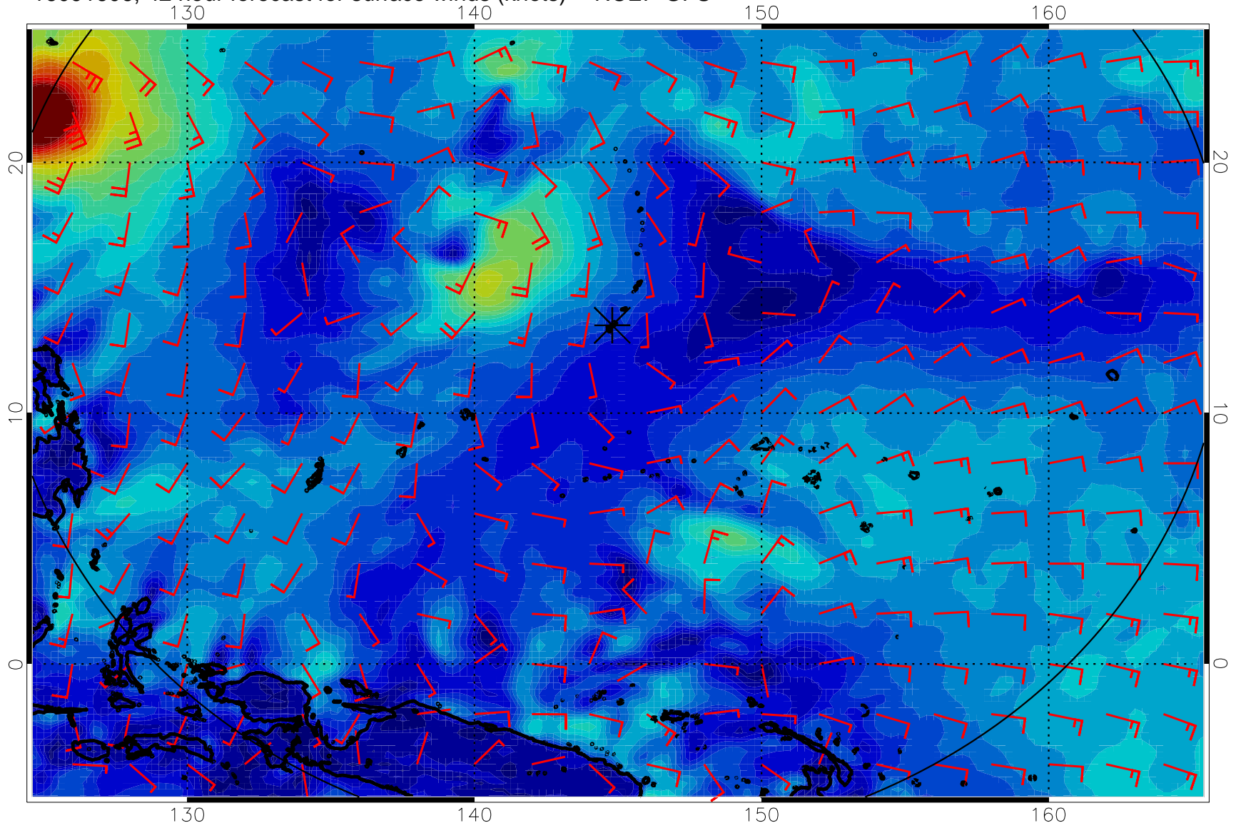
16091606, 42 hour forecast for surface winds (knots) -- NCEP GFS
