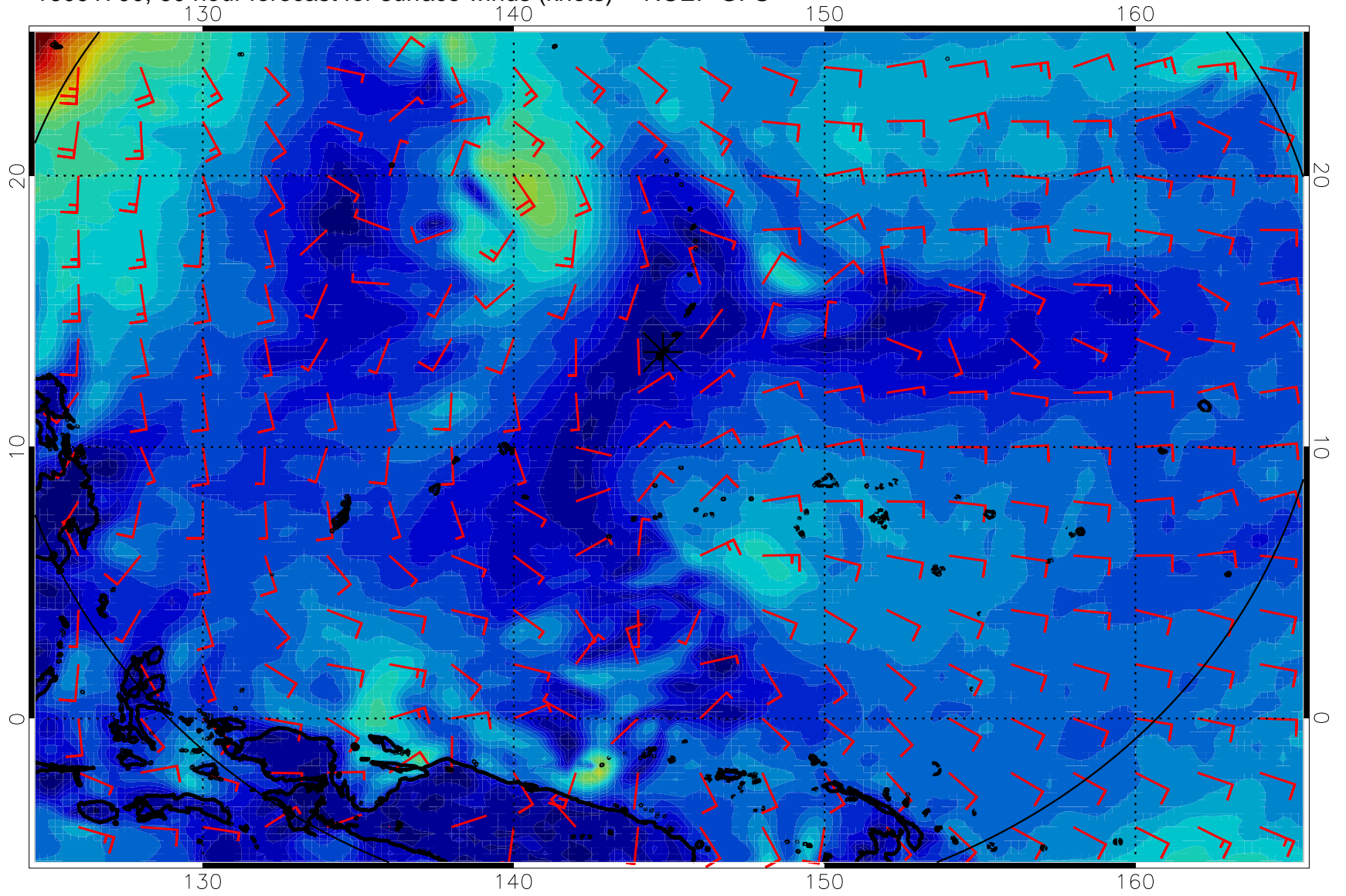
16091700, 60 hour forecast for surface winds (knots) -- NCEP GFS
