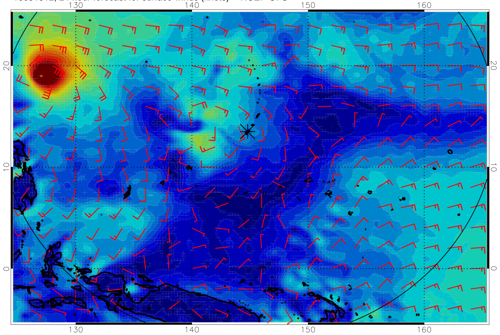
16091512, 24 hour forecast for surface winds (knots) -- NCEP GFS
