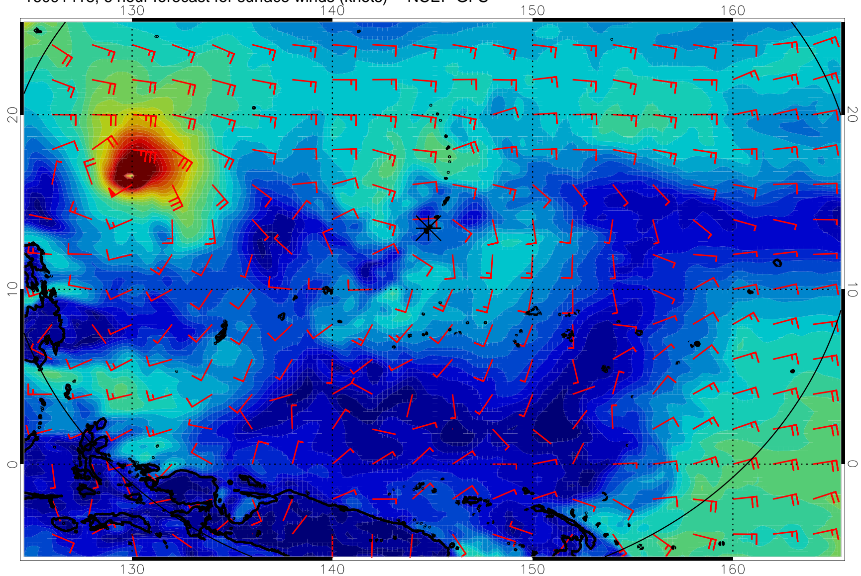
16091418, 6 hour forecast for surface winds (knots) -- NCEP GFS
