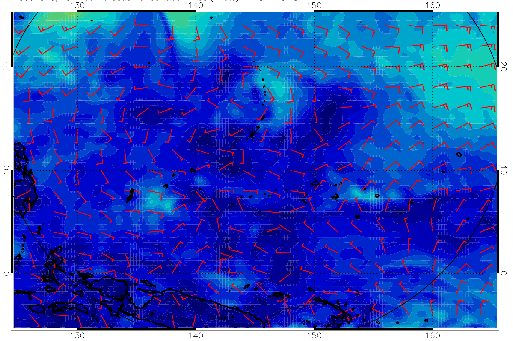
16091818, 102 hour forecast for surface winds (knots) -- NCEP GFS
