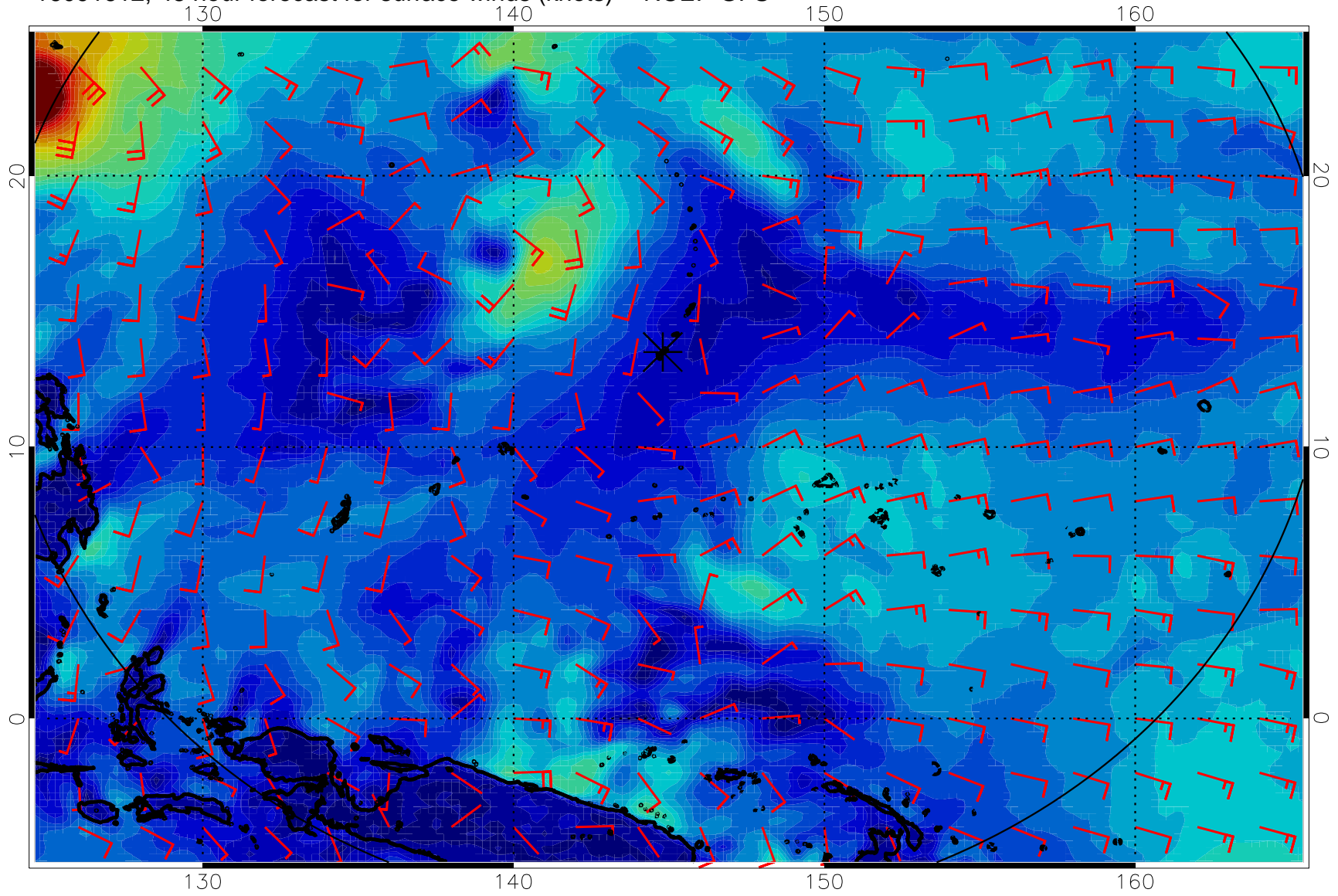
16091612, 48 hour forecast for surface winds (knots) -- NCEP GFS
