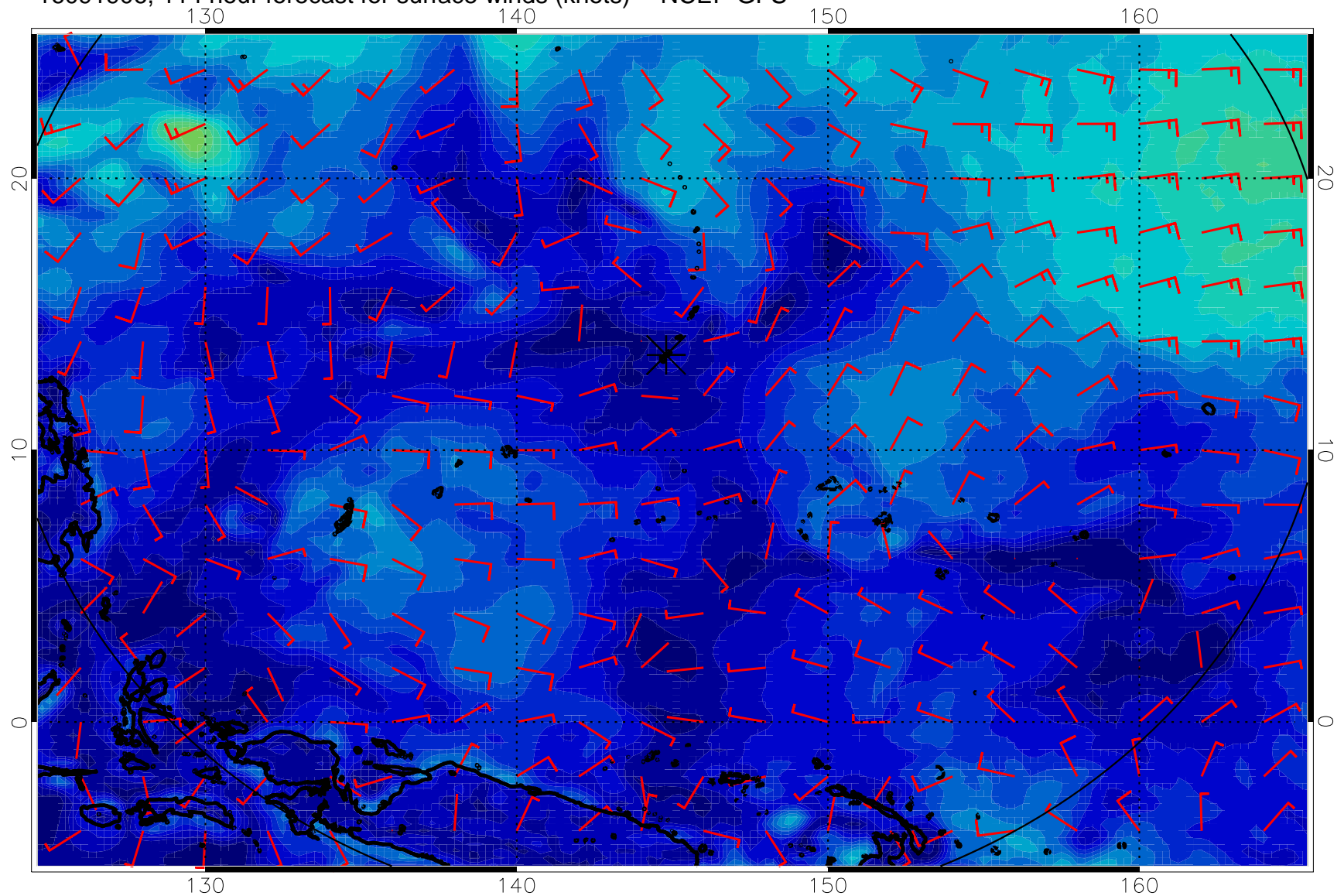
16091906, 114 hour forecast for surface winds (knots) -- NCEP GFS
