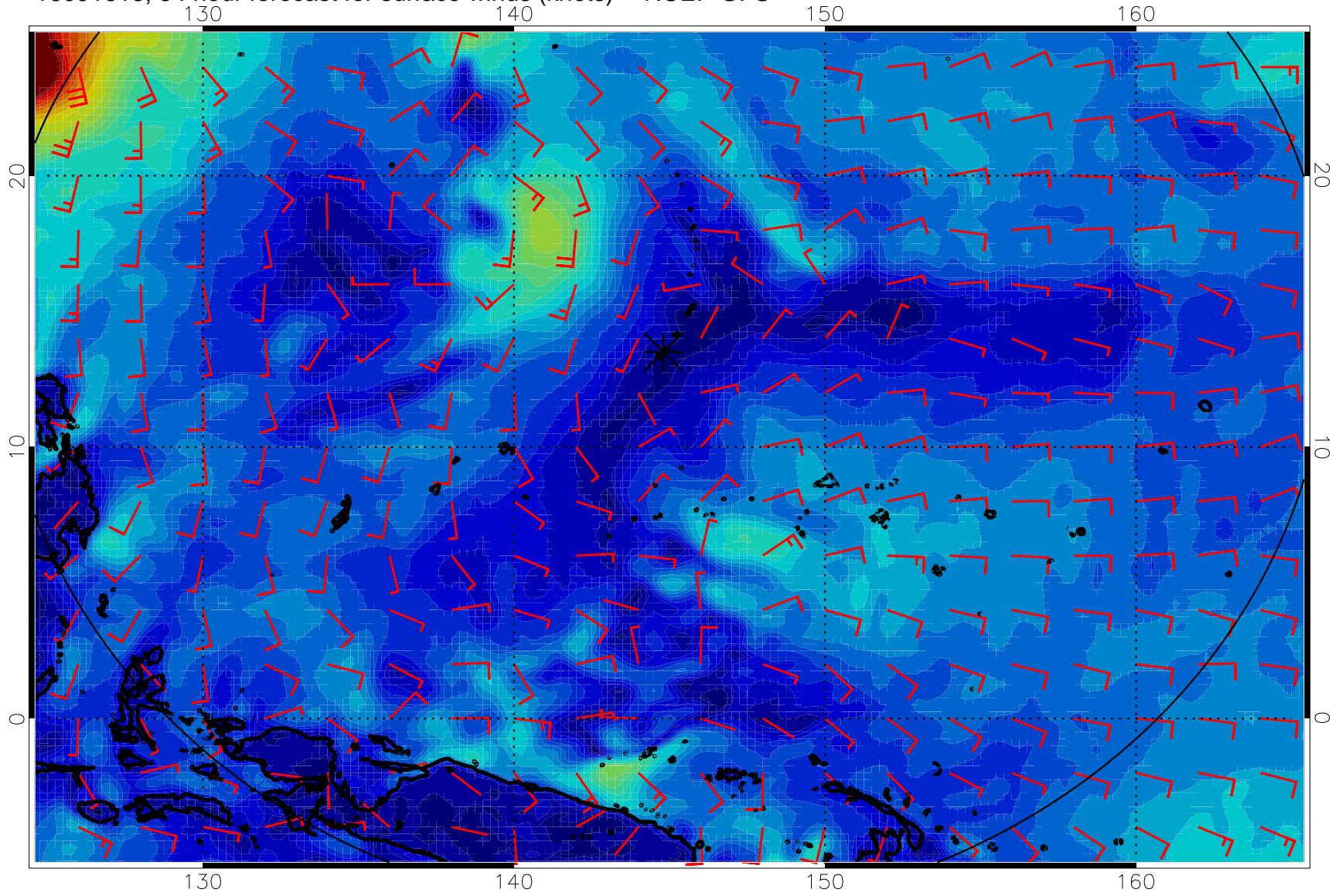
16091618, 54 hour forecast for surface winds (knots) -- NCEP GFS
