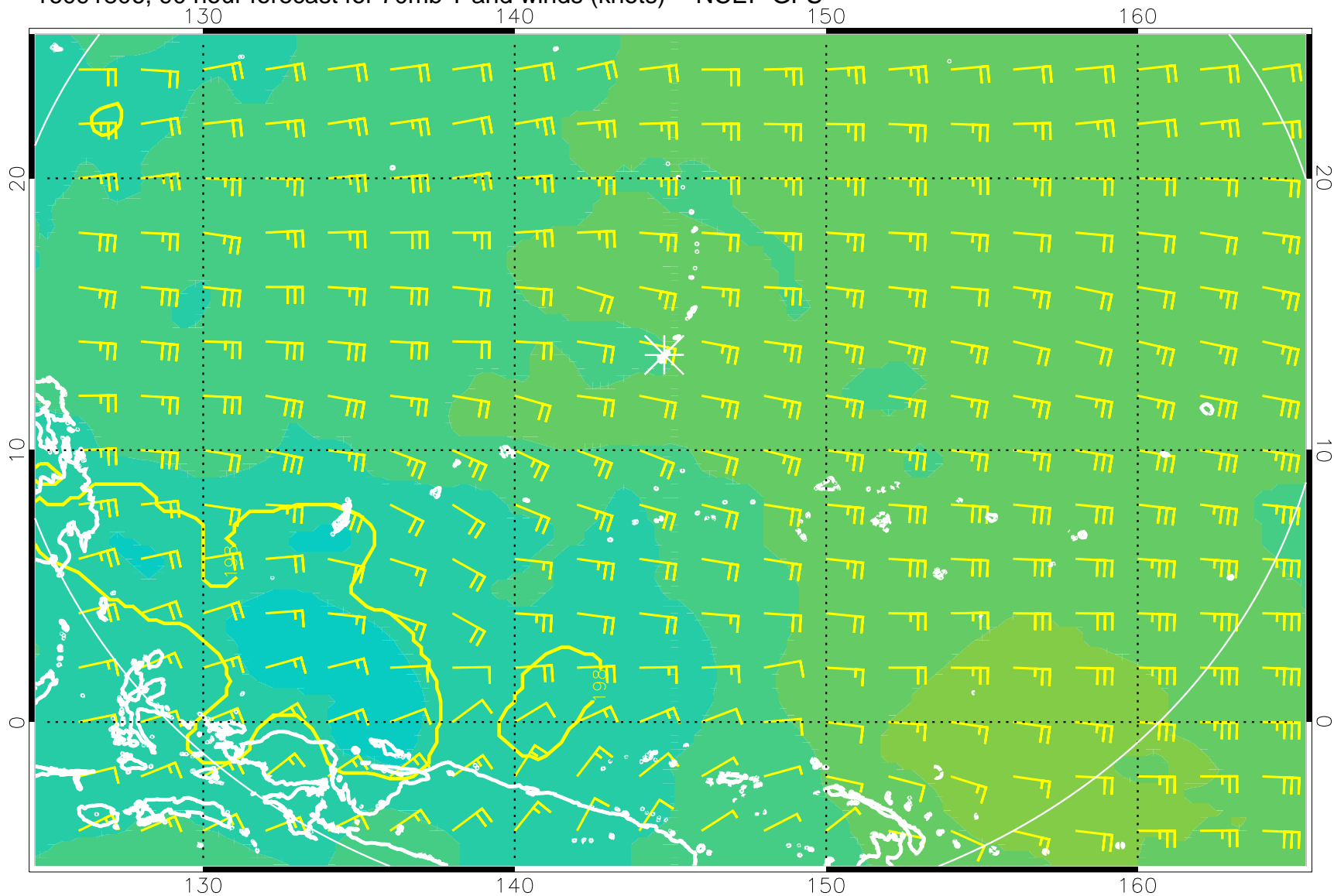
16091806, 90 hour forecast for 70mb T and winds (knots) -- NCEP GFS
