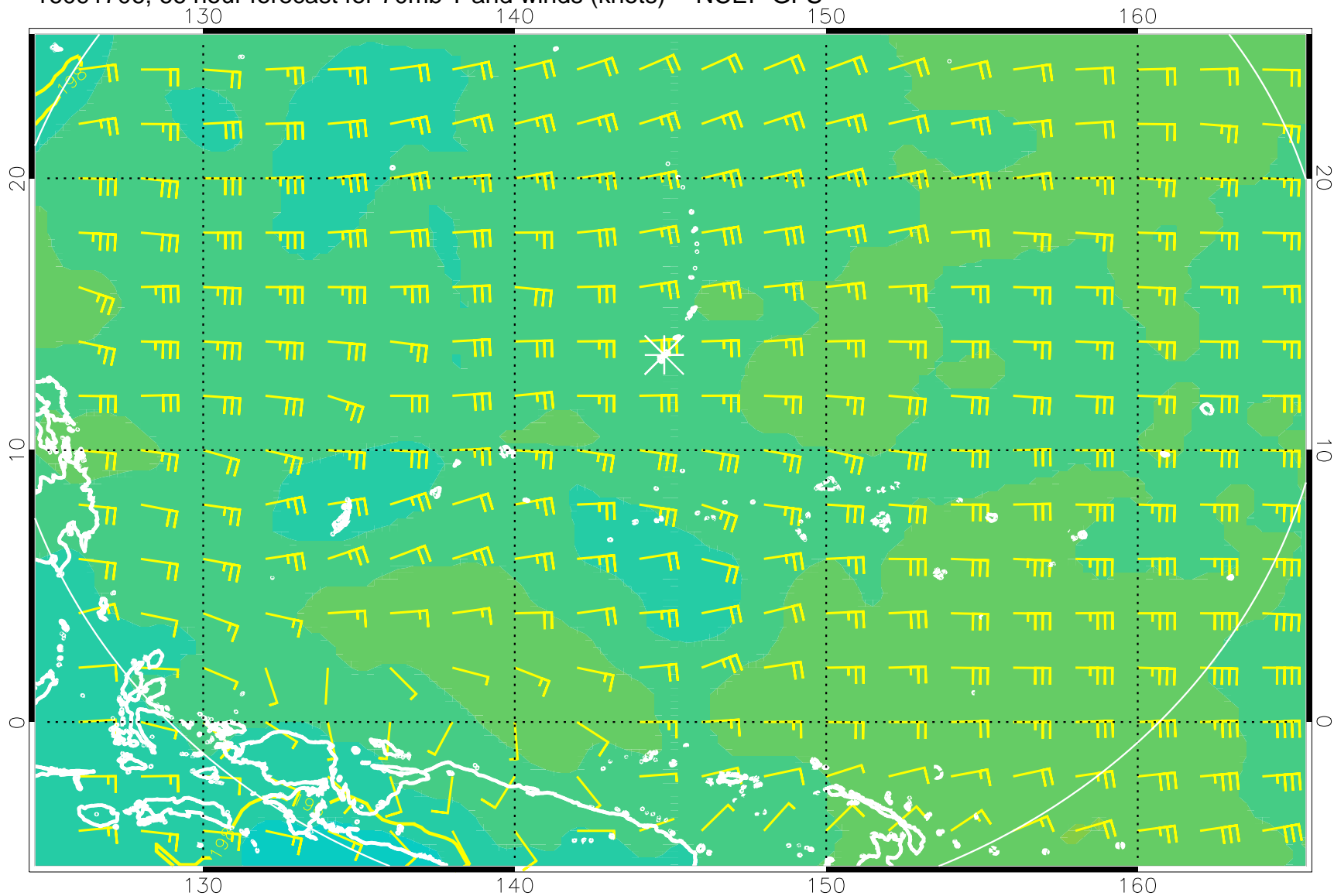
16091706, 66 hour forecast for 70mb T and winds (knots) -- NCEP GFS
