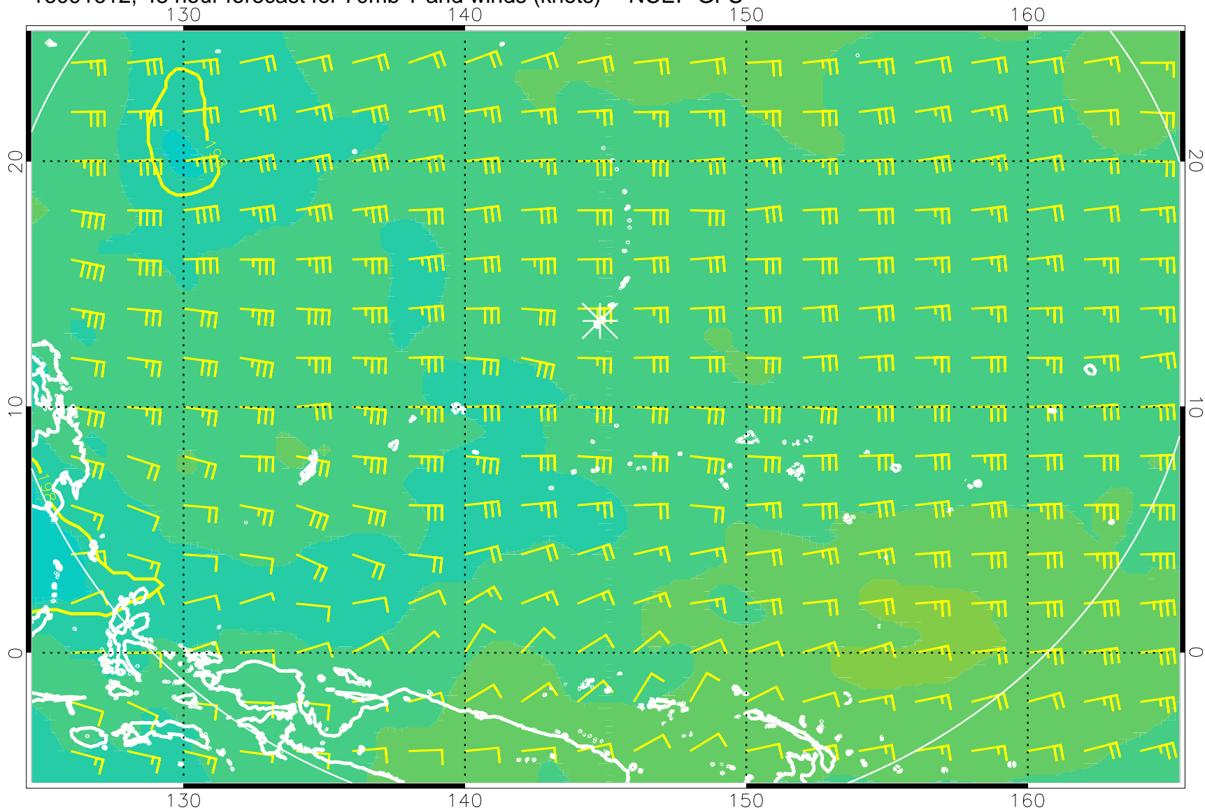
16091612, 48 hour forecast for 70mb T and winds (knots) -- NCEP GFS
