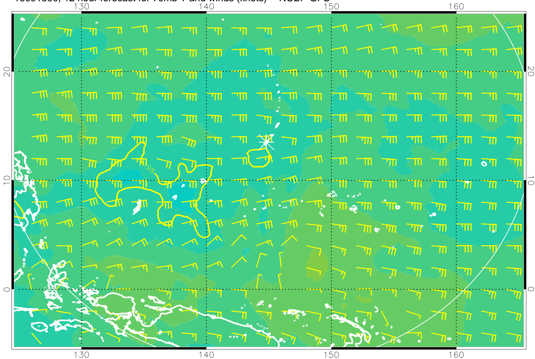
16091500, 12 hour forecast for 70mb T and winds (knots) -- NCEP GFS
