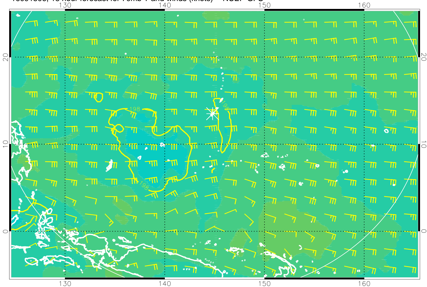
16091506, 18 hour forecast for 70mb T and winds (knots) -- NCEP GFS
