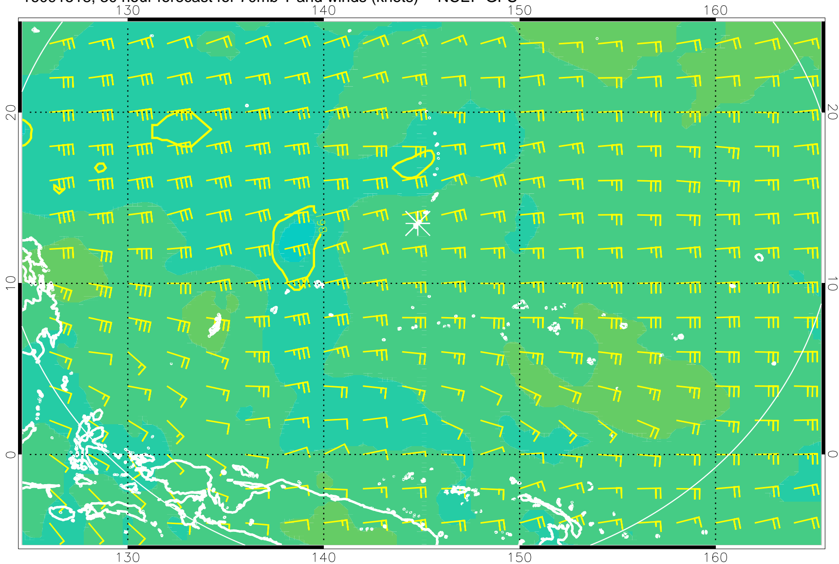
16091518, 30 hour forecast for 70mb T and winds (knots) -- NCEP GFS
