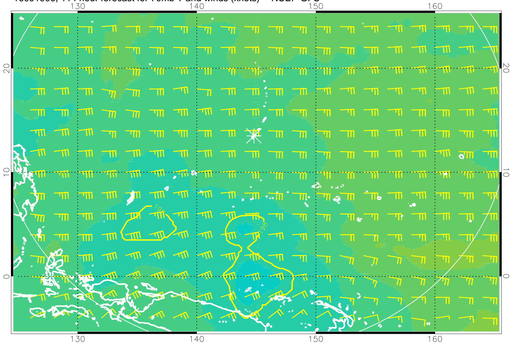
16091906, 114 hour forecast for 70mb T and winds (knots) -- NCEP GFS
