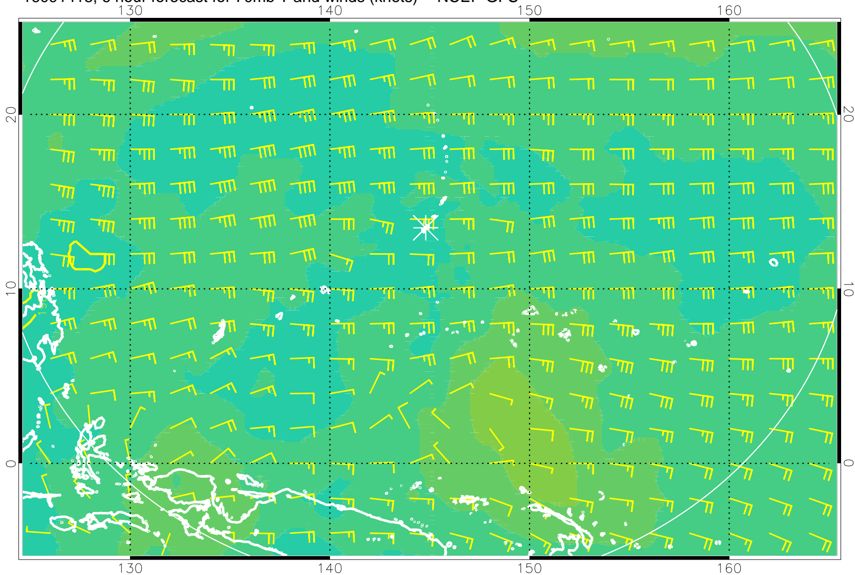
16091418, 6 hour forecast for 70mb T and winds (knots) -- NCEP GFS
