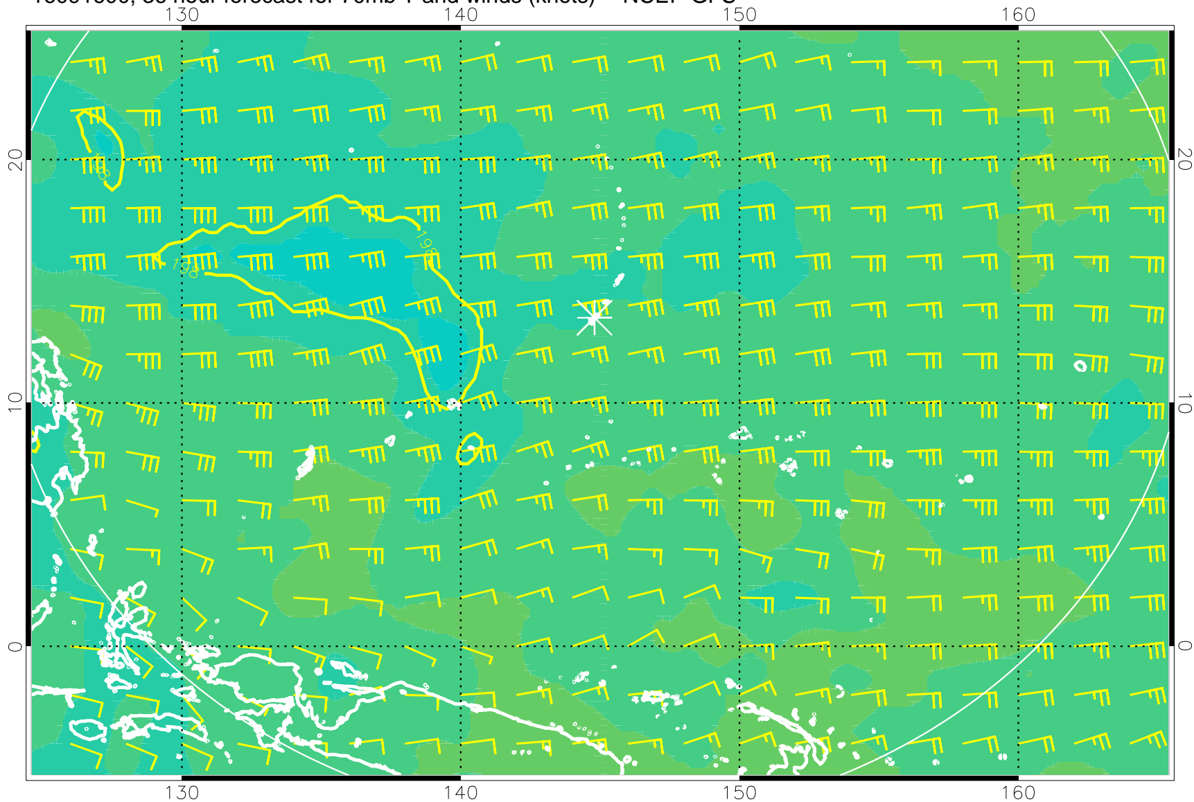
16091600, 36 hour forecast for 70mb T and winds (knots) -- NCEP GFS
