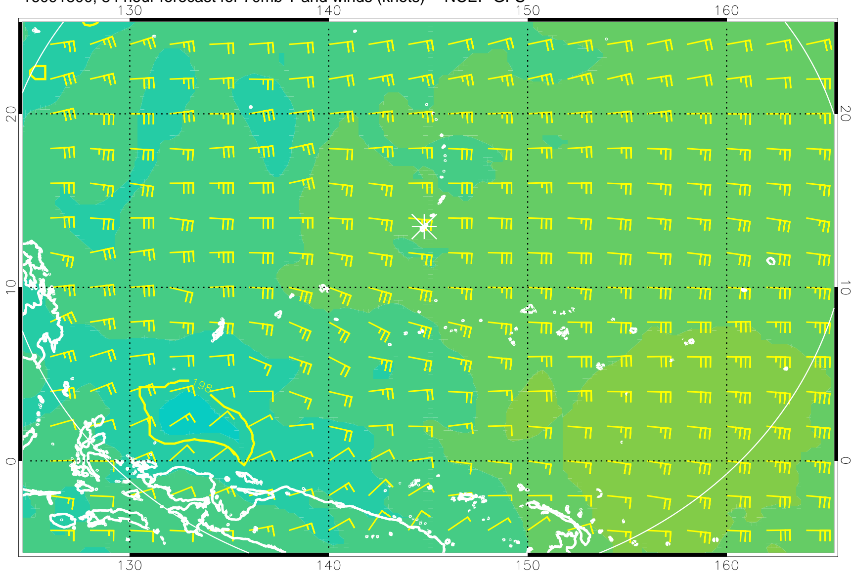
16091800, 84 hour forecast for 70mb T and winds (knots) -- NCEP GFS
