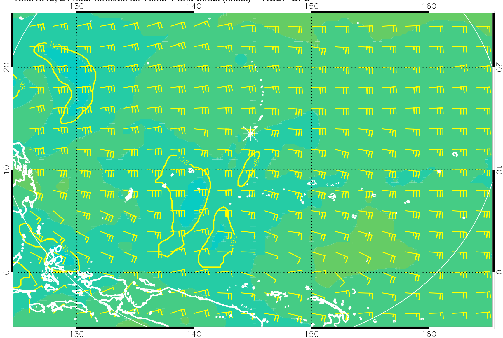
16091512, 24 hour forecast for 70mb T and winds (knots) -- NCEP GFS
