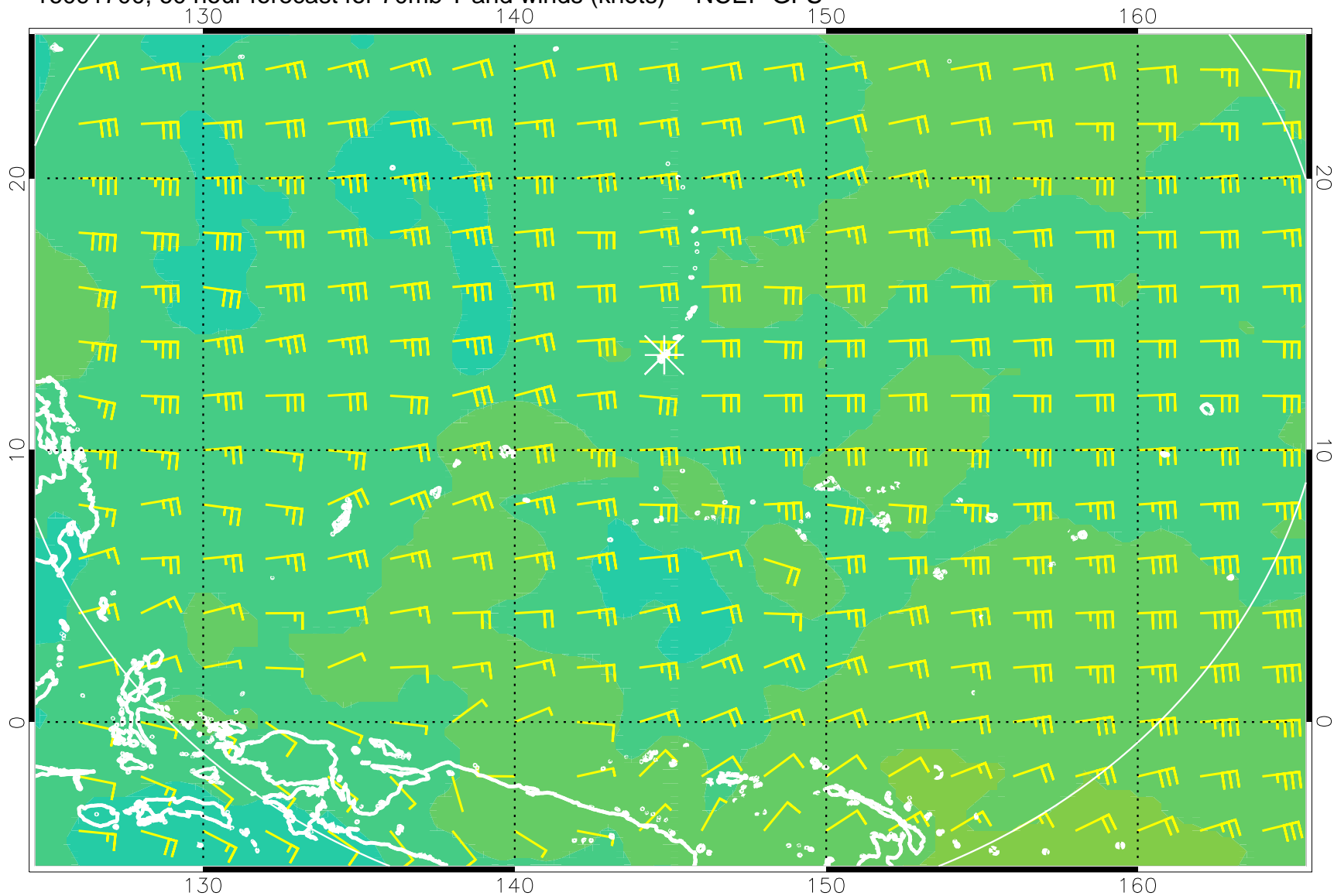
16091700, 60 hour forecast for 70mb T and winds (knots) -- NCEP GFS
