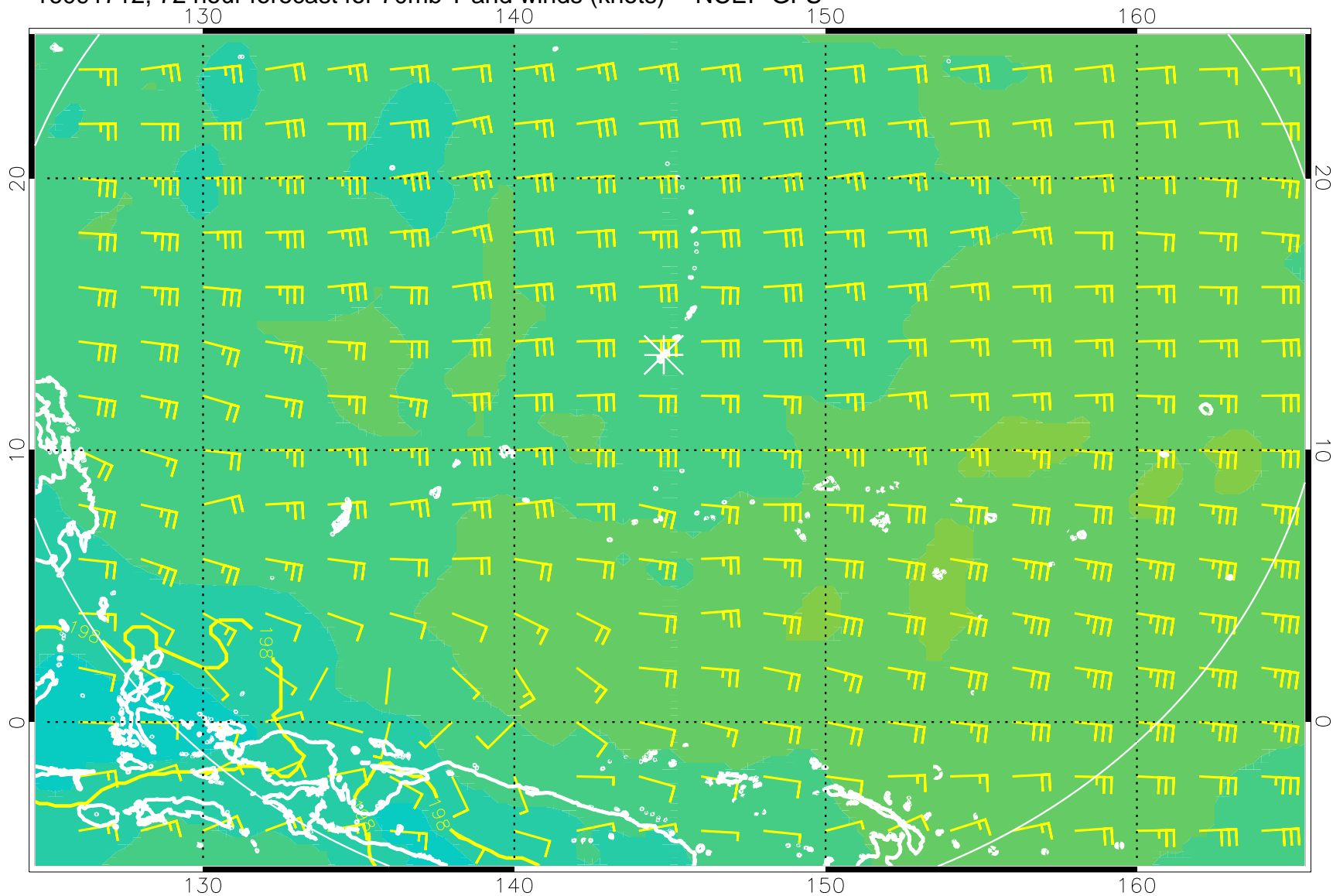
16091712, 72 hour forecast for 70mb T and winds (knots) -- NCEP GFS
