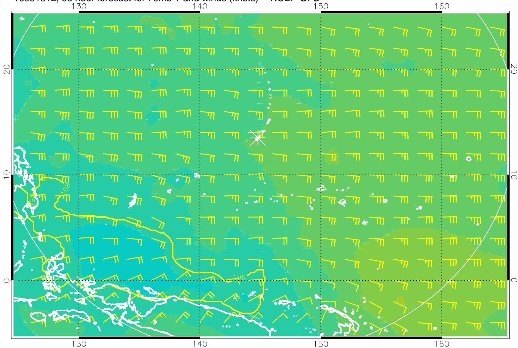
16091812, 96 hour forecast for 70mb T and winds (knots) -- NCEP GFS
