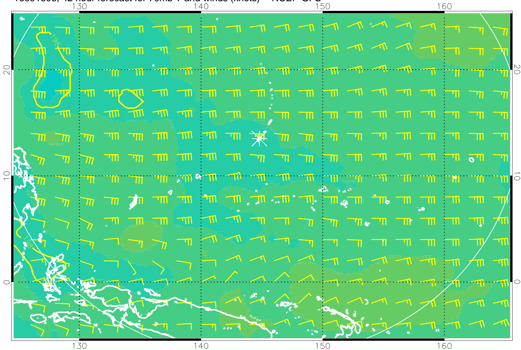
16091606, 42 hour forecast for 70mb T and winds (knots) -- NCEP GFS
