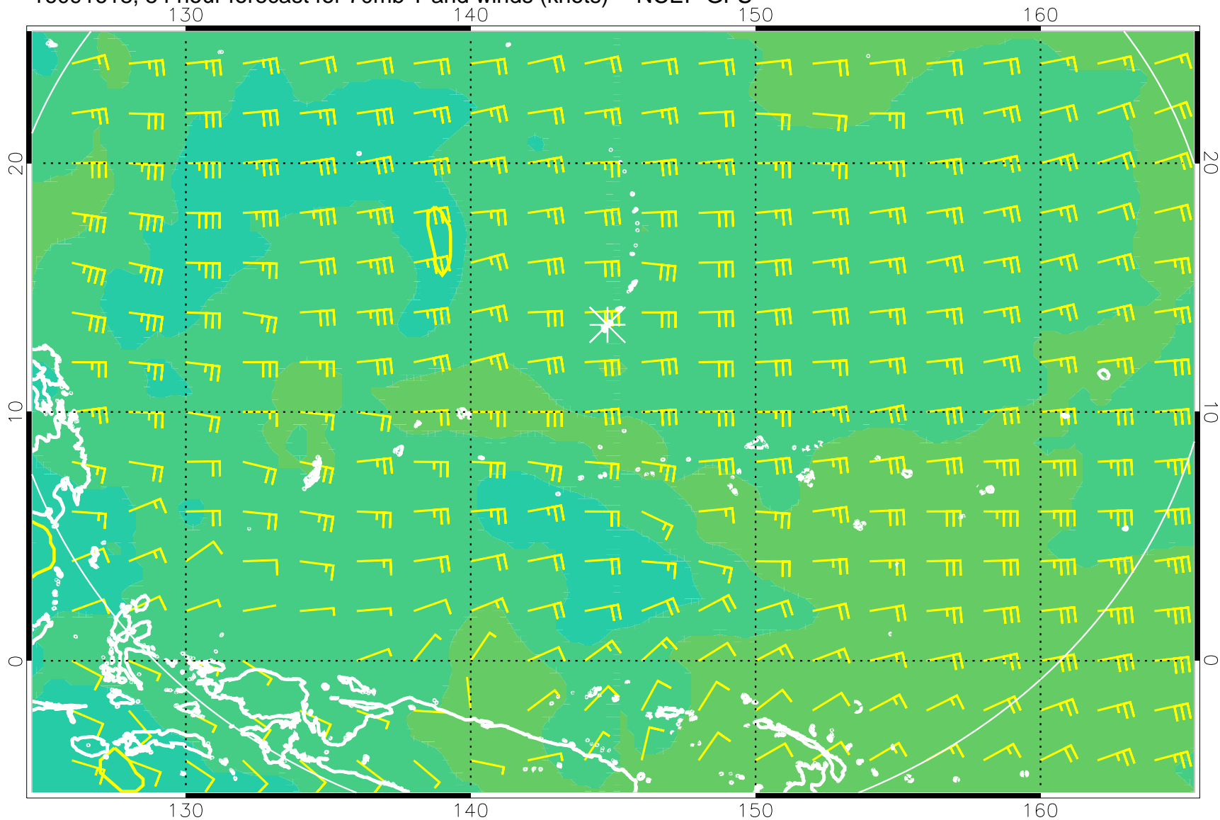
16091618, 54 hour forecast for 70mb T and winds (knots) -- NCEP GFS
