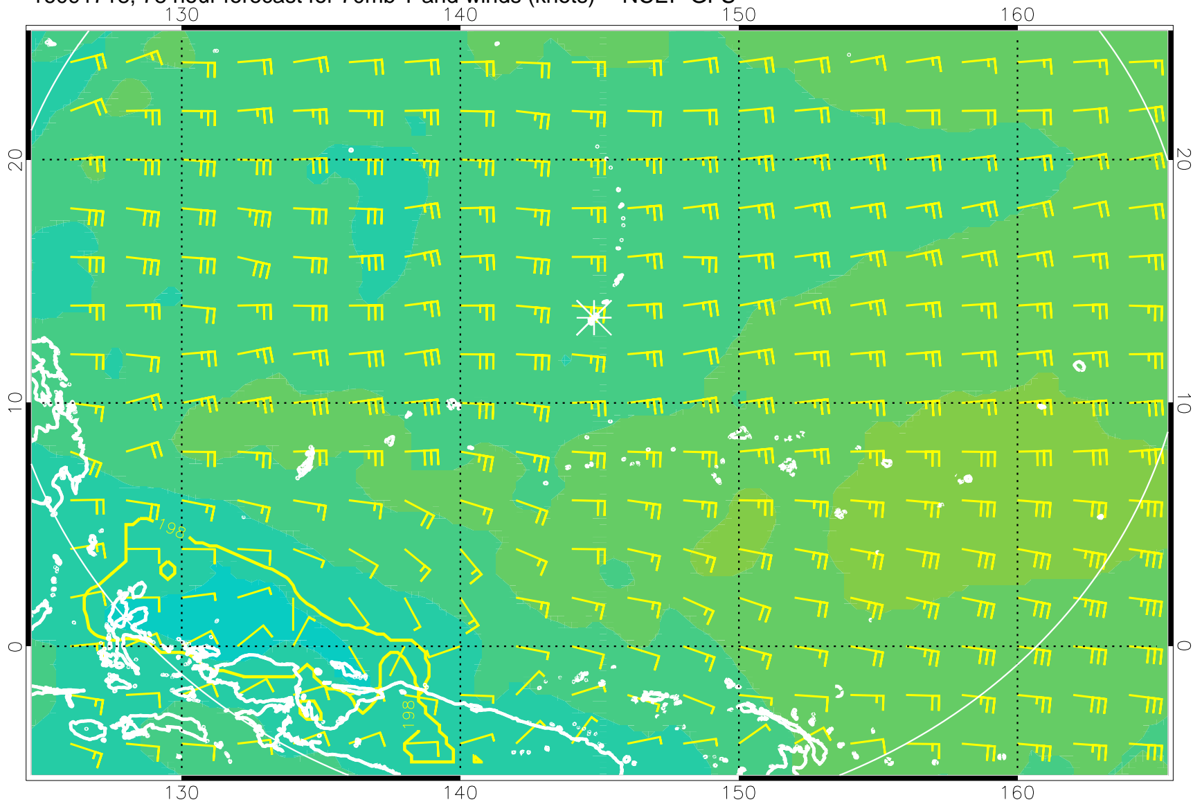
16091718, 78 hour forecast for 70mb T and winds (knots) -- NCEP GFS
