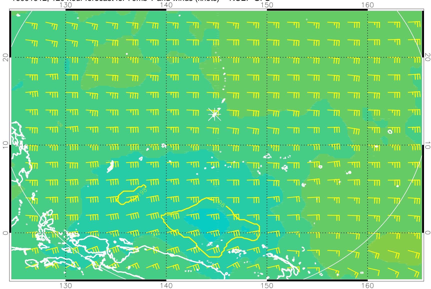
16091912, 120 hour forecast for 70mb T and winds (knots) -- NCEP GFS
