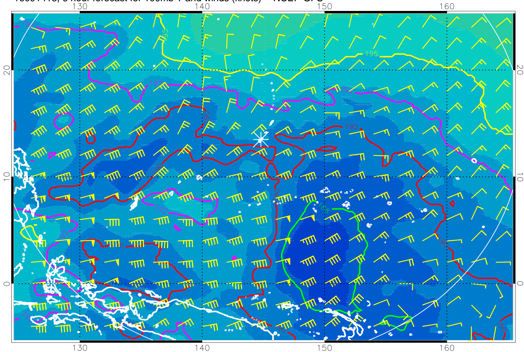
16091418, 6 hour forecast for 100mb T and winds (knots) -- NCEP GFS
