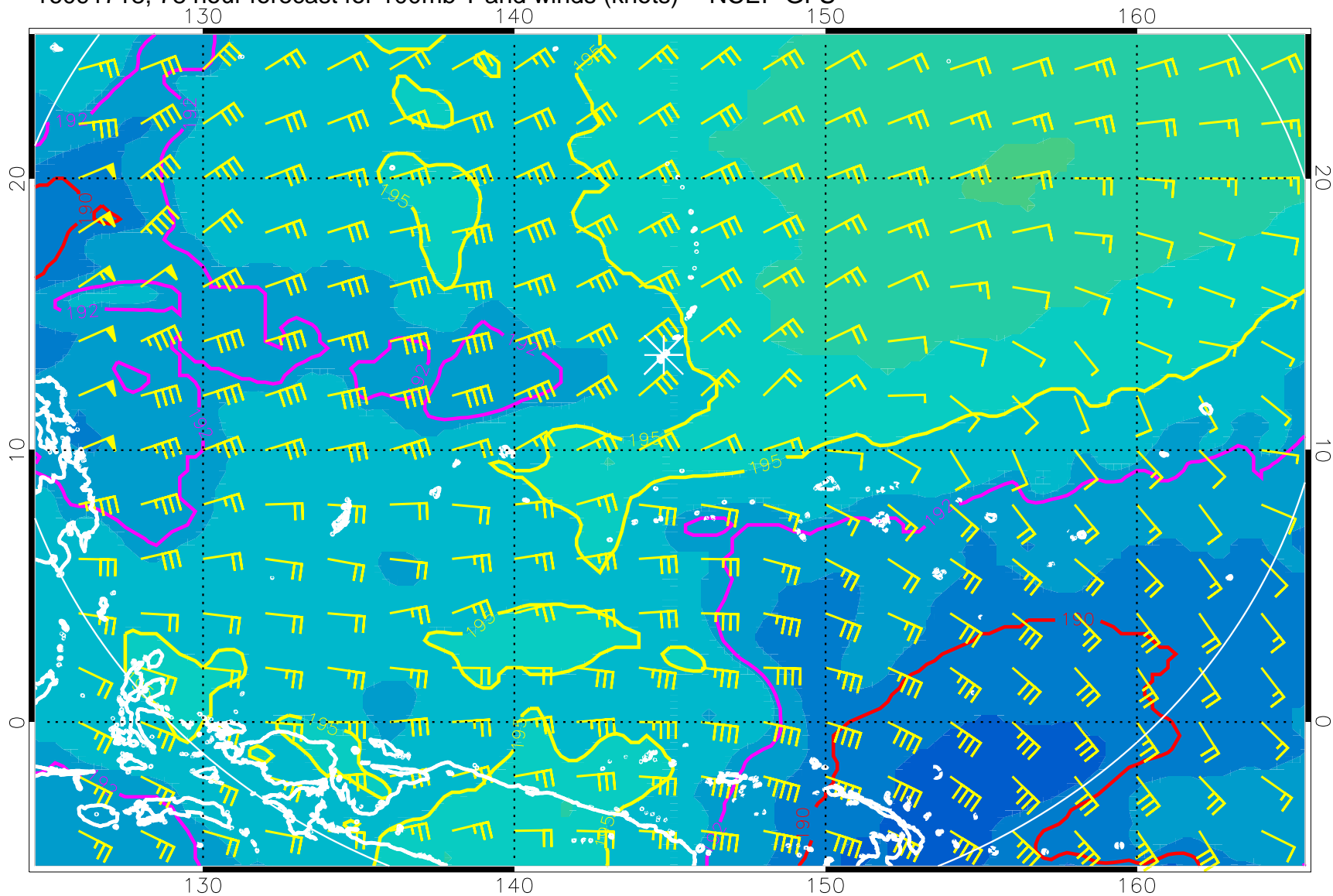
16091718, 78 hour forecast for 100mb T and winds (knots) -- NCEP GFS
