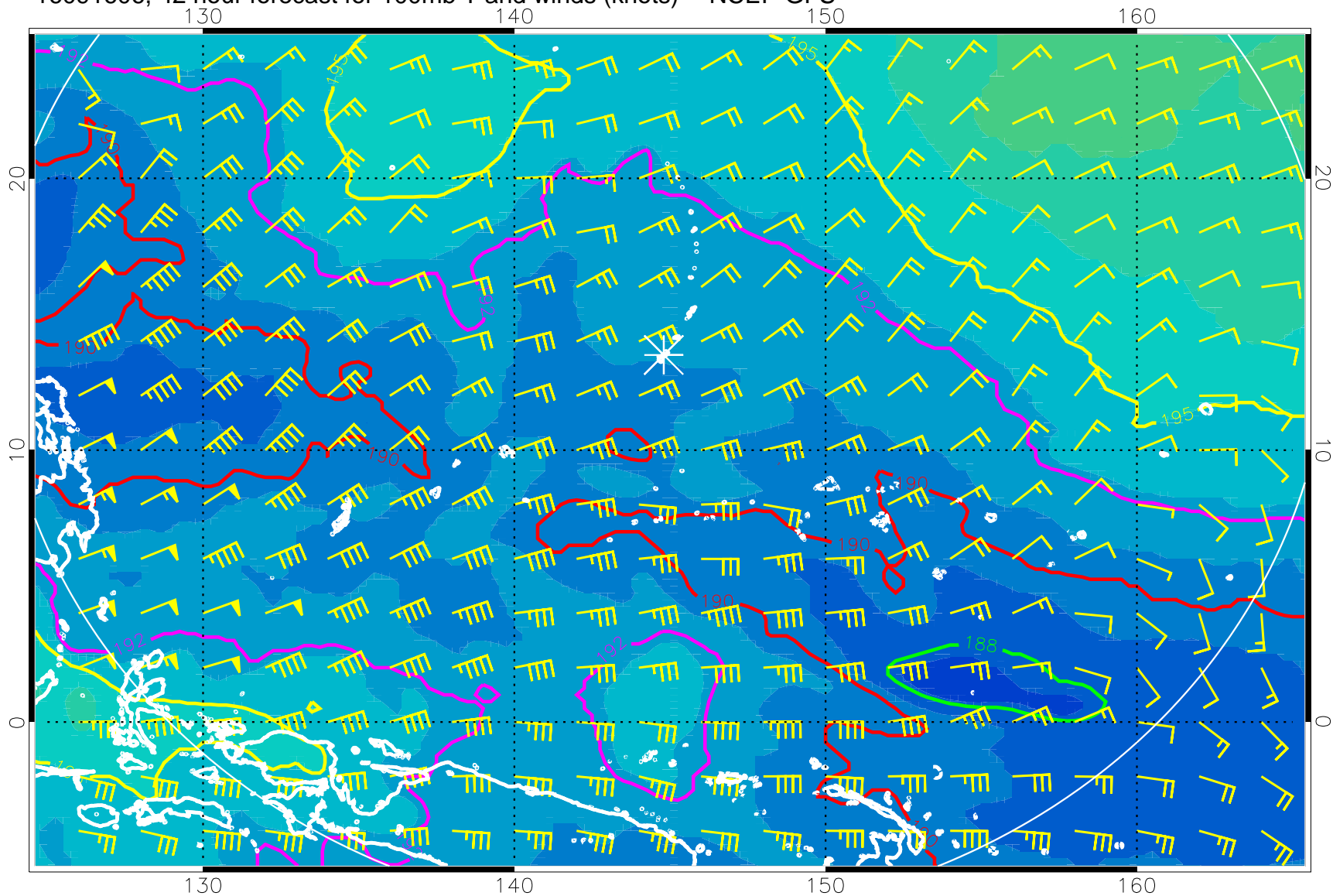
16091606, 42 hour forecast for 100mb T and winds (knots) -- NCEP GFS
