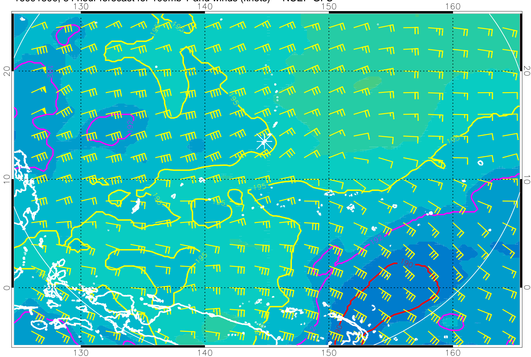
16091800, 84 hour forecast for 100mb T and winds (knots) -- NCEP GFS
