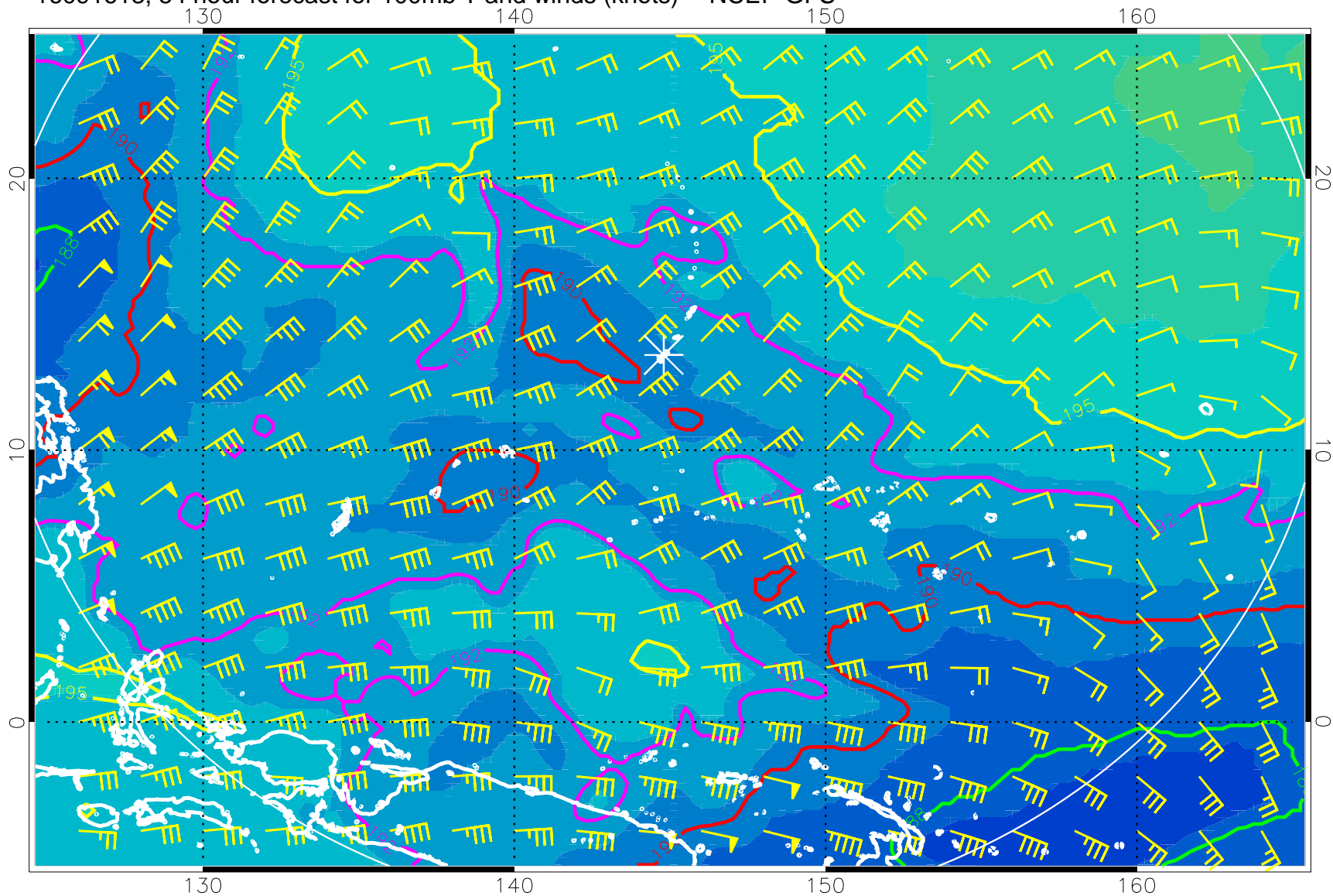
16091618, 54 hour forecast for 100mb T and winds (knots) -- NCEP GFS
