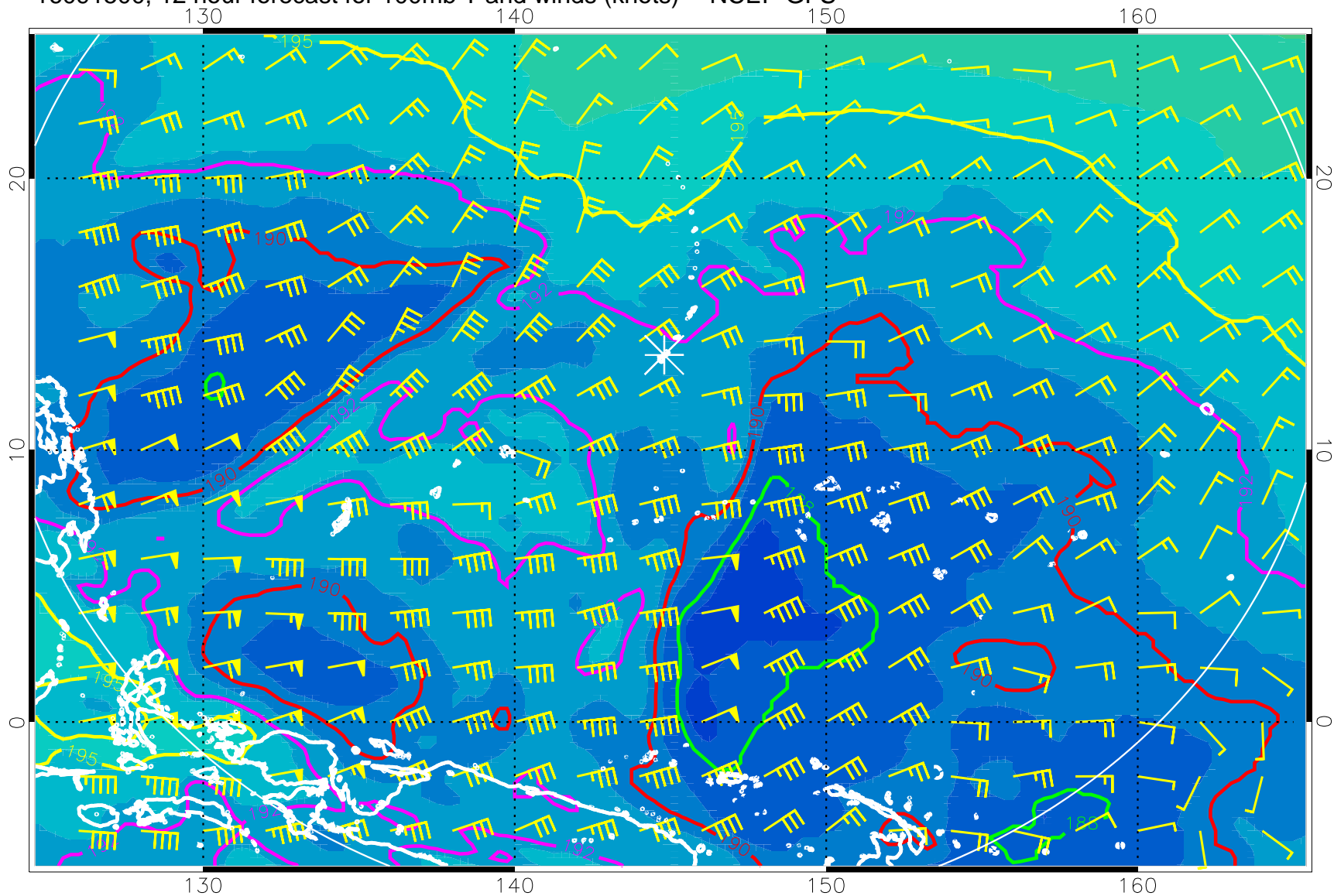
16091500, 12 hour forecast for 100mb T and winds (knots) -- NCEP GFS
