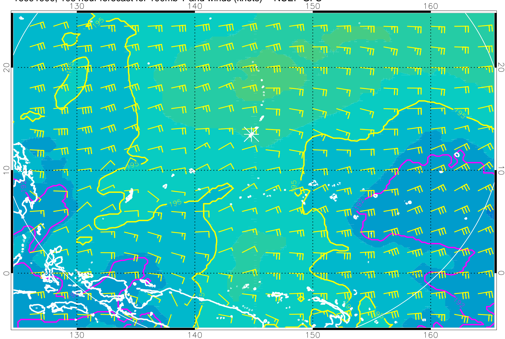
16091900, 108 hour forecast for 100mb T and winds (knots) -- NCEP GFS
