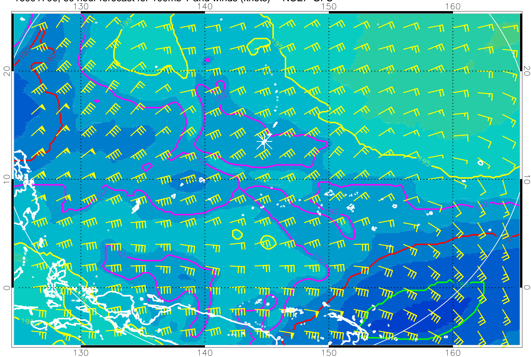
16091700, 60 hour forecast for 100mb T and winds (knots) -- NCEP GFS
