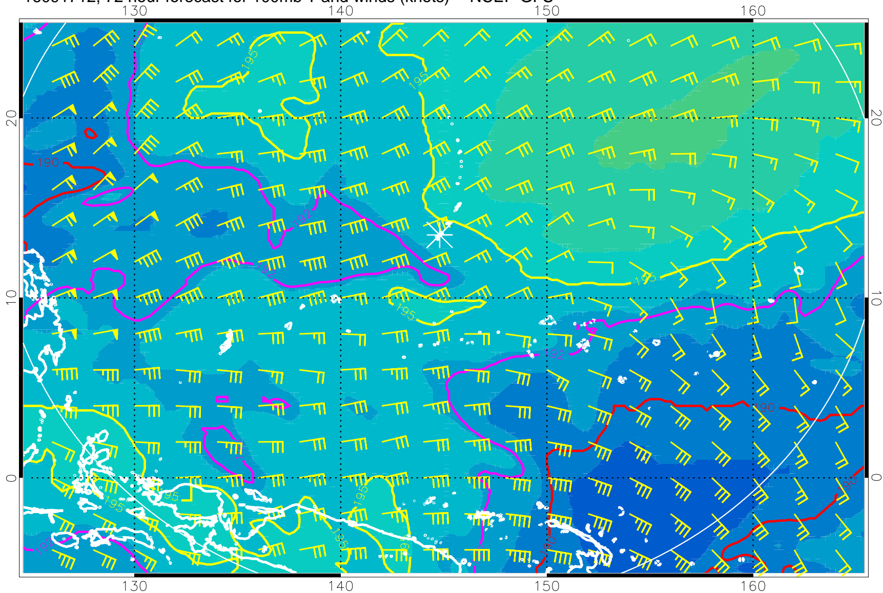
16091712, 72 hour forecast for 100mb T and winds (knots) -- NCEP GFS
