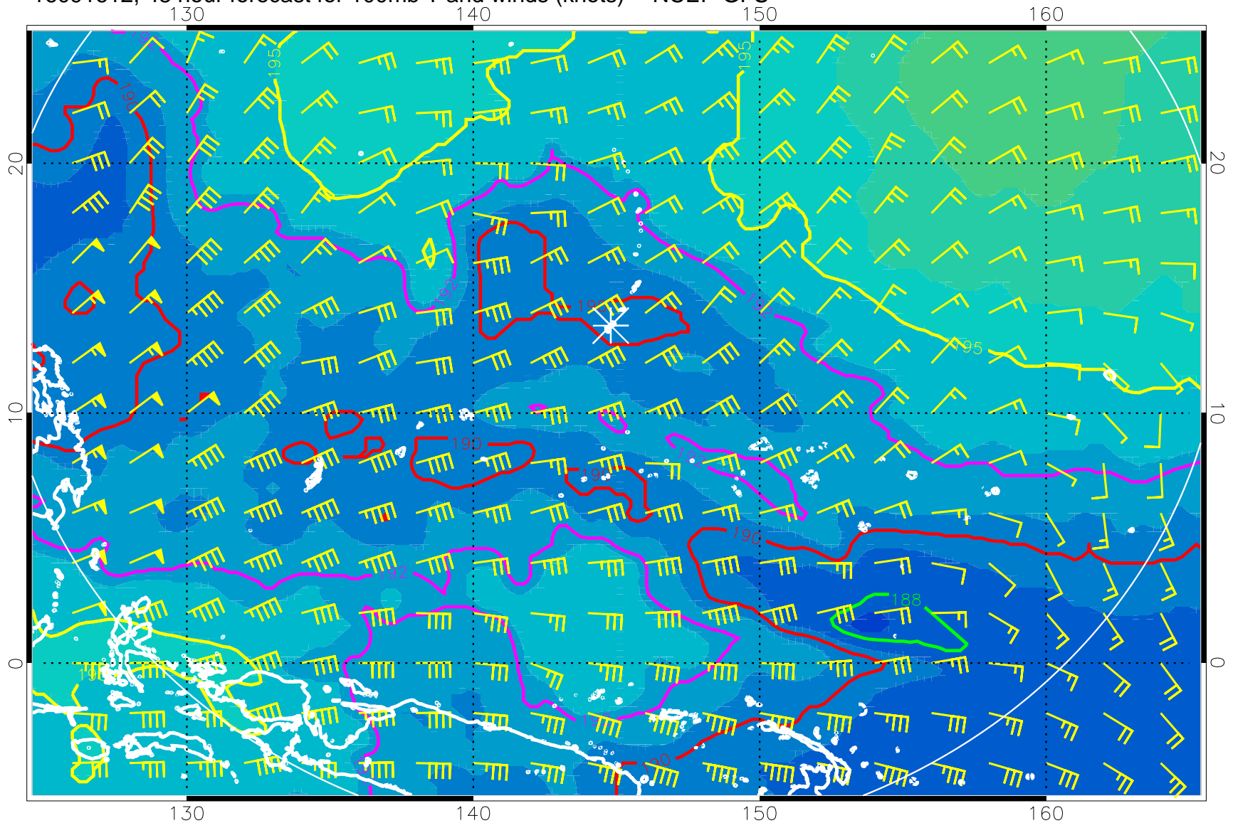
16091612, 48 hour forecast for 100mb T and winds (knots) -- NCEP GFS
