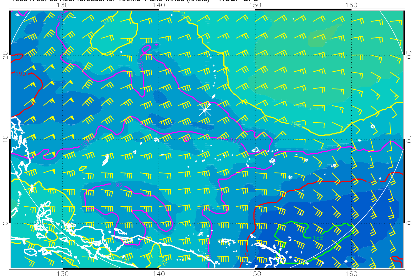
16091706, 66 hour forecast for 100mb T and winds (knots) -- NCEP GFS
