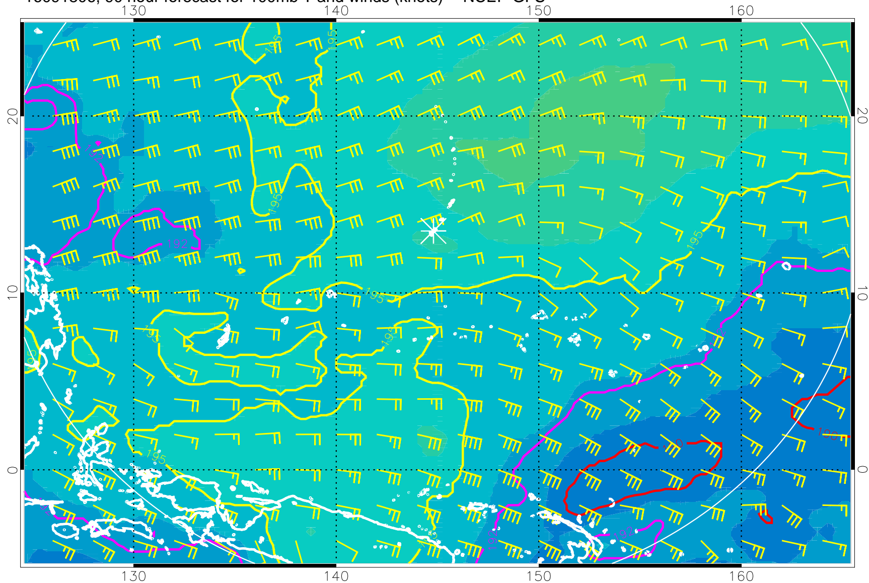
16091806, 90 hour forecast for 100mb T and winds (knots) -- NCEP GFS
