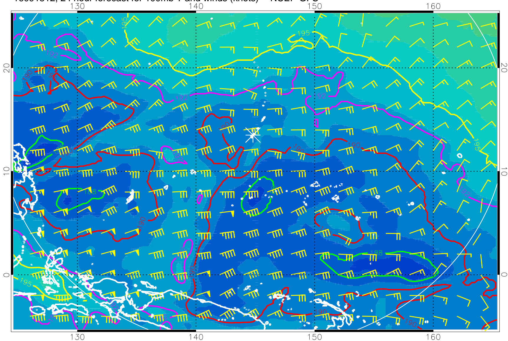
16091512, 24 hour forecast for 100mb T and winds (knots) -- NCEP GFS
