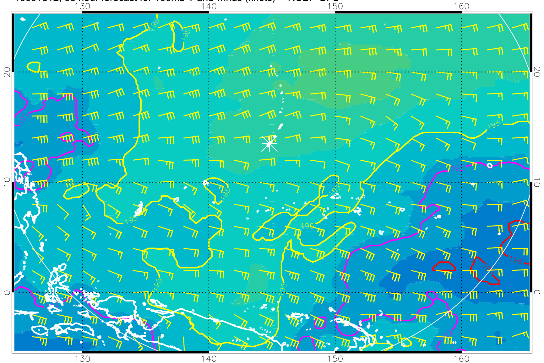
16091812, 96 hour forecast for 100mb T and winds (knots) -- NCEP GFS
