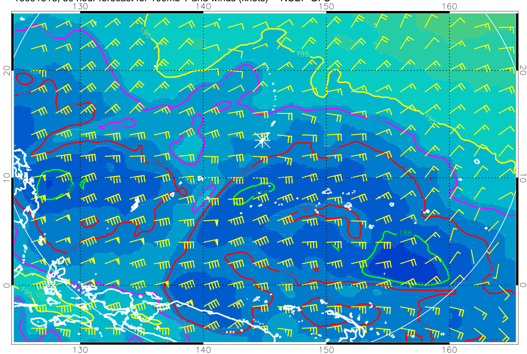
16091518, 30 hour forecast for 100mb T and winds (knots) -- NCEP GFS
