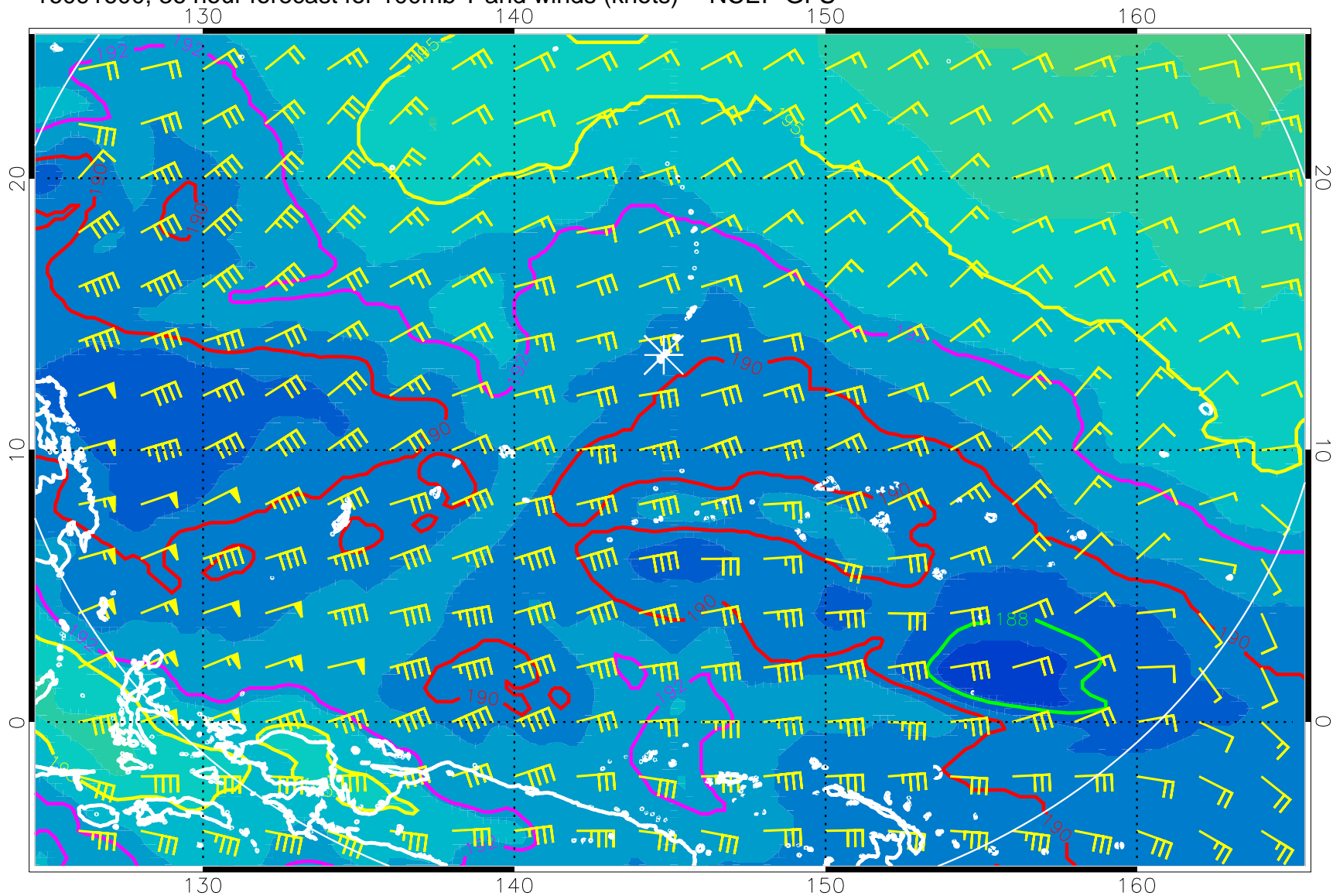
16091600, 36 hour forecast for 100mb T and winds (knots) -- NCEP GFS
