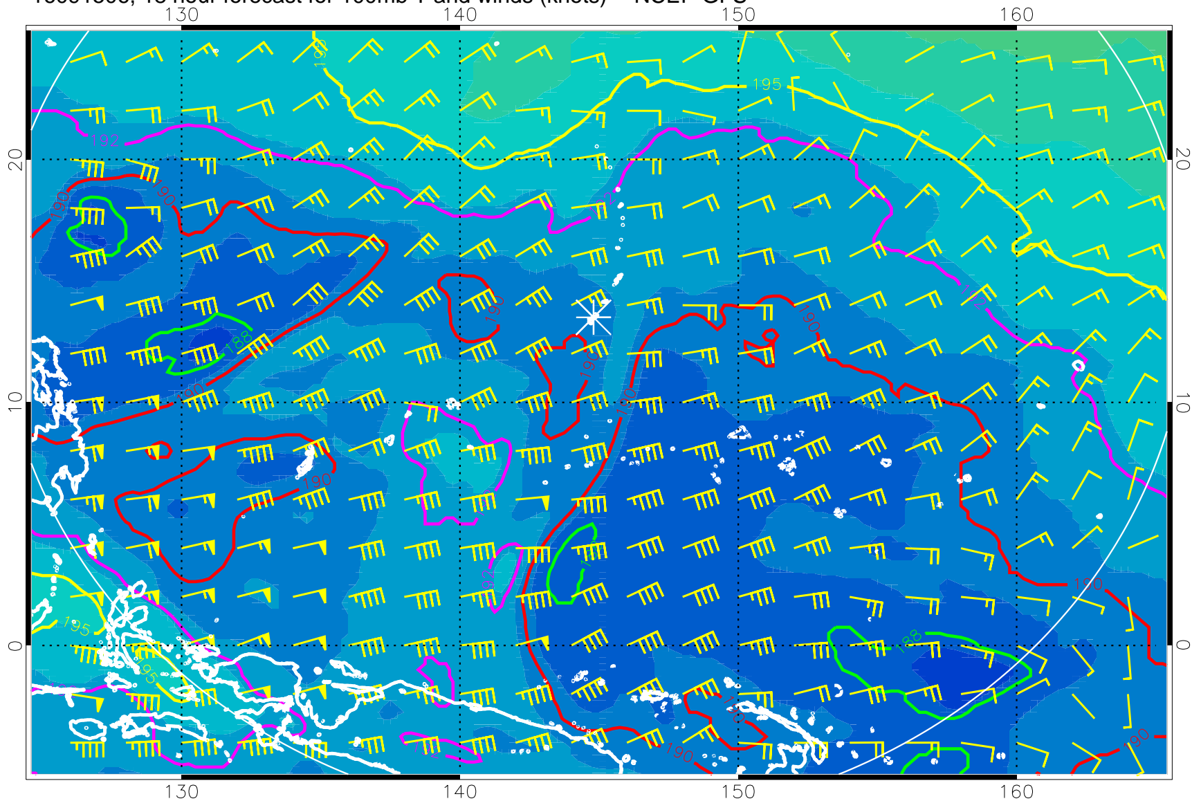
16091506, 18 hour forecast for 100mb T and winds (knots) -- NCEP GFS
