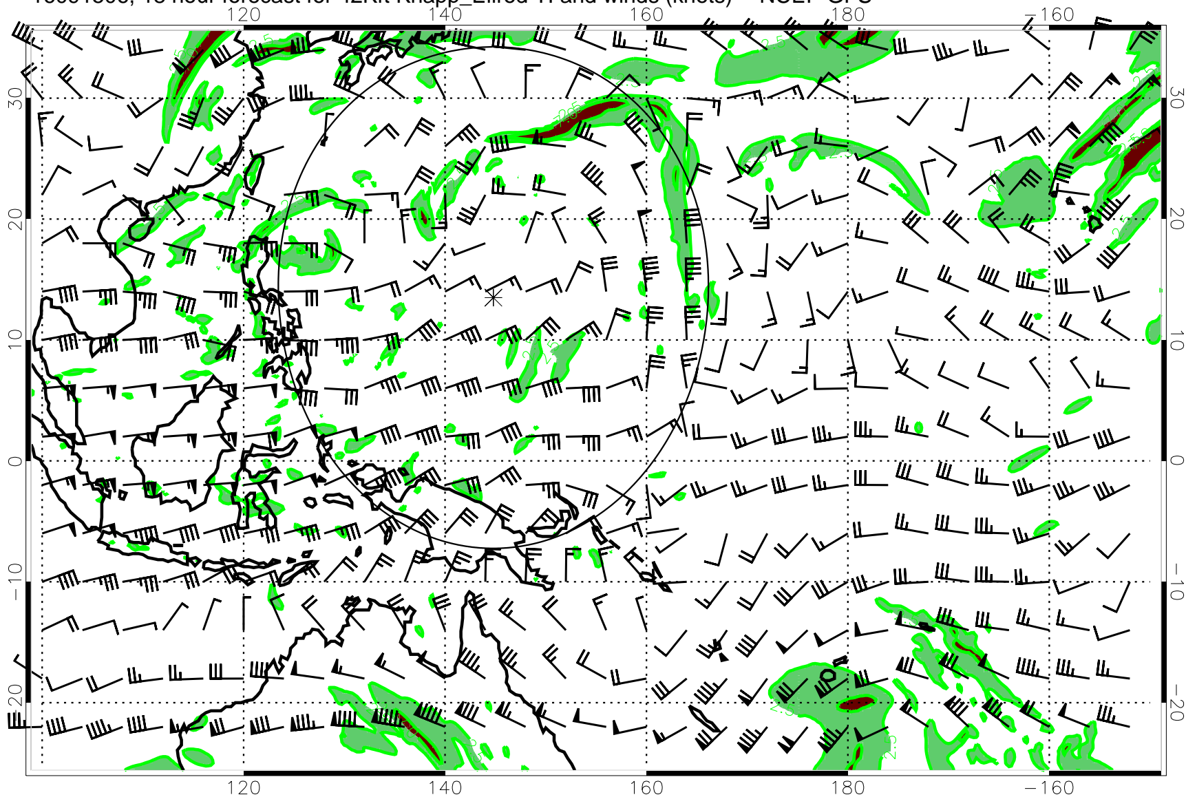
16091506, 18 hour forecast for 42Kft Knapp_Ellrod TI and winds (knots) -- NCEP GFS
