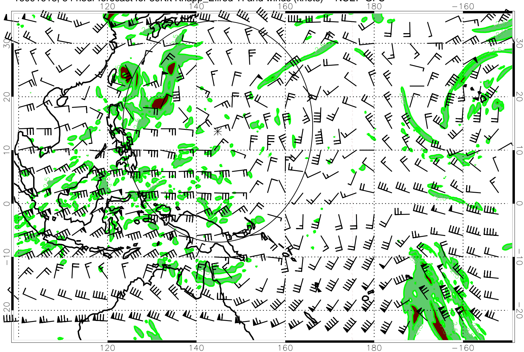
16091618, 54 hour forecast for 39Kft Knapp_Ellrod TI and winds (knots) -- NCEP GFS
