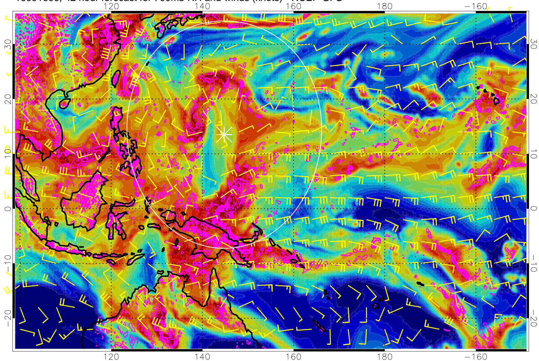
16091606, 42 hour forecast for 700mb RH and winds (knots) - NCEP GFS
