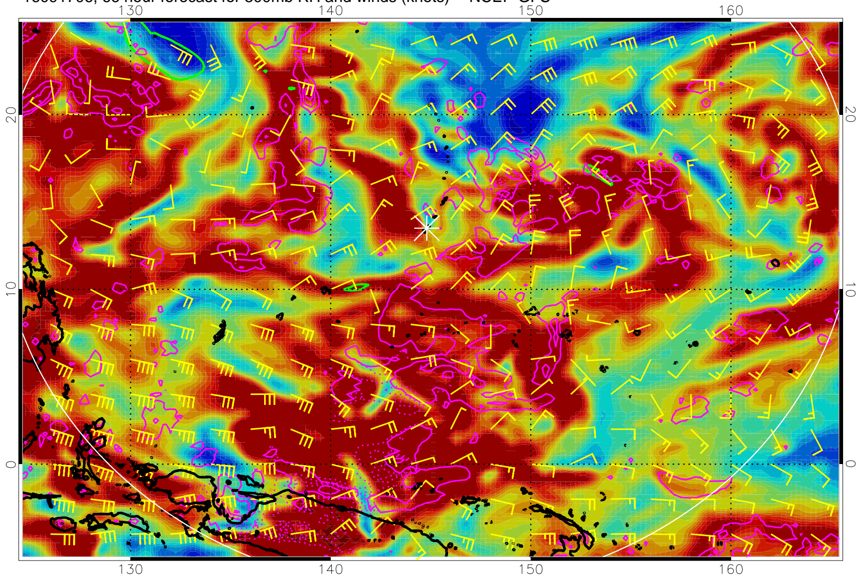
16091706, 66 hour forecast for 300mb RH and winds (knots) -- NCEP GFS
