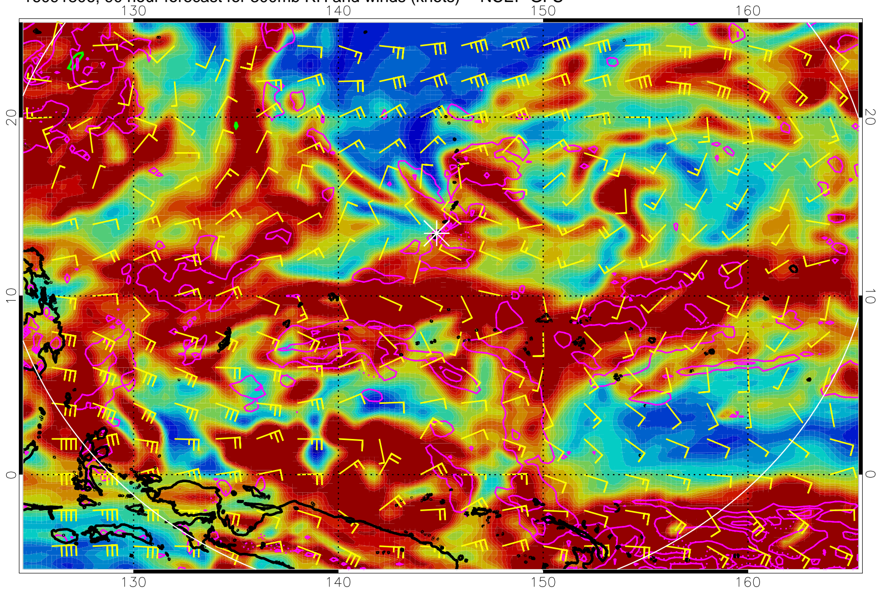
16091806, 90 hour forecast for 300mb RH and winds (knots) -- NCEP GFS
