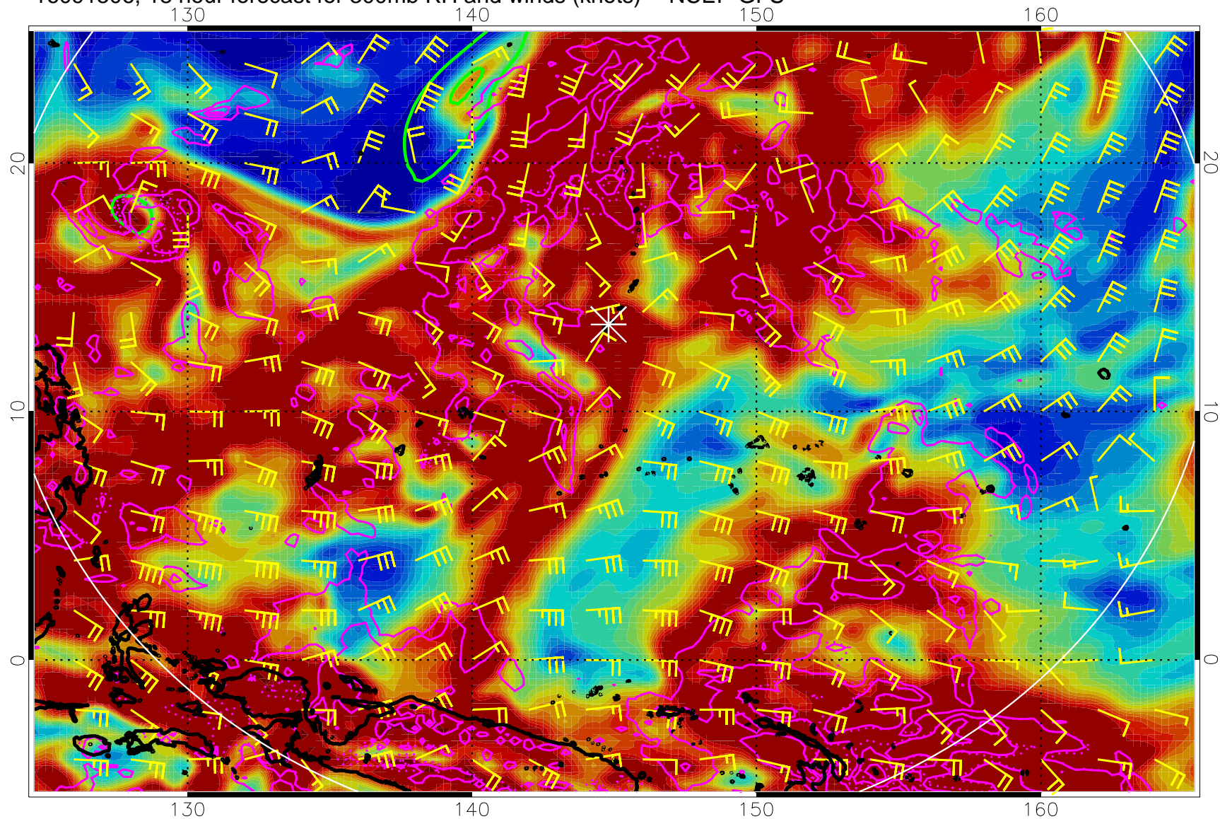
16091506, 18 hour forecast for 300mb RH and winds (knots) -- NCEP GFS
