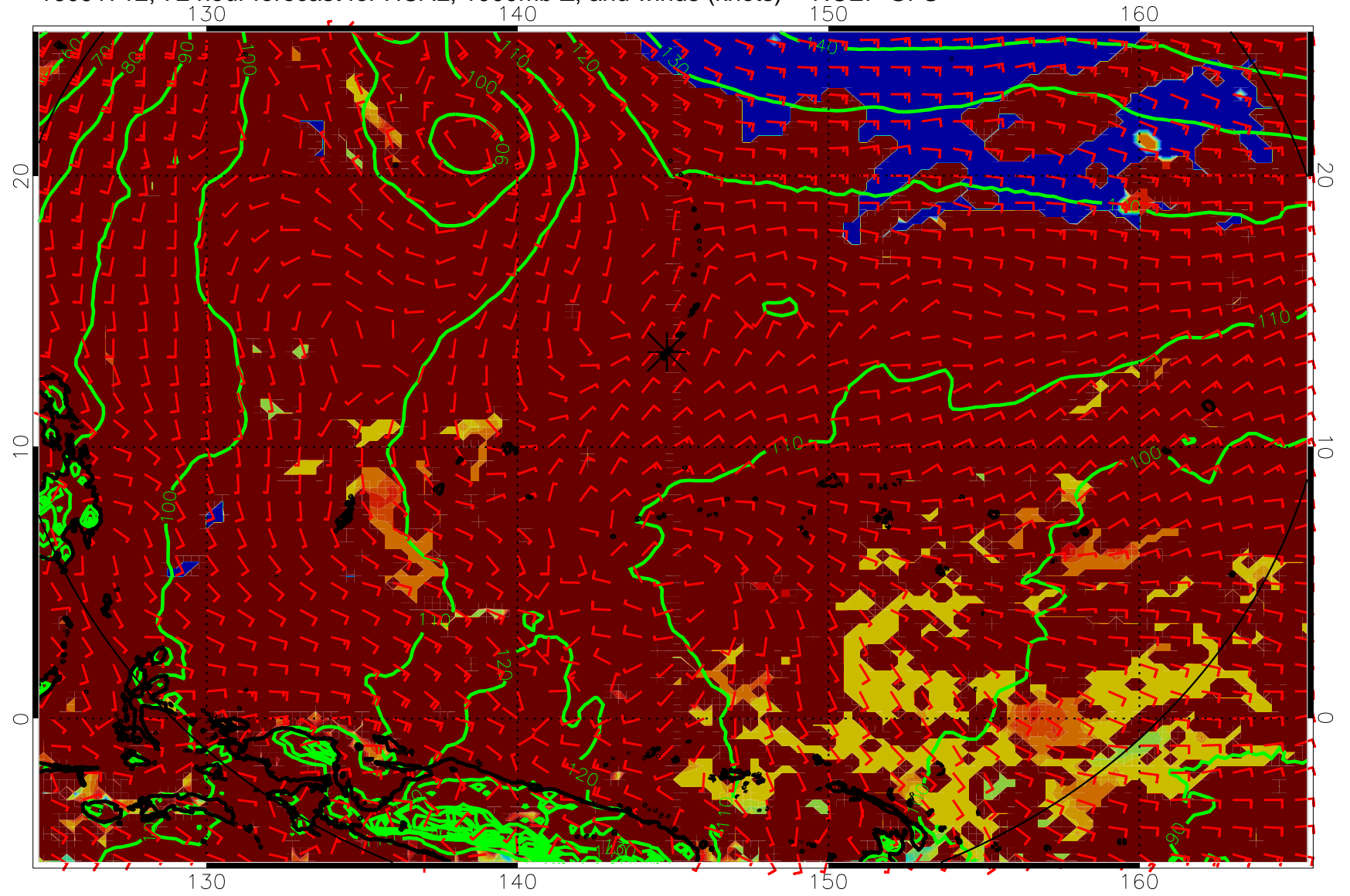
16091712, 72 hour forecast for HCAL, 1000mb Z, and winds (knots) -- NCEP GFS
