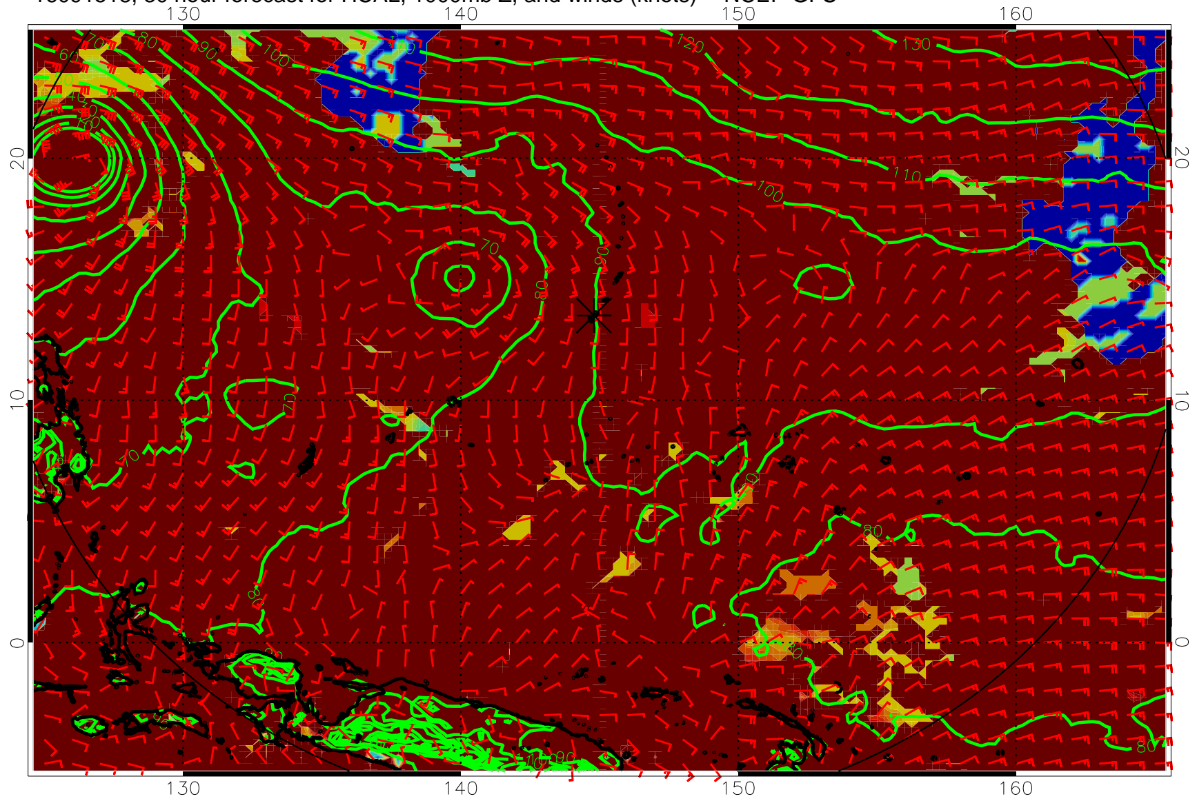
16091518, 30 hour forecast for HCAL, 1000mb Z, and winds (knots) -- NCEP GFS
