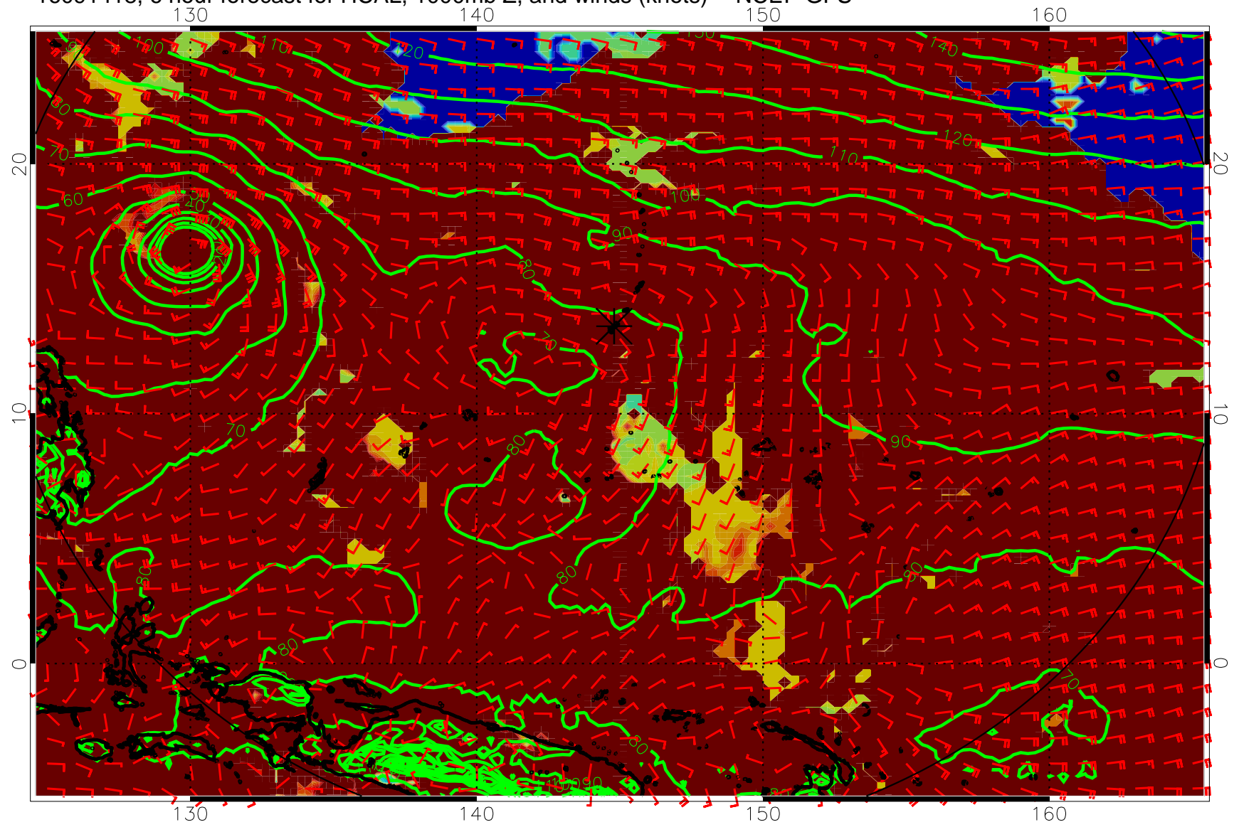
16091418, 6 hour forecast for HCAL, 1000mb Z, and winds (knots) -- NCEP GFS
