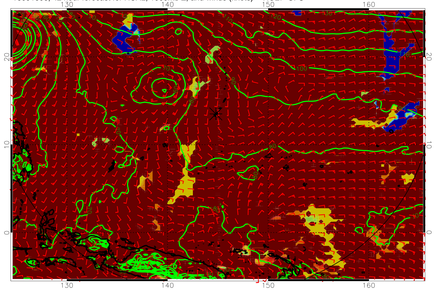
16091606, 42 hour forecast for HCAL, 1000mb Z, and winds (knots) -- NCEP GFS
