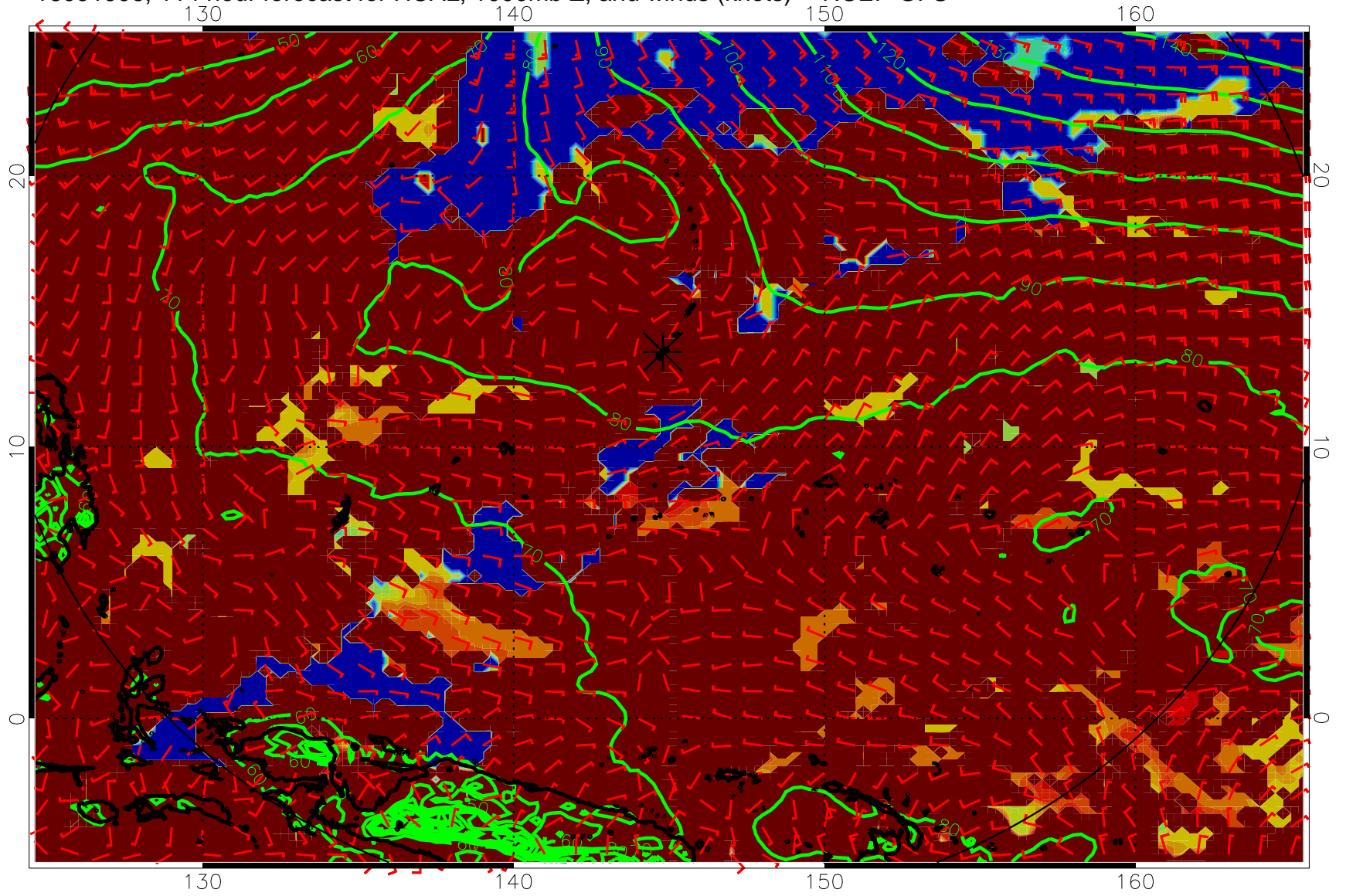
16091906, 114 hour forecast for HCAL, 1000mb Z, and winds (knots) -- NCEP GFS
