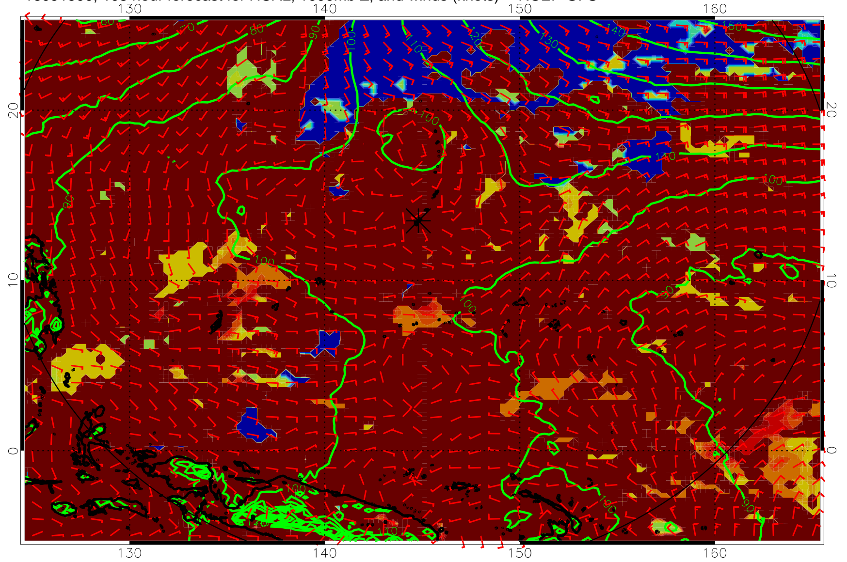
16091900, 108 hour forecast for HCAL, 1000mb Z, and winds (knots) -- NCEP GFS
