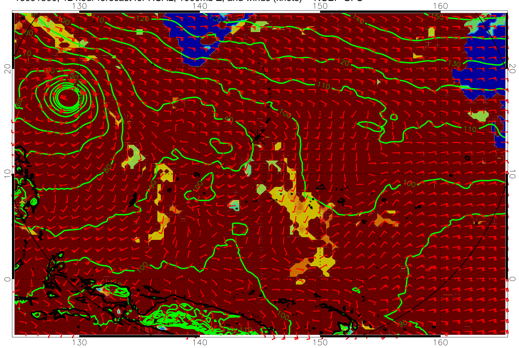
16091500, 12 hour forecast for HCAL, 1000mb Z, and winds (knots) -- NCEP GFS
