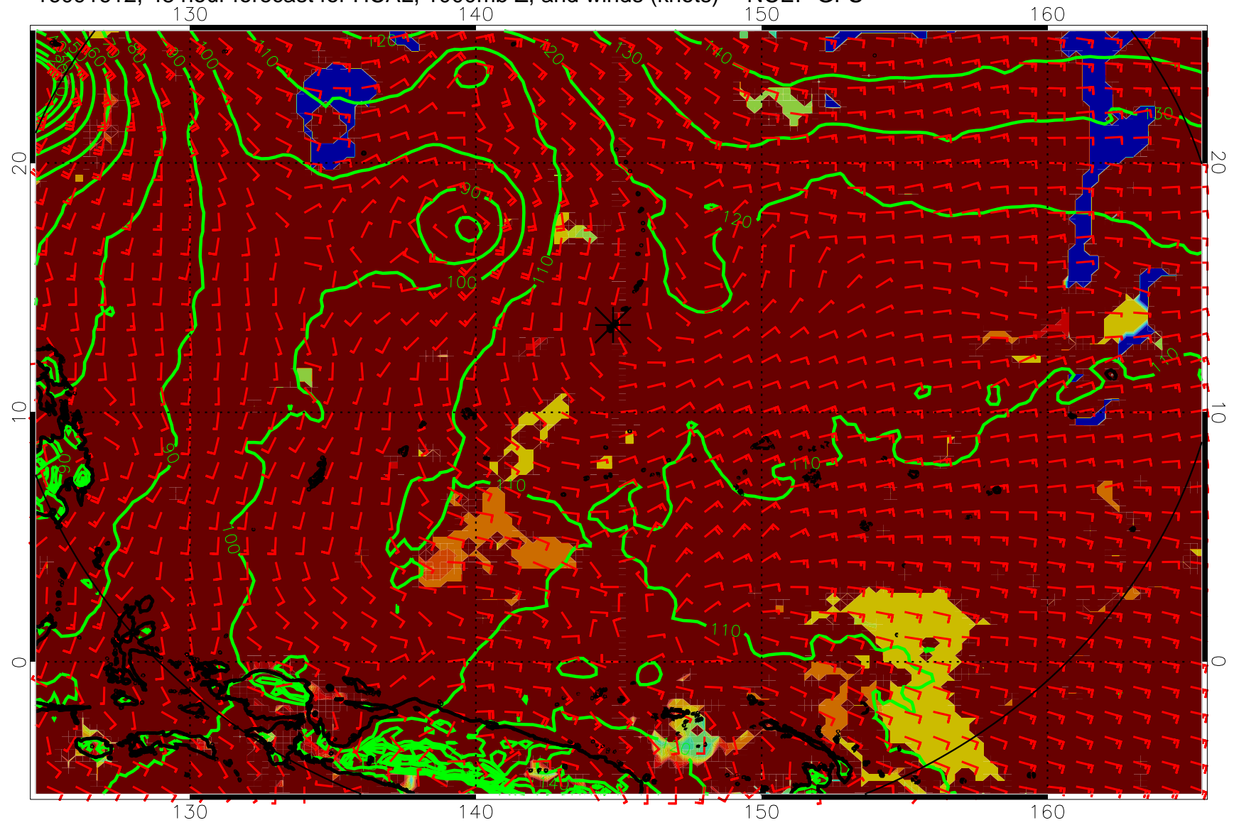
16091612, 48 hour forecast for HCAL, 1000mb Z, and winds (knots) -- NCEP GFS
