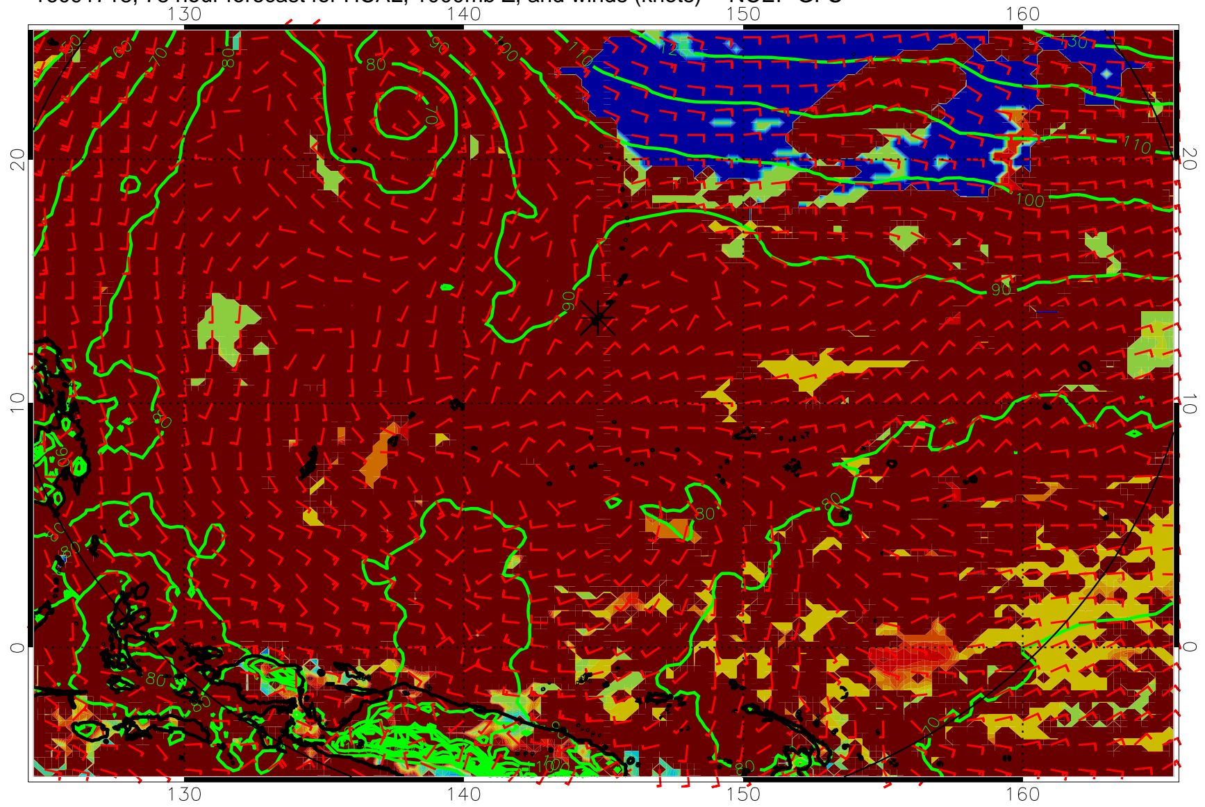
16091718, 78 hour forecast for HCAL, 1000mb Z, and winds (knots) -- NCEP GFS
