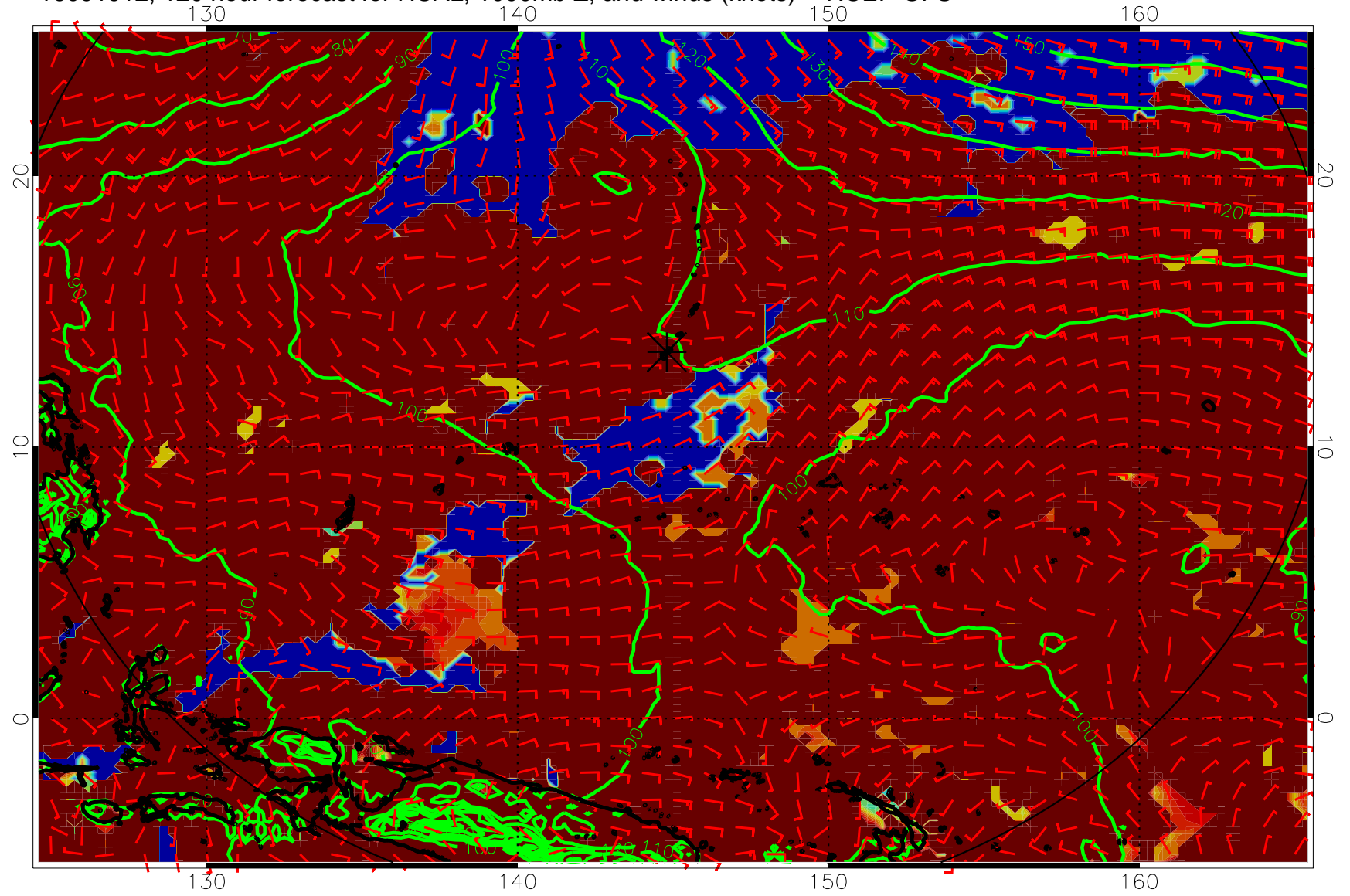
16091912, 120 hour forecast for HCAL, 1000mb Z, and winds (knots) -- NCEP GFS
