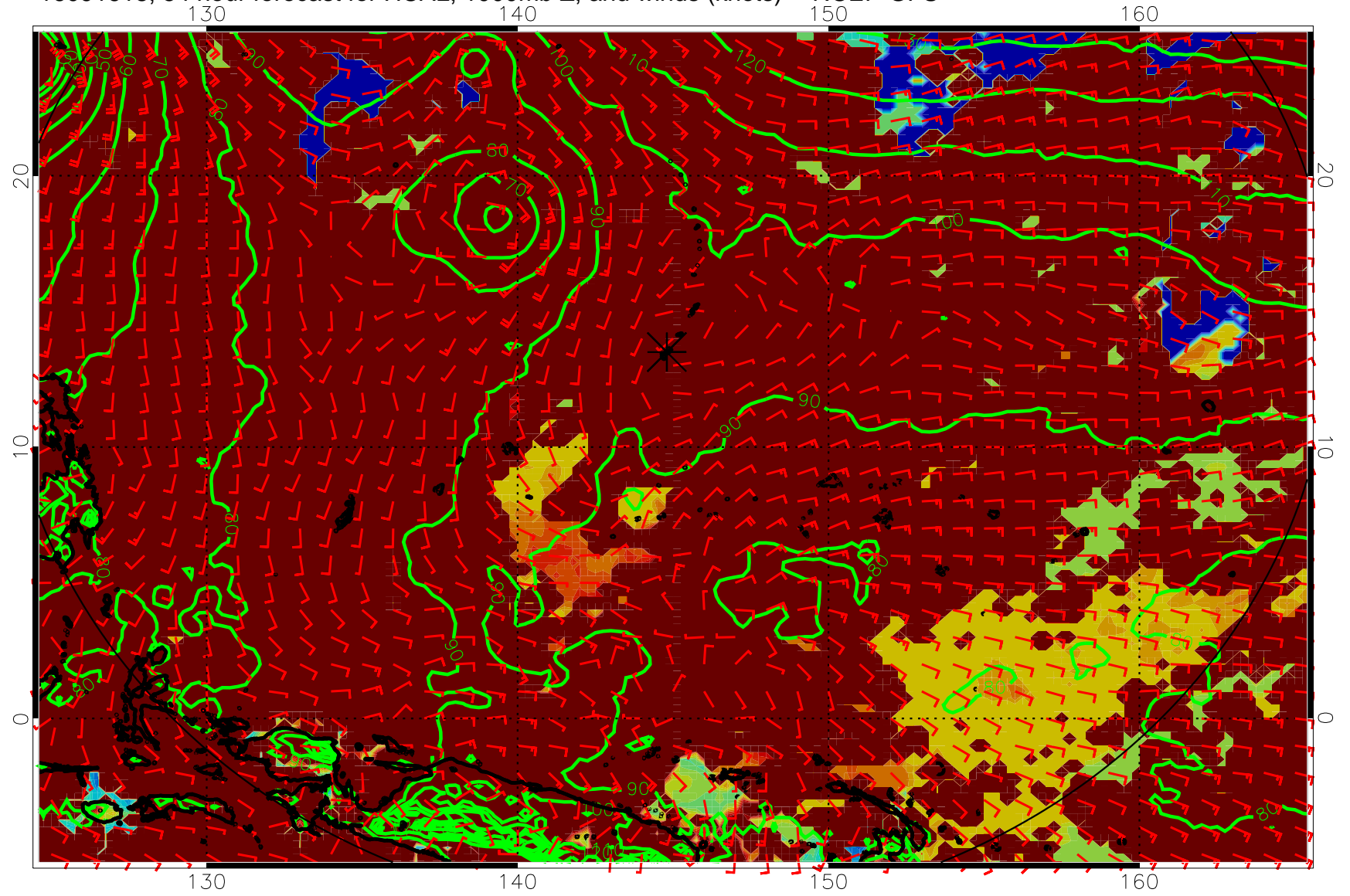
16091618, 54 hour forecast for HCAL, 1000mb Z, and winds (knots) -- NCEP GFS
