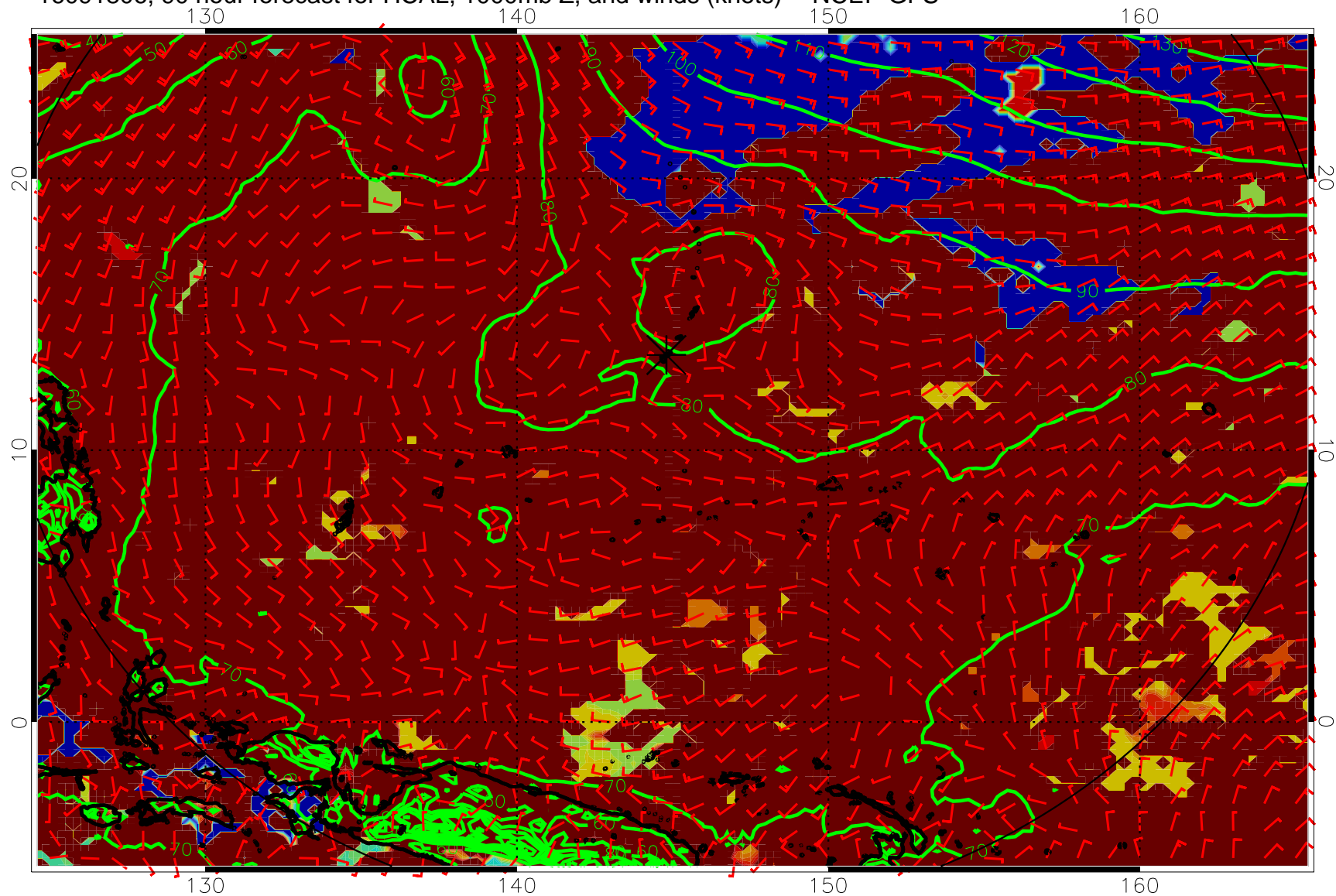
16091806, 90 hour forecast for HCAL, 1000mb Z, and winds (knots) -- NCEP GFS
