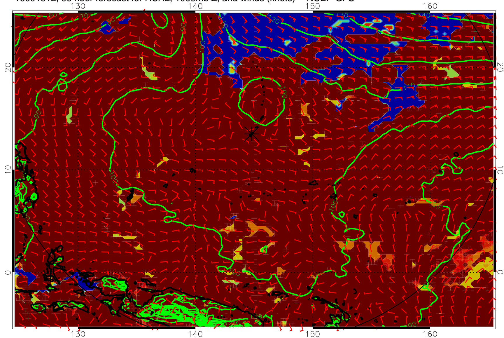
16091812, 96 hour forecast for HCAL, 1000mb Z, and winds (knots) -- NCEP GFS
