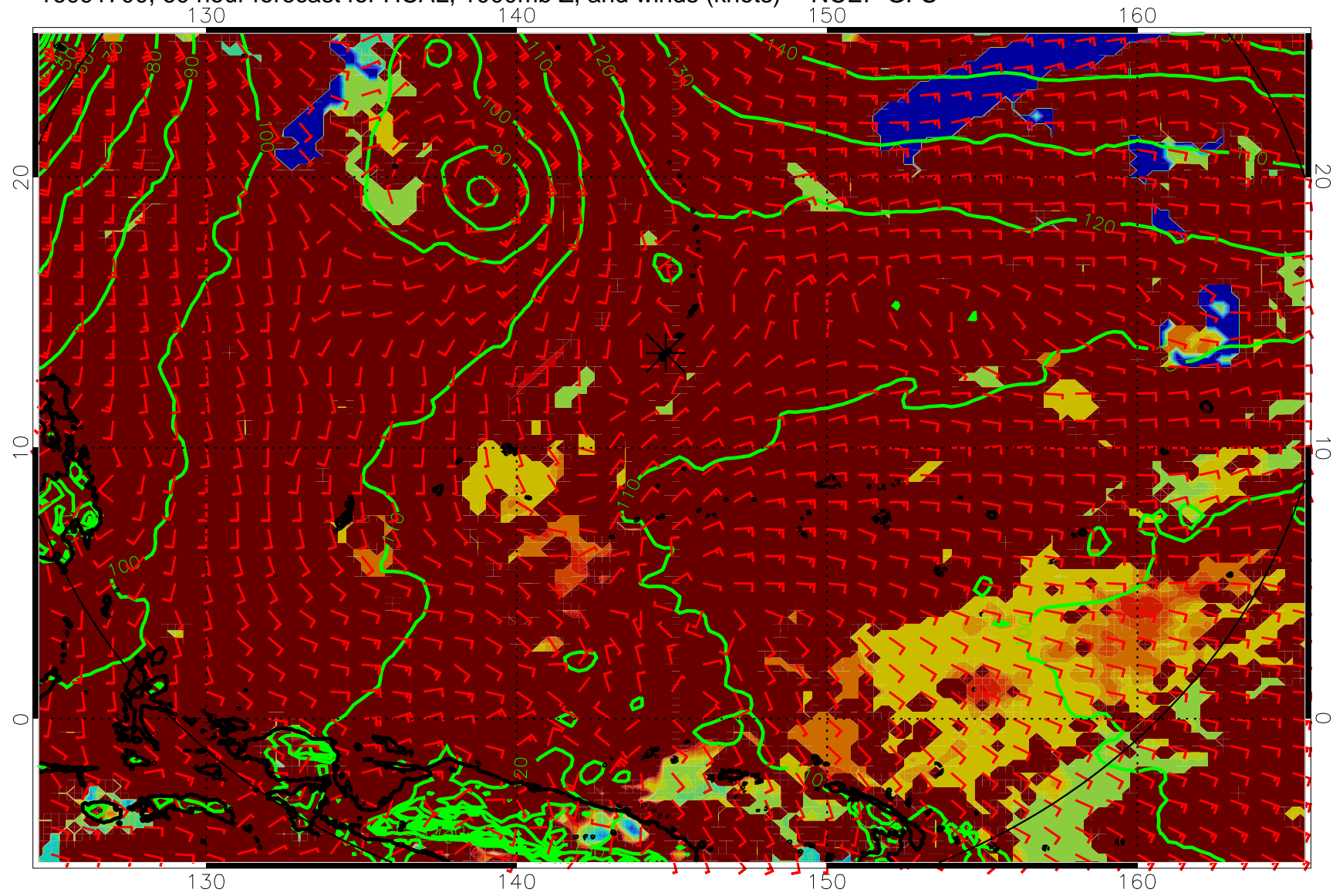
16091700, 60 hour forecast for HCAL, 1000mb Z, and winds (knots) -- NCEP GFS
