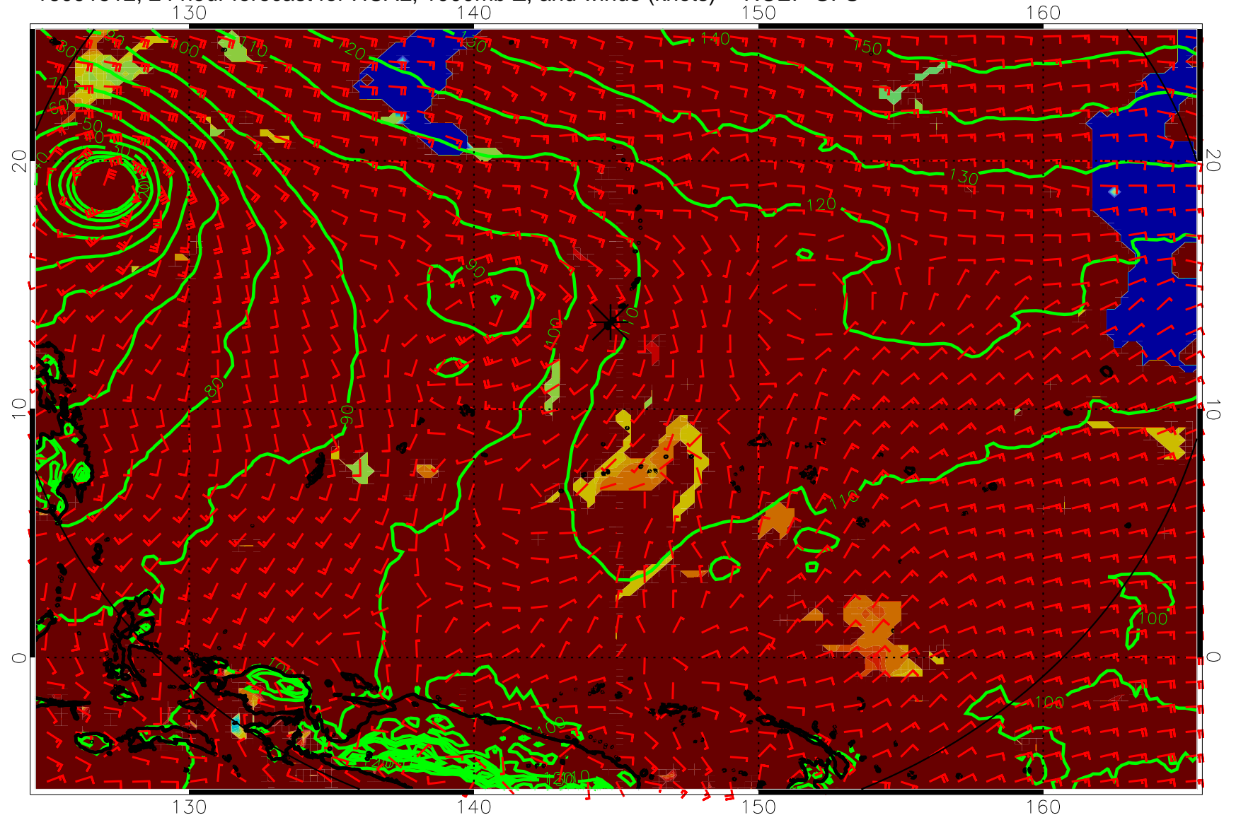
16091512, 24 hour forecast for HCAL, 1000mb Z, and winds (knots) -- NCEP GFS
