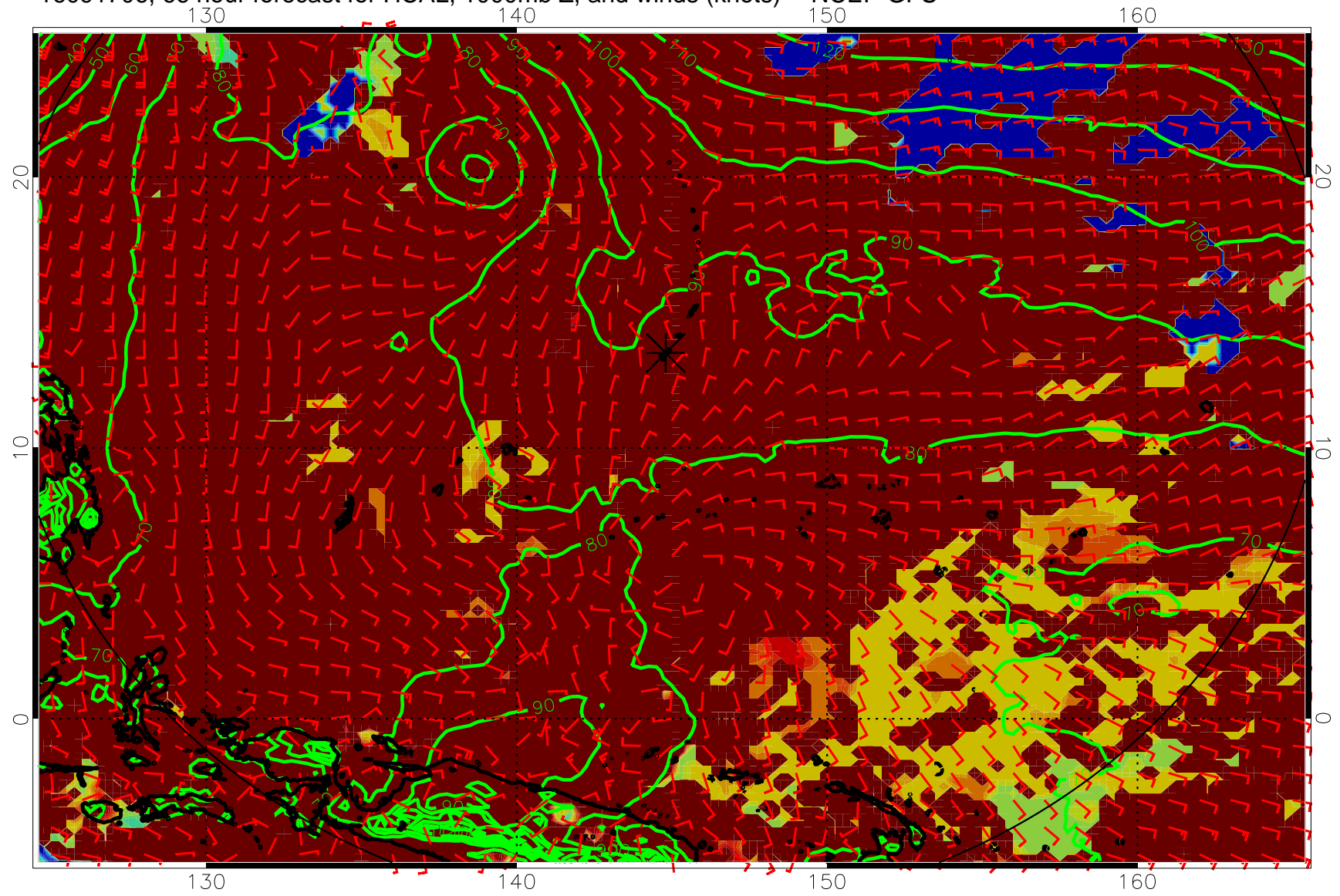
16091706, 66 hour forecast for HCAL, 1000mb Z, and winds (knots) -- NCEP GFS
