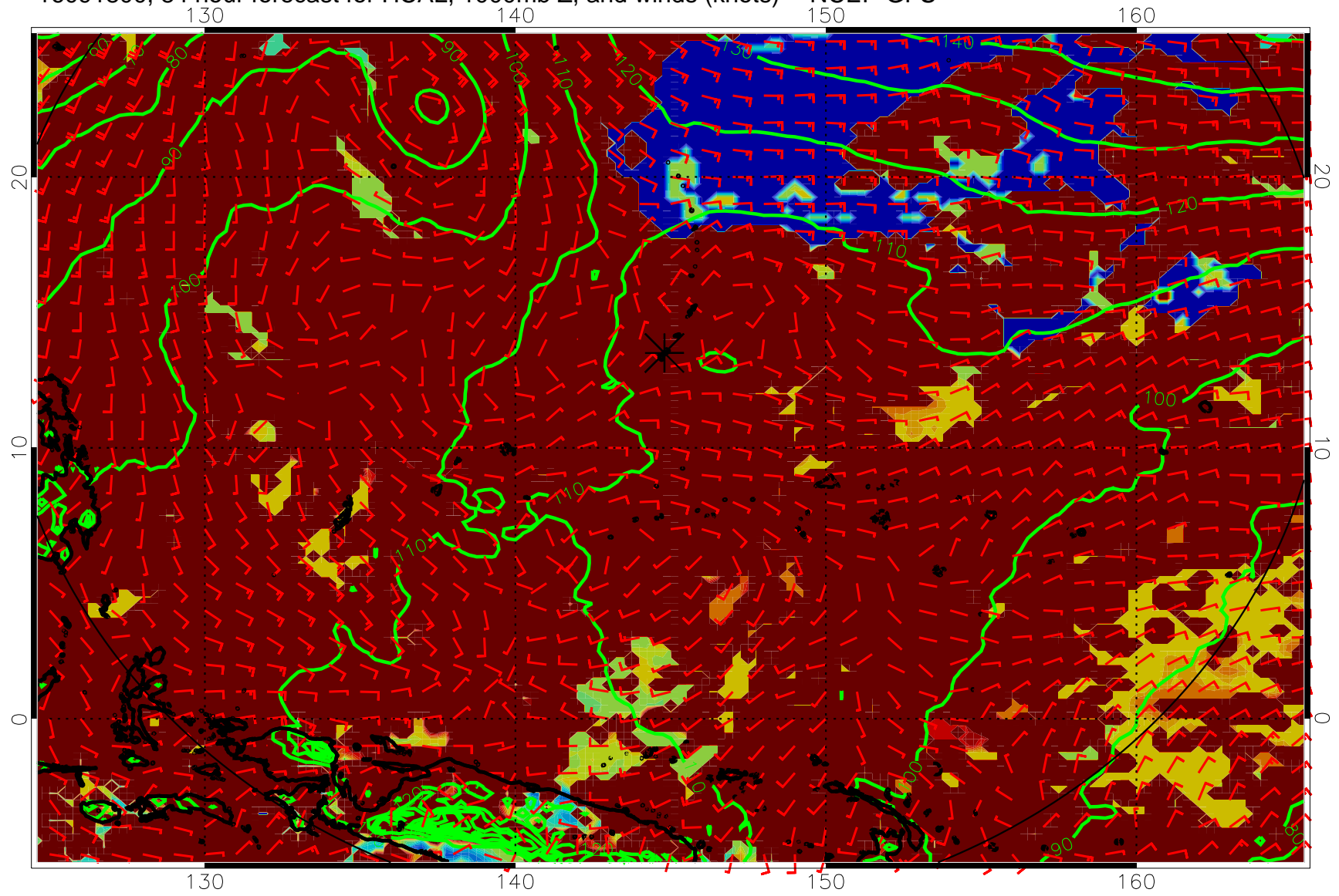
16091800, 84 hour forecast for HCAL, 1000mb Z, and winds (knots) -- NCEP GFS
