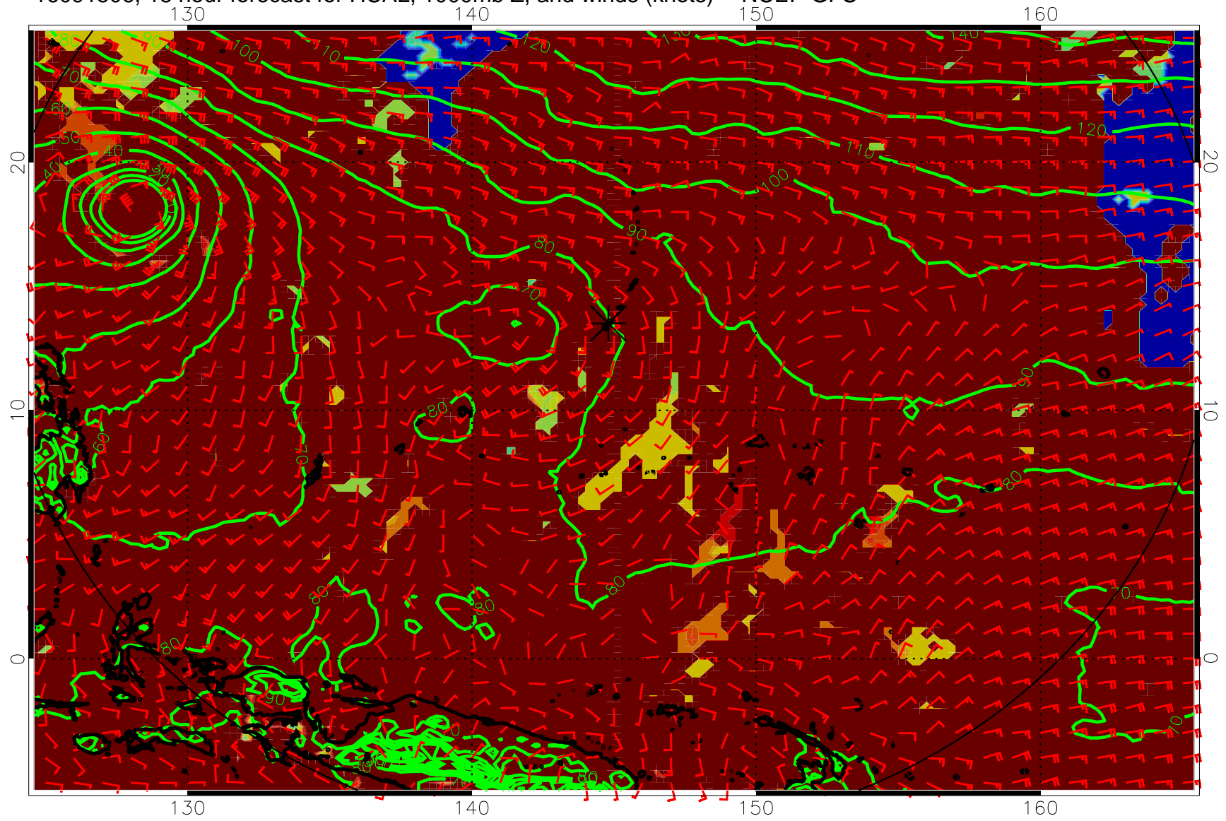
16091506, 18 hour forecast for HCAL, 1000mb Z, and winds (knots) -- NCEP GFS
