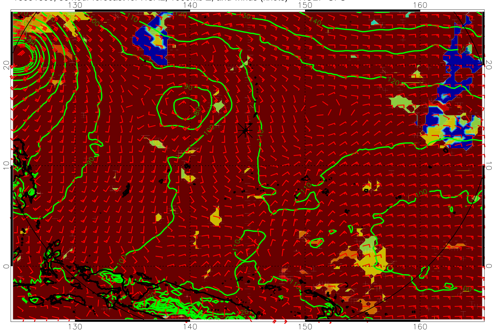
16091600, 36 hour forecast for HCAL, 1000mb Z, and winds (knots) -- NCEP GFS
