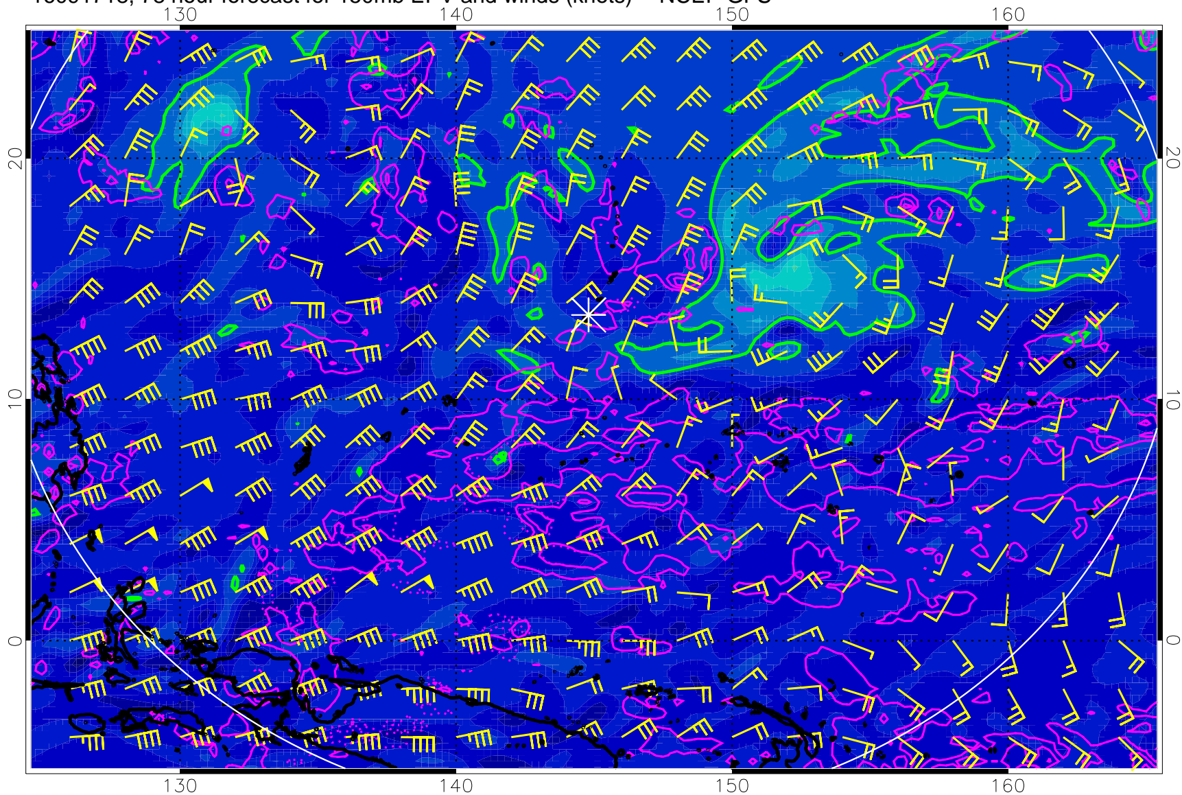
16091718, 78 hour forecast for 150mb EPV and winds (knots) -- NCEP GFS
