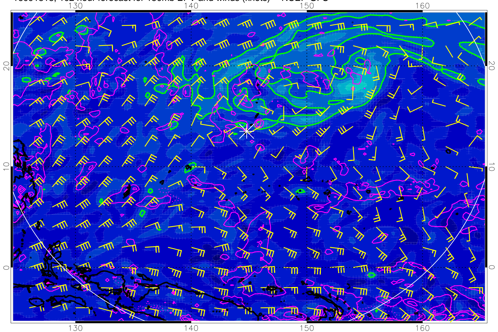
16091818, 102 hour forecast for 150mb EPV and winds (knots) -- NCEP GFS
