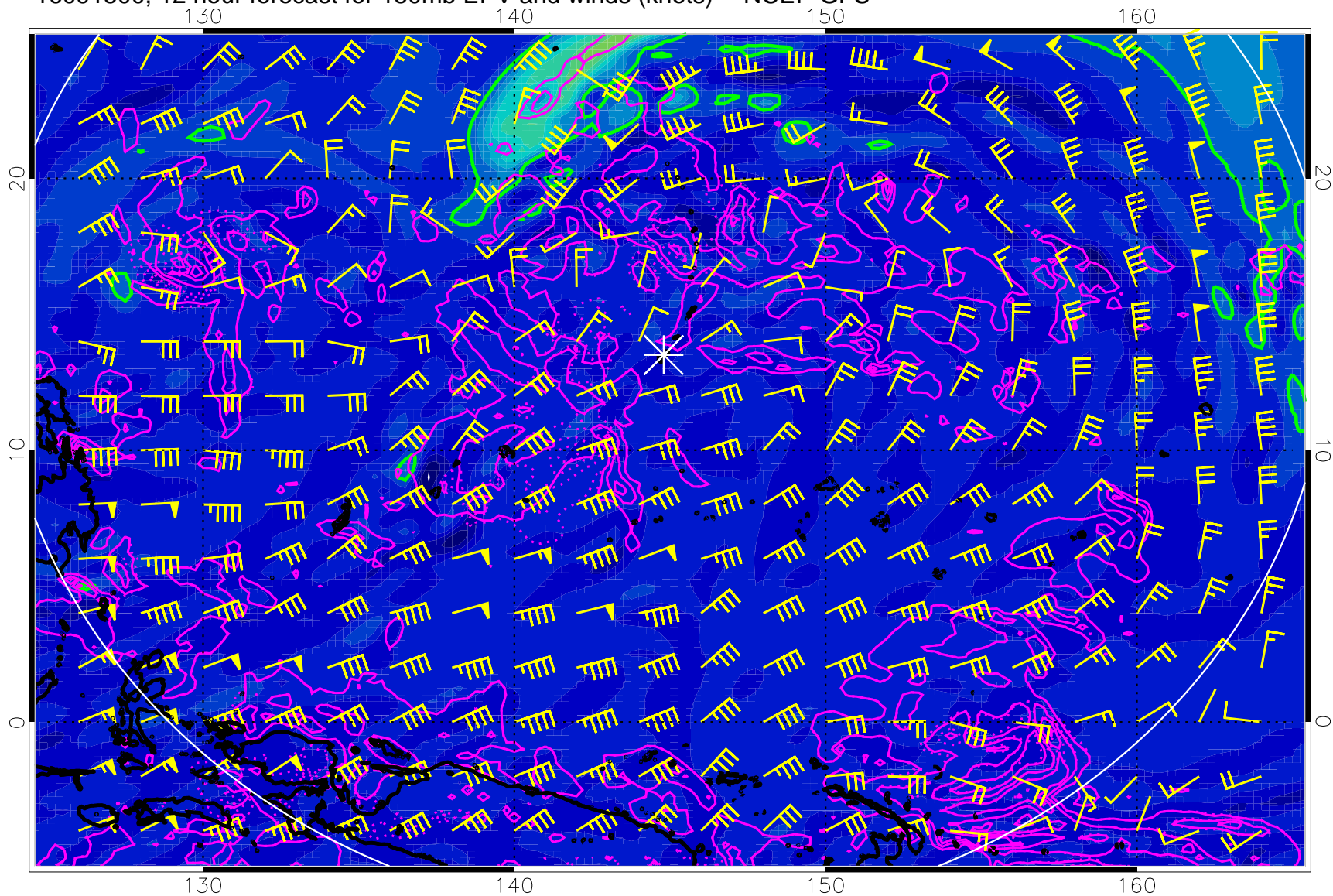
16091500, 12 hour forecast for 150mb EPV and winds (knots) -- NCEP GFS
