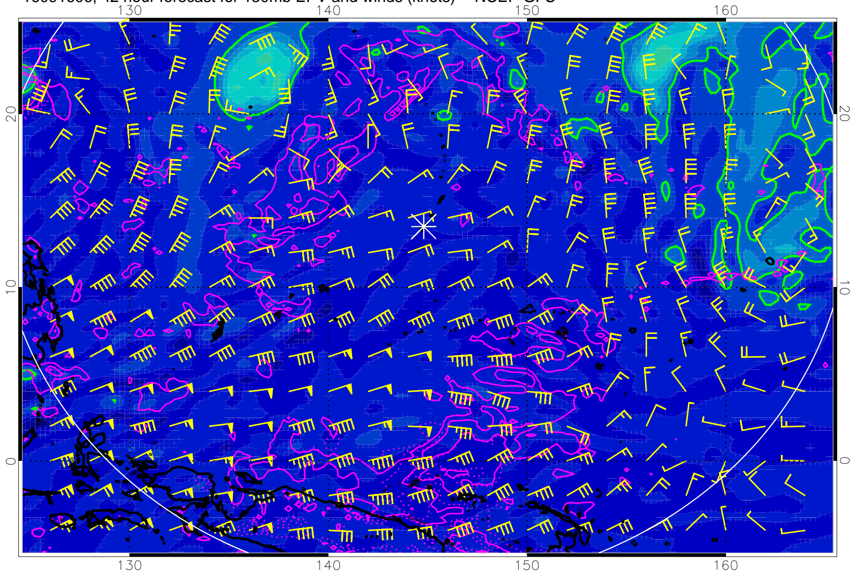
16091606, 42 hour forecast for 150mb EPV and winds (knots) -- NCEP GFS
