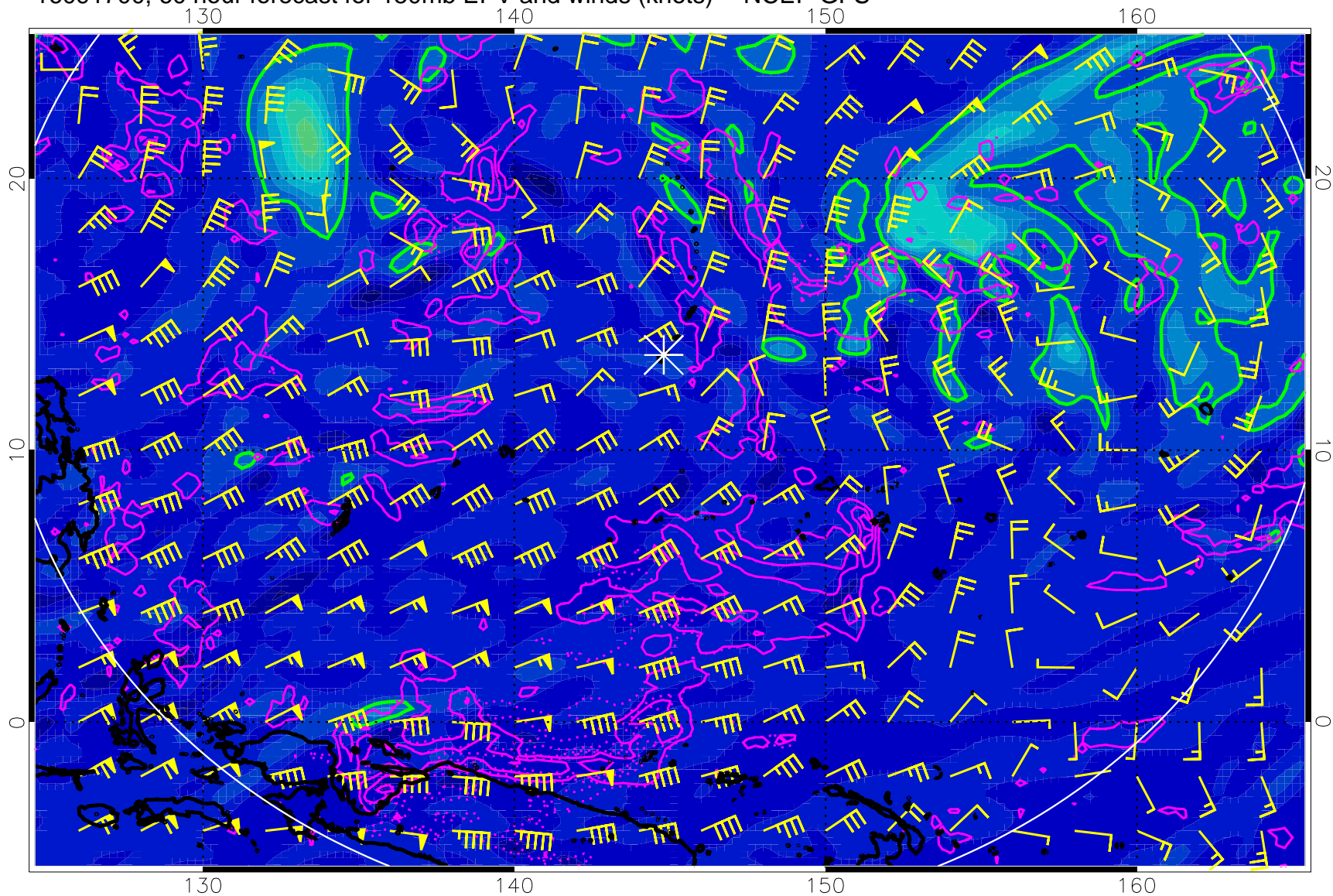
16091700, 60 hour forecast for 150mb EPV and winds (knots) -- NCEP GFS
