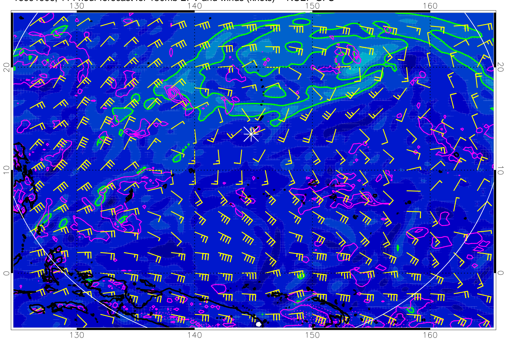
16091906, 114 hour forecast for 150mb EPV and winds (knots) -- NCEP GFS
