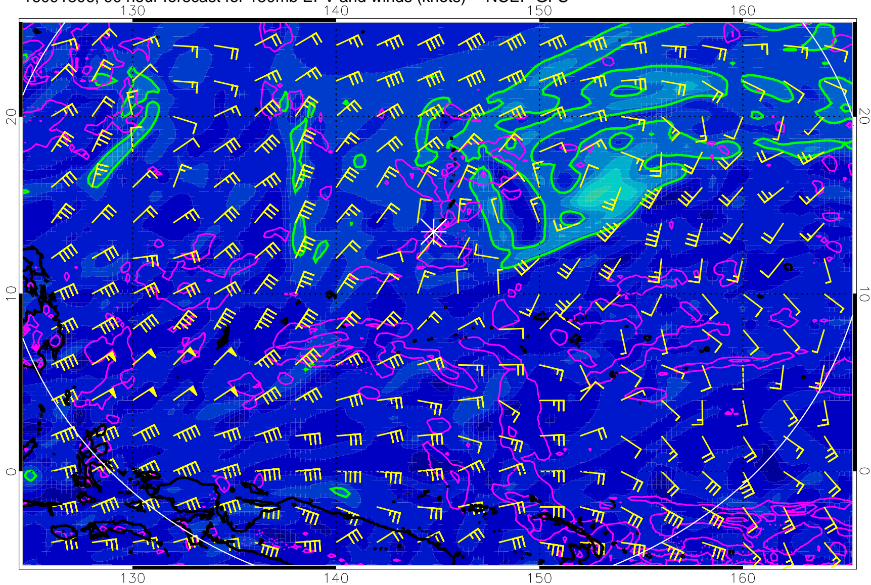
16091806, 90 hour forecast for 150mb EPV and winds (knots) -- NCEP GFS
