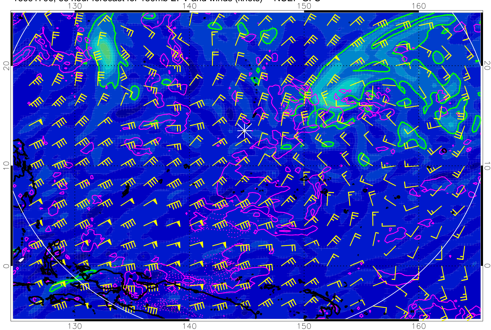
16091706, 66 hour forecast for 150mb EPV and winds (knots) -- NCEP GFS
