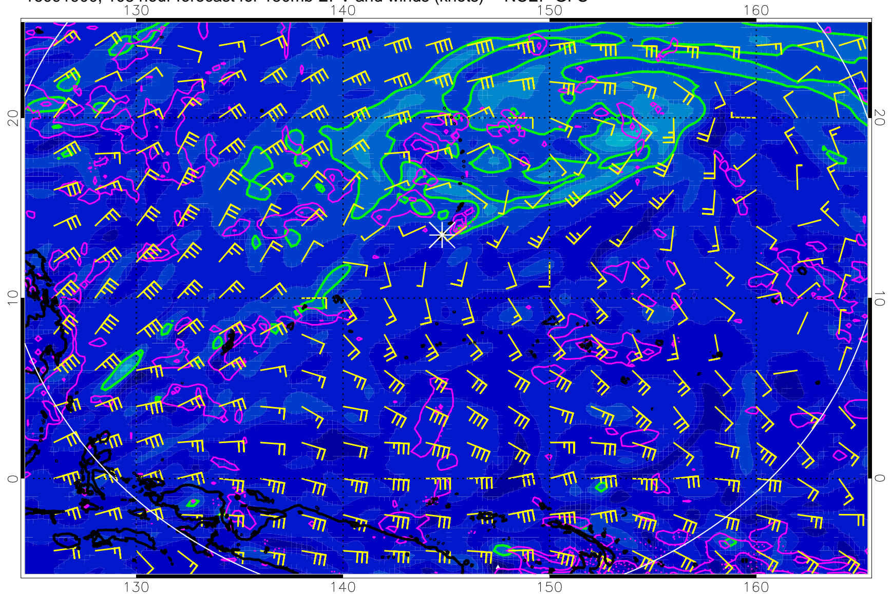
16091900, 108 hour forecast for 150mb EPV and winds (knots) -- NCEP GFS
