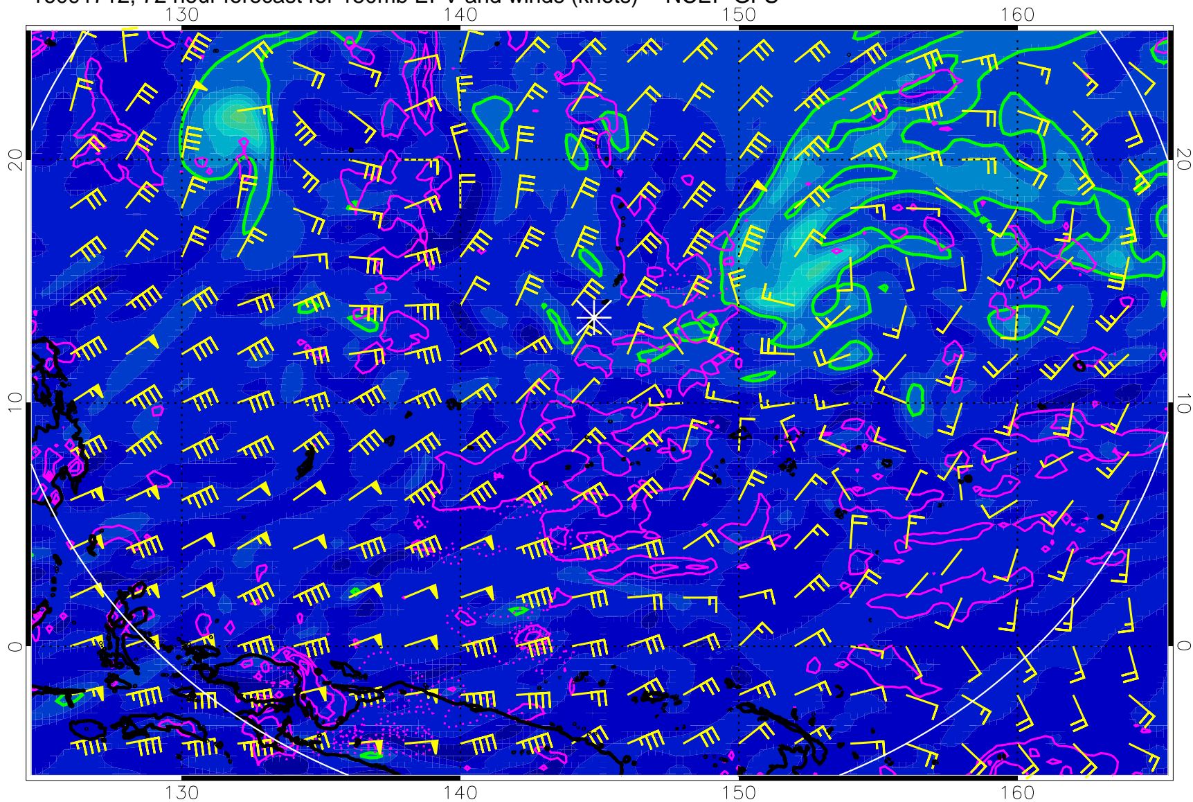
16091712, 72 hour forecast for 150mb EPV and winds (knots) -- NCEP GFS
