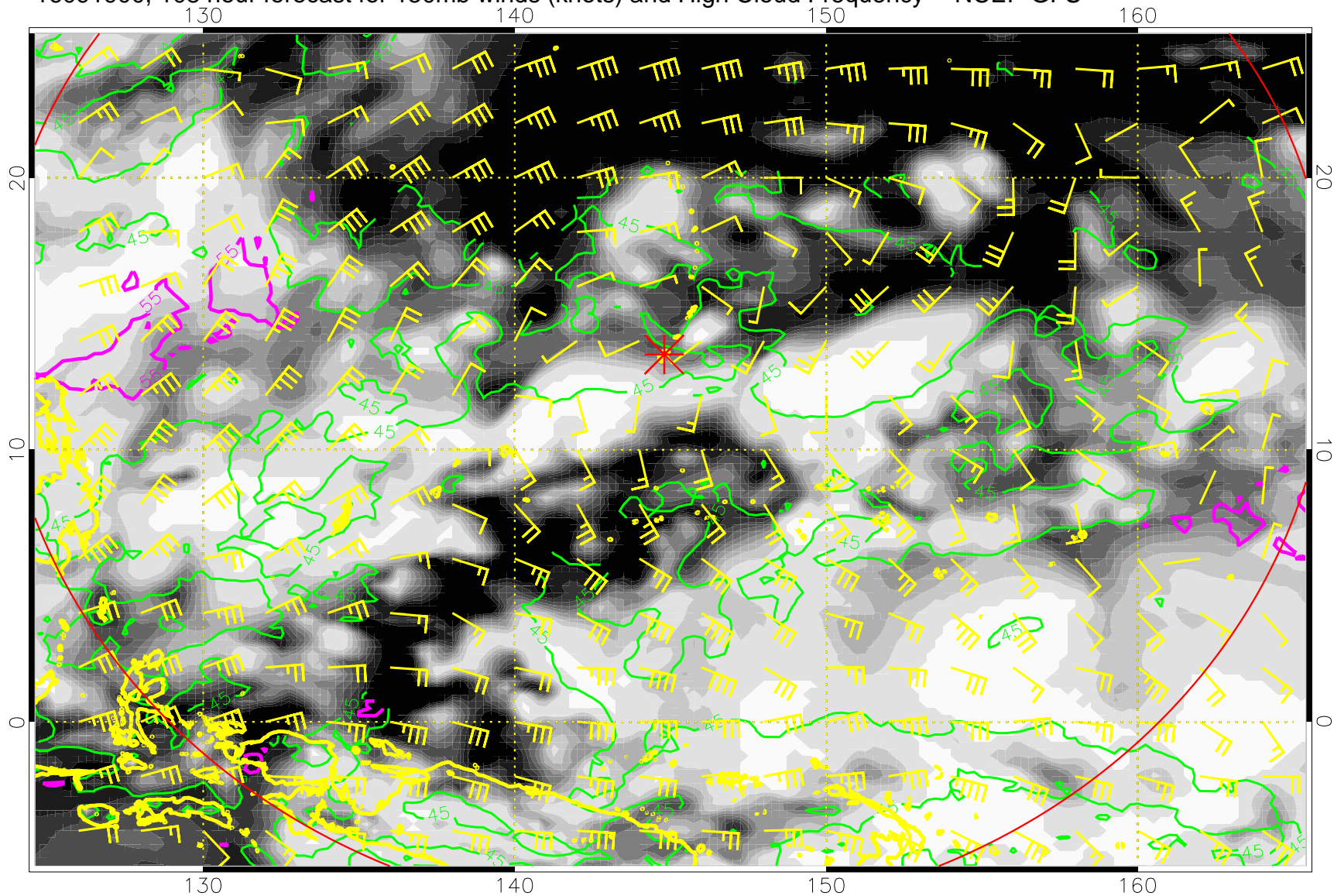
16091900, 108 hour forecast for 150mb winds (knots) and High Cloud Frequency -- NCEP GFS
