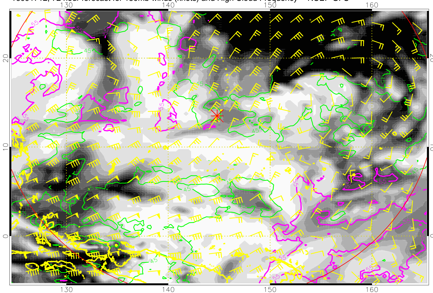
16091712, 72 hour forecast for 150mb winds (knots) and High Cloud Frequency -- NCEP GFS
