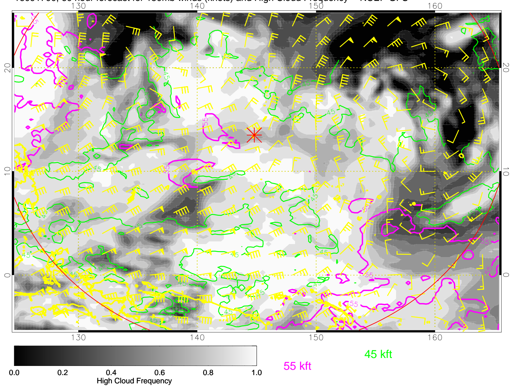
16091700, 60 hour forecast for 150mb winds (knots) and High Cloud Frequency -- NCEP GFS
