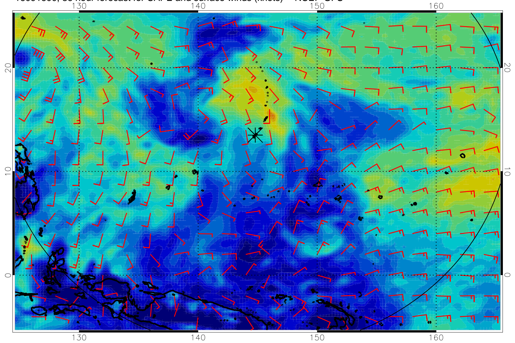
16091600, 36 hour forecast for CAPE and surface winds (knots) -- NCEP GFS
