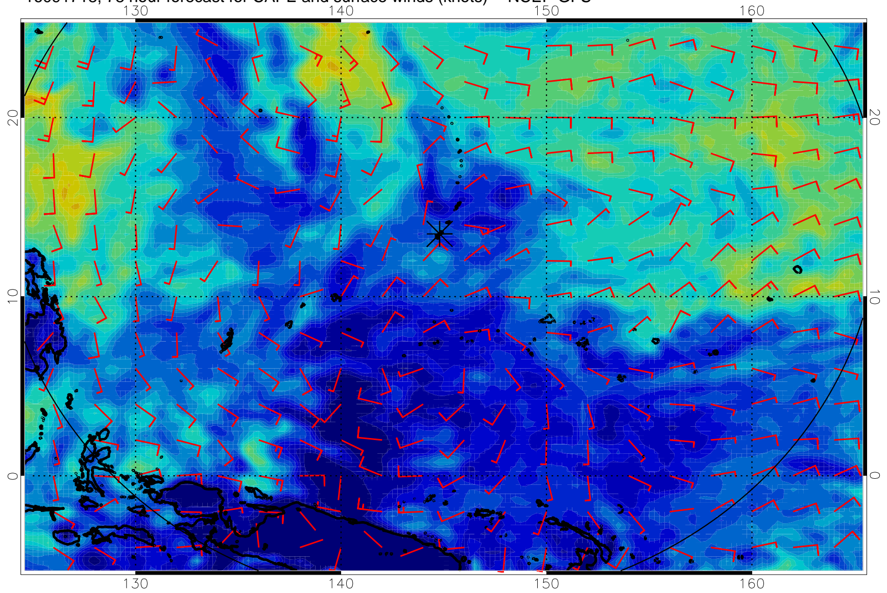
16091718, 78 hour forecast for CAPE and surface winds (knots) -- NCEP GFS
