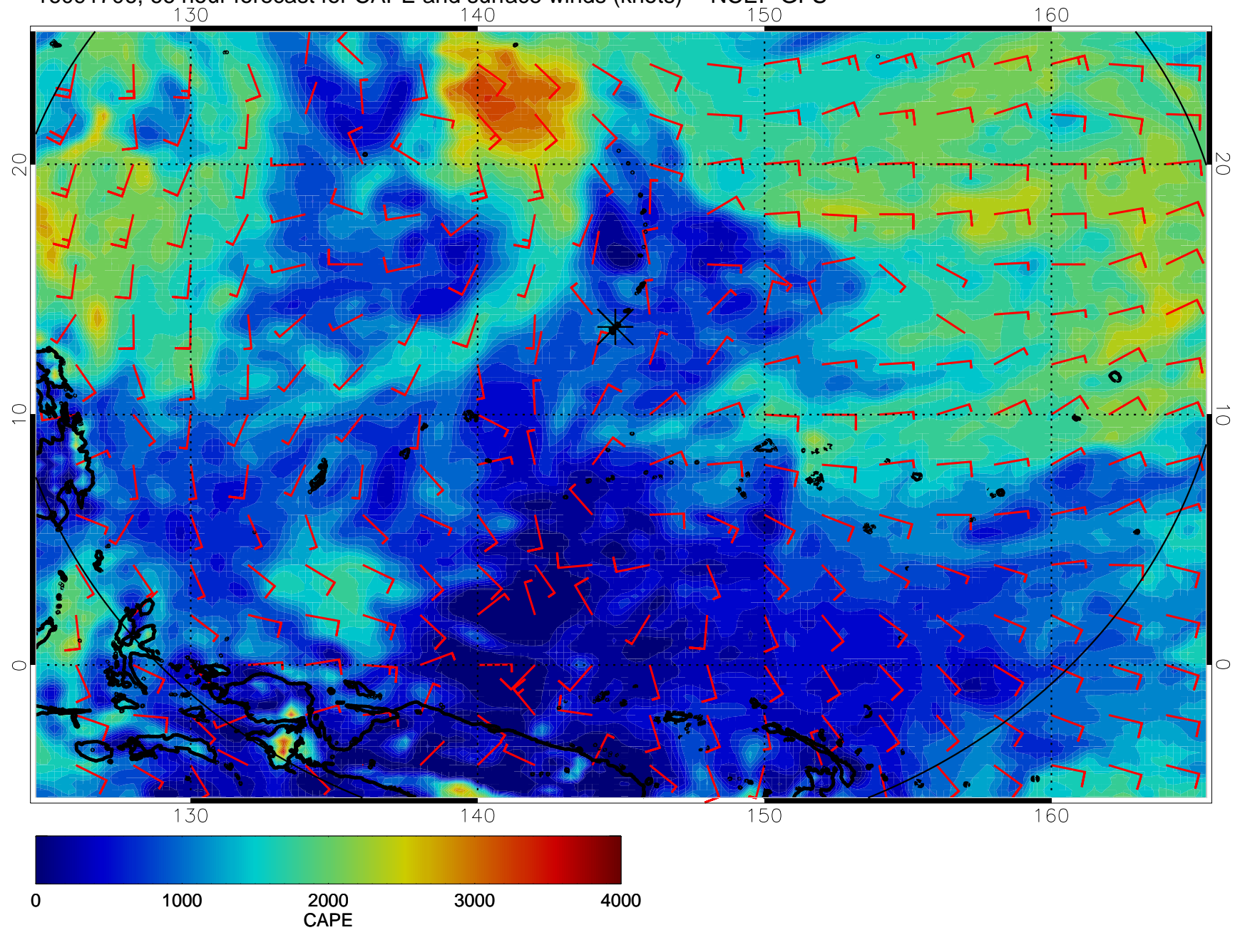
16091706, 66 hour forecast for CAPE and surface winds (knots) -- NCEP GFS
