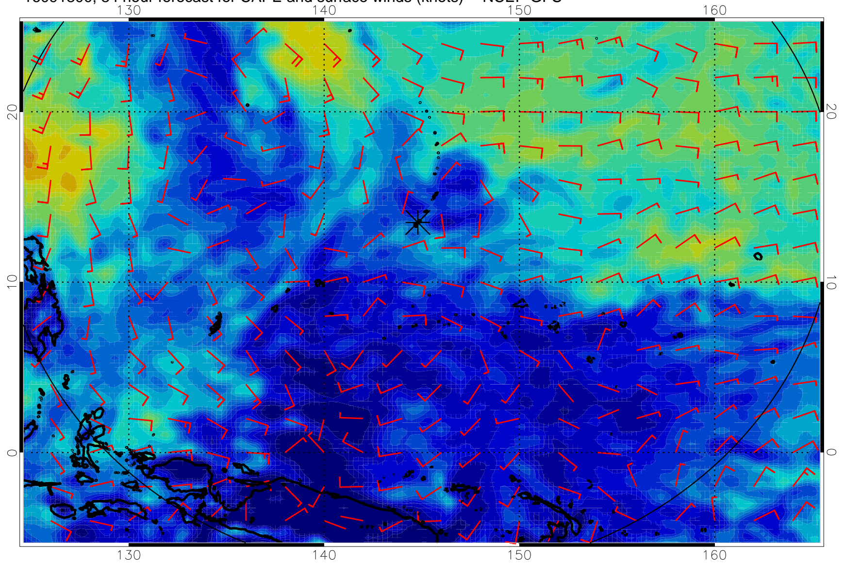
16091800, 84 hour forecast for CAPE and surface winds (knots) -- NCEP GFS
