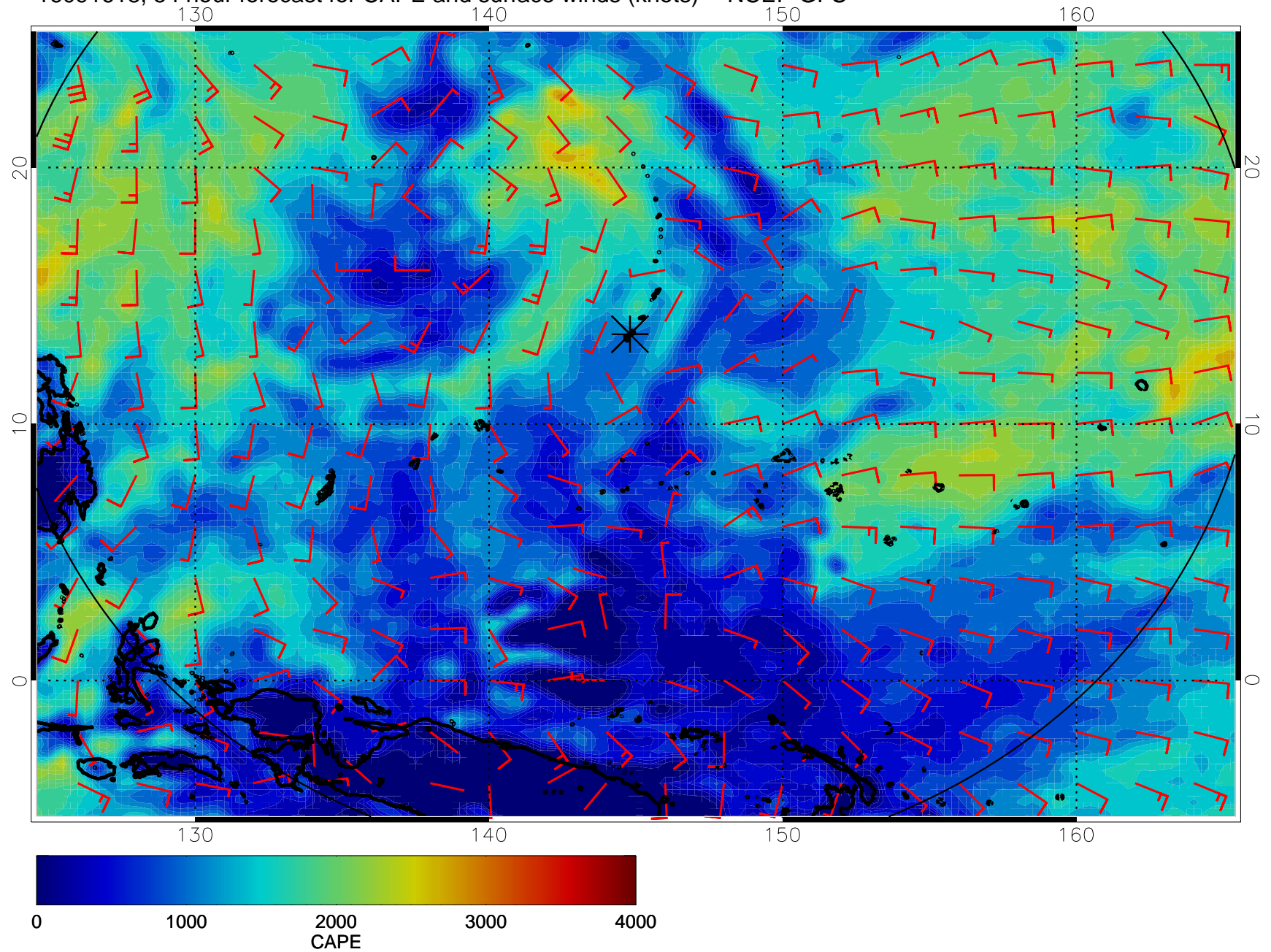
16091618, 54 hour forecast for CAPE and surface winds (knots) -- NCEP GFS
