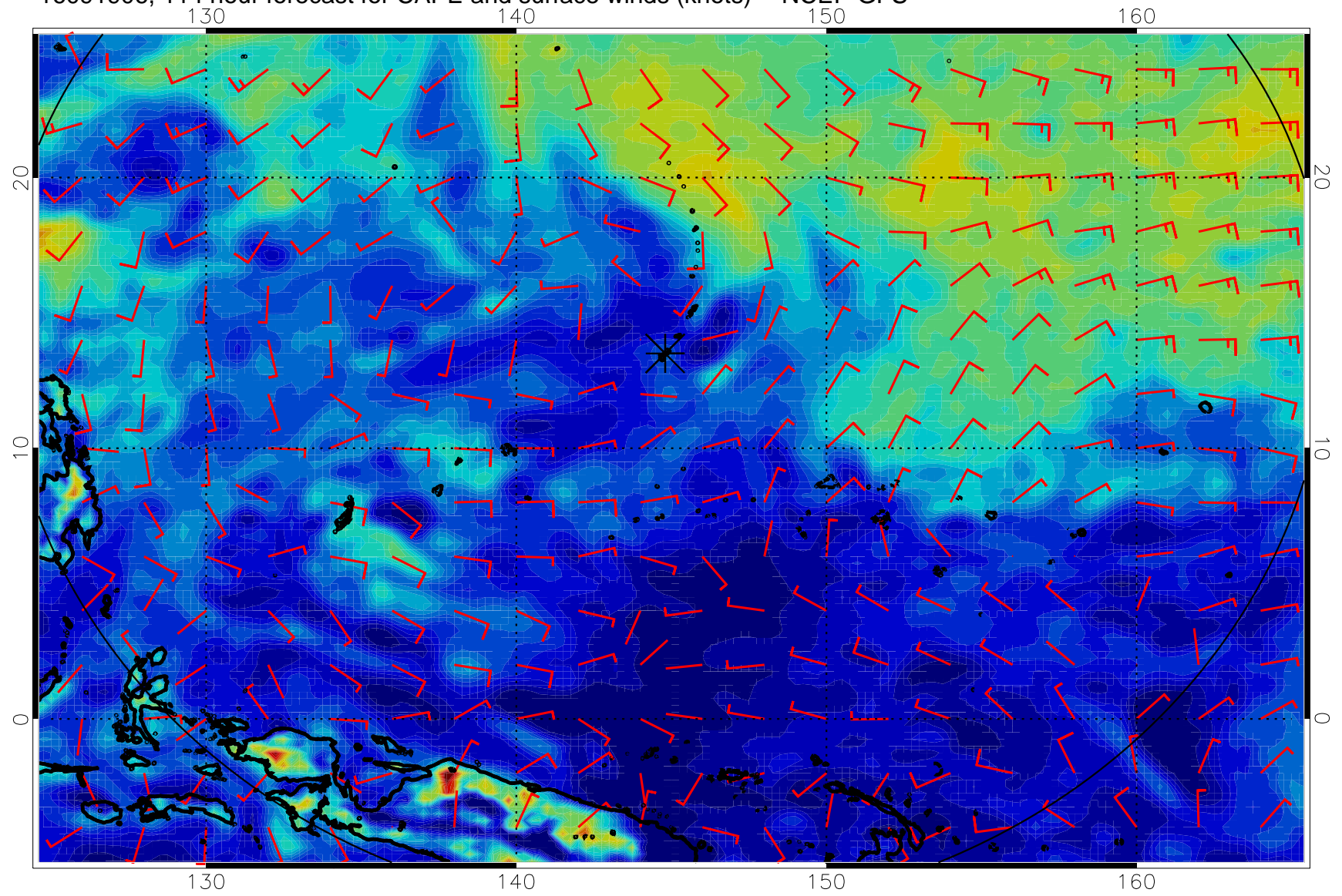
16091906, 114 hour forecast for CAPE and surface winds (knots) -- NCEP GFS
