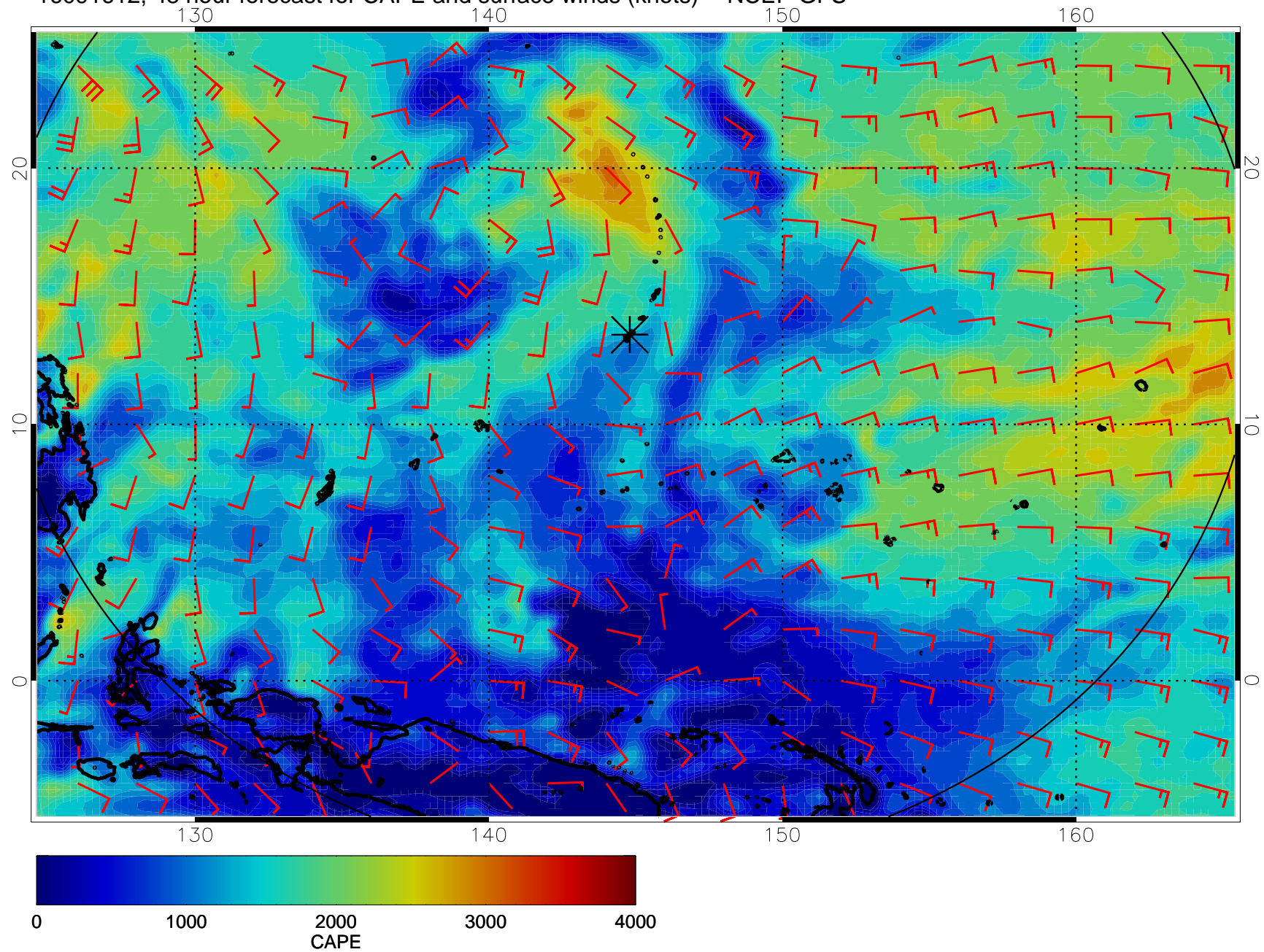
16091612, 48 hour forecast for CAPE and surface winds (knots) -- NCEP GFS
