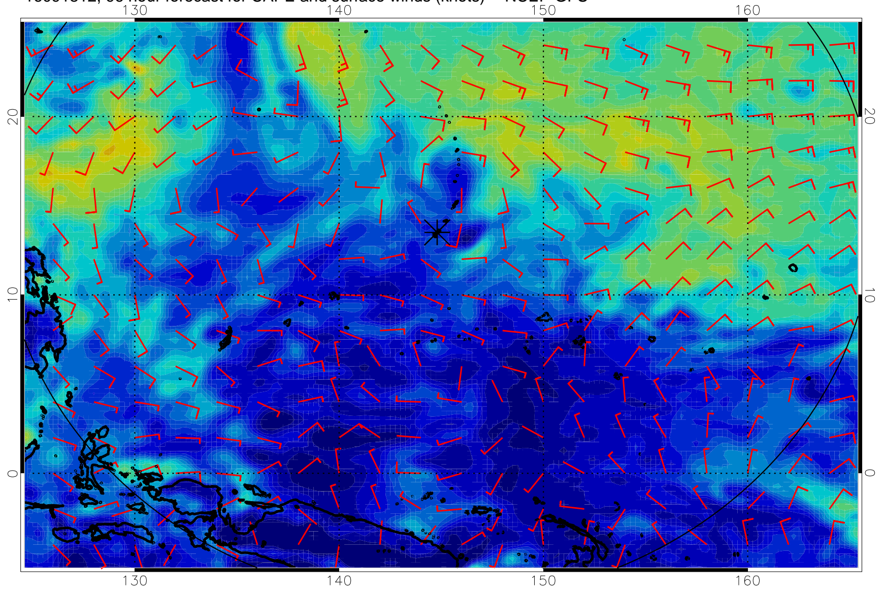
16091812, 96 hour forecast for CAPE and surface winds (knots) -- NCEP GFS
