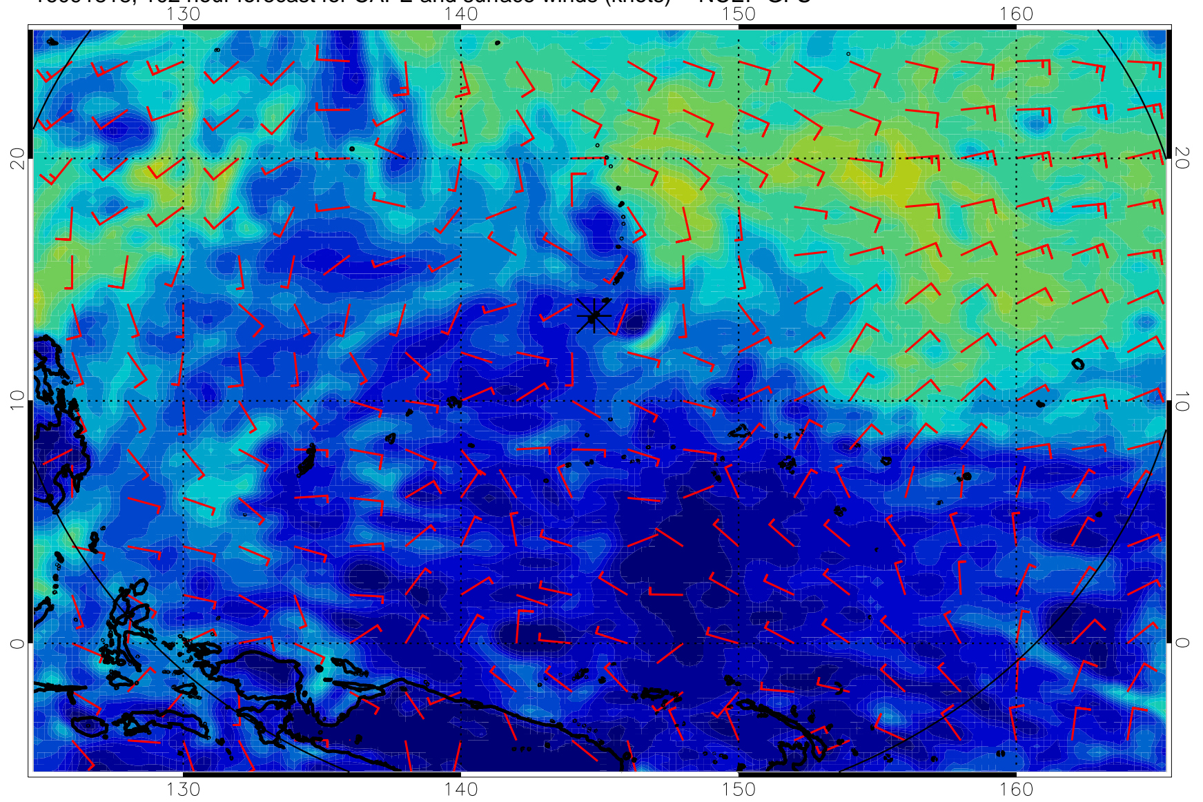
16091818, 102 hour forecast for CAPE and surface winds (knots) -- NCEP GFS
