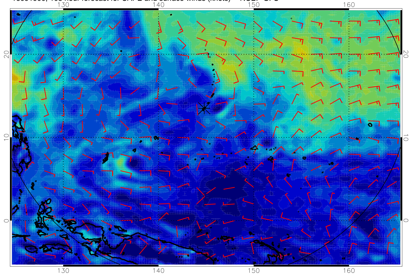
16091900, 108 hour forecast for CAPE and surface winds (knots) -- NCEP GFS
