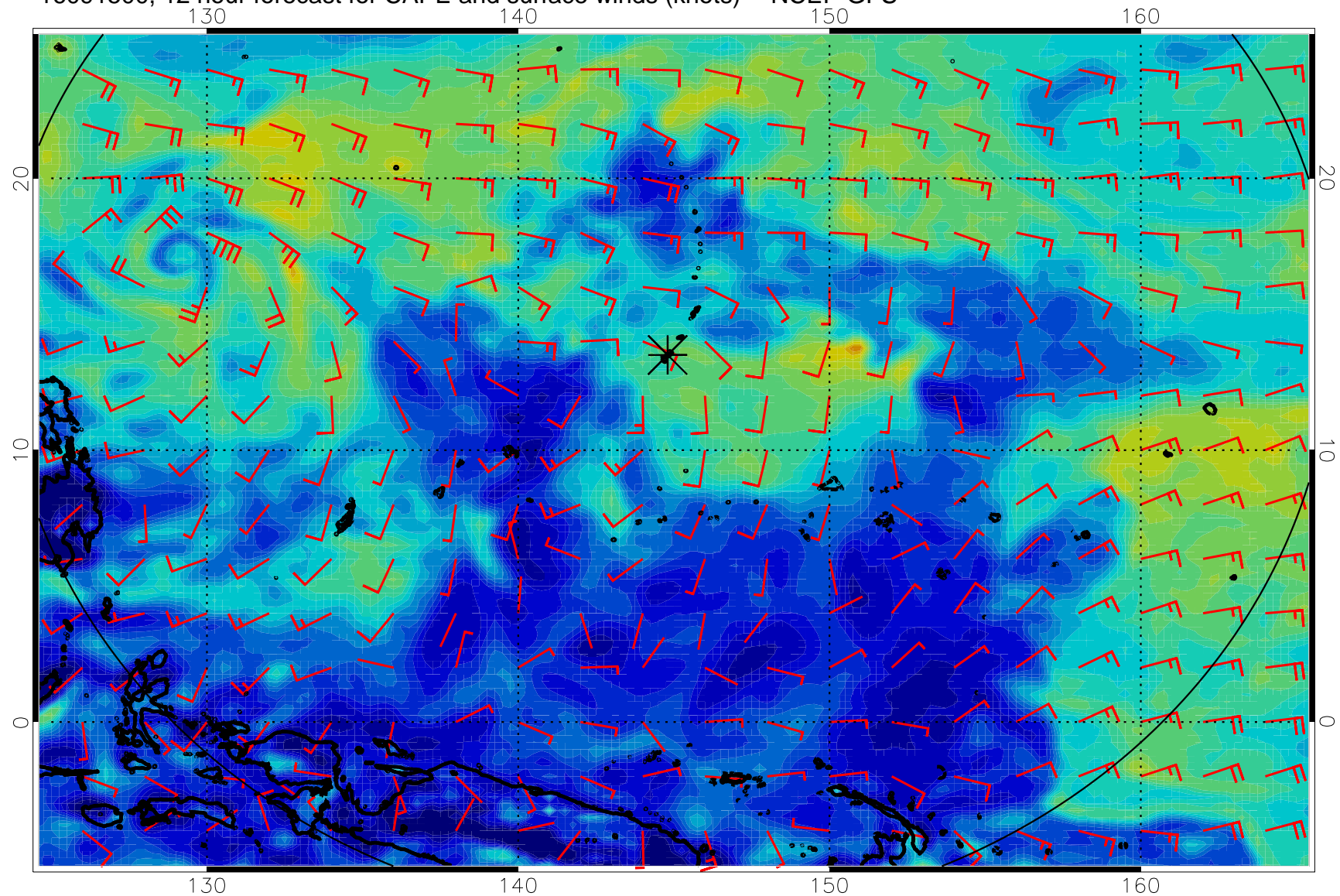
16091500, 12 hour forecast for CAPE and surface winds (knots) -- NCEP GFS
