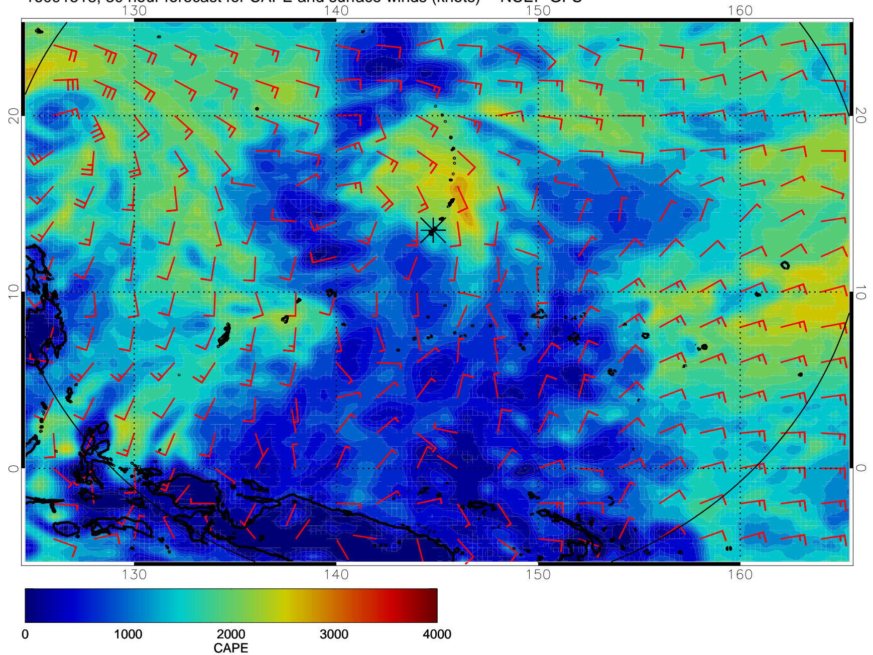
16091518, 30 hour forecast for CAPE and surface winds (knots) -- NCEP GFS
