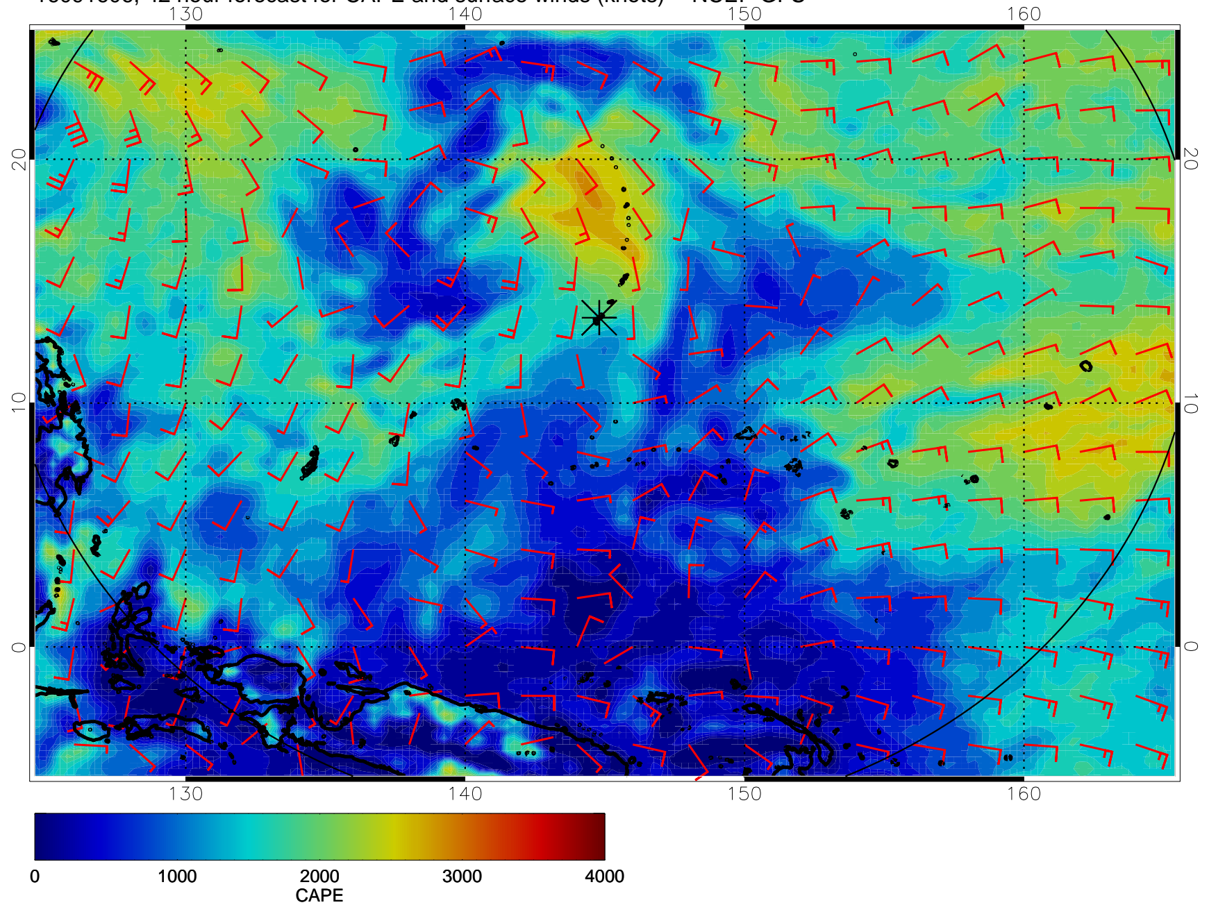
16091606, 42 hour forecast for CAPE and surface winds (knots) -- NCEP GFS
