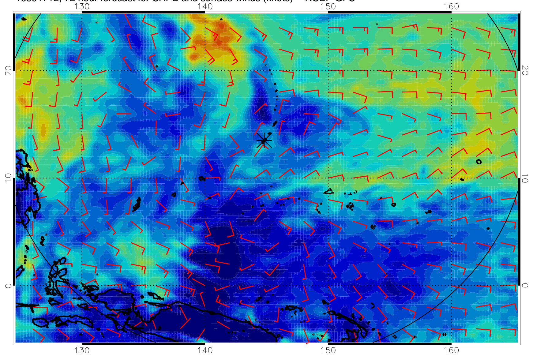
16091712, 72 hour forecast for CAPE and surface winds (knots) -- NCEP GFS
