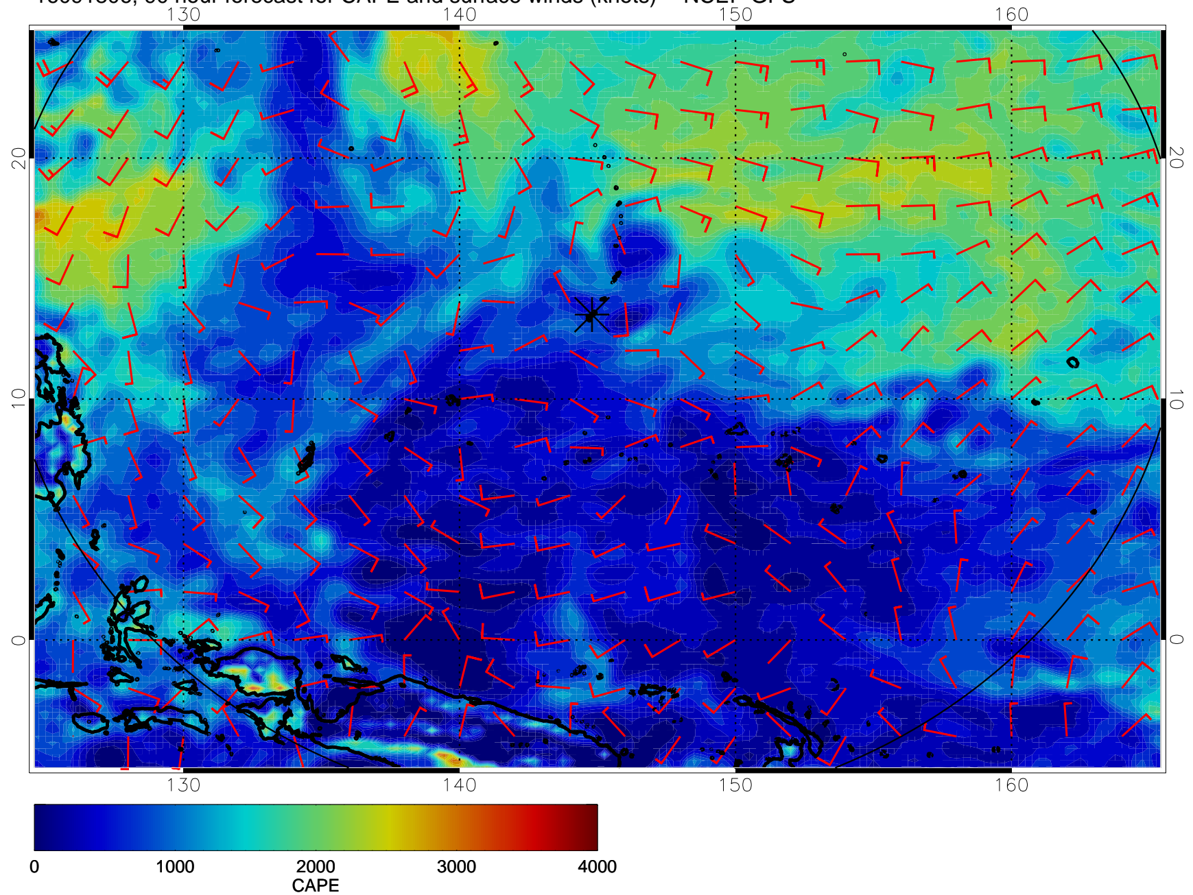
16091806, 90 hour forecast for CAPE and surface winds (knots) -- NCEP GFS
