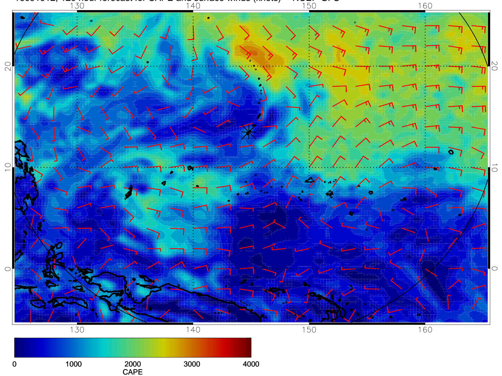
16091912, 120 hour forecast for CAPE and surface winds (knots) -- NCEP GFS
