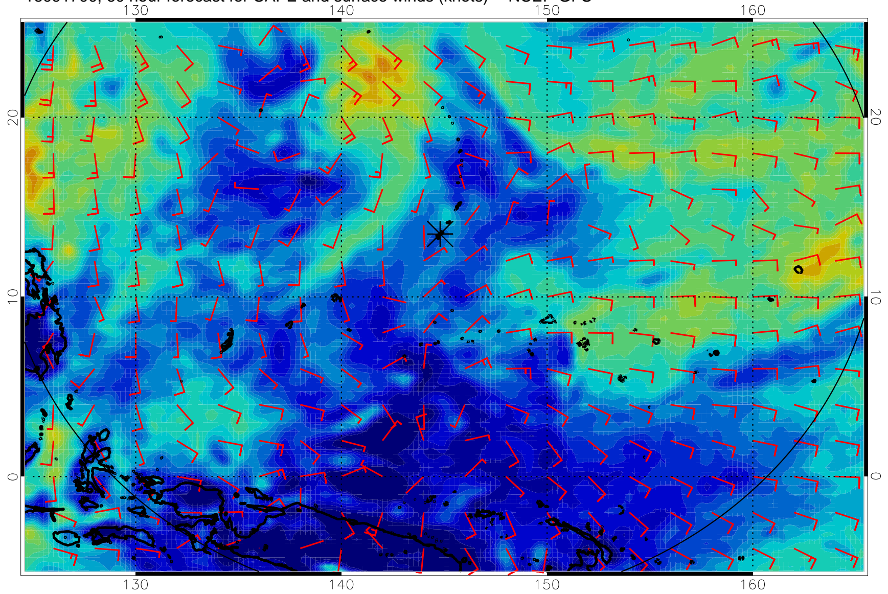
16091700, 60 hour forecast for CAPE and surface winds (knots) -- NCEP GFS
