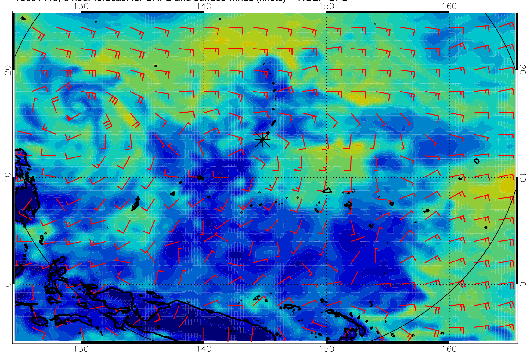
16091418, 6 hour forecast for CAPE and surface winds (knots) -- NCEP GFS
