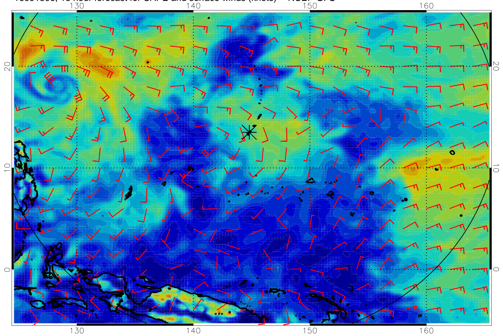
16091506, 18 hour forecast for CAPE and surface winds (knots) -- NCEP GFS
