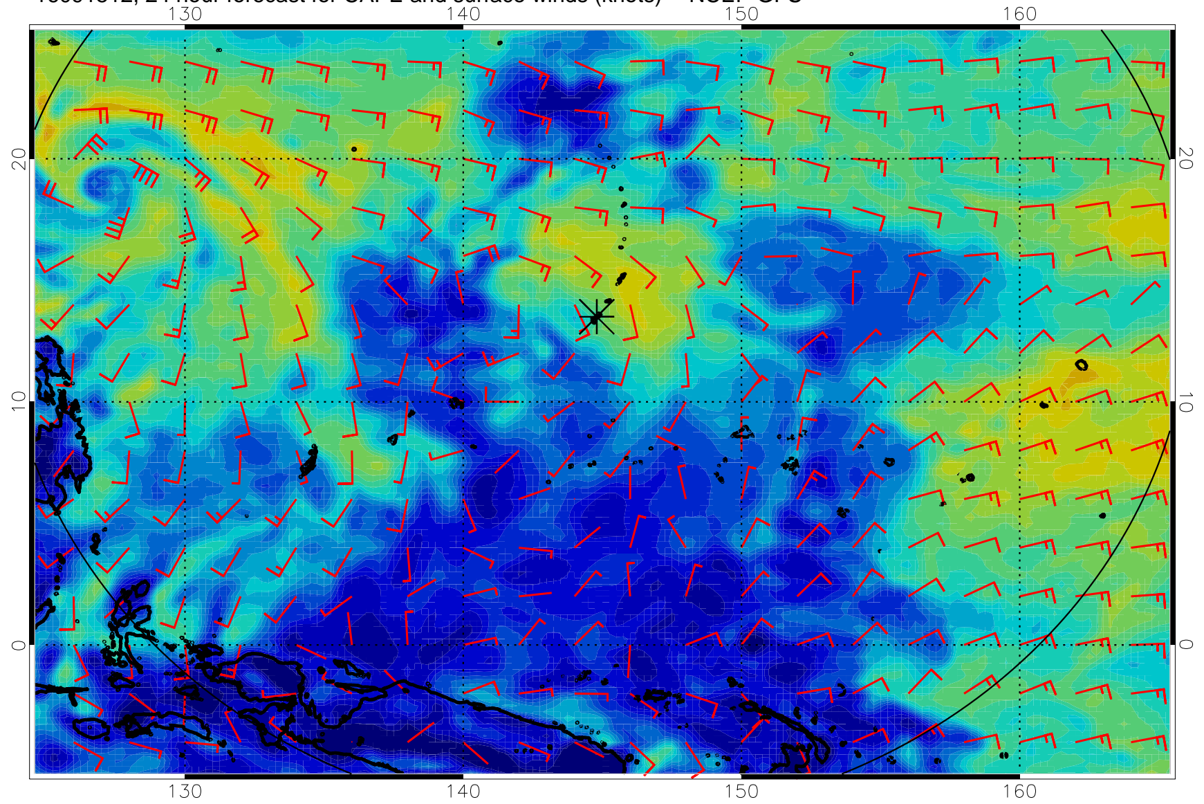
16091512, 24 hour forecast for CAPE and surface winds (knots) -- NCEP GFS
