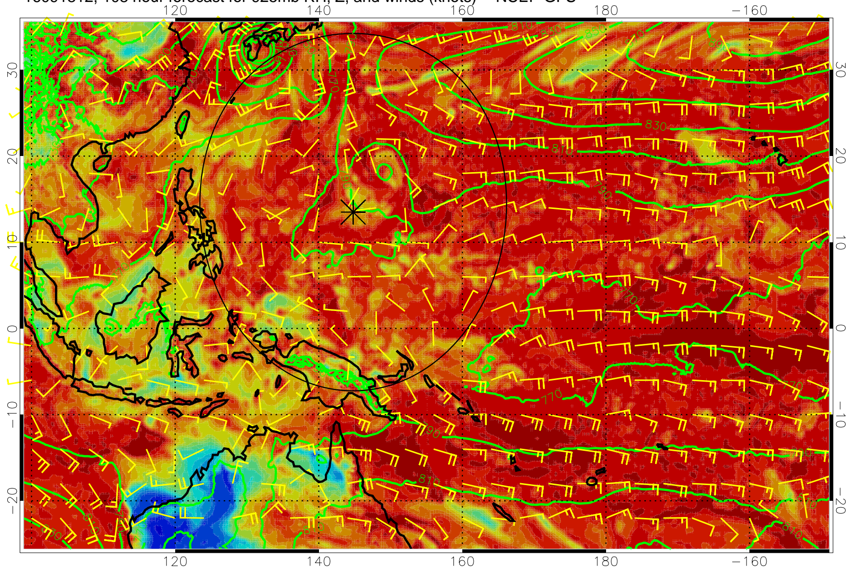
16091812, 108 hour forecast for 925mb RH, Z, and winds (knots) -- NCEP GFS
