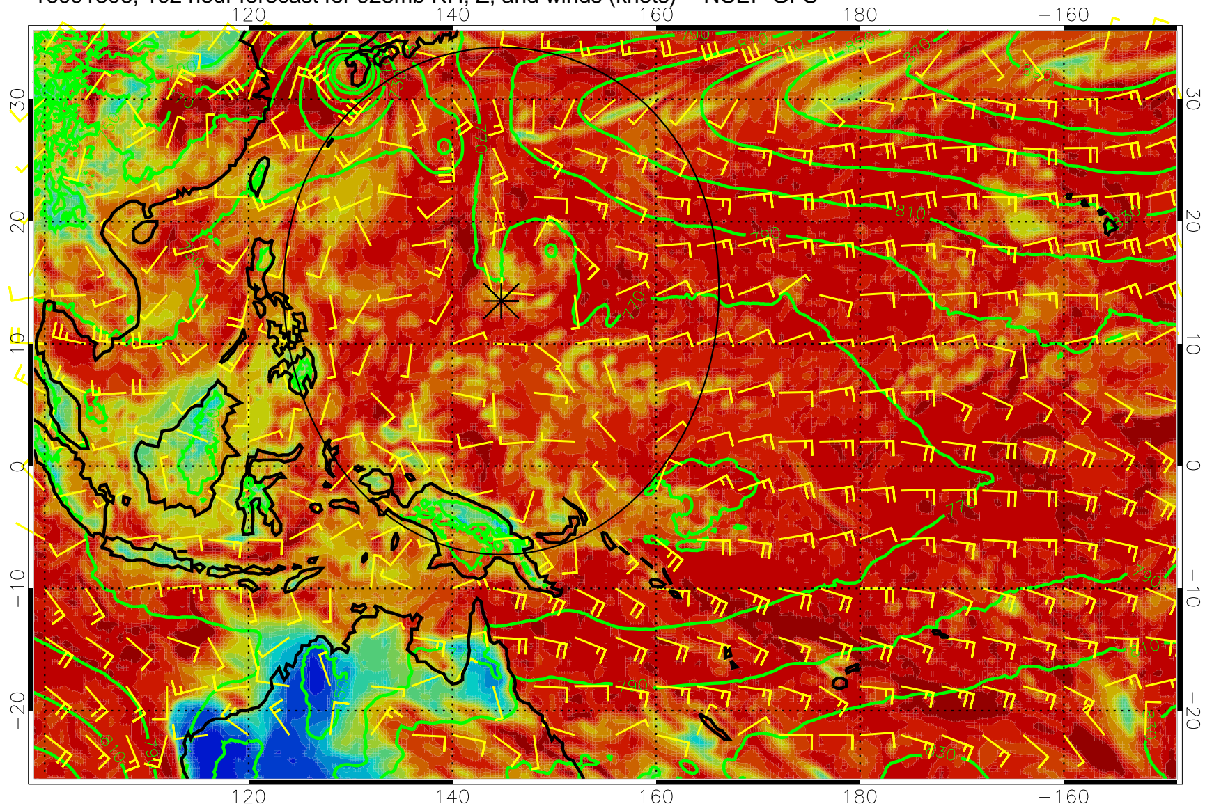
16091806, 102 hour forecast for 925mb RH, Z, and winds (knots) -- NCEP GFS
