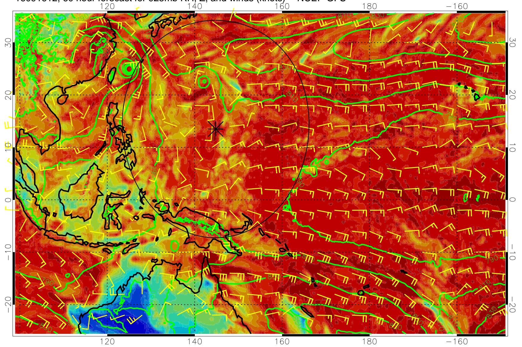
16091612, 60 hour forecast for 925mb RH, Z, and winds (knots) -- NCEP GFS
