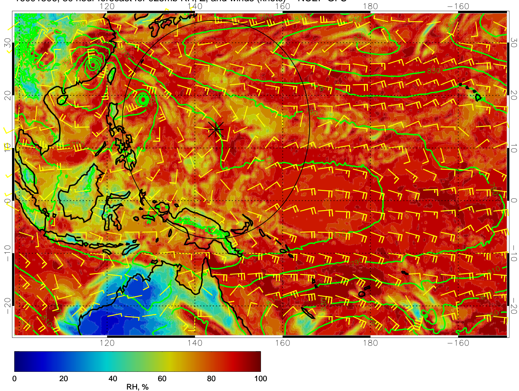
16091506, 30 hour forecast for 925mb RH, Z, and winds (knots) -- NCEP GFS
