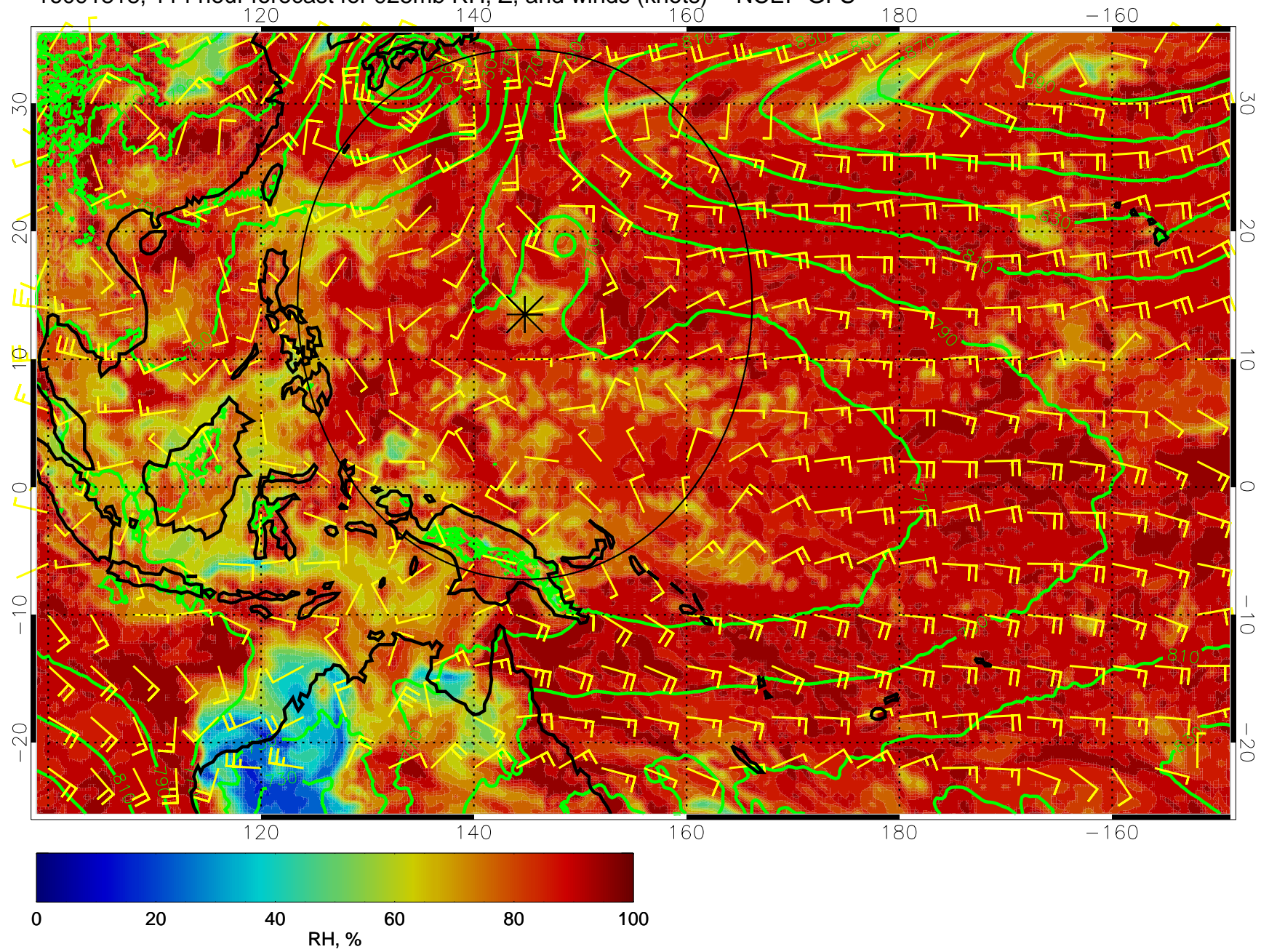
16091818, 114 hour forecast for 925mb RH, Z, and winds (knots) -- NCEP GFS
