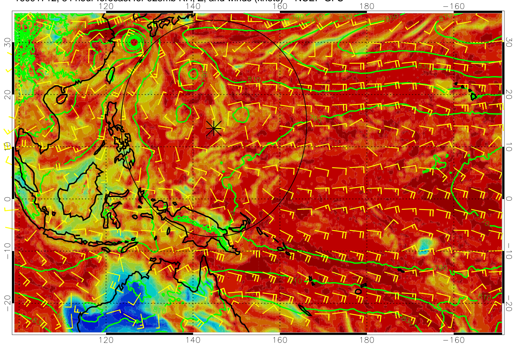
16091712, 84 hour forecast for 925mb RH, Z, and winds (knots) -- NCEP GFS
