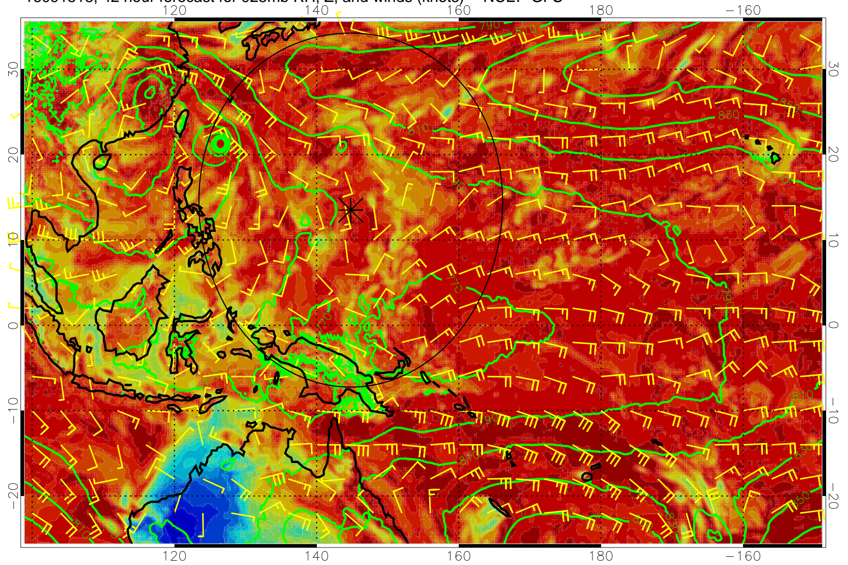
16091518, 42 hour forecast for 925mb RH, Z, and winds (knots) -- NCEP GFS
