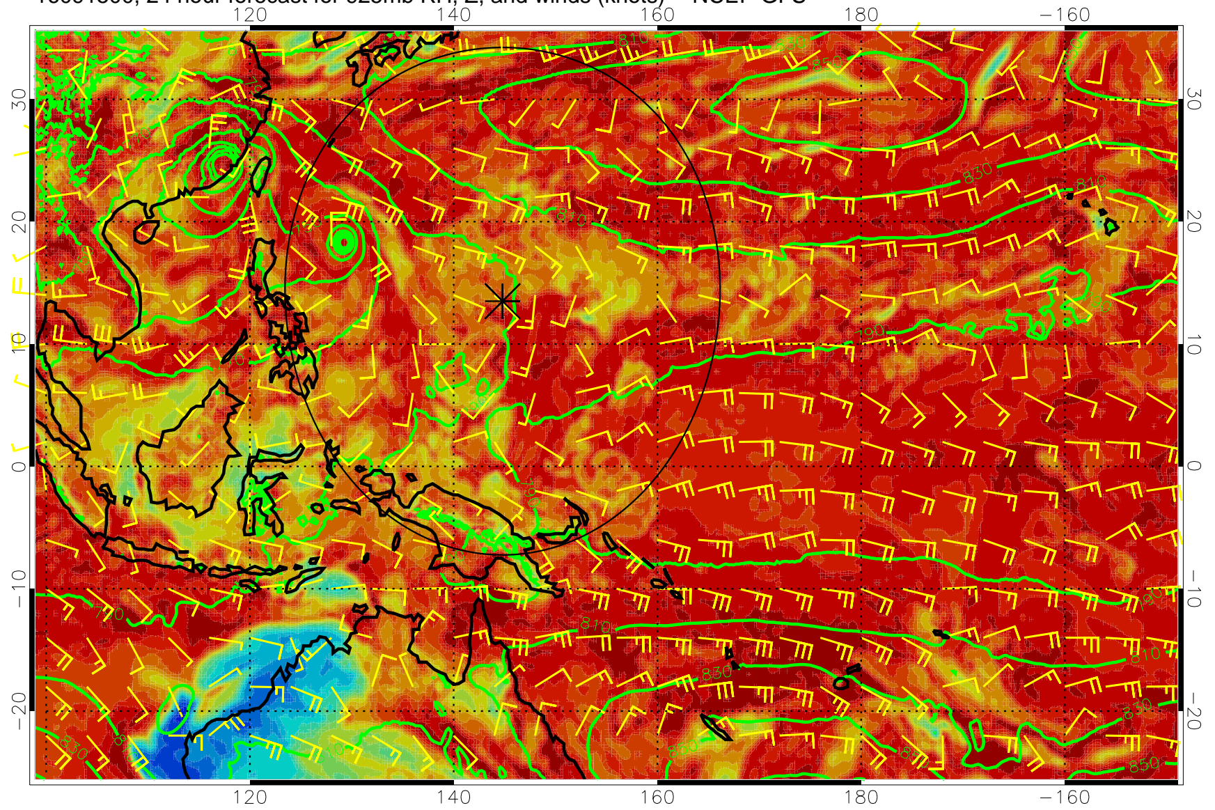
16091500, 24 hour forecast for 925mb RH, Z, and winds (knots) -- NCEP GFS
