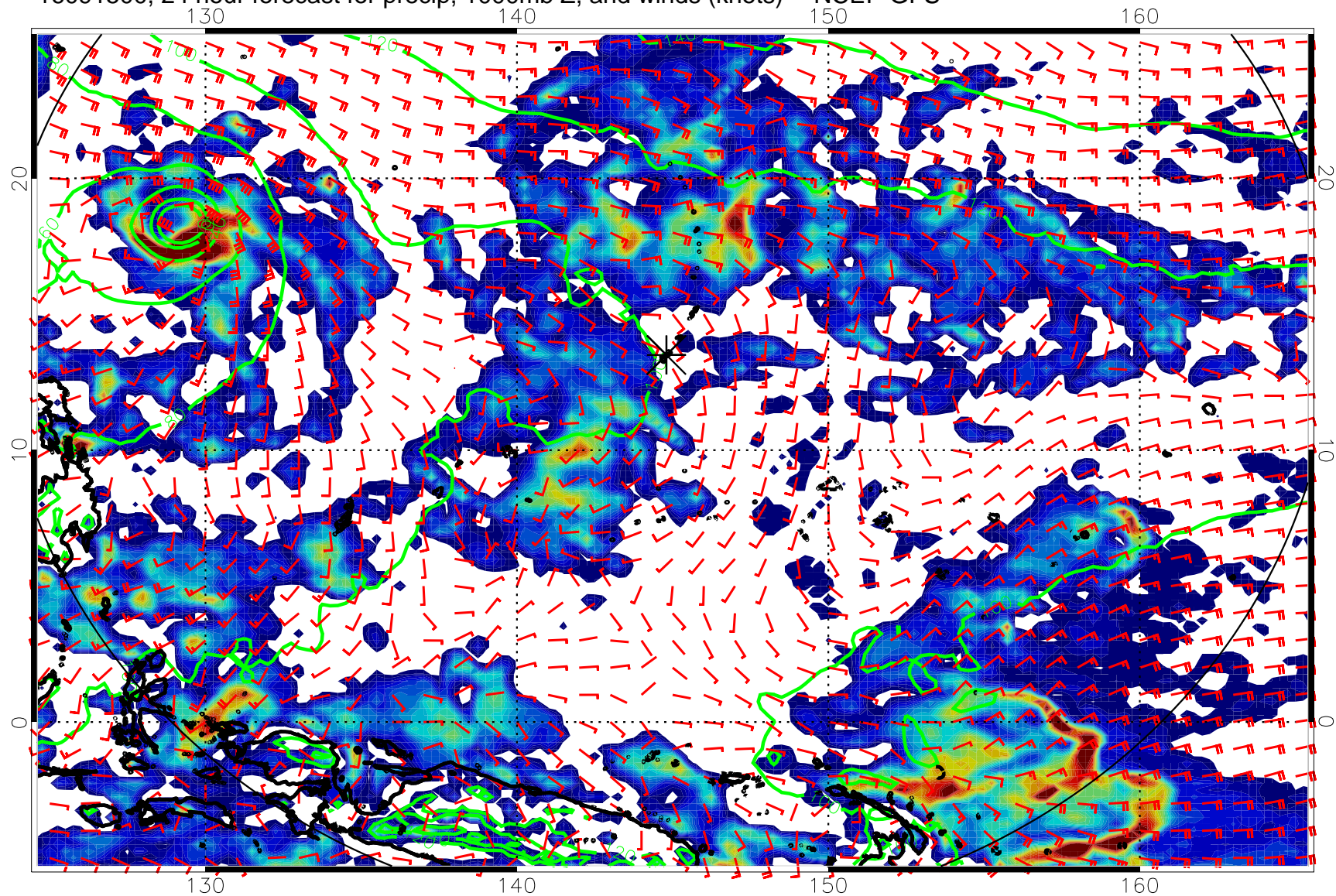
16091500, 24 hour forecast for precip, 1000mb Z, and winds (knots) -- NCEP GFS
