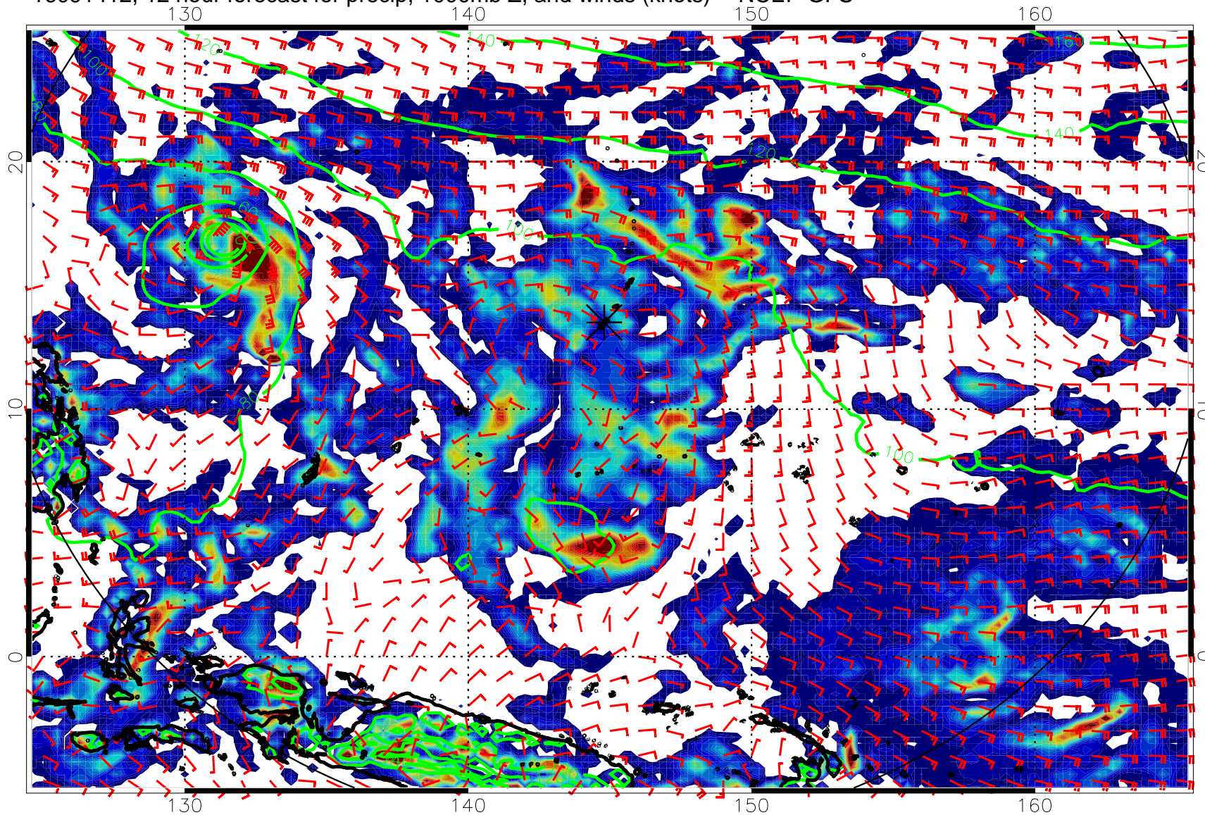
16091412, 12 hour forecast for precip, 1000mb Z, and winds (knots) -- NCEP GFS
