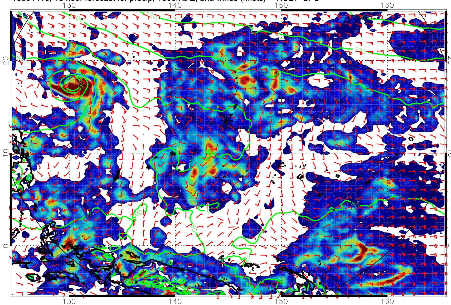
16091418, 18 hour forecast for precip, 1000mb Z, and winds (knots) -- NCEP GFS
