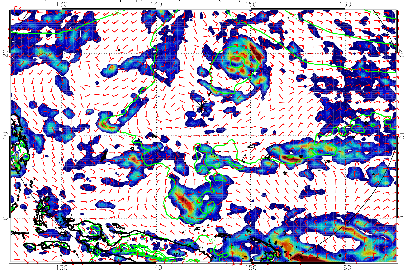
16091818, 114 hour forecast for precip, 1000mb Z, and winds (knots) -- NCEP GFS
