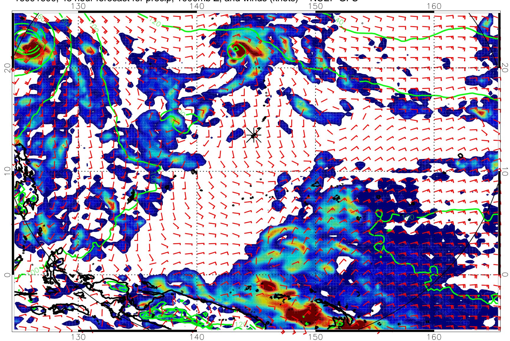
16091600, 48 hour forecast for precip, 1000mb Z, and winds (knots) -- NCEP GFS
