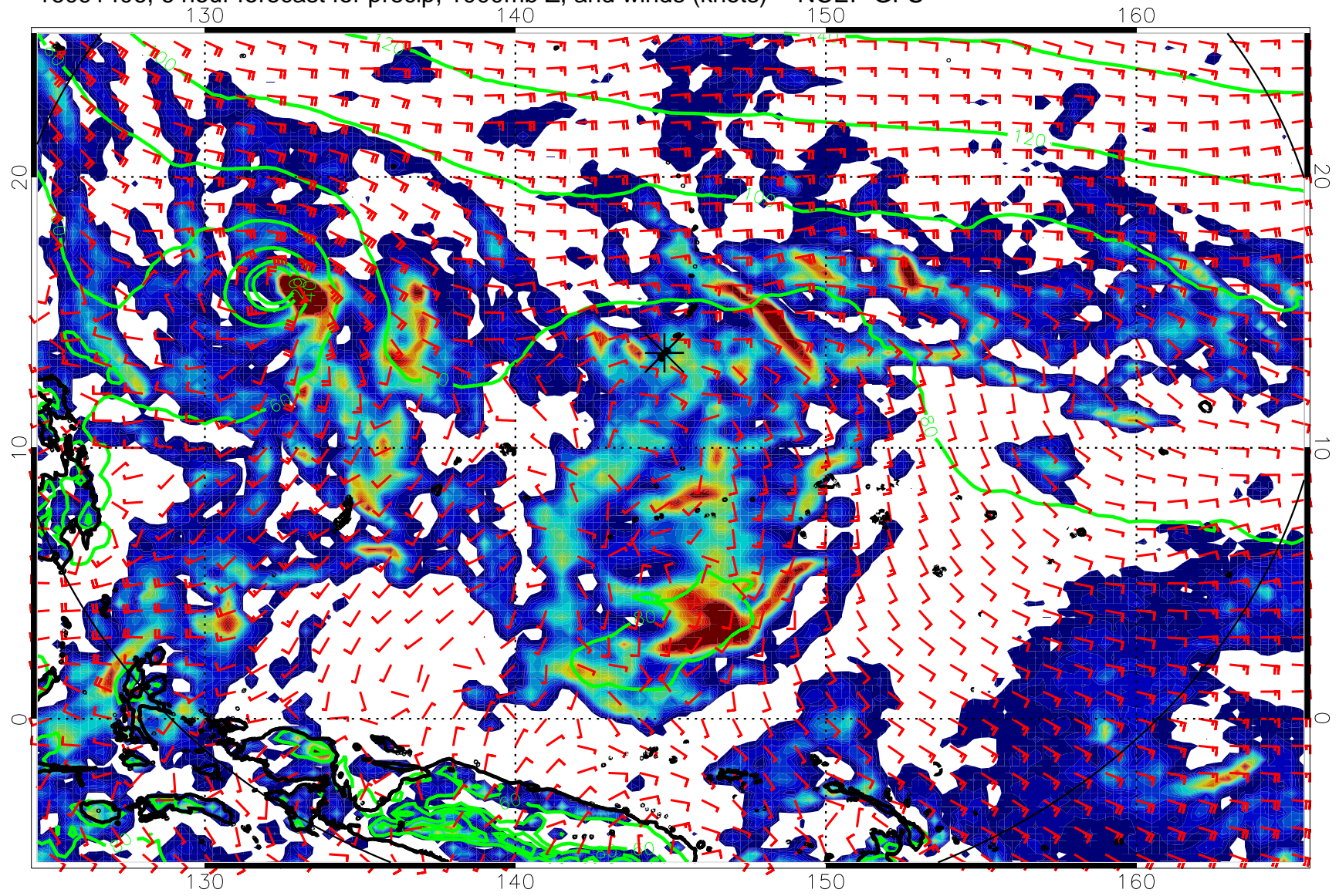
16091406, 6 hour forecast for precip, 1000mb Z, and winds (knots) -- NCEP GFS
