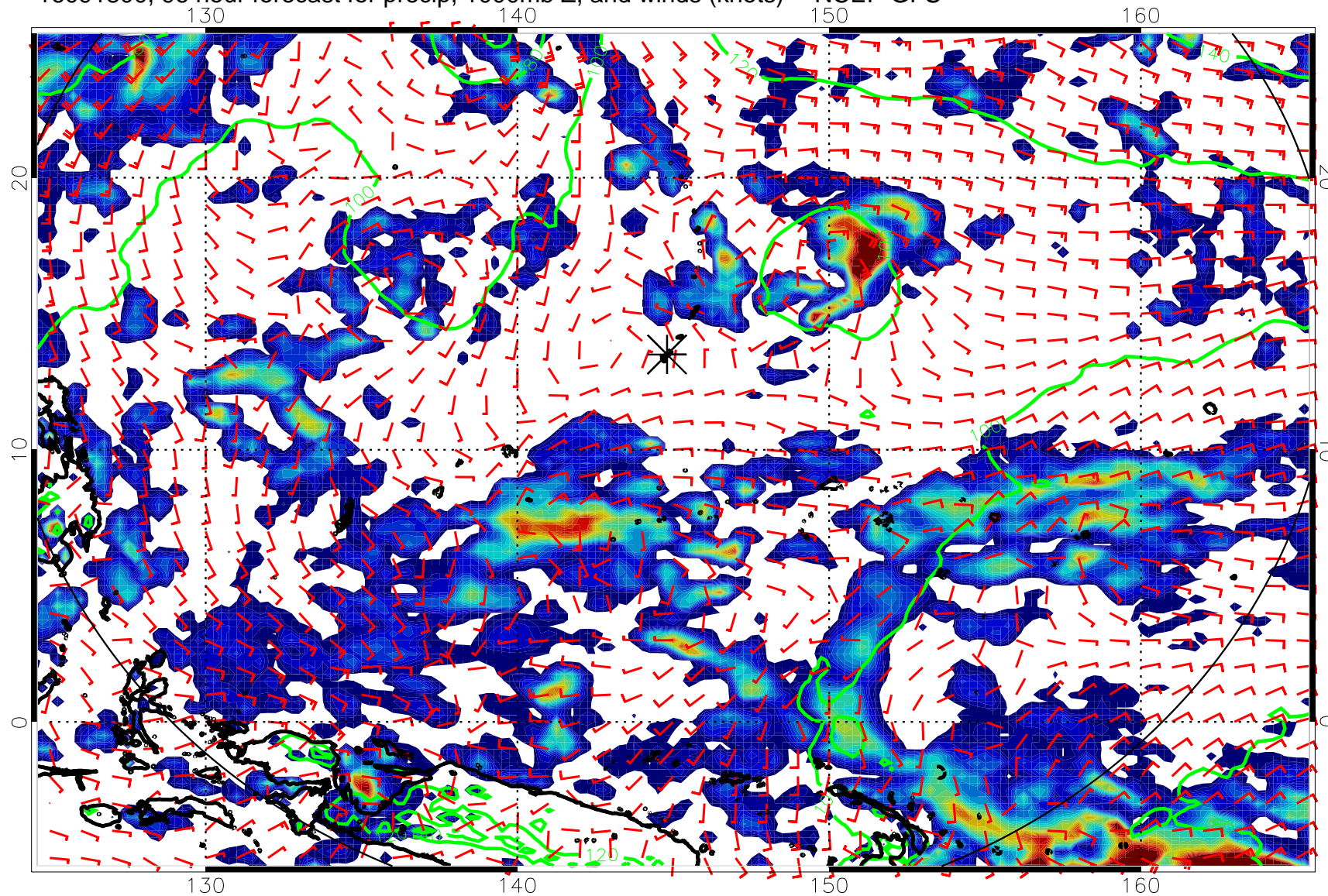
16091800, 96 hour forecast for precip, 1000mb Z, and winds (knots) -- NCEP GFS
