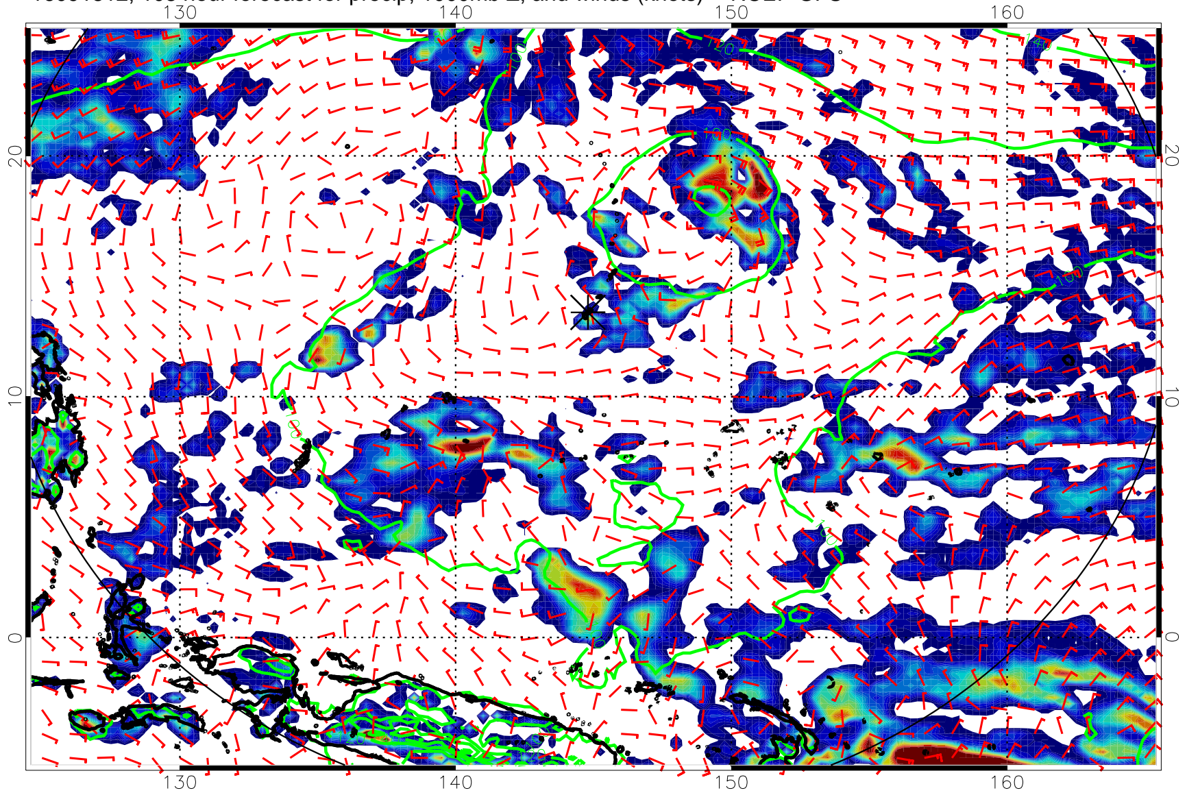
16091812, 108 hour forecast for precip, 1000mb Z, and winds (knots) -- NCEP GFS
