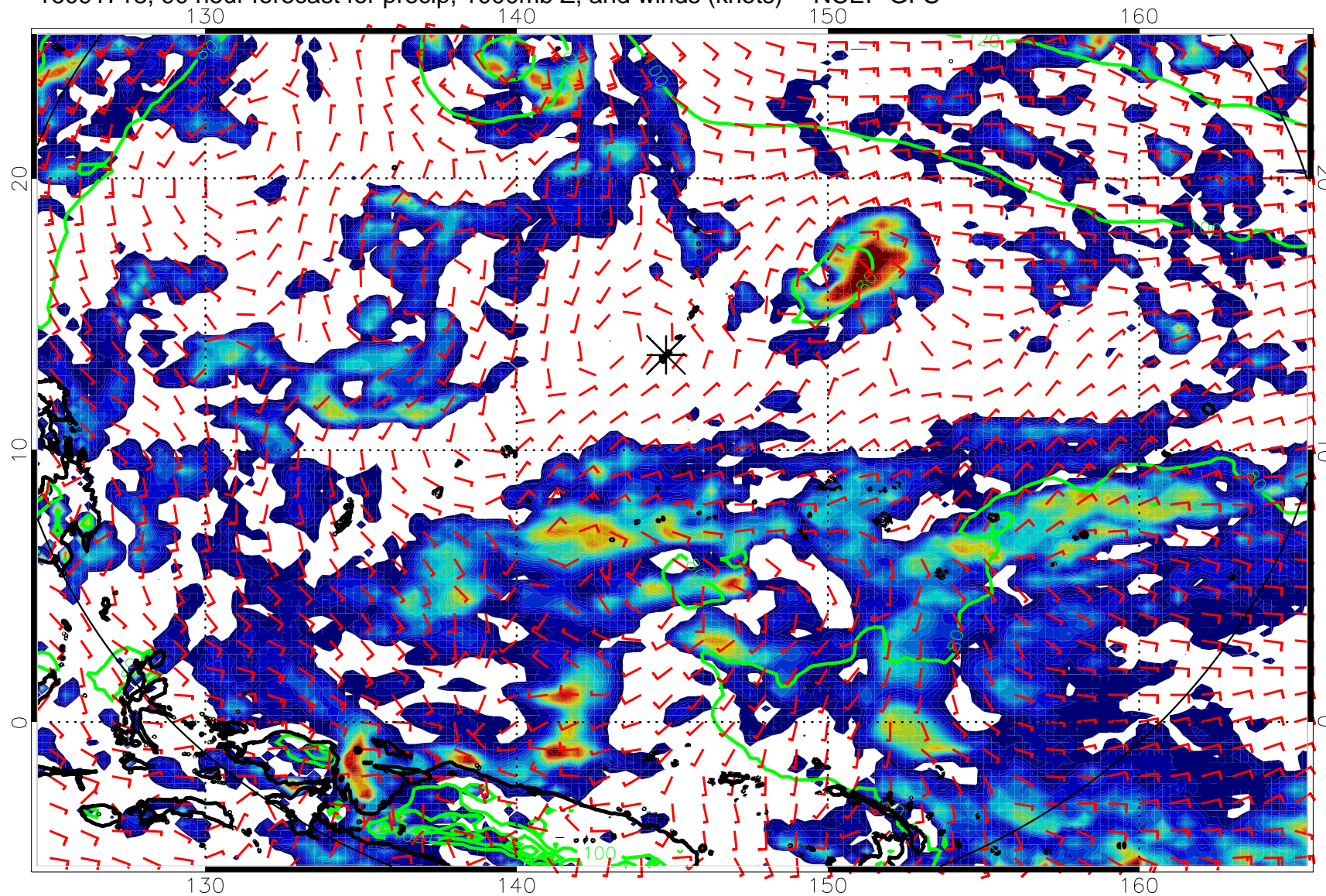
16091718, 90 hour forecast for precip, 1000mb Z, and winds (knots) -- NCEP GFS
