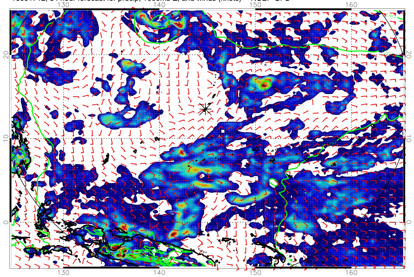
16091712, 84 hour forecast for precip, 1000mb Z, and winds (knots) -- NCEP GFS
