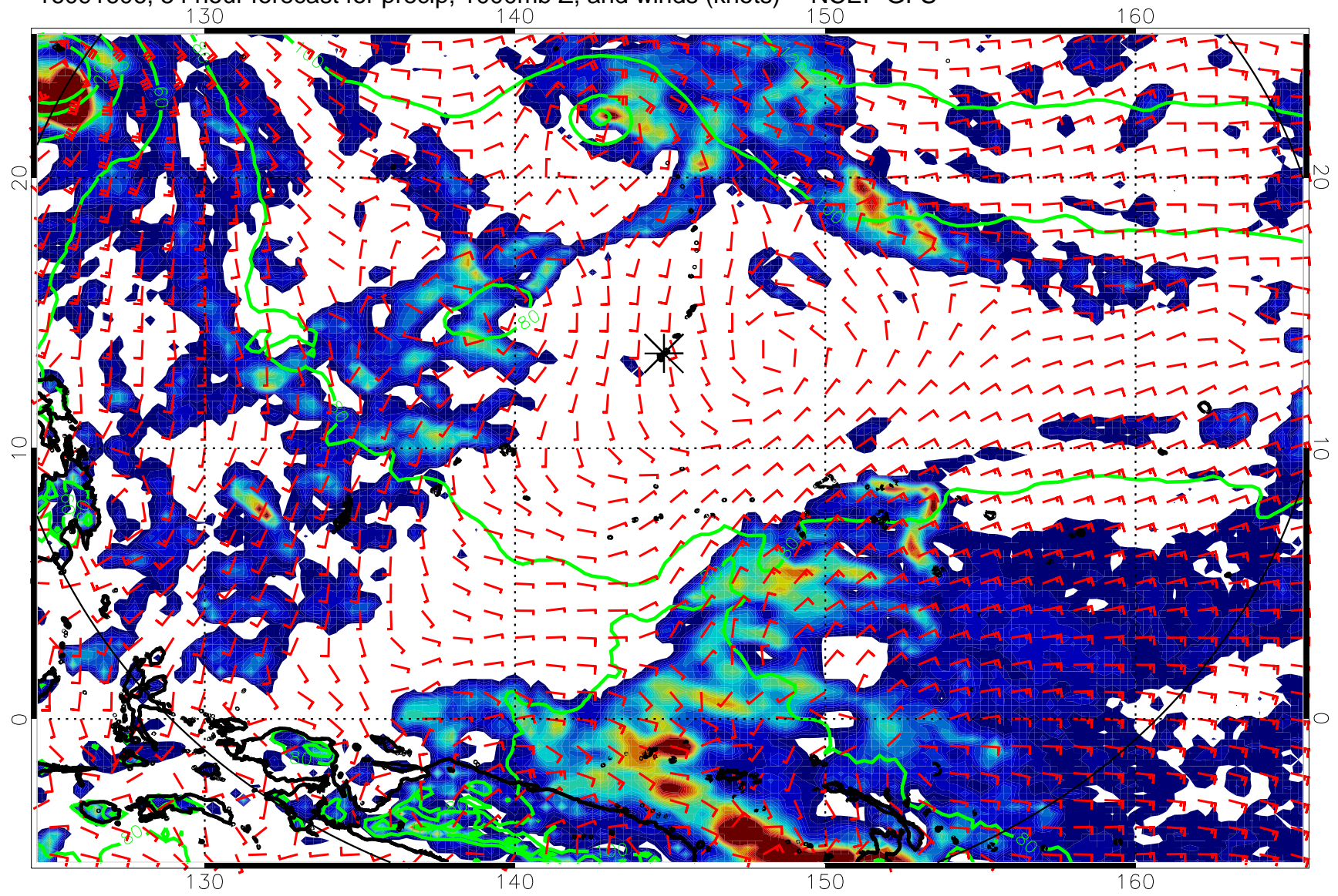
16091606, 54 hour forecast for precip, 1000mb Z, and winds (knots) -- NCEP GFS
