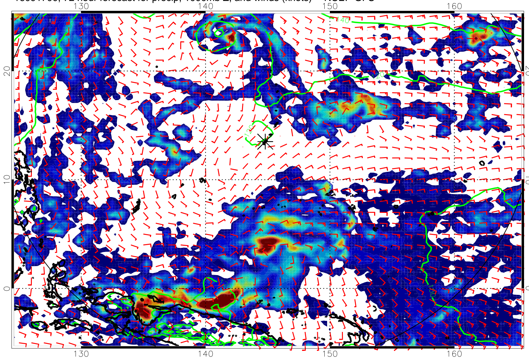
16091700, 72 hour forecast for precip, 1000mb Z, and winds (knots) -- NCEP GFS
