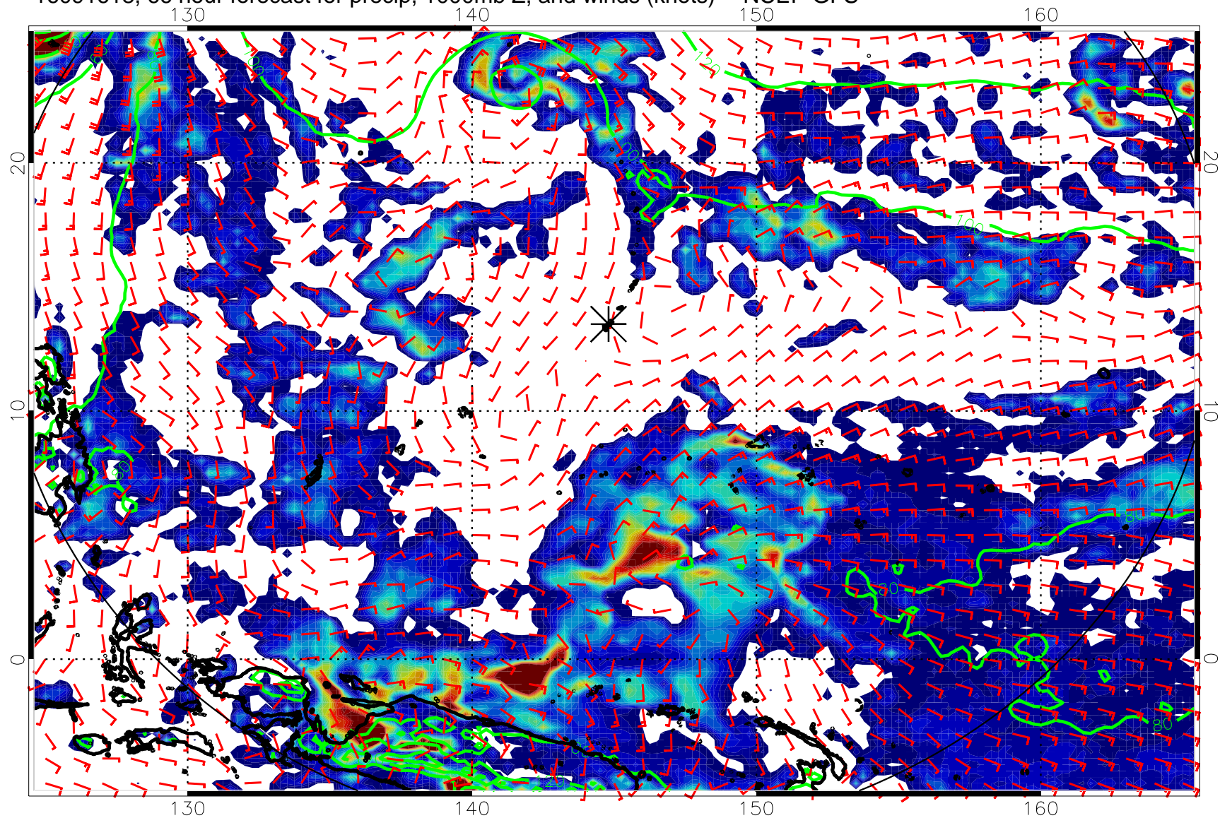
16091618, 66 hour forecast for precip, 1000mb Z, and winds (knots) -- NCEP GFS
