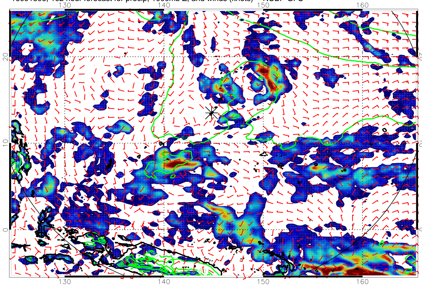
16091806, 102 hour forecast for precip, 1000mb Z, and winds (knots) -- NCEP GFS
