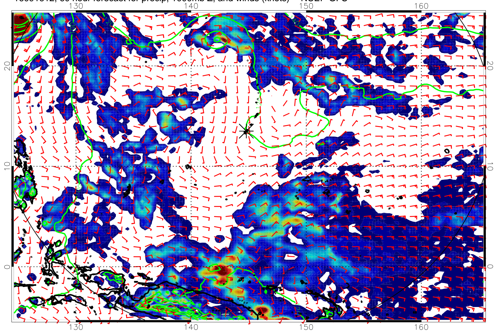
16091612, 60 hour forecast for precip, 1000mb Z, and winds (knots) -- NCEP GFS
