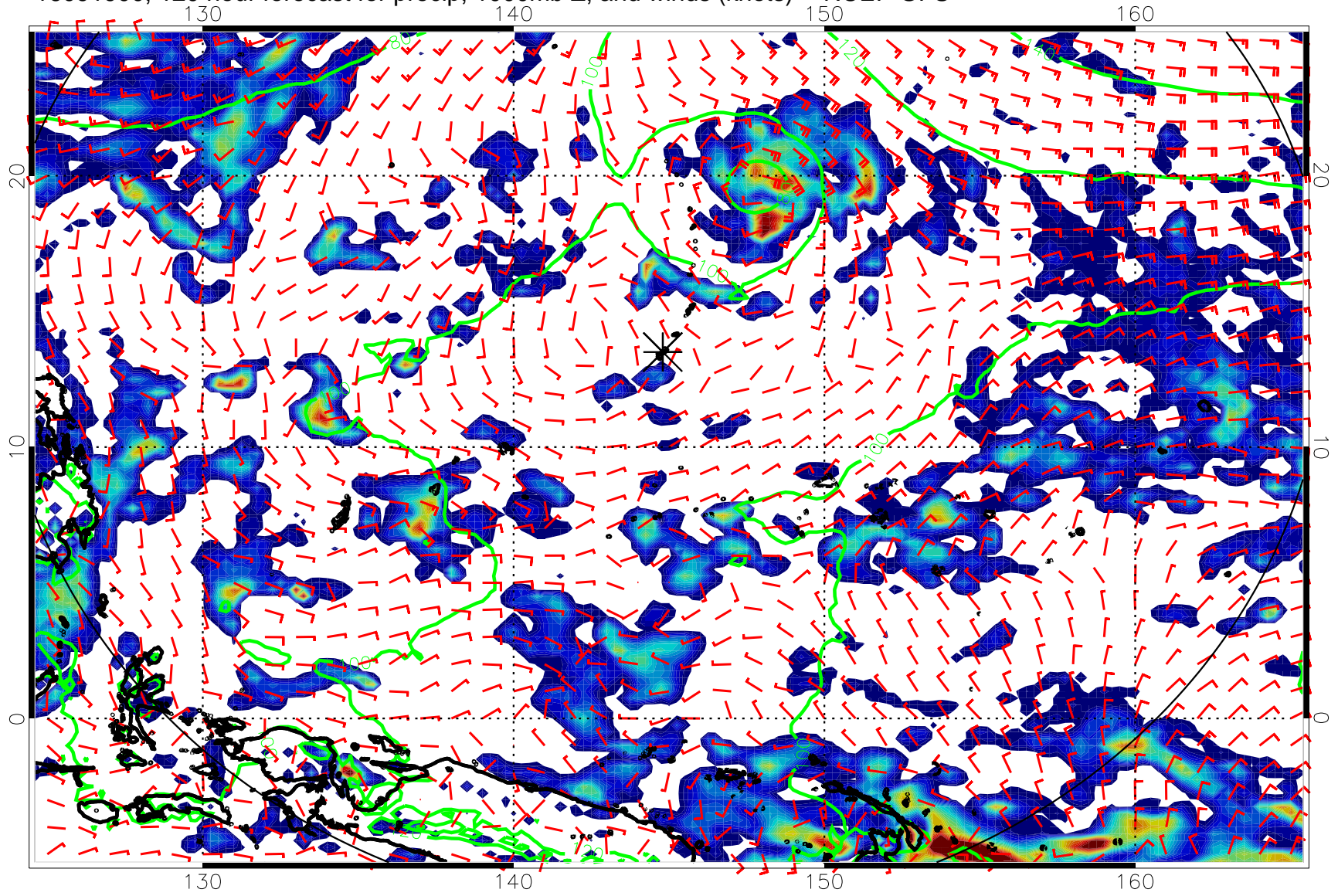
16091900, 120 hour forecast for precip, 1000mb Z, and winds (knots) -- NCEP GFS
