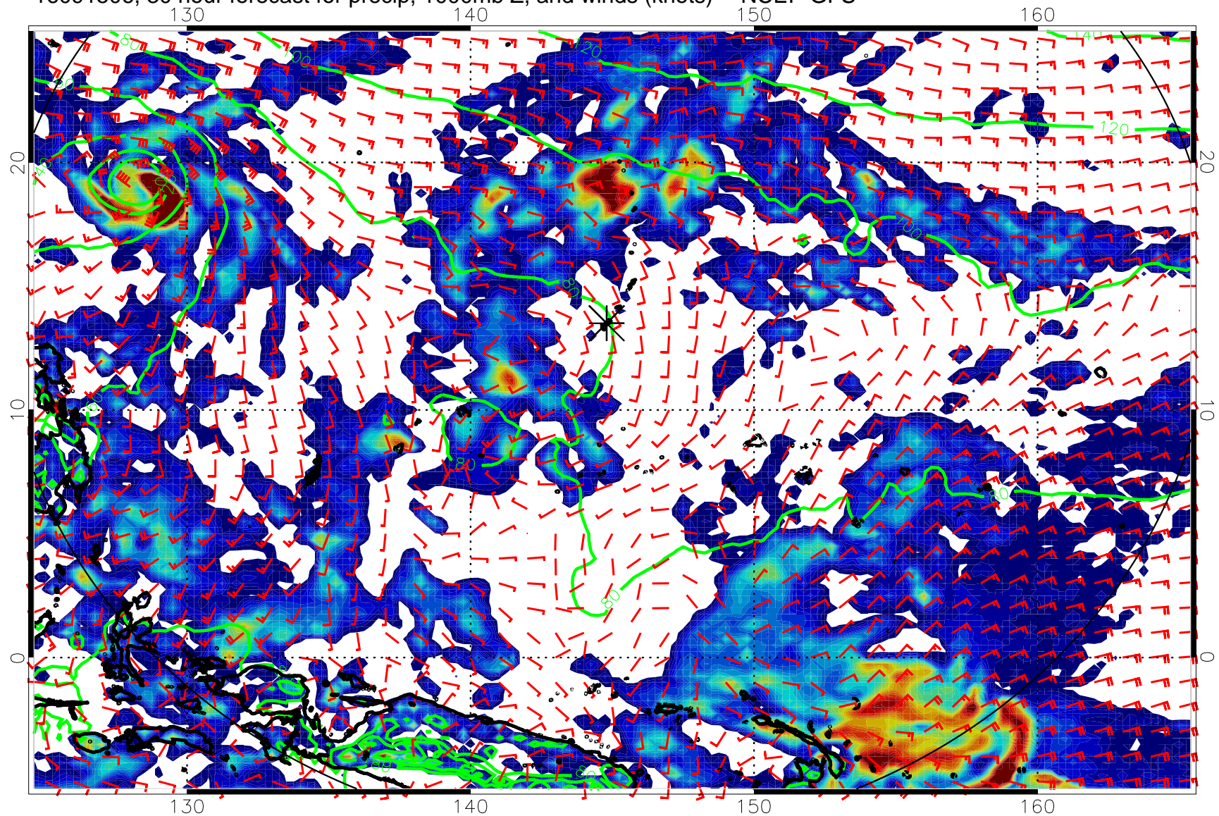
16091506, 30 hour forecast for precip, 1000mb Z, and winds (knots) -- NCEP GFS
