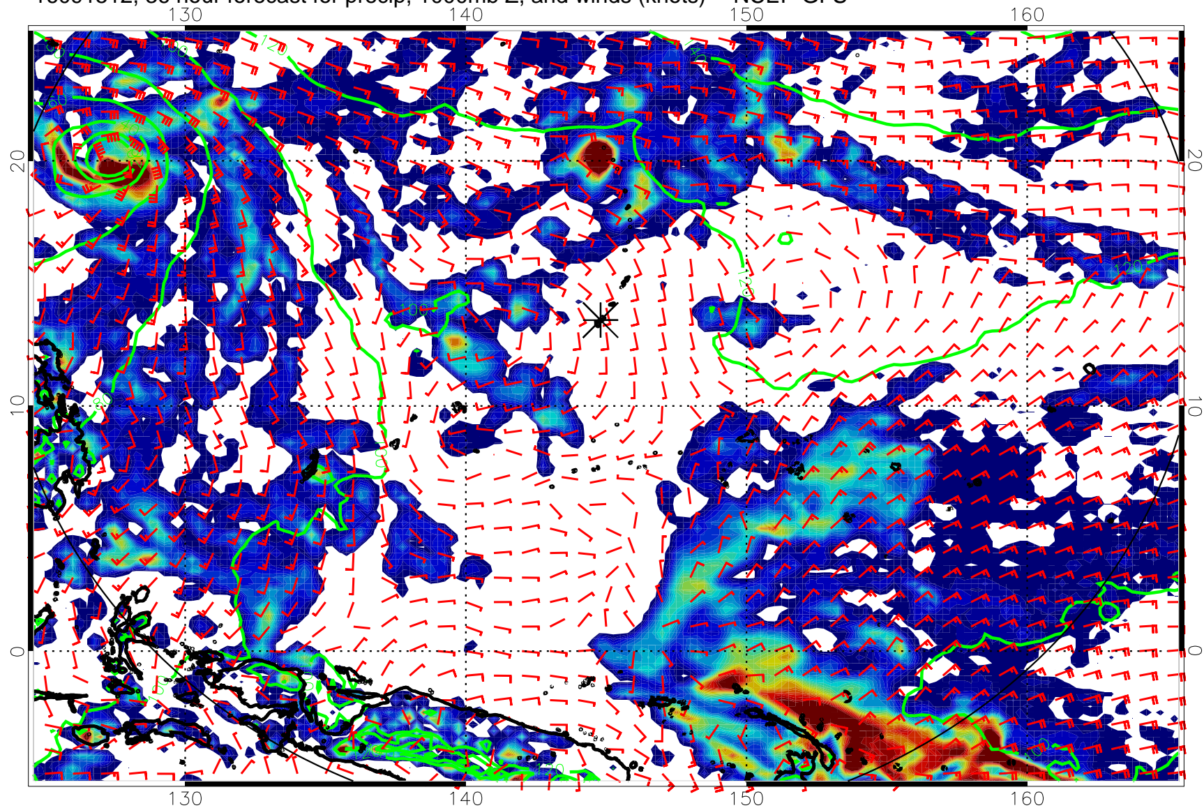
16091512, 36 hour forecast for precip, 1000mb Z, and winds (knots) -- NCEP GFS
