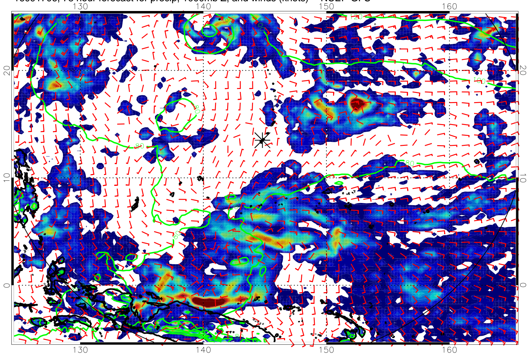
16091706, 78 hour forecast for precip, 1000mb Z, and winds (knots) -- NCEP GFS
