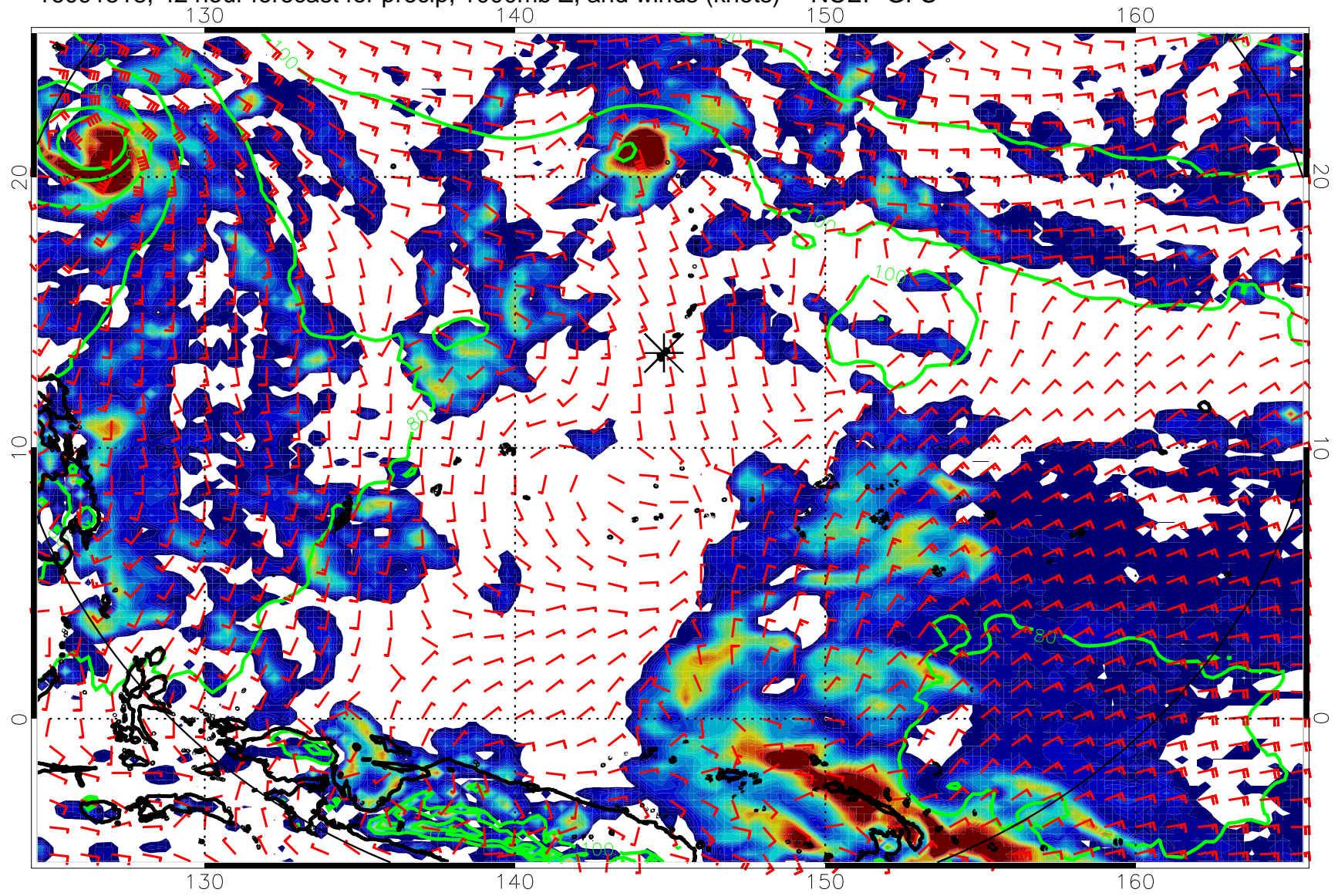
16091518, 42 hour forecast for precip, 1000mb Z, and winds (knots) -- NCEP GFS
