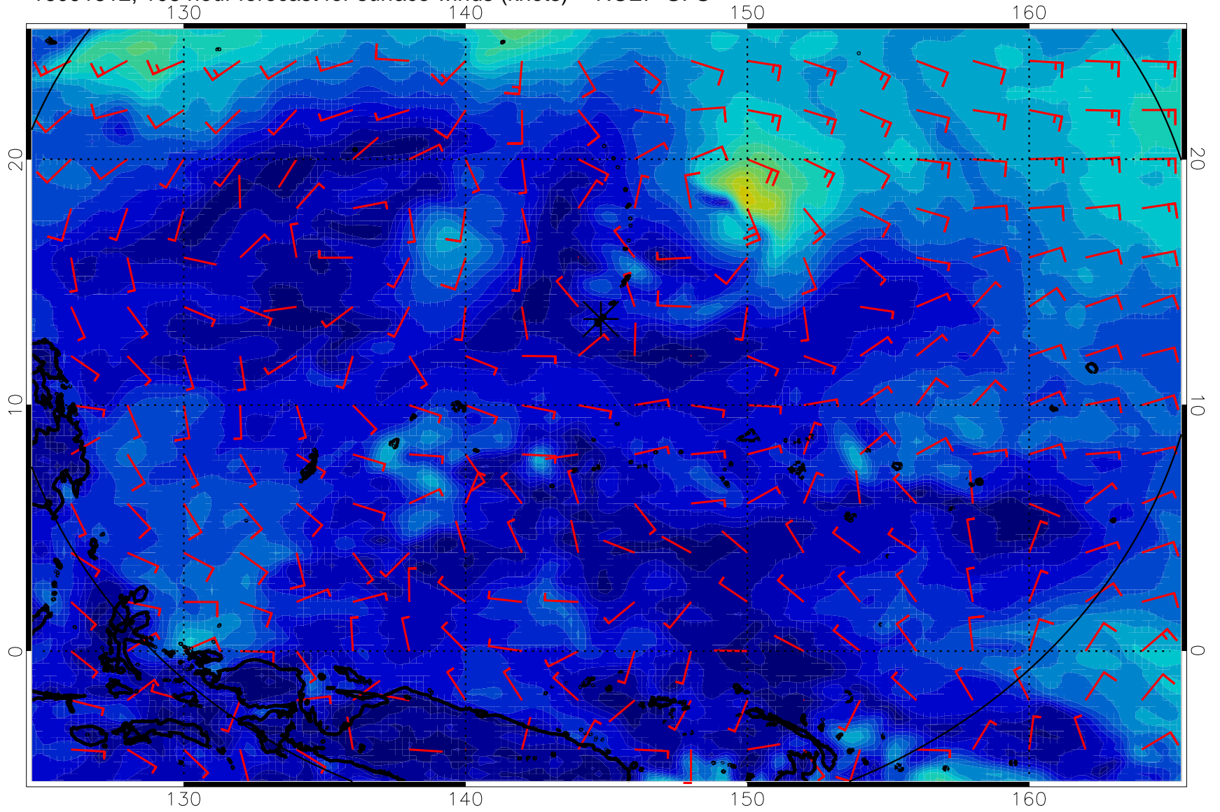
16091812, 108 hour forecast for surface winds (knots) -- NCEP GFS
