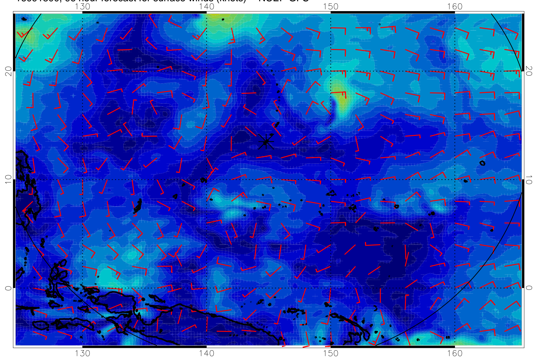
16091800, 96 hour forecast for surface winds (knots) -- NCEP GFS
