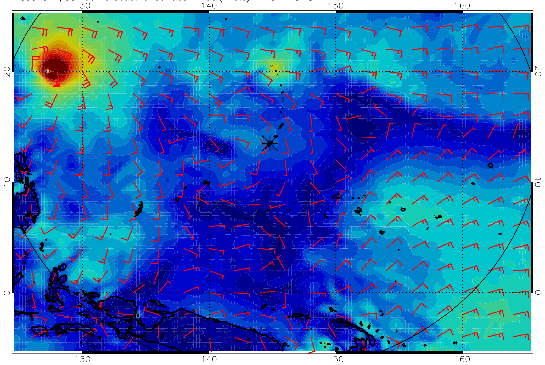
16091512, 36 hour forecast for surface winds (knots) -- NCEP GFS
