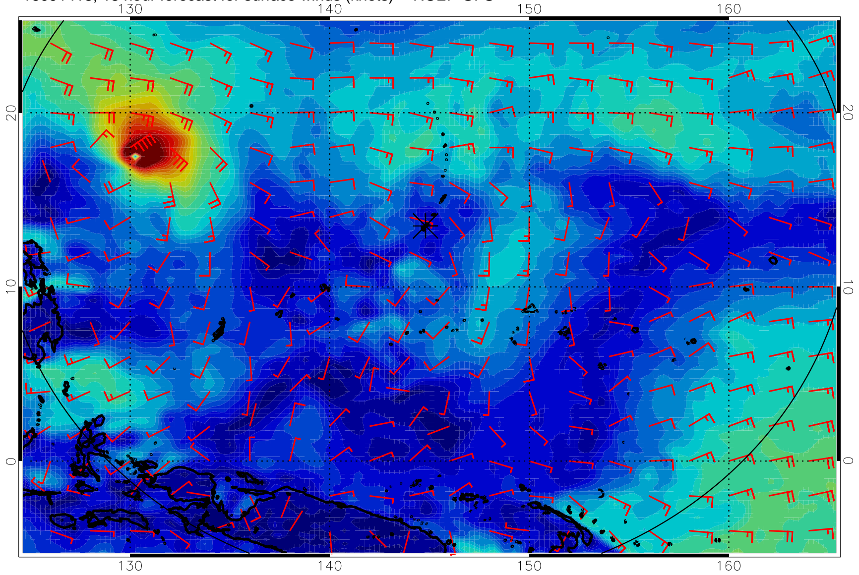
16091418, 18 hour forecast for surface winds (knots) -- NCEP GFS
