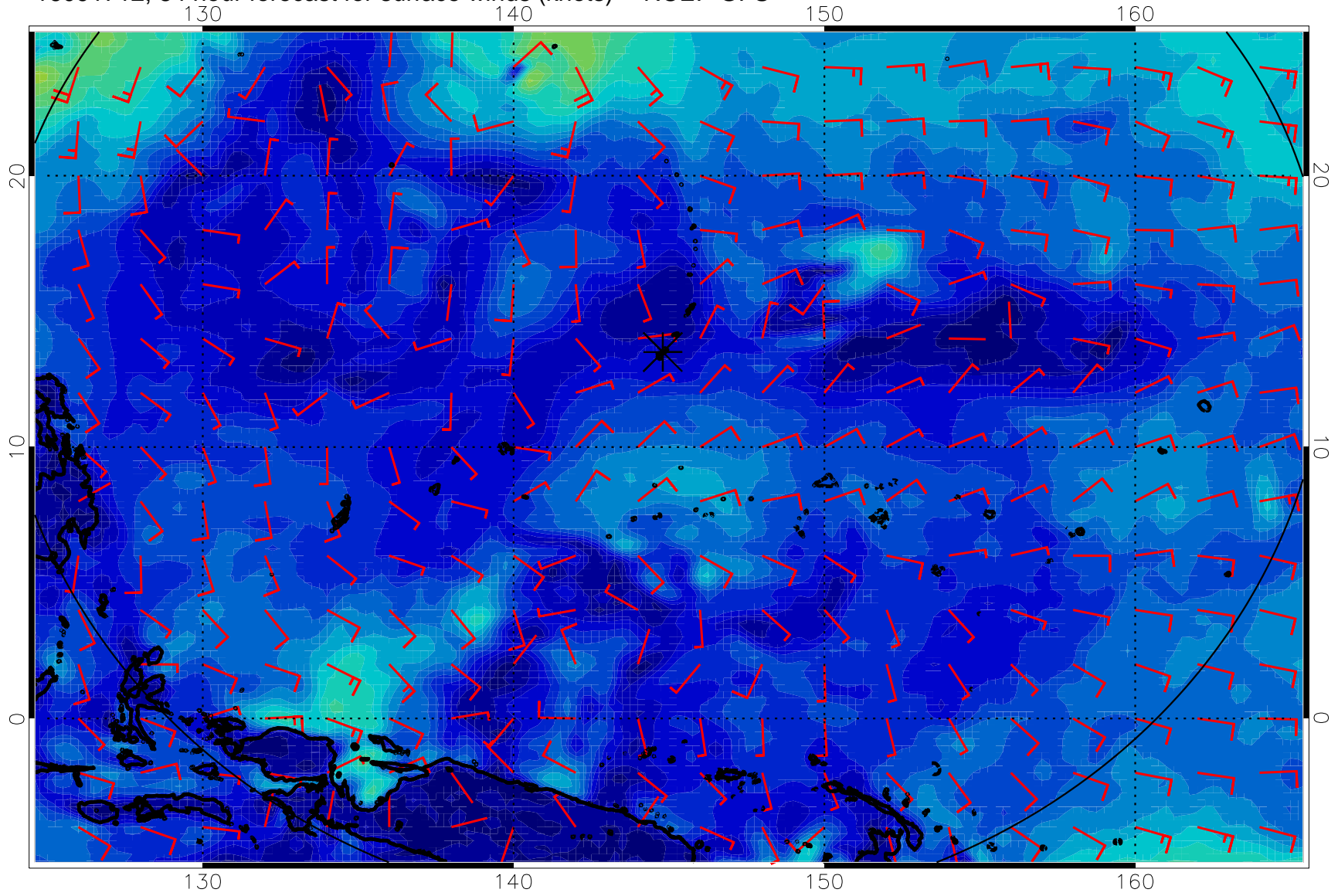
16091712, 84 hour forecast for surface winds (knots) -- NCEP GFS
