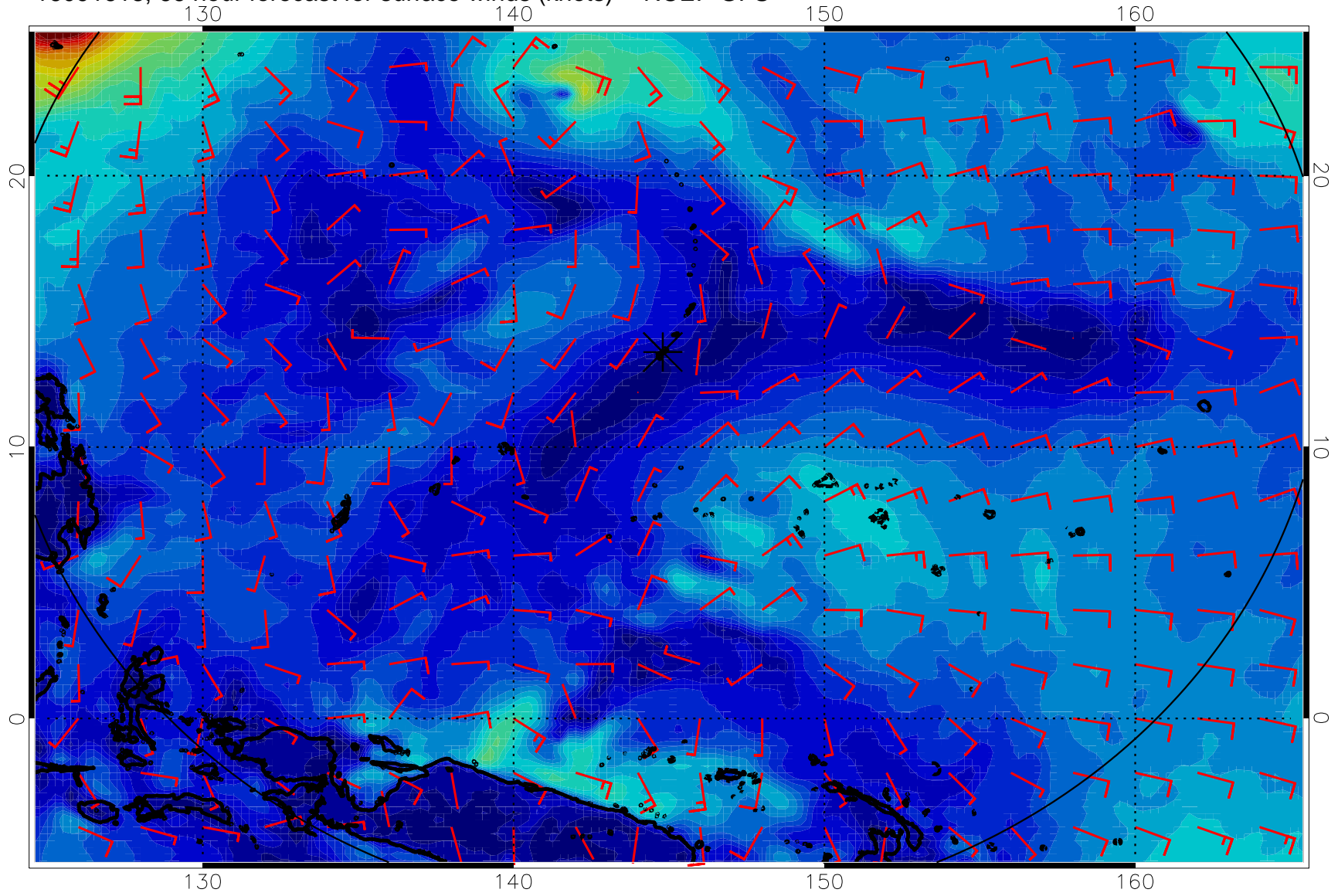
16091618, 66 hour forecast for surface winds (knots) -- NCEP GFS
