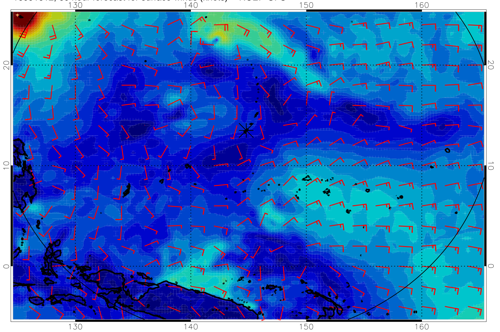
16091612, 60 hour forecast for surface winds (knots) -- NCEP GFS
