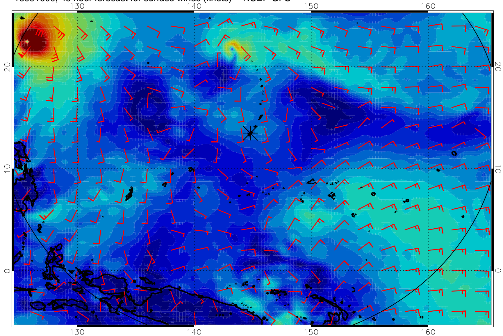
16091600, 48 hour forecast for surface winds (knots) -- NCEP GFS
