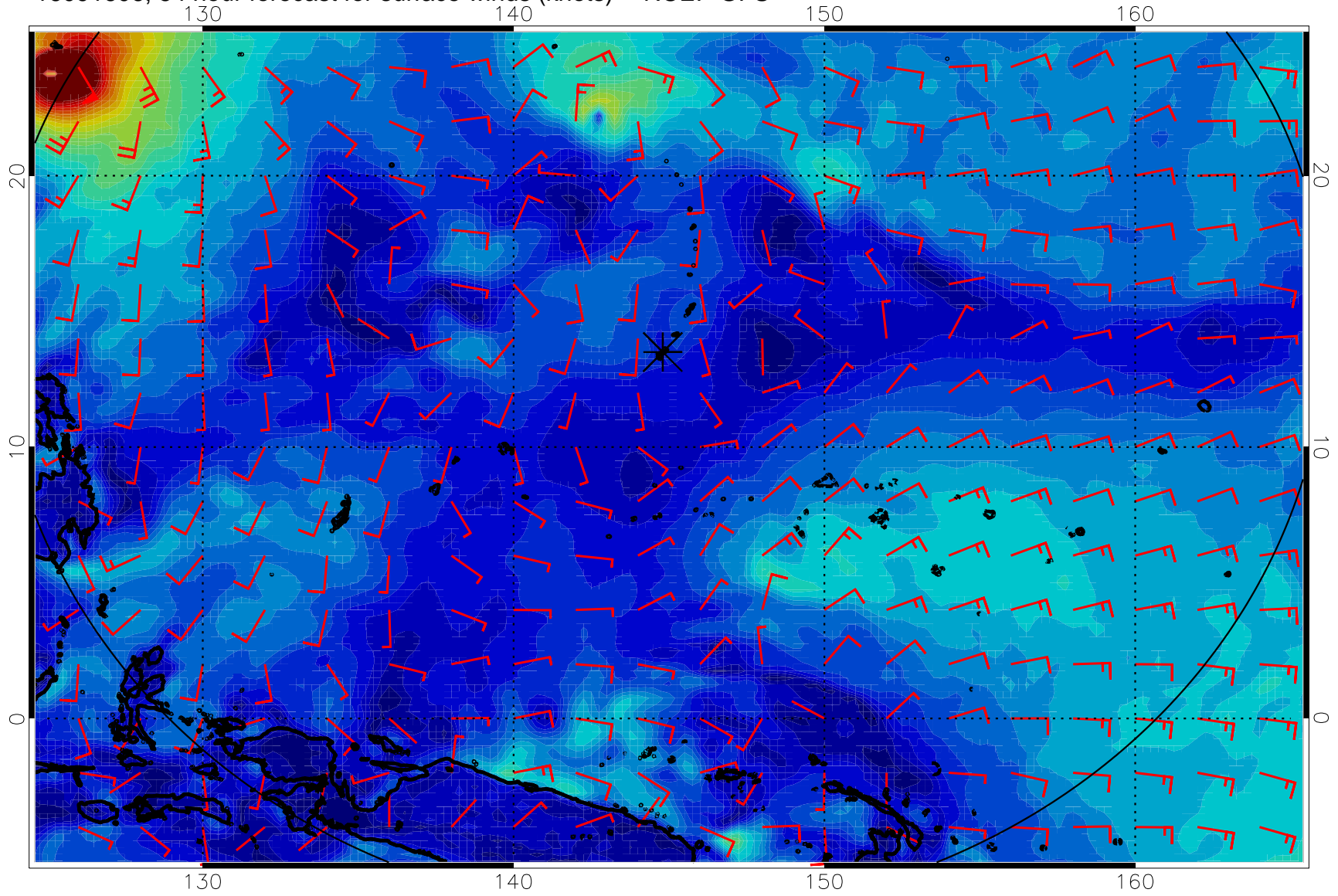
16091606, 54 hour forecast for surface winds (knots) -- NCEP GFS
