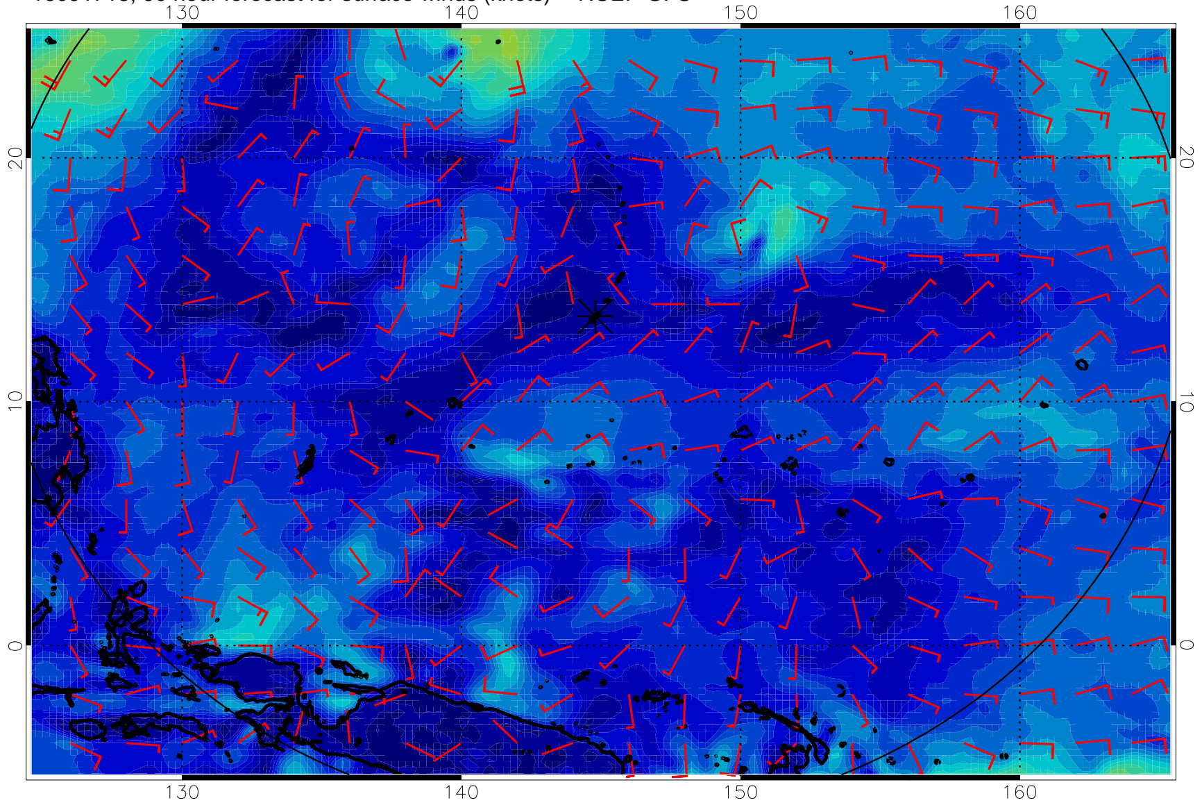
16091718, 90 hour forecast for surface winds (knots) -- NCEP GFS
