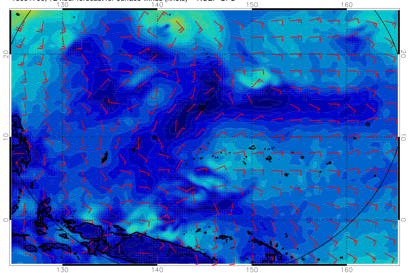
16091700, 72 hour forecast for surface winds (knots) -- NCEP GFS
