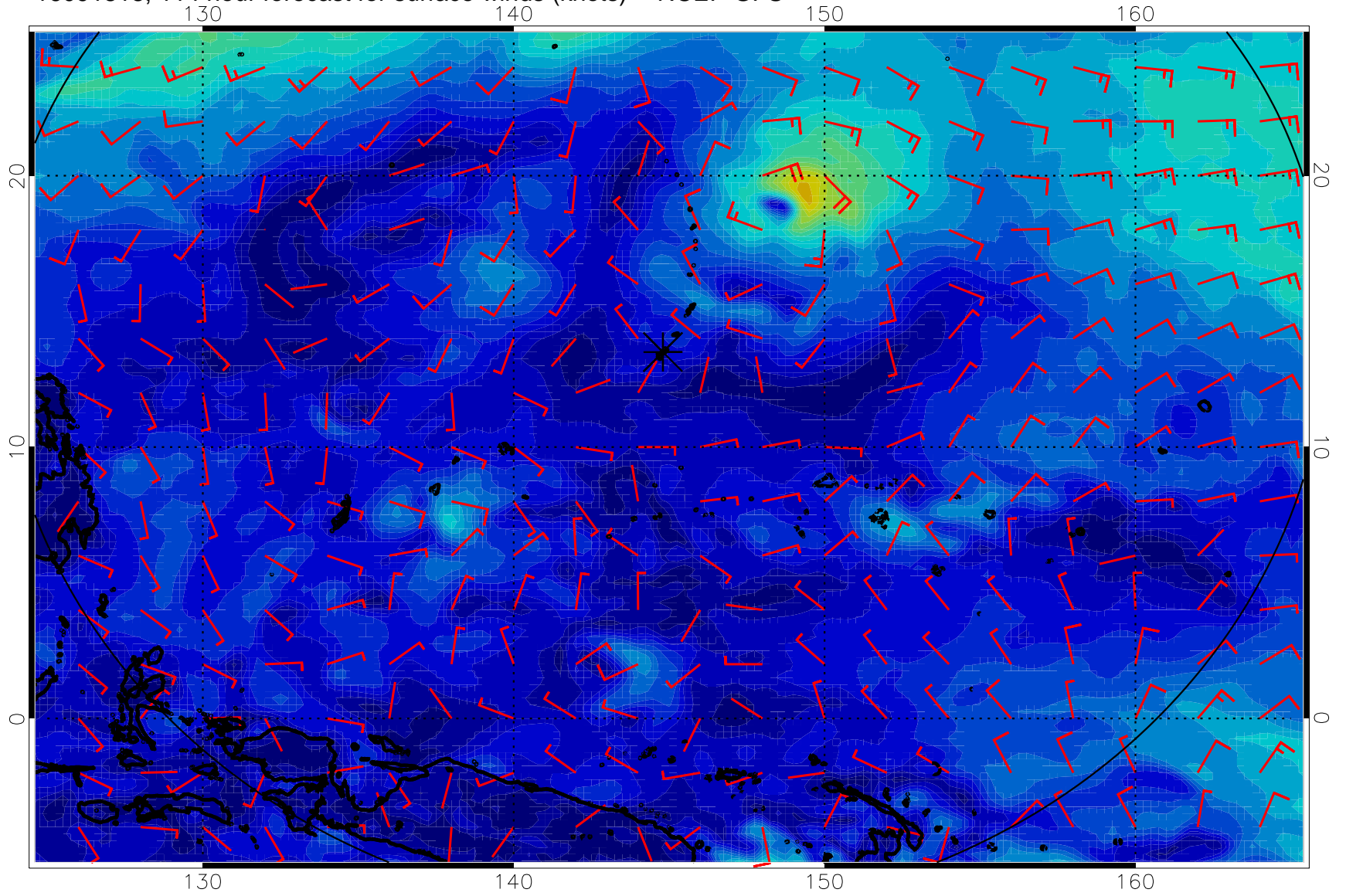
16091818, 114 hour forecast for surface winds (knots) -- NCEP GFS
