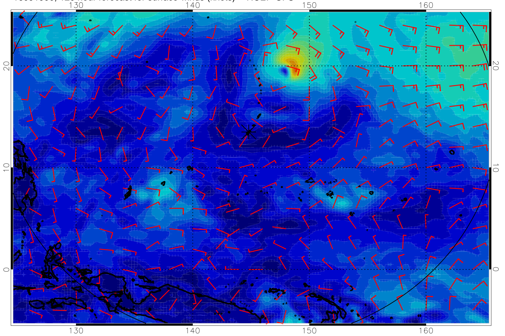
16091900, 120 hour forecast for surface winds (knots) -- NCEP GFS
