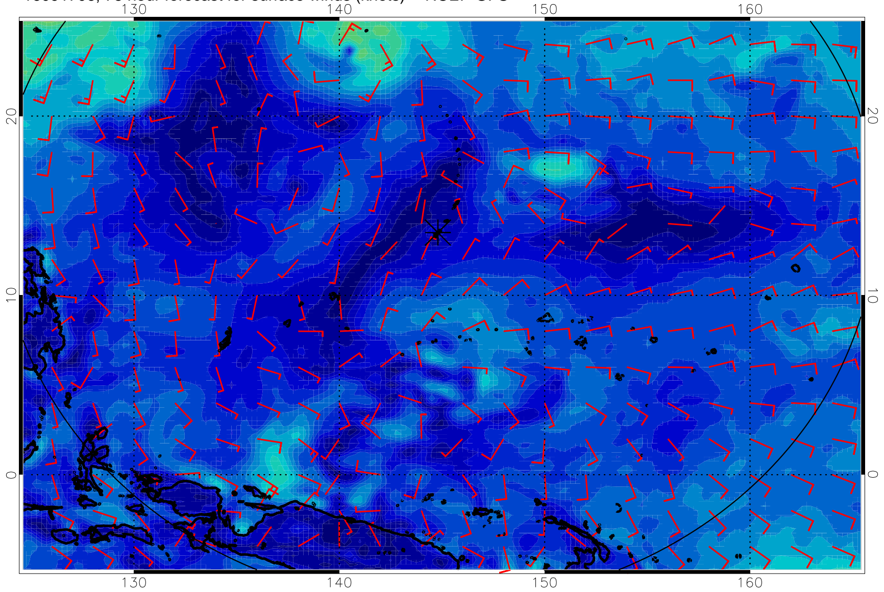
16091706, 78 hour forecast for surface winds (knots) -- NCEP GFS
