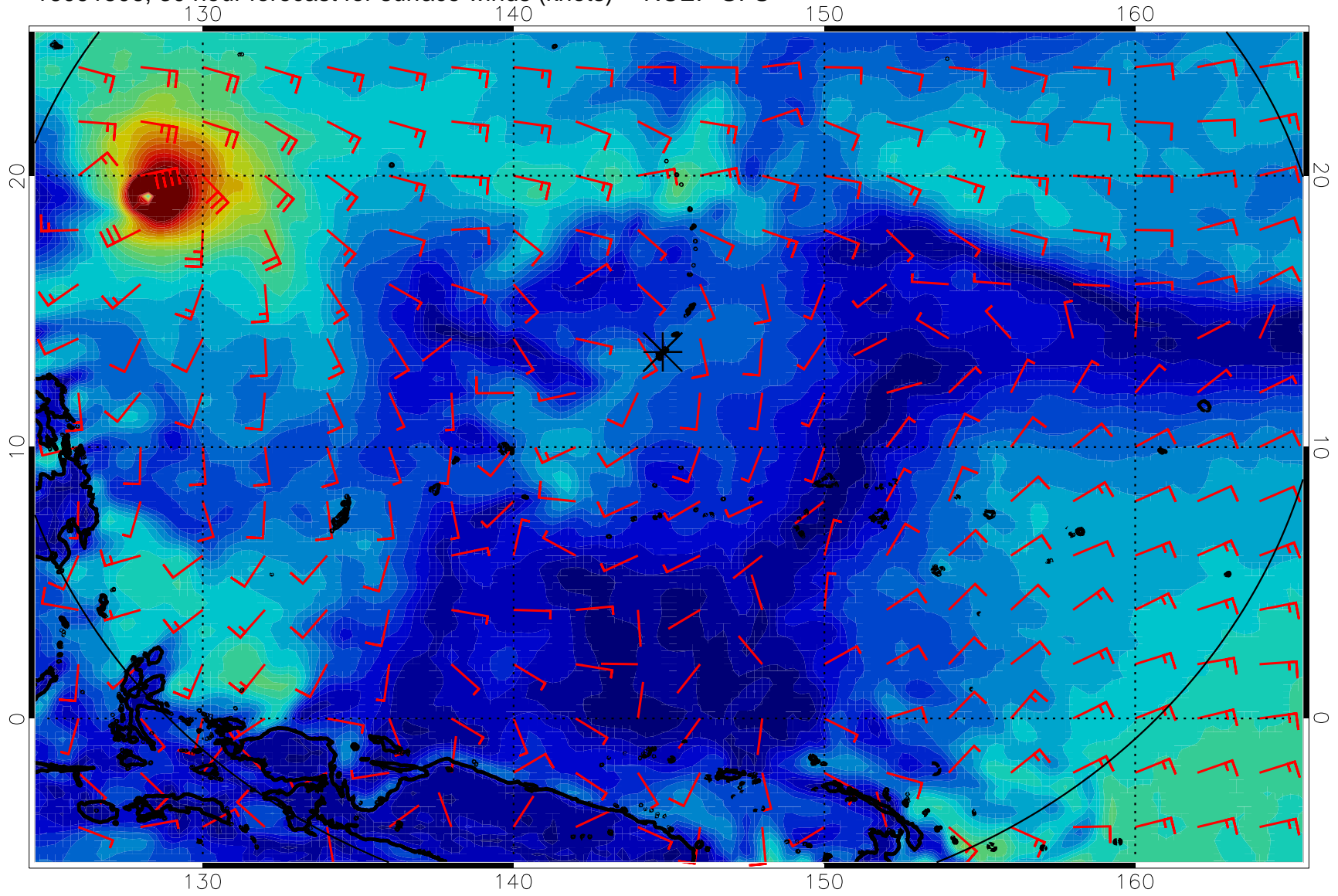
16091506, 30 hour forecast for surface winds (knots) -- NCEP GFS
