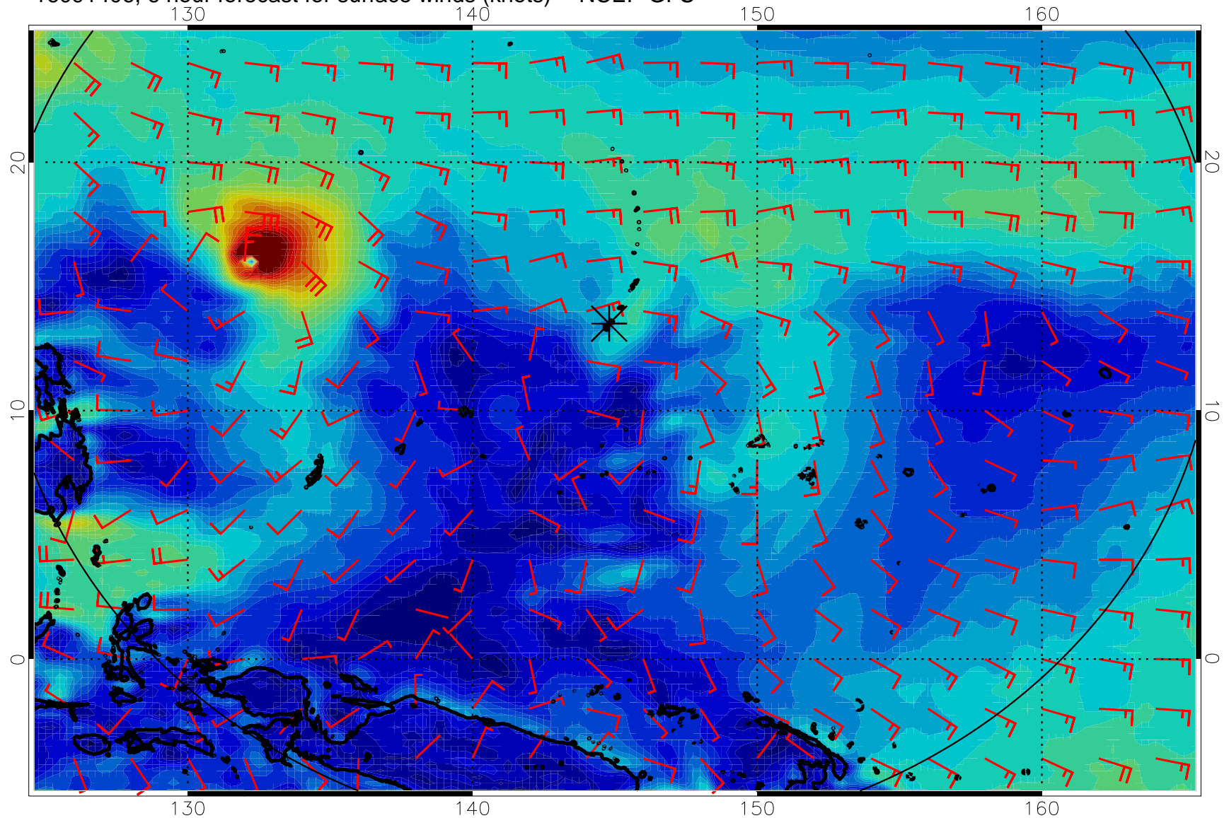
16091406, 6 hour forecast for surface winds (knots) -- NCEP GFS
