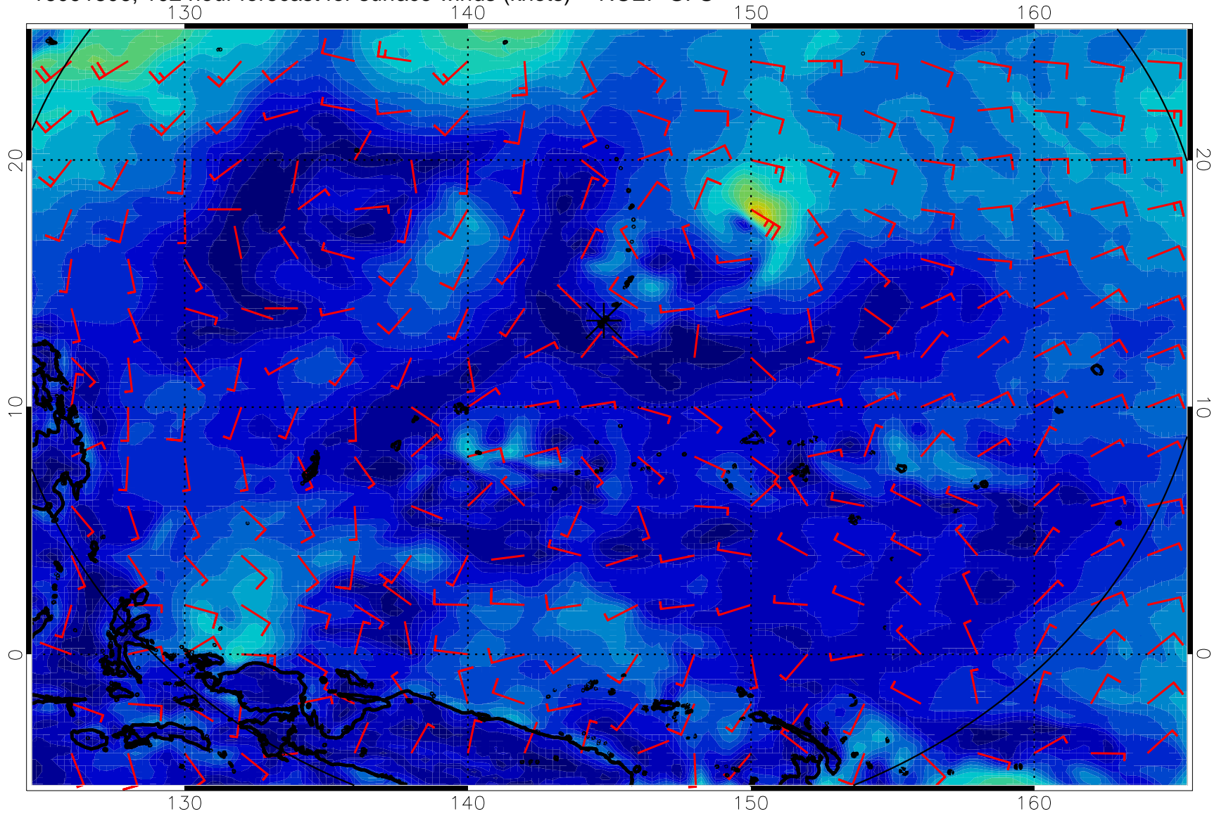
16091806, 102 hour forecast for surface winds (knots) -- NCEP GFS
