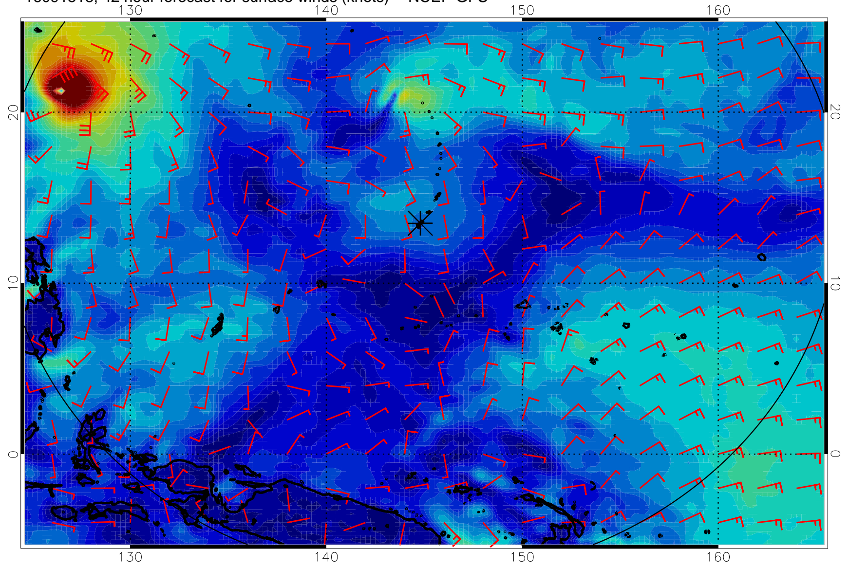
16091518, 42 hour forecast for surface winds (knots) -- NCEP GFS
