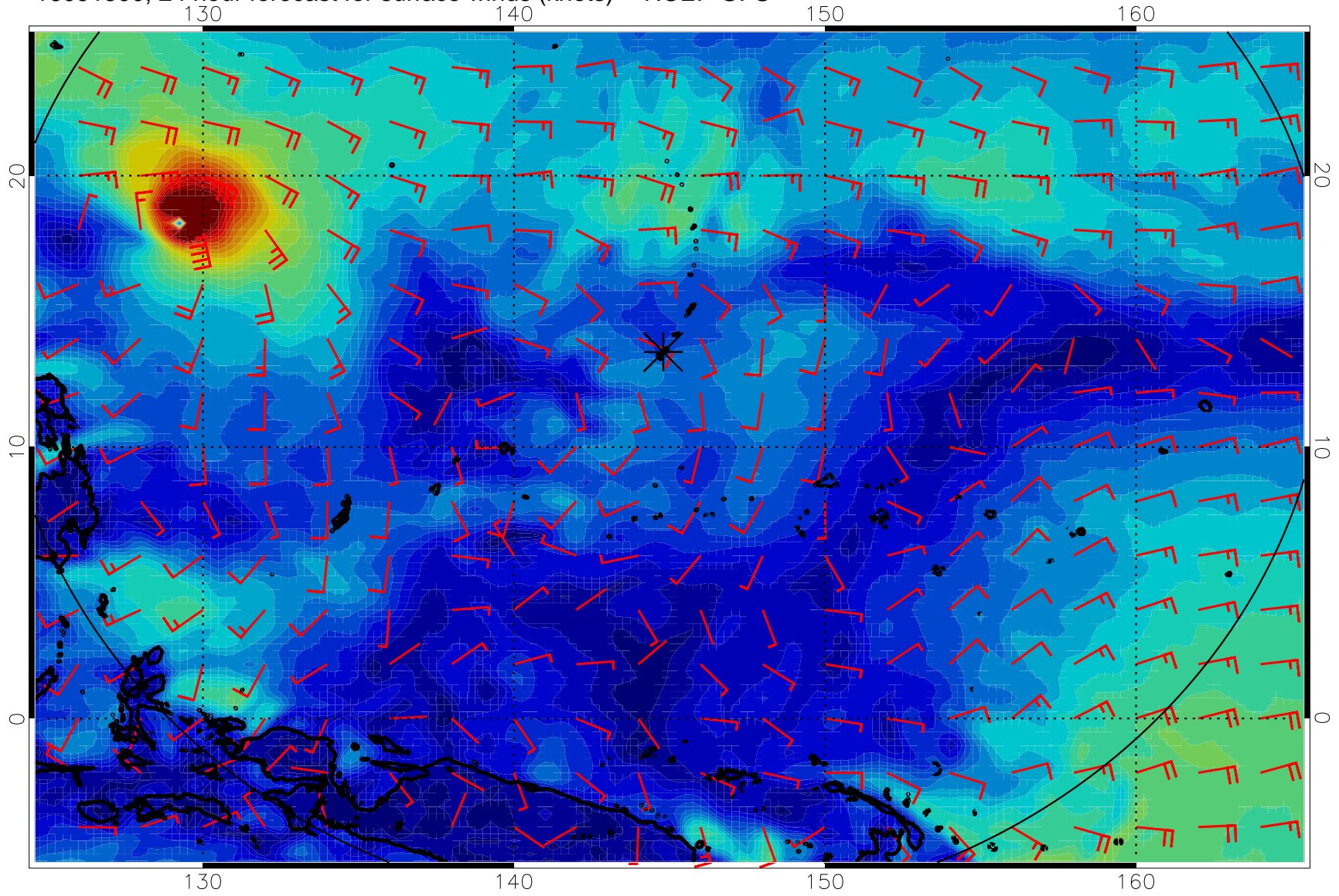
16091500, 24 hour forecast for surface winds (knots) -- NCEP GFS
