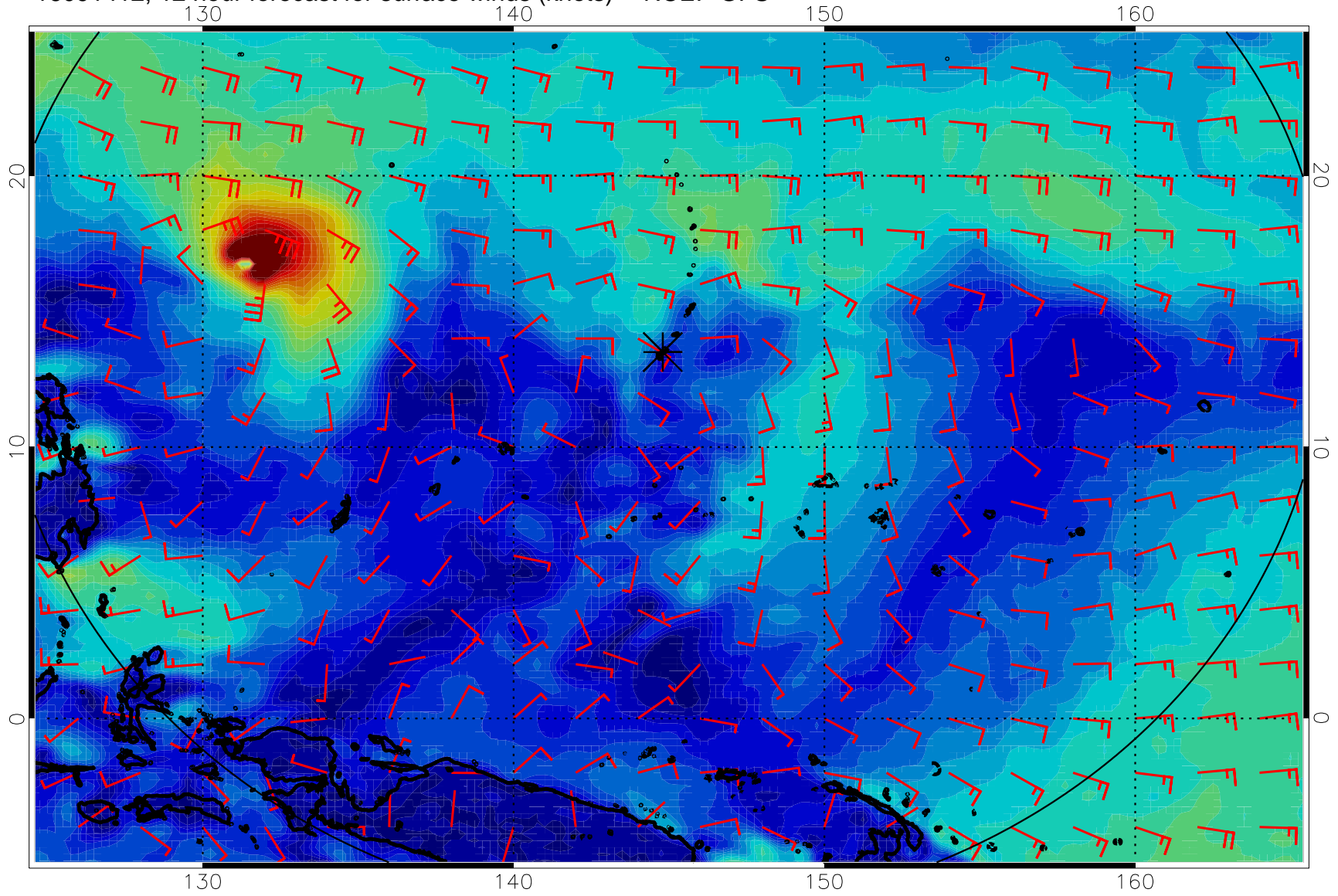
16091412, 12 hour forecast for surface winds (knots) -- NCEP GFS
