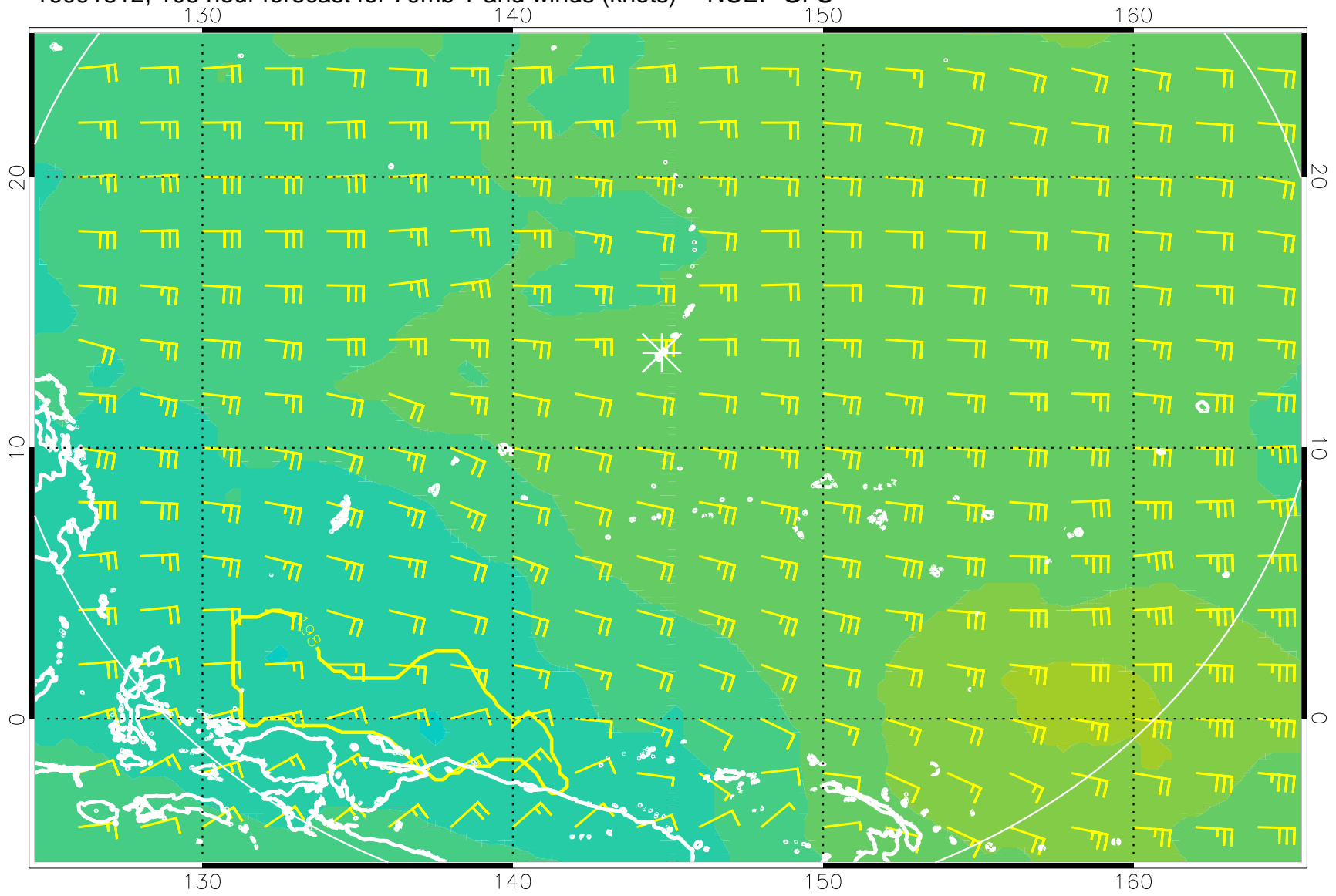
16091812, 108 hour forecast for 70mb T and winds (knots) -- NCEP GFS
