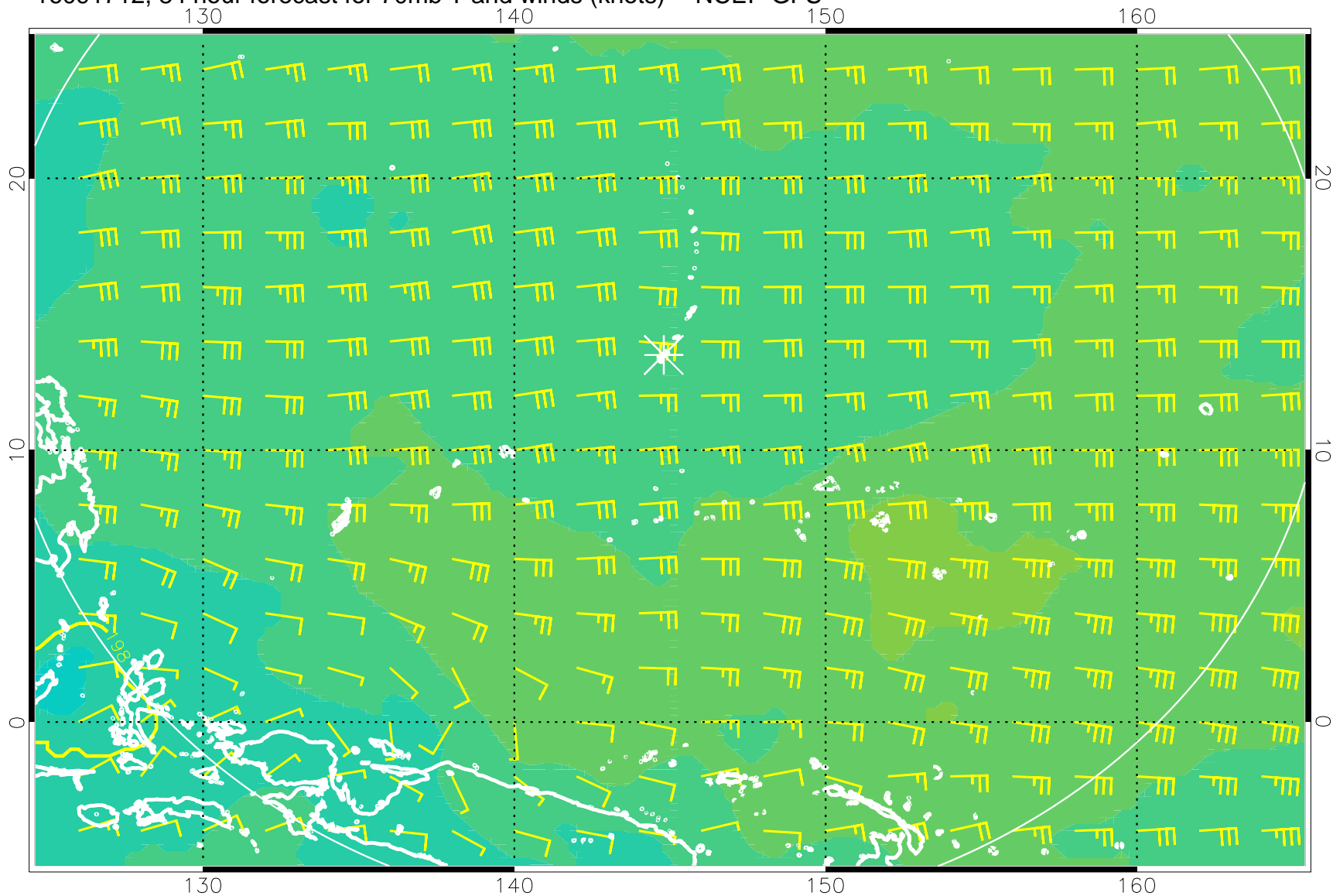
16091712, 84 hour forecast for 70mb T and winds (knots) -- NCEP GFS
