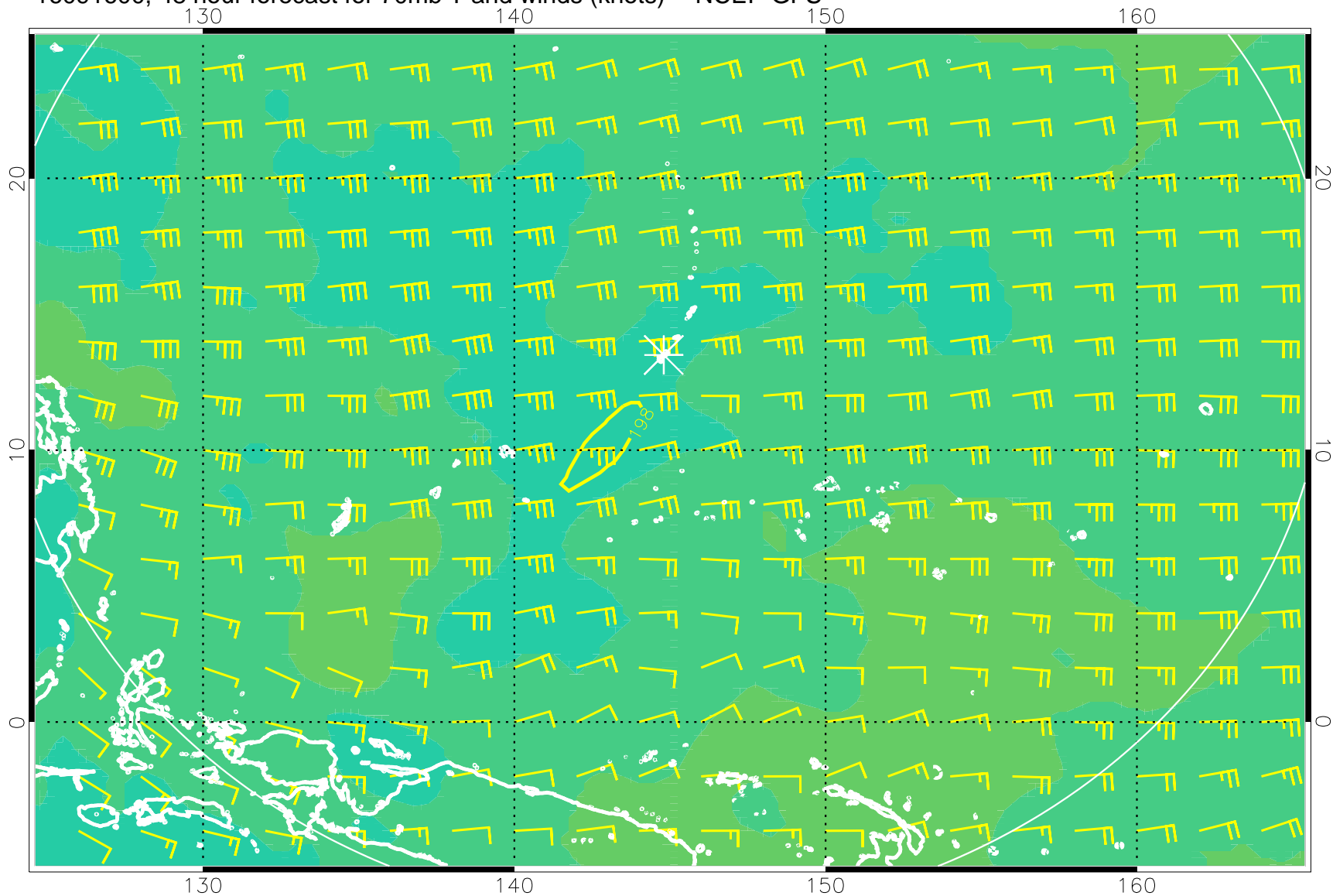
16091600, 48 hour forecast for 70mb T and winds (knots) -- NCEP GFS
