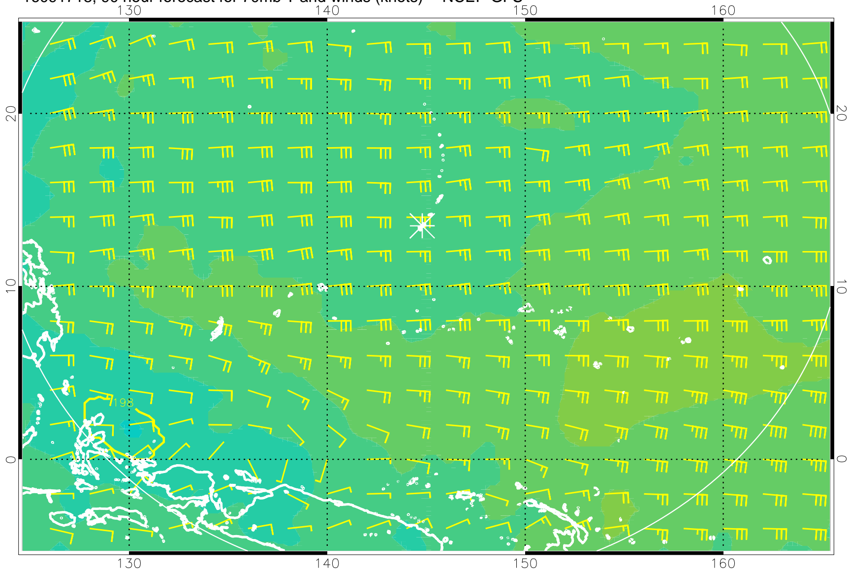
16091718, 90 hour forecast for 70mb T and winds (knots) -- NCEP GFS
