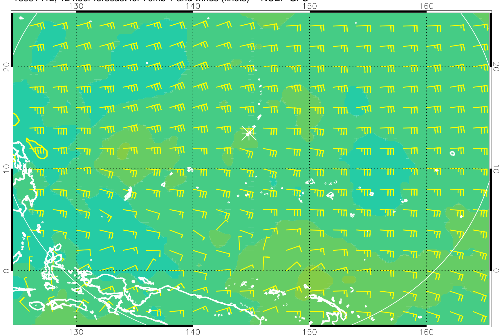
16091412, 12 hour forecast for 70mb T and winds (knots) -- NCEP GFS
