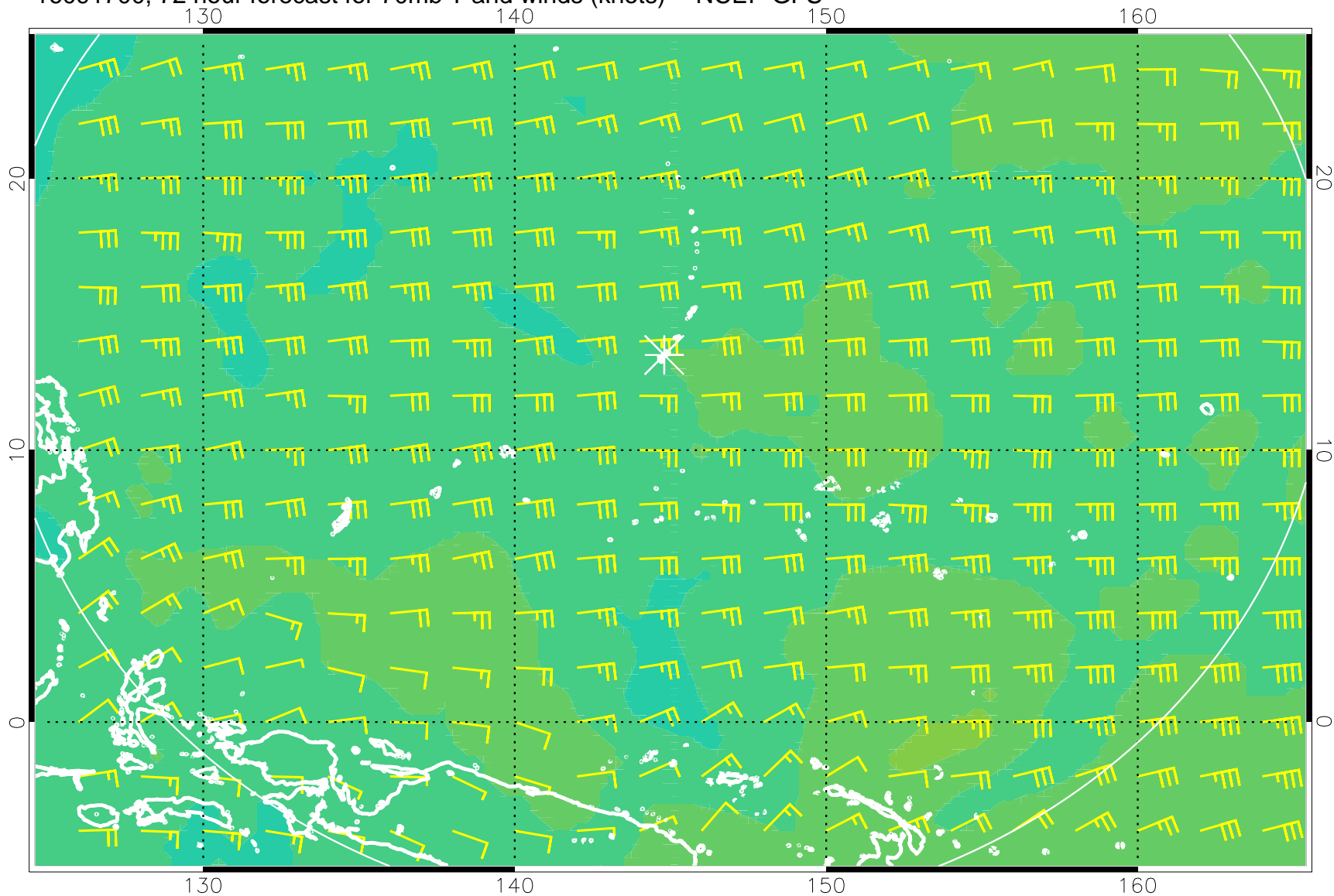
16091700, 72 hour forecast for 70mb T and winds (knots) -- NCEP GFS
