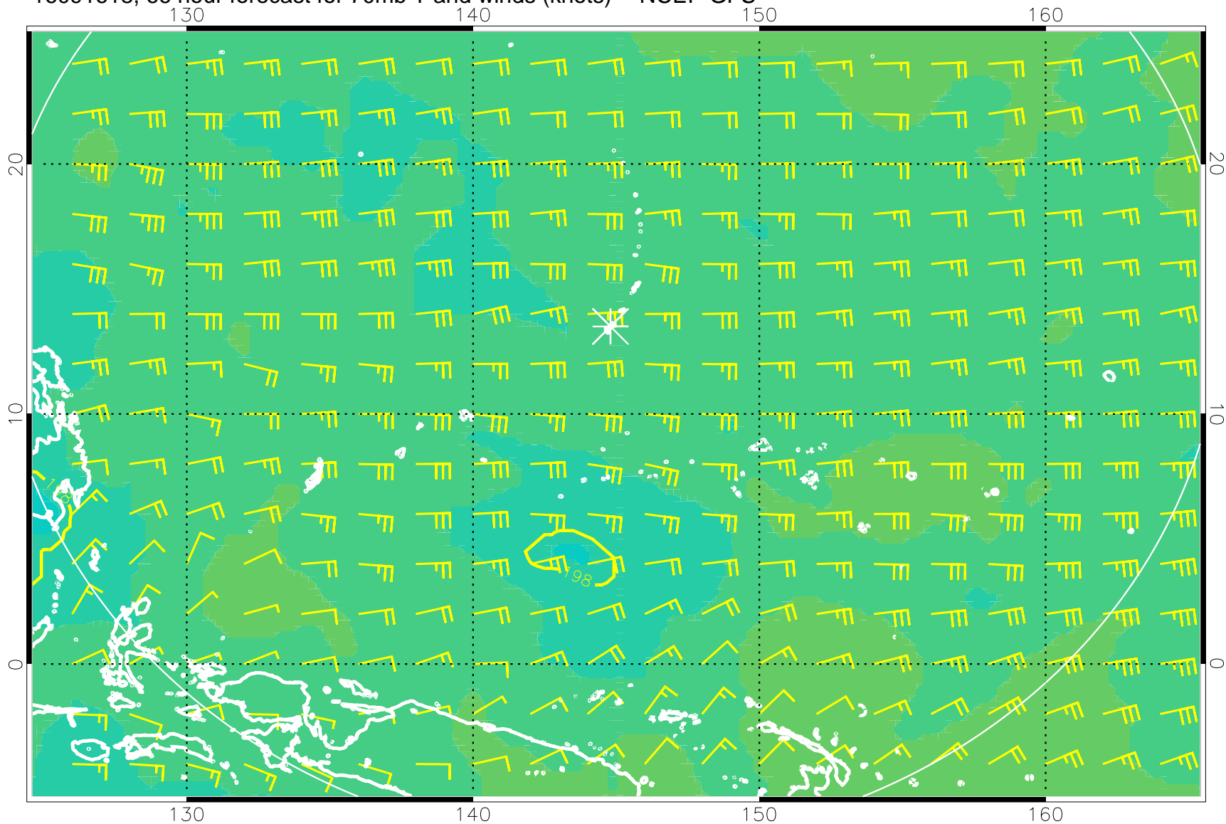
16091618, 66 hour forecast for 70mb T and winds (knots) -- NCEP GFS
