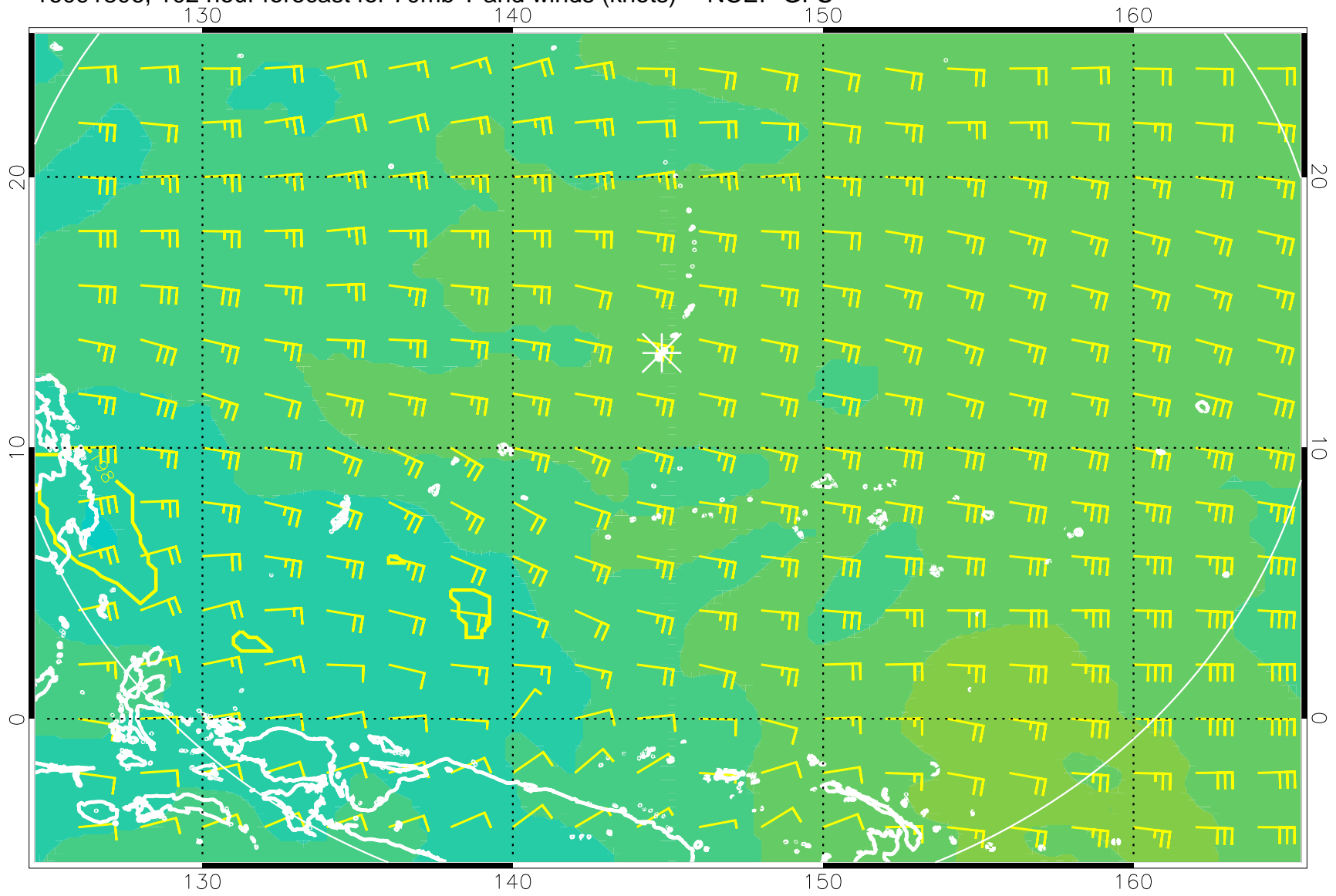
16091806, 102 hour forecast for 70mb T and winds (knots) -- NCEP GFS
