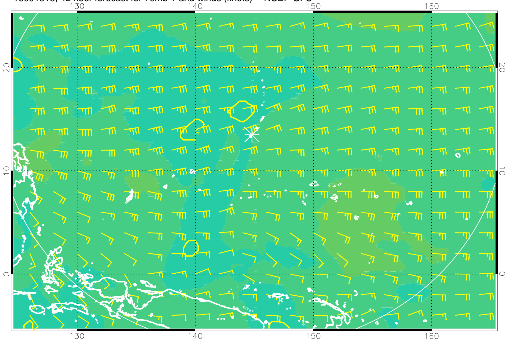
16091518, 42 hour forecast for 70mb T and winds (knots) -- NCEP GFS
