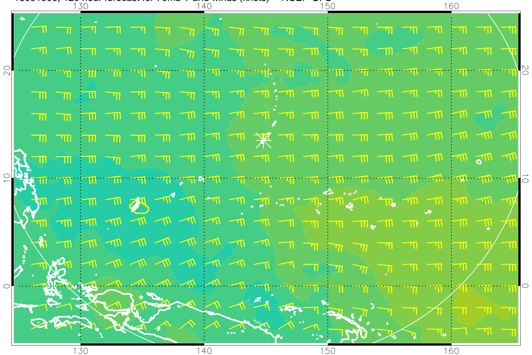
16091900, 120 hour forecast for 70mb T and winds (knots) -- NCEP GFS
