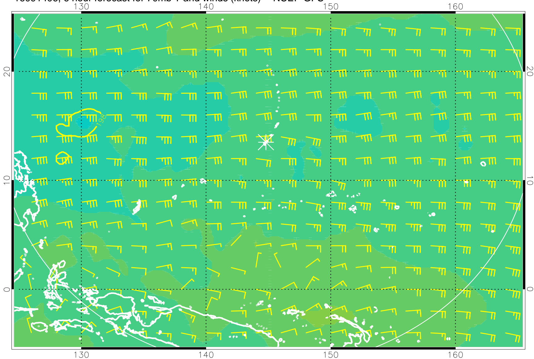
16091406, 6 hour forecast for 70mb T and winds (knots) -- NCEP GFS
