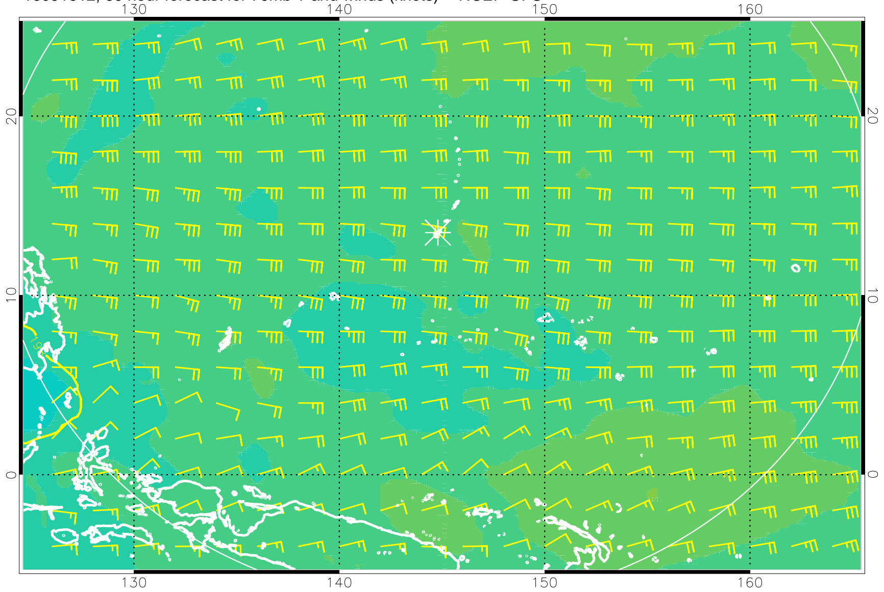
16091612, 60 hour forecast for 70mb T and winds (knots) -- NCEP GFS
