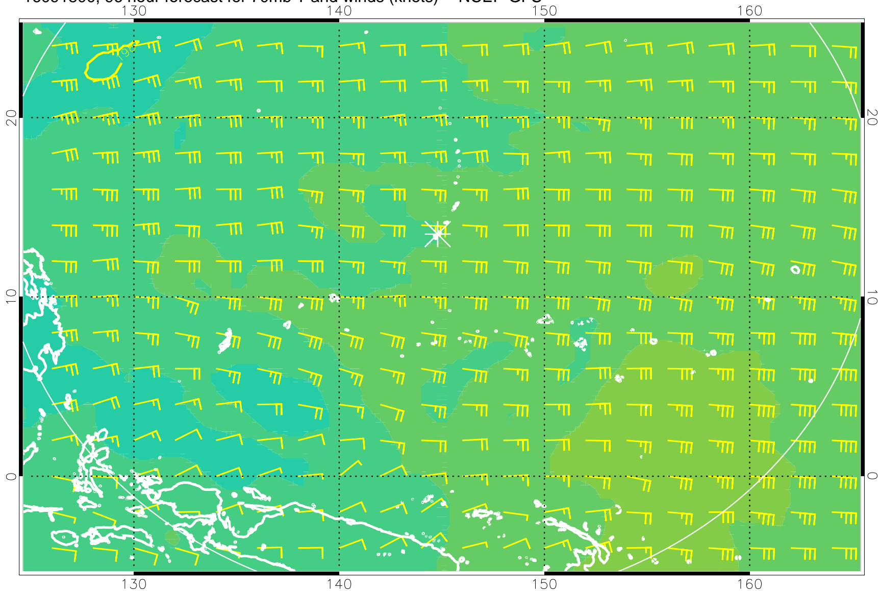
16091800, 96 hour forecast for 70mb T and winds (knots) -- NCEP GFS
