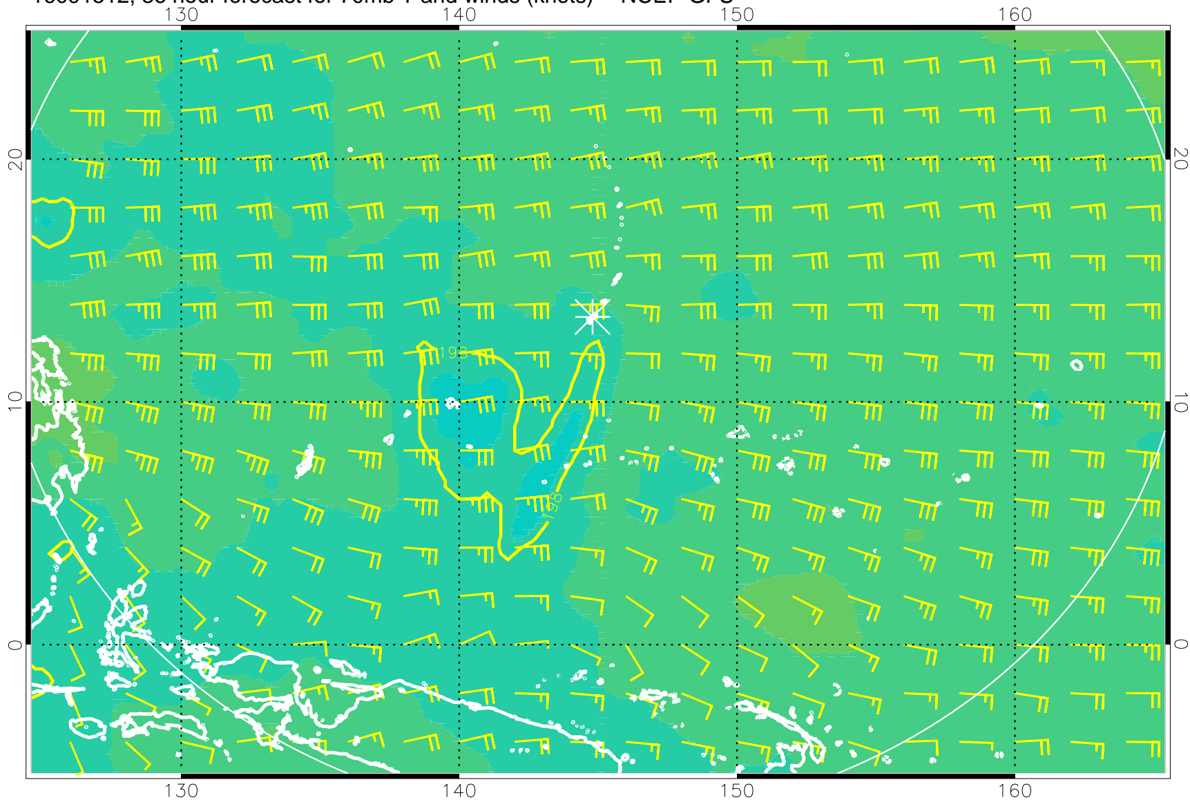
16091512, 36 hour forecast for 70mb T and winds (knots) -- NCEP GFS
