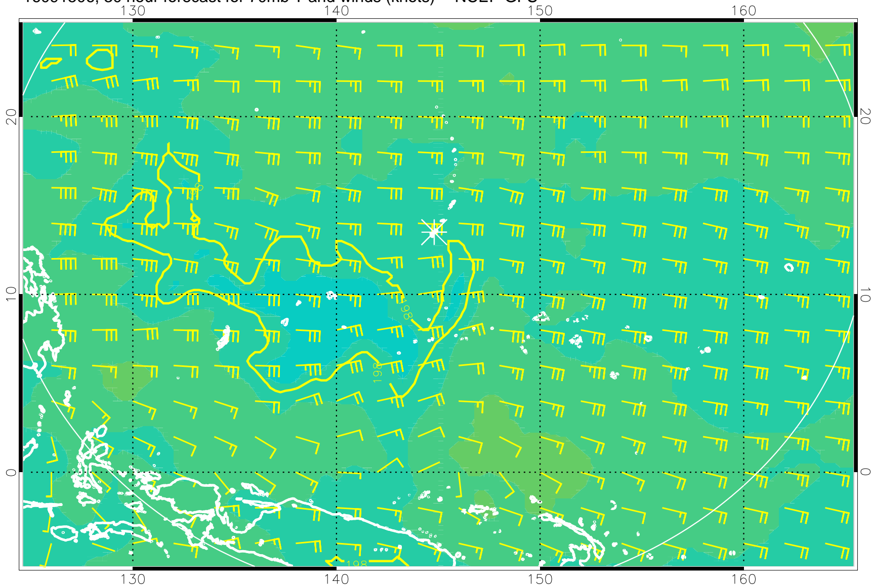
16091506, 30 hour forecast for 70mb T and winds (knots) -- NCEP GFS
