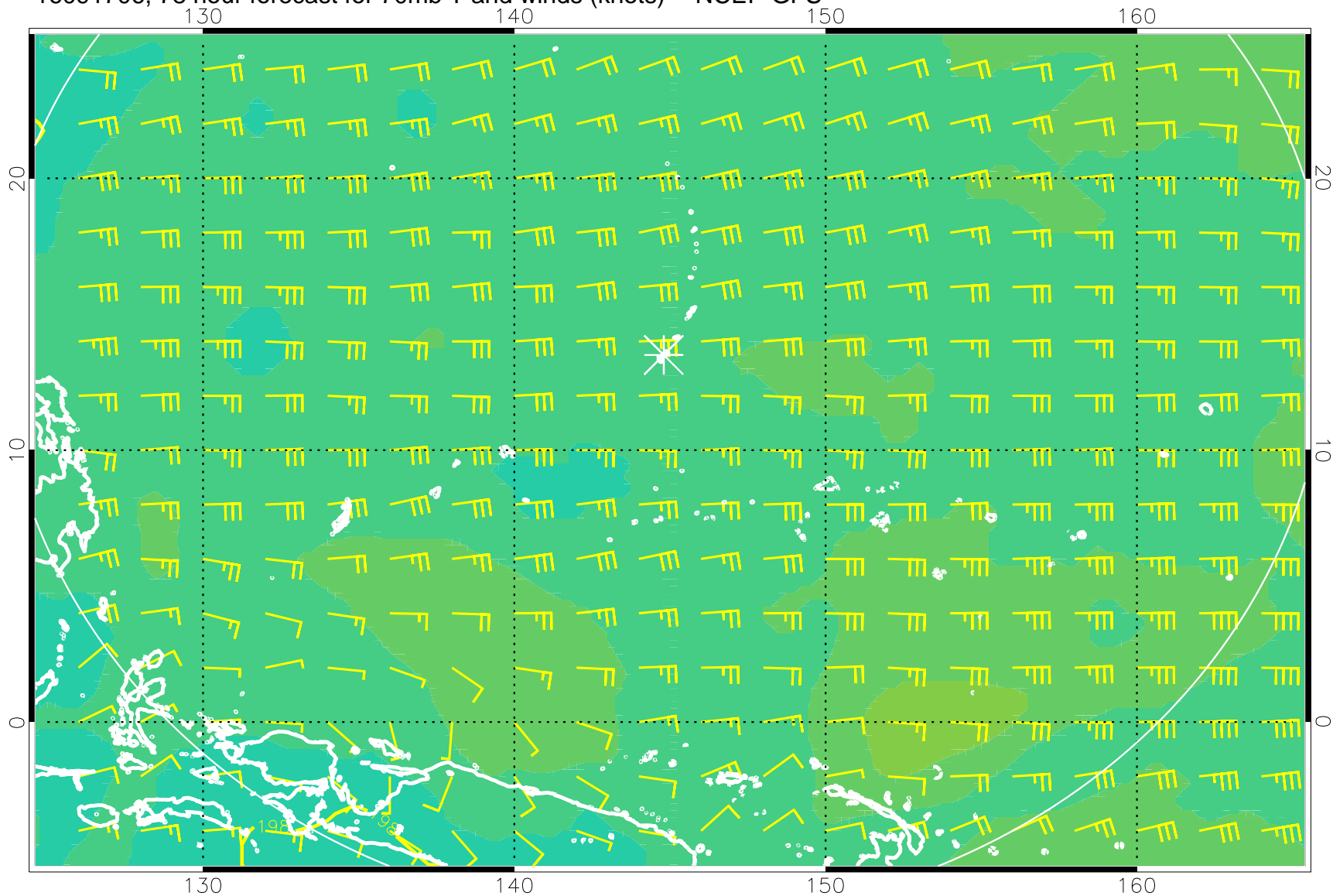
16091706, 78 hour forecast for 70mb T and winds (knots) -- NCEP GFS
