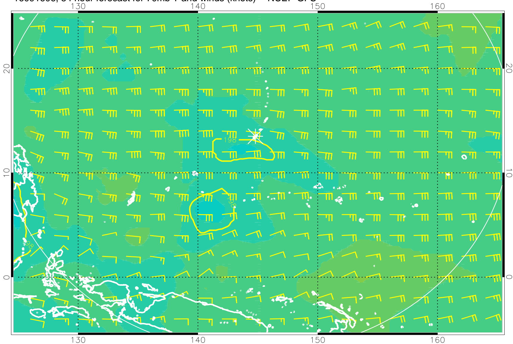
16091606, 54 hour forecast for 70mb T and winds (knots) -- NCEP GFS
