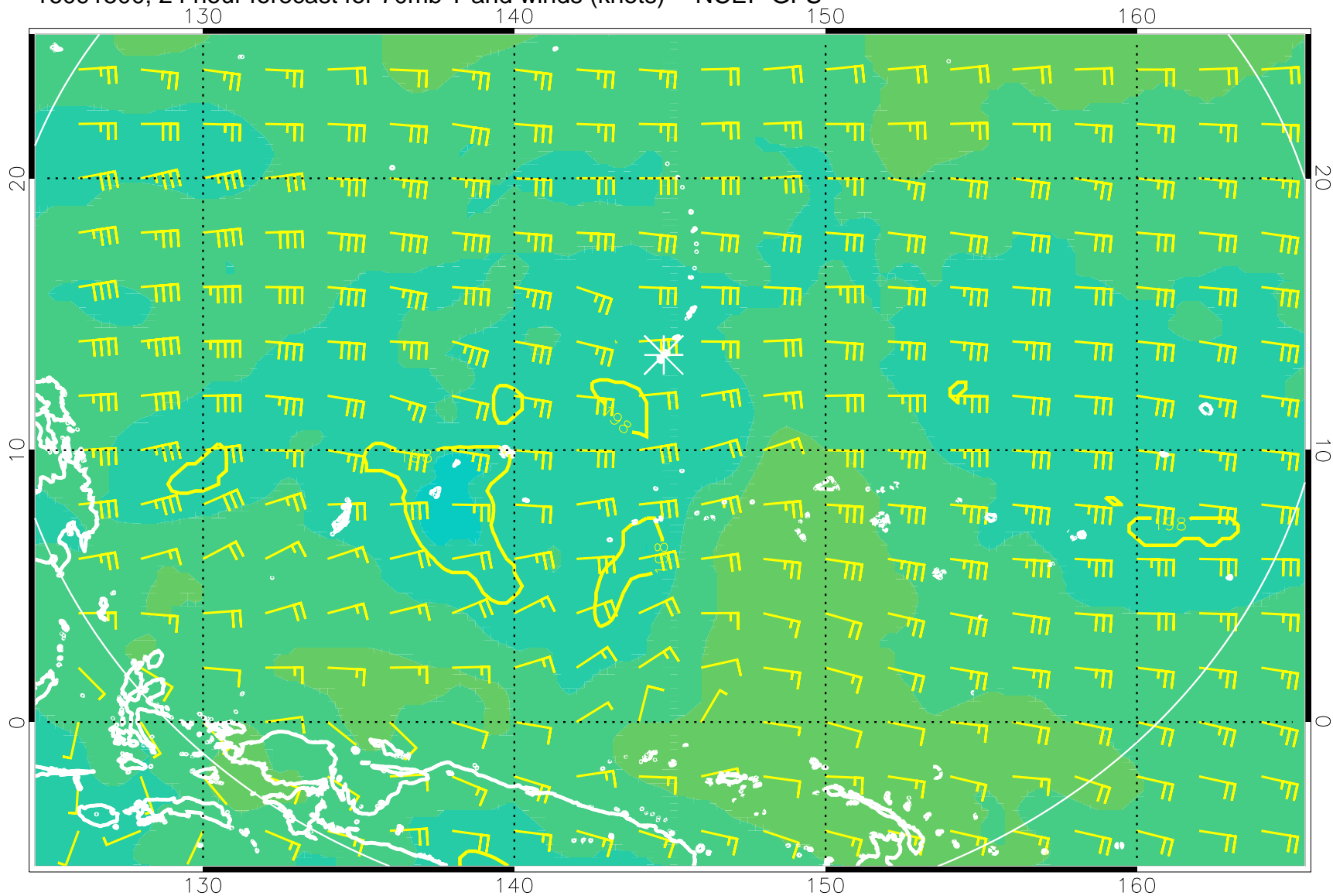
16091500, 24 hour forecast for 70mb T and winds (knots) -- NCEP GFS
