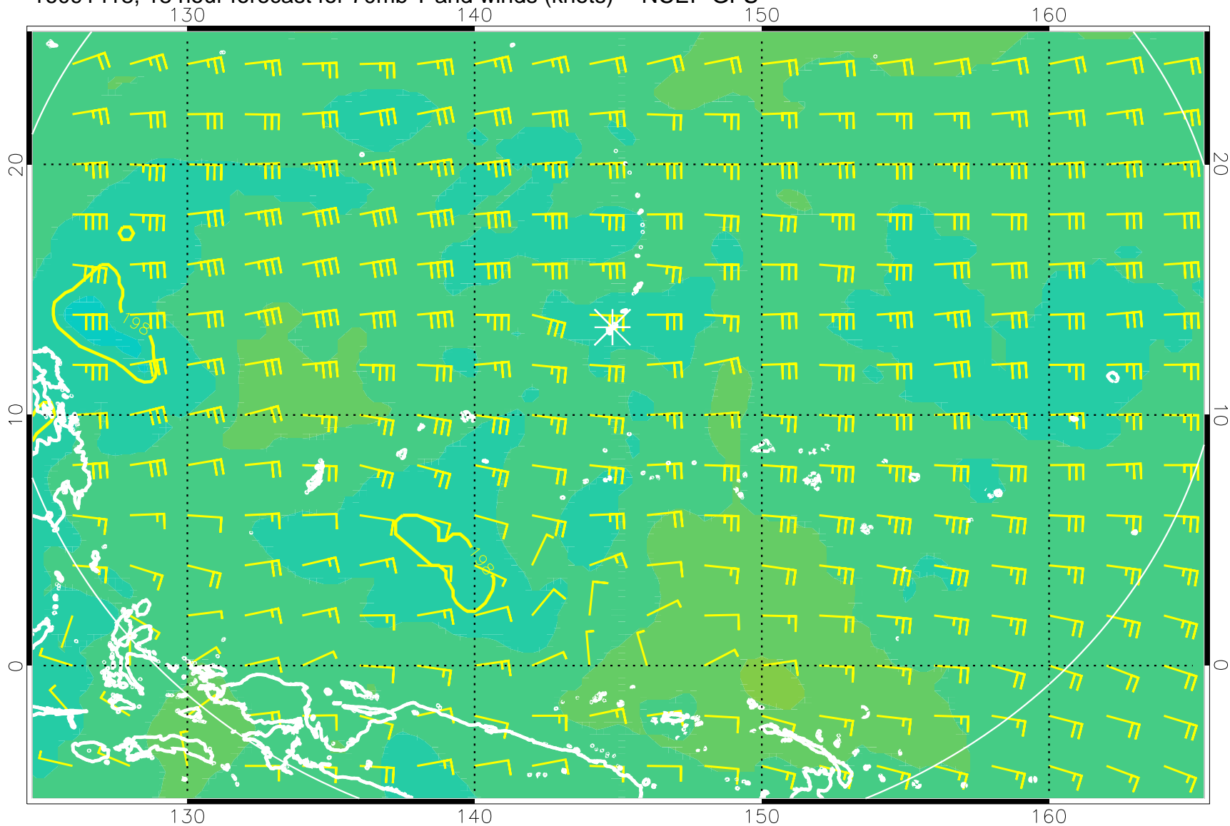
16091418, 18 hour forecast for 70mb T and winds (knots) -- NCEP GFS
