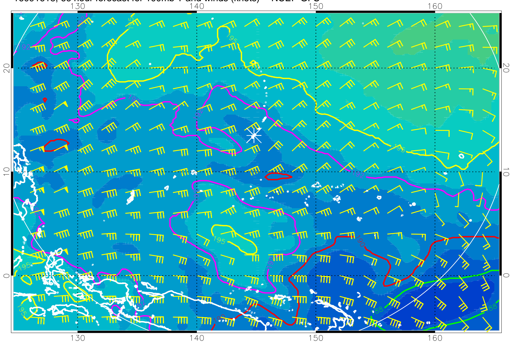
16091618, 66 hour forecast for 100mb T and winds (knots) -- NCEP GFS
