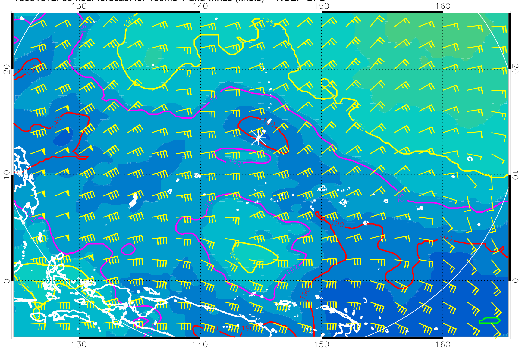
16091612, 60 hour forecast for 100mb T and winds (knots) -- NCEP GFS
