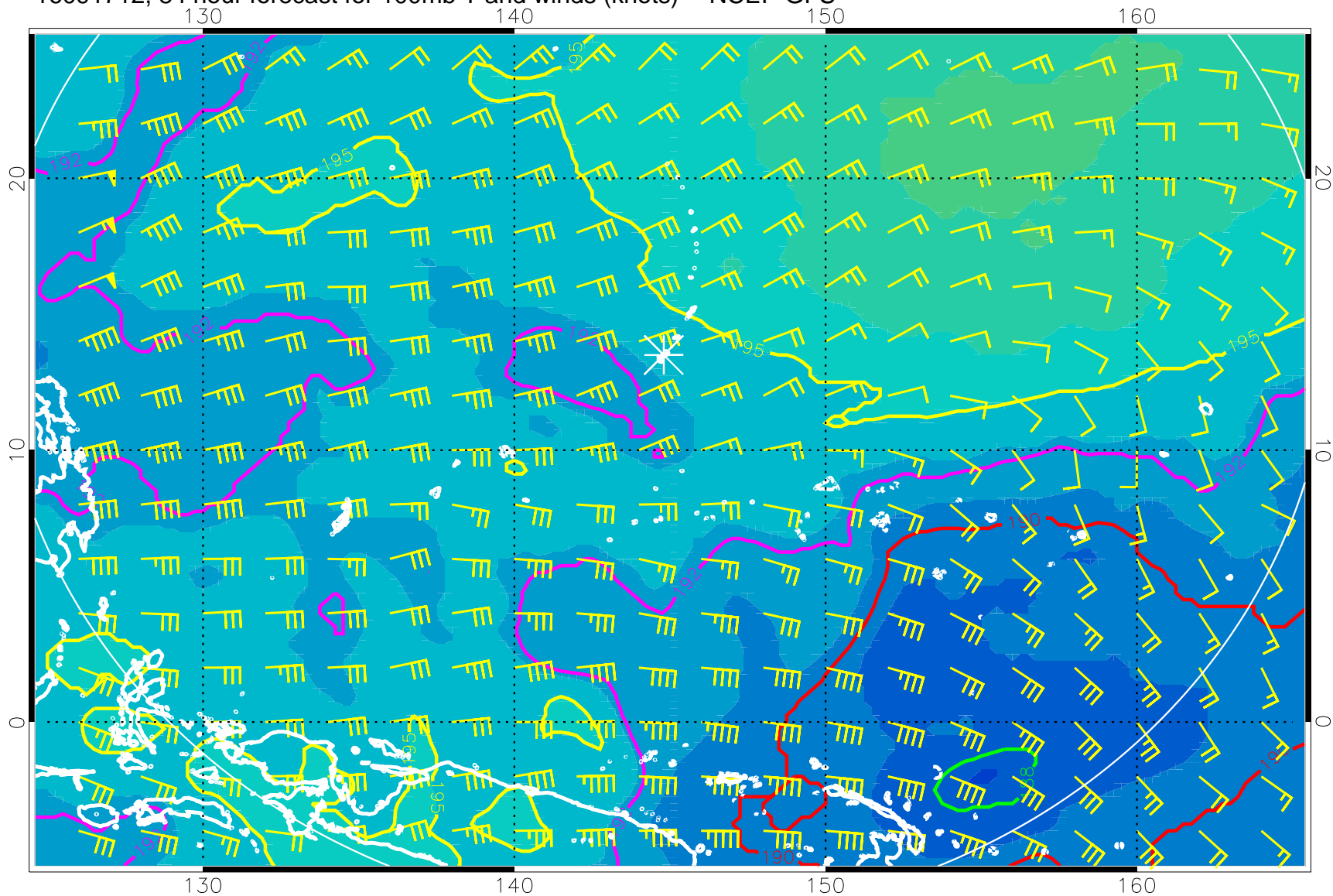
16091712, 84 hour forecast for 100mb T and winds (knots) -- NCEP GFS
