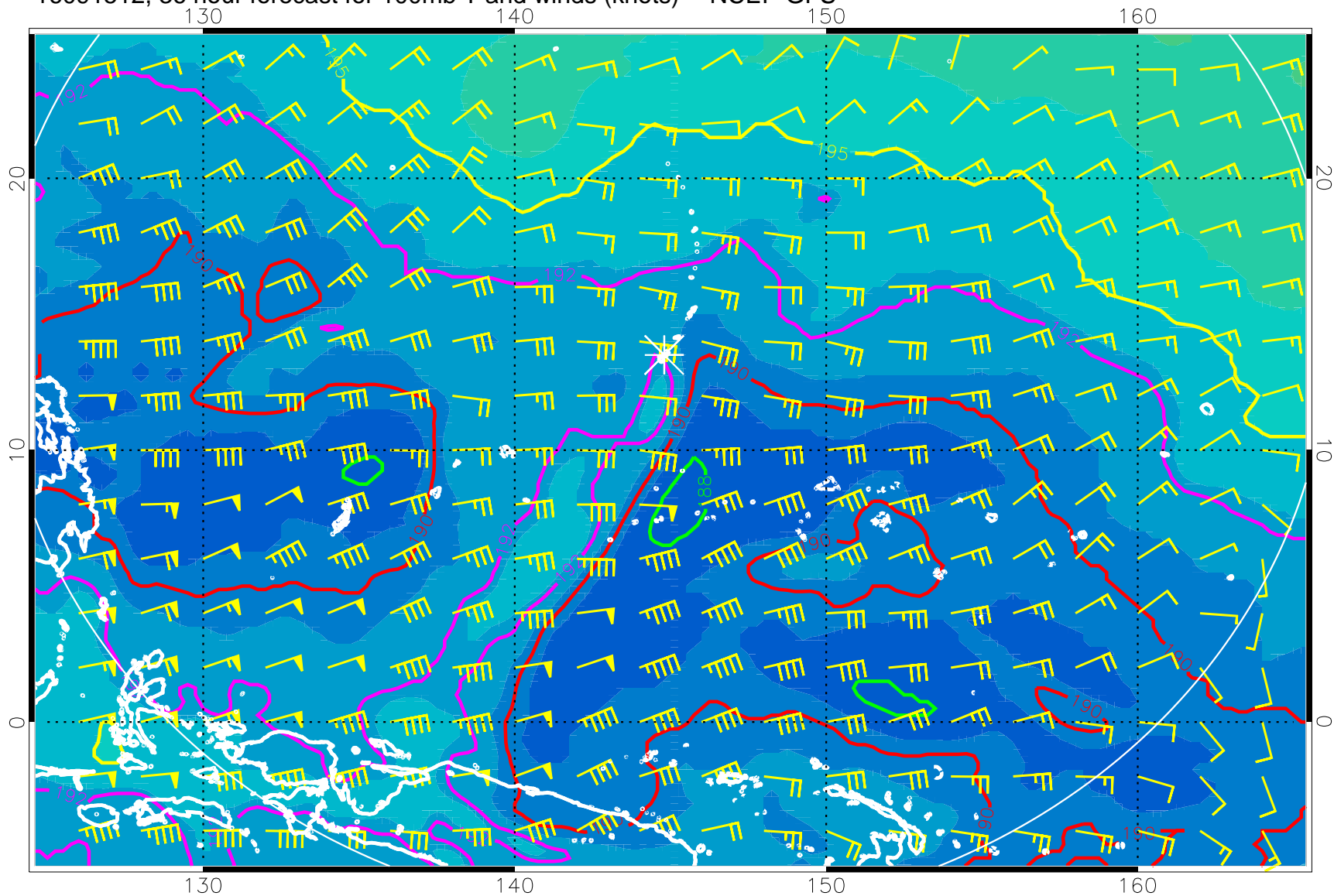
16091512, 36 hour forecast for 100mb T and winds (knots) -- NCEP GFS
