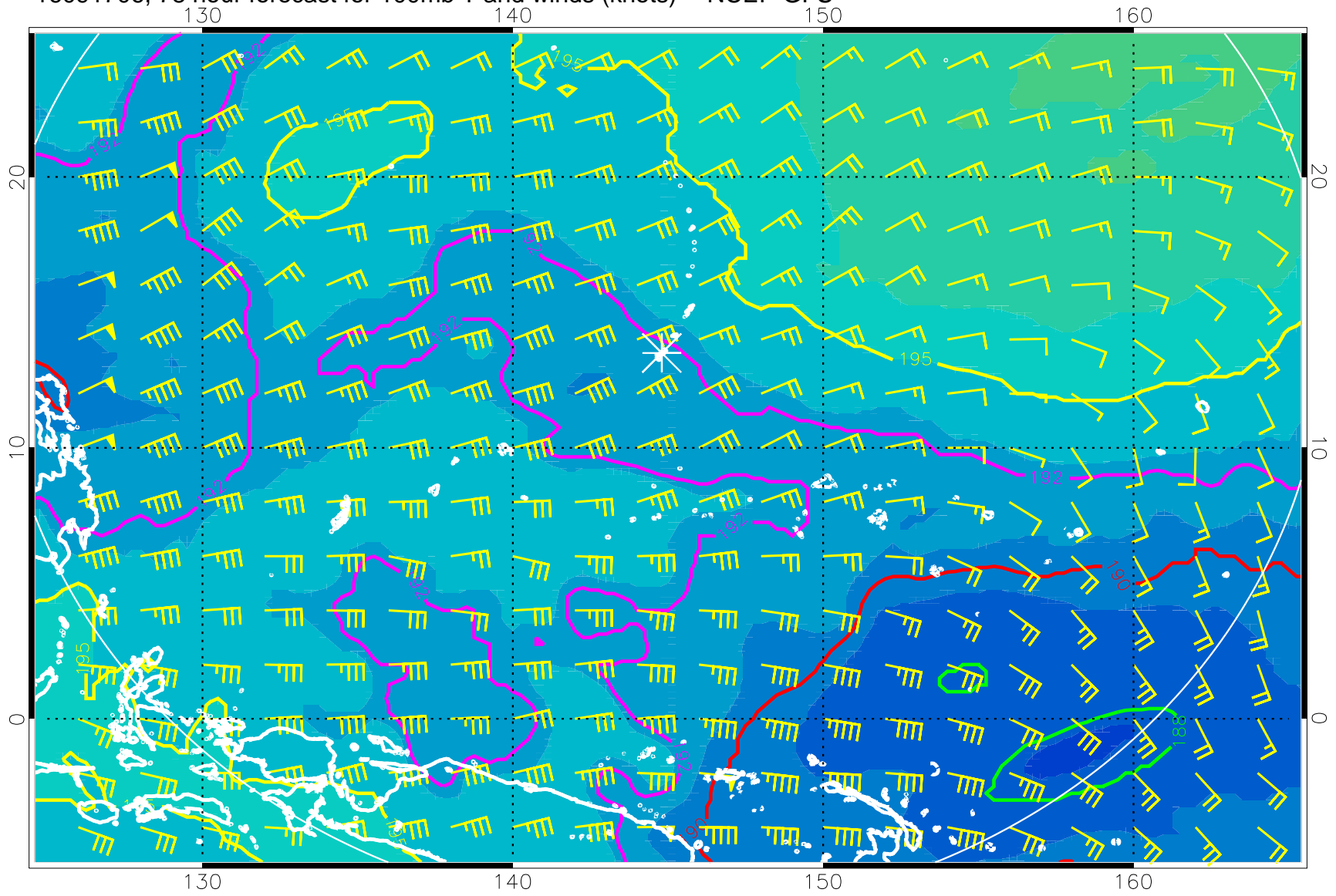
16091706, 78 hour forecast for 100mb T and winds (knots) -- NCEP GFS
