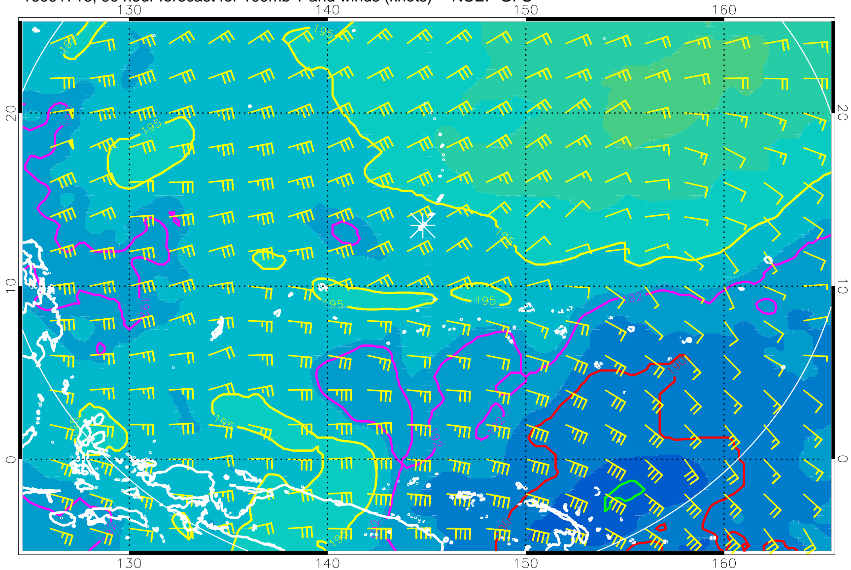
16091718, 90 hour forecast for 100mb T and winds (knots) -- NCEP GFS
