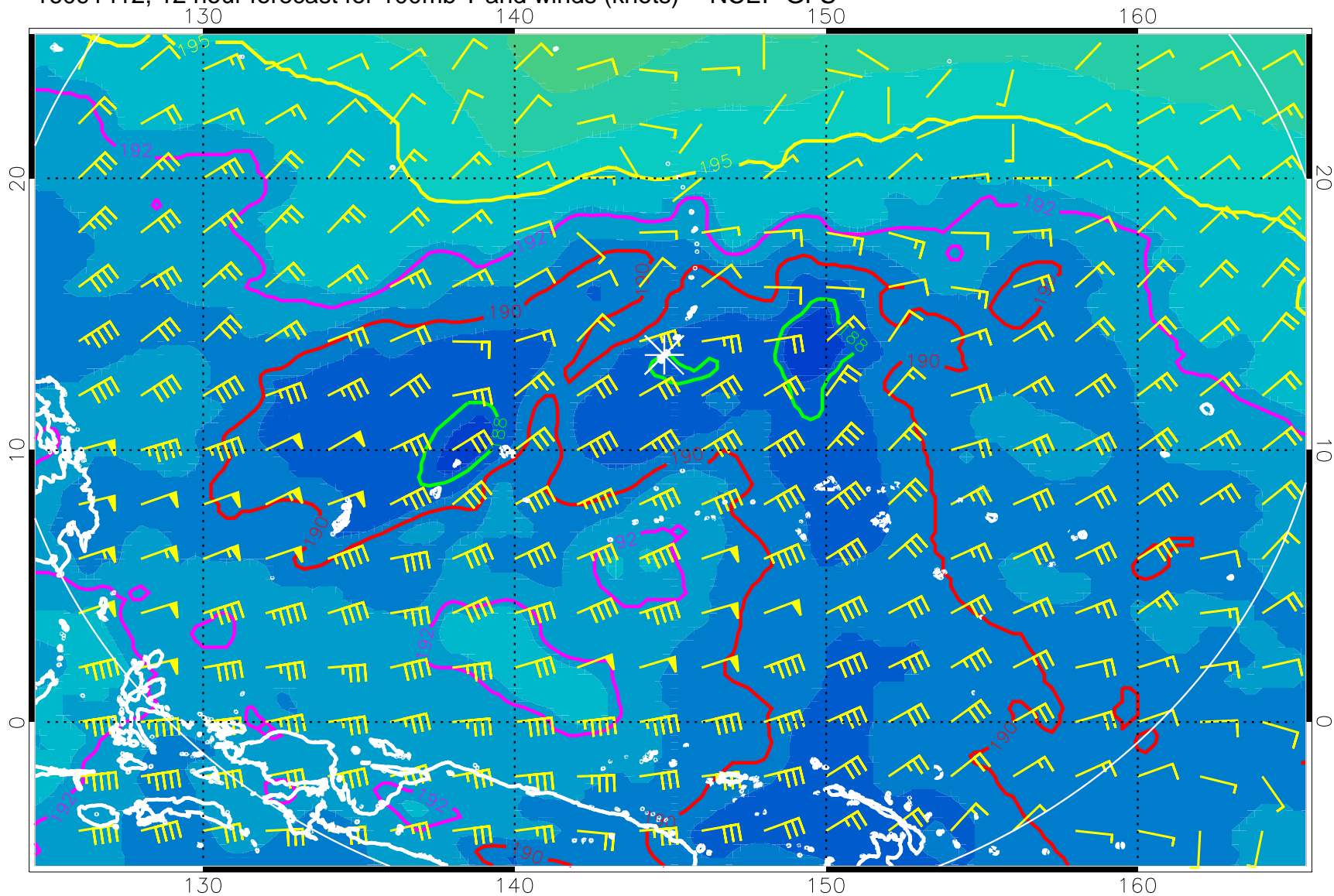
16091412, 12 hour forecast for 100mb T and winds (knots) -- NCEP GFS
