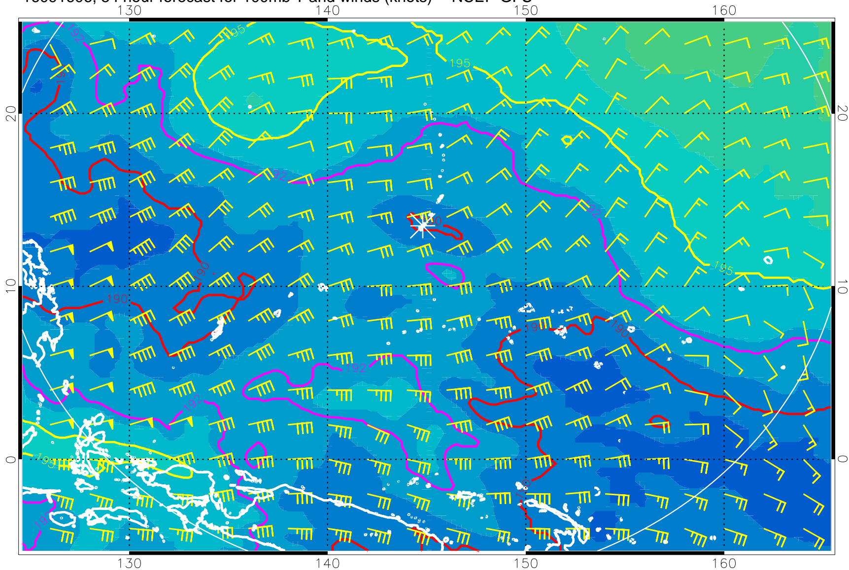
16091606, 54 hour forecast for 100mb T and winds (knots) -- NCEP GFS
