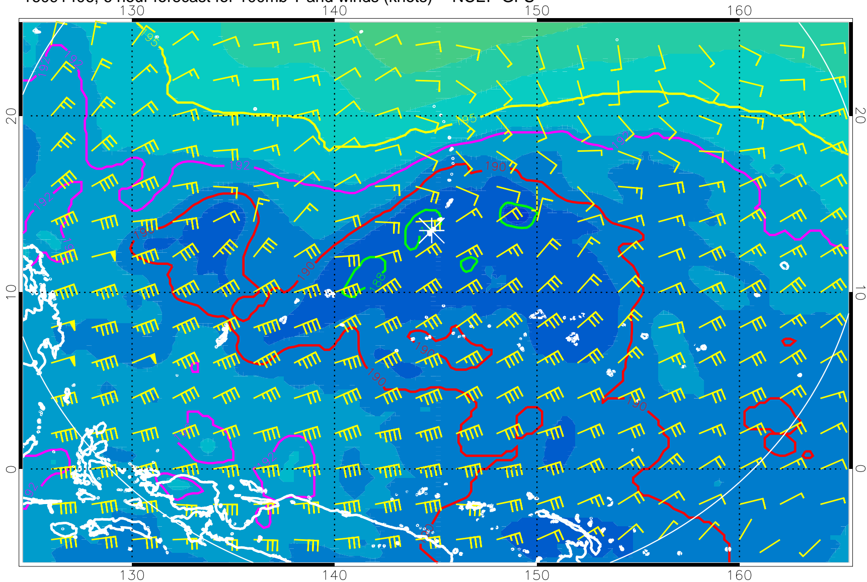
16091406, 6 hour forecast for 100mb T and winds (knots) -- NCEP GFS
