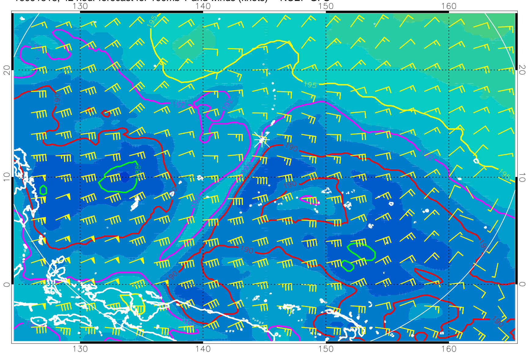
16091518, 42 hour forecast for 100mb T and winds (knots) -- NCEP GFS
