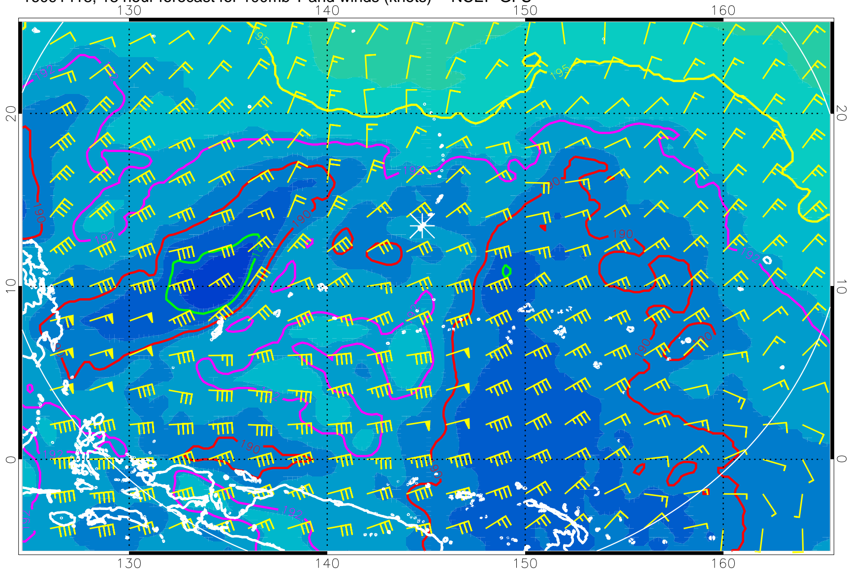
16091418, 18 hour forecast for 100mb T and winds (knots) -- NCEP GFS
