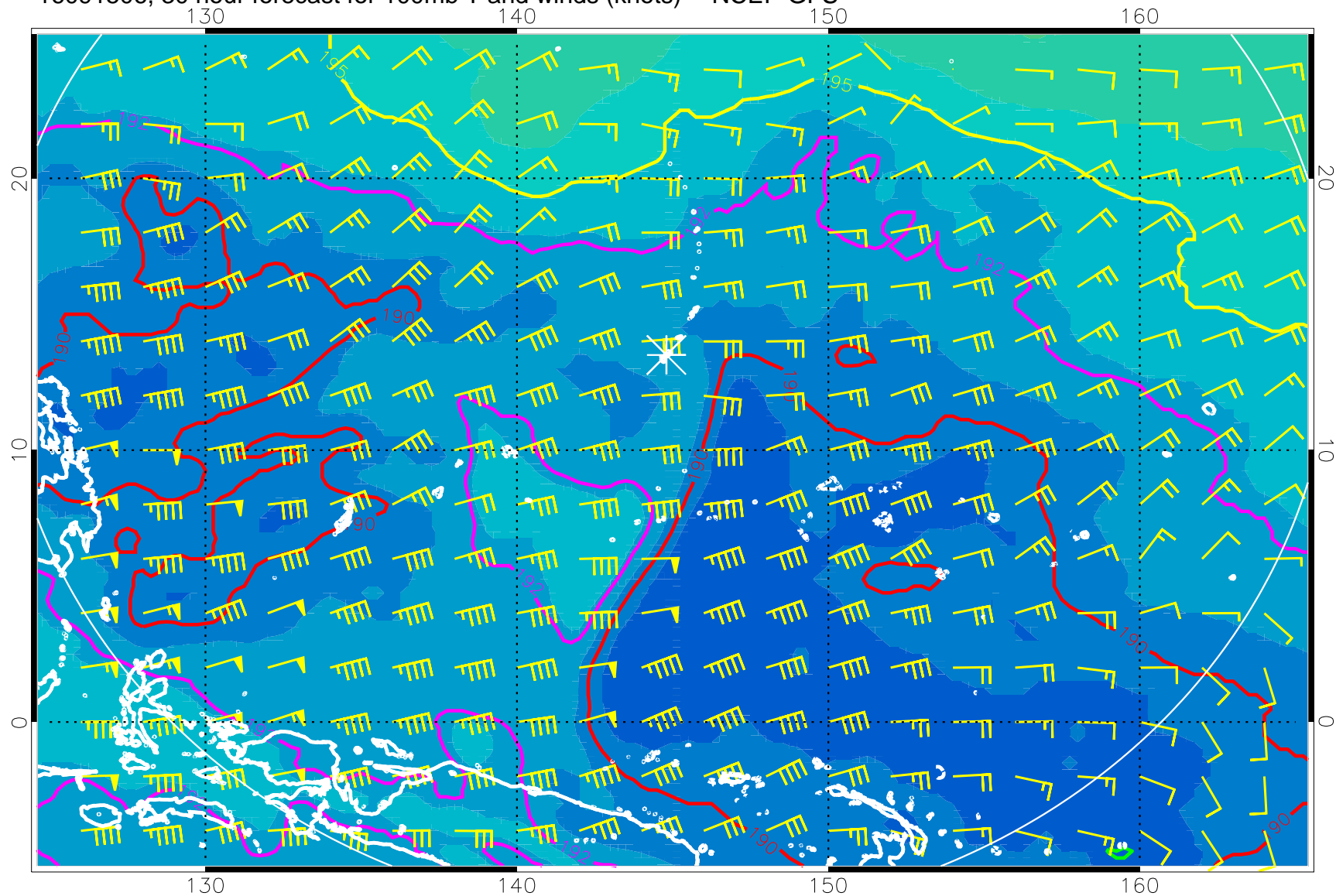
16091506, 30 hour forecast for 100mb T and winds (knots) -- NCEP GFS
