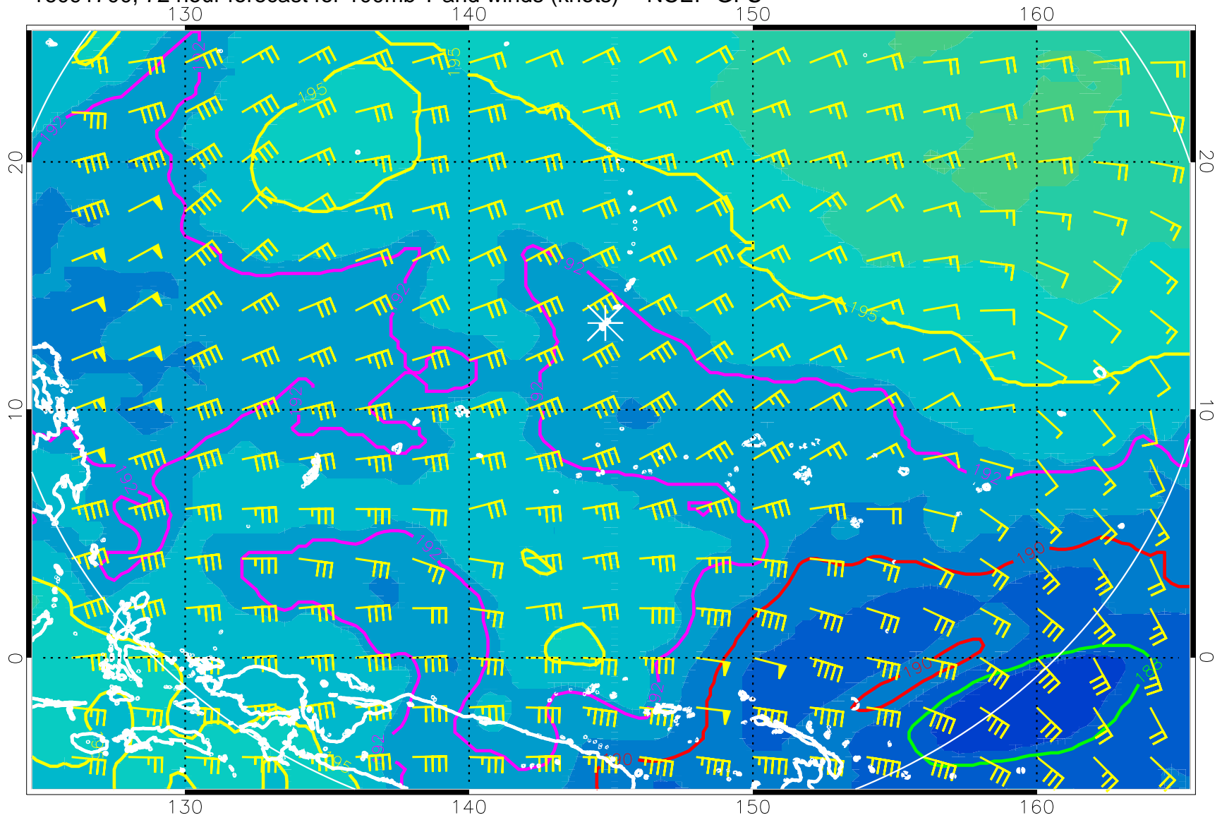
16091700, 72 hour forecast for 100mb T and winds (knots) -- NCEP GFS
