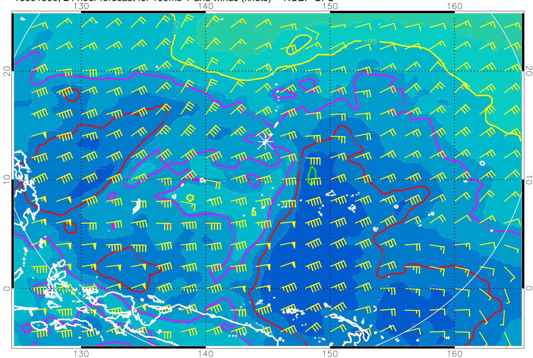
16091500, 24 hour forecast for 100mb T and winds (knots) -- NCEP GFS
