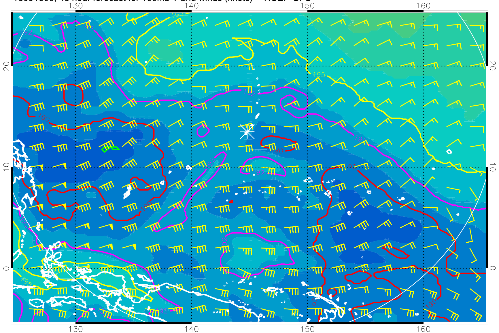
16091600, 48 hour forecast for 100mb T and winds (knots) -- NCEP GFS
