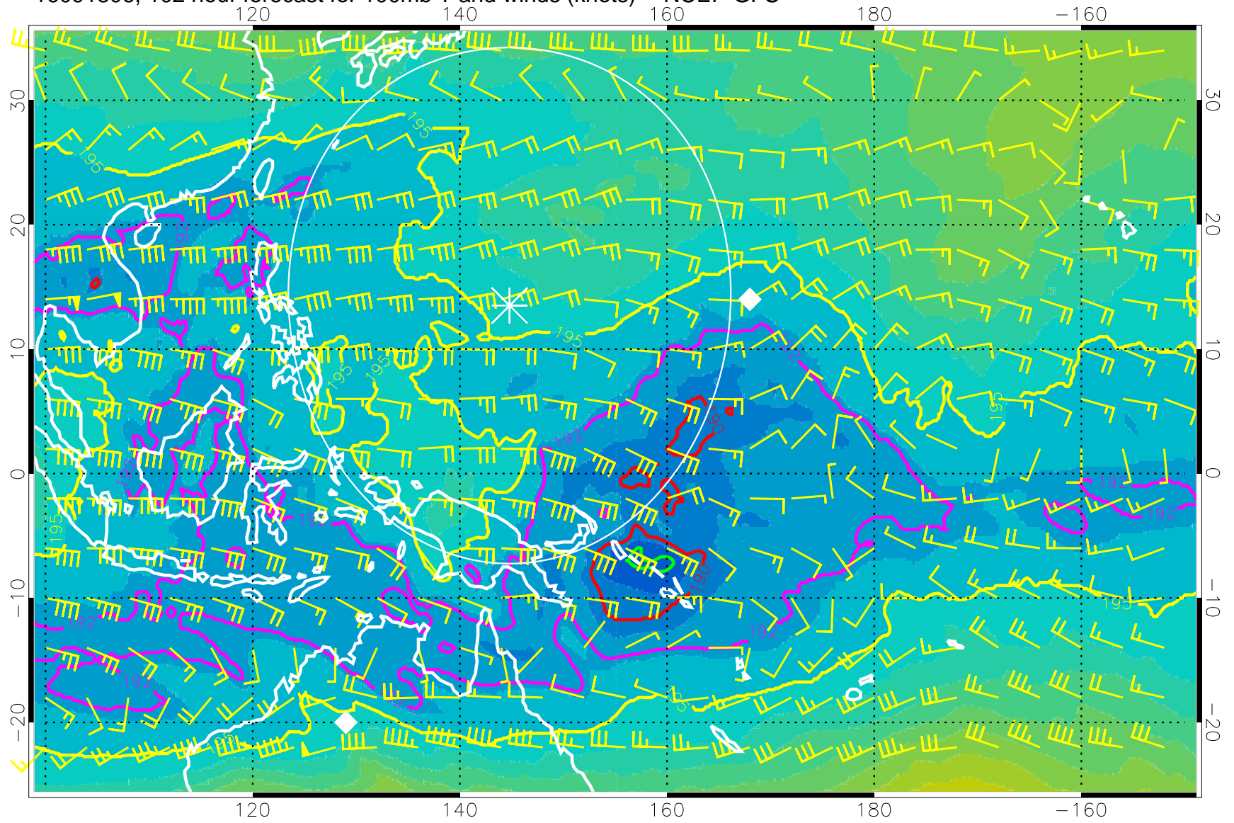
16091806, 102 hour forecast for 100mb T and winds (knots) -- NCEP GFS
