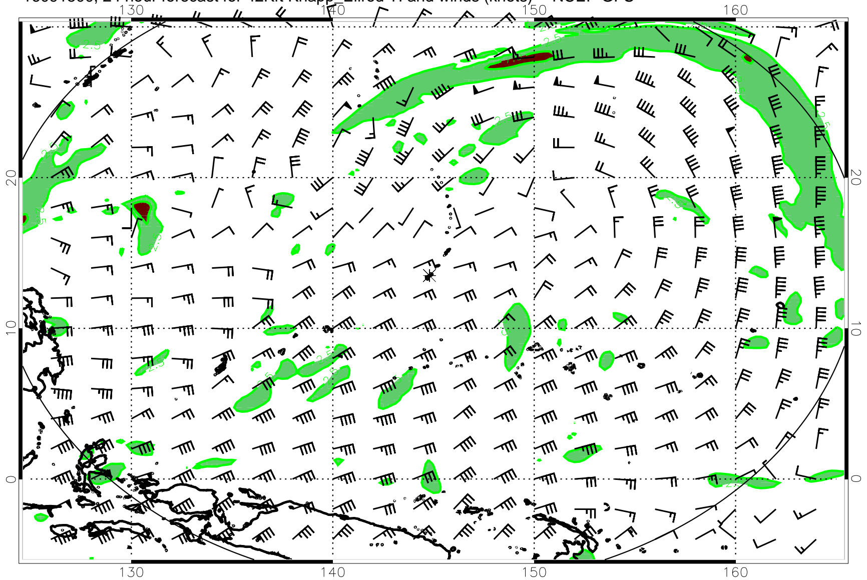
16091500, 24 hour forecast for 42Kft Knapp_Ellrod TI and winds (knots) -- NCEP GFS
