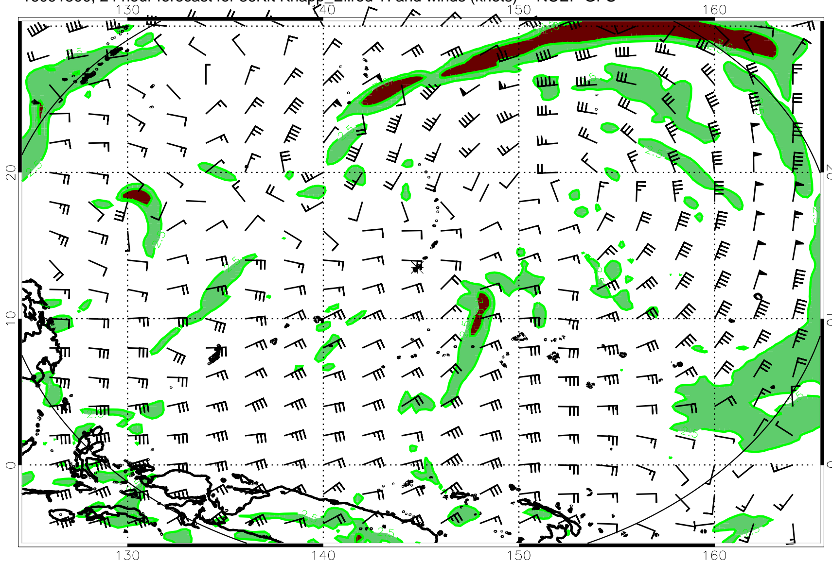
16091500, 24 hour forecast for 36Kft Knapp_Ellrod TI and winds (knots) -- NCEP GFS
