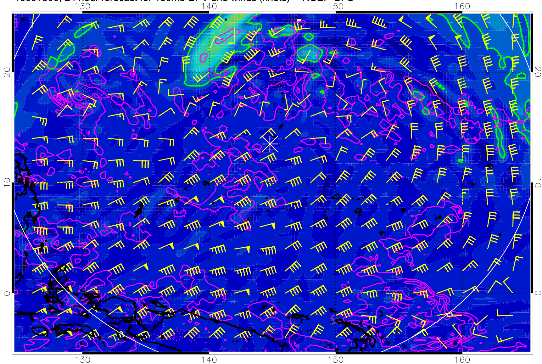
16091500, 24 hour forecast for 150mb EPV and winds (knots) -- NCEP GFS
