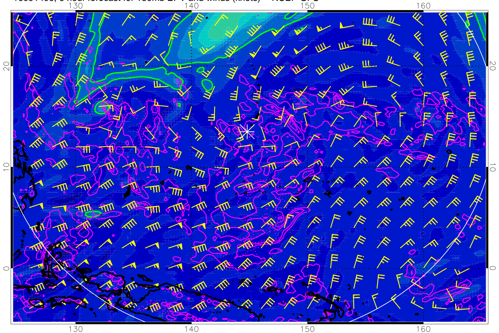
16091406, 6 hour forecast for 150mb EPV and winds (knots) -- NCEP GFS
