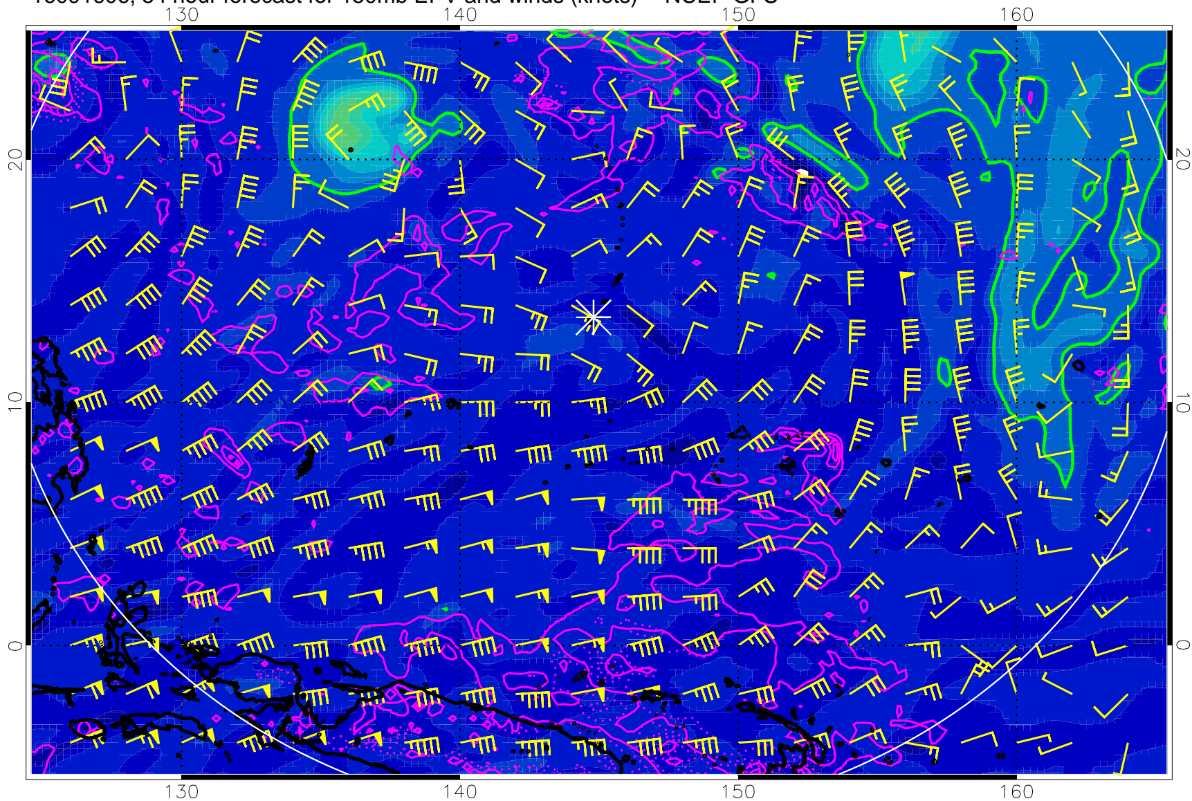
16091606, 54 hour forecast for 150mb EPV and winds (knots) -- NCEP GFS
