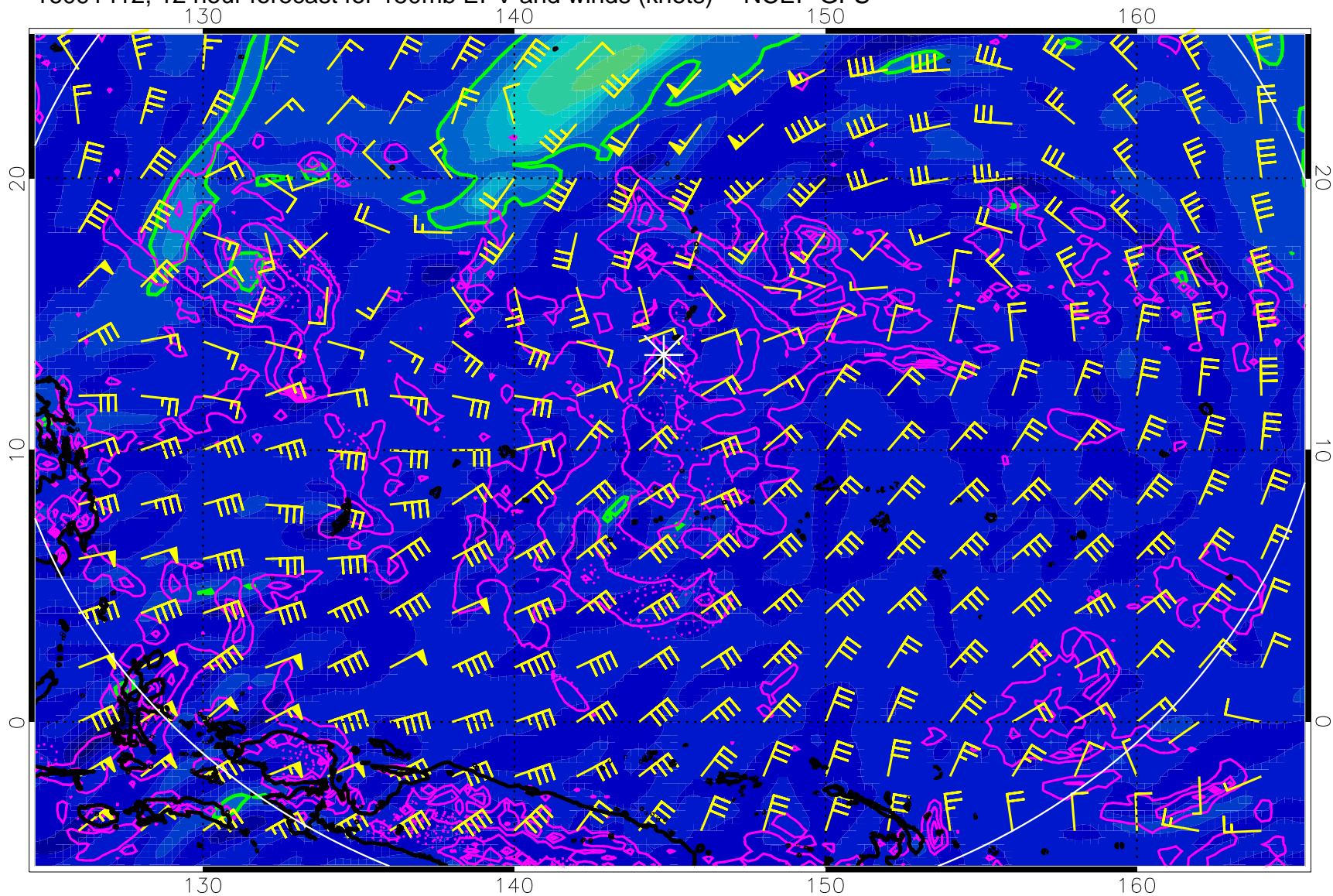
16091412, 12 hour forecast for 150mb EPV and winds (knots) -- NCEP GFS
