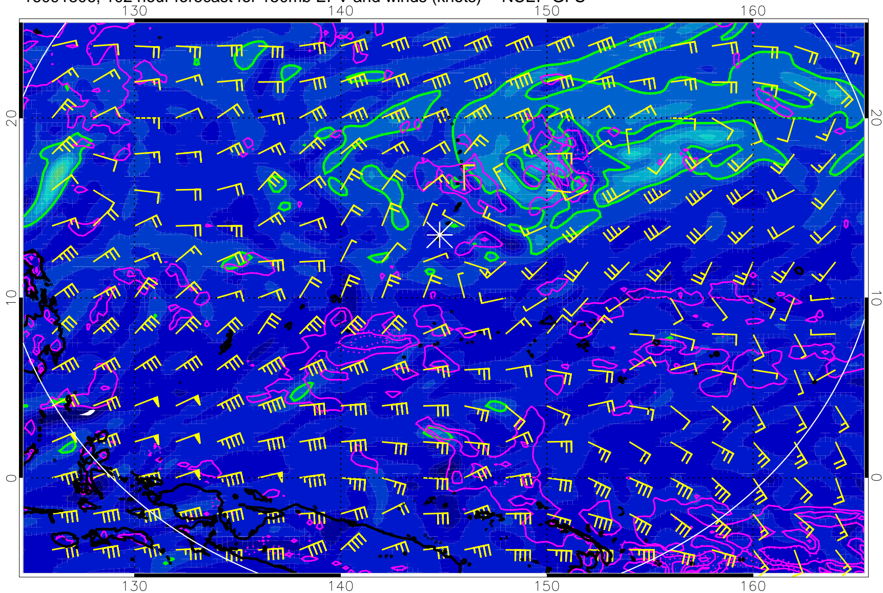
16091806, 102 hour forecast for 150mb EPV and winds (knots) -- NCEP GFS
