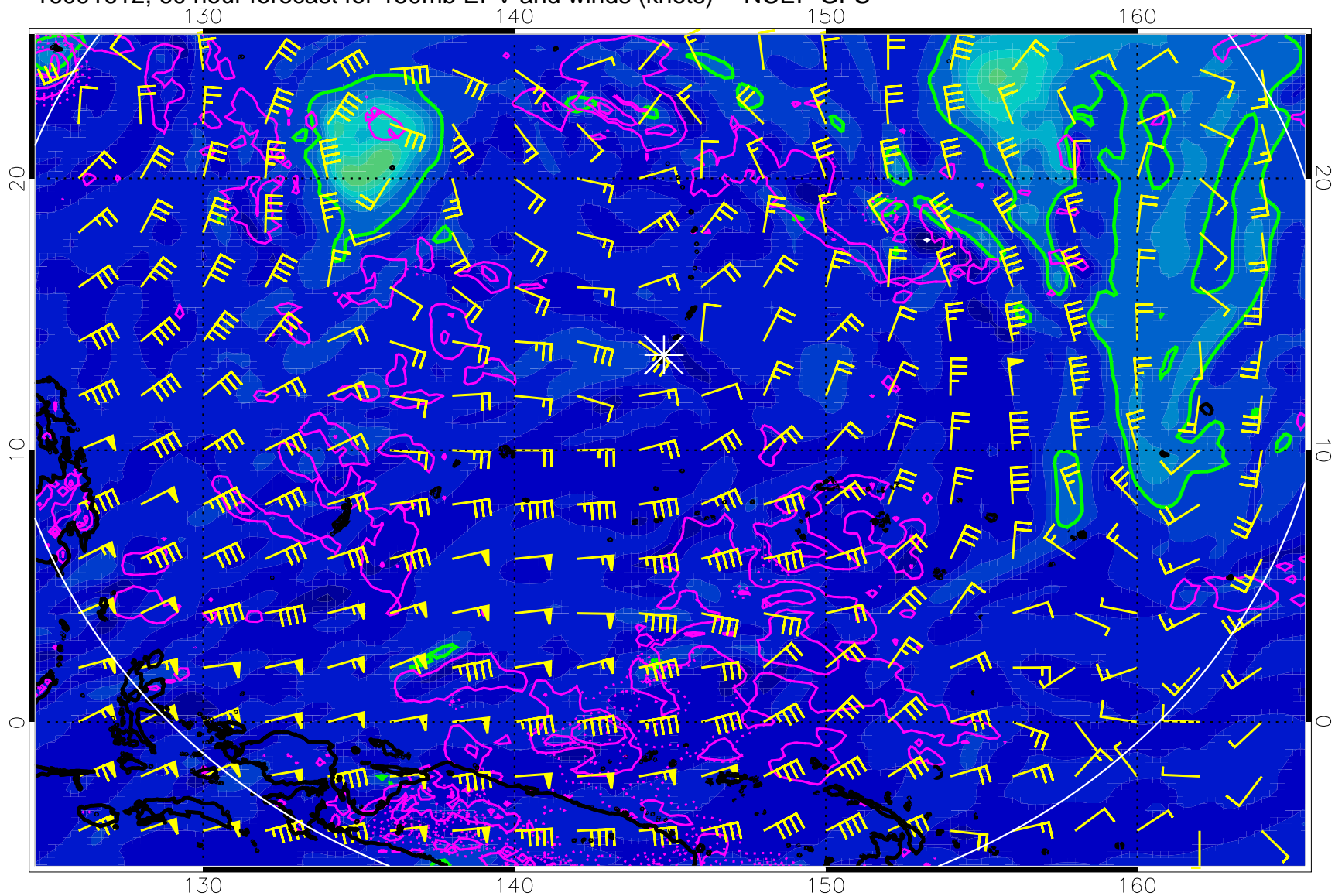
16091612, 60 hour forecast for 150mb EPV and winds (knots) -- NCEP GFS
