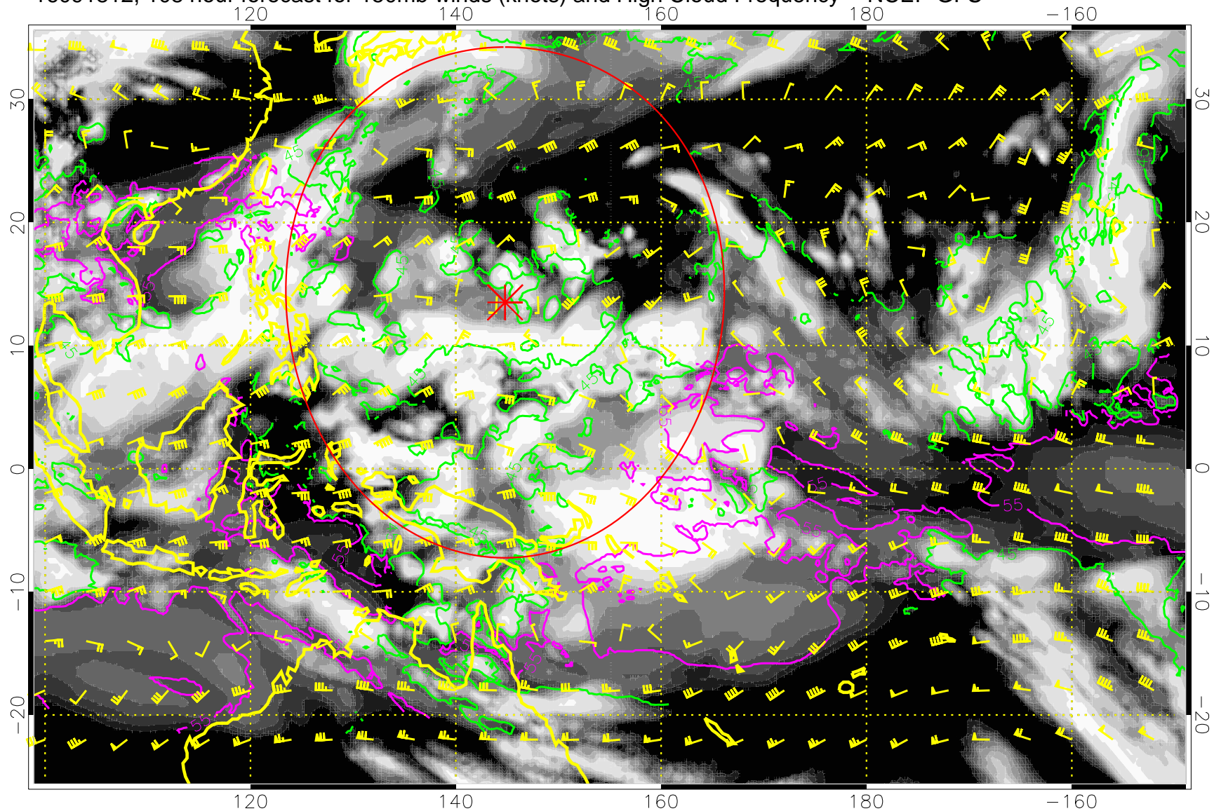
16091812, 108 hour forecast for 150mb winds (knots) and High Cloud Frequency -- NCEP GFS
