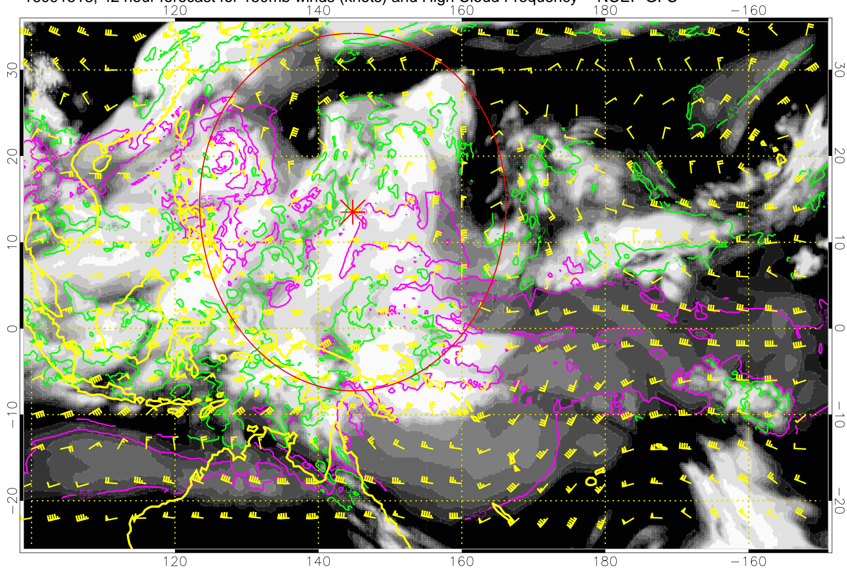
16091518, 42 hour forecast for 150mb winds (knots) and High Cloud Frequency -- NCEP GFS
