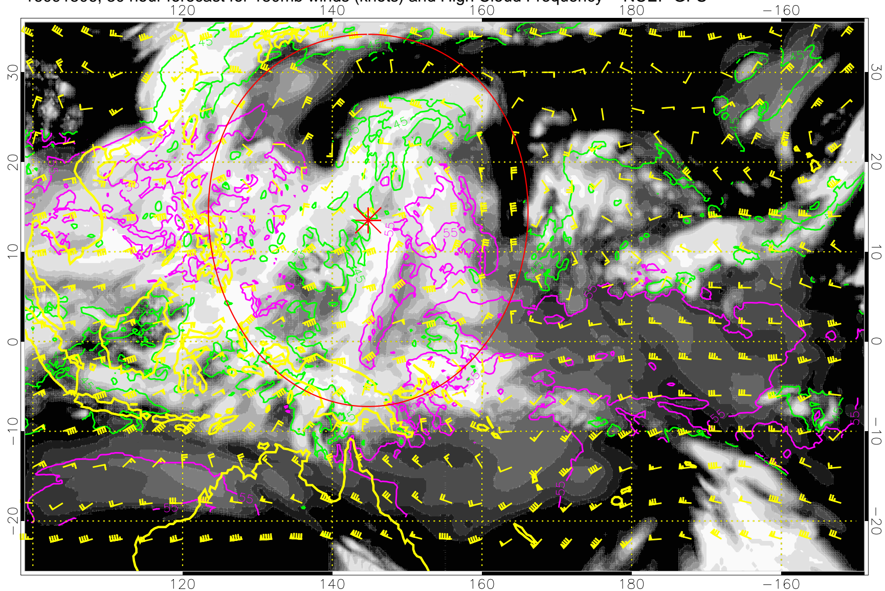
16091506, 30 hour forecast for 150mb winds (knots) and High Cloud Frequency -- NCEP GFS
