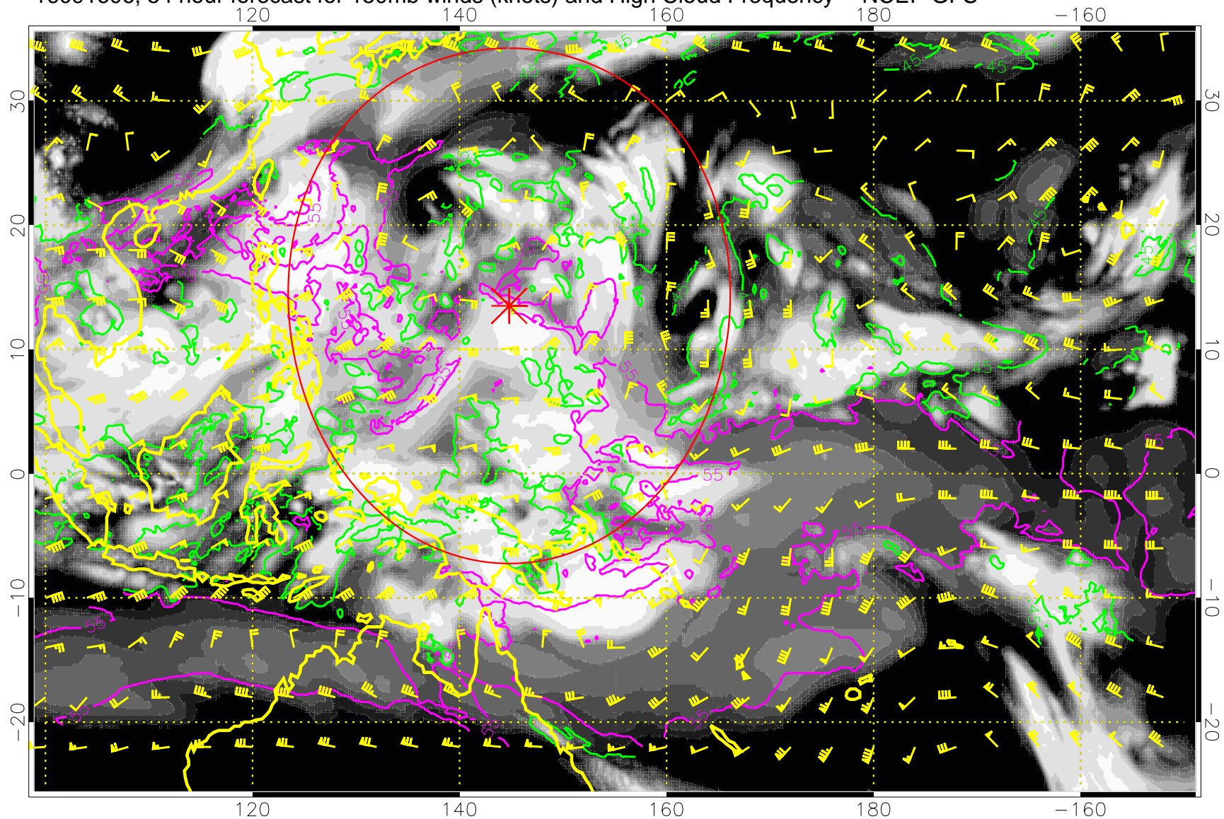
16091606, 54 hour forecast for 150mb winds (knots) and High Cloud Frequency -- NCEP GFS
