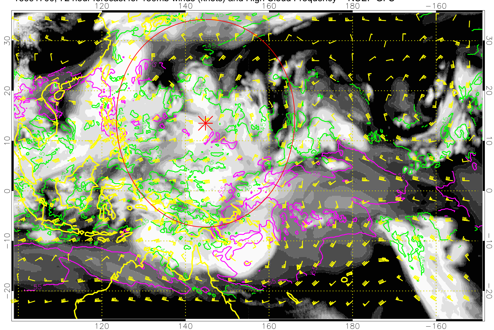
16091700, 72 hour forecast for 150mb winds (knots) and High Cloud Frequency -- NCEP GFS
