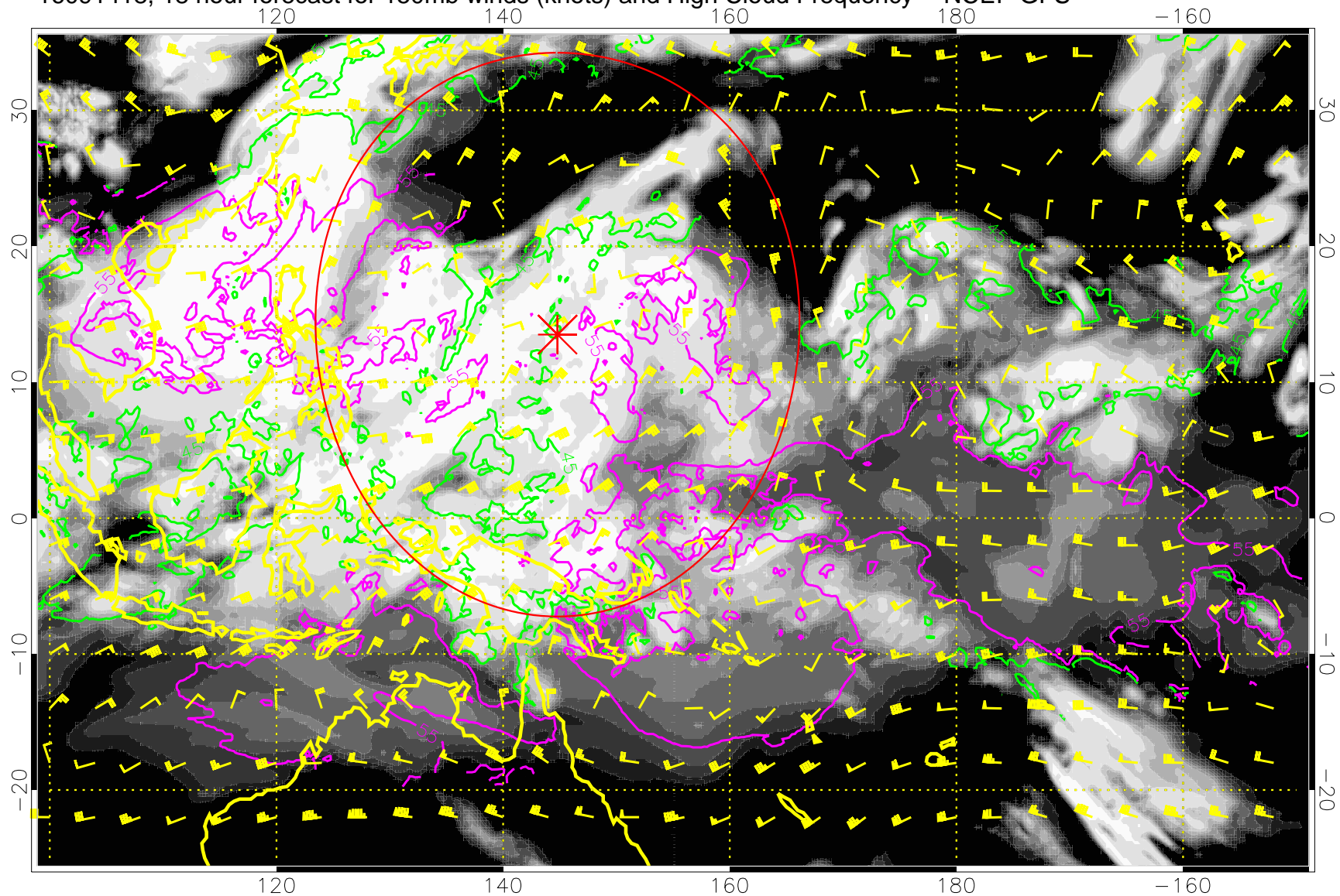
16091418, 18 hour forecast for 150mb winds (knots) and High Cloud Frequency -- NCEP GFS
