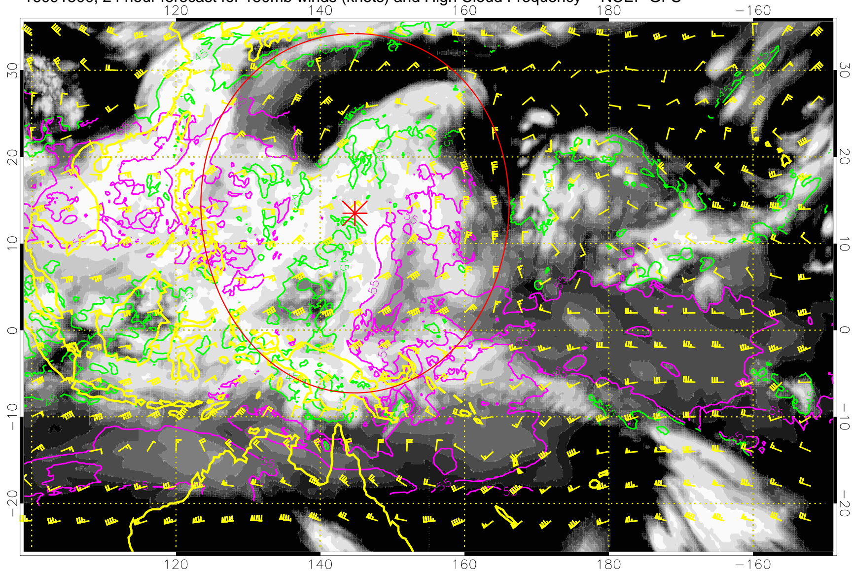
16091500, 24 hour forecast for 150mb winds (knots) and High Cloud Frequency -- NCEP GFS
