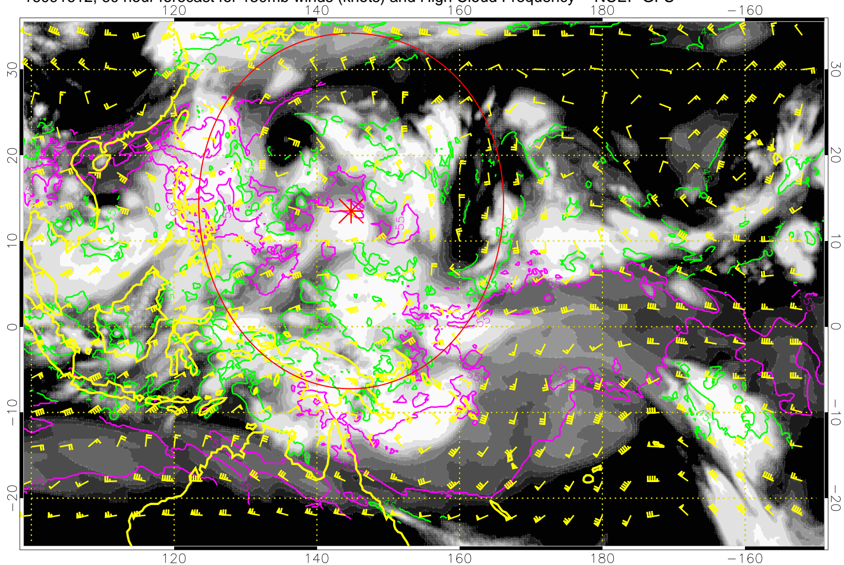
16091612, 60 hour forecast for 150mb winds (knots) and High Cloud Frequency -- NCEP GFS
