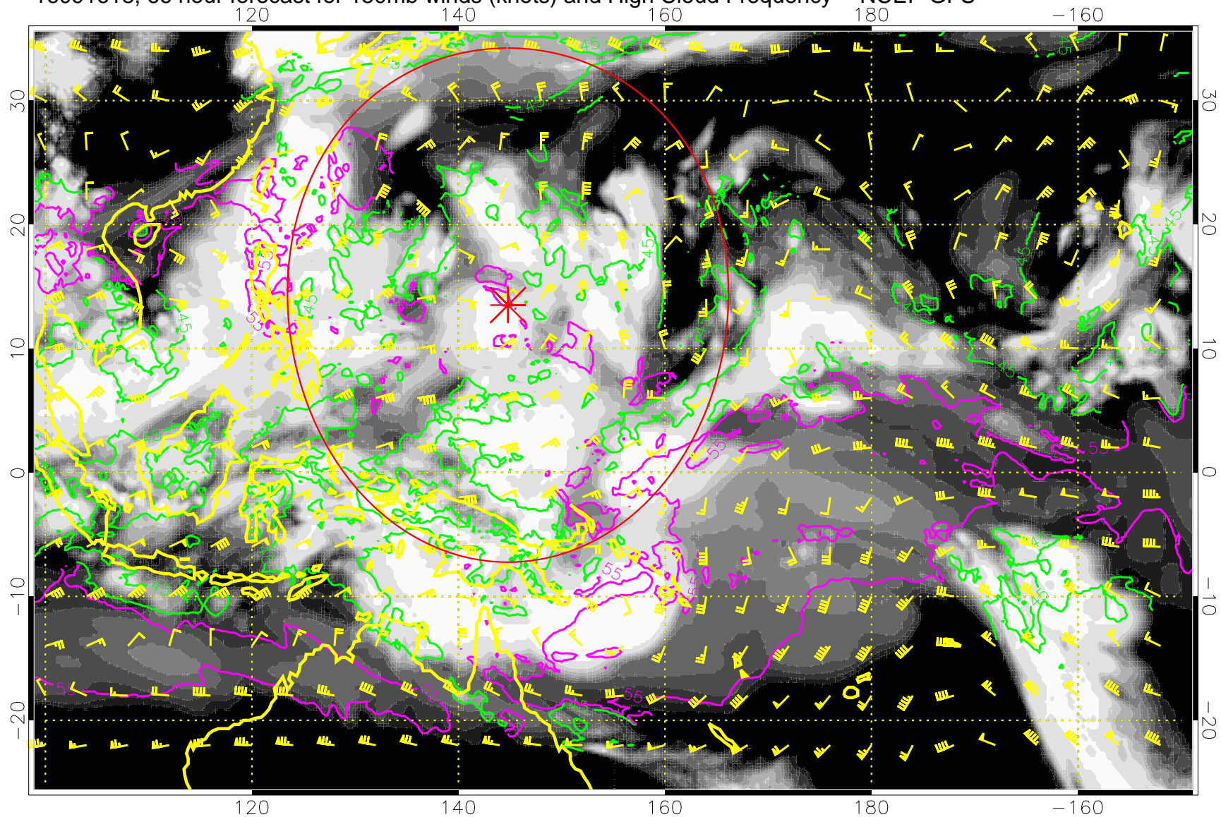
16091618, 66 hour forecast for 150mb winds (knots) and High Cloud Frequency -- NCEP GFS
