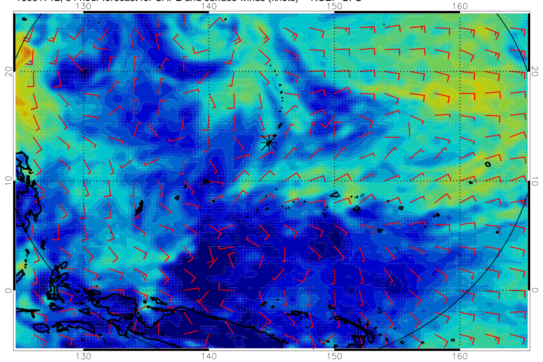
16091712, 84 hour forecast for CAPE and surface winds (knots) -- NCEP GFS
