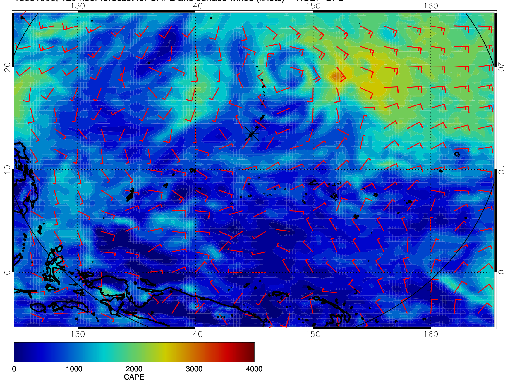
16091900, 120 hour forecast for CAPE and surface winds (knots) -- NCEP GFS
