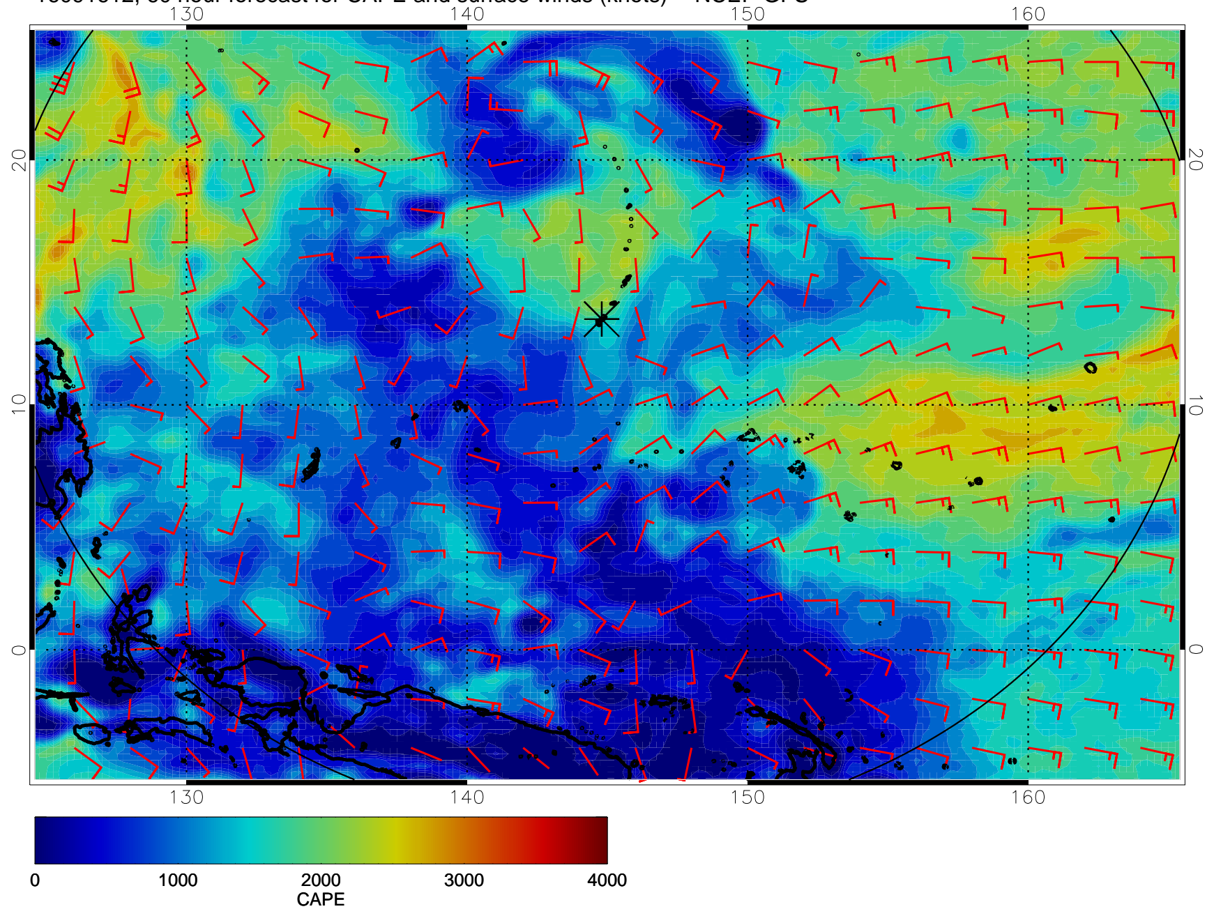
16091612, 60 hour forecast for CAPE and surface winds (knots) -- NCEP GFS
