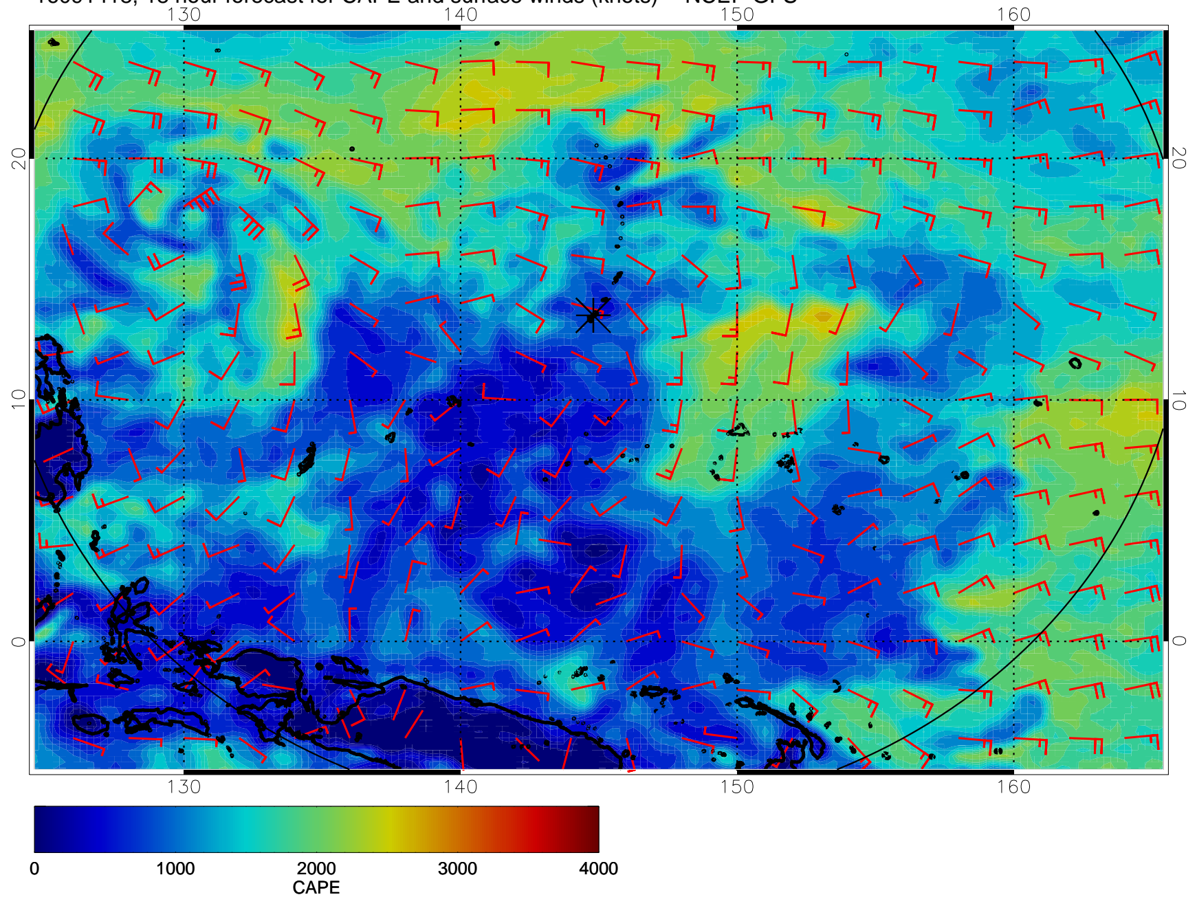
16091418, 18 hour forecast for CAPE and surface winds (knots) -- NCEP GFS
