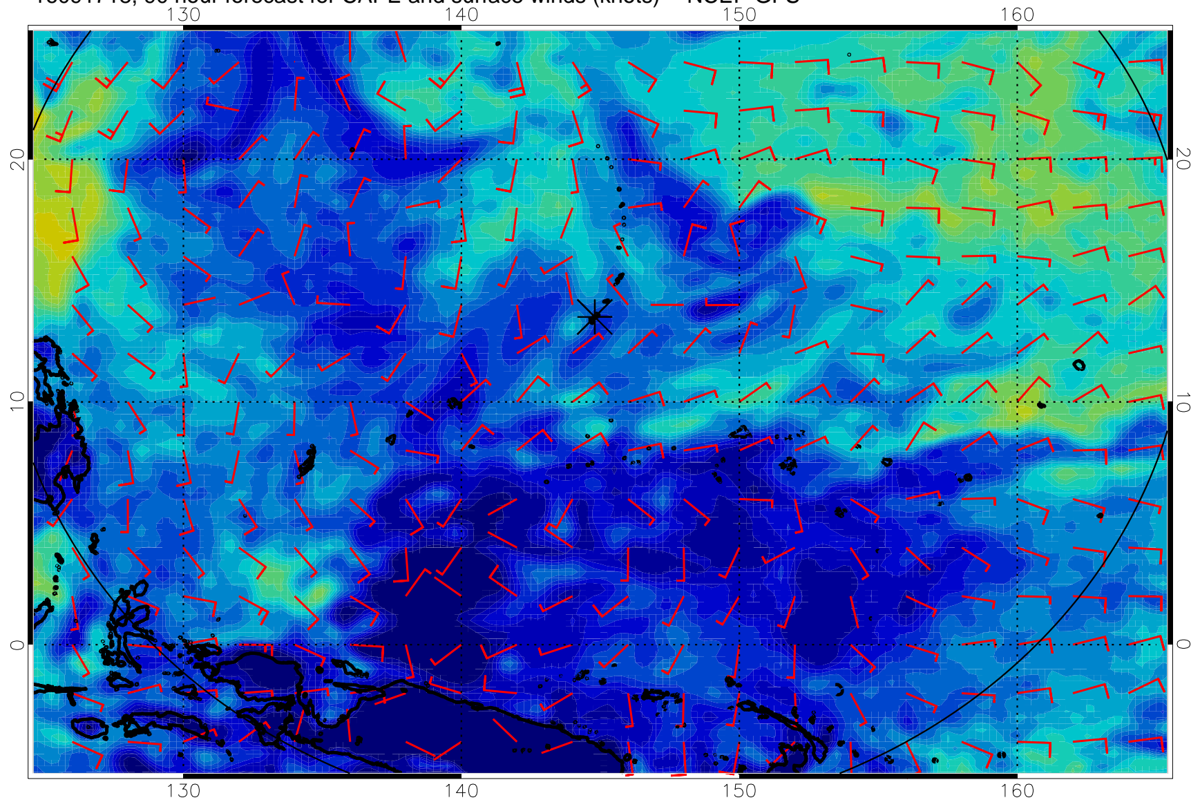
16091718, 90 hour forecast for CAPE and surface winds (knots) -- NCEP GFS
