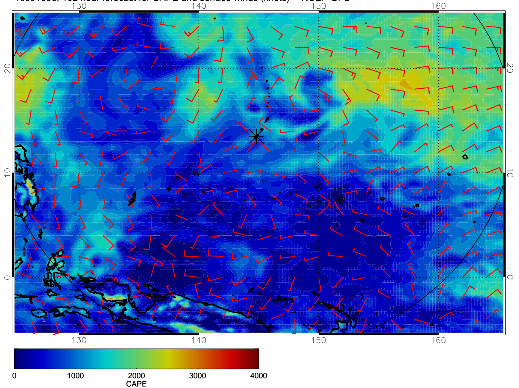
16091806, 102 hour forecast for CAPE and surface winds (knots) -- NCEP GFS
