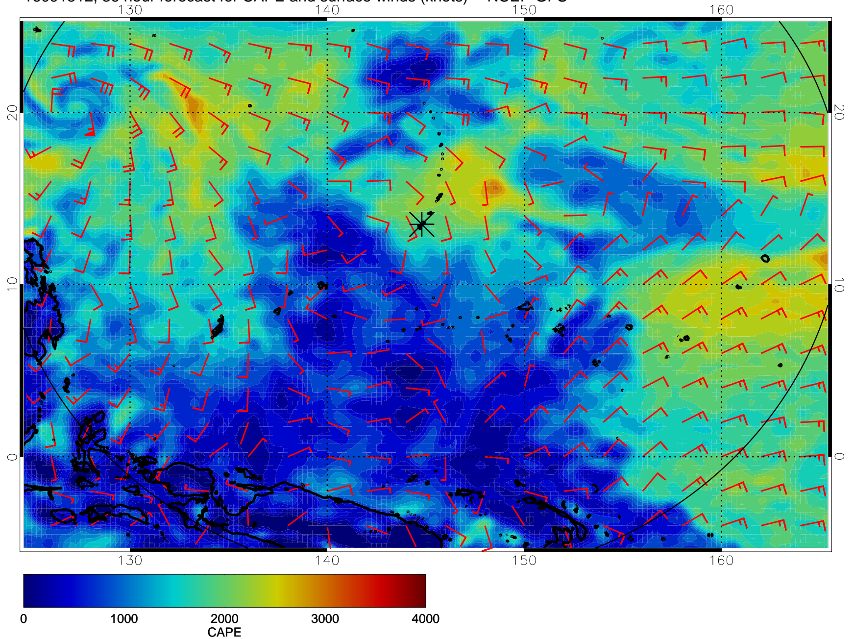
16091512, 36 hour forecast for CAPE and surface winds (knots) -- NCEP GFS
