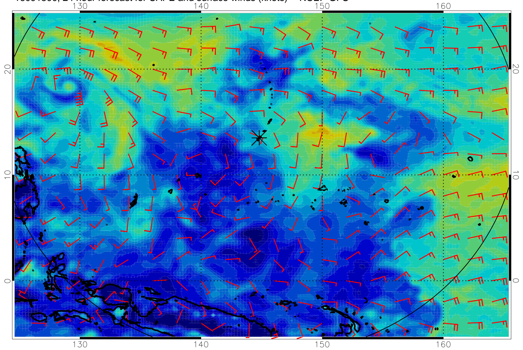
16091500, 24 hour forecast for CAPE and surface winds (knots) -- NCEP GFS
