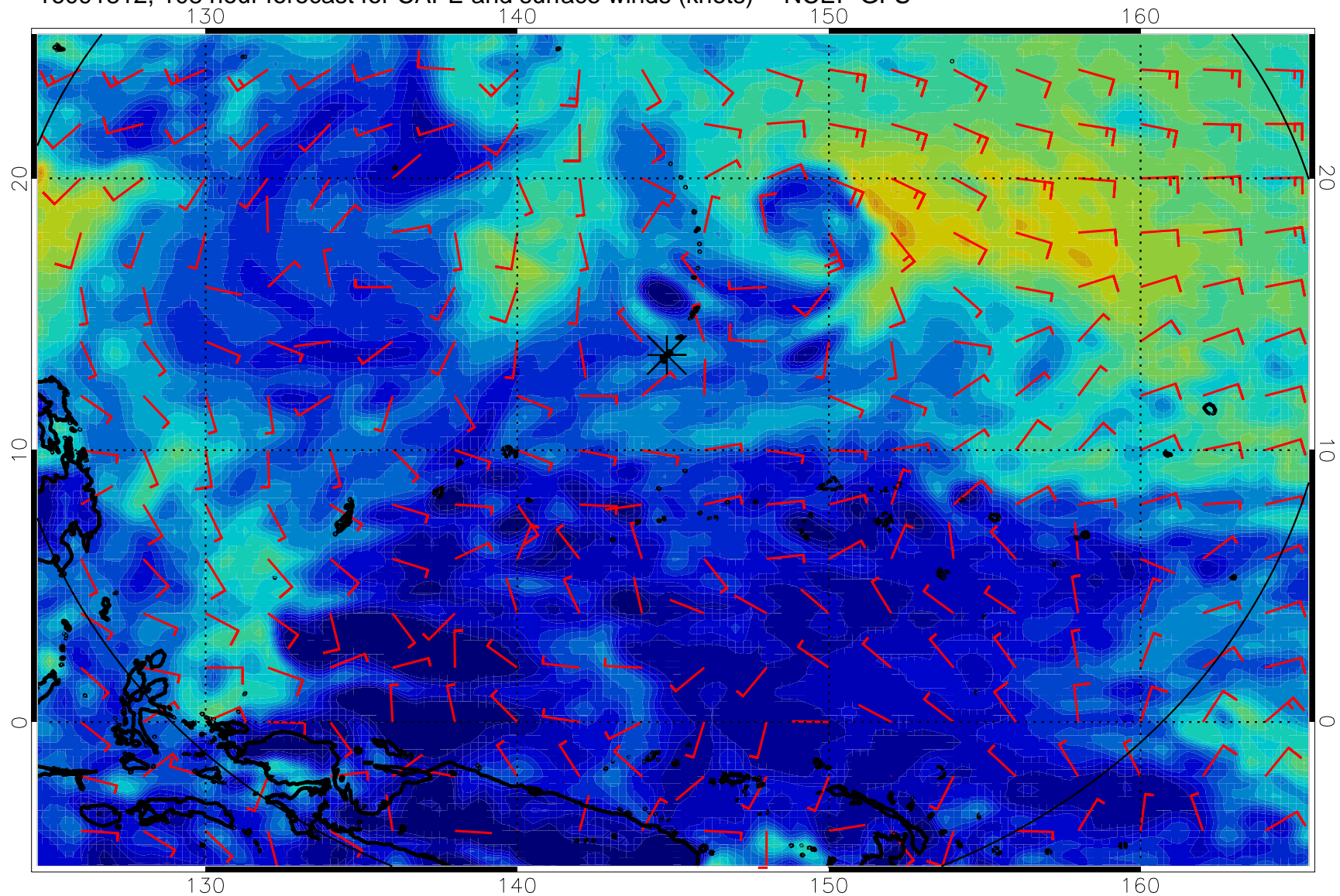
16091812, 108 hour forecast for CAPE and surface winds (knots) -- NCEP GFS
