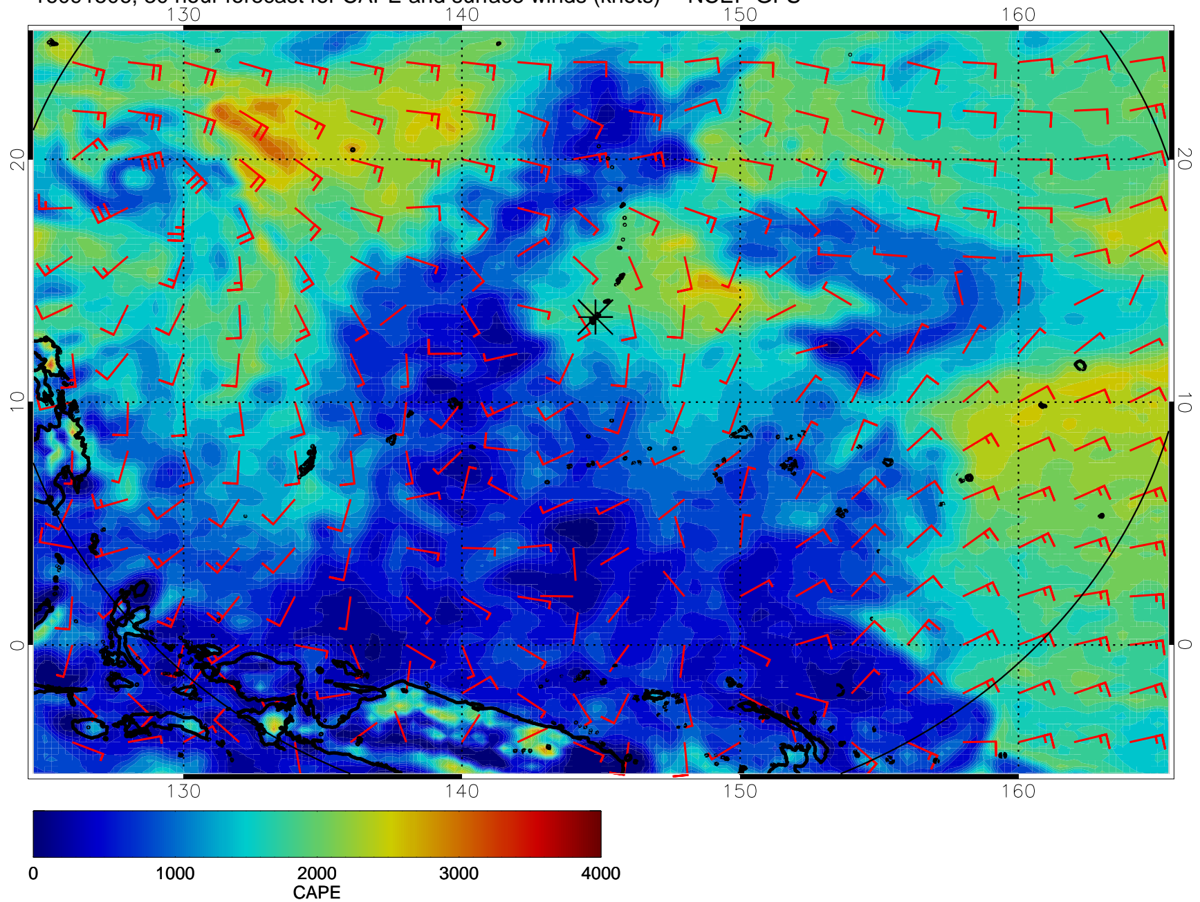
16091506, 30 hour forecast for CAPE and surface winds (knots) -- NCEP GFS
