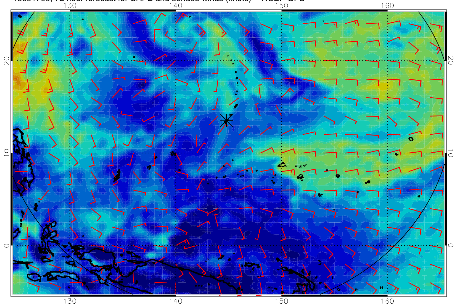
16091700, 72 hour forecast for CAPE and surface winds (knots) -- NCEP GFS
