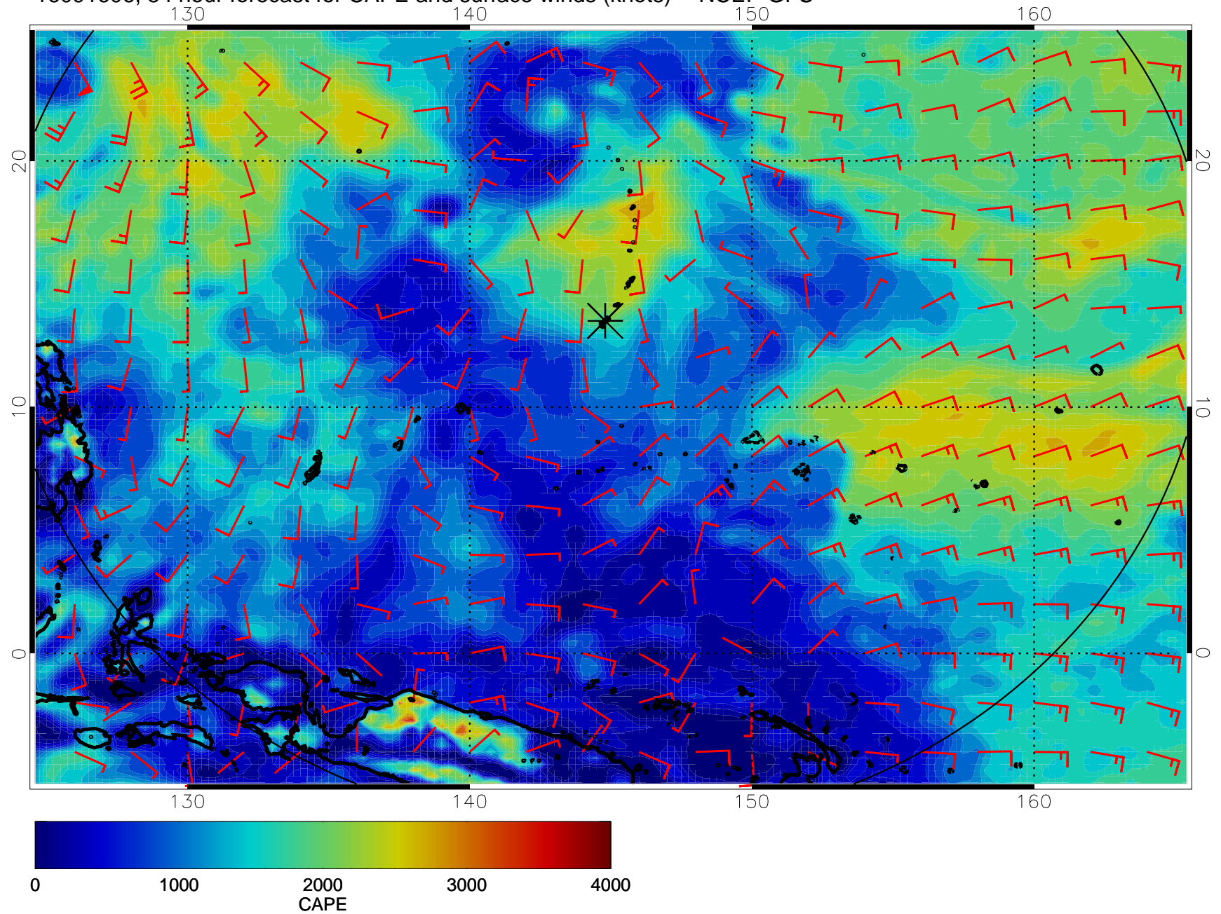
16091606, 54 hour forecast for CAPE and surface winds (knots) -- NCEP GFS
