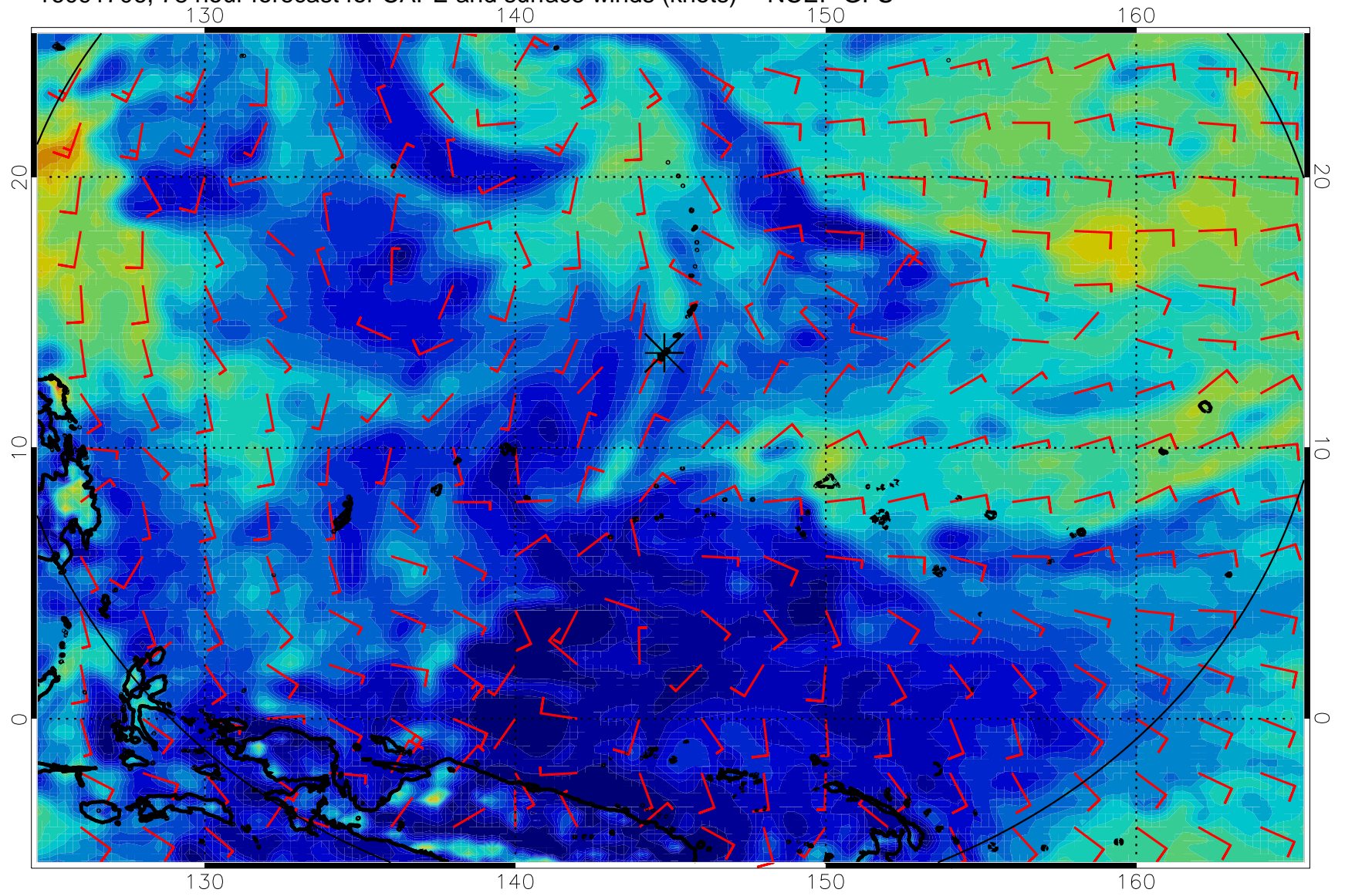
16091706, 78 hour forecast for CAPE and surface winds (knots) -- NCEP GFS
