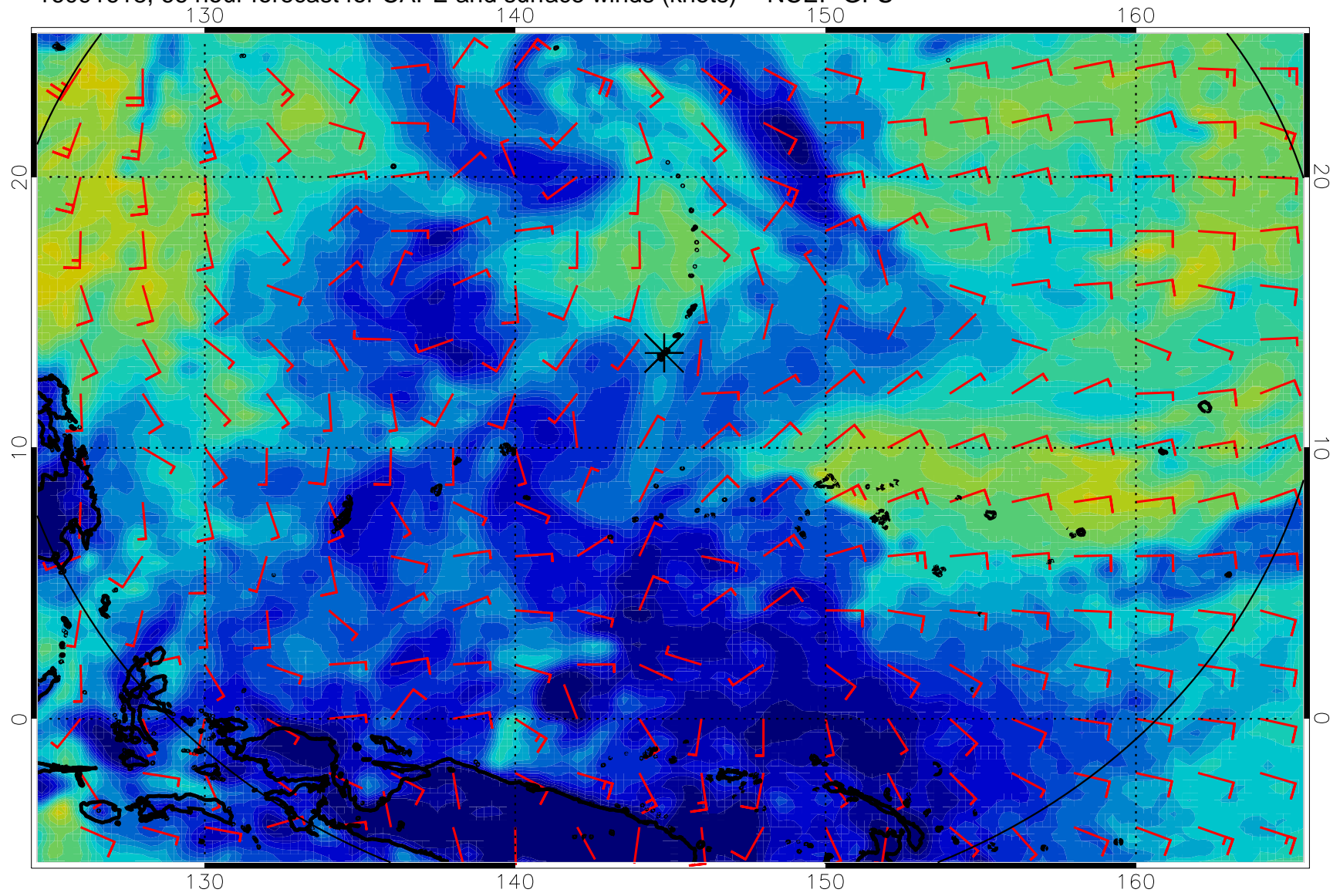
16091618, 66 hour forecast for CAPE and surface winds (knots) -- NCEP GFS
