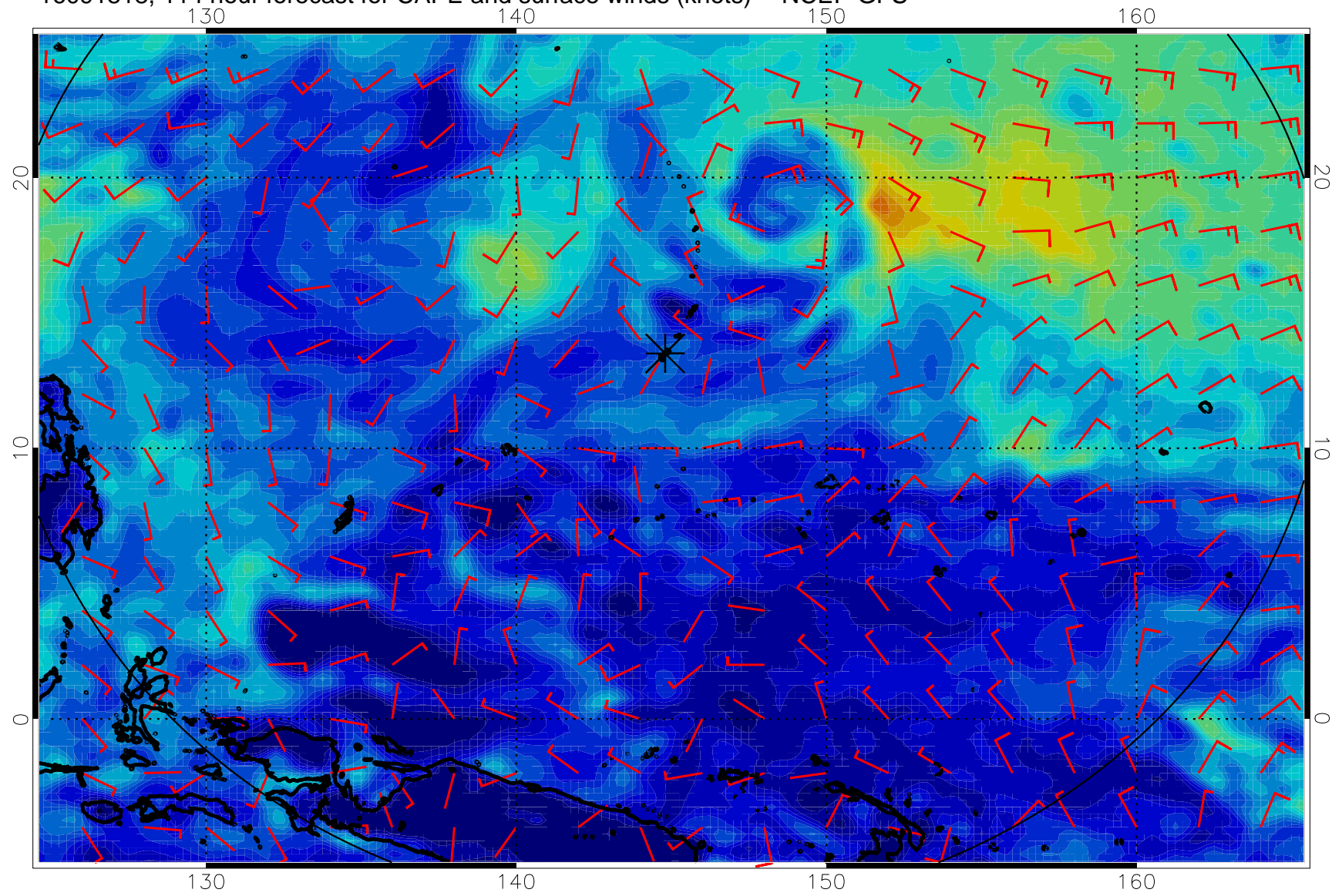
16091818, 114 hour forecast for CAPE and surface winds (knots) -- NCEP GFS
