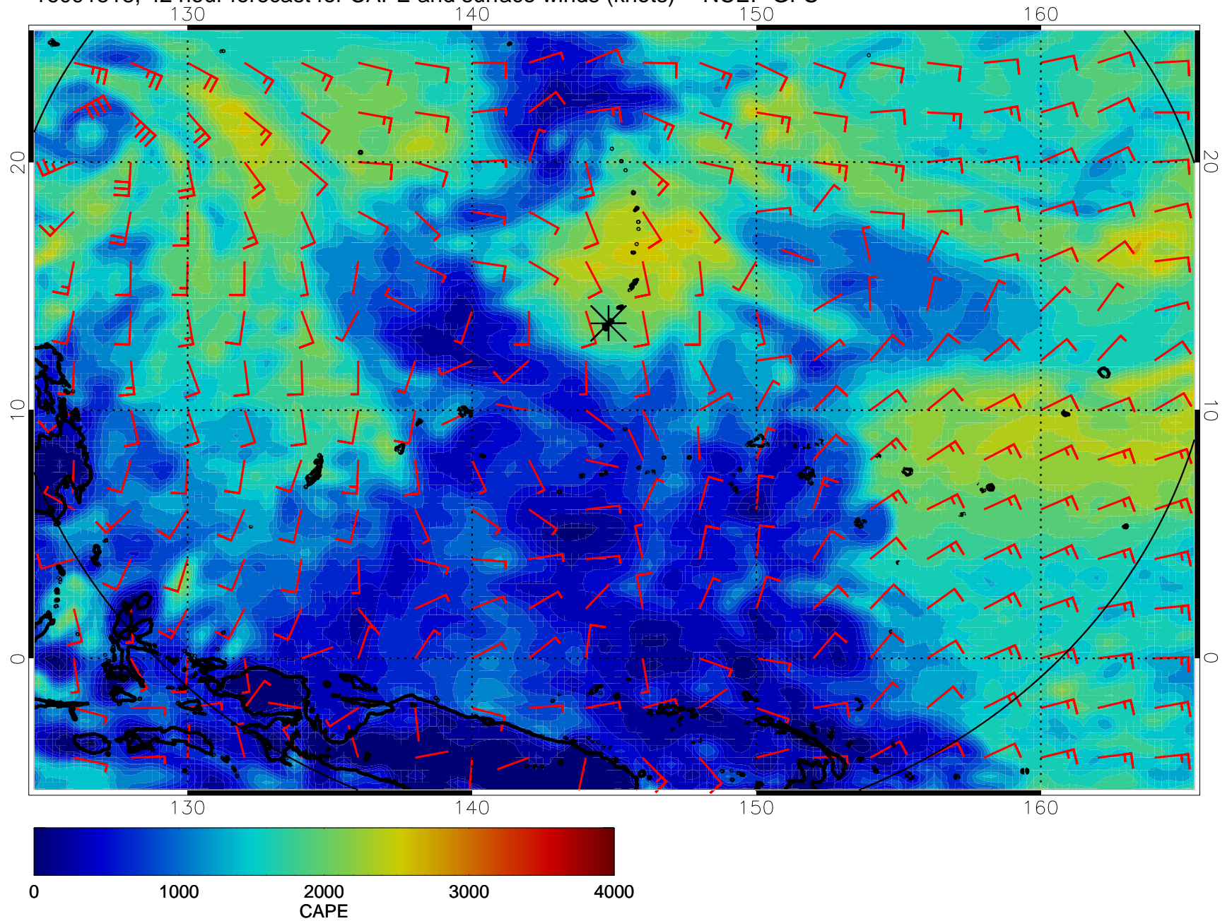
16091518, 42 hour forecast for CAPE and surface winds (knots) -- NCEP GFS
