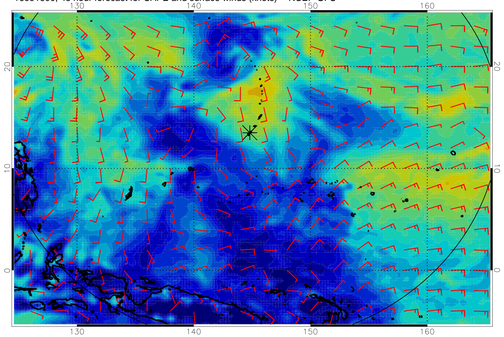
16091600, 48 hour forecast for CAPE and surface winds (knots) -- NCEP GFS
