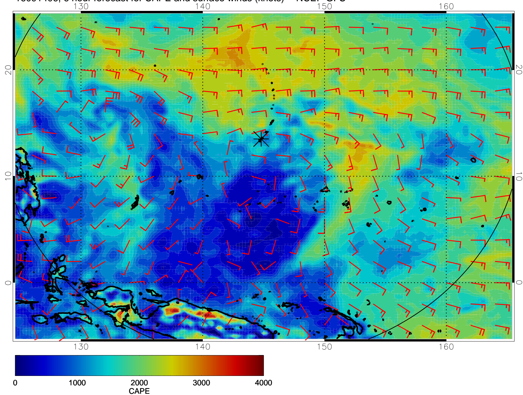
16091406, 6 hour forecast for CAPE and surface winds (knots) -- NCEP GFS
