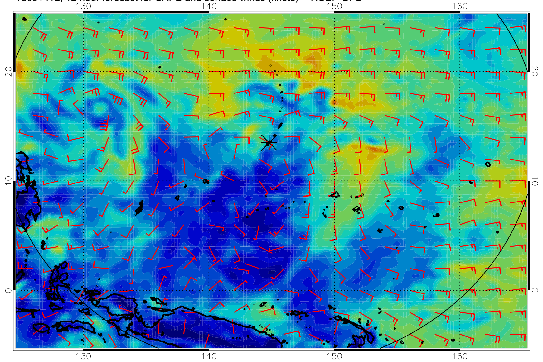
16091412, 12 hour forecast for CAPE and surface winds (knots) -- NCEP GFS
