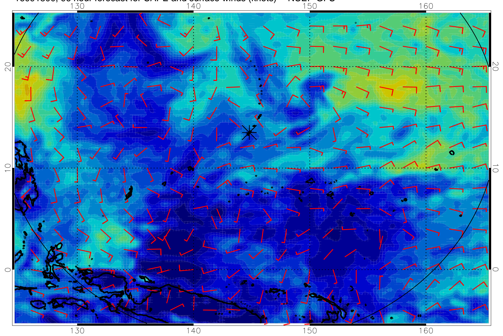
16091800, 96 hour forecast for CAPE and surface winds (knots) -- NCEP GFS
