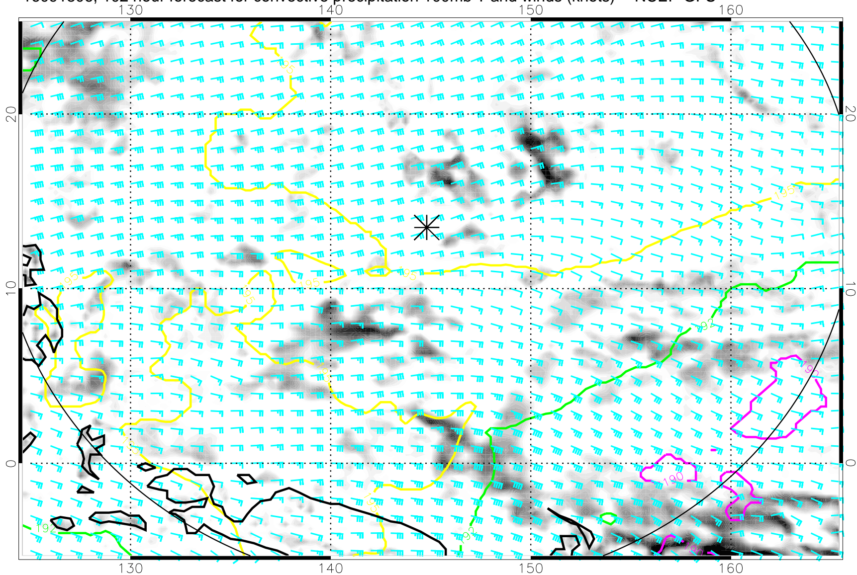
16091806, 102 hour forecast for convective precipitation 100mb T and winds (knots) -- NCEP GFS
