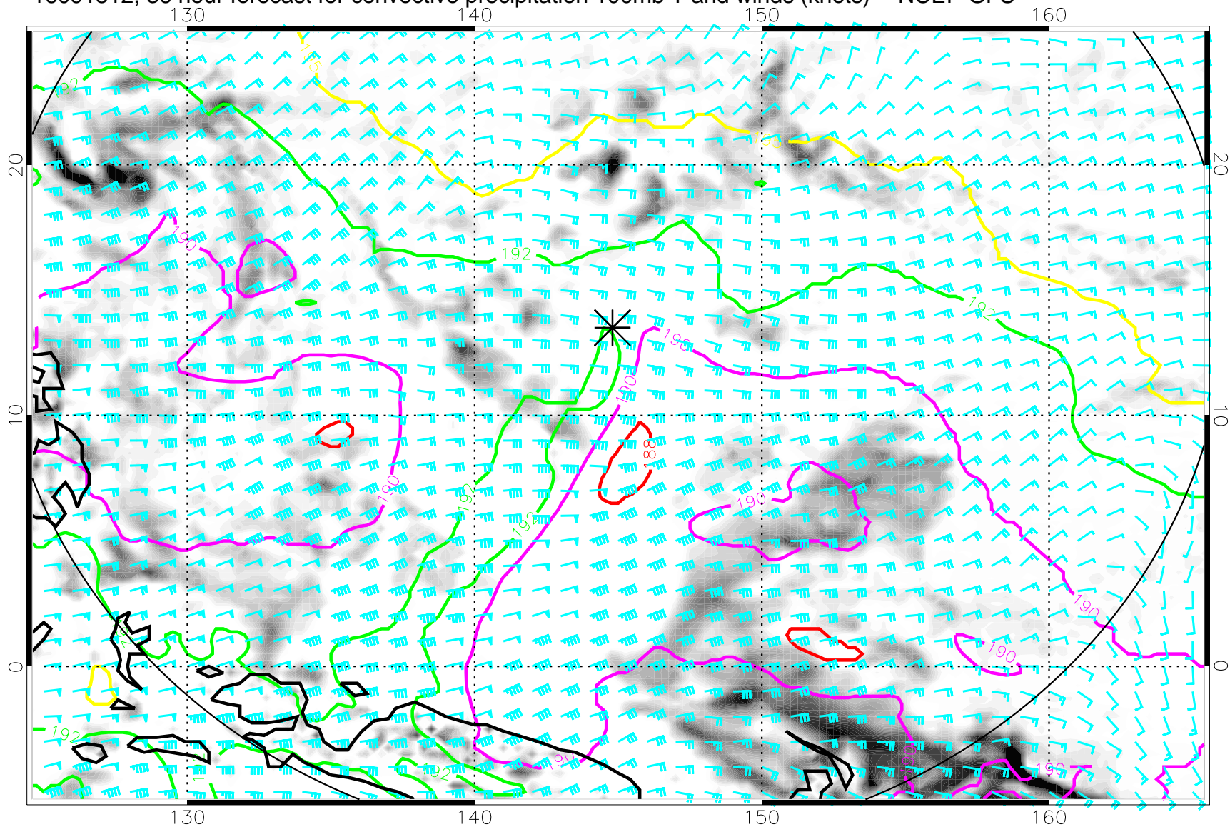
16091512, 36 hour forecast for convective precipitation 100mb T and winds (knots) -- NCEP GFS
