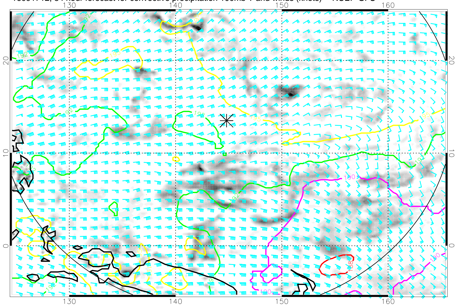
16091712, 84 hour forecast for convective precipitation 100mb T and winds (knots) -- NCEP GFS
