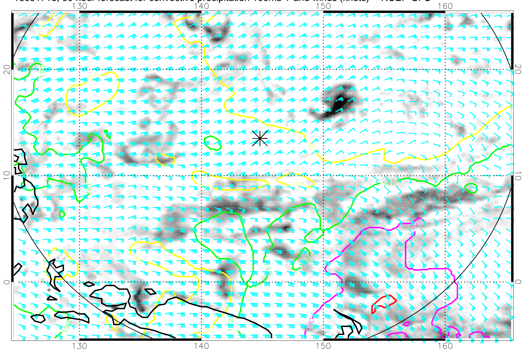
16091718, 90 hour forecast for convective precipitation 100mb T and winds (knots) -- NCEP GFS
