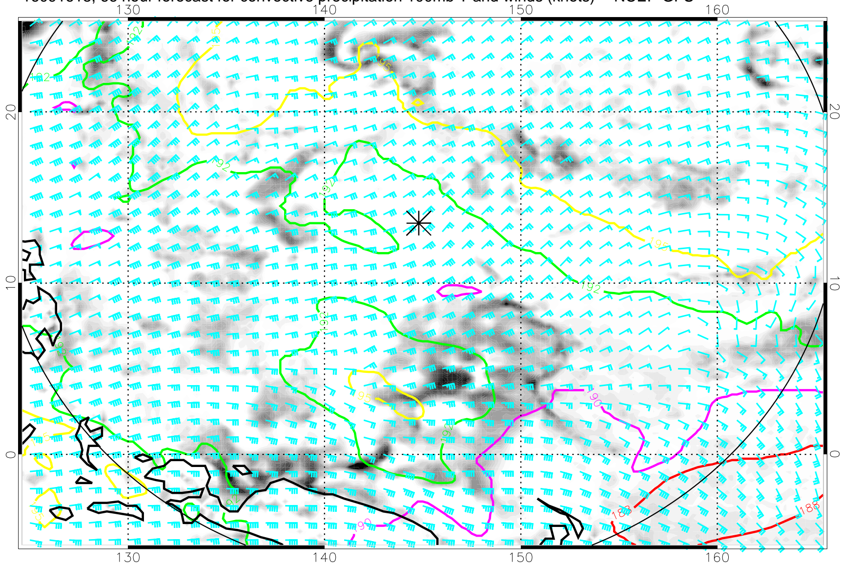
16091618, 66 hour forecast for convective precipitation 100mb T and winds (knots) -- NCEP GFS
