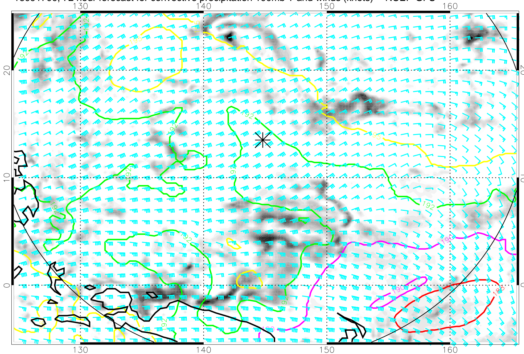
16091700, 72 hour forecast for convective precipitation 100mb T and winds (knots) -- NCEP GFS
