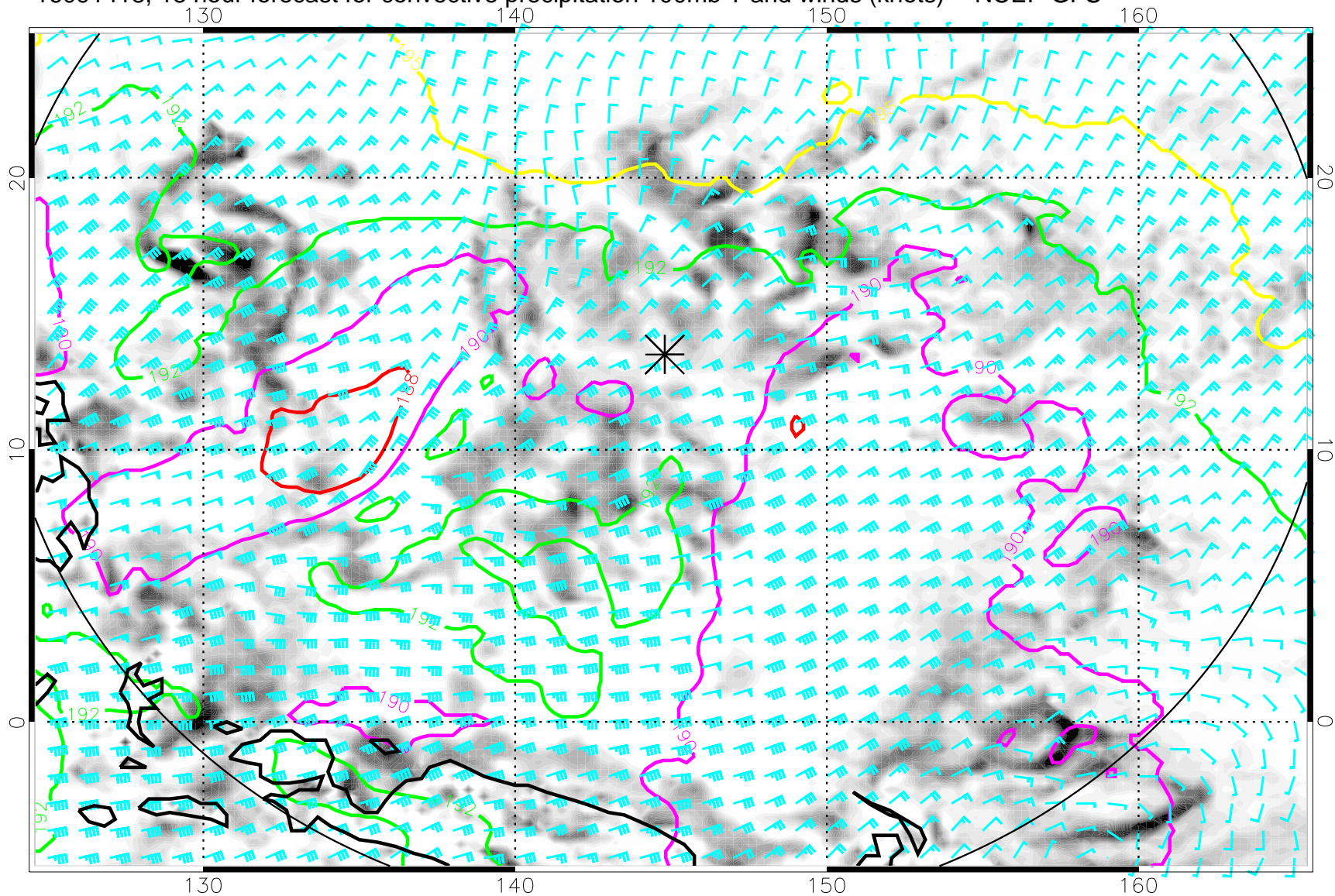
16091418, 18 hour forecast for convective precipitation 100mb T and winds (knots) -- NCEP GFS
