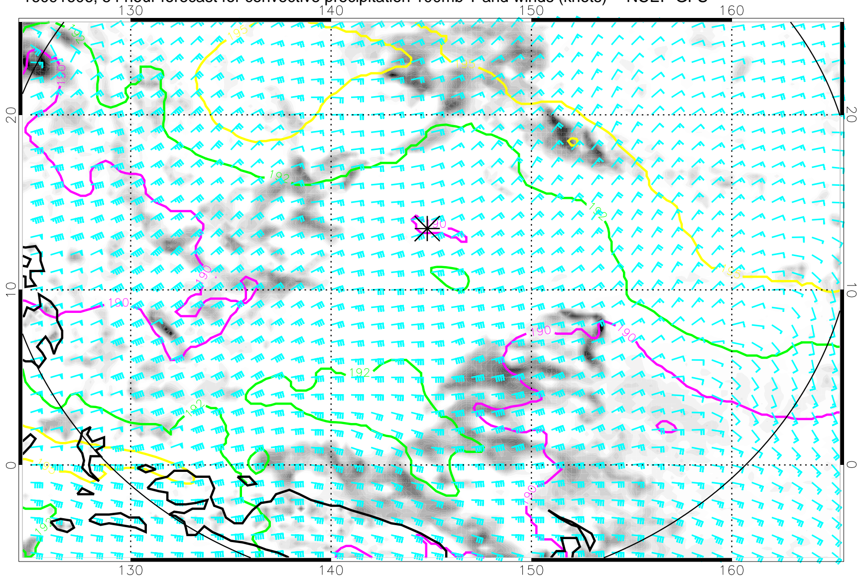
16091606, 54 hour forecast for convective precipitation 100mb T and winds (knots) -- NCEP GFS
