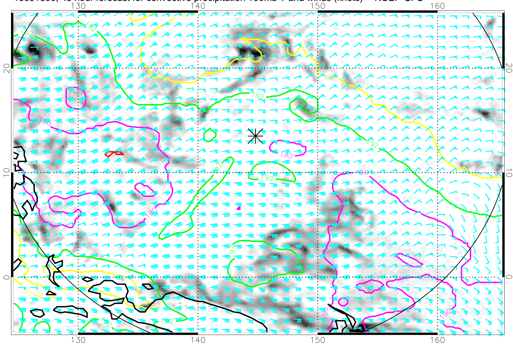
16091600, 48 hour forecast for convective precipitation 100mb T and winds (knots) -- NCEP GFS
