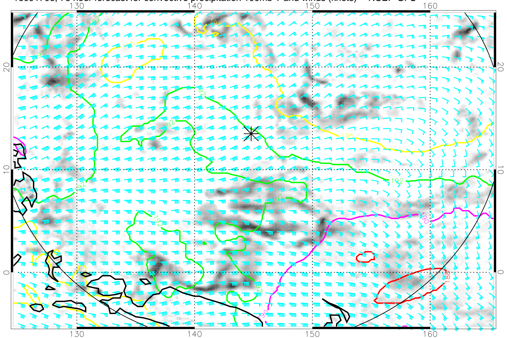
16091706, 78 hour forecast for convective precipitation 100mb T and winds (knots) -- NCEP GFS
