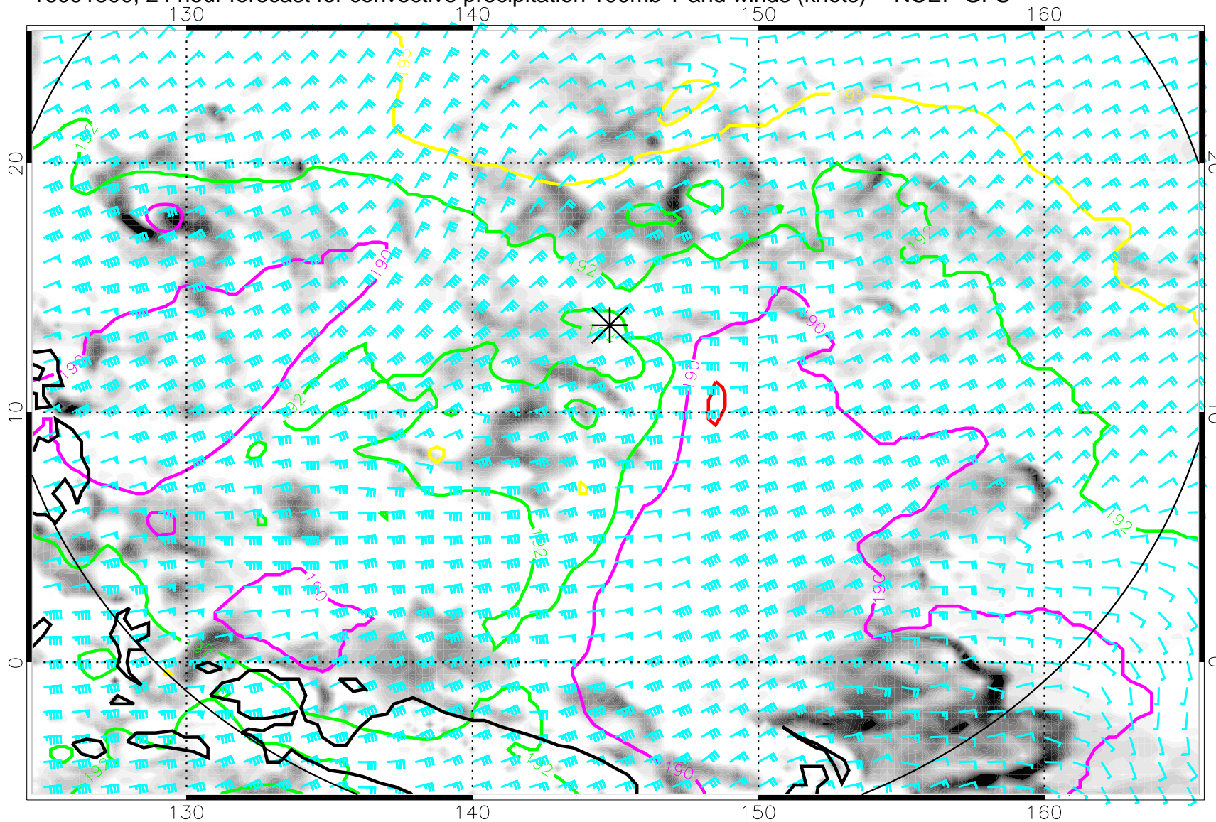
16091500, 24 hour forecast for convective precipitation 100mb T and winds (knots) -- NCEP GFS
