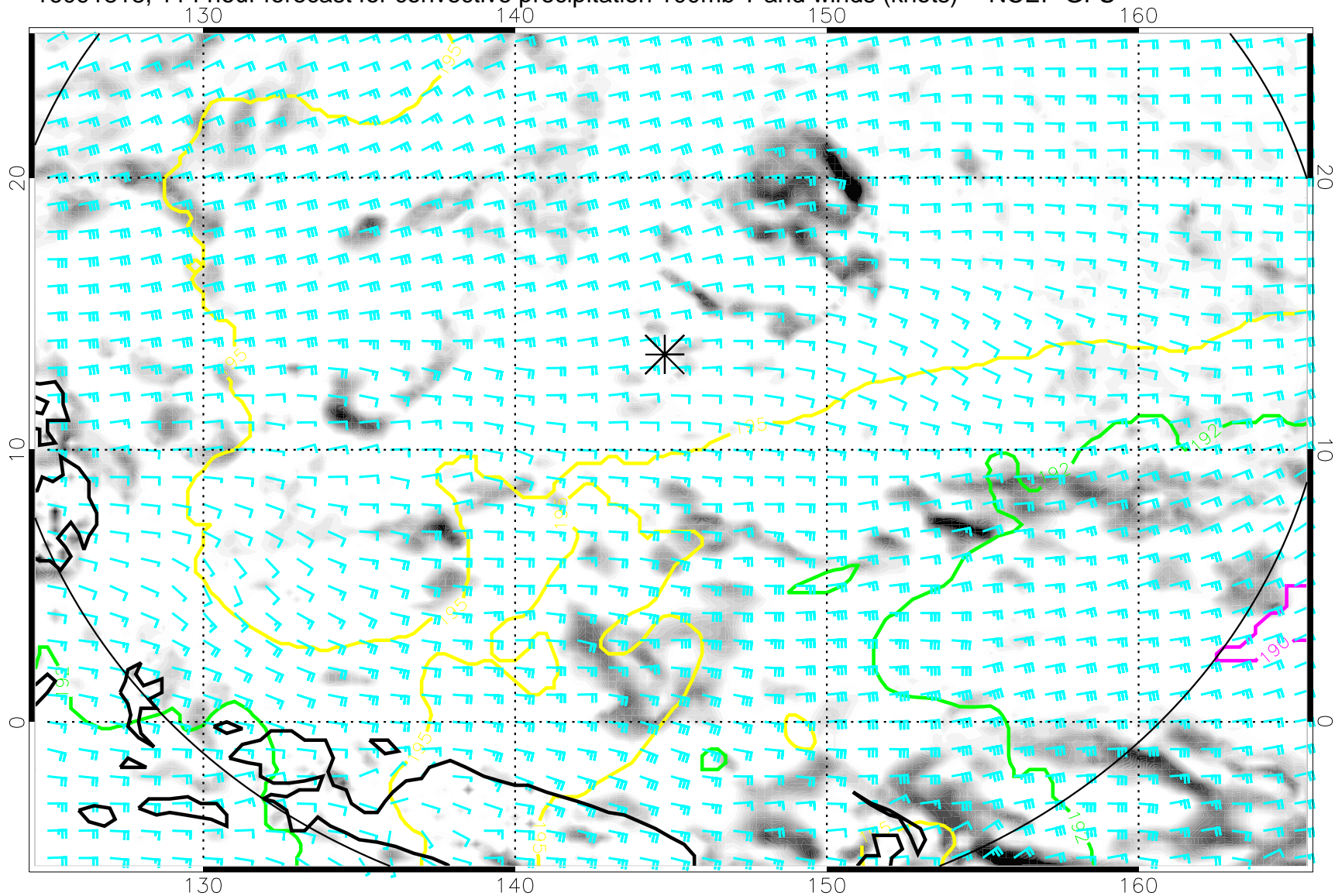
16091818, 114 hour forecast for convective precipitation 100mb T and winds (knots) -- NCEP GFS
