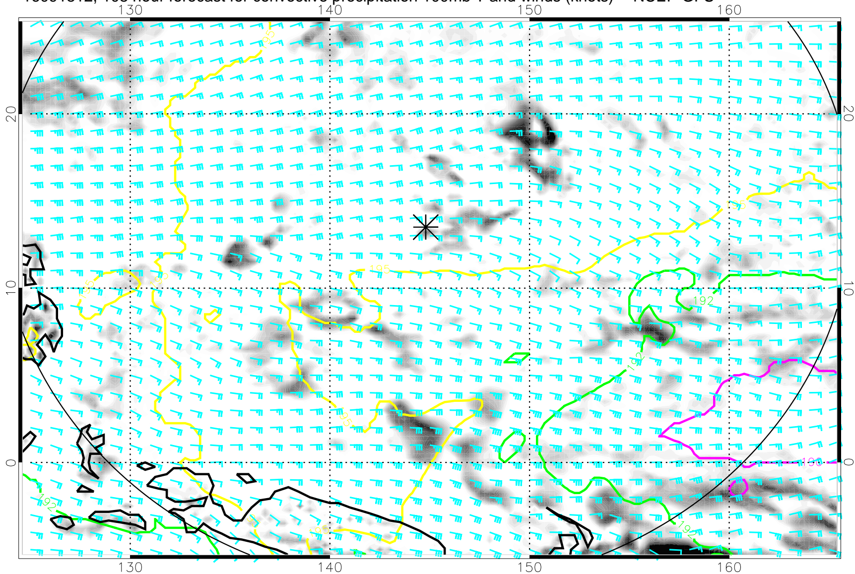
16091812, 108 hour forecast for convective precipitation 100mb T and winds (knots) -- NCEP GFS
