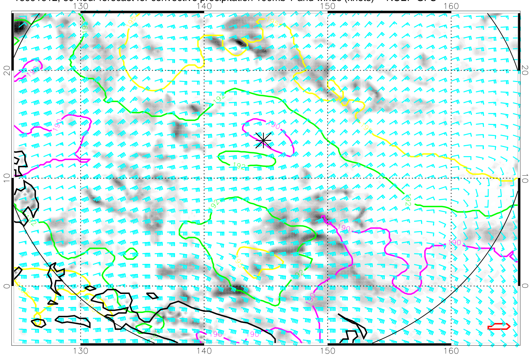
16091612, 60 hour forecast for convective precipitation 100mb T and winds (knots) -- NCEP GFS
