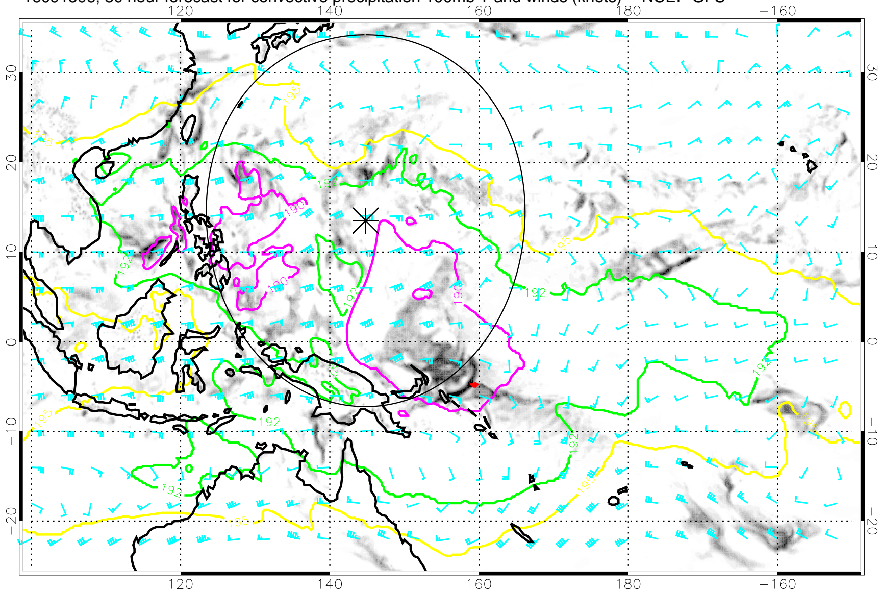
16091506, 30 hour forecast for convective precipitation 100mb T and winds (knots) -- NCEP GFS
