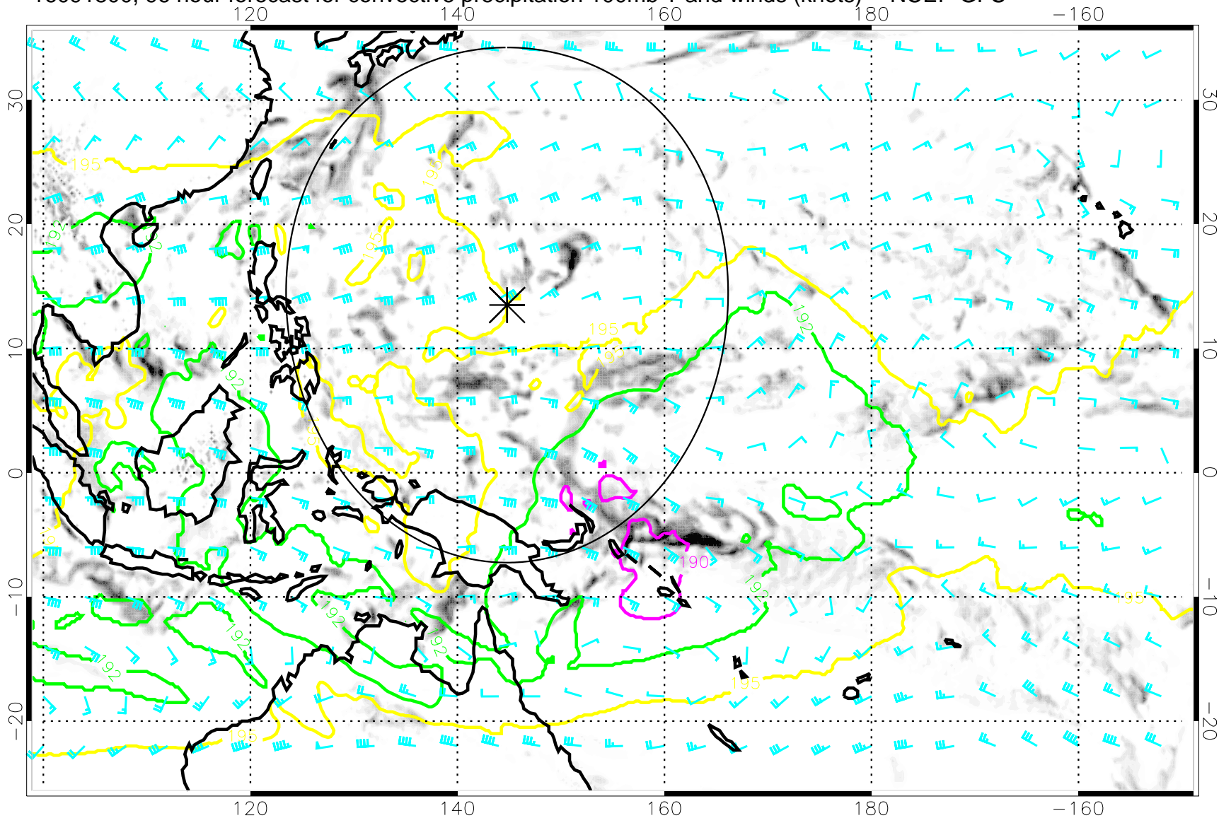
16091800, 96 hour forecast for convective precipitation 100mb T and winds (knots) -- NCEP GFS
