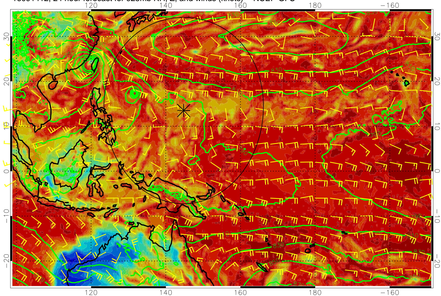
16091412, 24 hour forecast for 925mb RH, Z, and winds (knots) -- NCEP GFS
