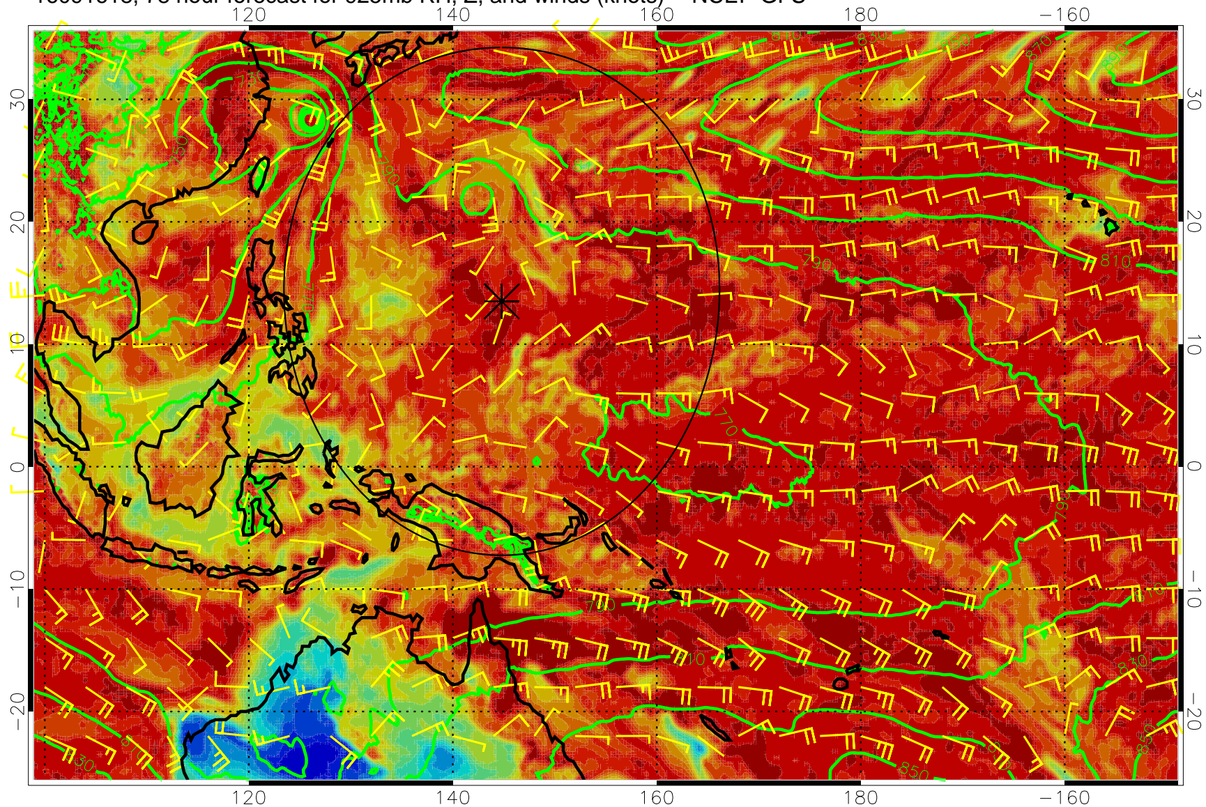
16091618, 78 hour forecast for 925mb RH, Z, and winds (knots) -- NCEP GFS
