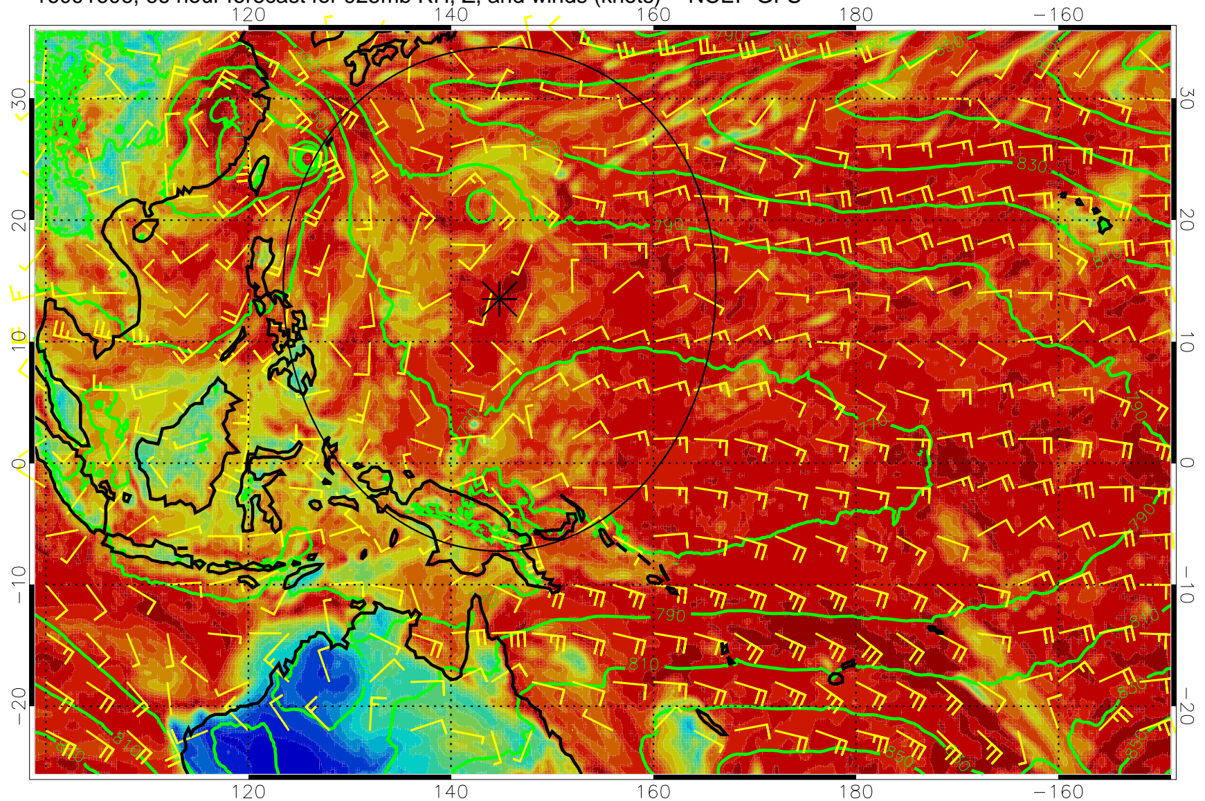
16091606, 66 hour forecast for 925mb RH, Z, and winds (knots) -- NCEP GFS
