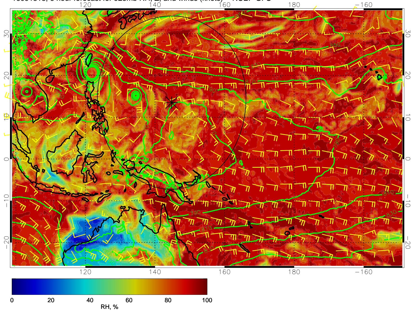
16091318, 6 hour forecast for 925mb RH, Z, and winds (knots) -- NCEP GFS
