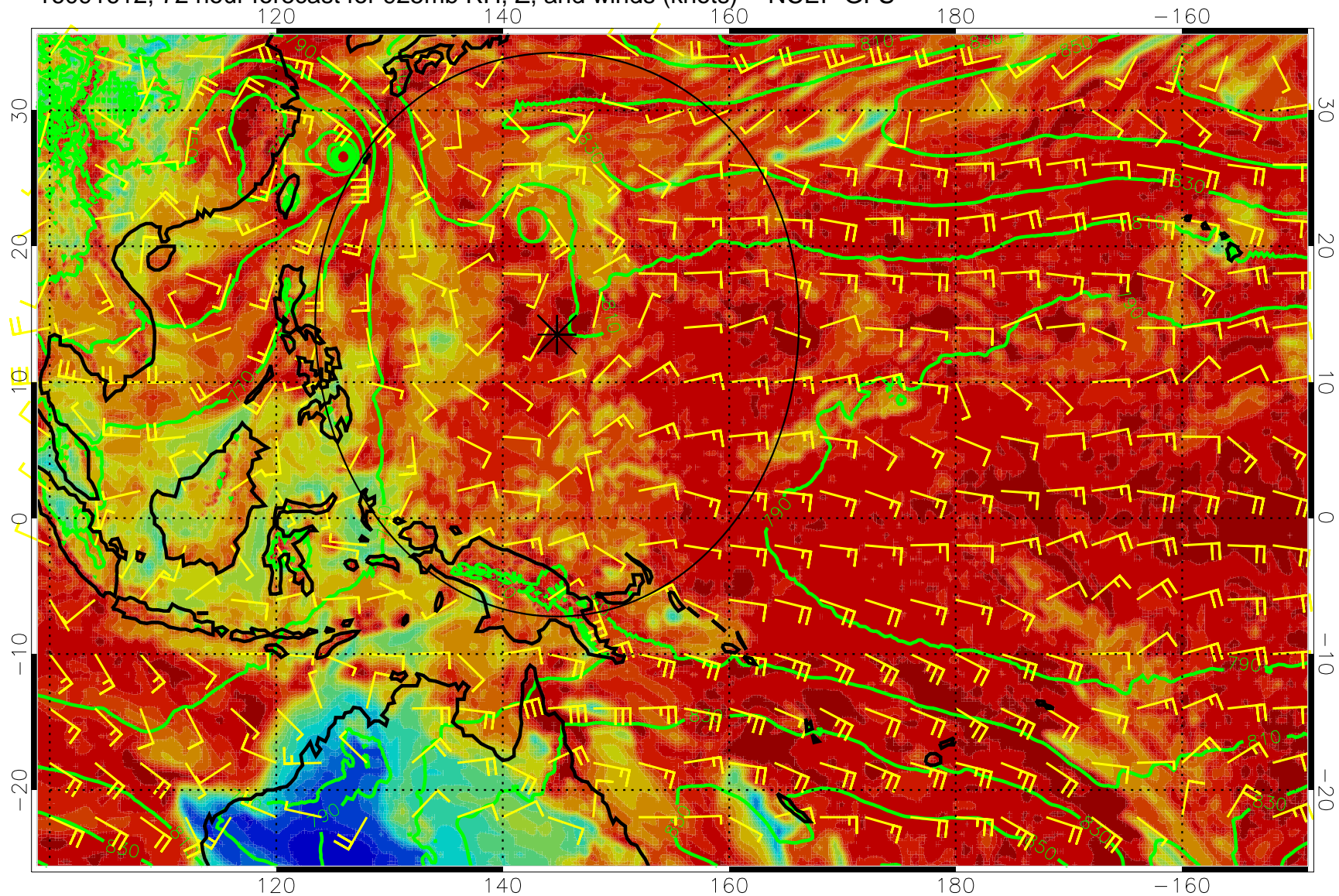
16091612, 72 hour forecast for 925mb RH, Z, and winds (knots) -- NCEP GFS
