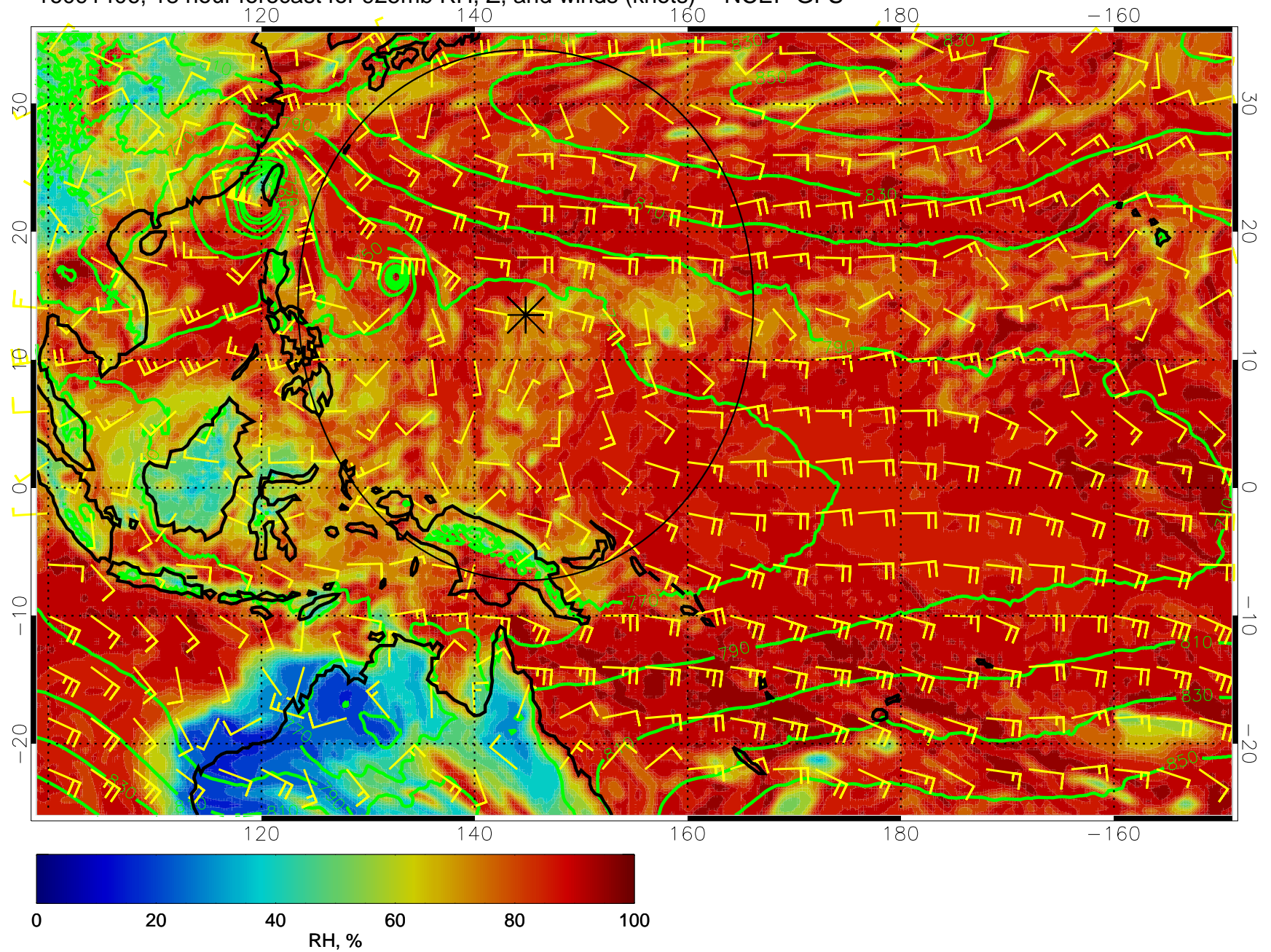
16091406, 18 hour forecast for 925mb RH, Z, and winds (knots) -- NCEP GFS
