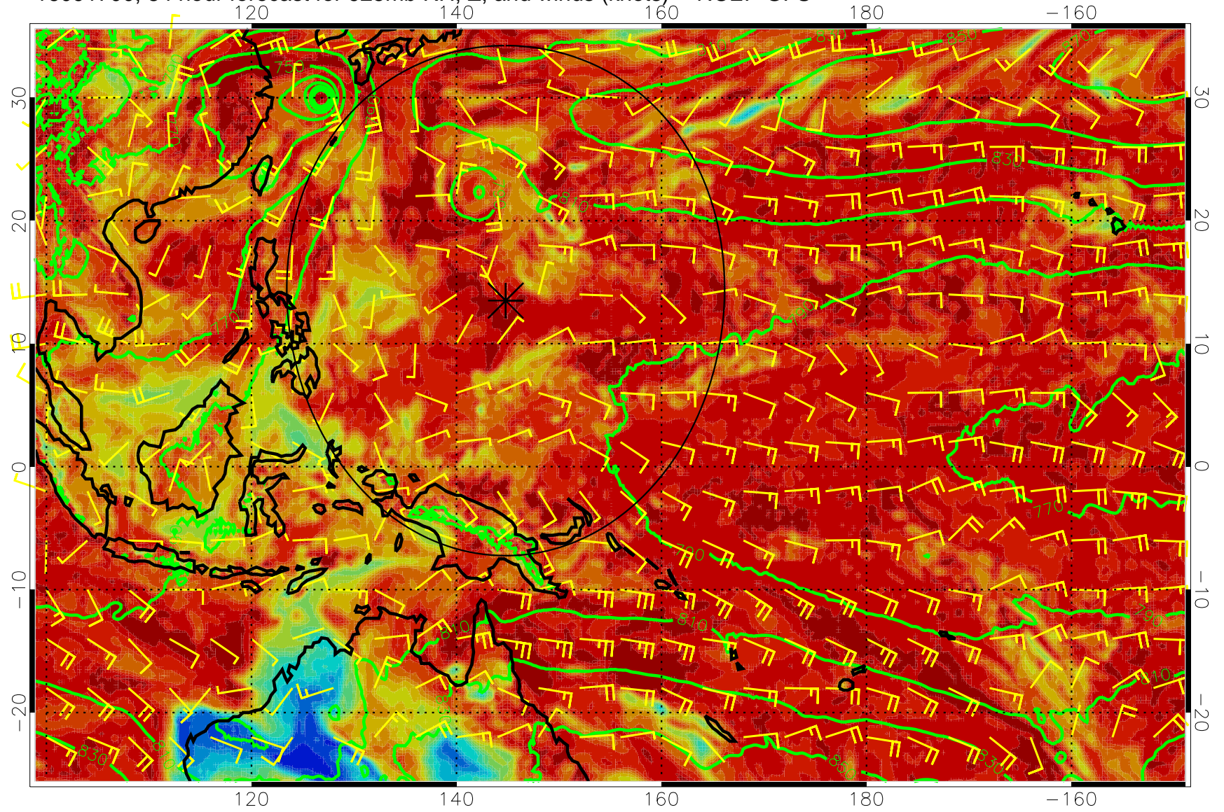
16091700, 84 hour forecast for 925mb RH, Z, and winds (knots) -- NCEP GFS
