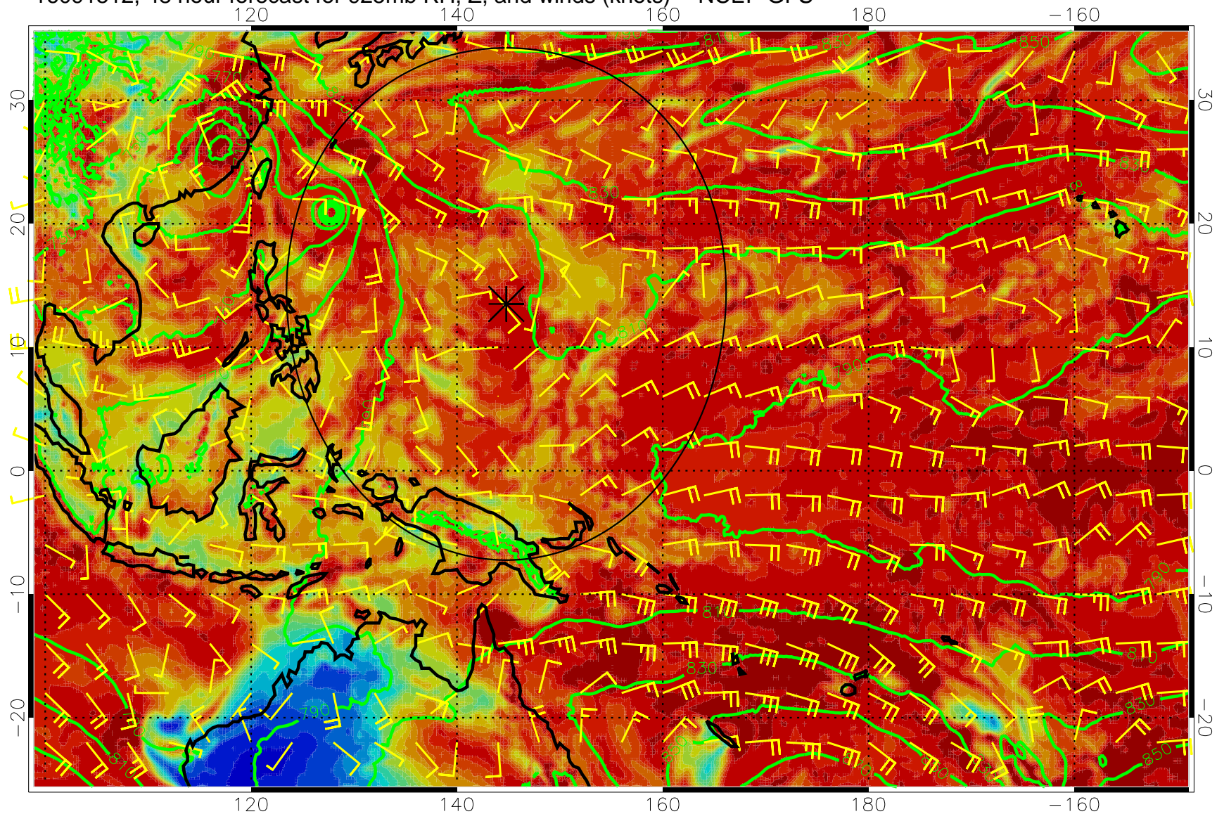
16091512, 48 hour forecast for 925mb RH, Z, and winds (knots) -- NCEP GFS
