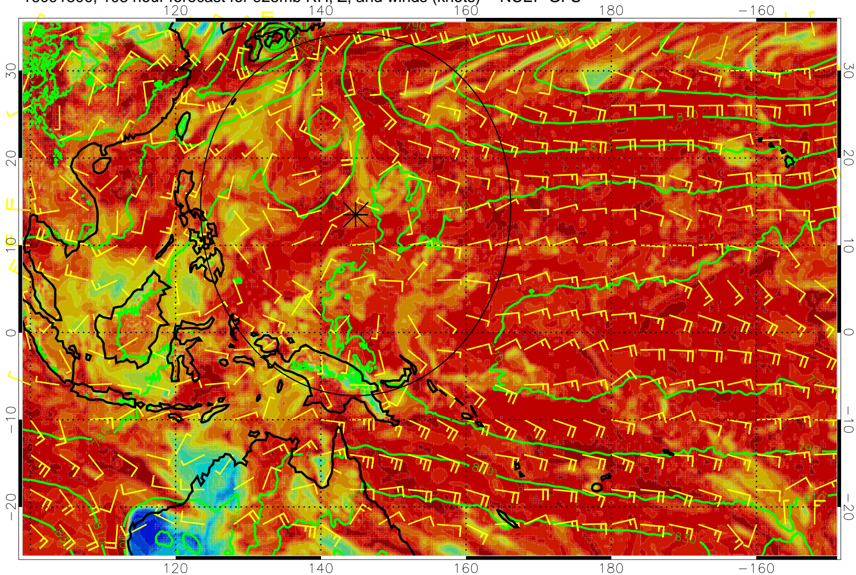
16091800, 108 hour forecast for 925mb RH, Z, and winds (knots) -- NCEP GFS
