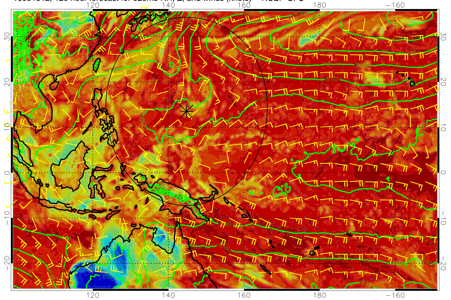
16091812, 120 hour forecast for 925mb RH, Z, and winds (knots) -- NCEP GFS
