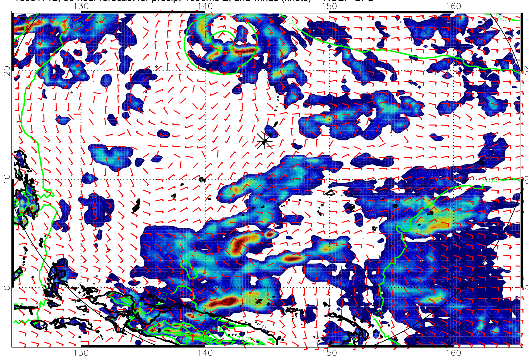
16091712, 96 hour forecast for precip, 1000mb Z, and winds (knots) -- NCEP GFS
