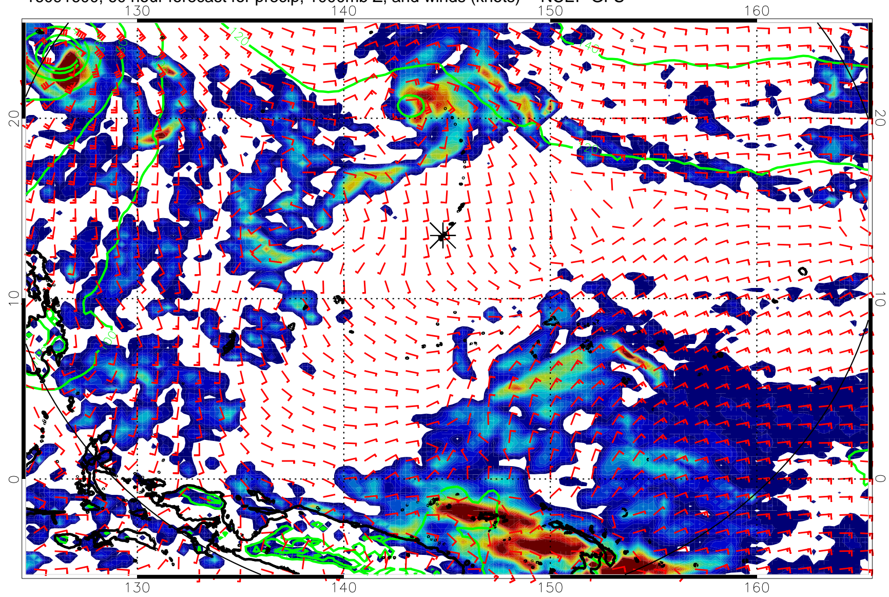
16091600, 60 hour forecast for precip, 1000mb Z, and winds (knots) -- NCEP GFS
