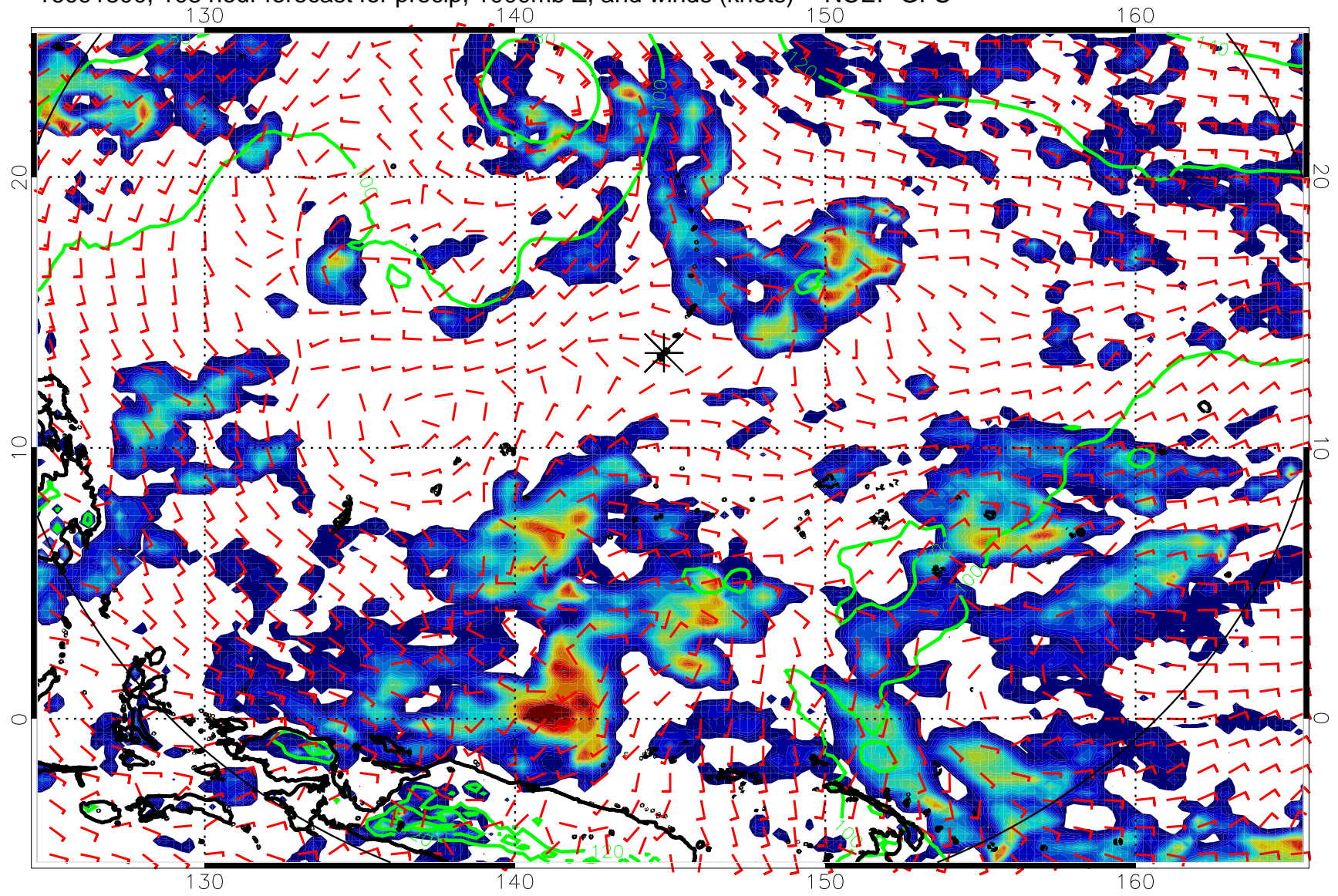
16091800, 108 hour forecast for precip, 1000mb Z, and winds (knots) -- NCEP GFS
