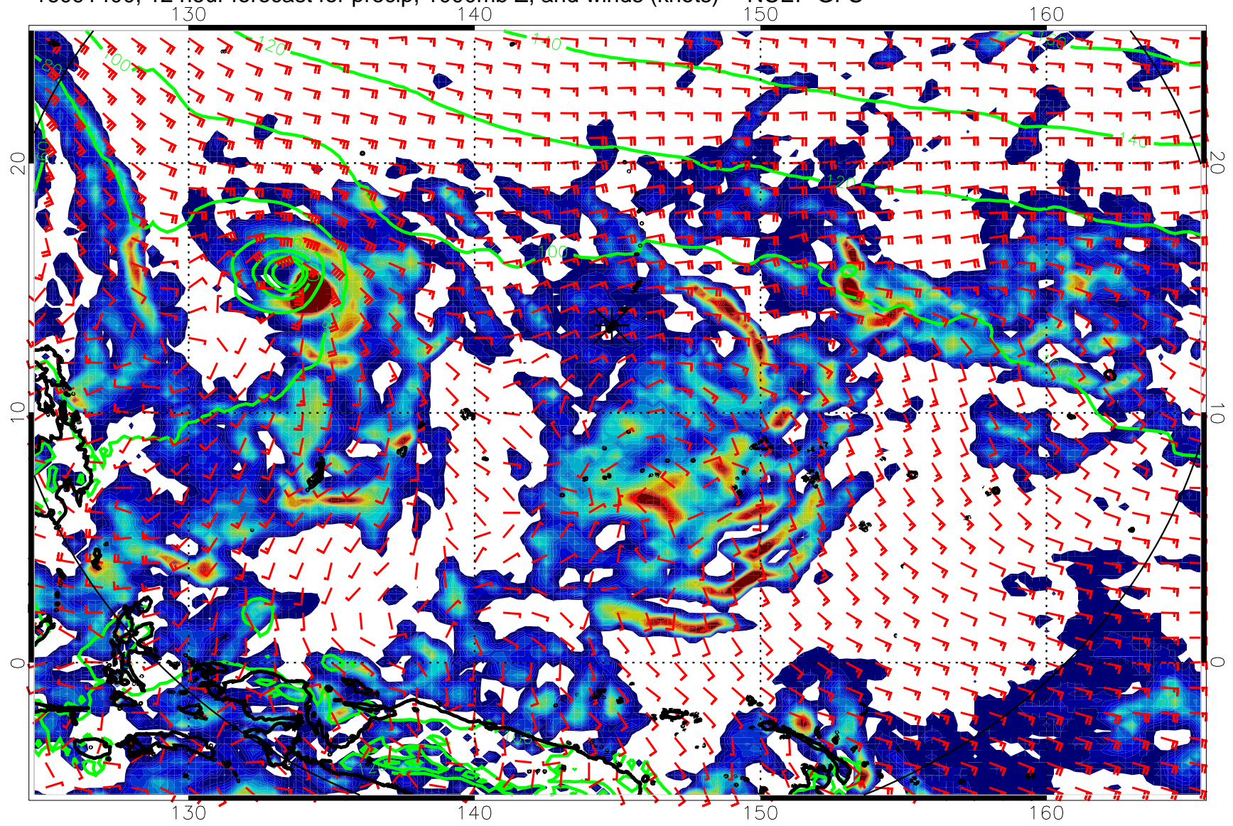
16091400, 12 hour forecast for precip, 1000mb Z, and winds (knots) -- NCEP GFS
