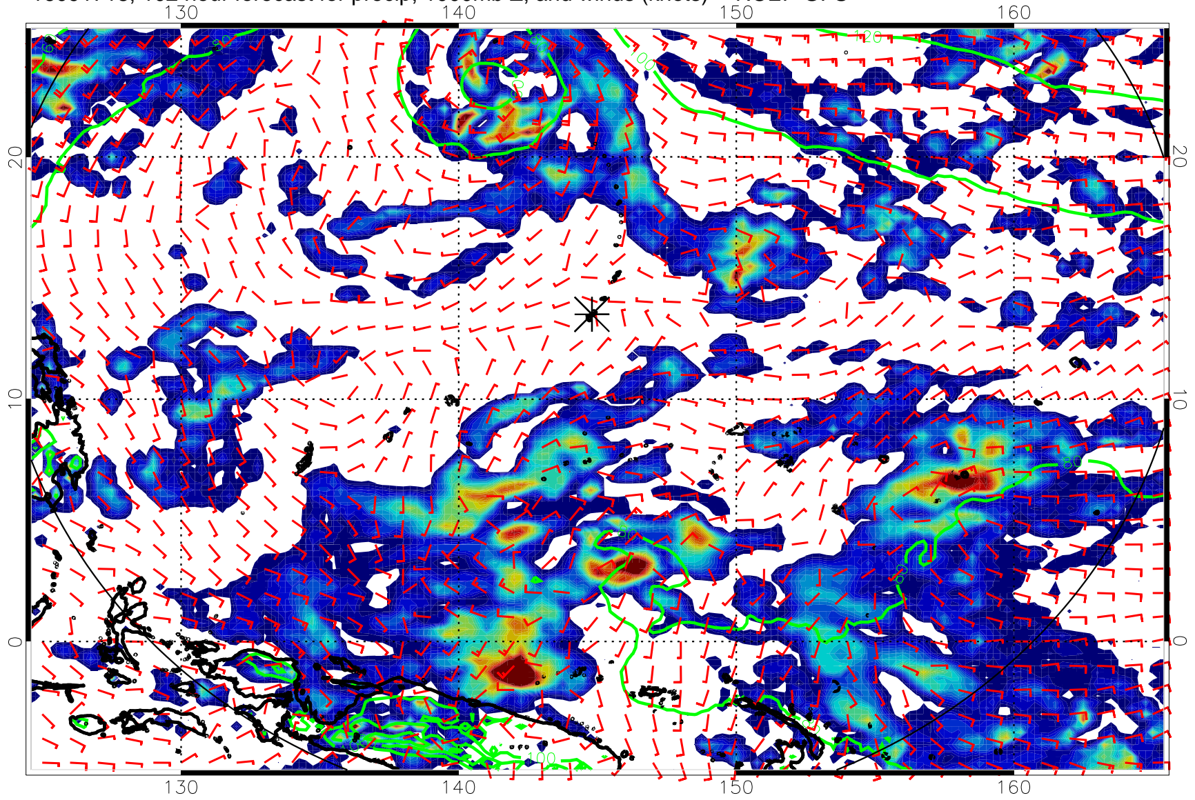
16091718, 102 hour forecast for precip, 1000mb Z, and winds (knots) -- NCEP GFS
