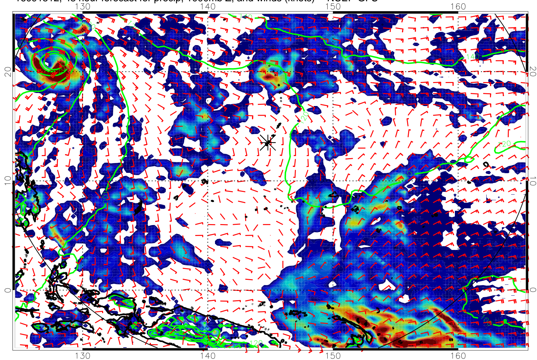
16091512, 48 hour forecast for precip, 1000mb Z, and winds (knots) -- NCEP GFS
