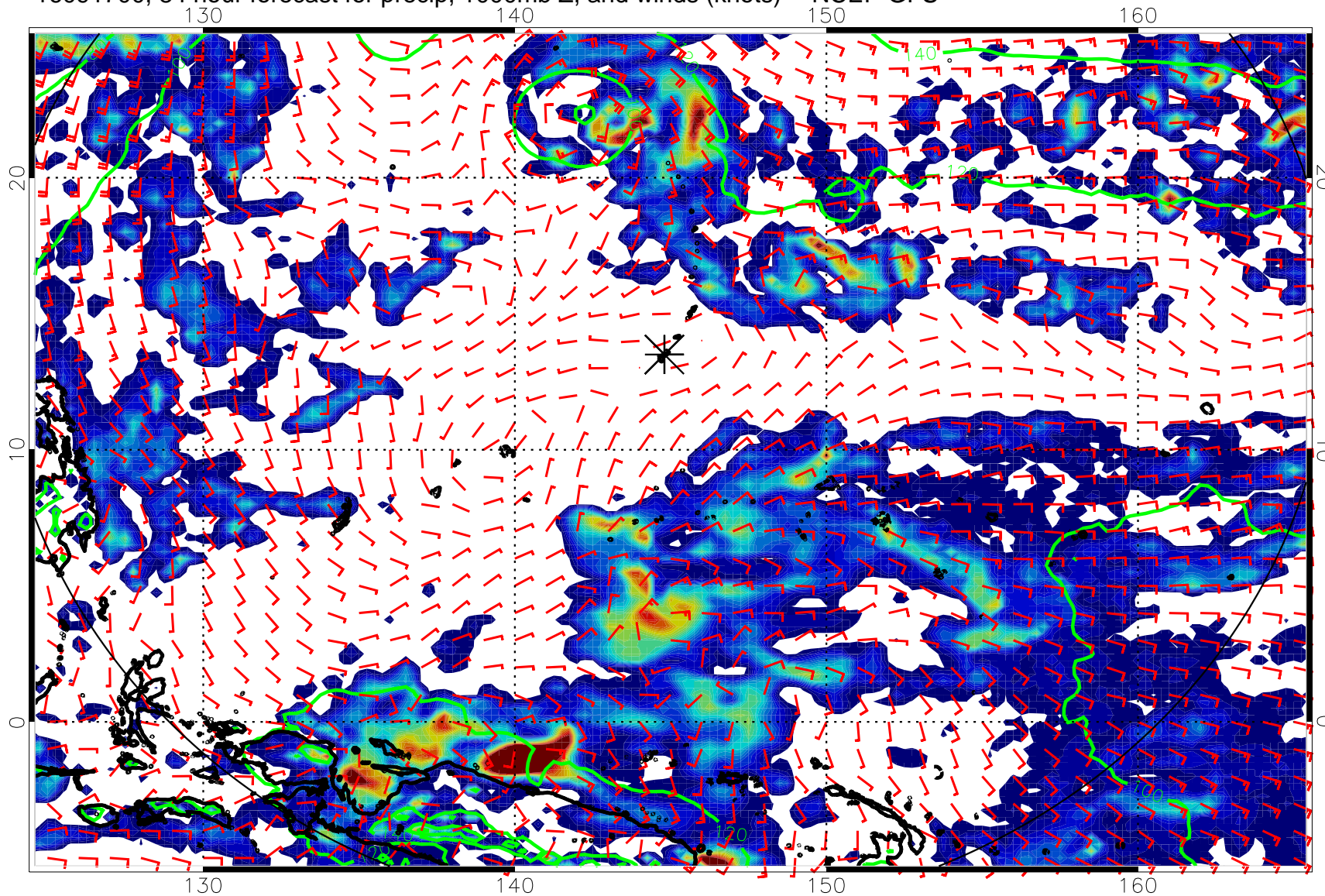
16091700, 84 hour forecast for precip, 1000mb Z, and winds (knots) -- NCEP GFS
