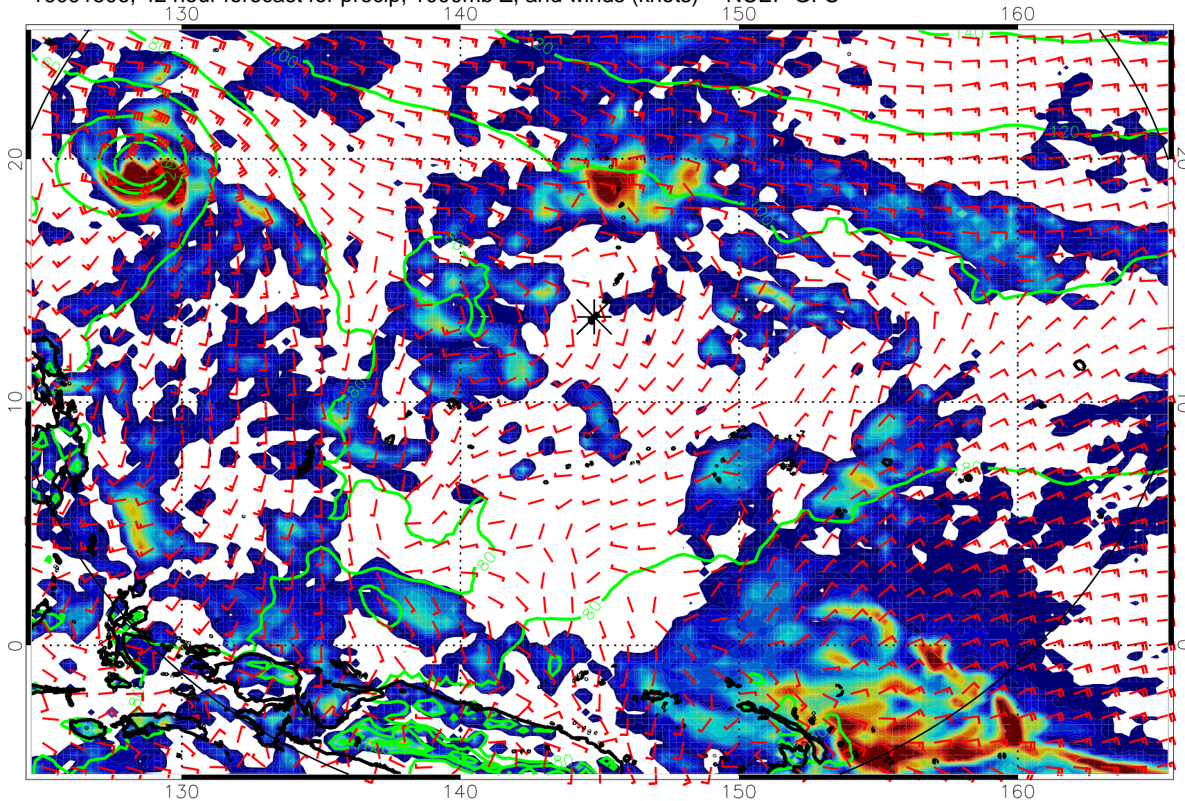
16091506, 42 hour forecast for precip, 1000mb Z, and winds (knots) -- NCEP GFS
