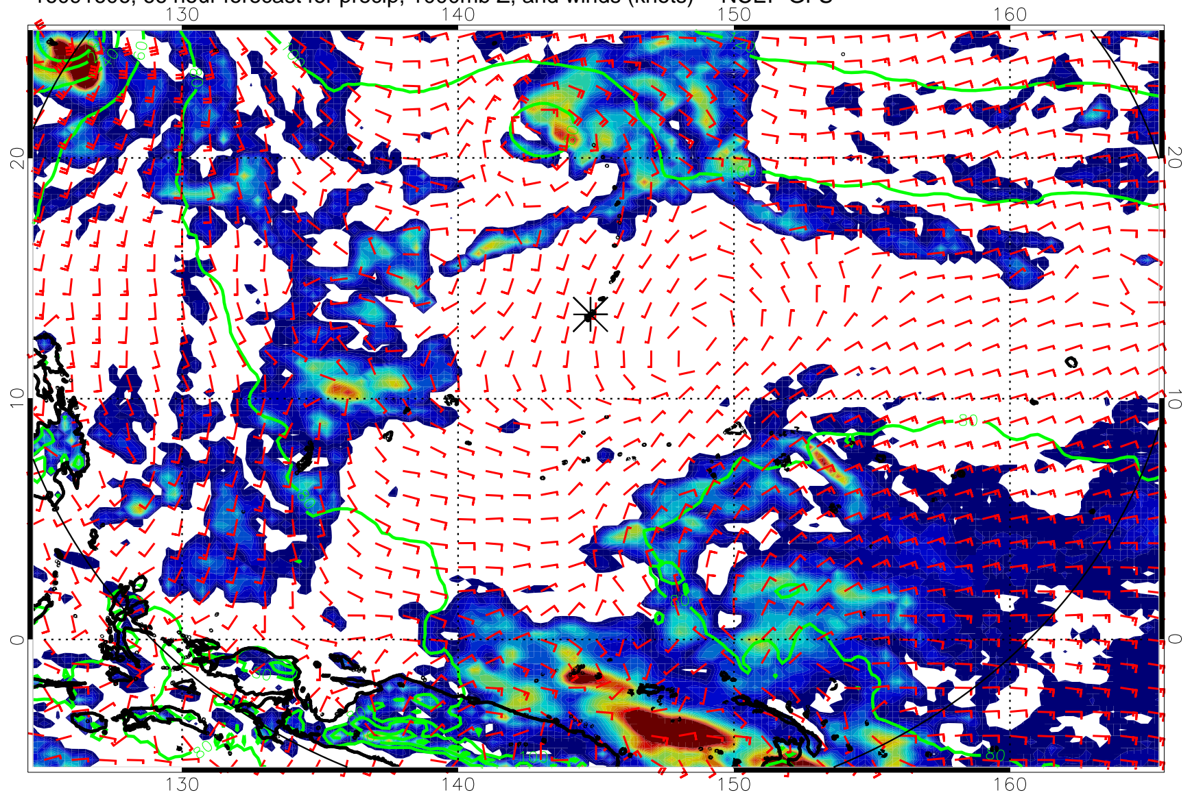
16091606, 66 hour forecast for precip, 1000mb Z, and winds (knots) -- NCEP GFS
