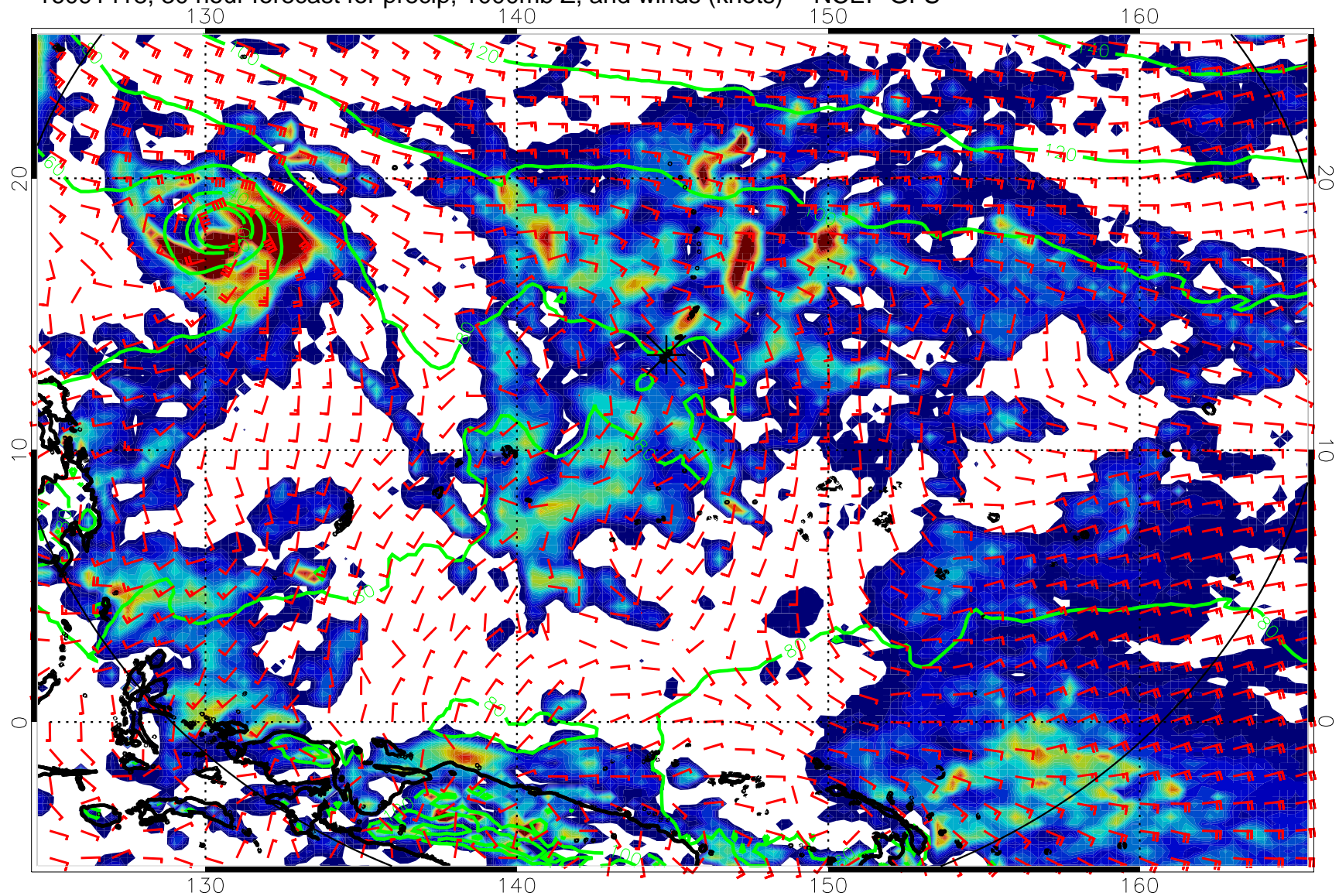
16091418, 30 hour forecast for precip, 1000mb Z, and winds (knots) -- NCEP GFS
