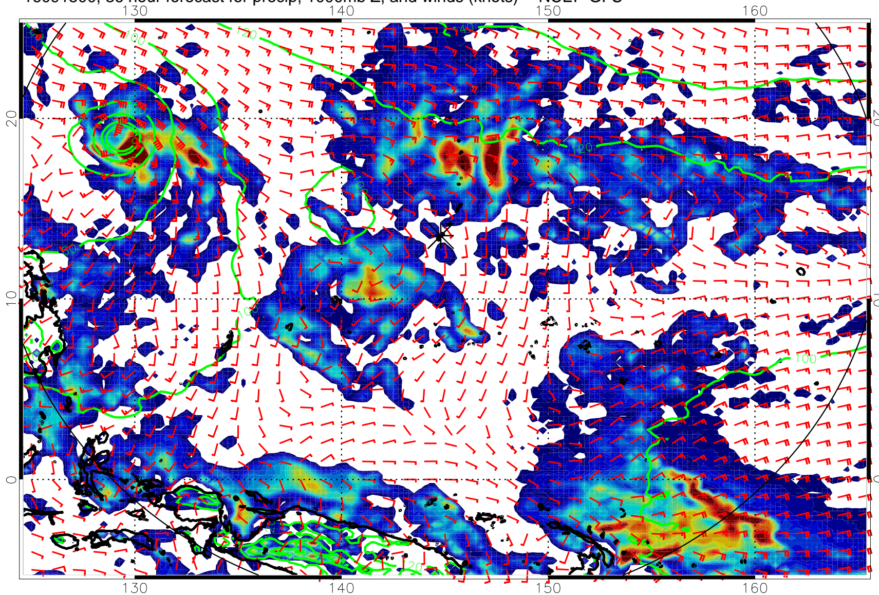
16091500, 36 hour forecast for precip, 1000mb Z, and winds (knots) -- NCEP GFS
