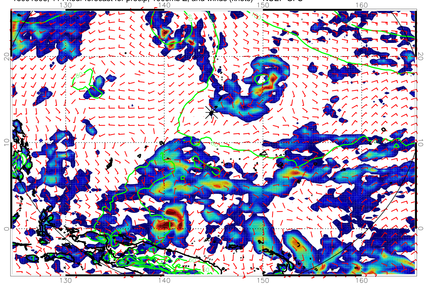
16091806, 114 hour forecast for precip, 1000mb Z, and winds (knots) -- NCEP GFS
