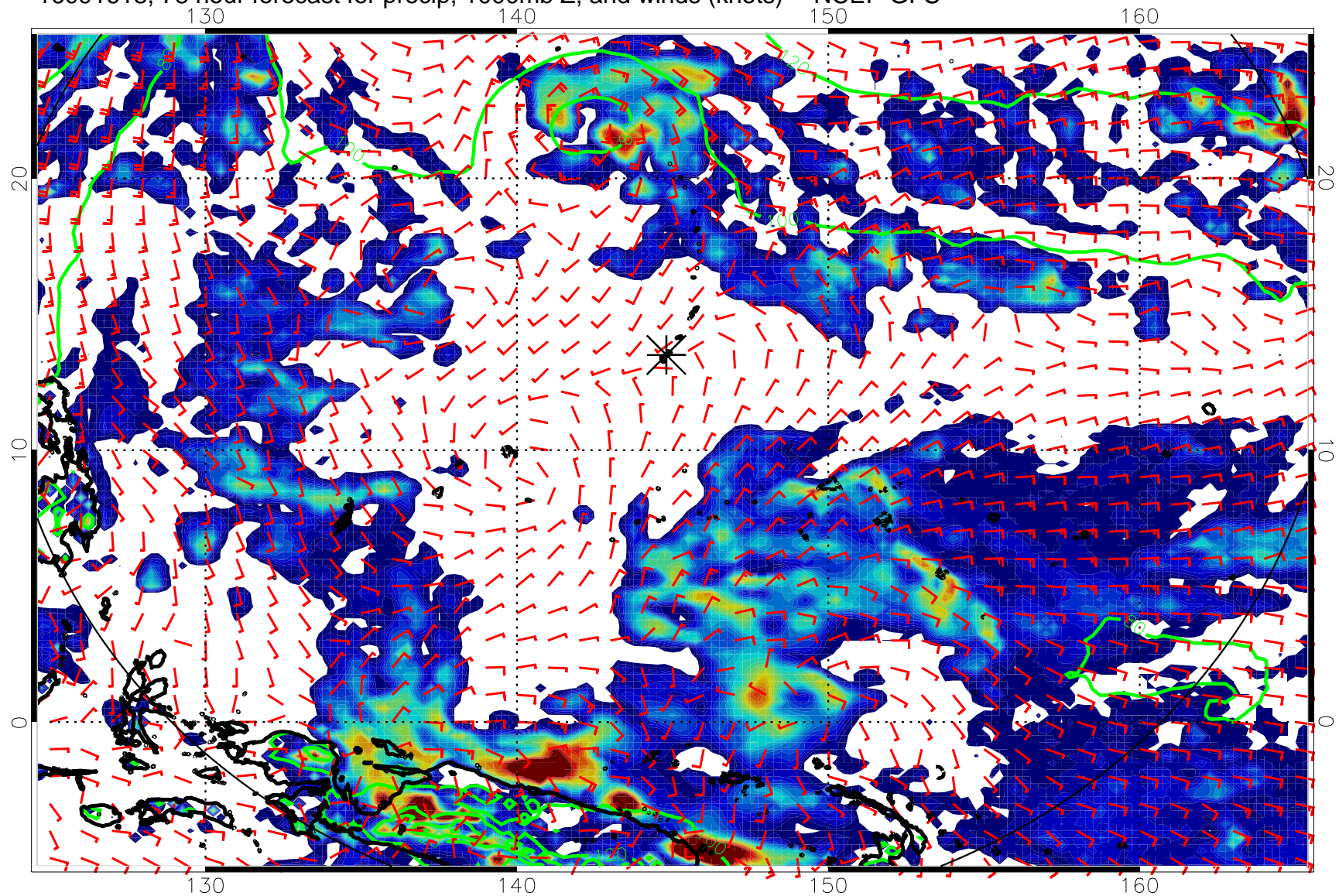
16091618, 78 hour forecast for precip, 1000mb Z, and winds (knots) -- NCEP GFS
