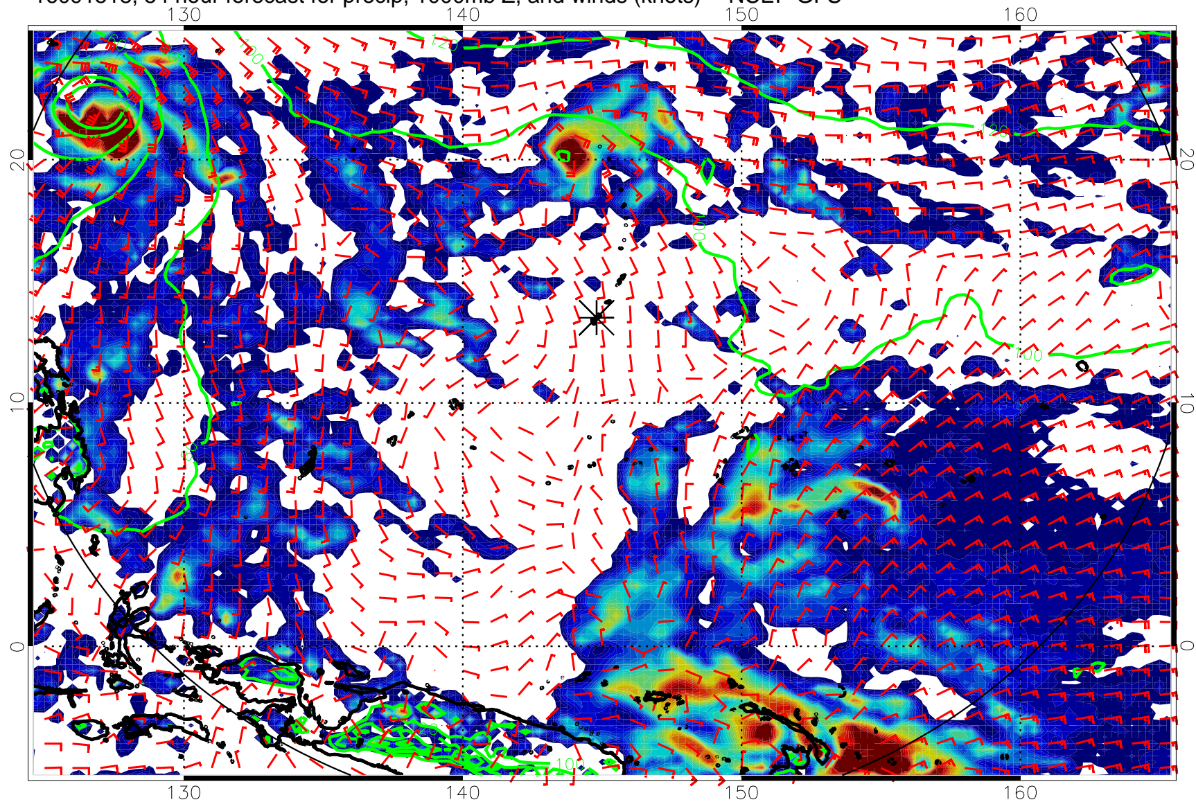
16091518, 54 hour forecast for precip, 1000mb Z, and winds (knots) -- NCEP GFS
