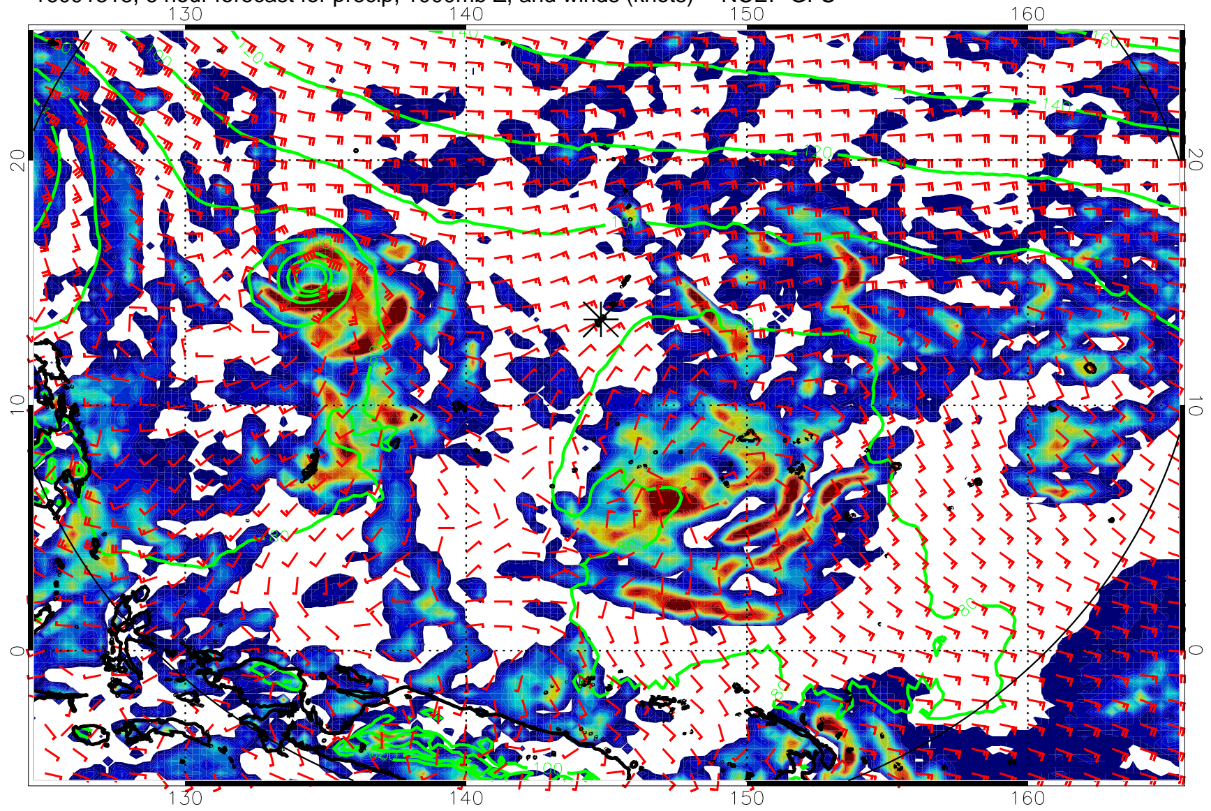
16091318, 6 hour forecast for precip, 1000mb Z, and winds (knots) -- NCEP GFS
