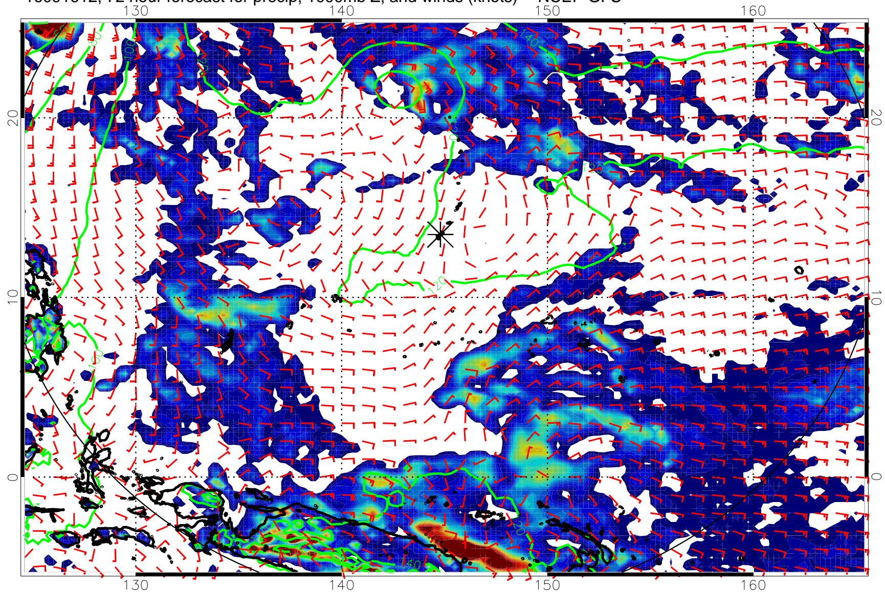
16091612, 72 hour forecast for precip, 1000mb Z, and winds (knots) -- NCEP GFS
