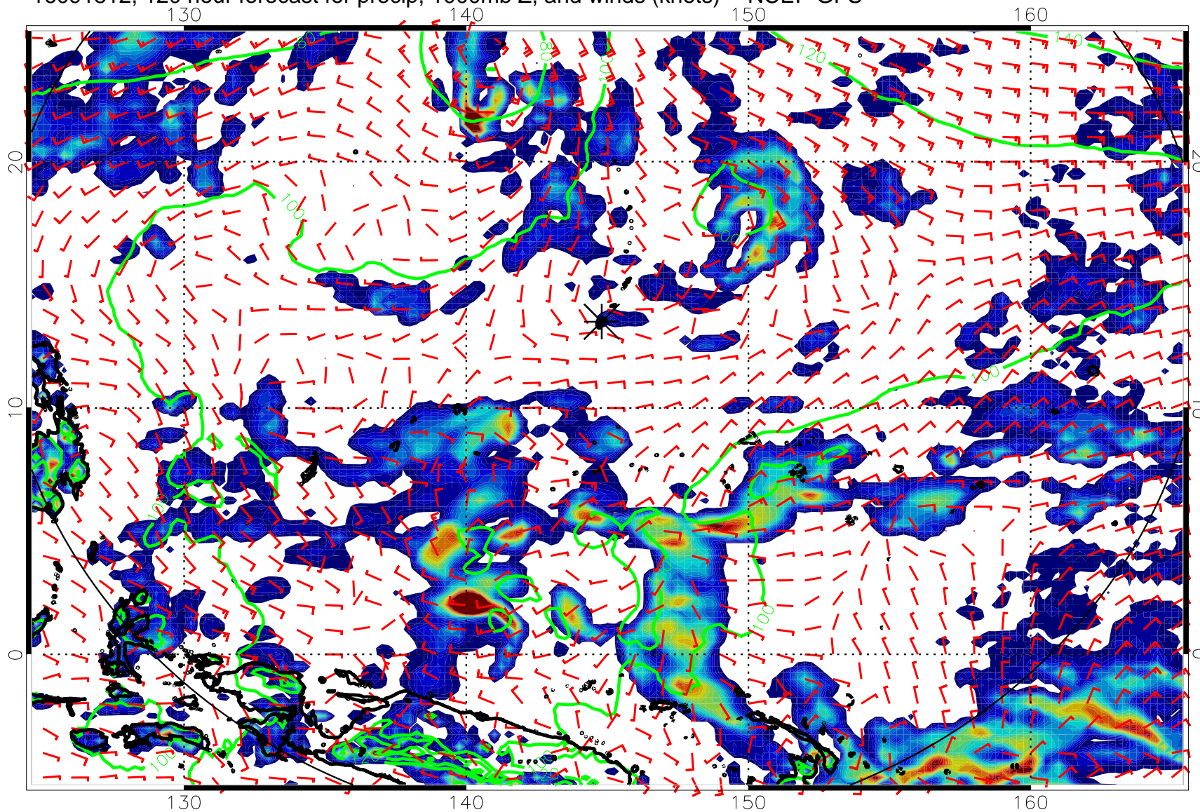
16091812, 120 hour forecast for precip, 1000mb Z, and winds (knots) -- NCEP GFS
