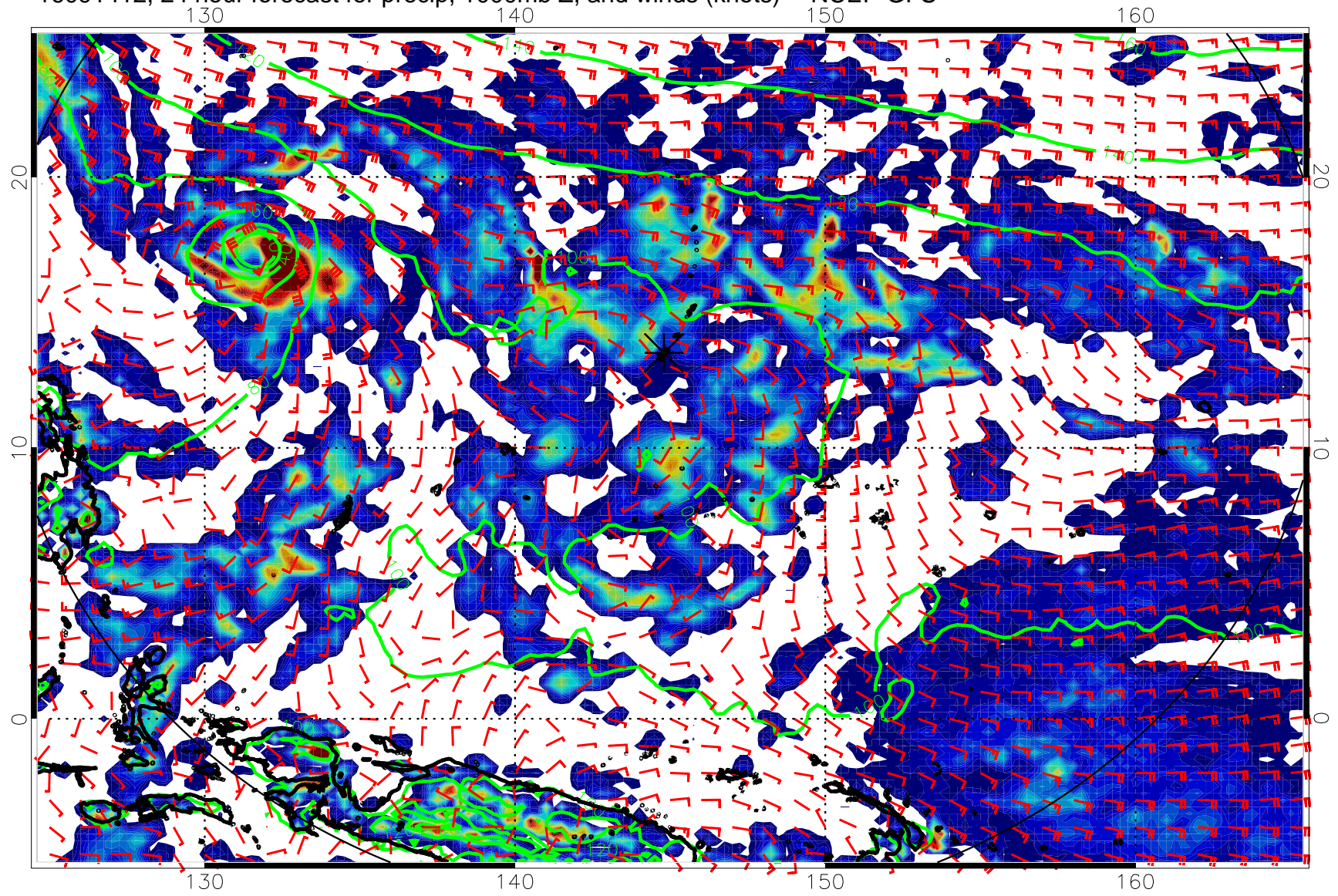
16091412, 24 hour forecast for precip, 1000mb Z, and winds (knots) -- NCEP GFS
