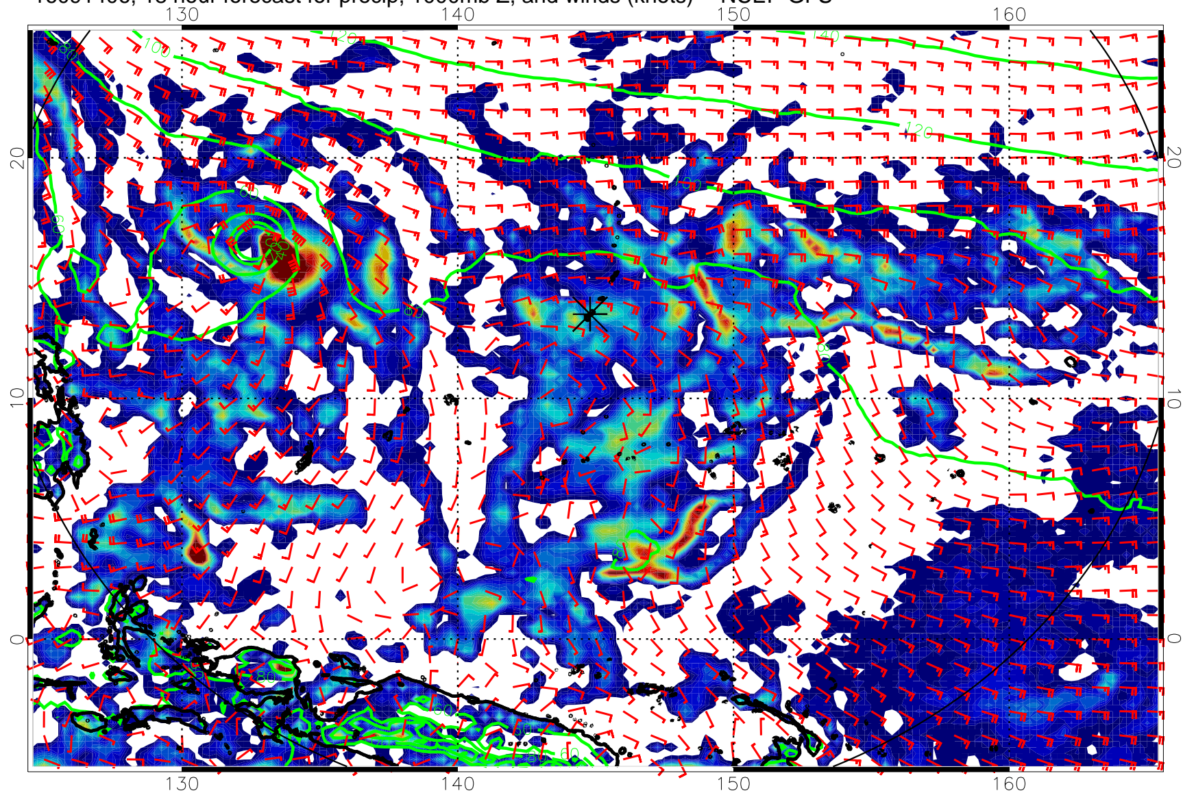
16091406, 18 hour forecast for precip, 1000mb Z, and winds (knots) -- NCEP GFS
