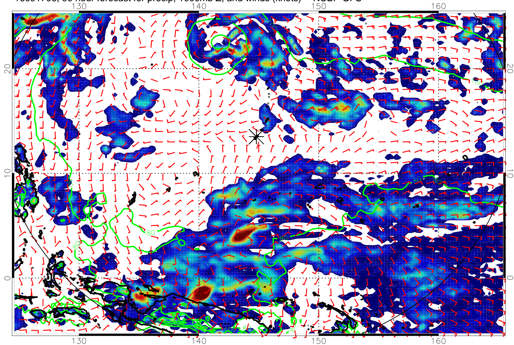
16091706, 90 hour forecast for precip, 1000mb Z, and winds (knots) -- NCEP GFS
