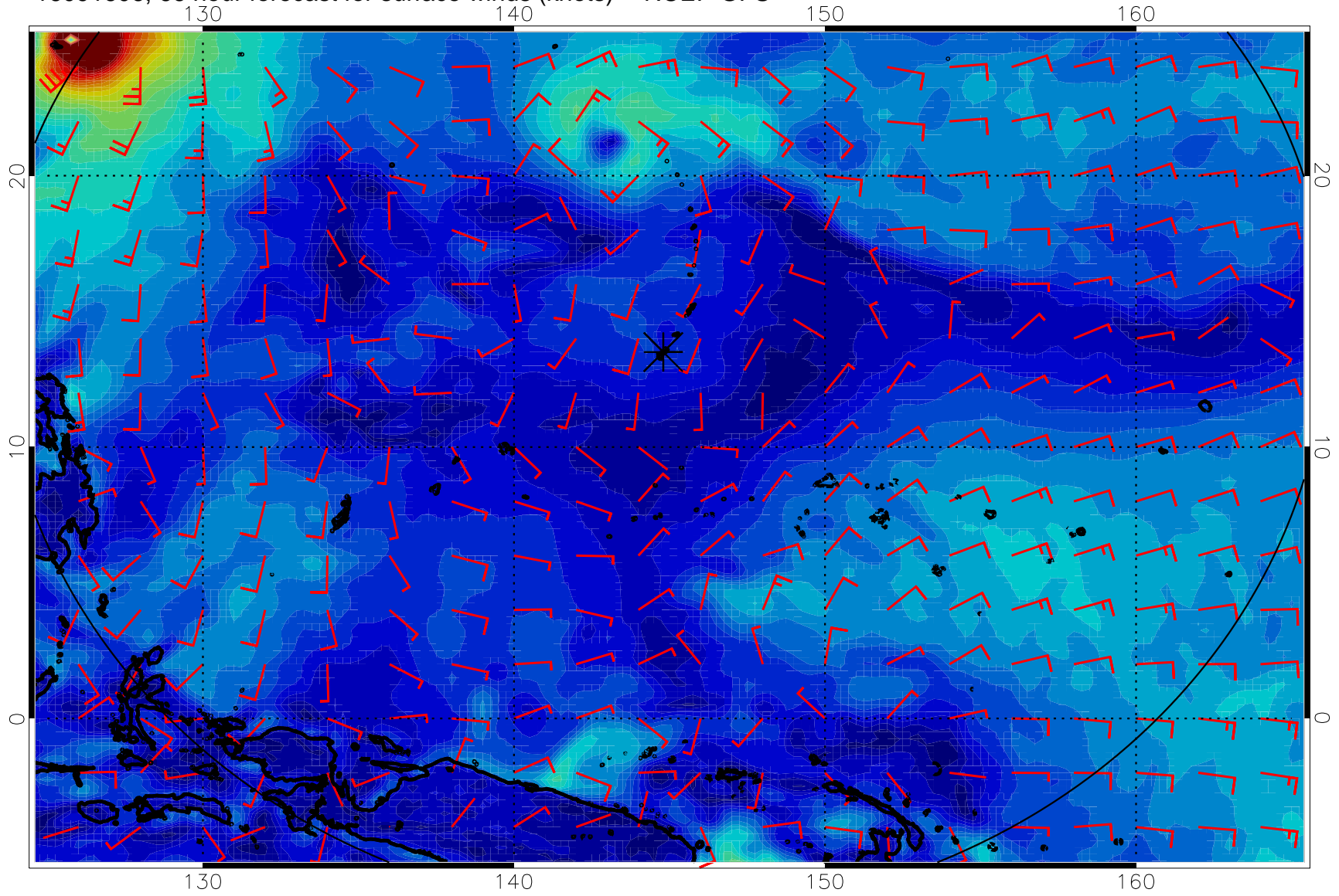
16091606, 66 hour forecast for surface winds (knots) -- NCEP GFS
