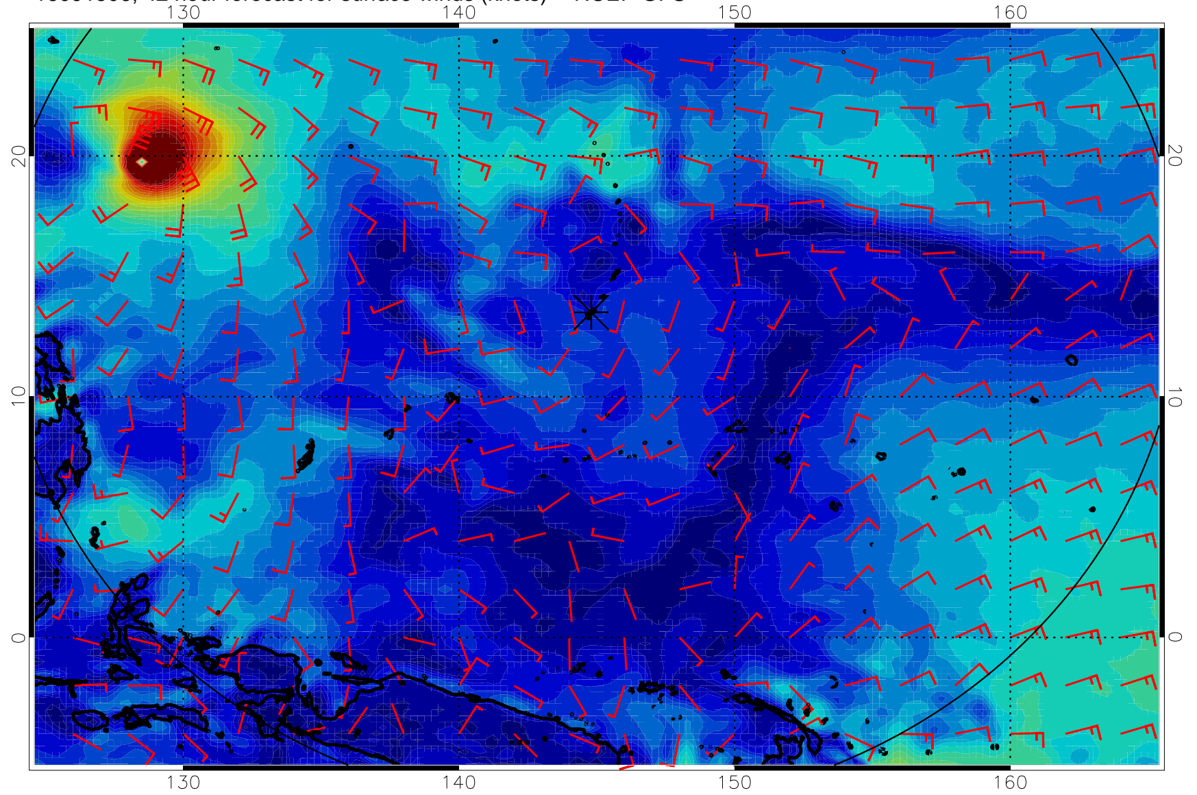
16091506, 42 hour forecast for surface winds (knots) -- NCEP GFS
