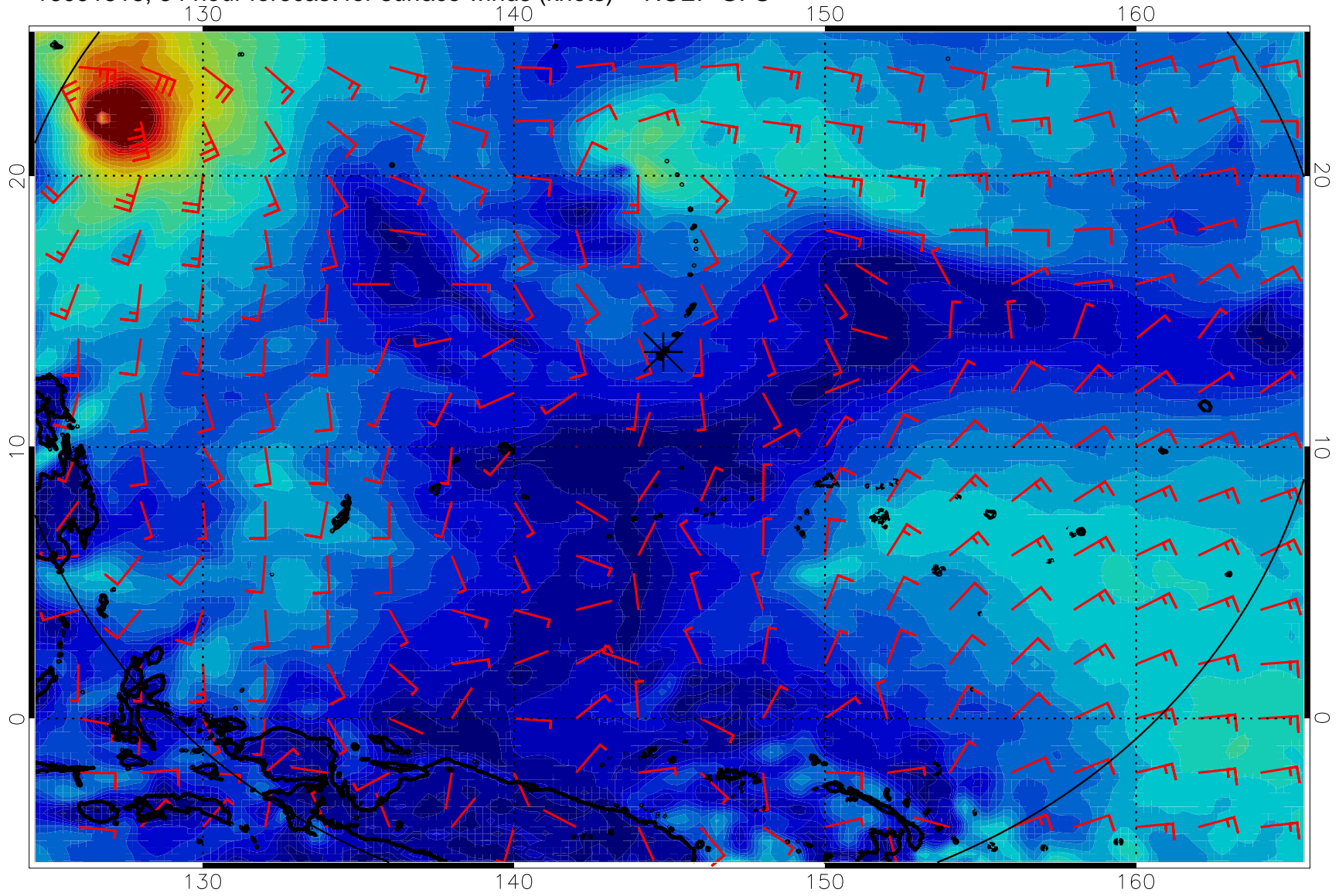
16091518, 54 hour forecast for surface winds (knots) -- NCEP GFS
