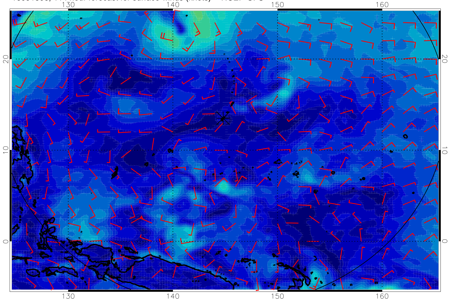
16091806, 114 hour forecast for surface winds (knots) -- NCEP GFS
