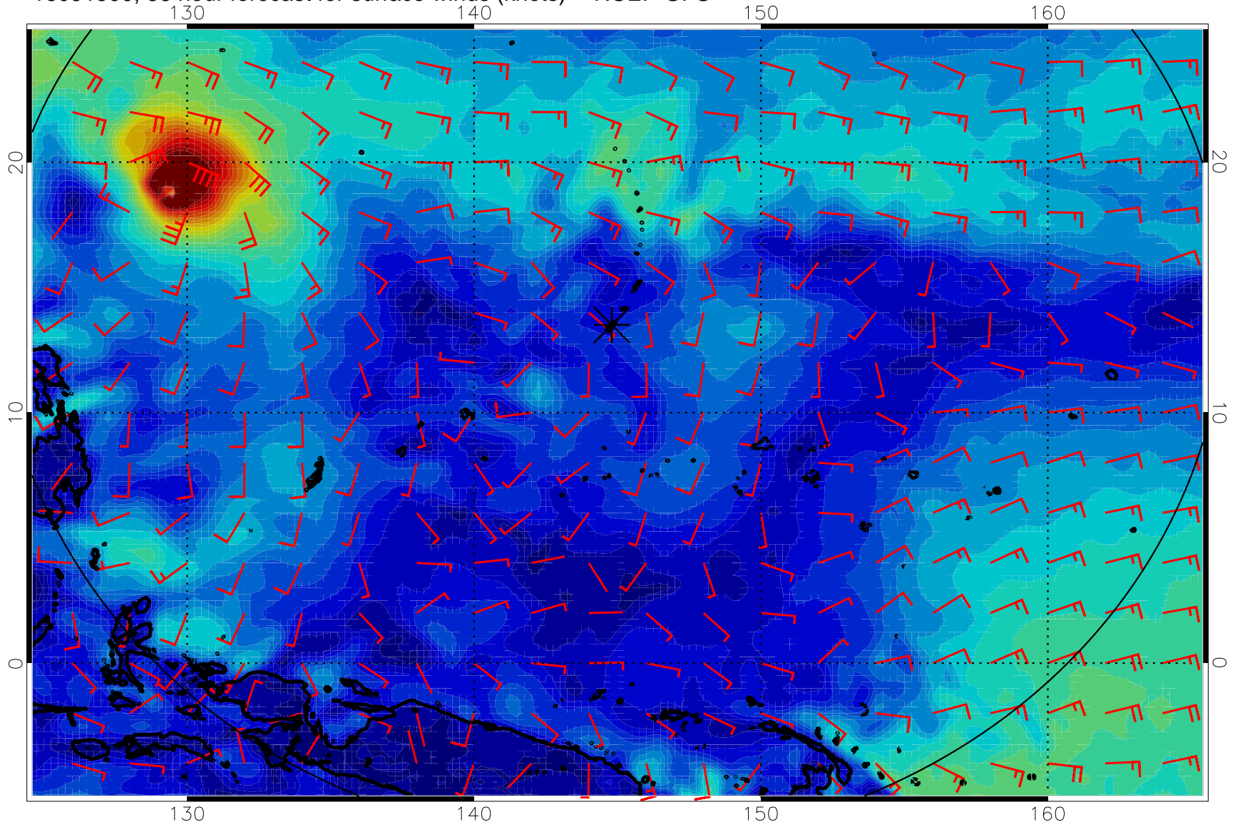
16091500, 36 hour forecast for surface winds (knots) -- NCEP GFS
