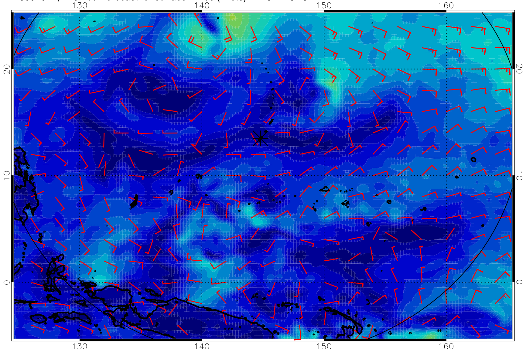
16091812, 120 hour forecast for surface winds (knots) -- NCEP GFS
