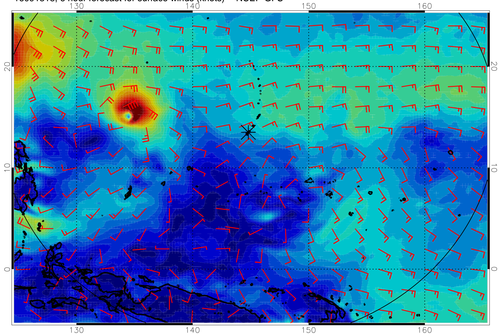
16091318, 6 hour forecast for surface winds (knots) -- NCEP GFS
