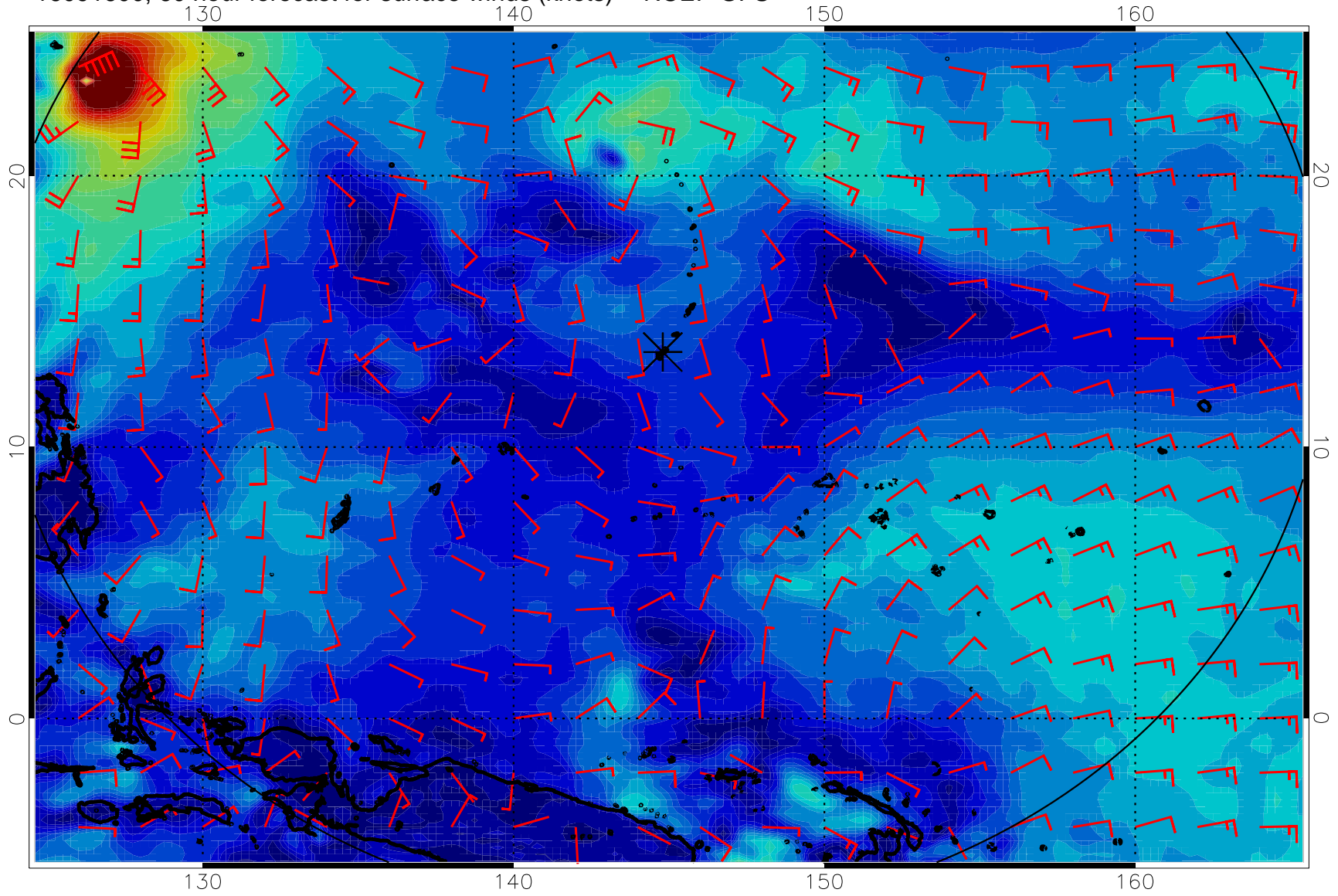
16091600, 60 hour forecast for surface winds (knots) -- NCEP GFS
