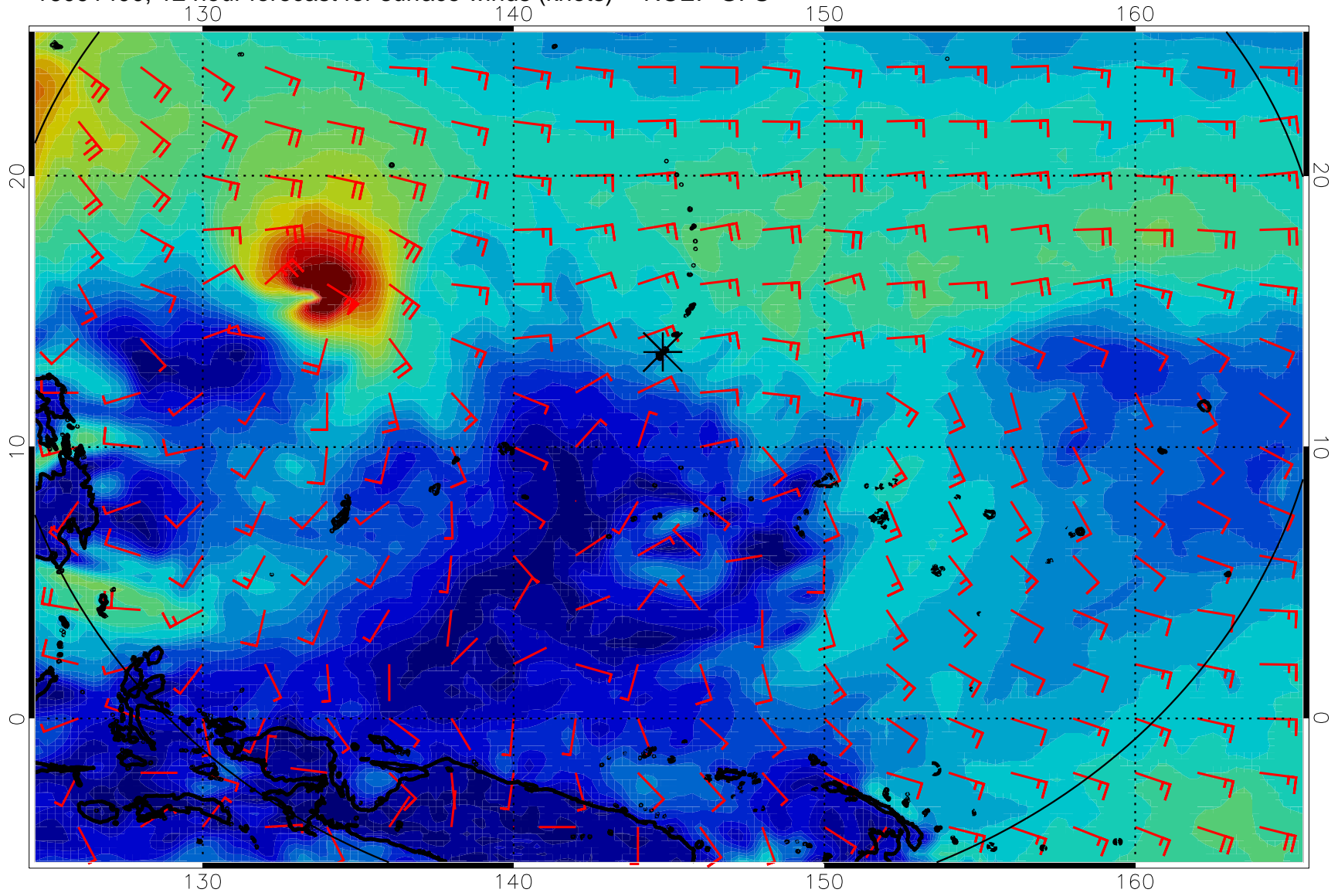
16091400, 12 hour forecast for surface winds (knots) -- NCEP GFS
