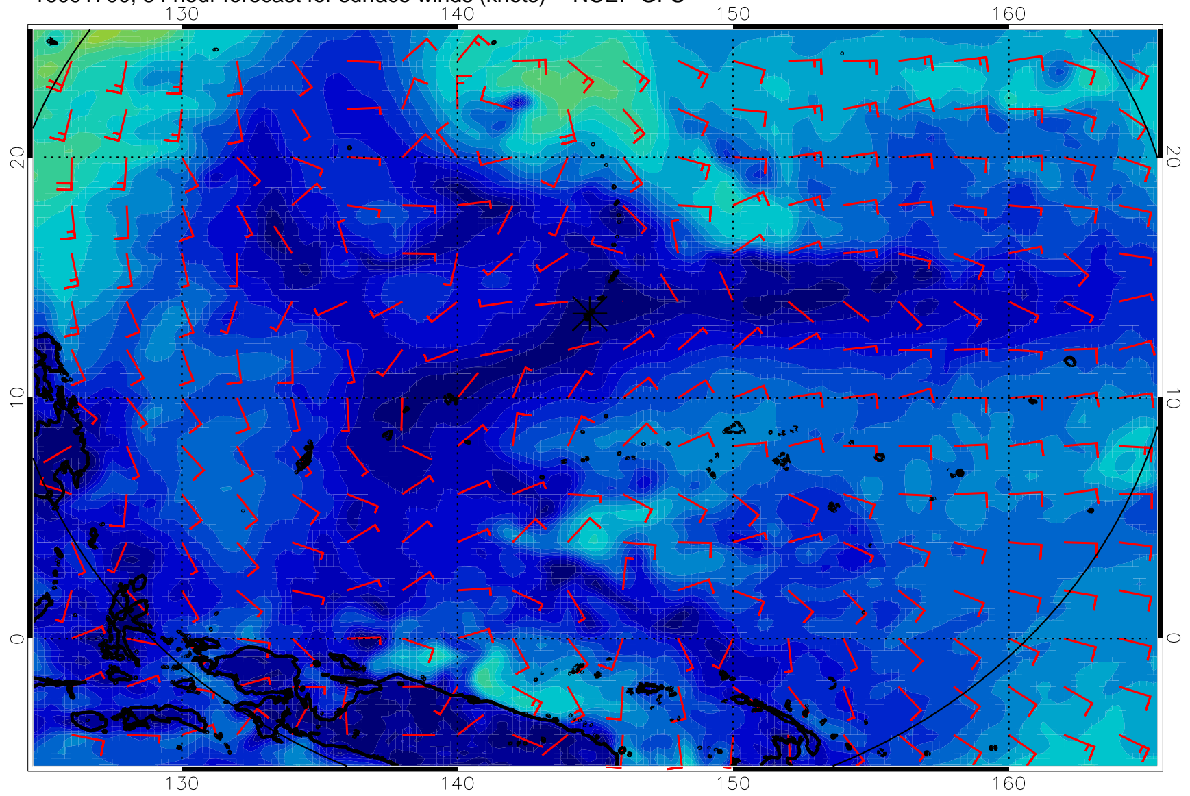
16091700, 84 hour forecast for surface winds (knots) -- NCEP GFS
