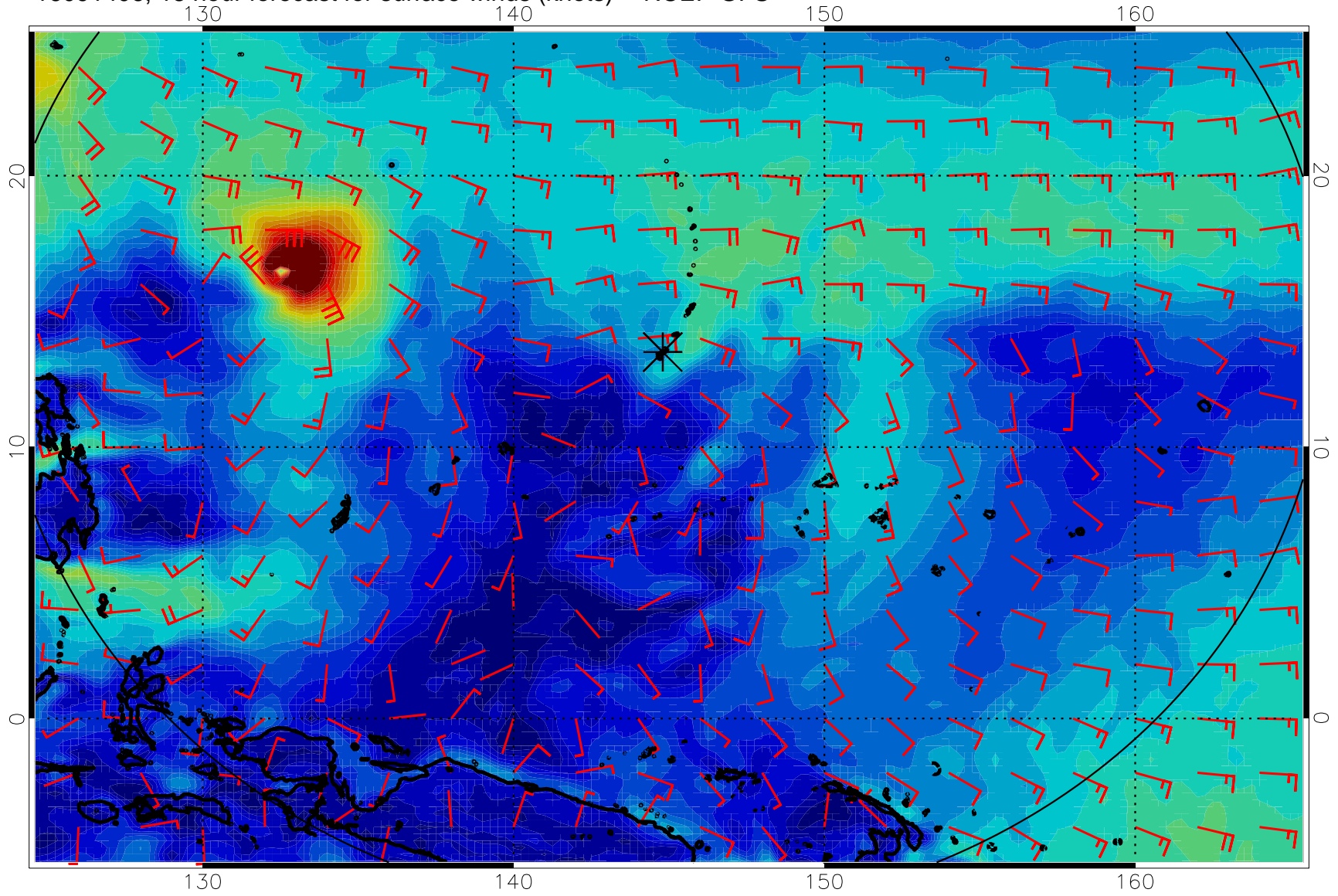
16091406, 18 hour forecast for surface winds (knots) -- NCEP GFS
