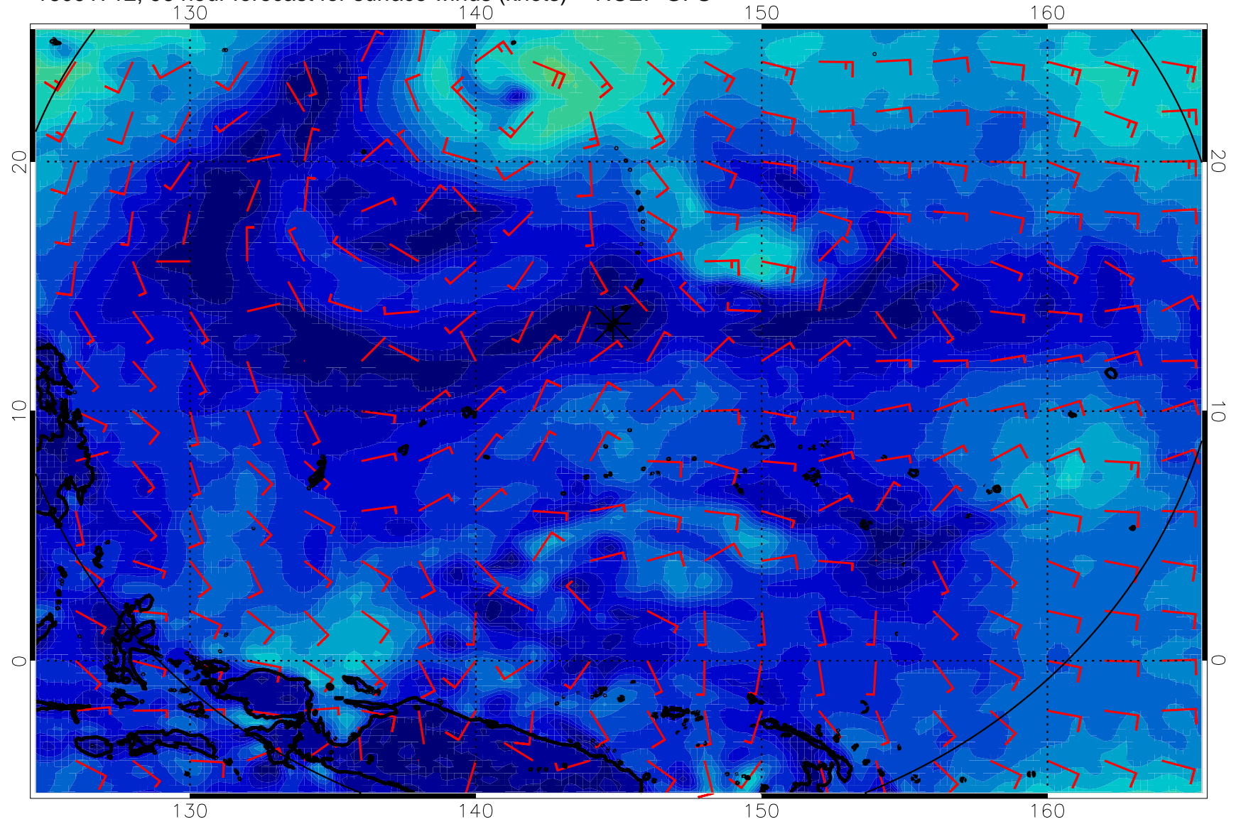
16091712, 96 hour forecast for surface winds (knots) -- NCEP GFS
