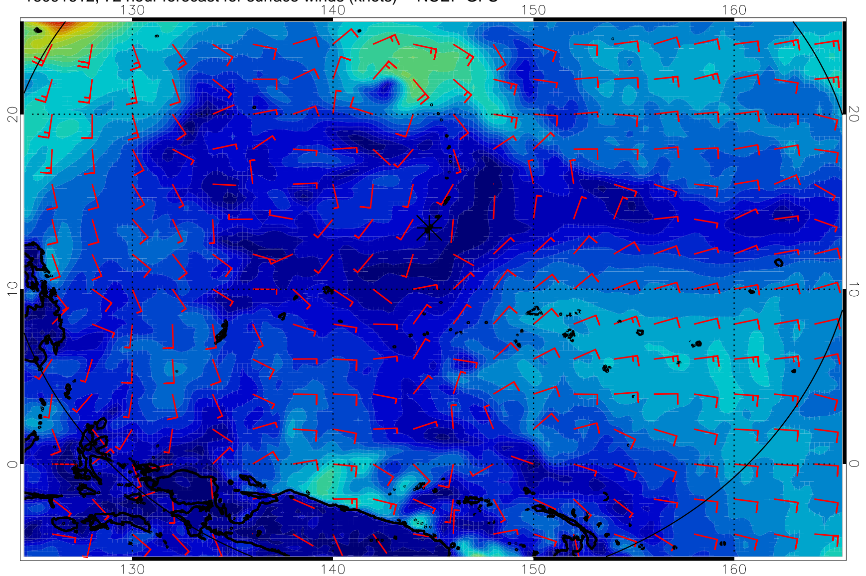
16091612, 72 hour forecast for surface winds (knots) -- NCEP GFS
