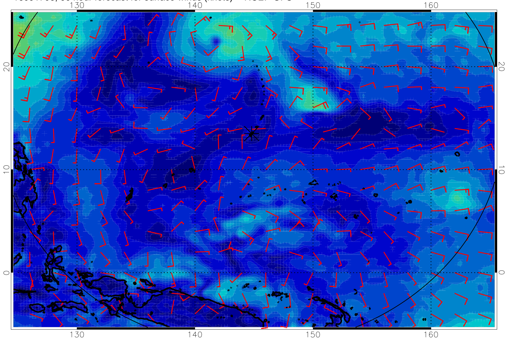
16091706, 90 hour forecast for surface winds (knots) -- NCEP GFS
