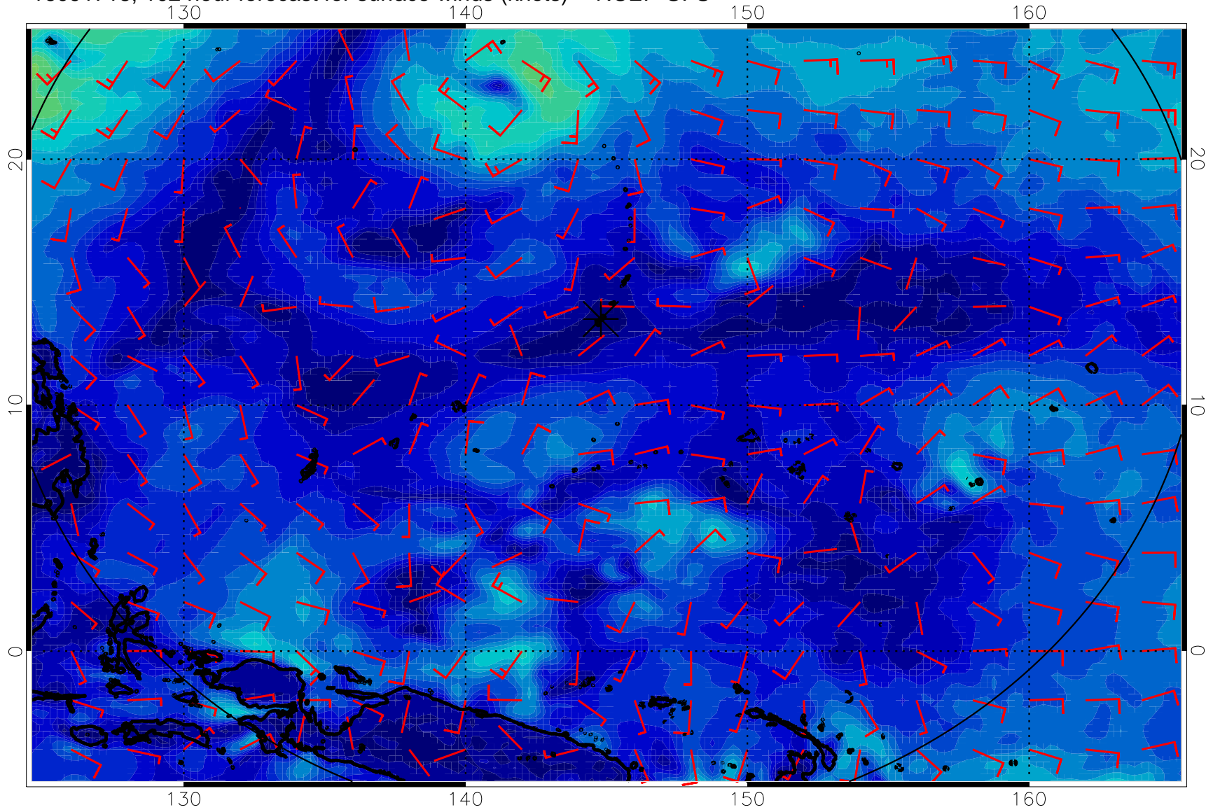
16091718, 102 hour forecast for surface winds (knots) -- NCEP GFS
