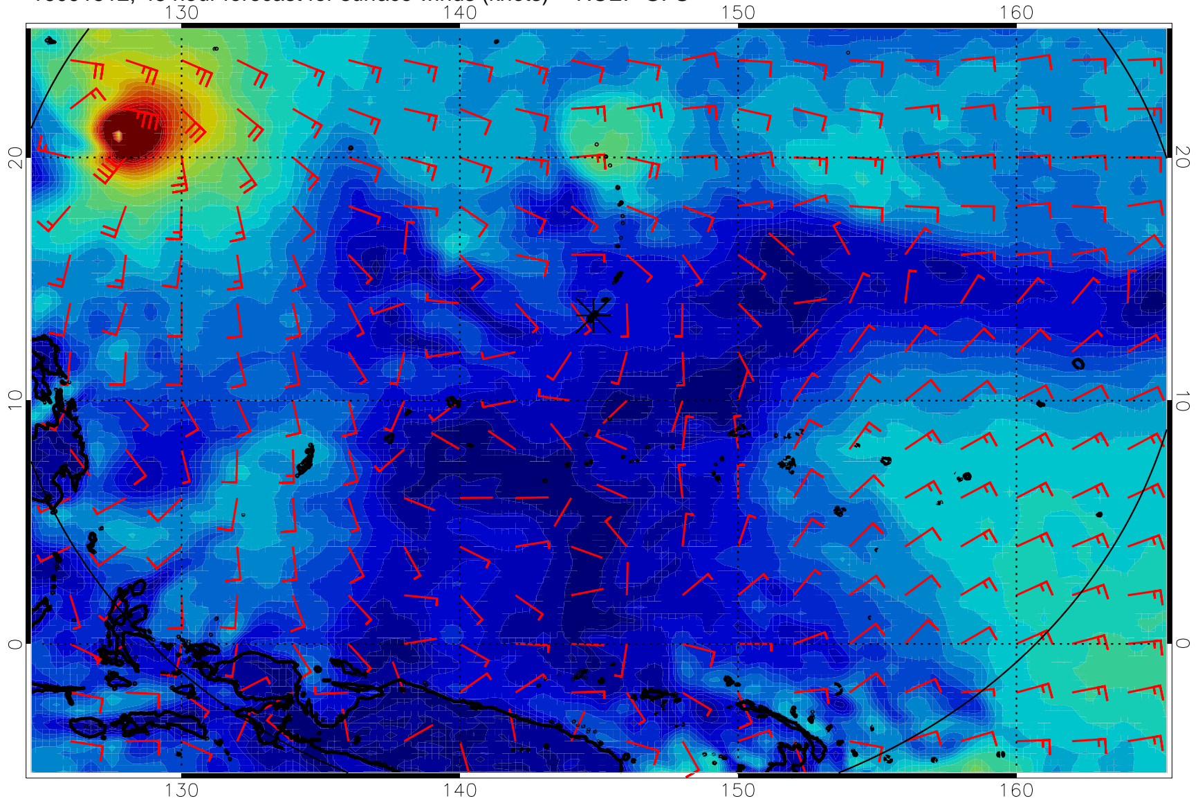
16091512, 48 hour forecast for surface winds (knots) -- NCEP GFS
