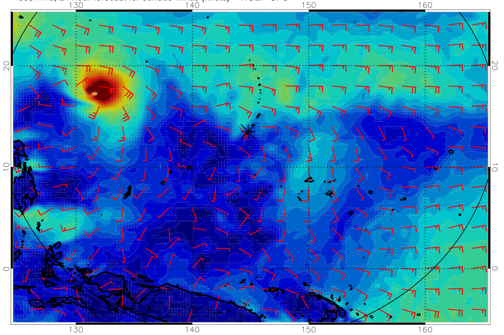
16091412, 24 hour forecast for surface winds (knots) -- NCEP GFS
