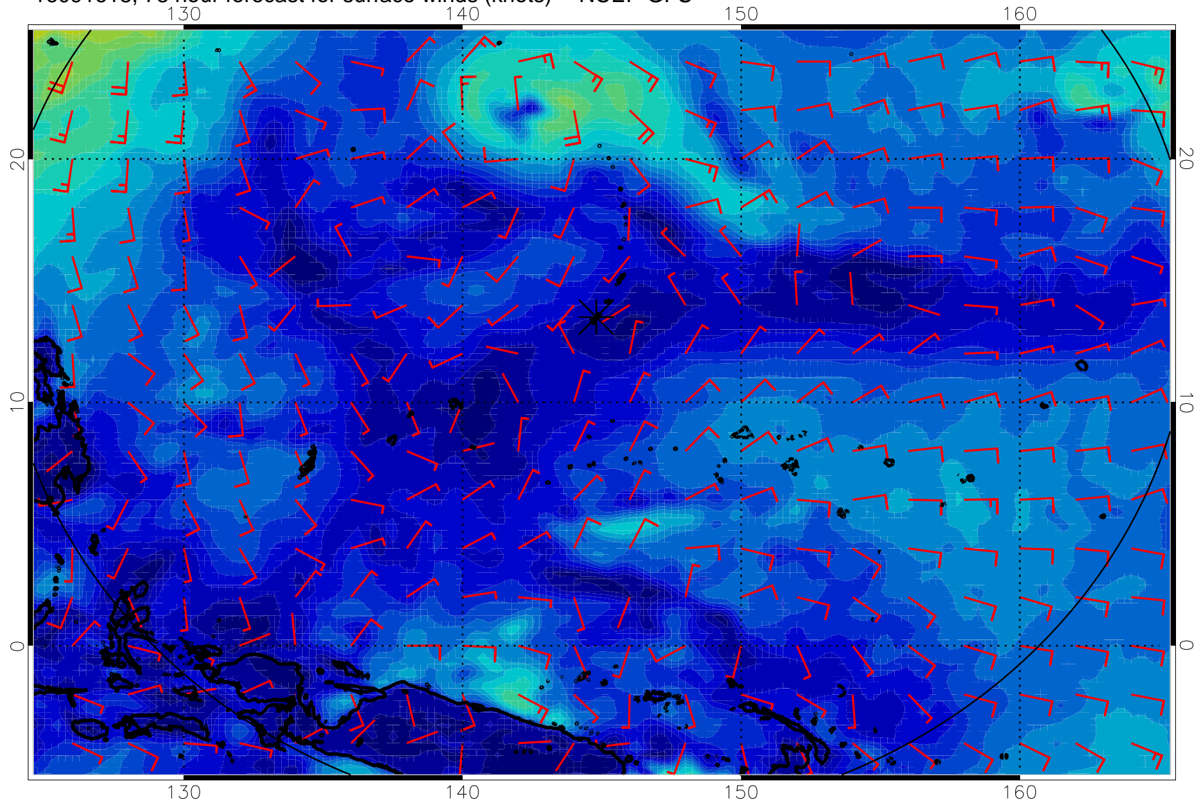
16091618, 78 hour forecast for surface winds (knots) -- NCEP GFS
