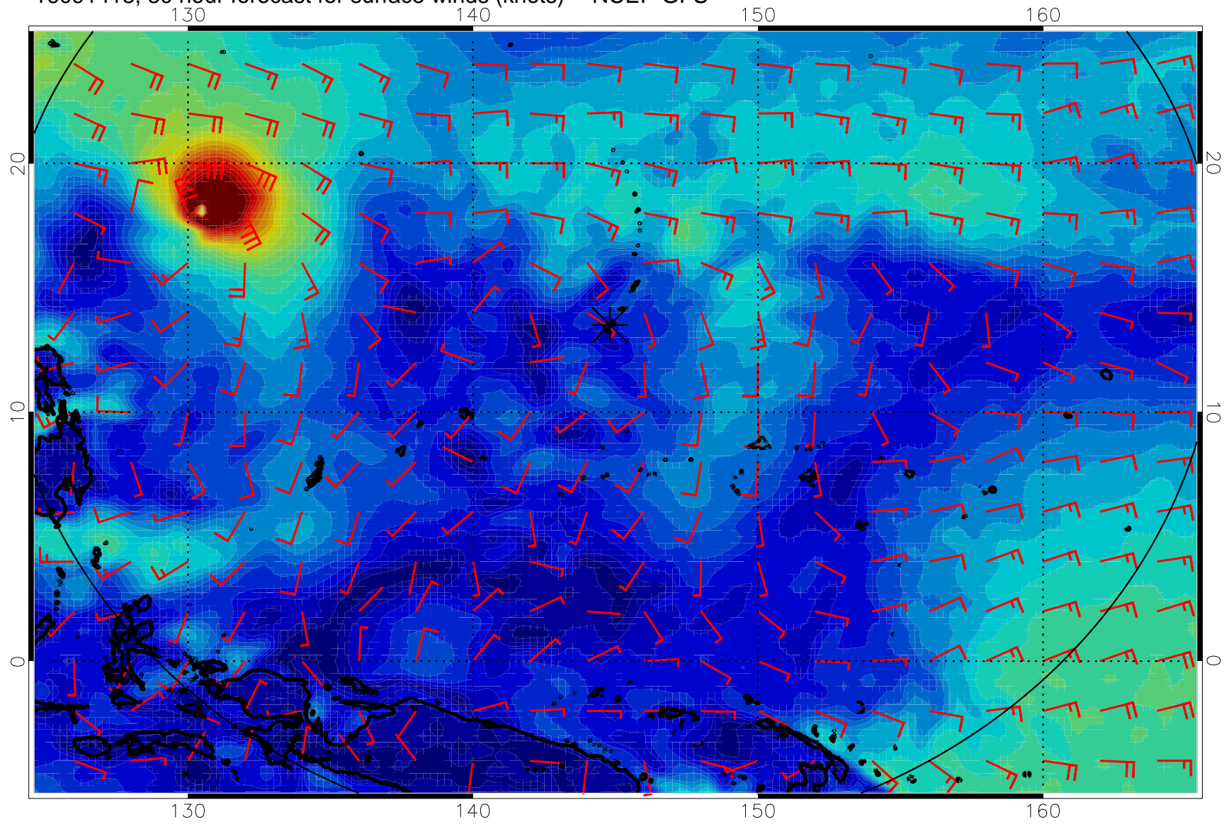
16091418, 30 hour forecast for surface winds (knots) -- NCEP GFS
