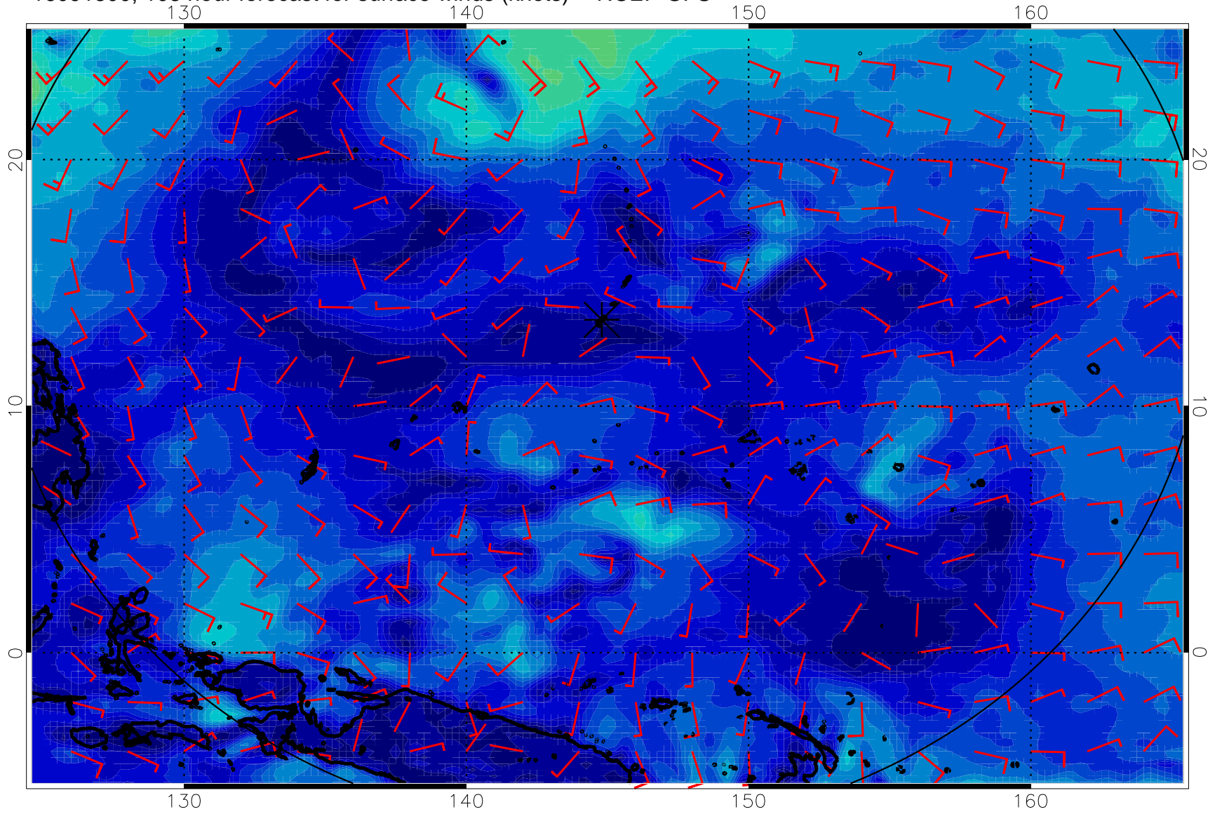
16091800, 108 hour forecast for surface winds (knots) -- NCEP GFS
