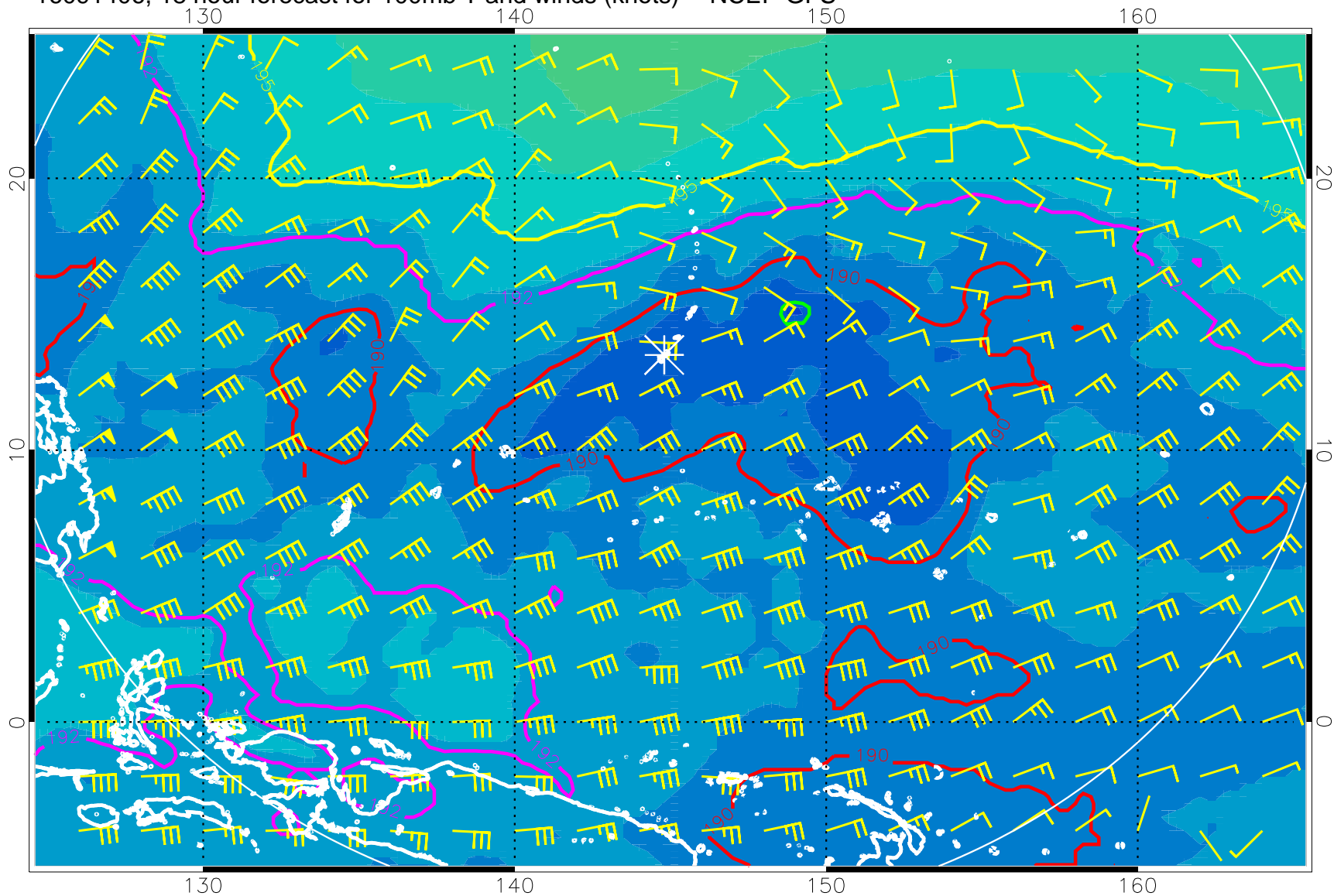
16091406, 18 hour forecast for 100mb T and winds (knots) -- NCEP GFS
