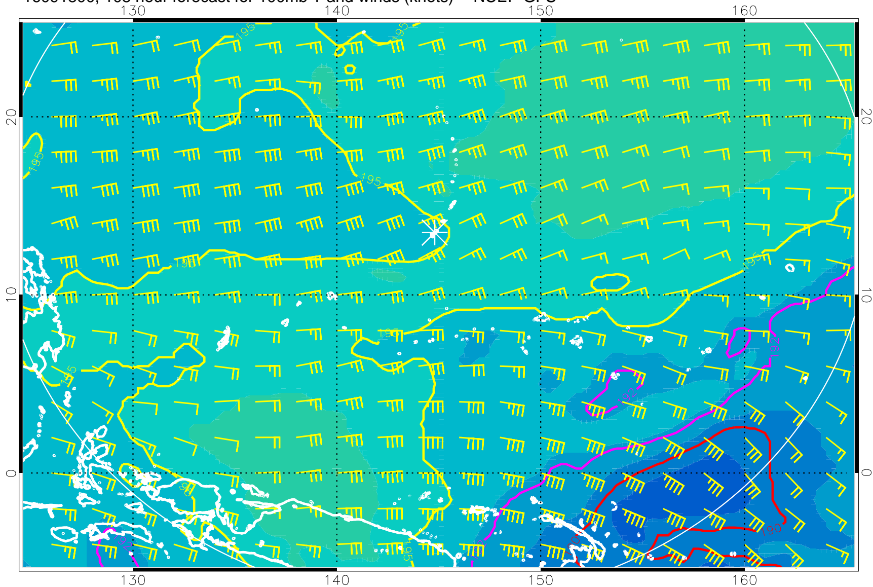
16091800, 108 hour forecast for 100mb T and winds (knots) -- NCEP GFS
