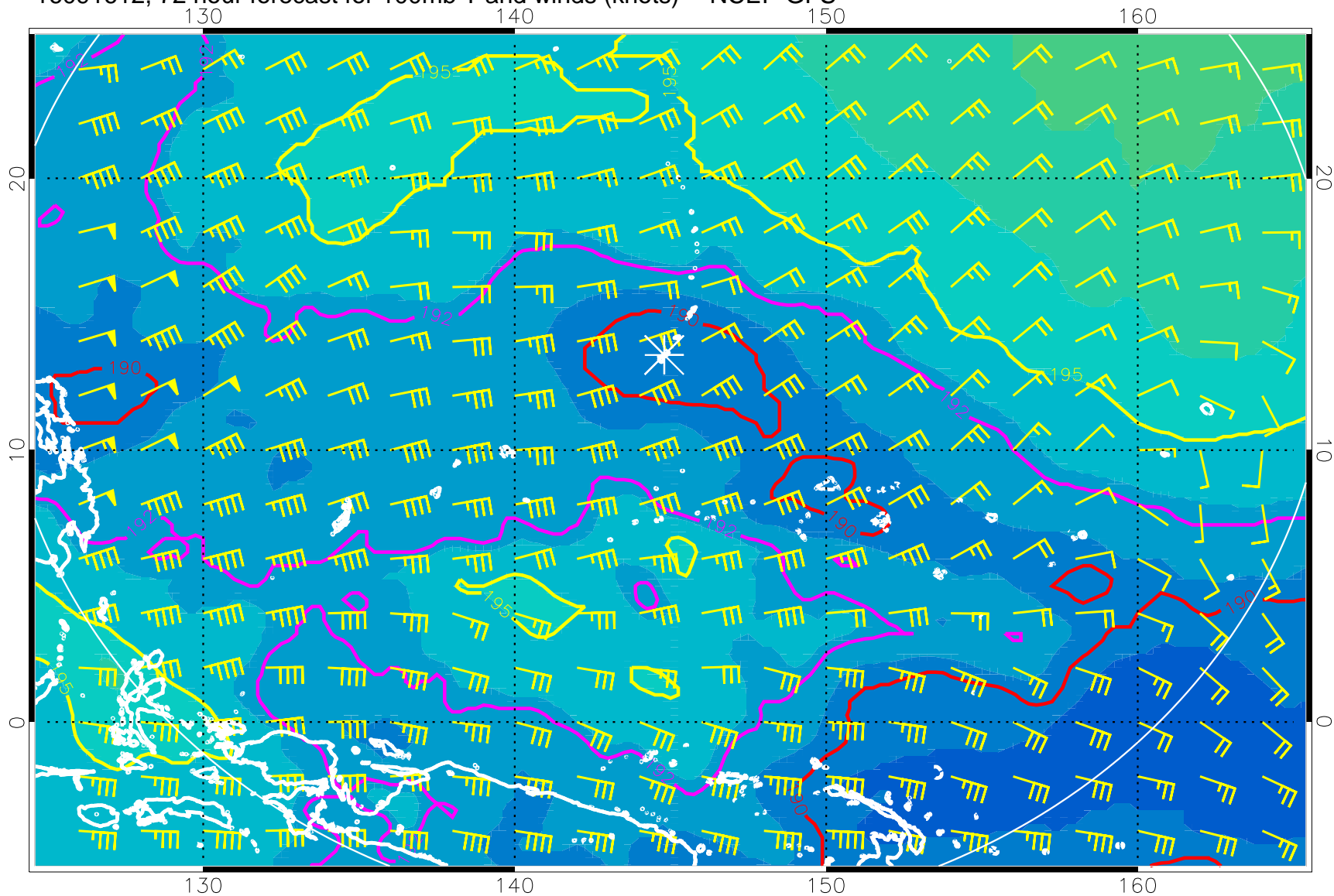
16091612, 72 hour forecast for 100mb T and winds (knots) -- NCEP GFS
