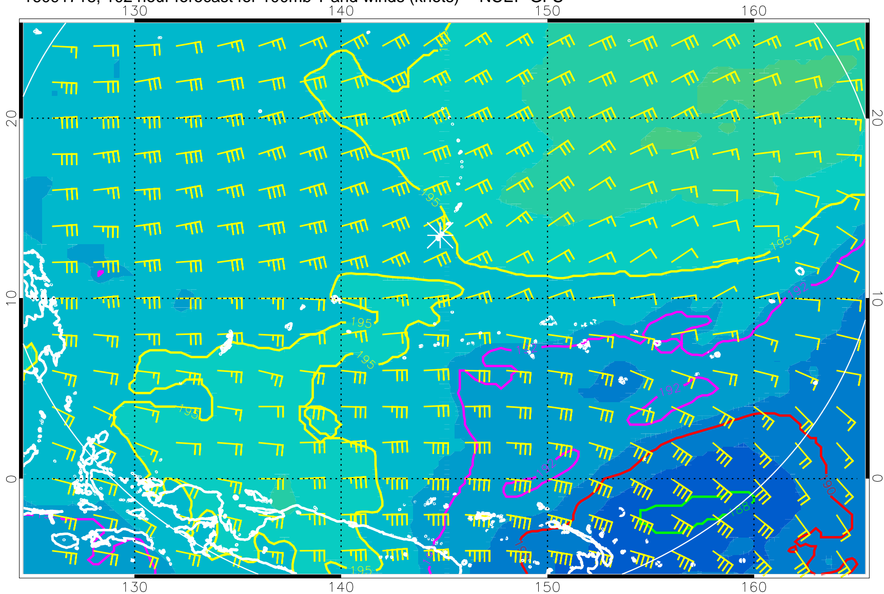
16091718, 102 hour forecast for 100mb T and winds (knots) -- NCEP GFS
