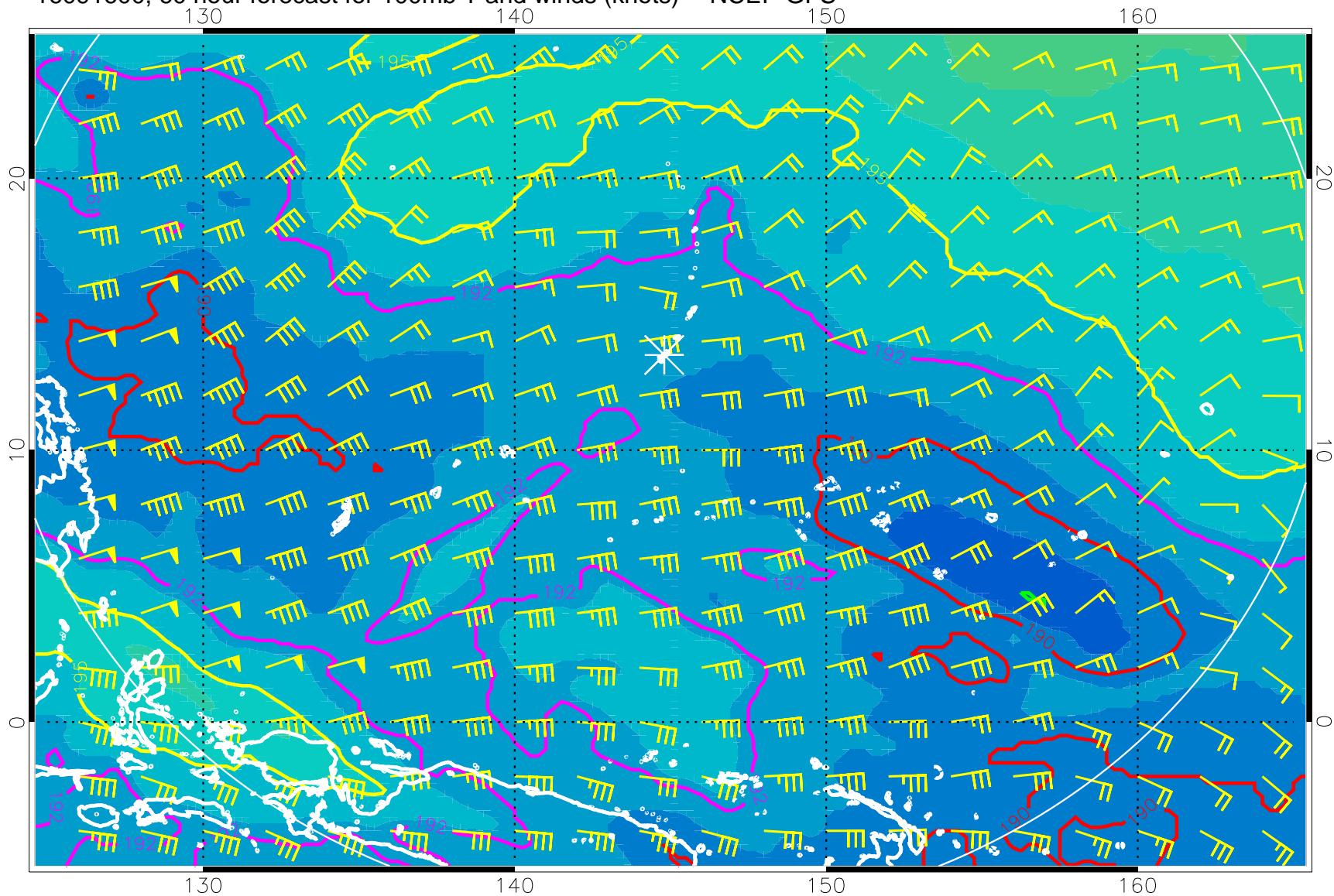
16091600, 60 hour forecast for 100mb T and winds (knots) -- NCEP GFS
