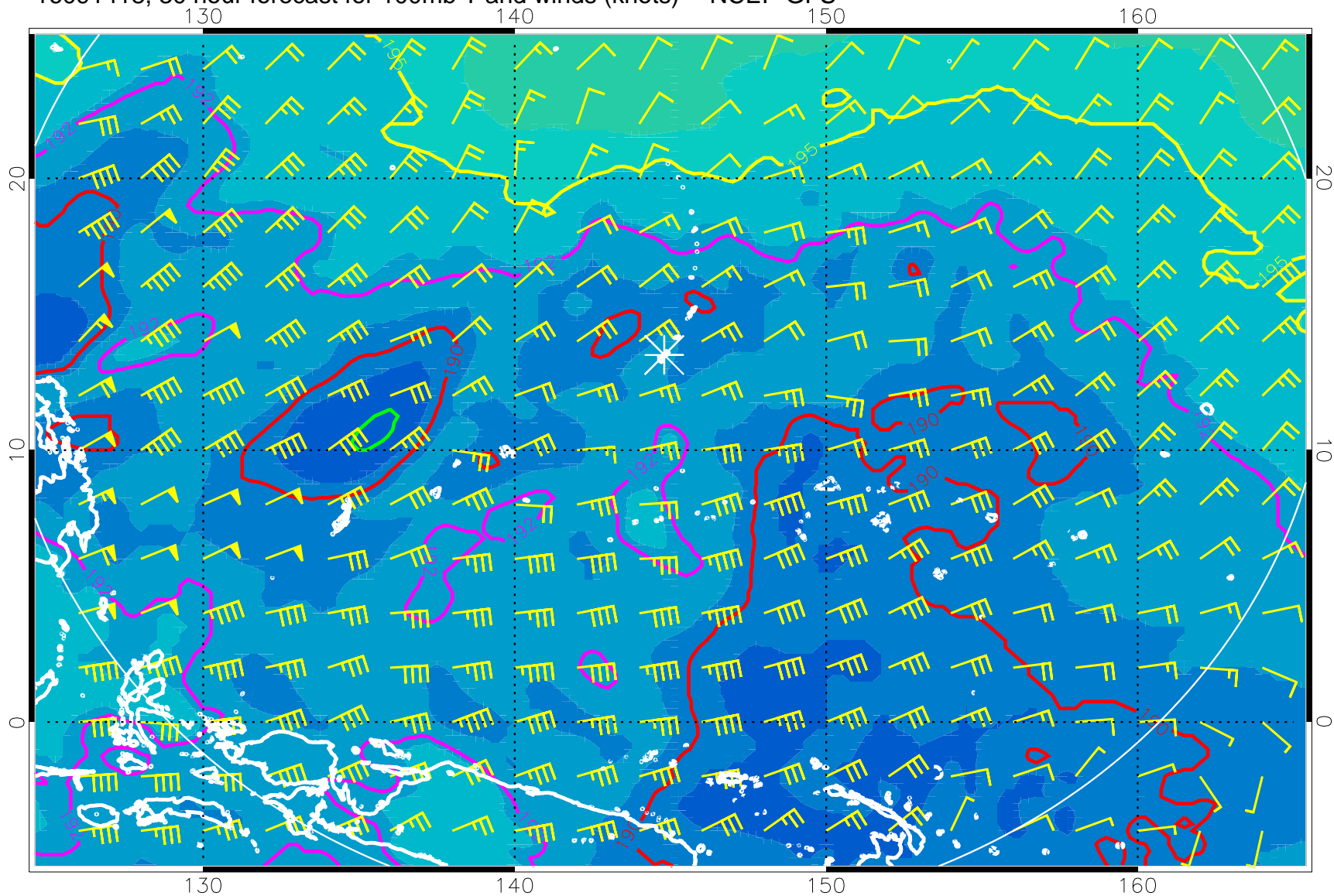
16091418, 30 hour forecast for 100mb T and winds (knots) -- NCEP GFS
