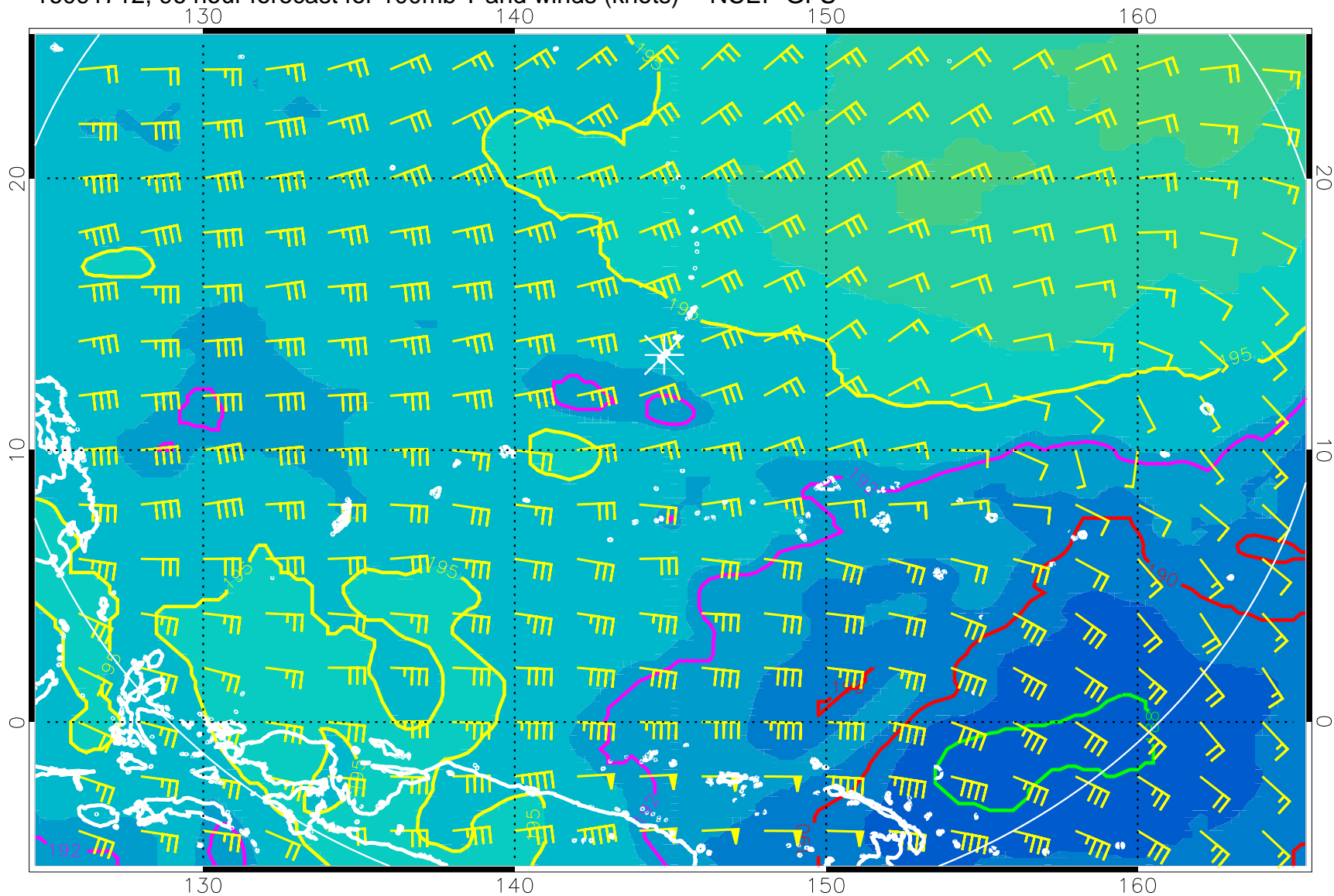
16091712, 96 hour forecast for 100mb T and winds (knots) -- NCEP GFS
