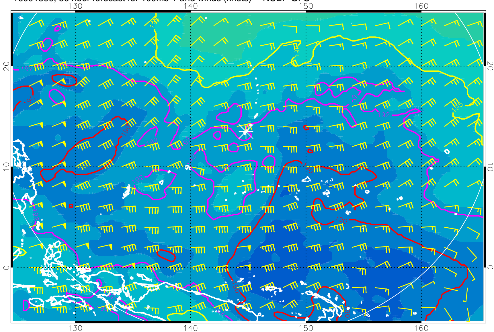
16091500, 36 hour forecast for 100mb T and winds (knots) -- NCEP GFS
