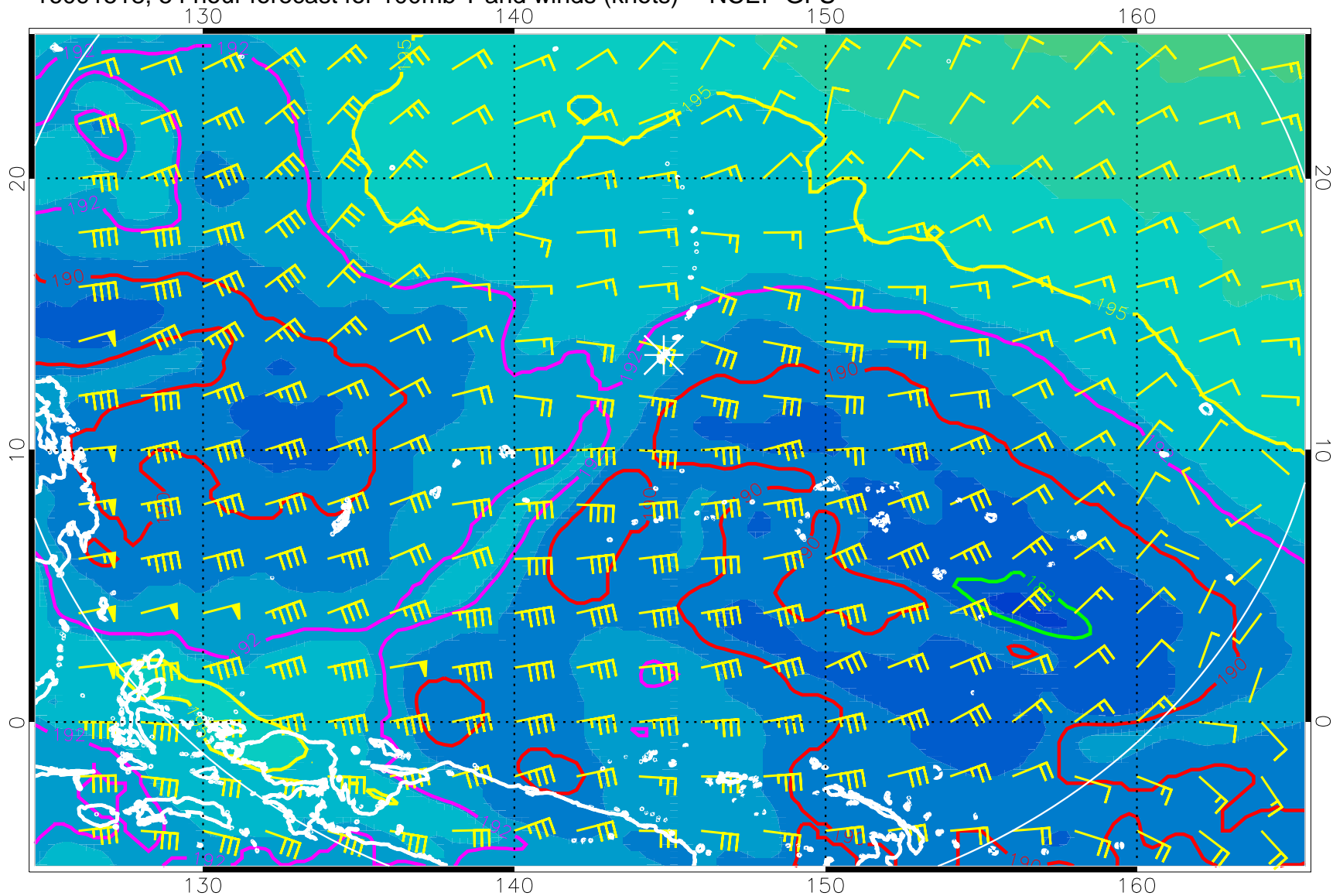
16091518, 54 hour forecast for 100mb T and winds (knots) -- NCEP GFS
