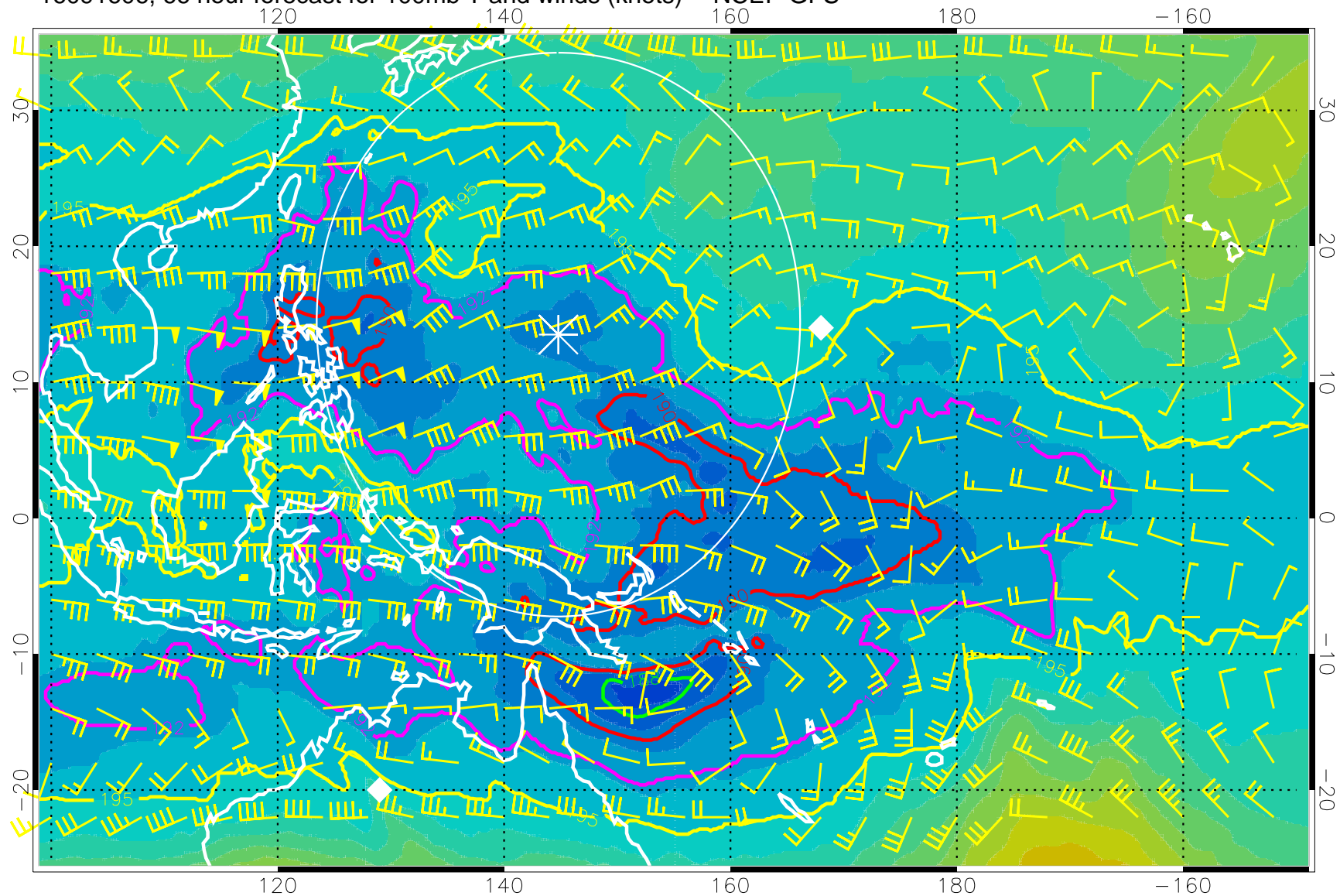
16091606, 66 hour forecast for 100mb T and winds (knots) -- NCEP GFS
