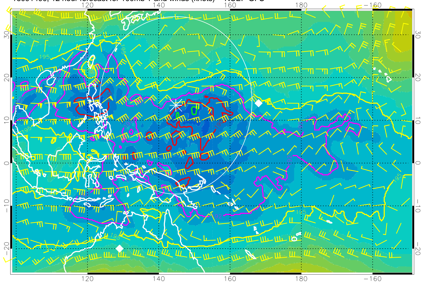
16091400, 12 hour forecast for 100mb T and winds (knots) -- NCEP GFS
