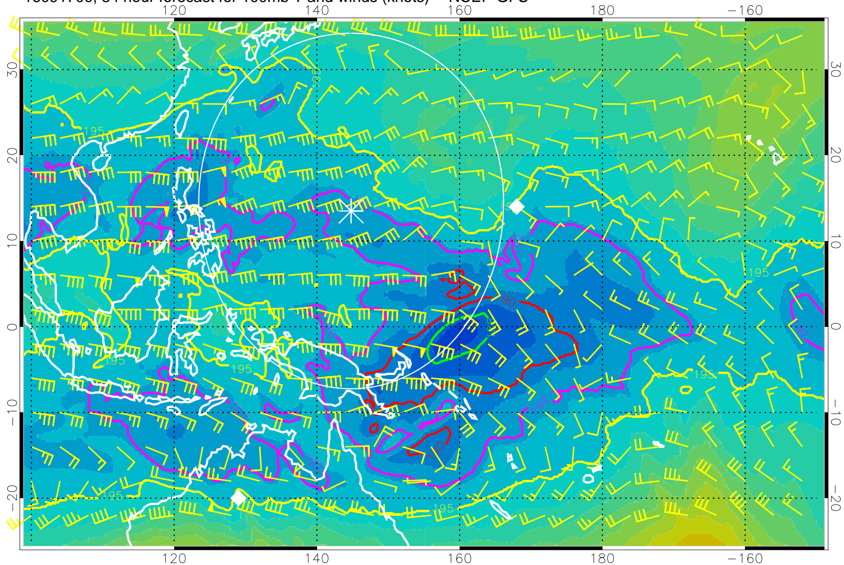
16091700, 84 hour forecast for 100mb T and winds (knots) -- NCEP GFS
