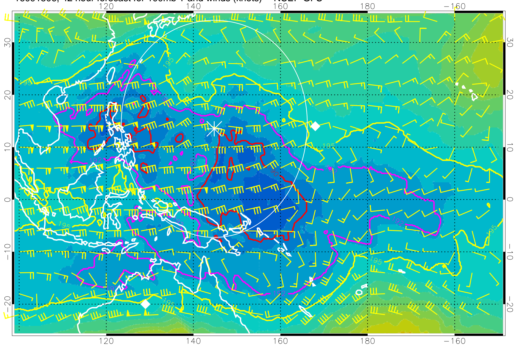
16091506, 42 hour forecast for 100mb T and winds (knots) -- NCEP GFS
