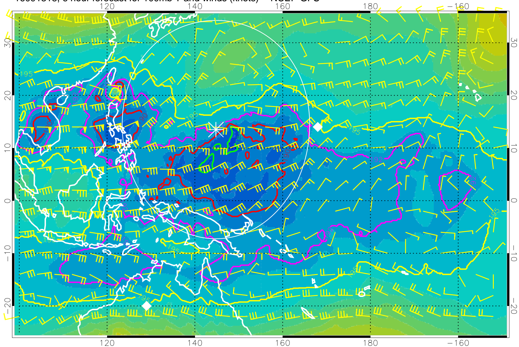
16091318, 6 hour forecast for 100mb T and winds (knots) -- NCEP GFS
