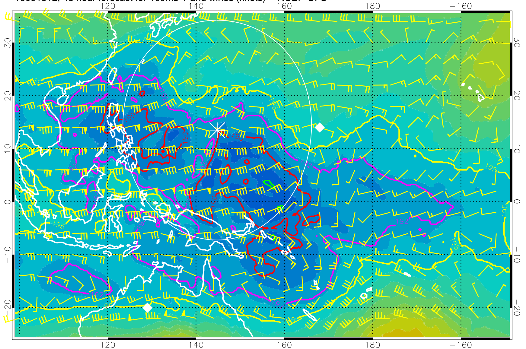
16091512, 48 hour forecast for 100mb T and winds (knots) -- NCEP GFS
