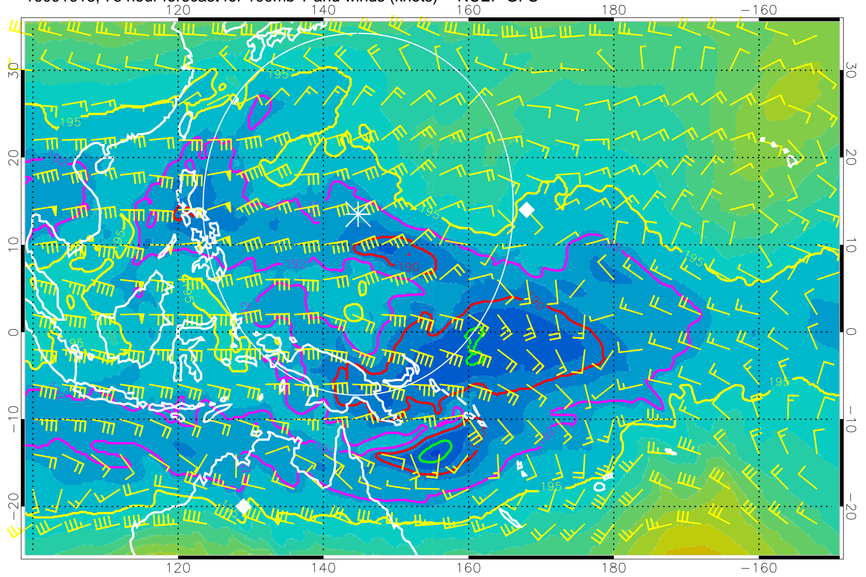
16091618, 78 hour forecast for 100mb T and winds (knots) -- NCEP GFS
