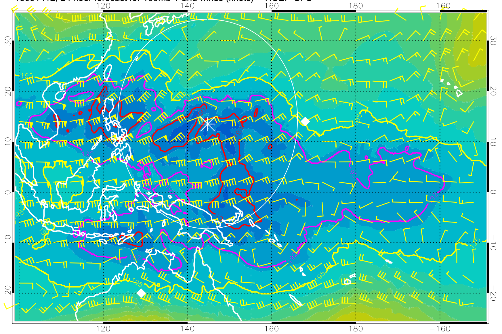
16091412, 24 hour forecast for 100mb T and winds (knots) -- NCEP GFS
