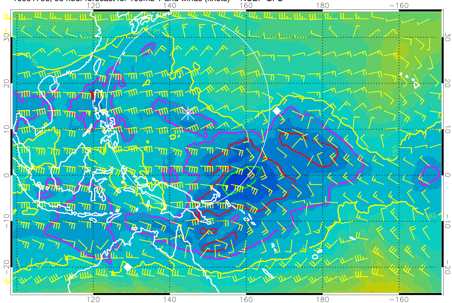
16091706, 90 hour forecast for 100mb T and winds (knots) -- NCEP GFS
