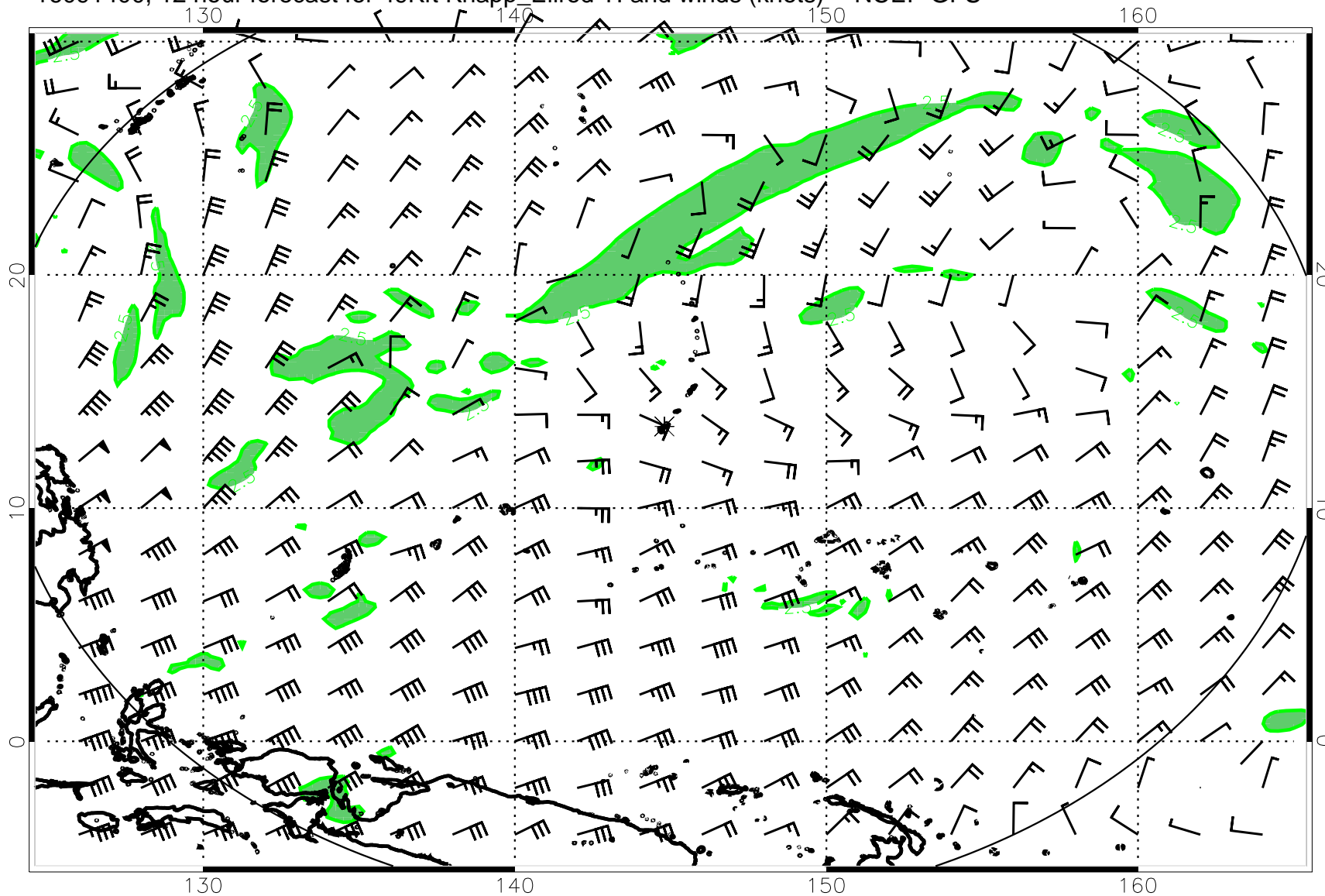
16091400, 12 hour forecast for 49Kft Knapp_Ellrod TI and winds (knots) -- NCEP GFS
