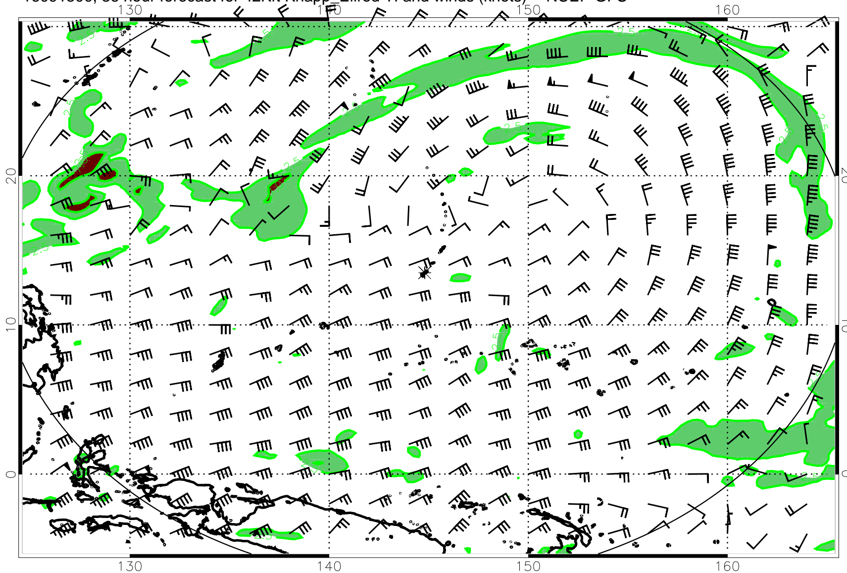
16091500, 36 hour forecast for 42Kft Knapp_Ellrod TI and winds (knots) -- NCEP GFS
