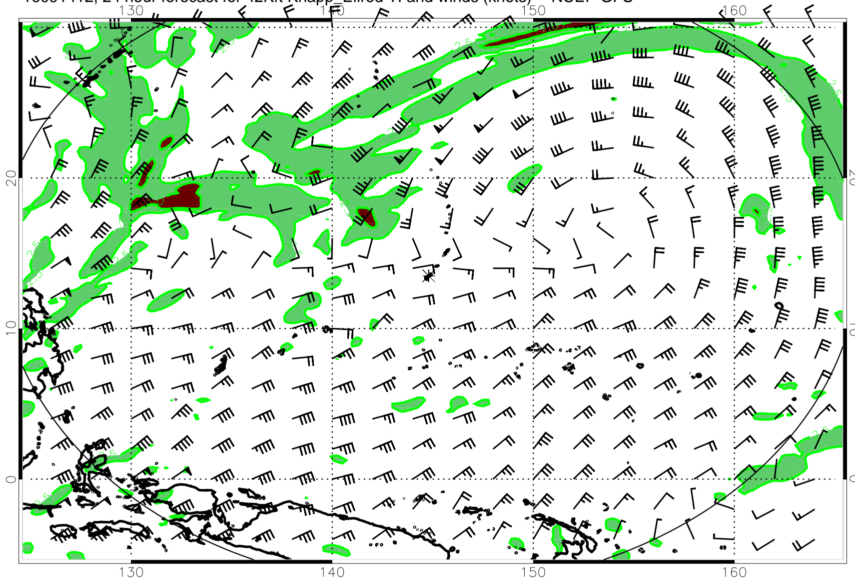
16091412, 24 hour forecast for 42Kft Knapp_Ellrod TI and winds (knots) -- NCEP GFS
