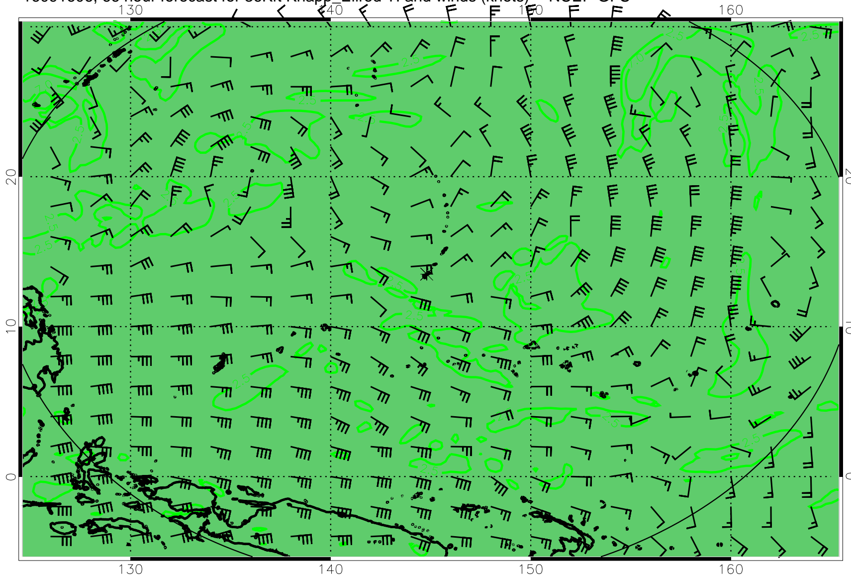
16091606, 66 hour forecast for 36Kft Knapp_Ellrod TI and winds (knots) -- NCEP GFS
