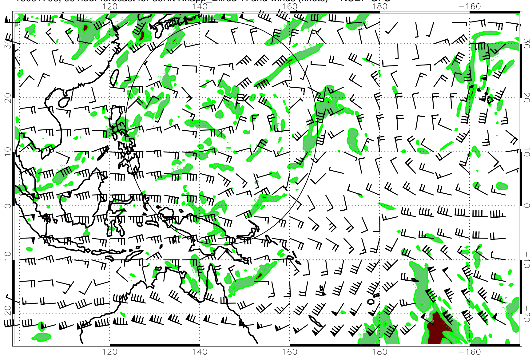
16091706, 90 hour forecast for 36Kft Knapp_Ellrod TI and winds (knots) -- NCEP GFS
