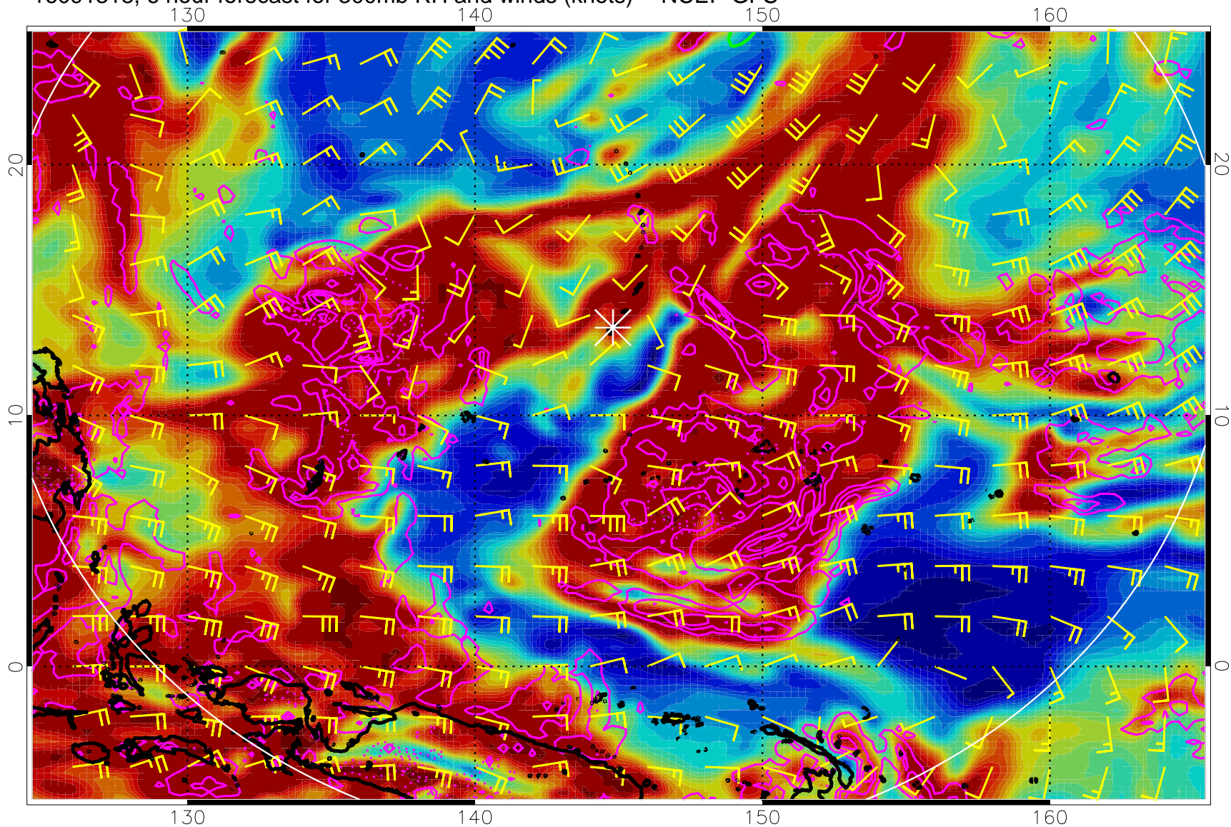
16091318, 6 hour forecast for 300mb RH and winds (knots) -- NCEP GFS
