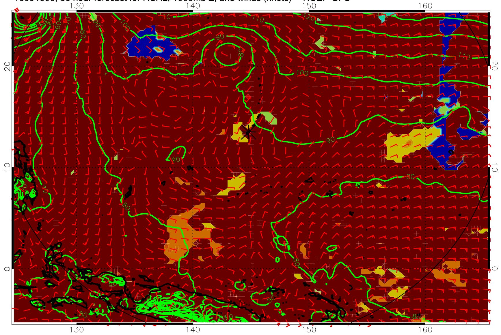
16091606, 66 hour forecast for HCAL, 1000mb Z, and winds (knots) -- NCEP GFS
