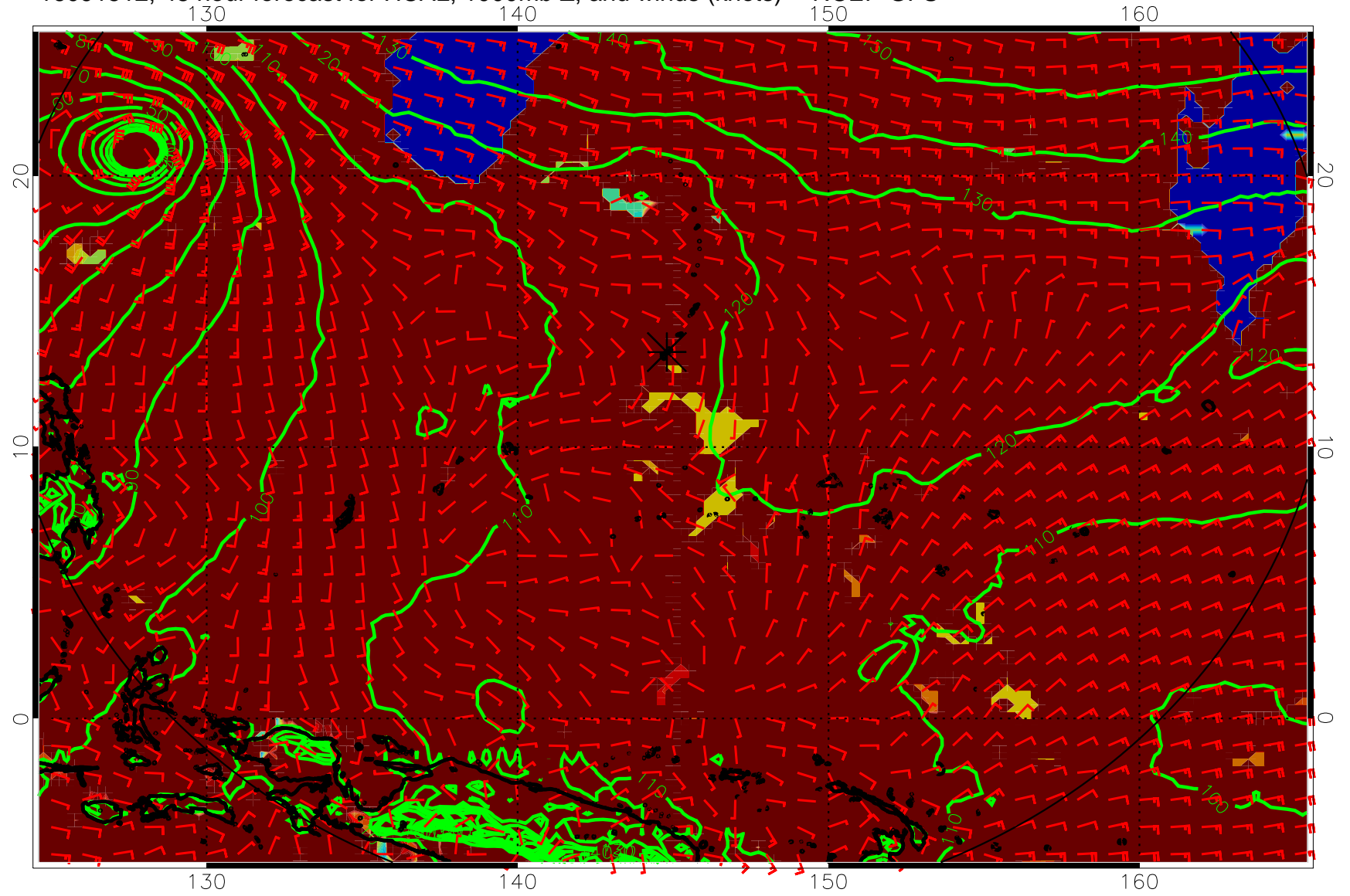
16091512, 48 hour forecast for HCAL, 1000mb Z, and winds (knots) -- NCEP GFS
