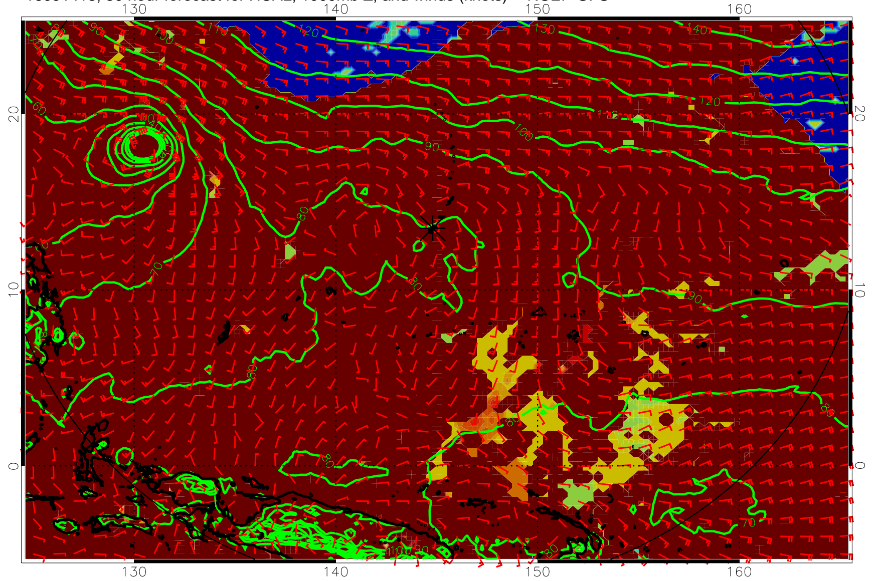
16091418, 30 hour forecast for HCAL, 1000mb Z, and winds (knots) -- NCEP GFS
