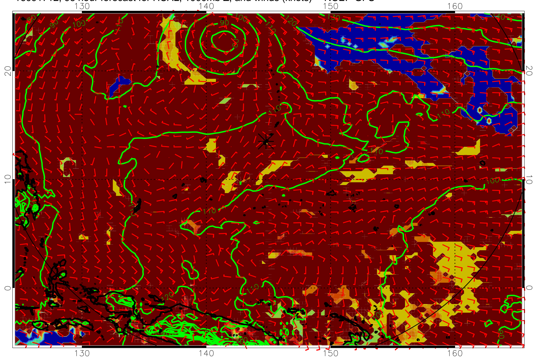
16091712, 96 hour forecast for HCAL, 1000mb Z, and winds (knots) -- NCEP GFS
