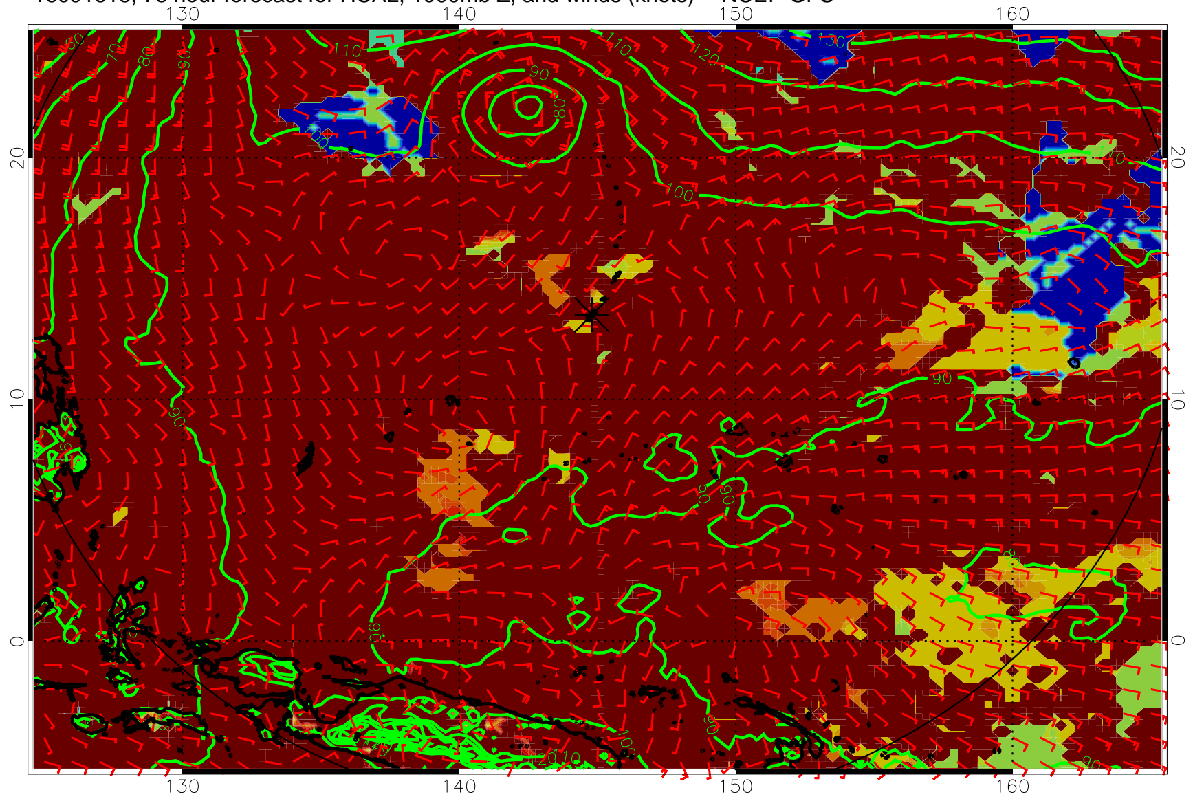
16091618, 78 hour forecast for HCAL, 1000mb Z, and winds (knots) -- NCEP GFS
