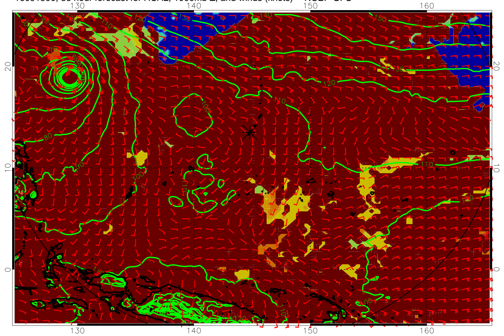
16091500, 36 hour forecast for HCAL, 1000mb Z, and winds (knots) -- NCEP GFS
