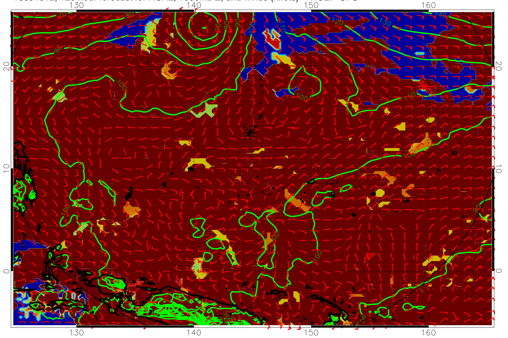
16091812, 120 hour forecast for HCAL, 1000mb Z, and winds (knots) -- NCEP GFS
