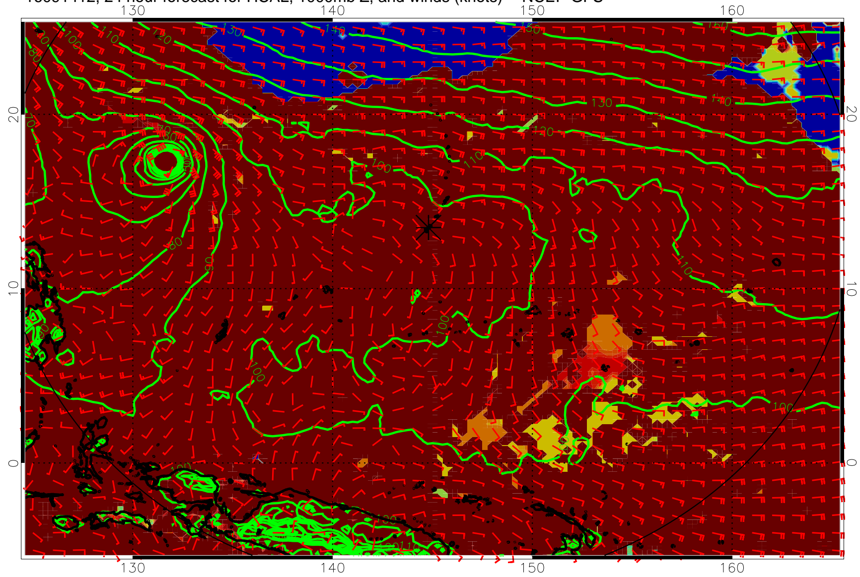
16091412, 24 hour forecast for HCAL, 1000mb Z, and winds (knots) -- NCEP GFS
