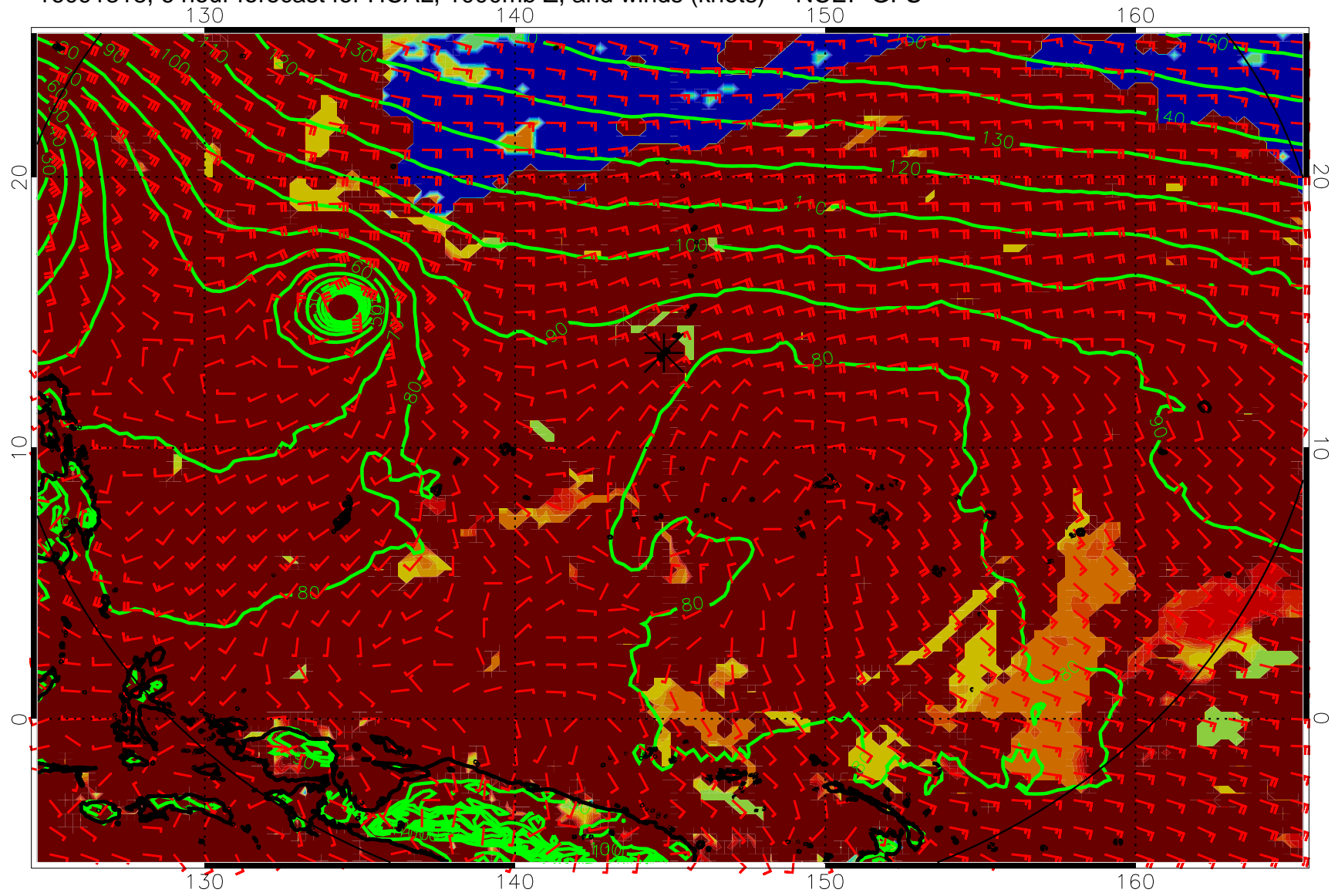
16091318, 6 hour forecast for HCAL, 1000mb Z, and winds (knots) -- NCEP GFS
