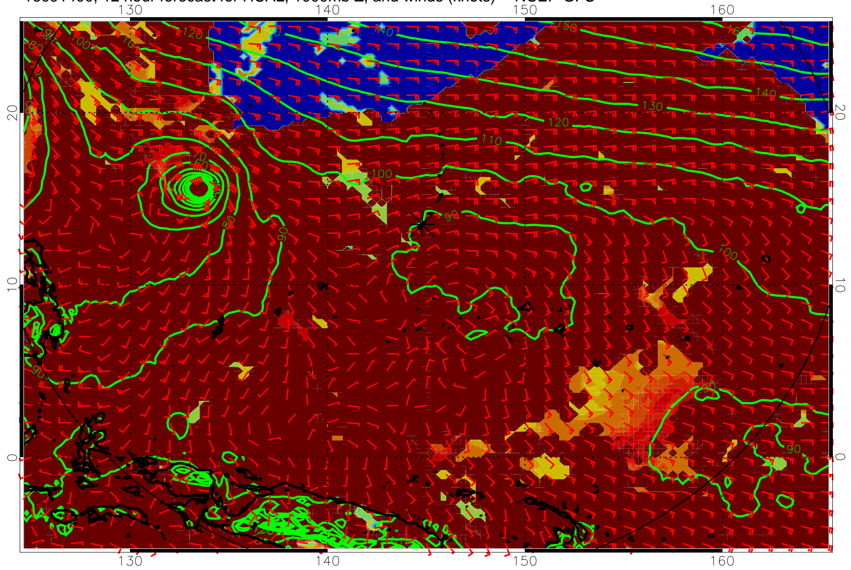
16091400, 12 hour forecast for HCAL, 1000mb Z, and winds (knots) -- NCEP GFS
