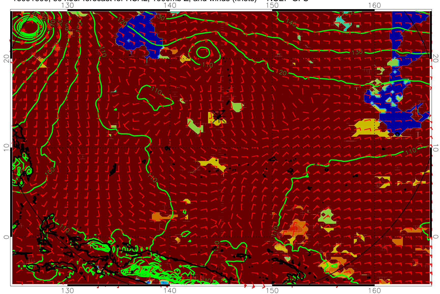
16091600, 60 hour forecast for HCAL, 1000mb Z, and winds (knots) -- NCEP GFS
