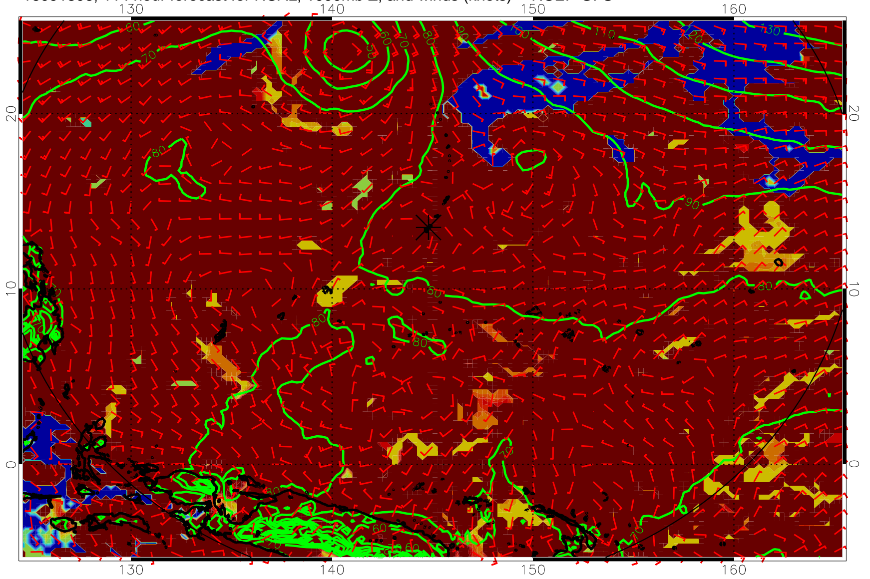
16091806, 114 hour forecast for HCAL, 1000mb Z, and winds (knots) -- NCEP GFS
