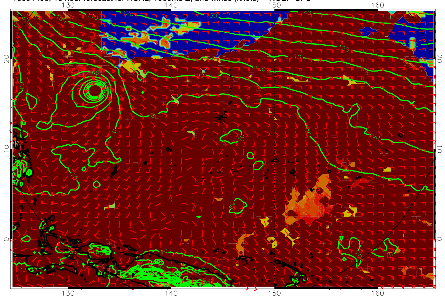
16091406, 18 hour forecast for HCAL, 1000mb Z, and winds (knots) -- NCEP GFS
