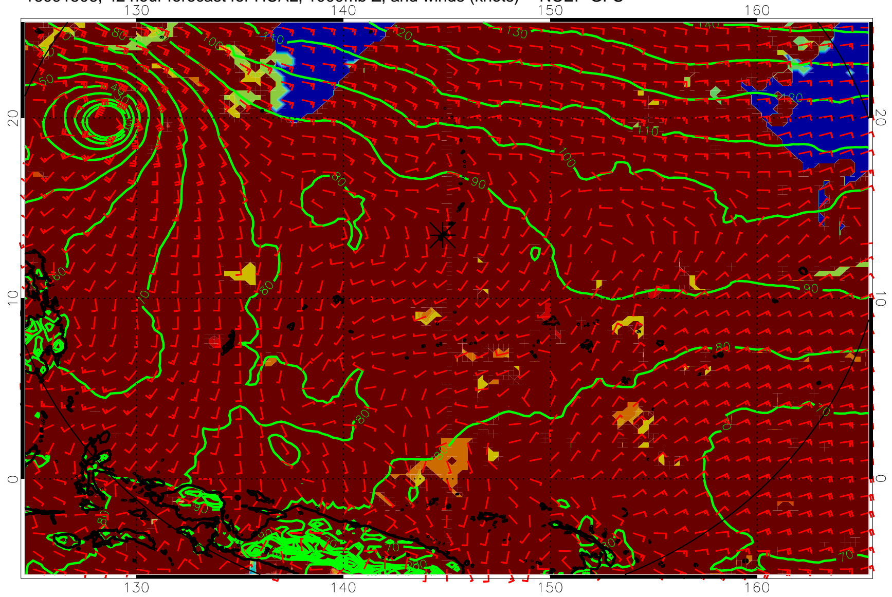
16091506, 42 hour forecast for HCAL, 1000mb Z, and winds (knots) -- NCEP GFS
