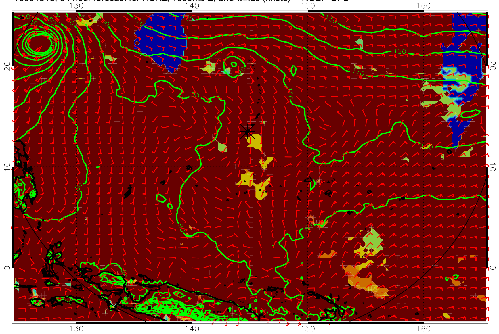
16091518, 54 hour forecast for HCAL, 1000mb Z, and winds (knots) -- NCEP GFS
