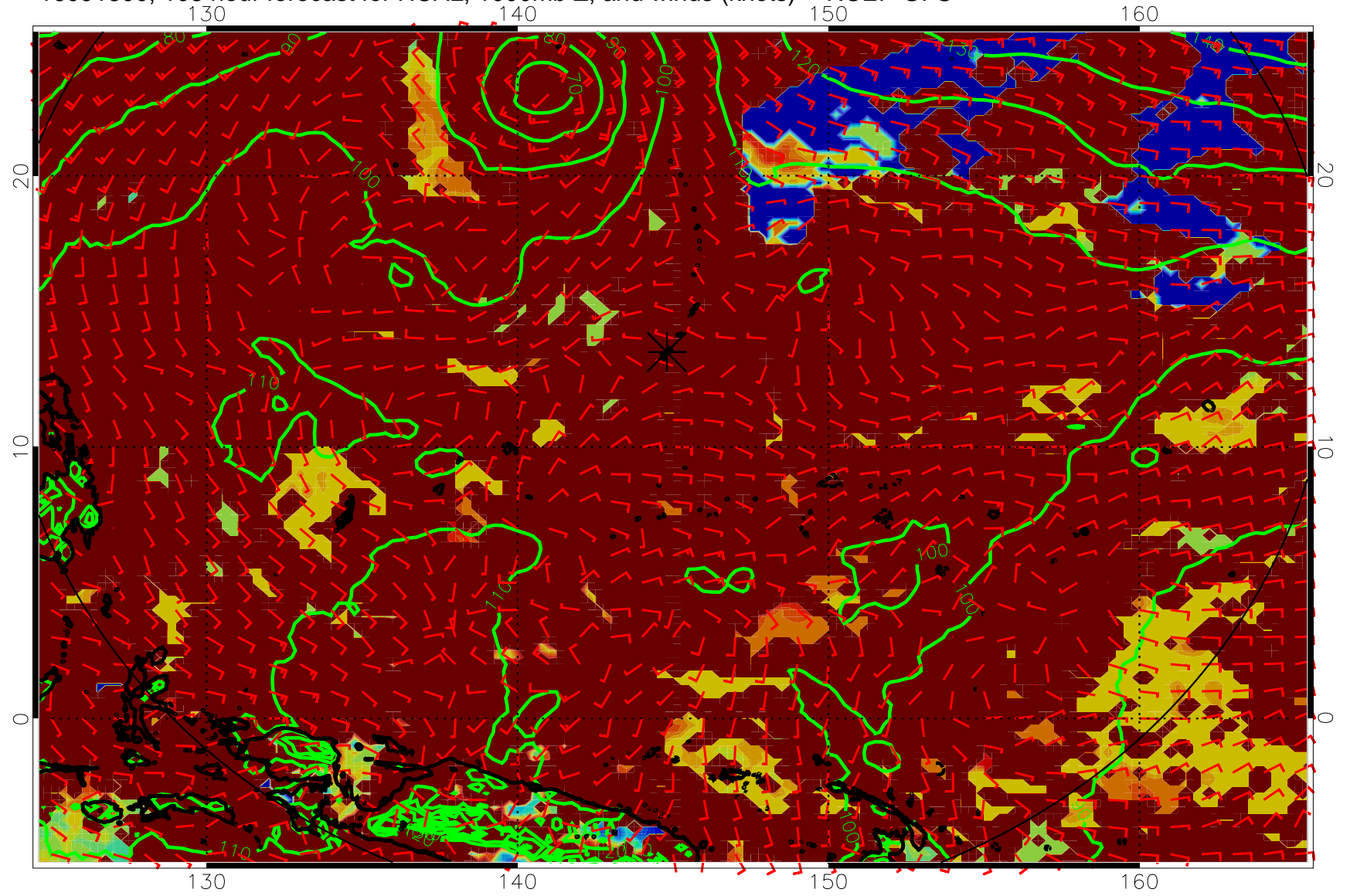
16091800, 108 hour forecast for HCAL, 1000mb Z, and winds (knots) -- NCEP GFS
