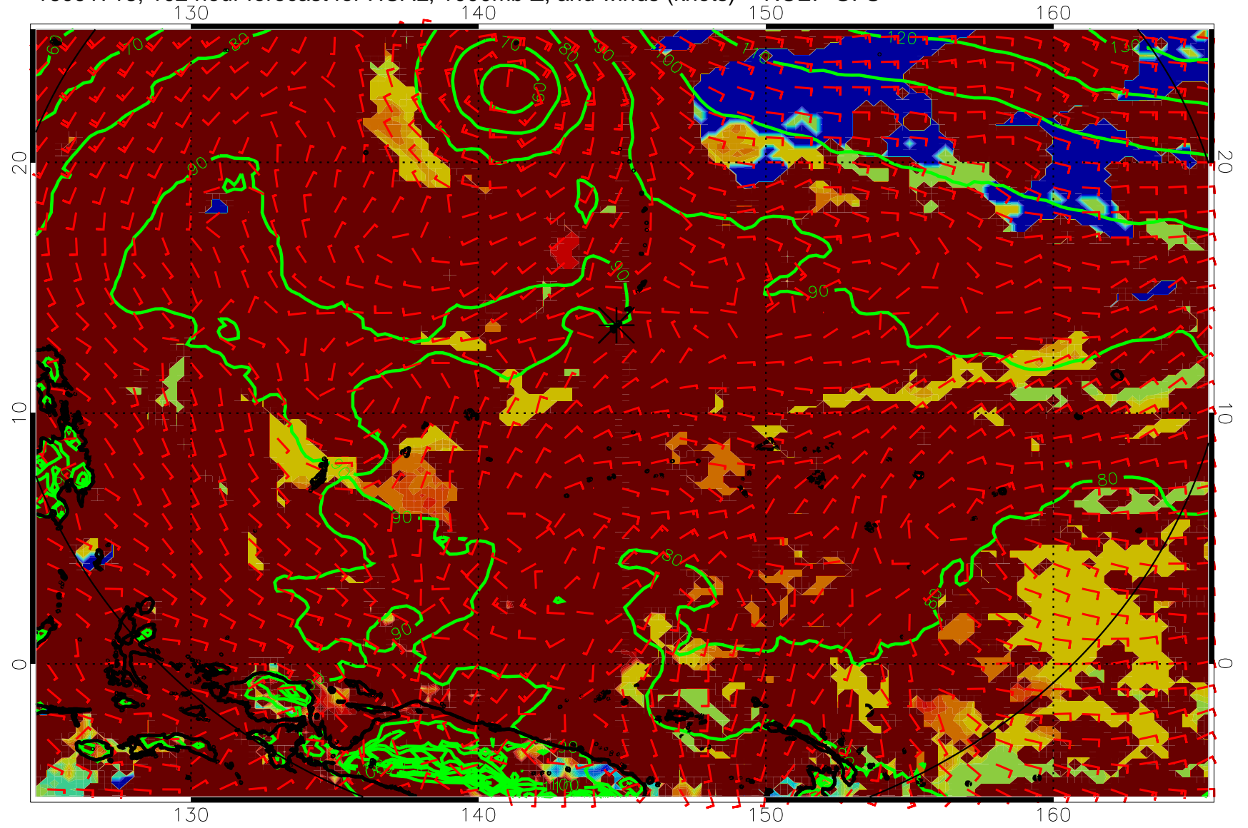
16091718, 102 hour forecast for HCAL, 1000mb Z, and winds (knots) -- NCEP GFS
