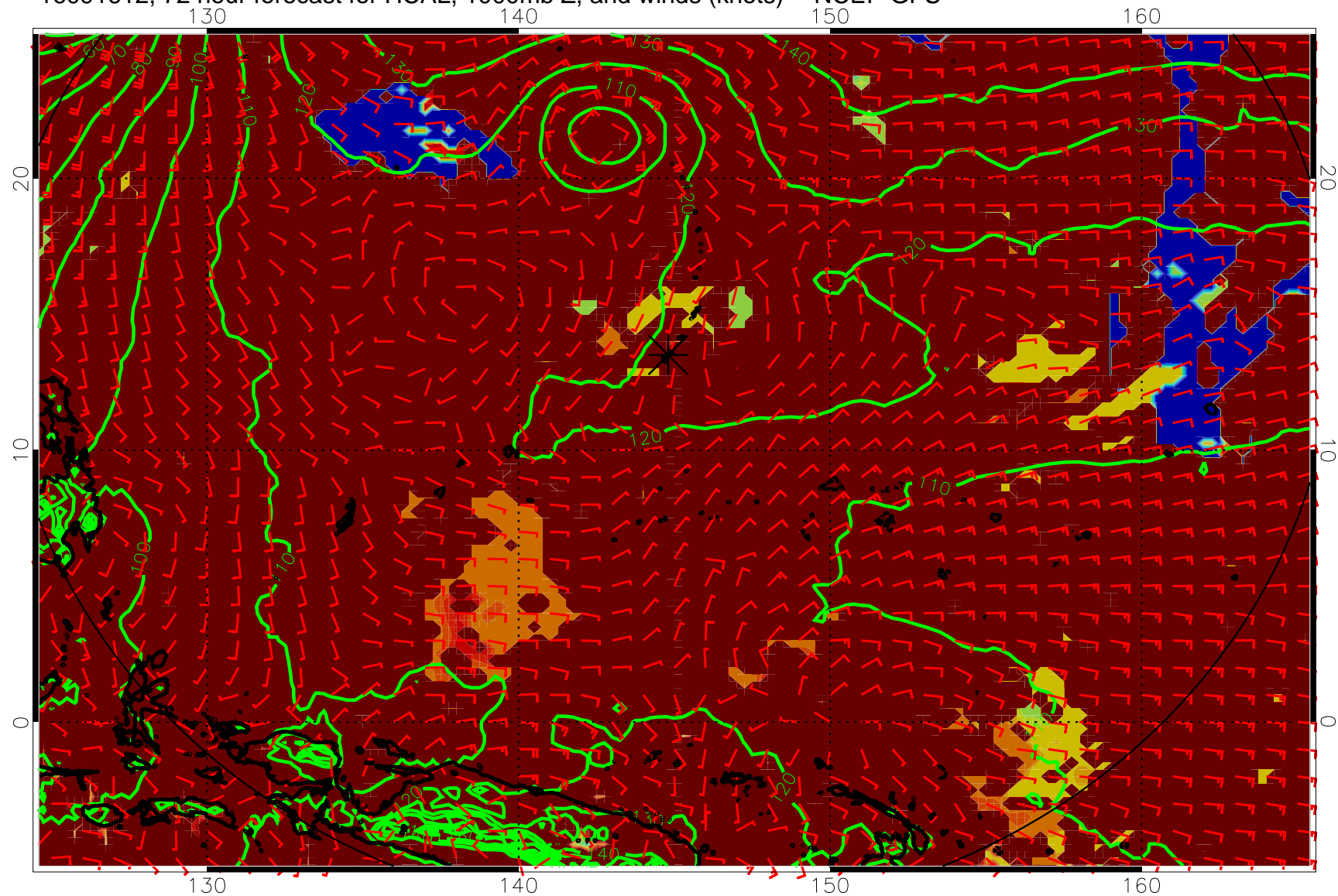
16091612, 72 hour forecast for HCAL, 1000mb Z, and winds (knots) -- NCEP GFS
