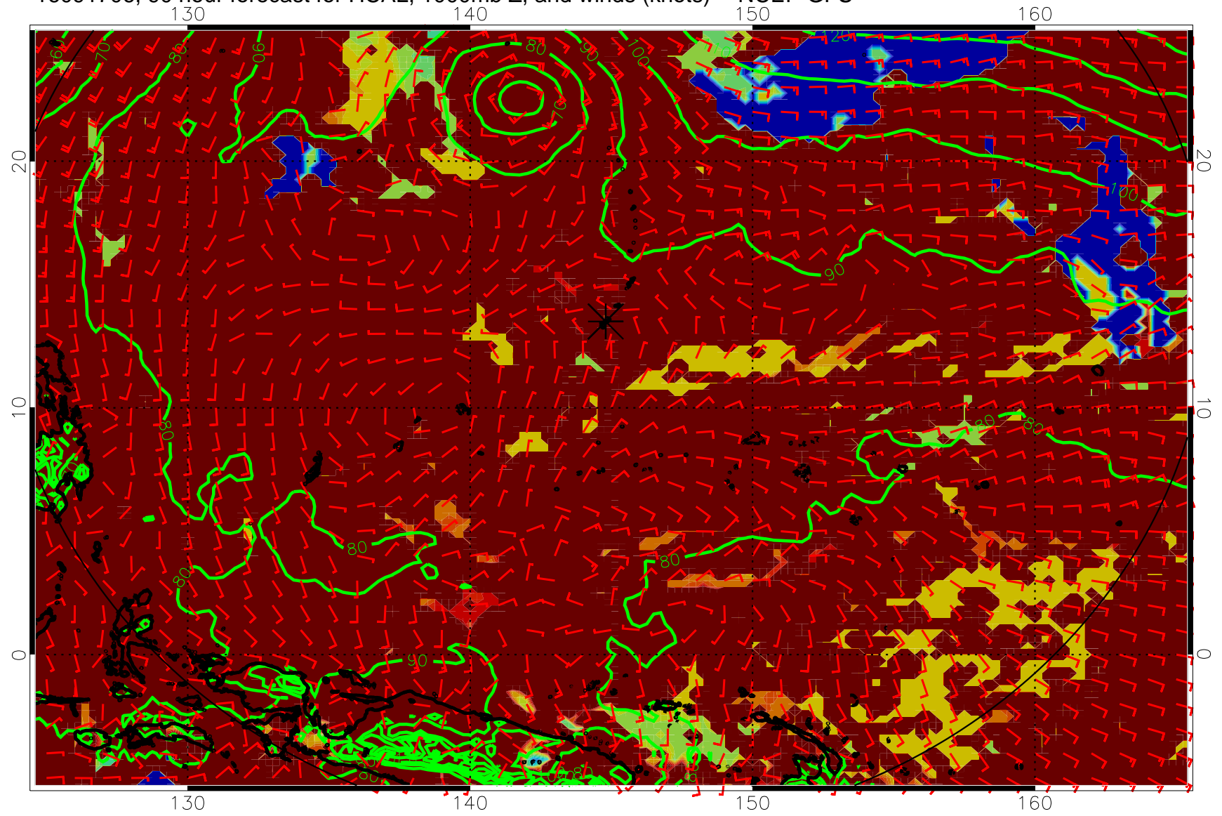
16091706, 90 hour forecast for HCAL, 1000mb Z, and winds (knots) -- NCEP GFS
