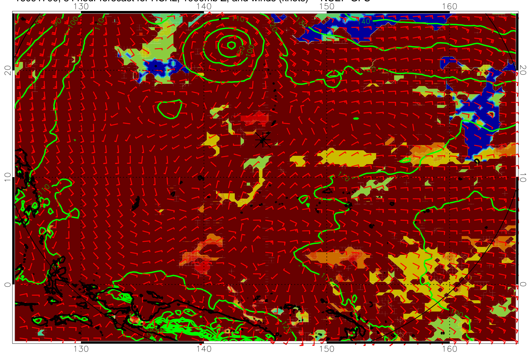
16091700, 84 hour forecast for HCAL, 1000mb Z, and winds (knots) -- NCEP GFS
