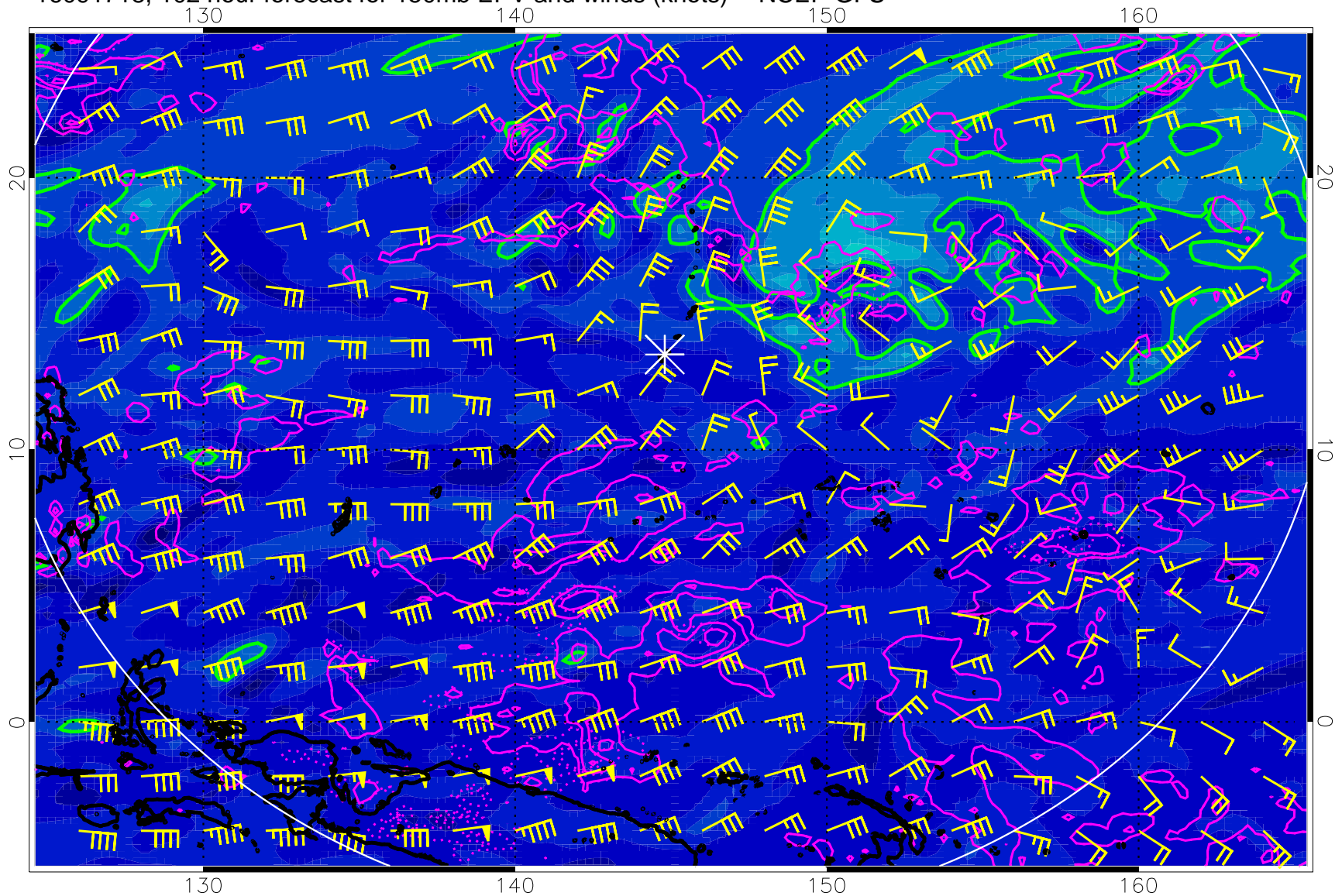
16091718, 102 hour forecast for 150mb EPV and winds (knots) -- NCEP GFS
