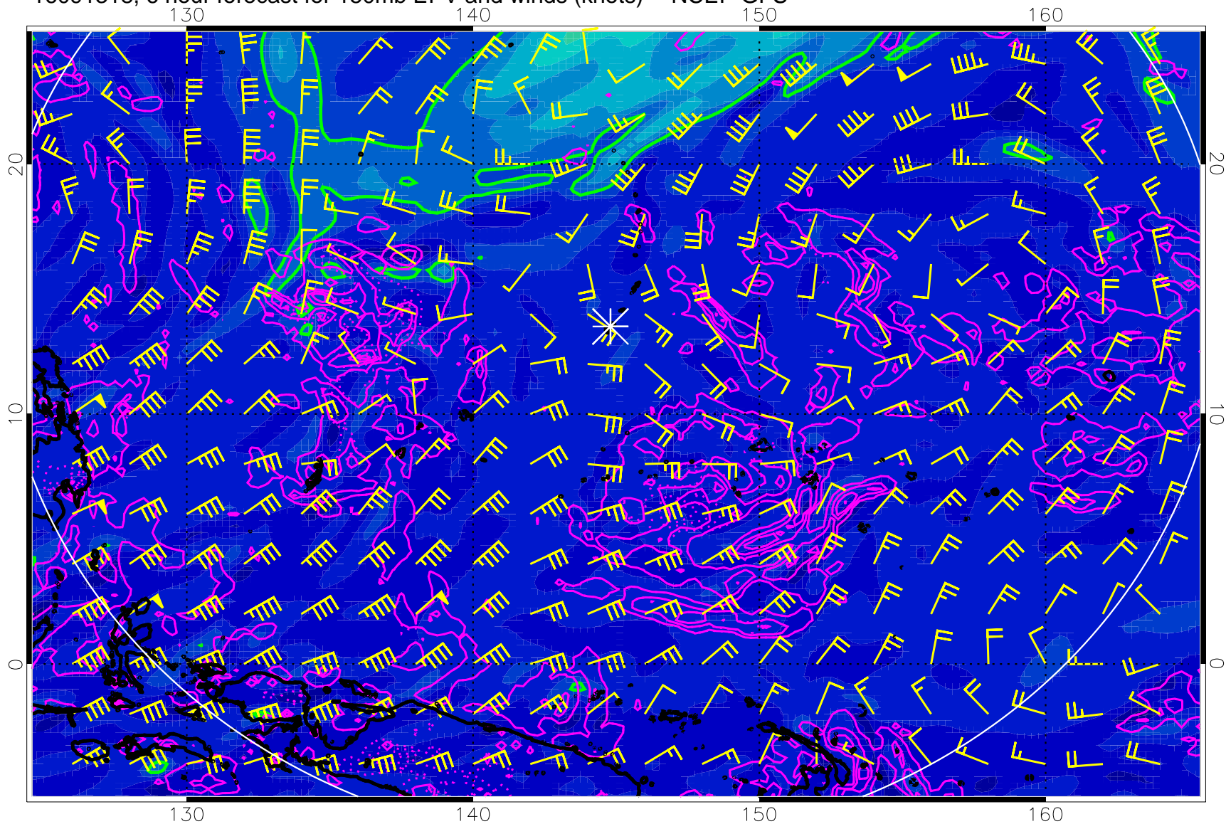
16091318, 6 hour forecast for 150mb EPV and winds (knots) -- NCEP GFS
