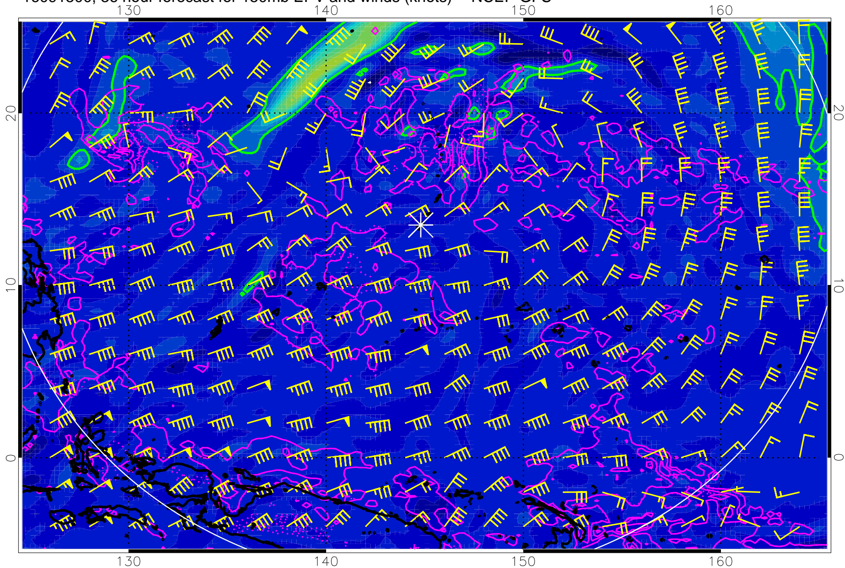
16091500, 36 hour forecast for 150mb EPV and winds (knots) -- NCEP GFS
