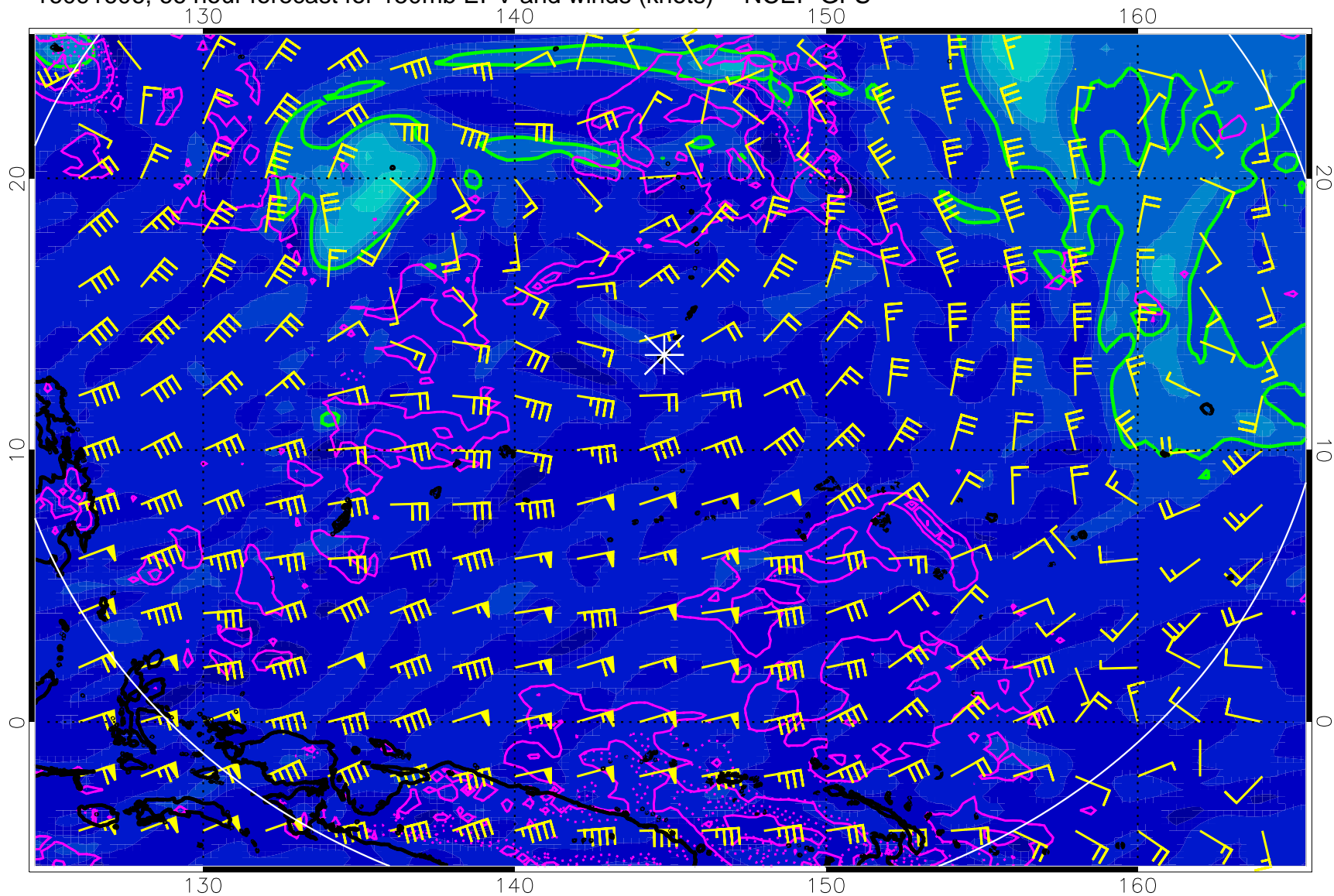
16091606, 66 hour forecast for 150mb EPV and winds (knots) -- NCEP GFS
