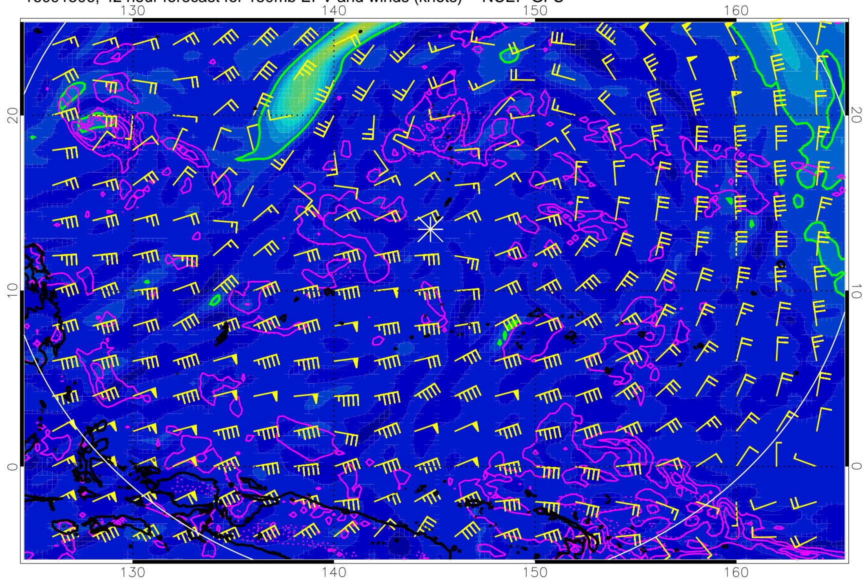
16091506, 42 hour forecast for 150mb EPV and winds (knots) -- NCEP GFS
