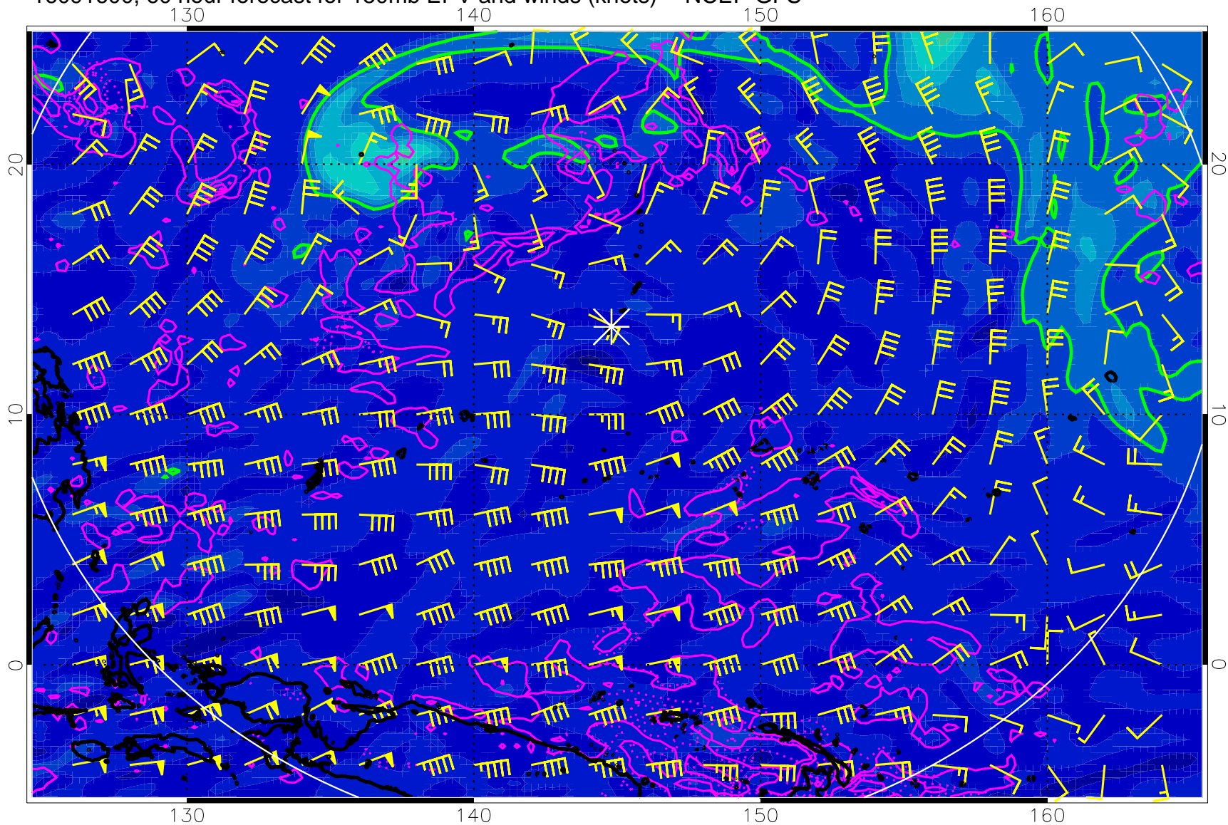
16091600, 60 hour forecast for 150mb EPV and winds (knots) -- NCEP GFS
