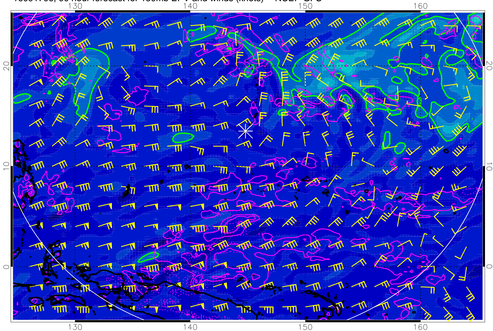
16091706, 90 hour forecast for 150mb EPV and winds (knots) -- NCEP GFS
