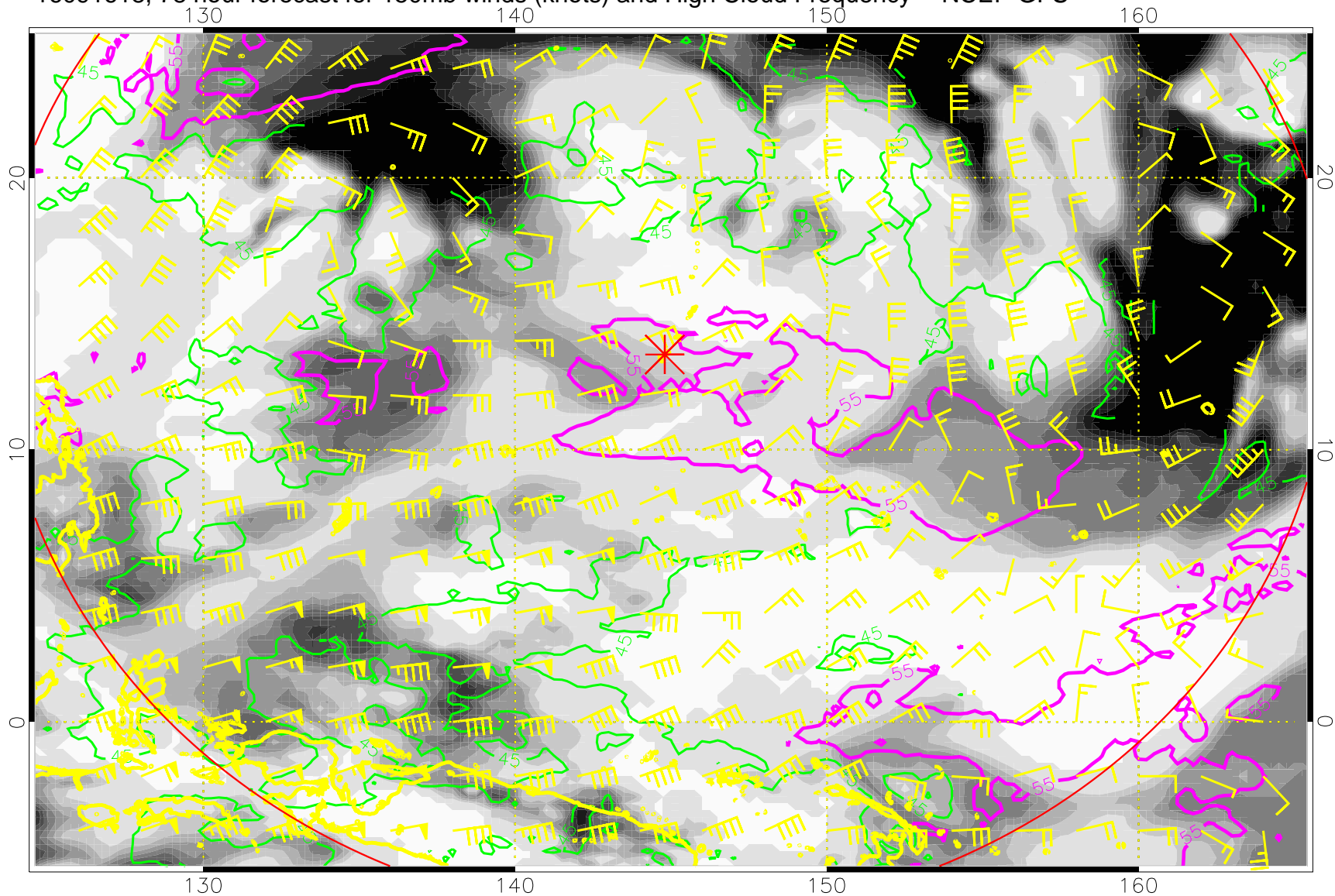
16091618, 78 hour forecast for 150mb winds (knots) and High Cloud Frequency -- NCEP GFS
