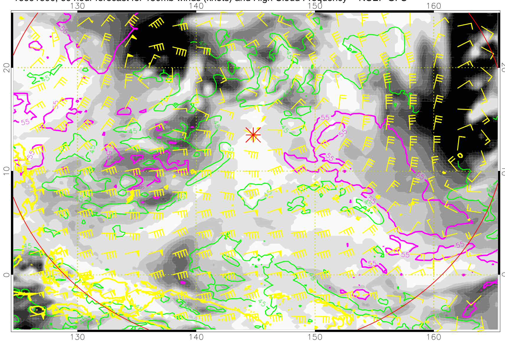
16091600, 60 hour forecast for 150mb winds (knots) and High Cloud Frequency -- NCEP GFS
