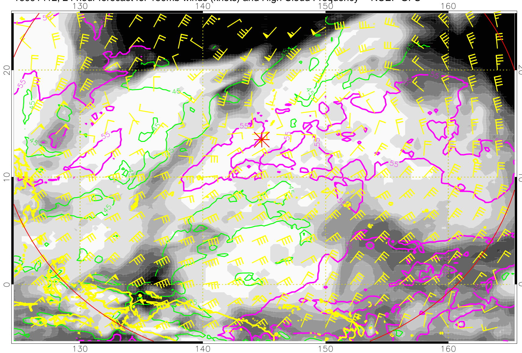
16091412, 24 hour forecast for 150mb winds (knots) and High Cloud Frequency -- NCEP GFS
