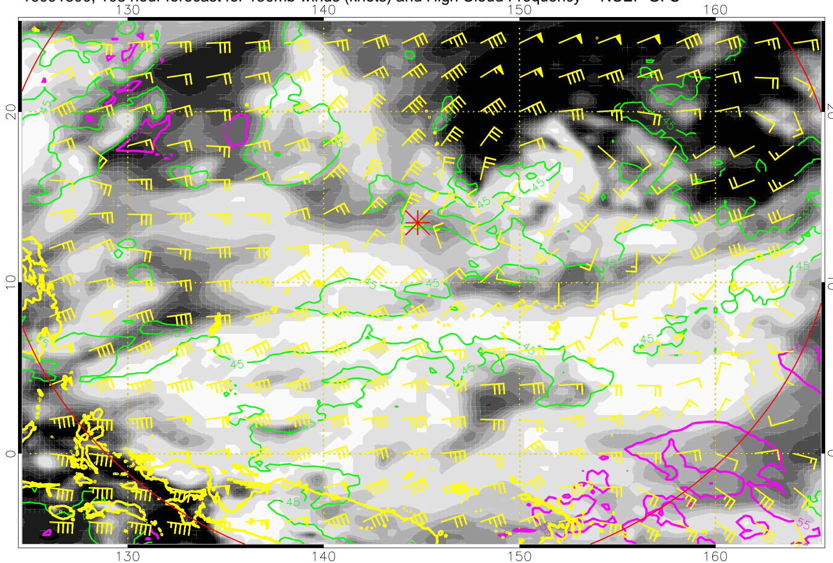
16091800, 108 hour forecast for 150mb winds (knots) and High Cloud Frequency -- NCEP GFS
