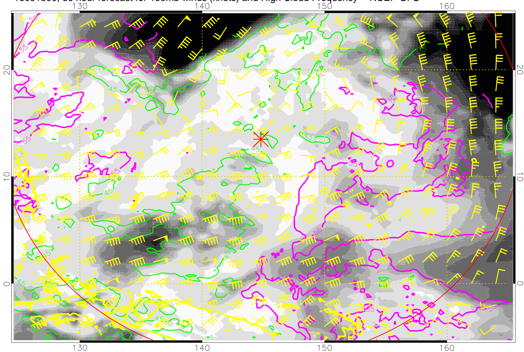
16091500, 36 hour forecast for 150mb winds (knots) and High Cloud Frequency -- NCEP GFS
