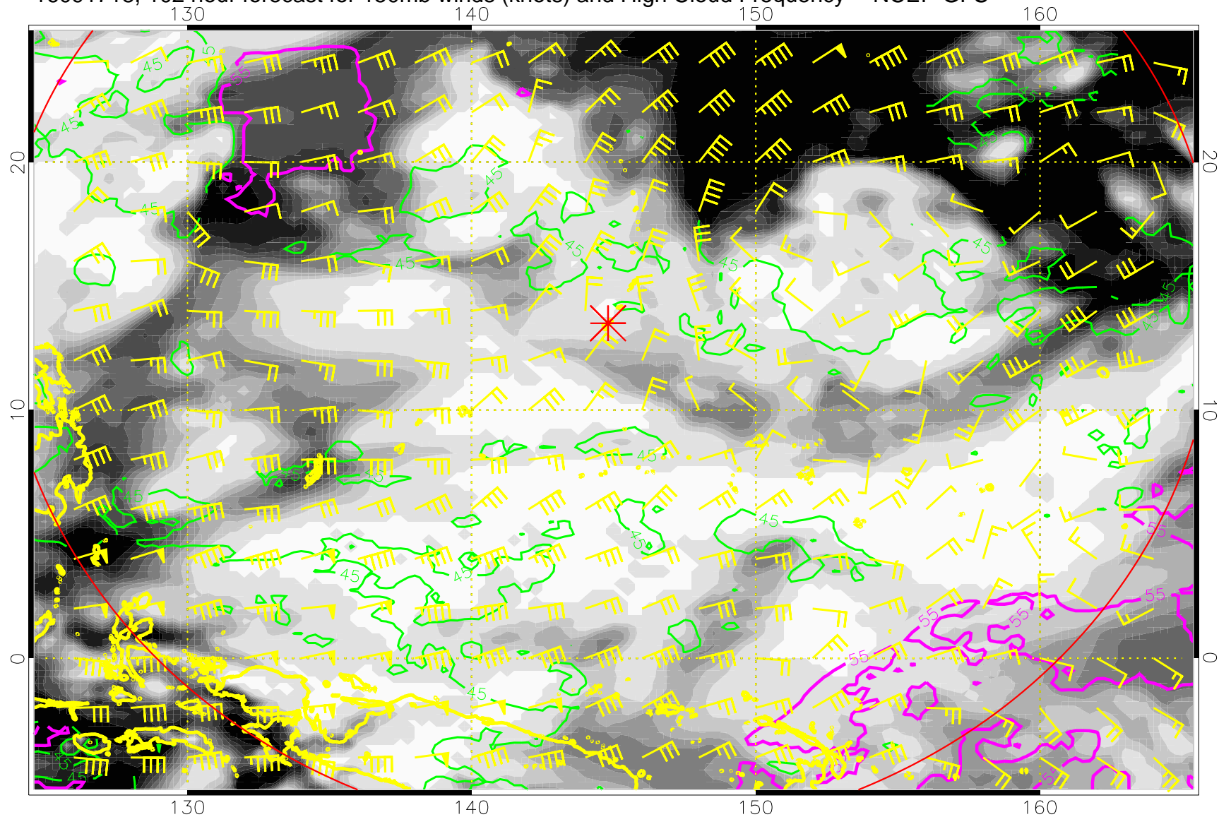
16091718, 102 hour forecast for 150mb winds (knots) and High Cloud Frequency -- NCEP GFS
