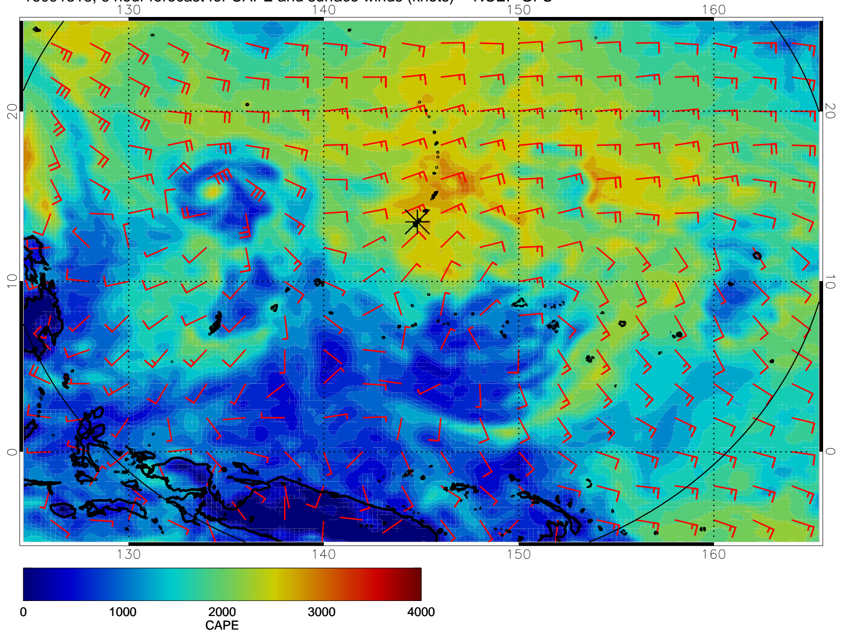
16091318, 6 hour forecast for CAPE and surface winds (knots) -- NCEP GFS
