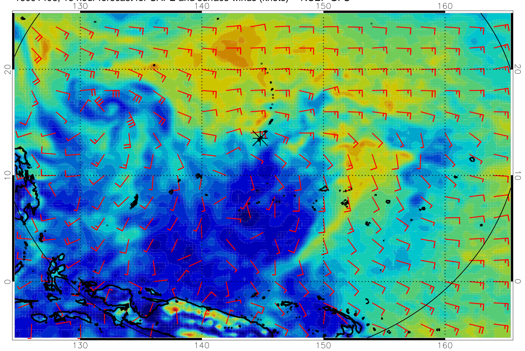
16091406, 18 hour forecast for CAPE and surface winds (knots) -- NCEP GFS
