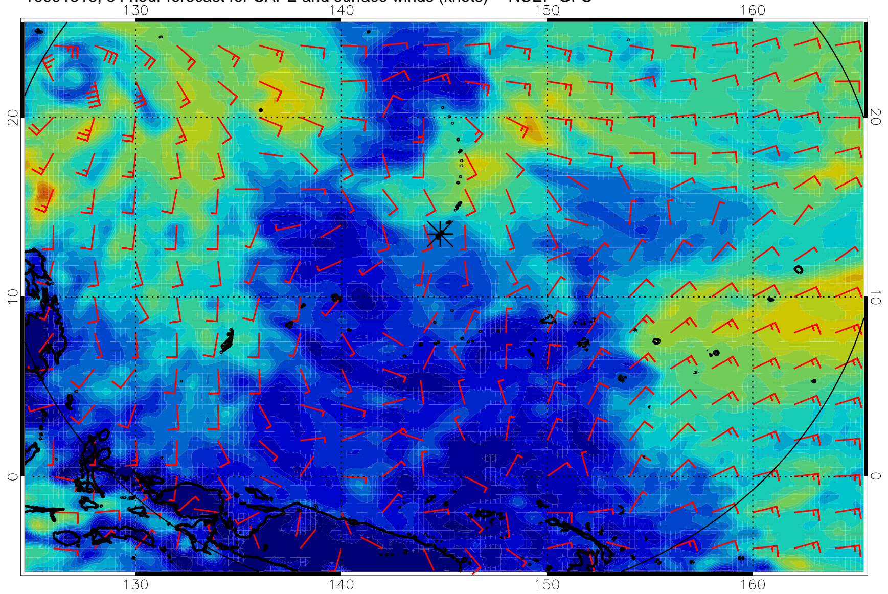
16091518, 54 hour forecast for CAPE and surface winds (knots) -- NCEP GFS
