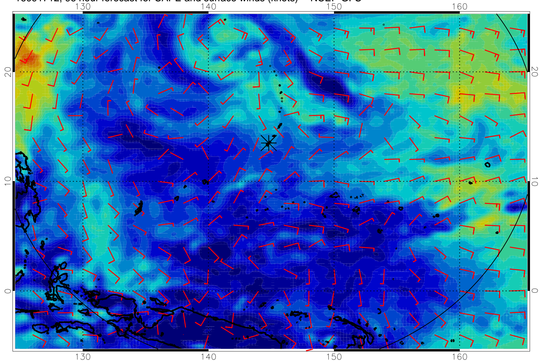
16091712, 96 hour forecast for CAPE and surface winds (knots) -- NCEP GFS
