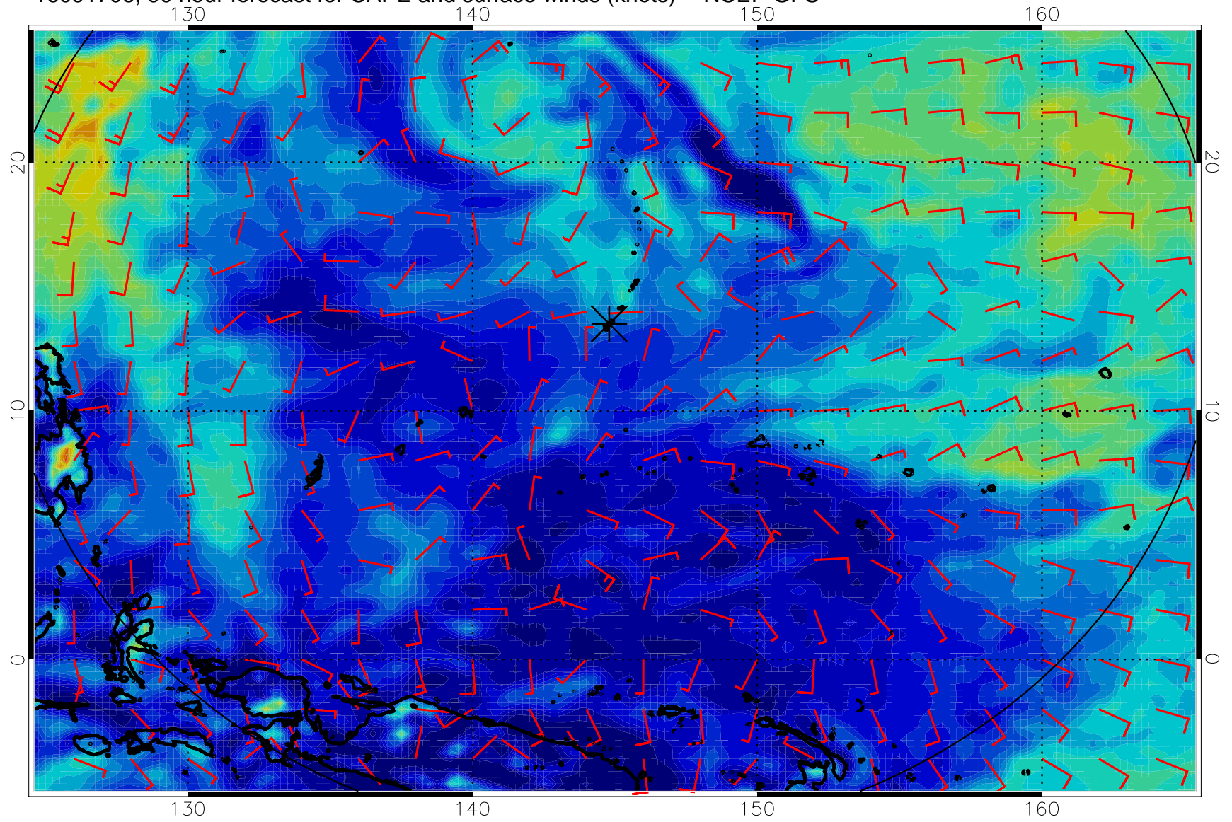
16091706, 90 hour forecast for CAPE and surface winds (knots) -- NCEP GFS
