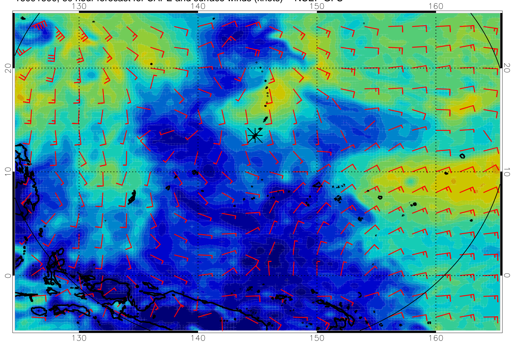
16091600, 60 hour forecast for CAPE and surface winds (knots) -- NCEP GFS
