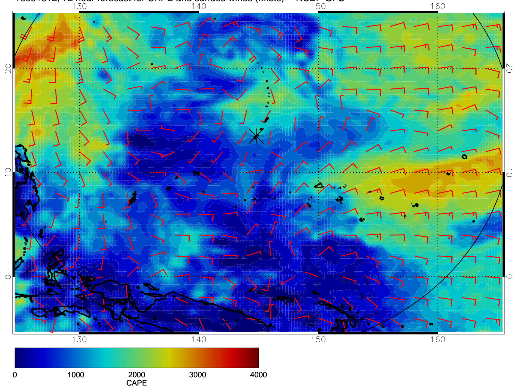
16091612, 72 hour forecast for CAPE and surface winds (knots) -- NCEP GFS
