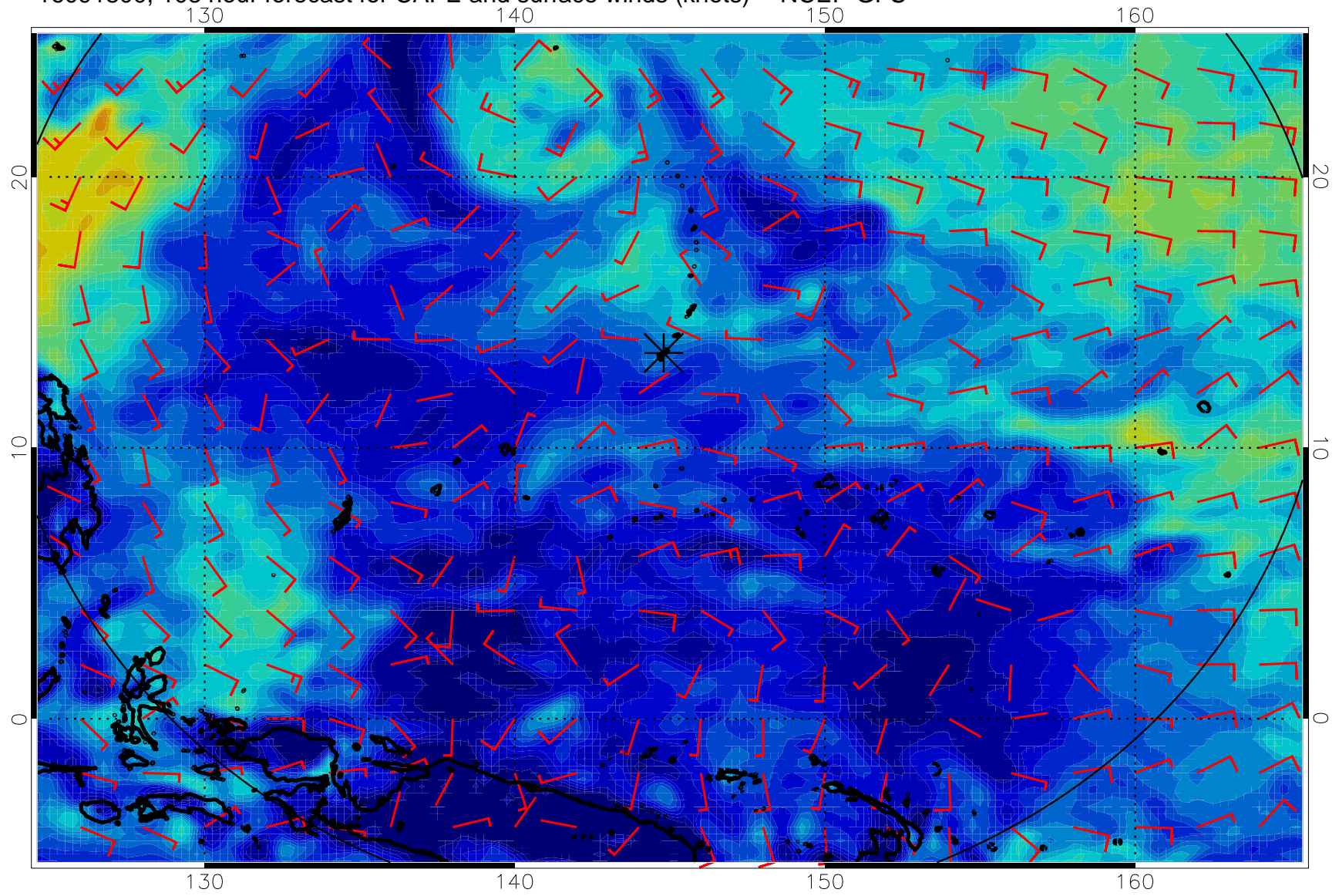
16091800, 108 hour forecast for CAPE and surface winds (knots) -- NCEP GFS
