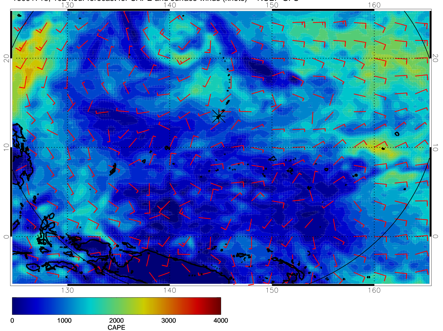
16091718, 102 hour forecast for CAPE and surface winds (knots) -- NCEP GFS
