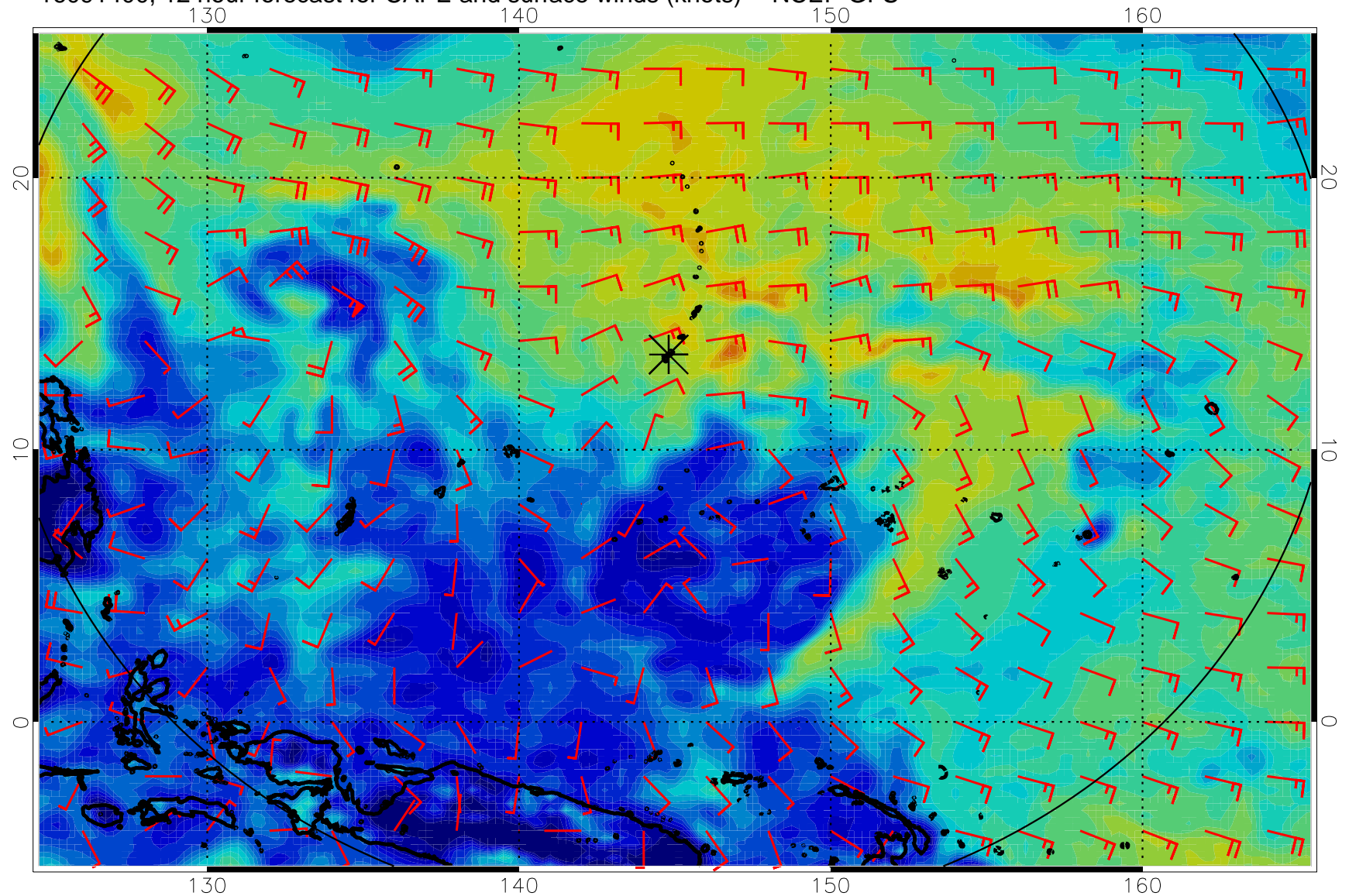
16091400, 12 hour forecast for CAPE and surface winds (knots) -- NCEP GFS
