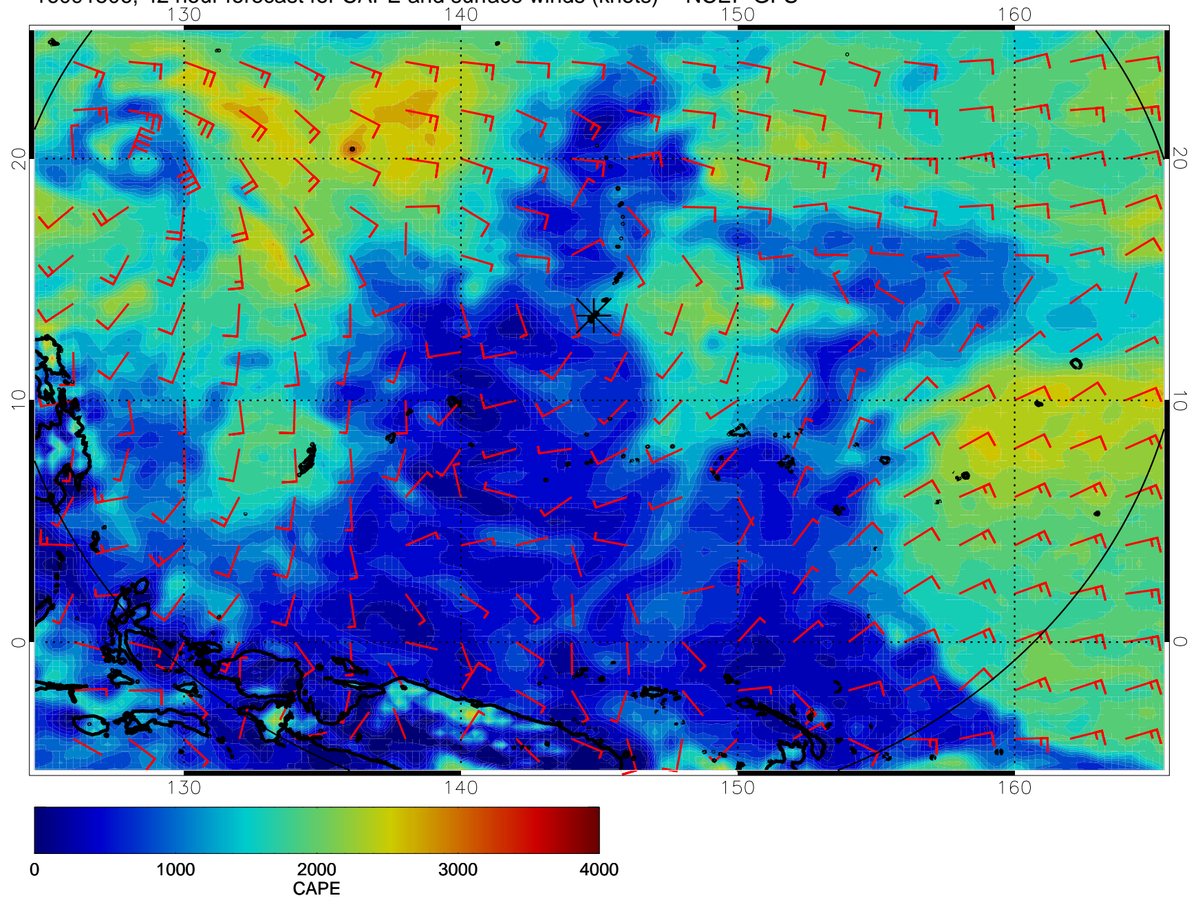
16091506, 42 hour forecast for CAPE and surface winds (knots) -- NCEP GFS
