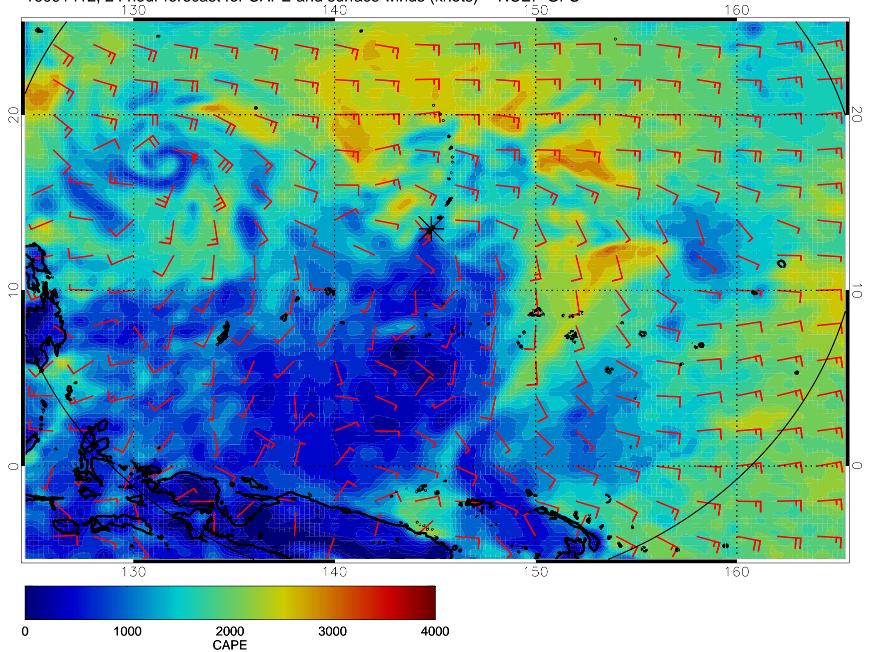
16091412, 24 hour forecast for CAPE and surface winds (knots) -- NCEP GFS
