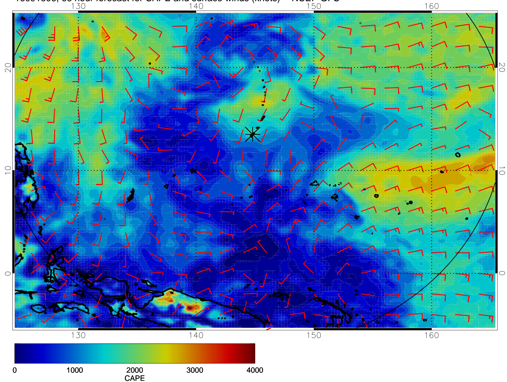
16091606, 66 hour forecast for CAPE and surface winds (knots) -- NCEP GFS
