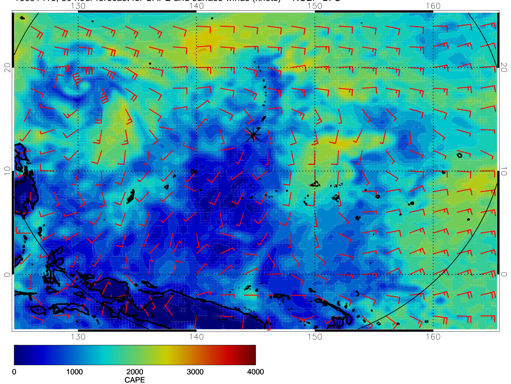
16091418, 30 hour forecast for CAPE and surface winds (knots) -- NCEP GFS
