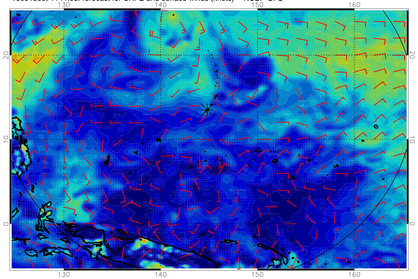
16091806, 114 hour forecast for CAPE and surface winds (knots) -- NCEP GFS
