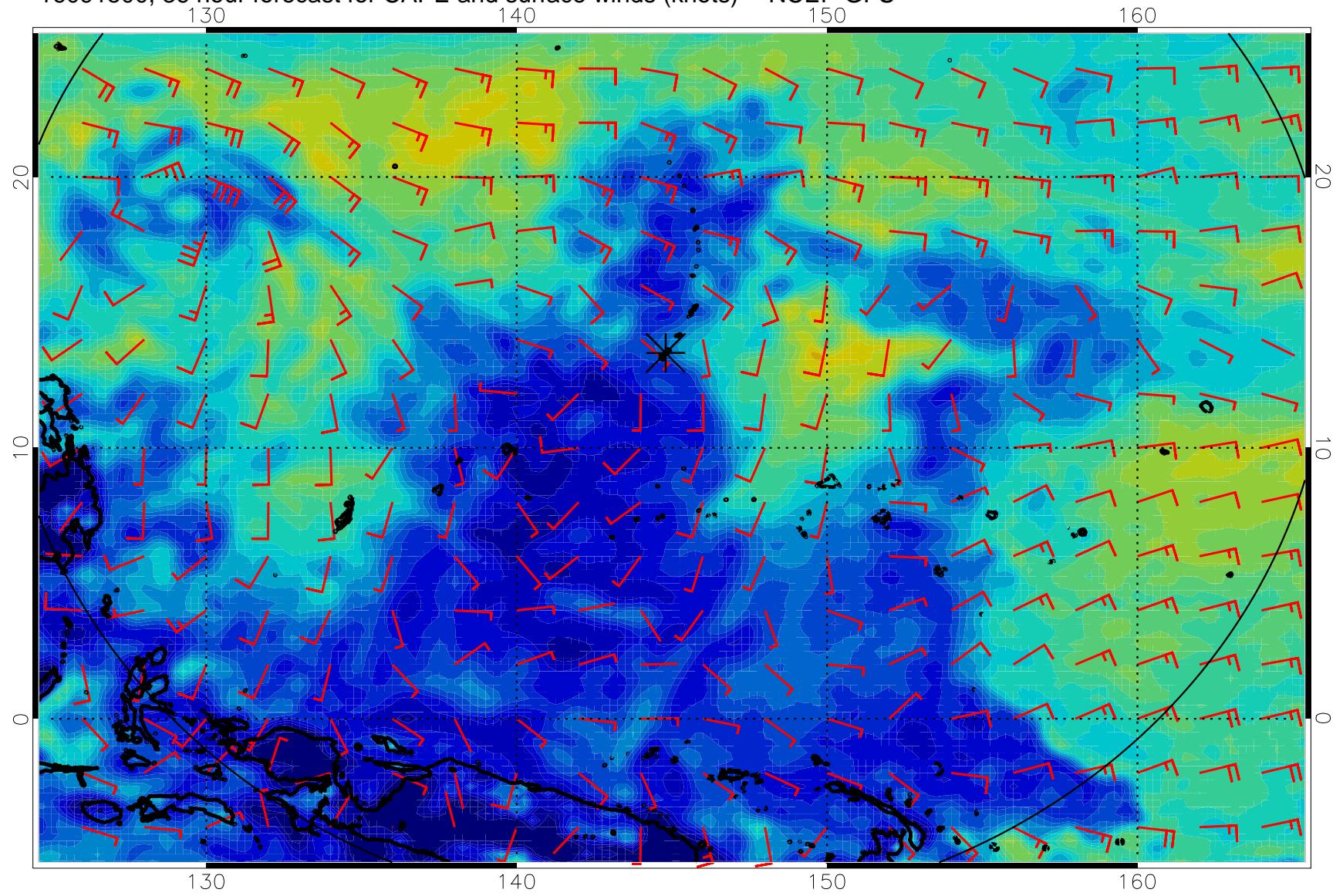
16091500, 36 hour forecast for CAPE and surface winds (knots) -- NCEP GFS
