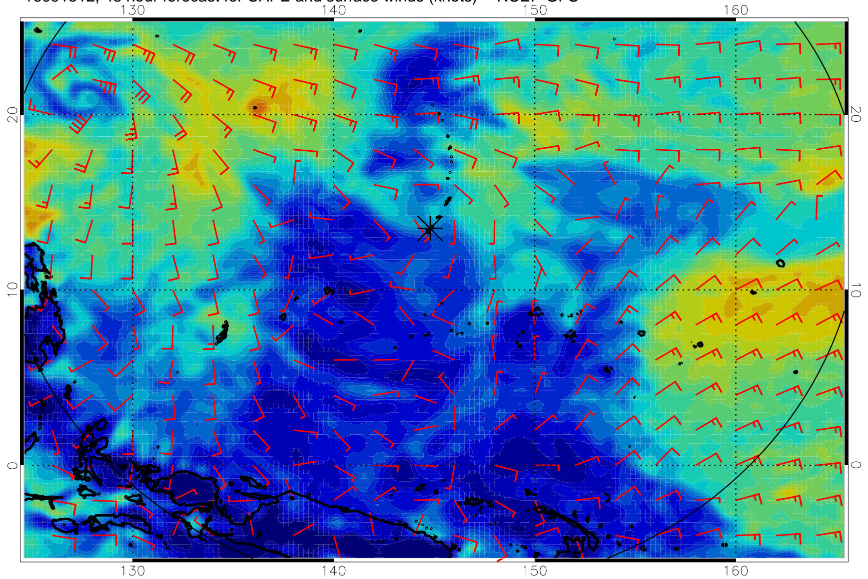
16091512, 48 hour forecast for CAPE and surface winds (knots) -- NCEP GFS
