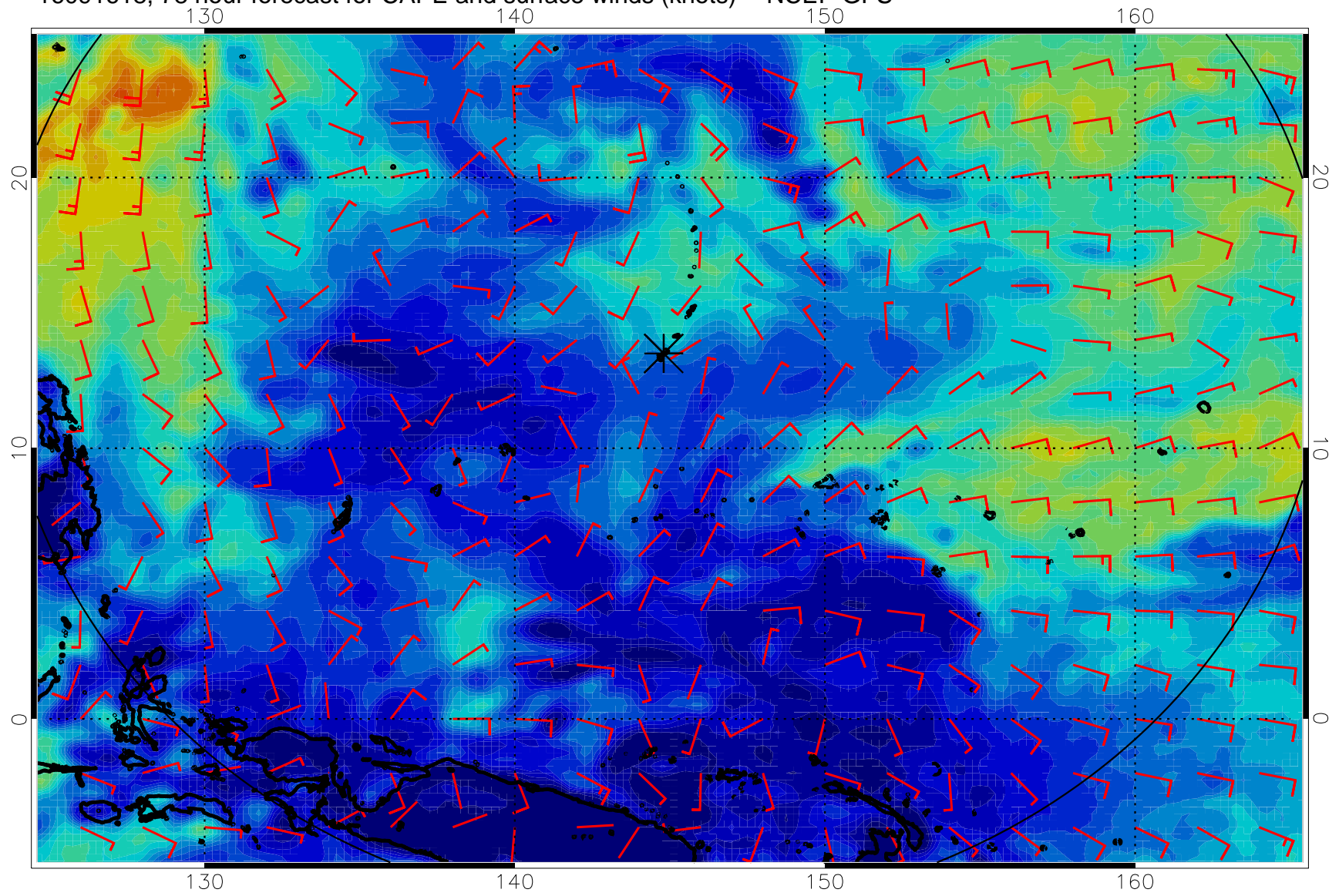
16091618, 78 hour forecast for CAPE and surface winds (knots) -- NCEP GFS
