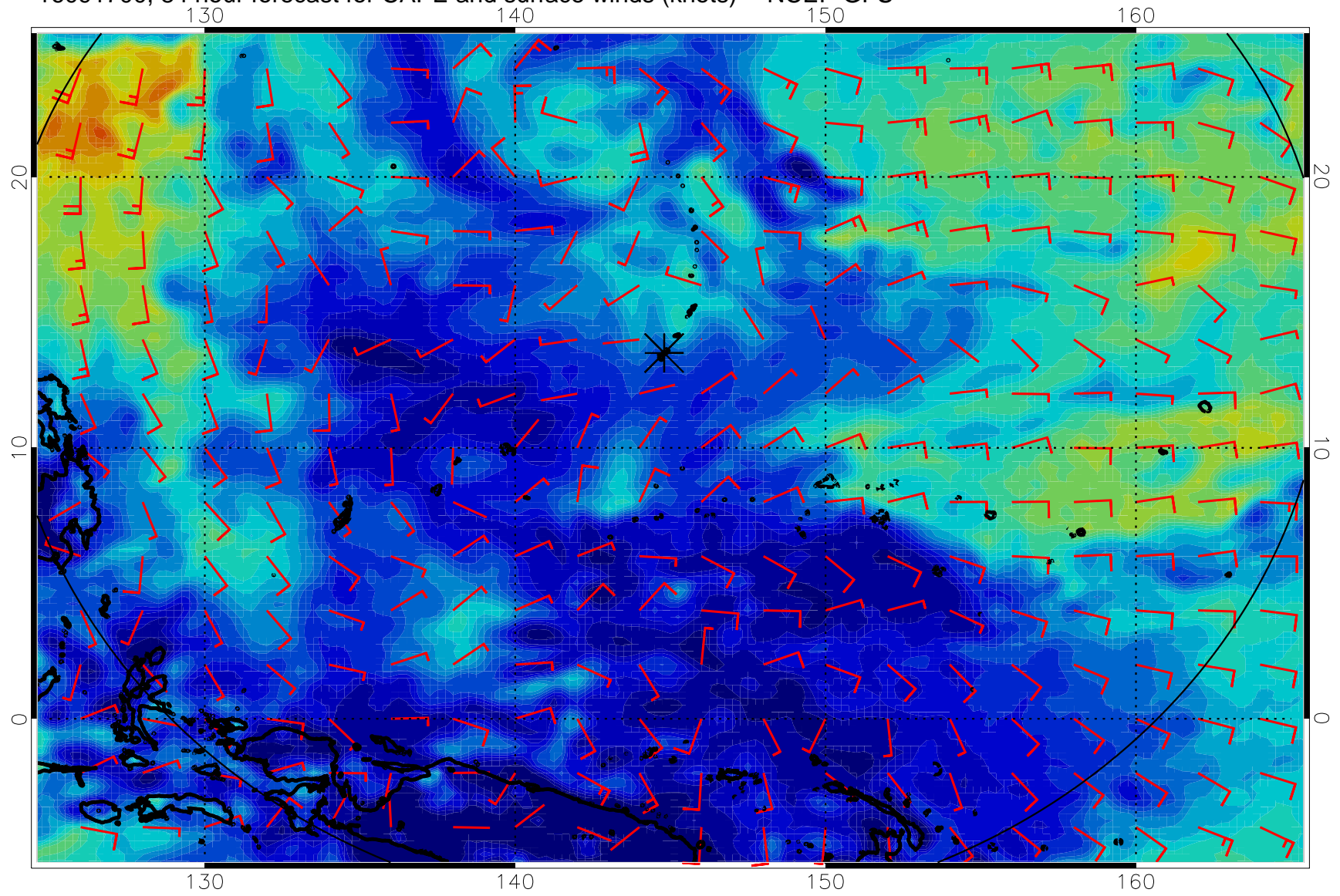
16091700, 84 hour forecast for CAPE and surface winds (knots) -- NCEP GFS
