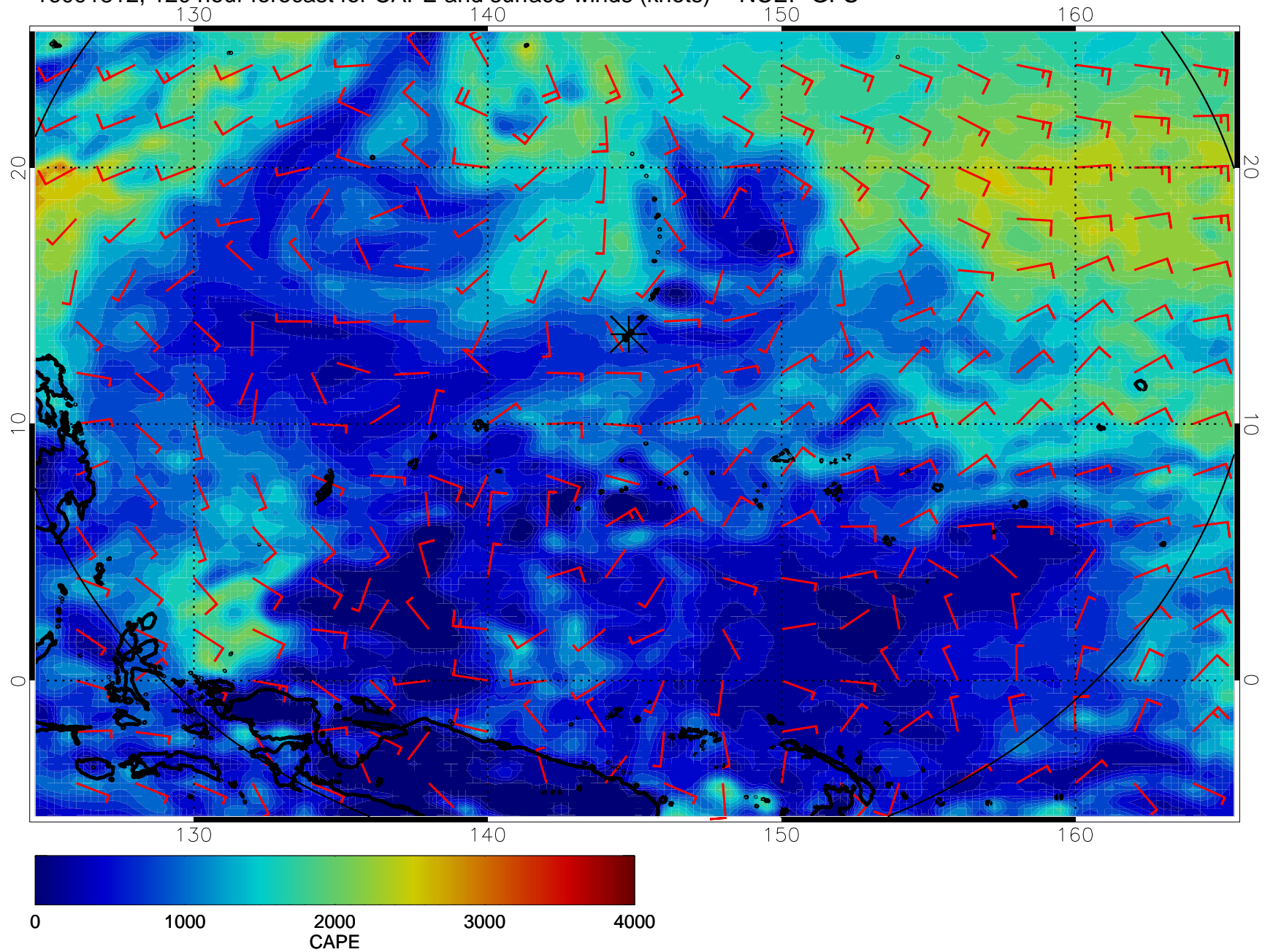
16091812, 120 hour forecast for CAPE and surface winds (knots) -- NCEP GFS
