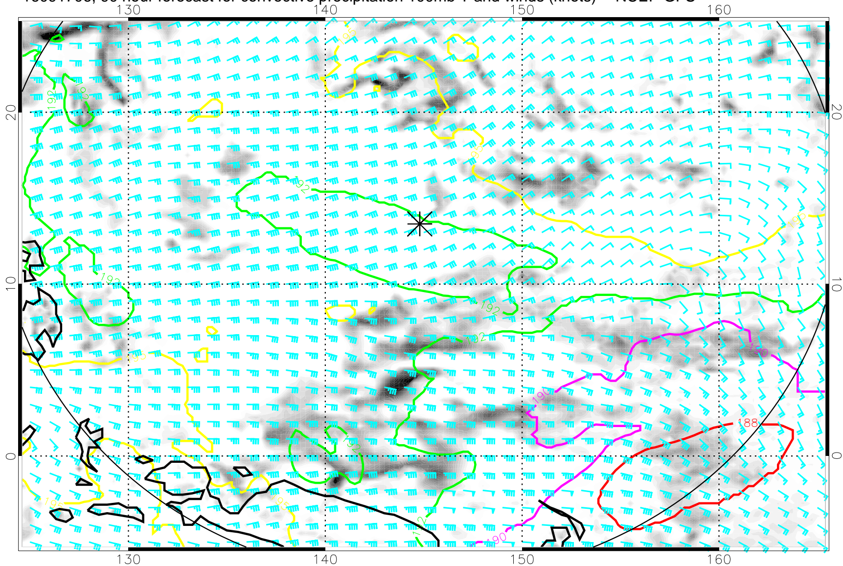
16091706, 90 hour forecast for convective precipitation 100mb T and winds (knots) -- NCEP GFS
