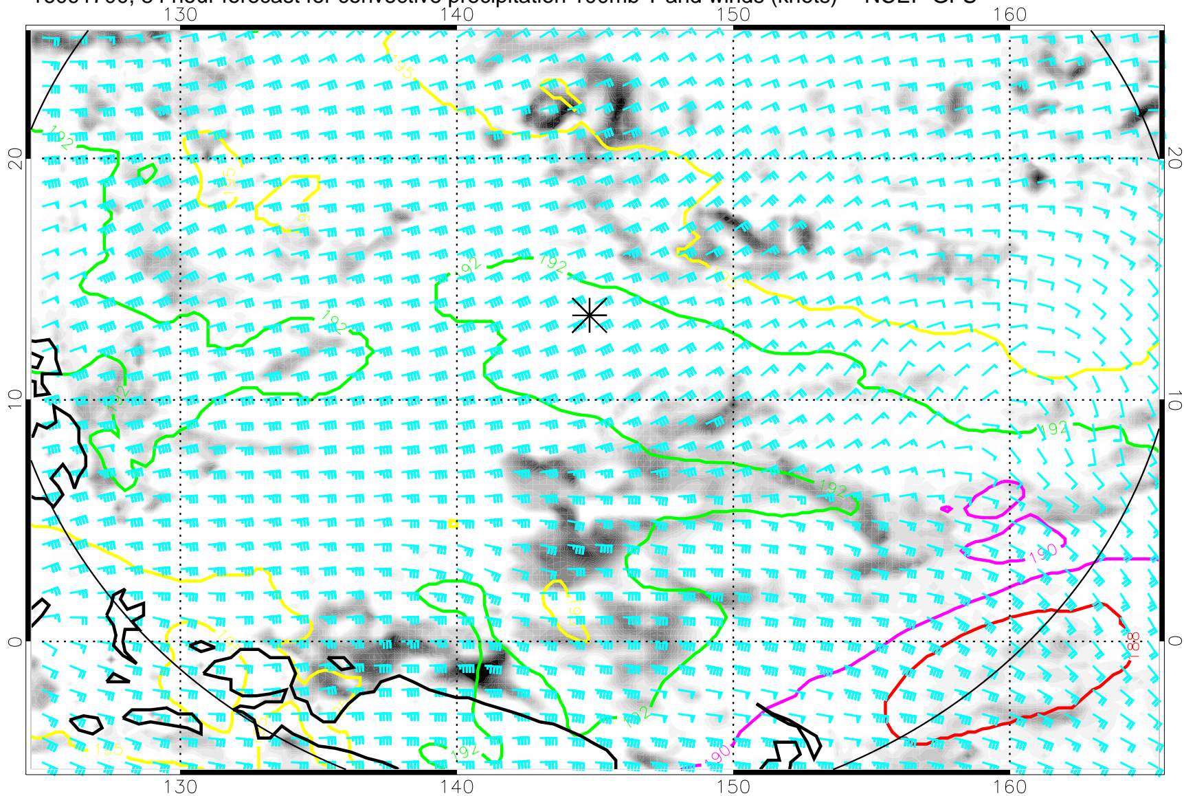
16091700, 84 hour forecast for convective precipitation 100mb T and winds (knots) -- NCEP GFS
