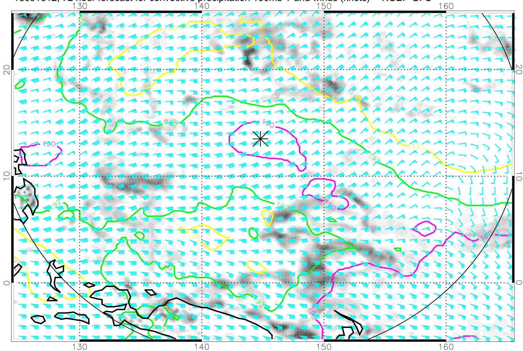
16091612, 72 hour forecast for convective precipitation 100mb T and winds (knots) -- NCEP GFS
