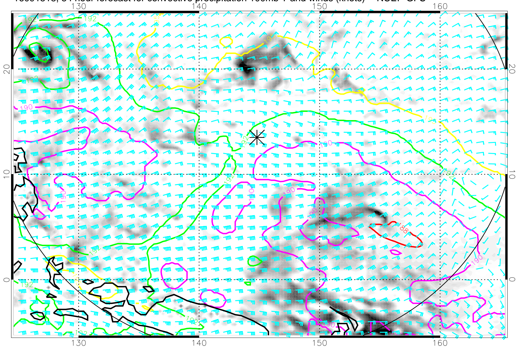
16091518, 54 hour forecast for convective precipitation 100mb T and winds (knots) -- NCEP GFS
