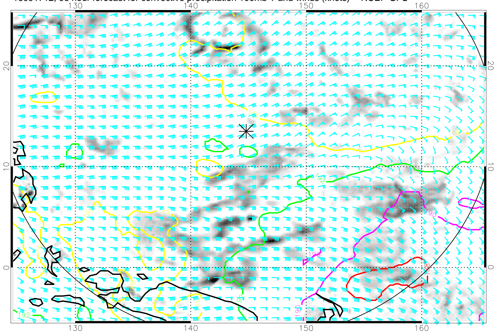
16091712, 96 hour forecast for convective precipitation 100mb T and winds (knots) -- NCEP GFS
