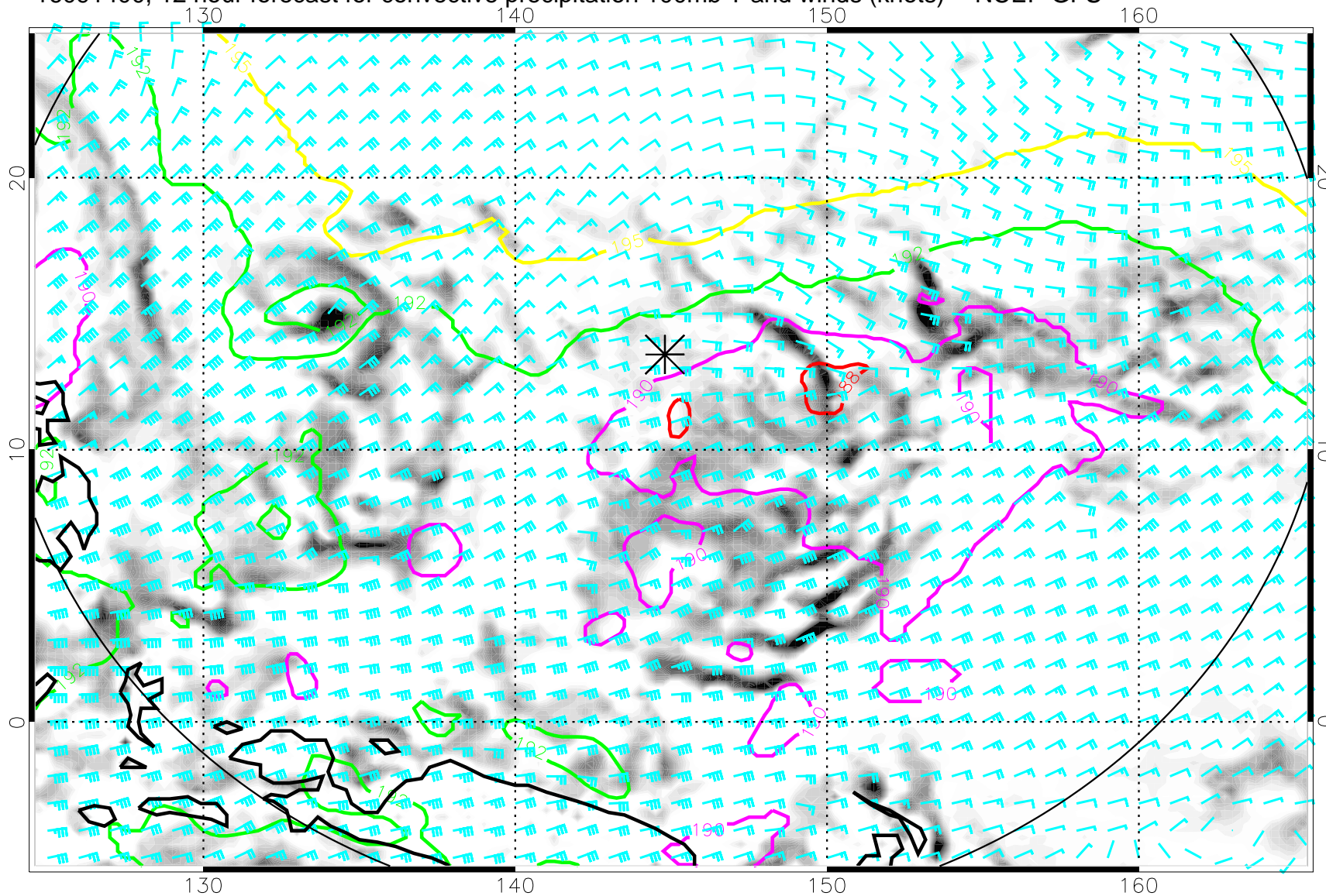
16091400, 12 hour forecast for convective precipitation 100mb T and winds (knots) -- NCEP GFS
