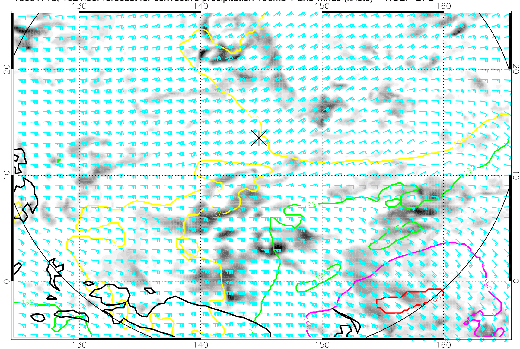
16091718, 102 hour forecast for convective precipitation 100mb T and winds (knots) -- NCEP GFS
