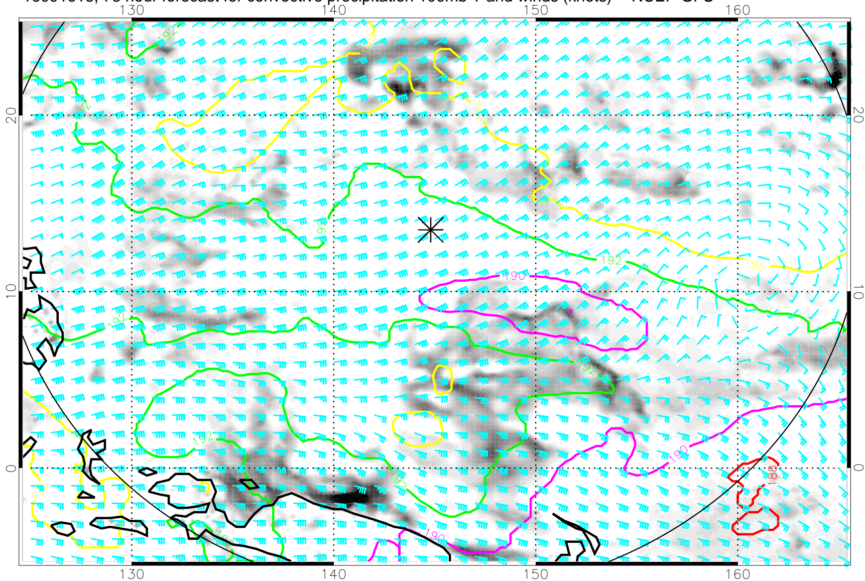
16091618, 78 hour forecast for convective precipitation 100mb T and winds (knots) -- NCEP GFS
