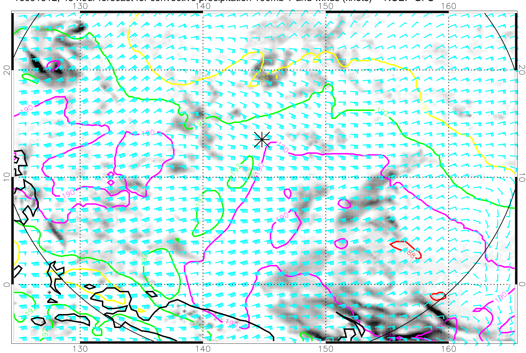
16091512, 48 hour forecast for convective precipitation 100mb T and winds (knots) -- NCEP GFS
