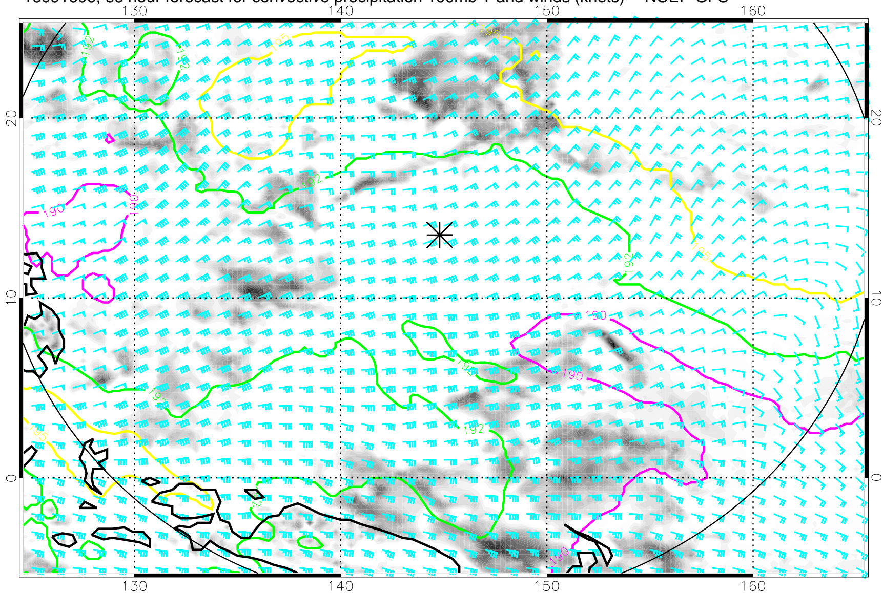
16091606, 66 hour forecast for convective precipitation 100mb T and winds (knots) -- NCEP GFS
