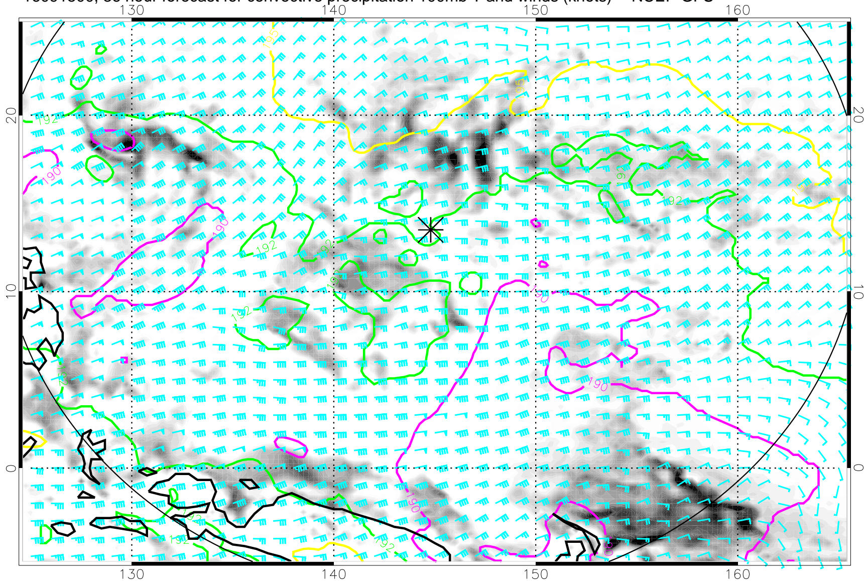
16091500, 36 hour forecast for convective precipitation 100mb T and winds (knots) -- NCEP GFS
