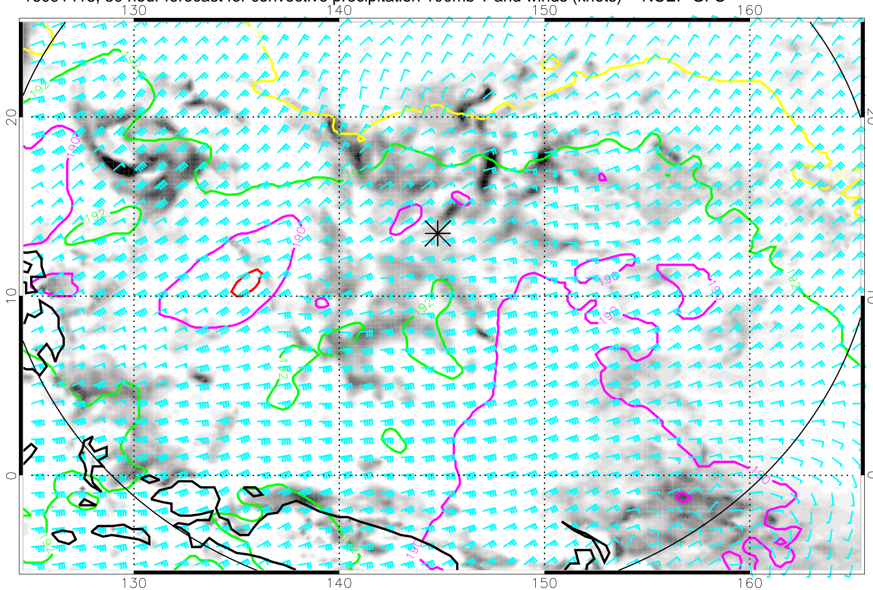
16091418, 30 hour forecast for convective precipitation 100mb T and winds (knots) -- NCEP GFS
