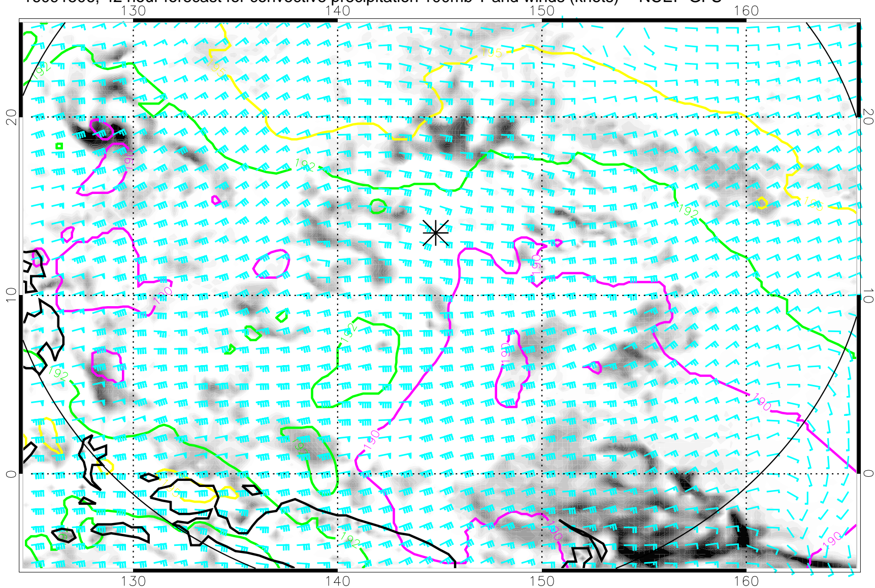
16091506, 42 hour forecast for convective precipitation 100mb T and winds (knots) -- NCEP GFS
