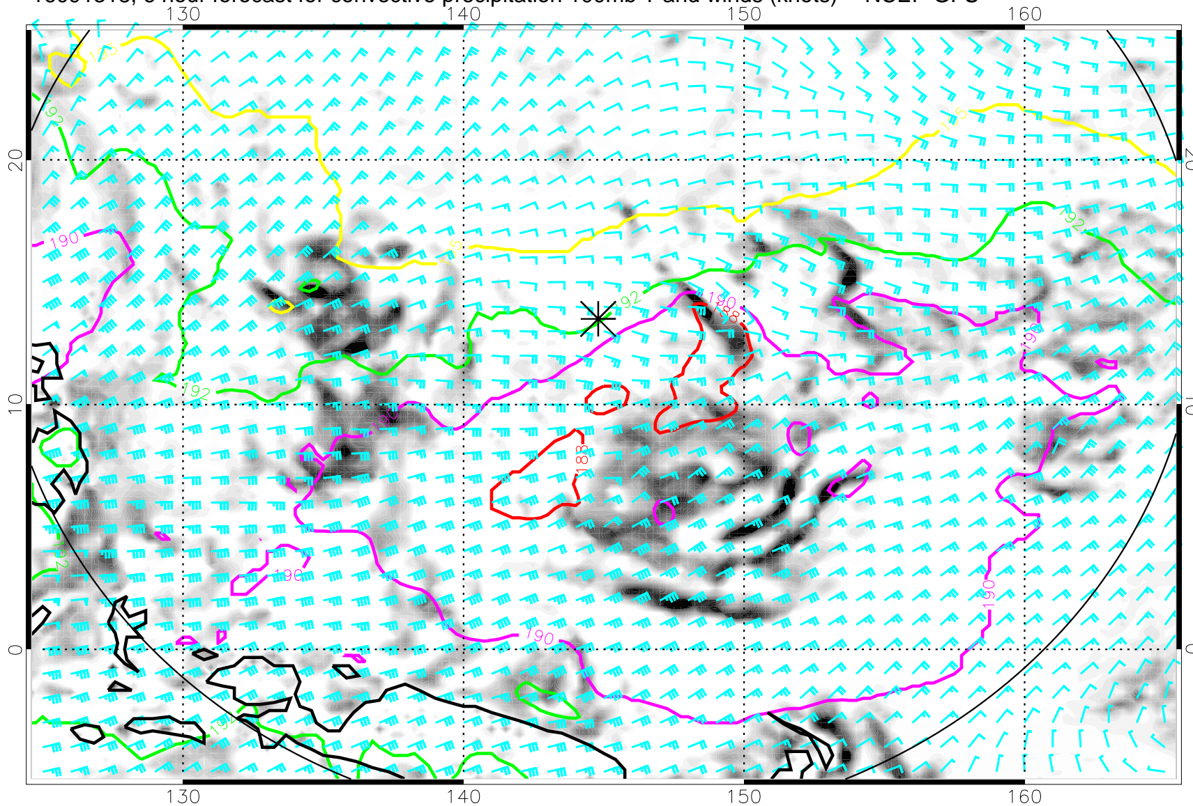
16091318, 6 hour forecast for convective precipitation 100mb T and winds (knots) -- NCEP GFS
