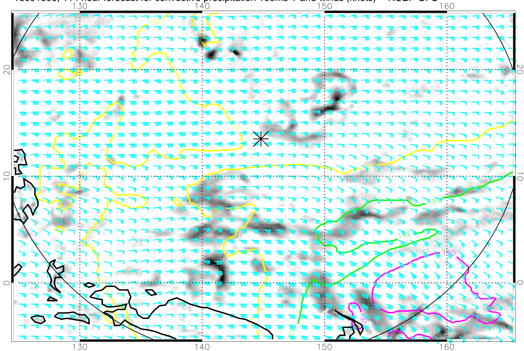
16091806, 114 hour forecast for convective precipitation 100mb T and winds (knots) -- NCEP GFS
