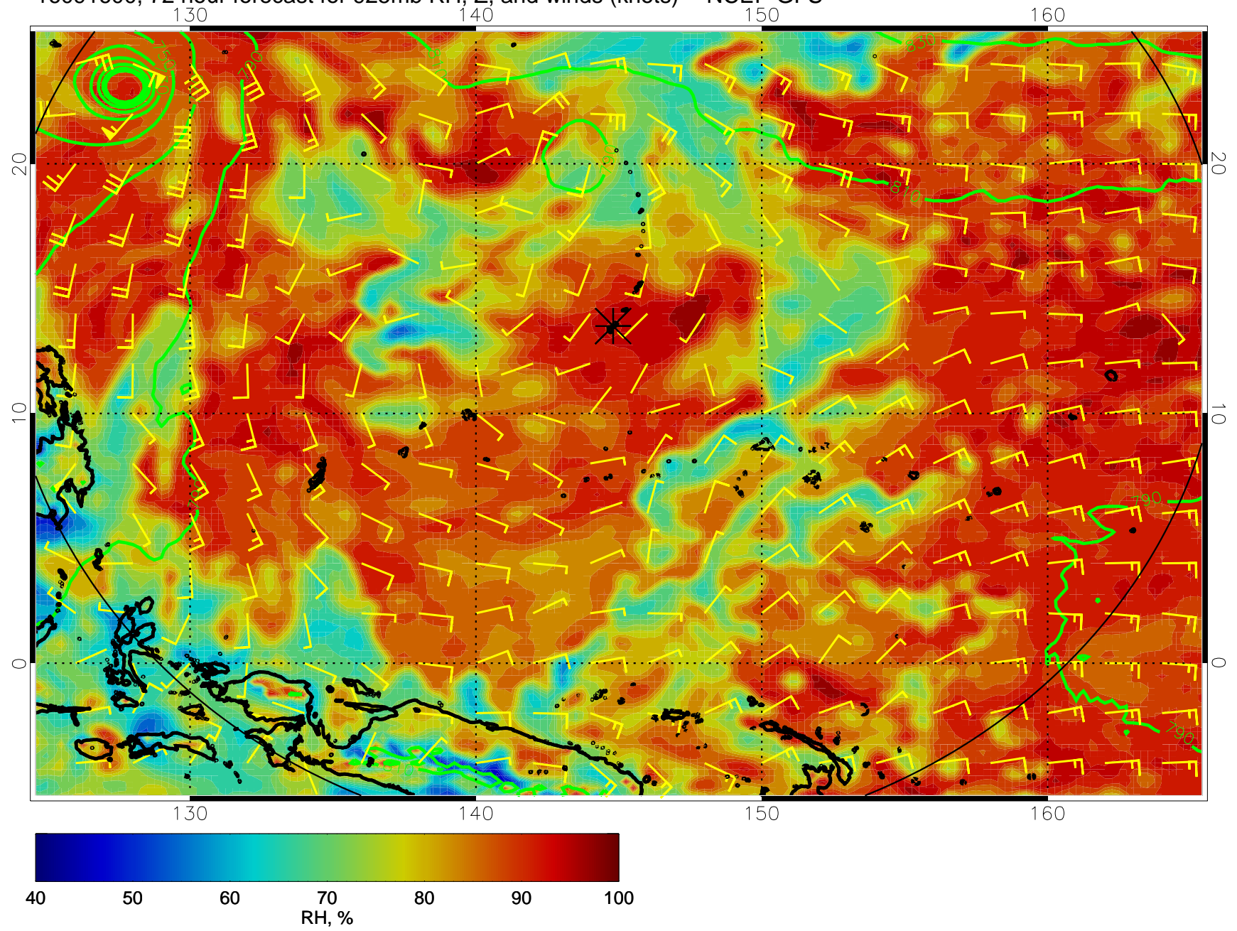
16091600, 72 hour forecast for 925mb RH, Z, and winds (knots) -- NCEP GFS
