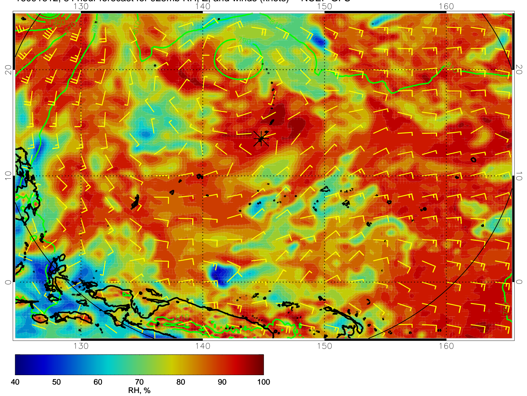
16091612, 84 hour forecast for 925mb RH, Z, and winds (knots) -- NCEP GFS
