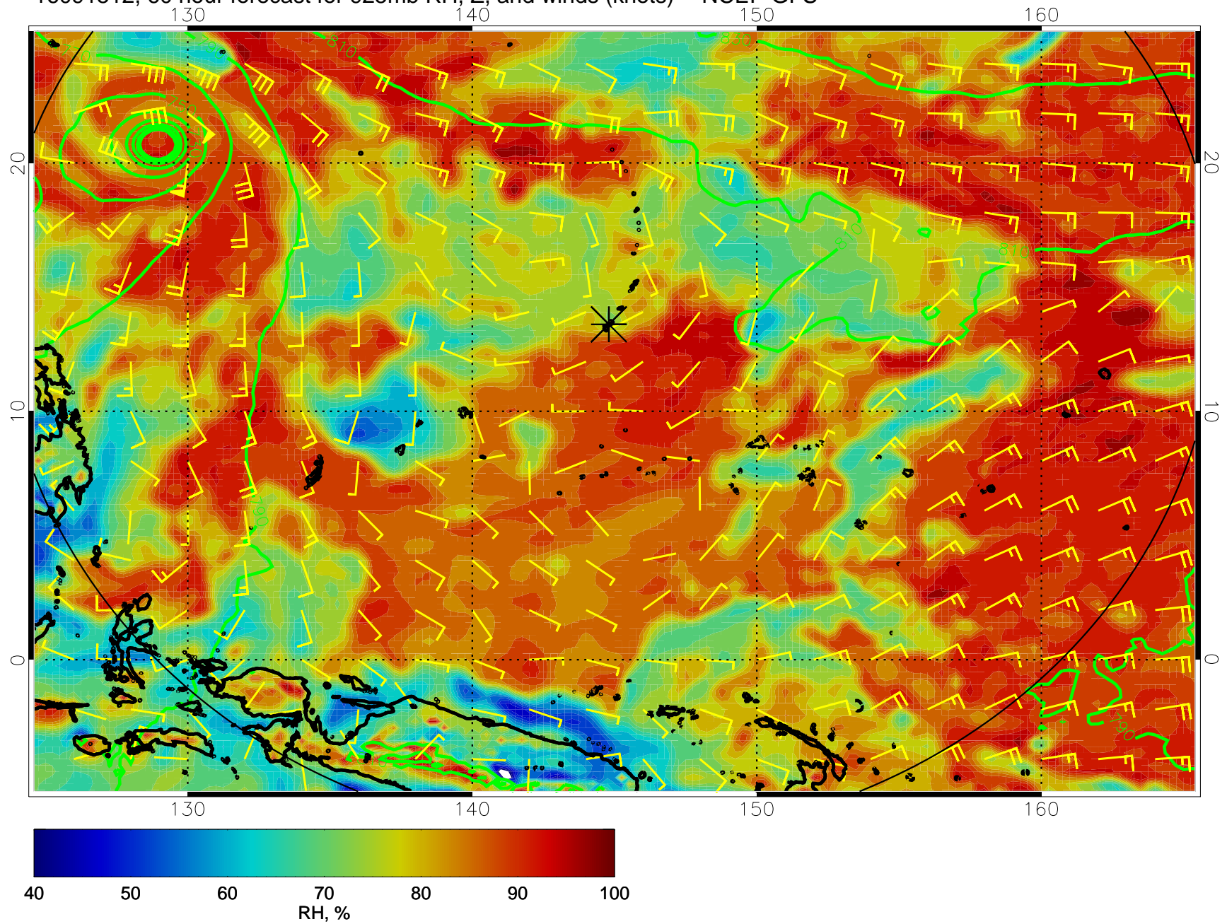
16091512, 60 hour forecast for 925mb RH, Z, and winds (knots) -- NCEP GFS
