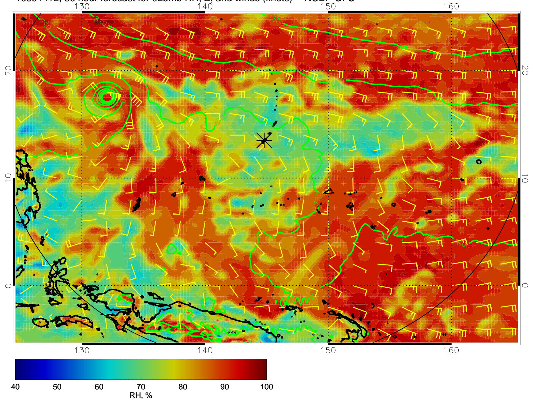
16091412, 36 hour forecast for 925mb RH, Z, and winds (knots) -- NCEP GFS
