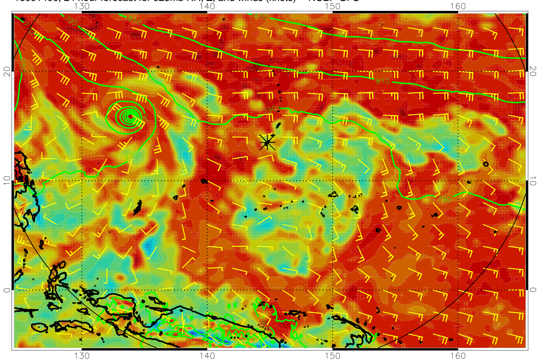
16091400, 24 hour forecast for 925mb RH, Z, and winds (knots) -- NCEP GFS
