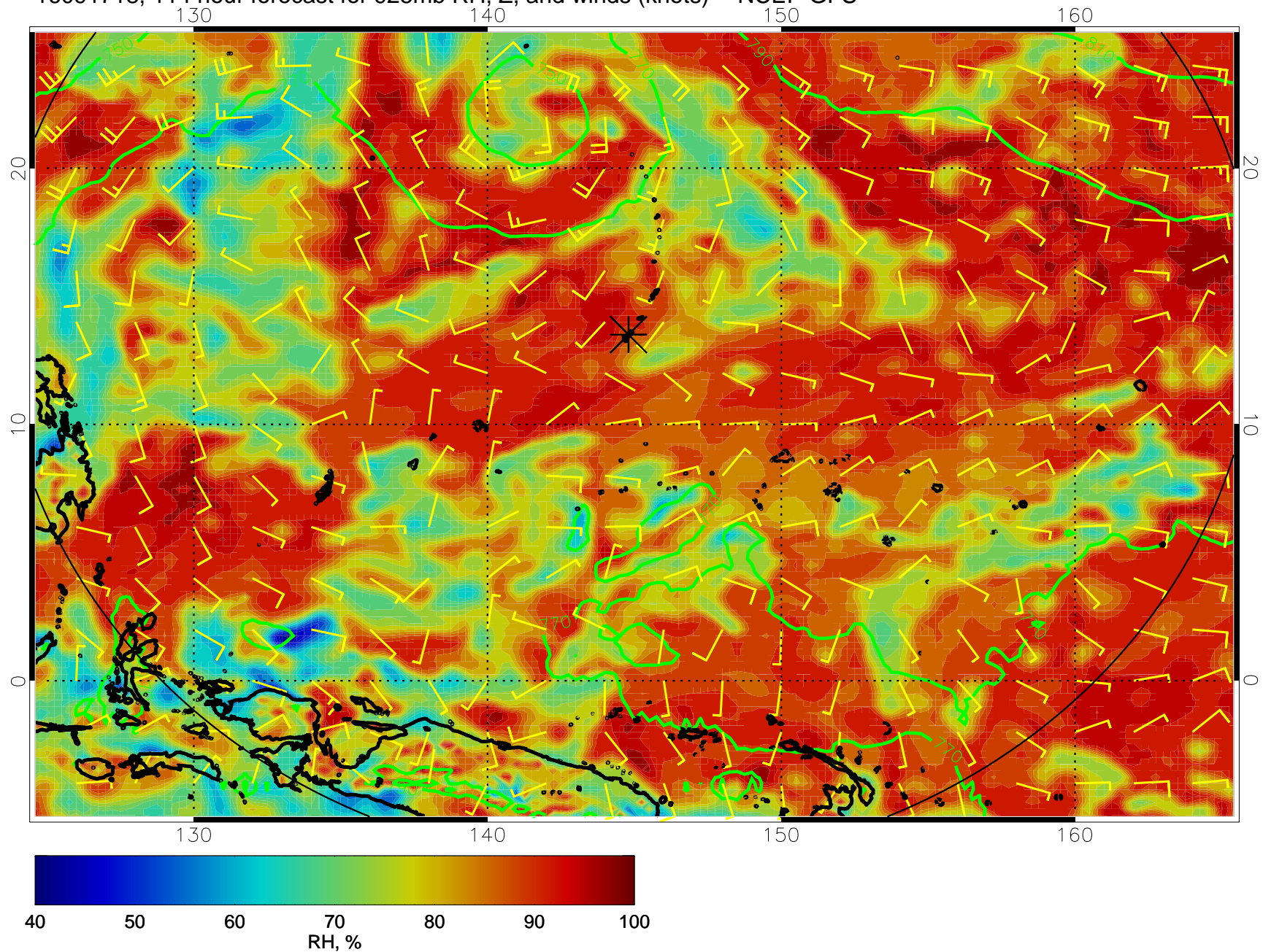
16091718, 114 hour forecast for 925mb RH, Z, and winds (knots) -- NCEP GFS
