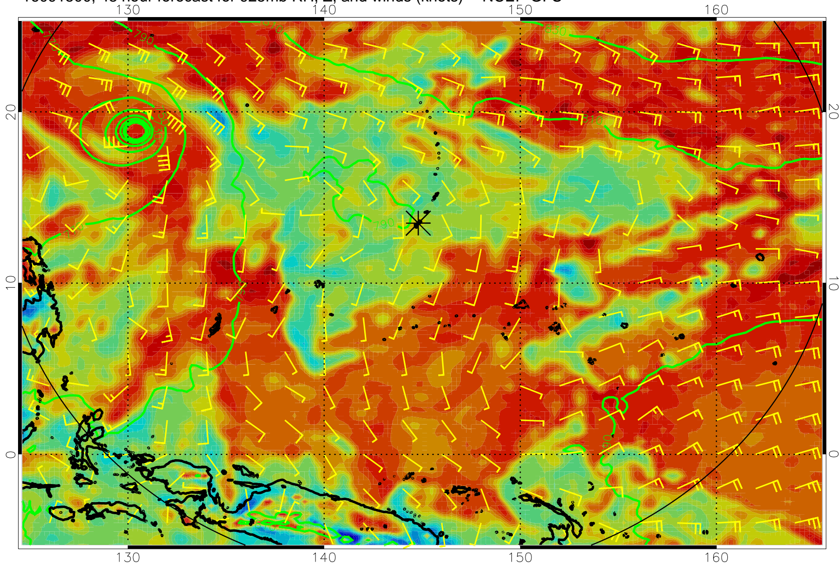
16091500, 48 hour forecast for 925mb RH, Z, and winds (knots) -- NCEP GFS
