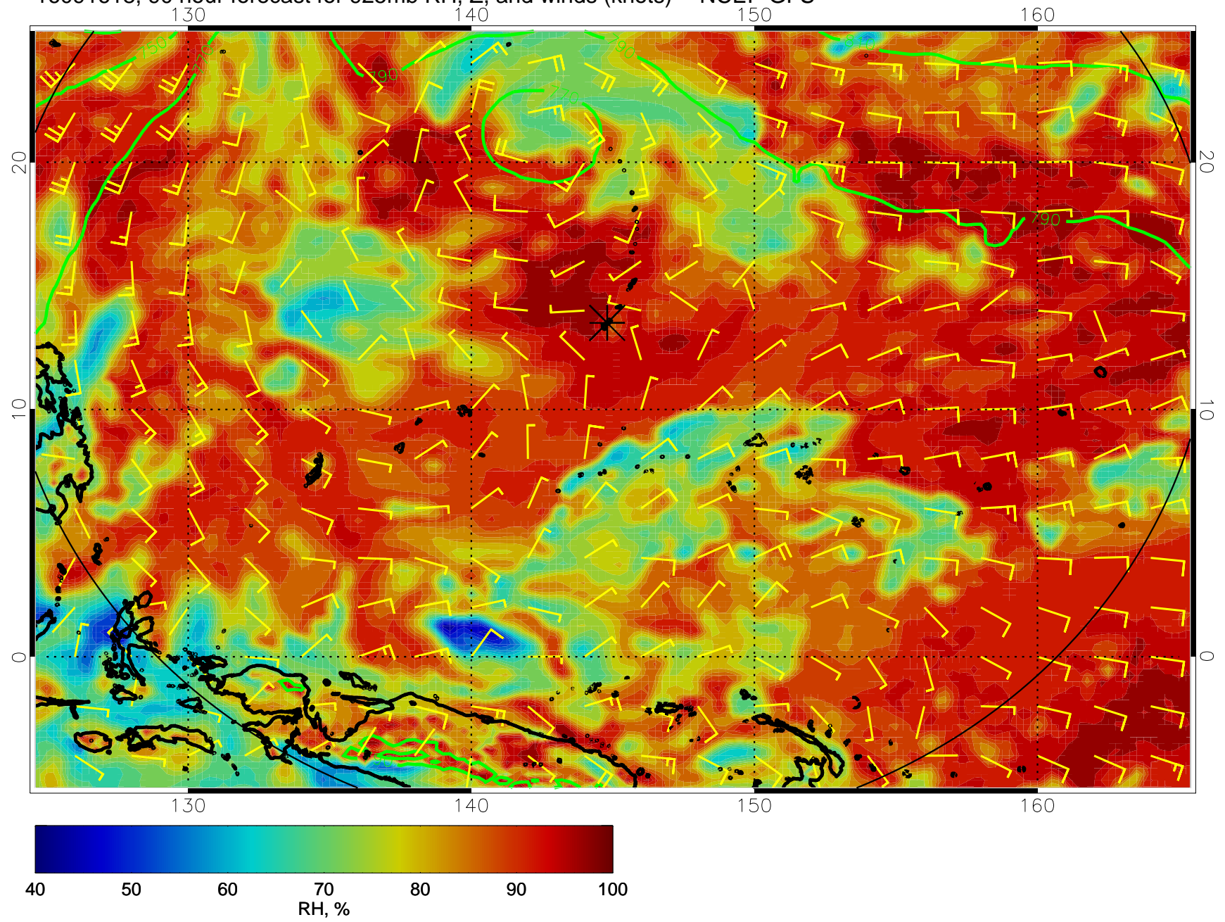
16091618, 90 hour forecast for 925mb RH, Z, and winds (knots) -- NCEP GFS
