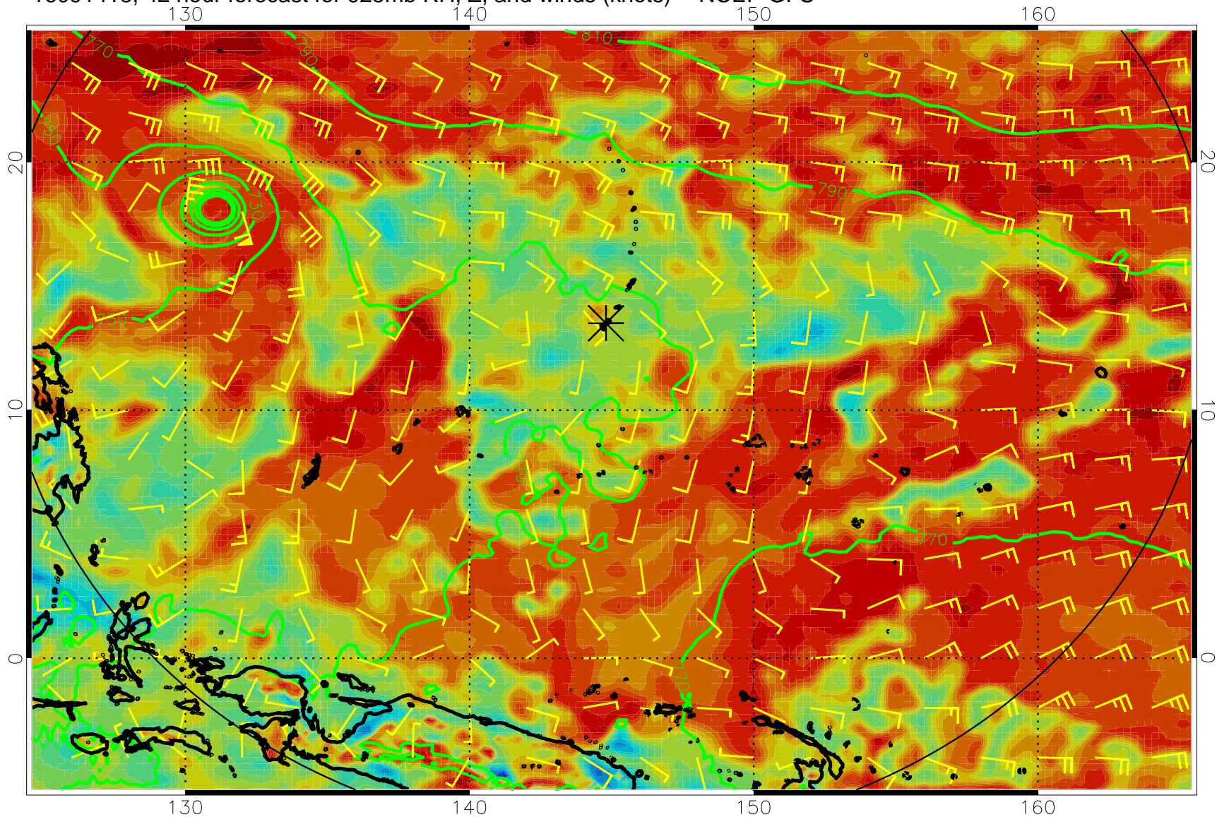
16091418, 42 hour forecast for 925mb RH, Z, and winds (knots) -- NCEP GFS
