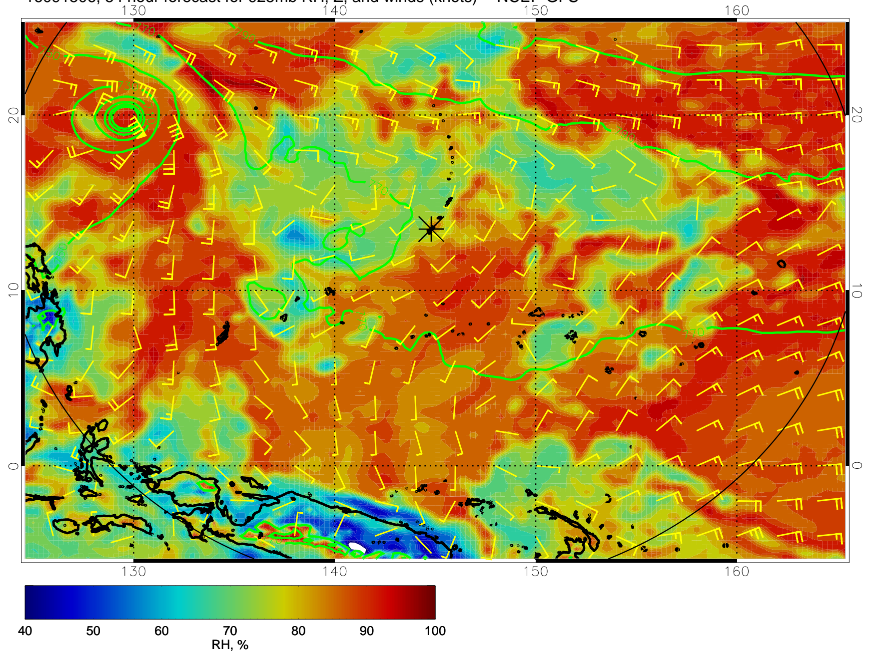
16091506, 54 hour forecast for 925mb RH, Z, and winds (knots) -- NCEP GFS
