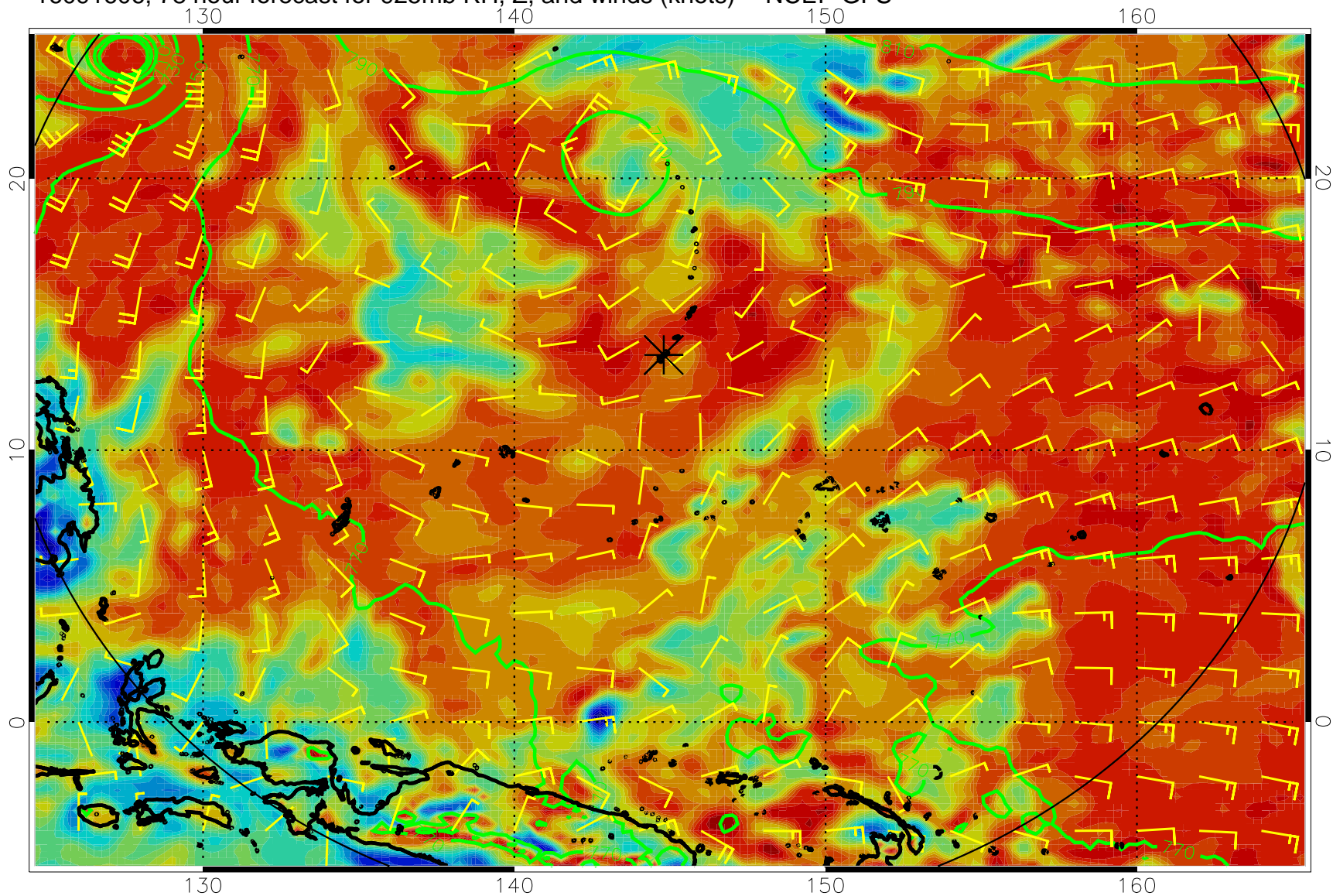
16091606, 78 hour forecast for 925mb RH, Z, and winds (knots) -- NCEP GFS
