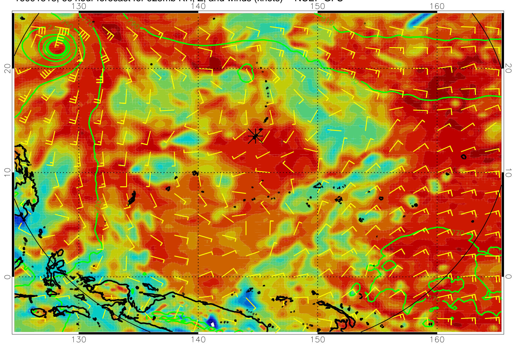
16091518, 66 hour forecast for 925mb RH, Z, and winds (knots) -- NCEP GFS
