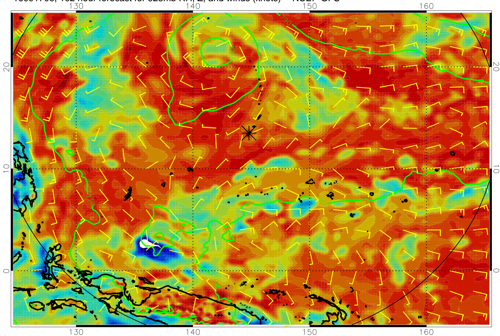
16091706, 102 hour forecast for 925mb RH, Z, and winds (knots) -- NCEP GFS
