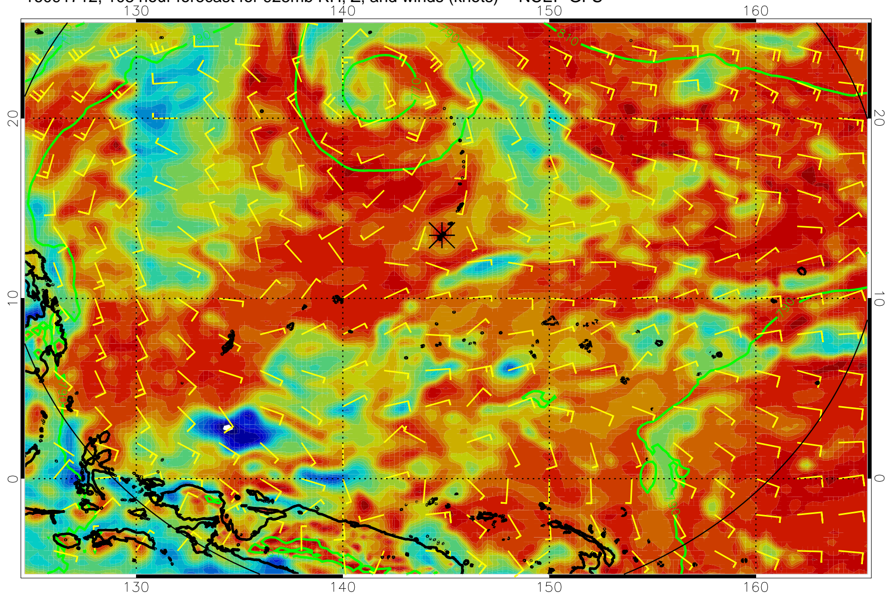
16091712, 108 hour forecast for 925mb RH, Z, and winds (knots) -- NCEP GFS
