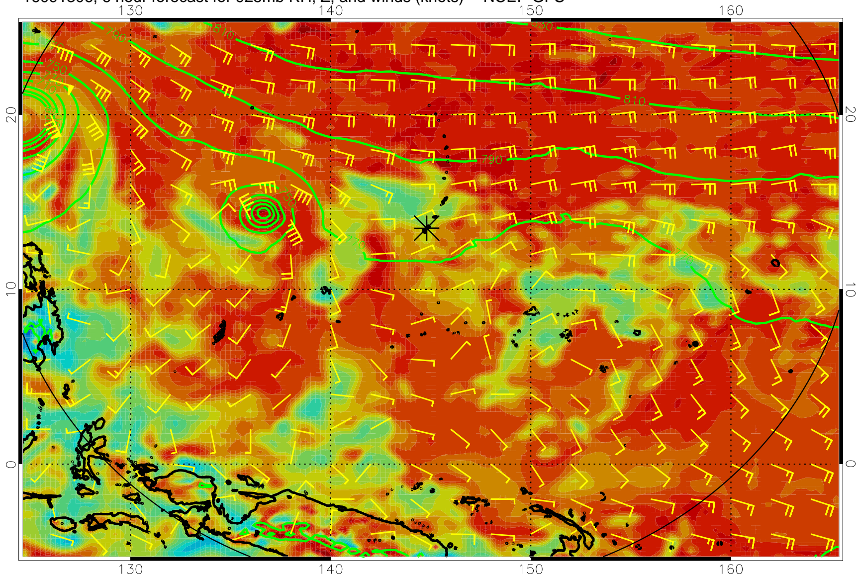
16091306, 6 hour forecast for 925mb RH, Z, and winds (knots) -- NCEP GFS
