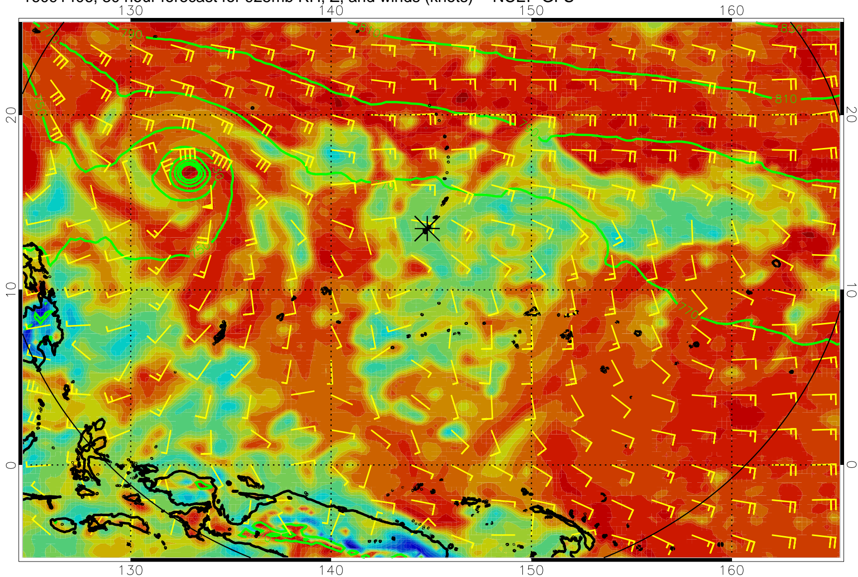
16091406, 30 hour forecast for 925mb RH, Z, and winds (knots) -- NCEP GFS
