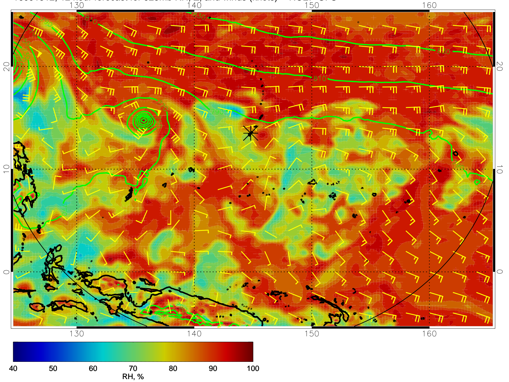
16091312, 12 hour forecast for 925mb RH, Z, and winds (knots) -- NCEP GFS
