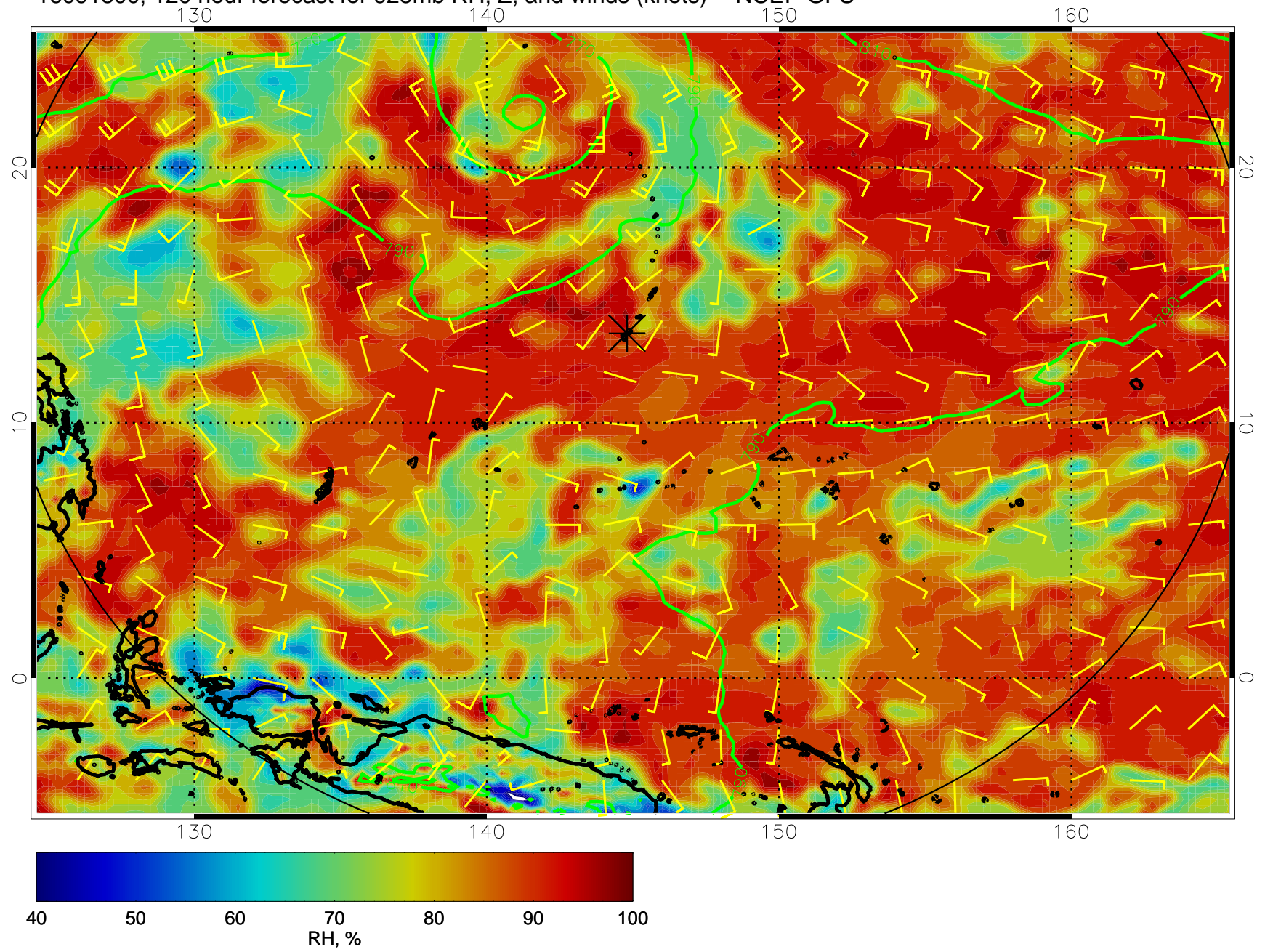
16091800, 120 hour forecast for 925mb RH, Z, and winds (knots) -- NCEP GFS
