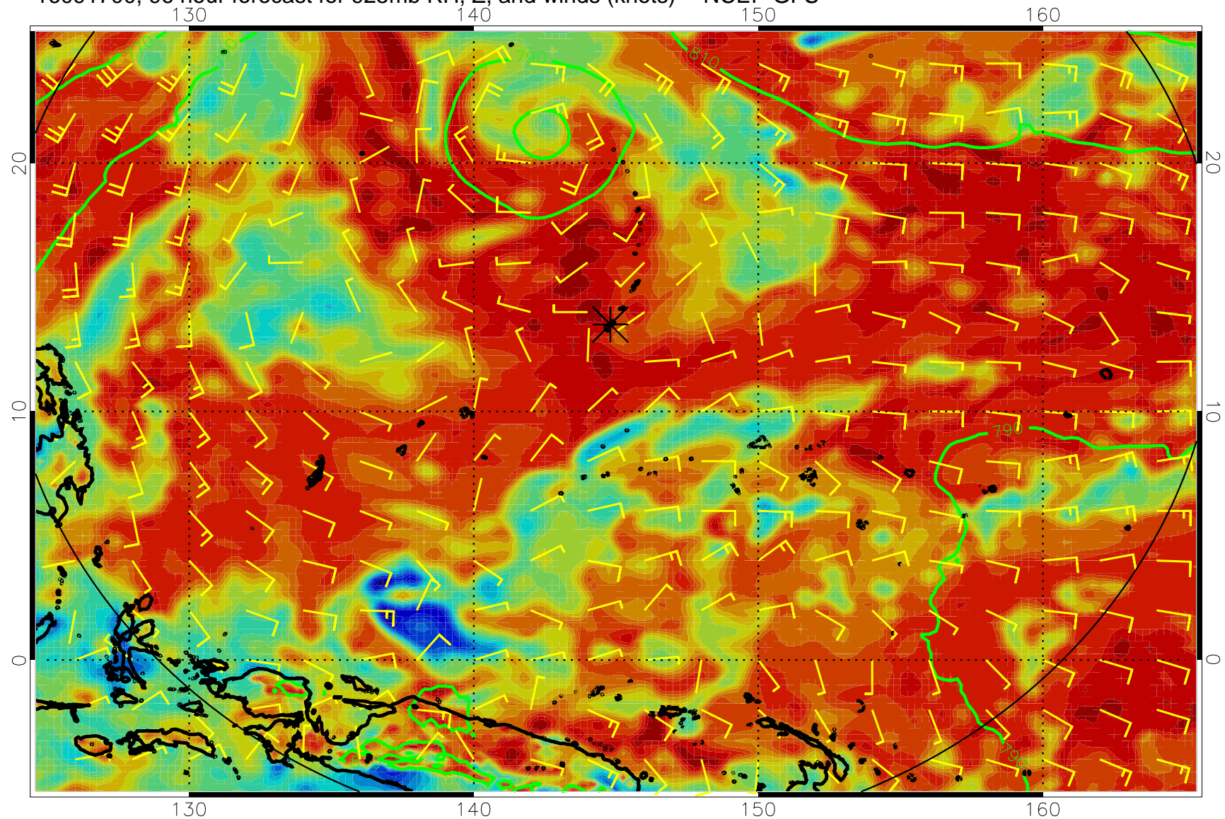
16091700, 96 hour forecast for 925mb RH, Z, and winds (knots) -- NCEP GFS
