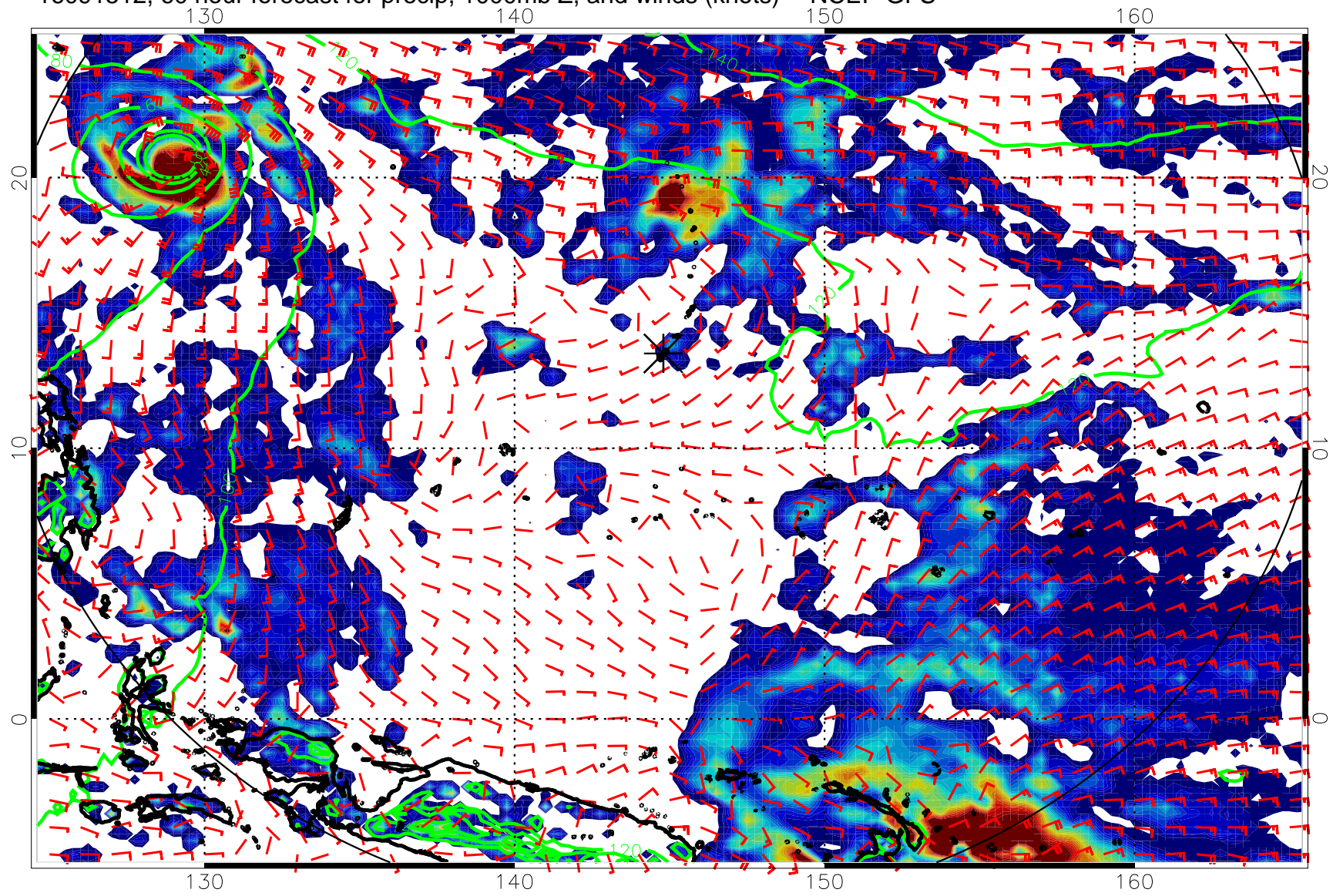
16091512, 60 hour forecast for precip, 1000mb Z, and winds (knots) -- NCEP GFS
