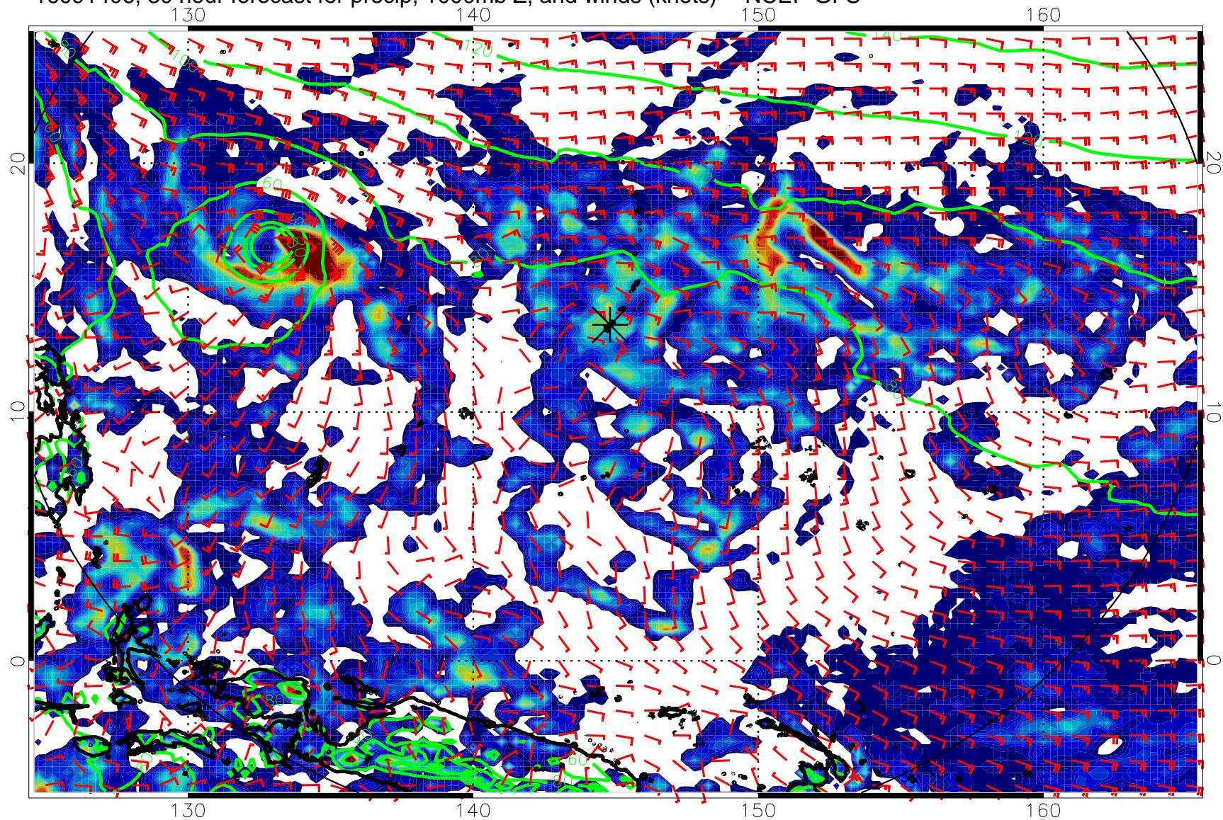
16091406, 30 hour forecast for precip, 1000mb Z, and winds (knots) -- NCEP GFS
