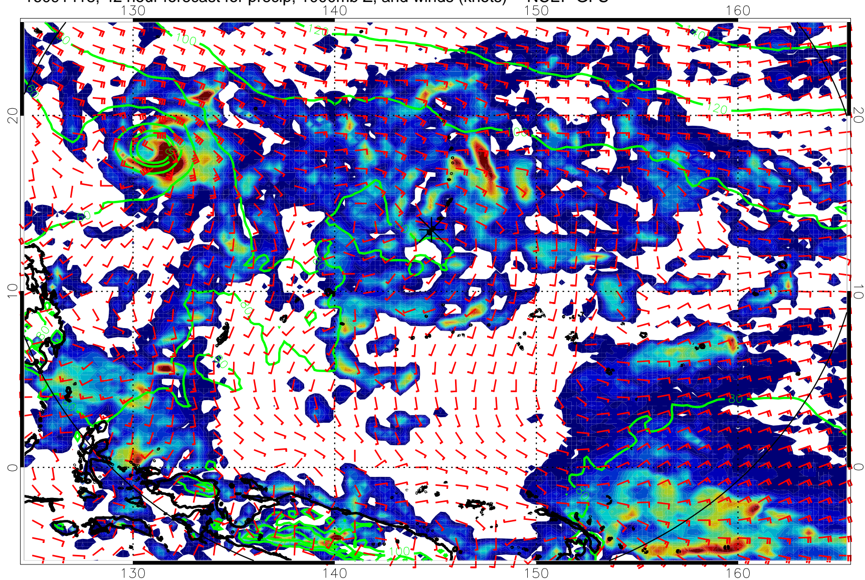
16091418, 42 hour forecast for precip, 1000mb Z, and winds (knots) -- NCEP GFS
