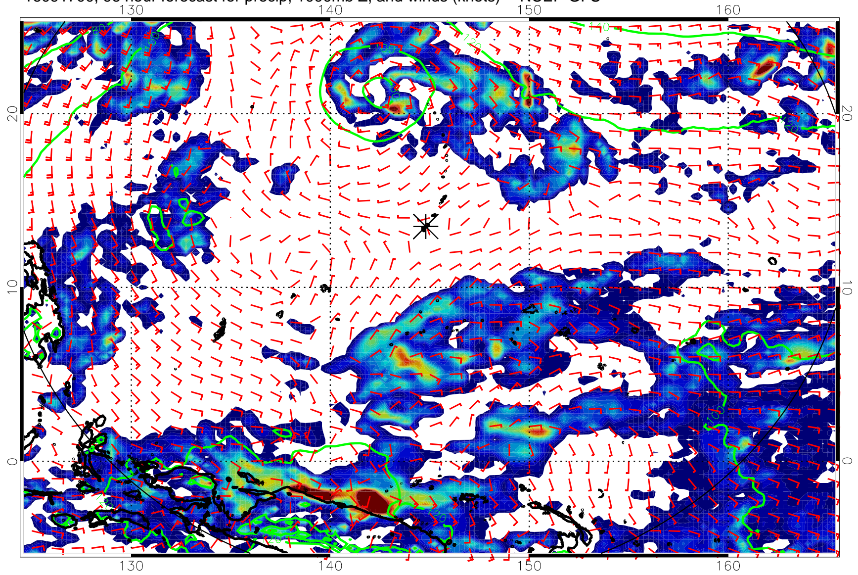
16091700, 96 hour forecast for precip, 1000mb Z, and winds (knots) -- NCEP GFS
