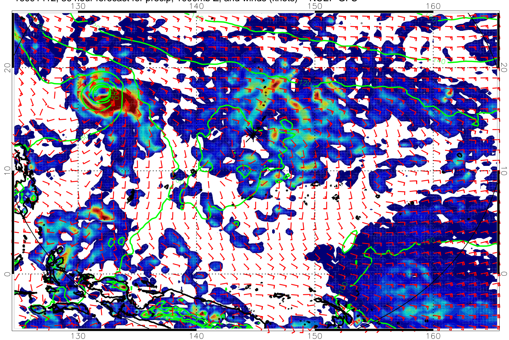
16091412, 36 hour forecast for precip, 1000mb Z, and winds (knots) -- NCEP GFS
