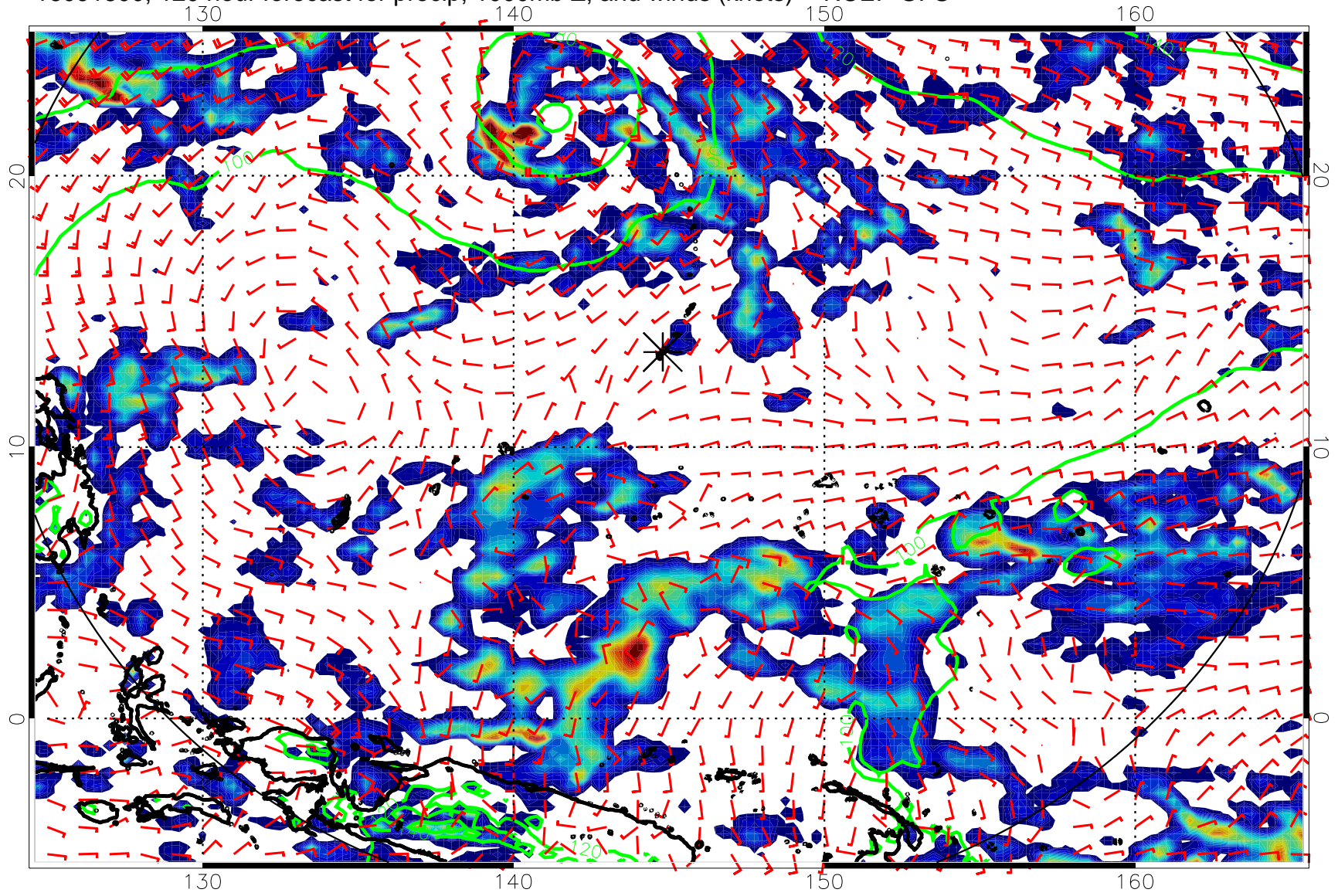
16091800, 120 hour forecast for precip, 1000mb Z, and winds (knots) -- NCEP GFS
