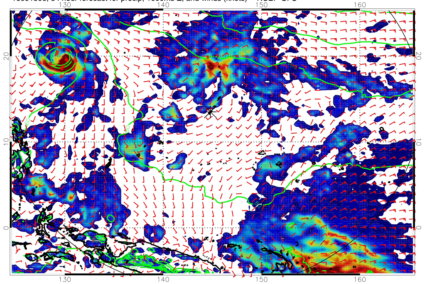
16091506, 54 hour forecast for precip, 1000mb Z, and winds (knots) -- NCEP GFS
