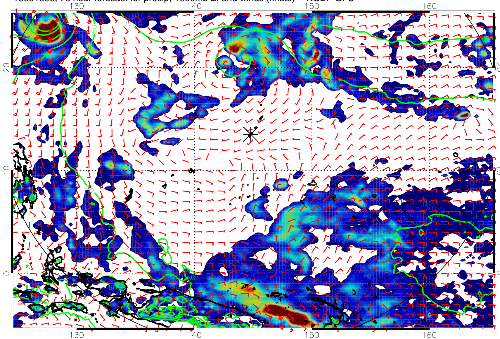
16091606, 78 hour forecast for precip, 1000mb Z, and winds (knots) -- NCEP GFS
