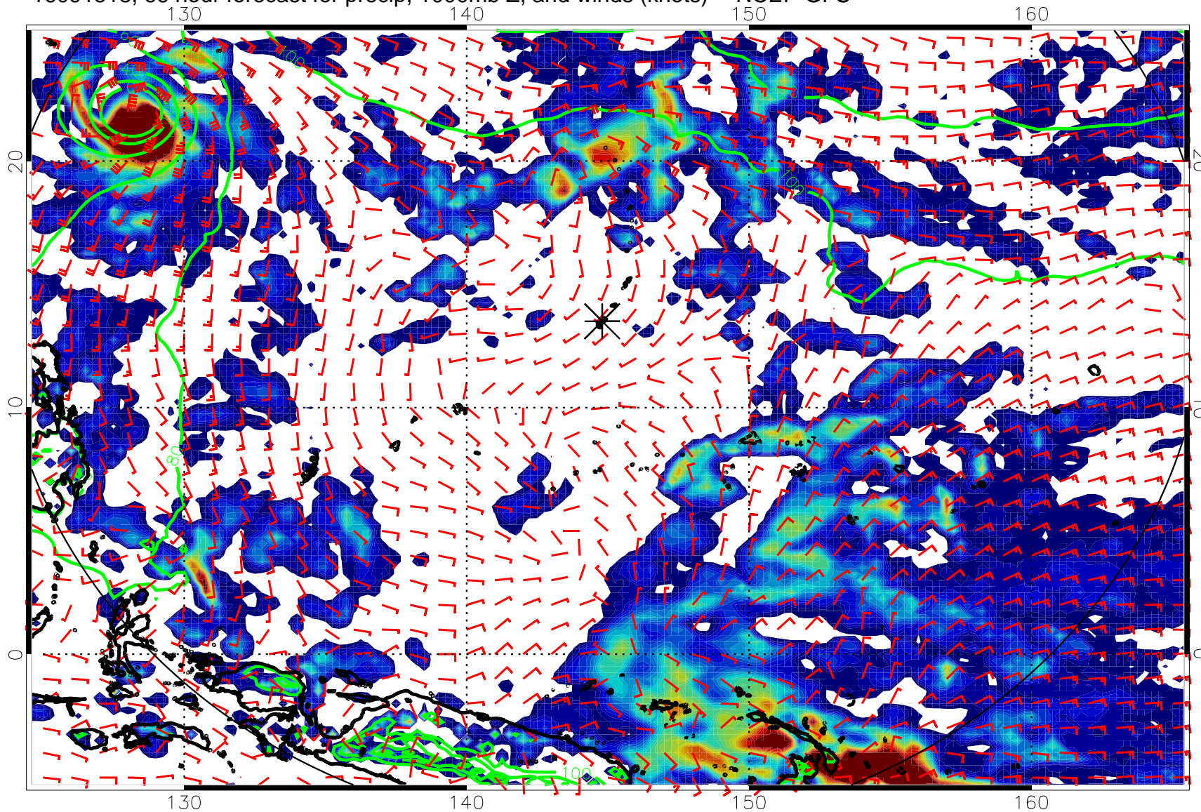
16091518, 66 hour forecast for precip, 1000mb Z, and winds (knots) -- NCEP GFS
