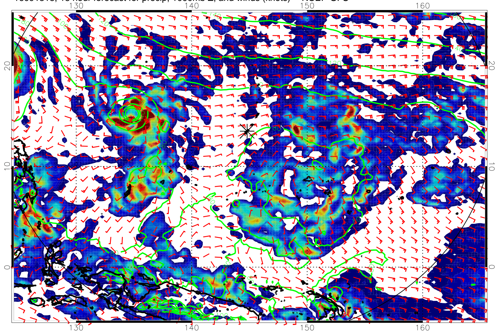
16091318, 18 hour forecast for precip, 1000mb Z, and winds (knots) -- NCEP GFS
