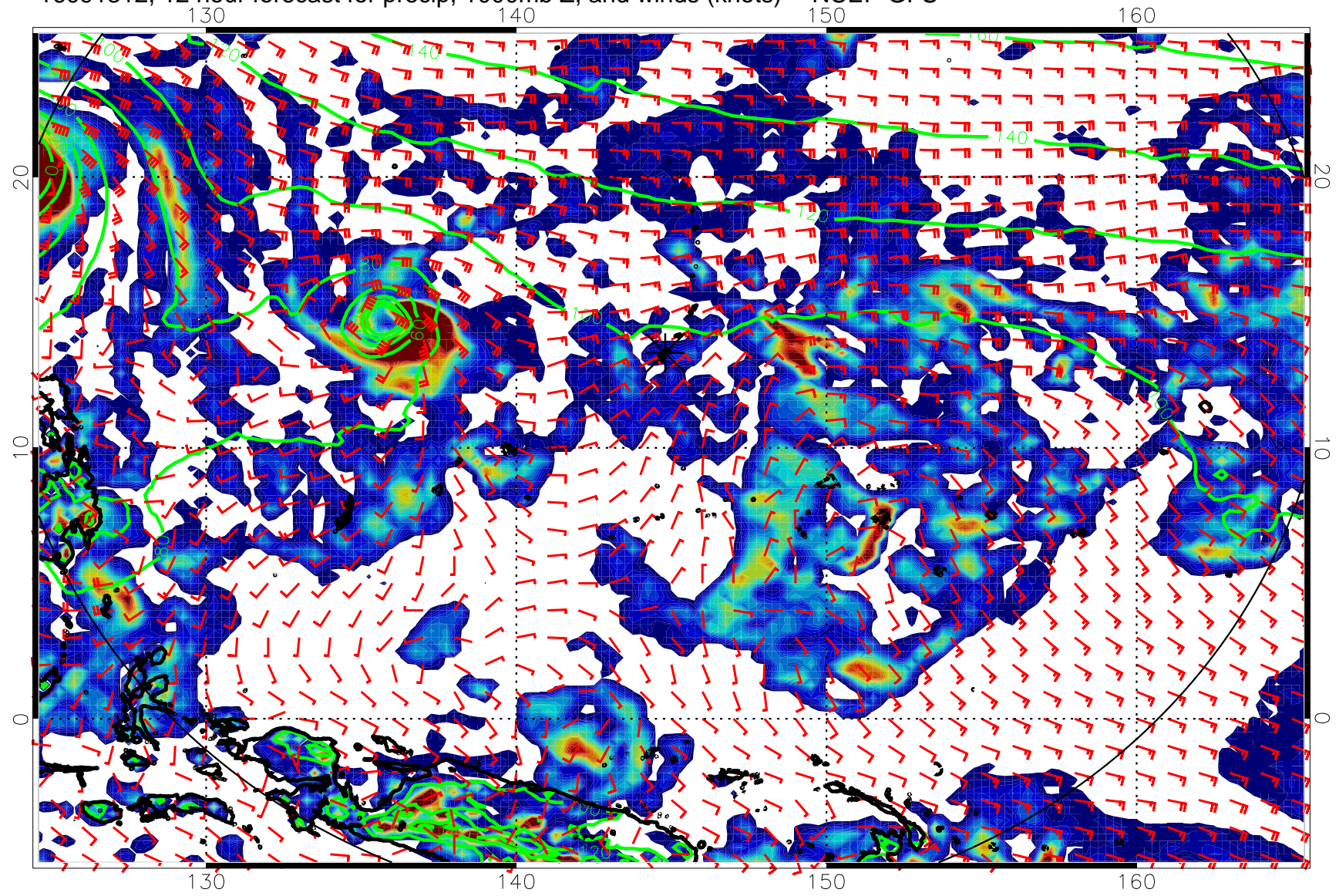
16091312, 12 hour forecast for precip, 1000mb Z, and winds (knots) -- NCEP GFS
