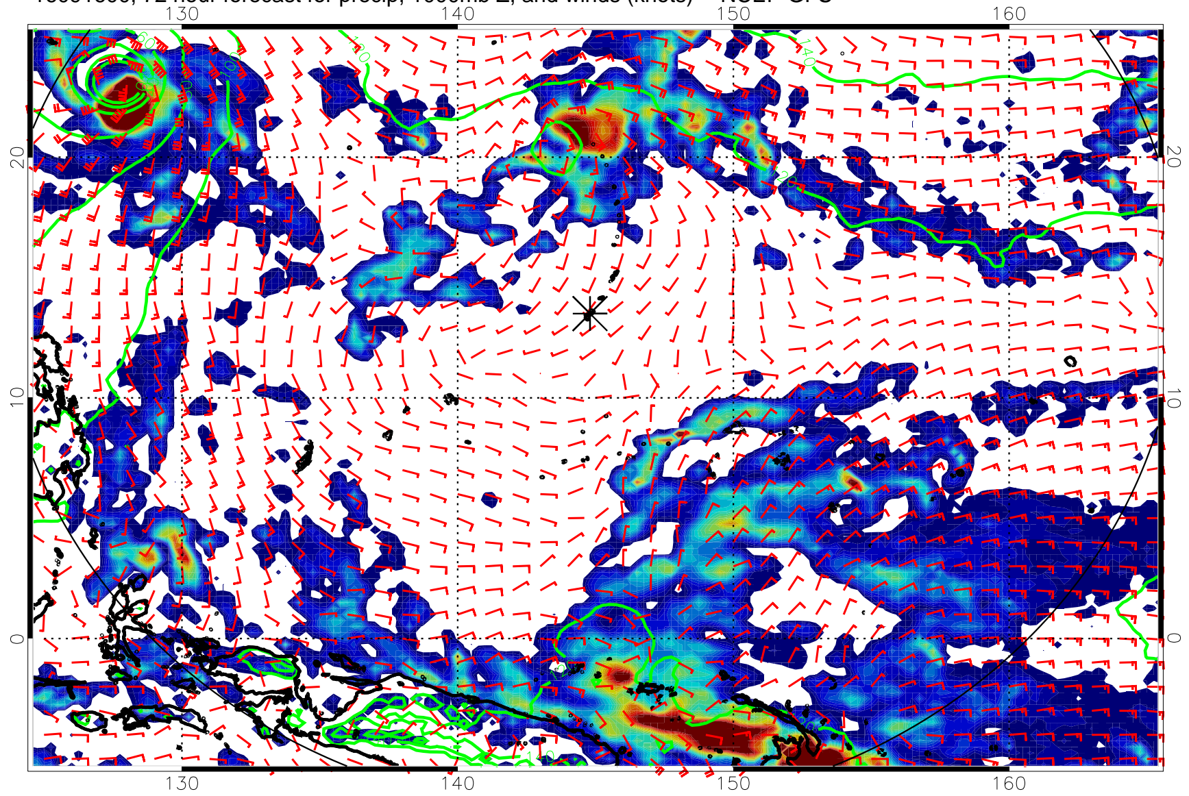
16091600, 72 hour forecast for precip, 1000mb Z, and winds (knots) -- NCEP GFS
