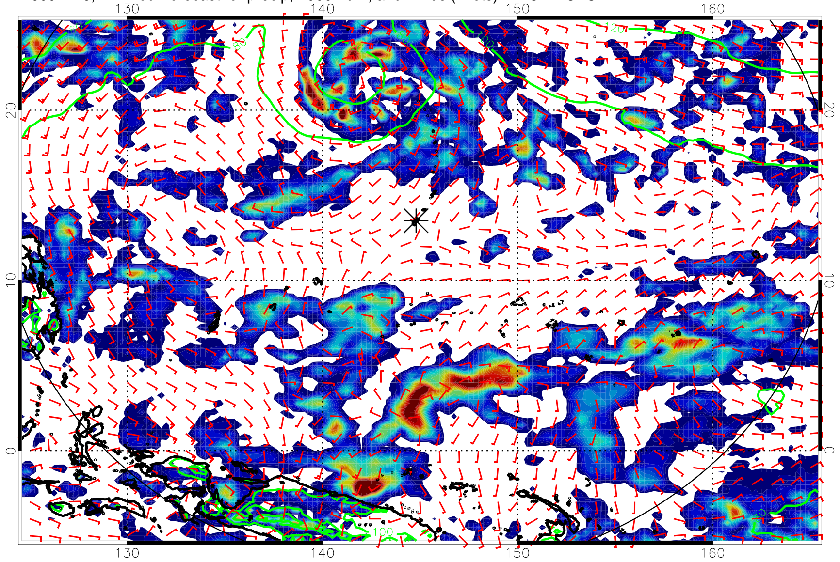
16091718, 114 hour forecast for precip, 1000mb Z, and winds (knots) -- NCEP GFS
