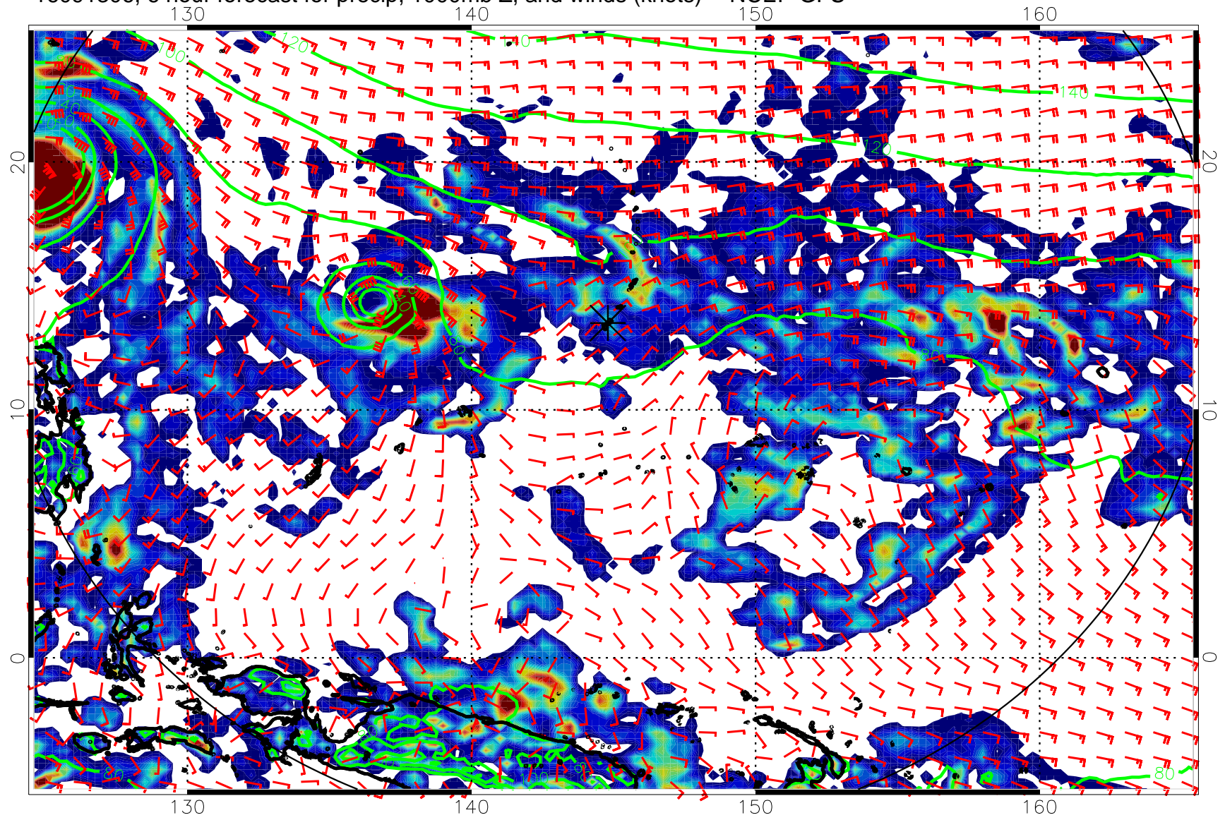
16091306, 6 hour forecast for precip, 1000mb Z, and winds (knots) -- NCEP GFS
