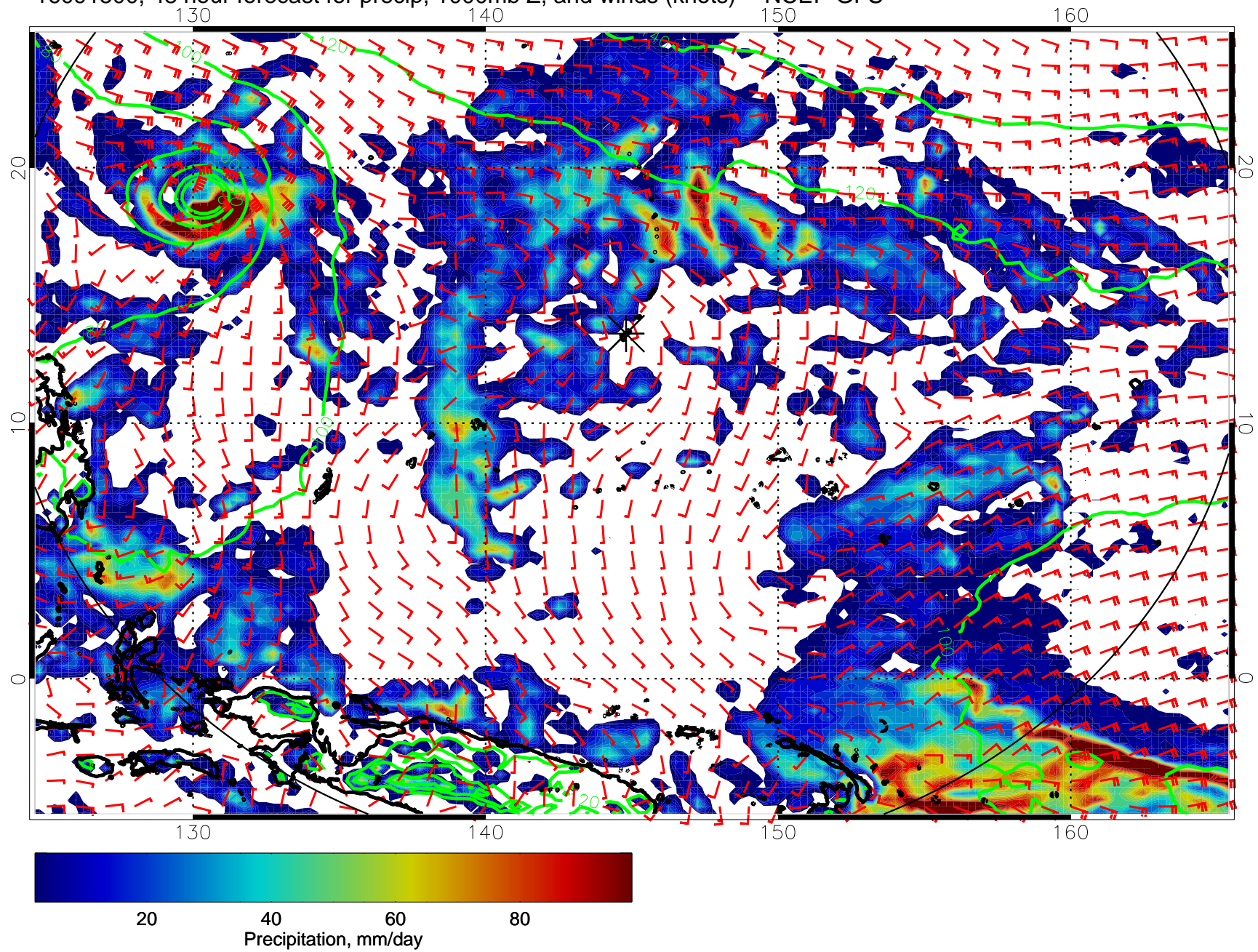
16091500, 48 hour forecast for precip, 1000mb Z, and winds (knots) -- NCEP GFS
