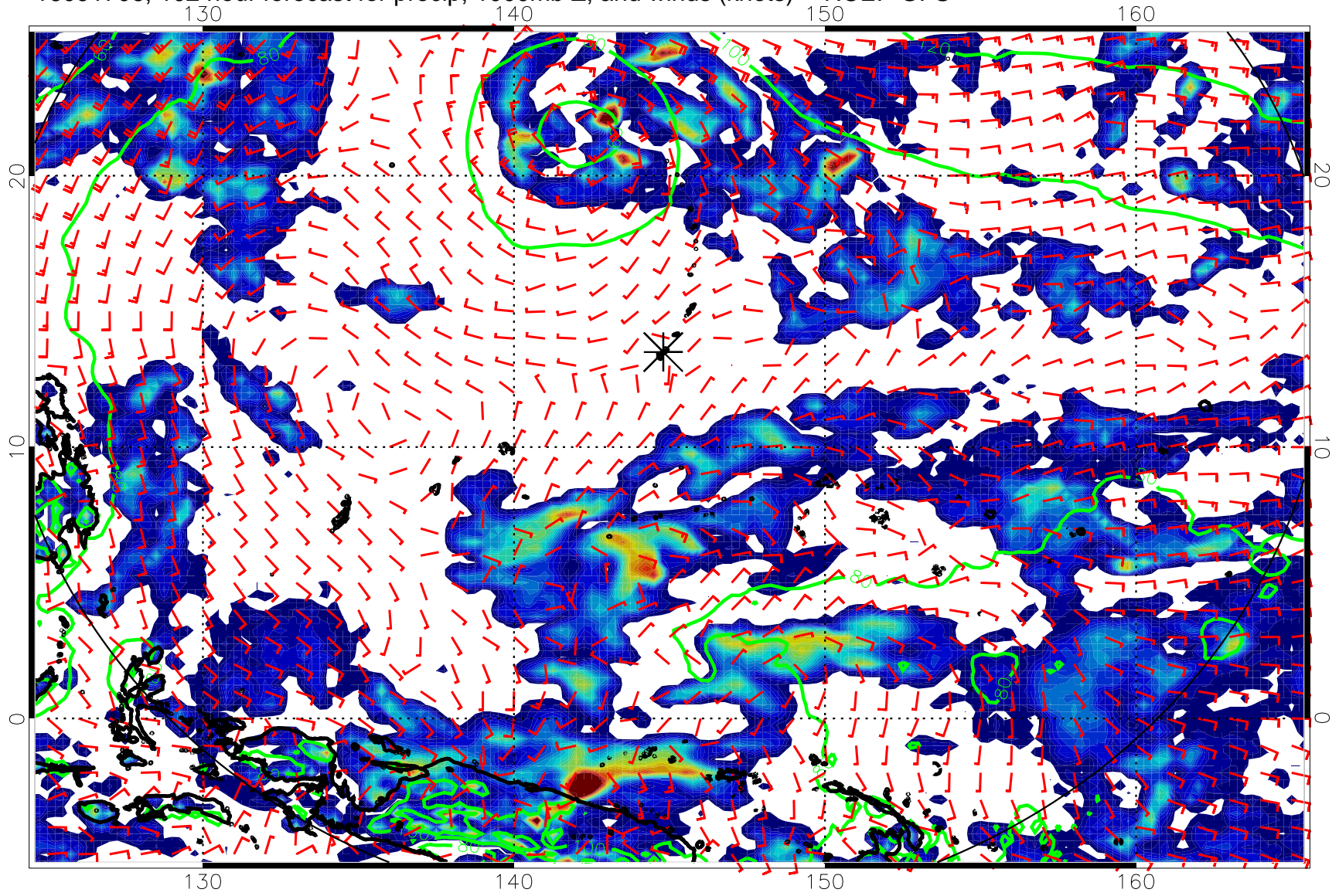
16091706, 102 hour forecast for precip, 1000mb Z, and winds (knots) -- NCEP GFS
