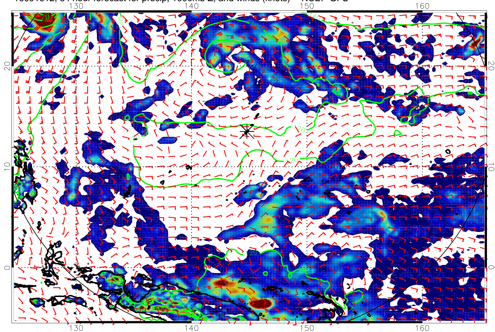
16091612, 84 hour forecast for precip, 1000mb Z, and winds (knots) -- NCEP GFS
