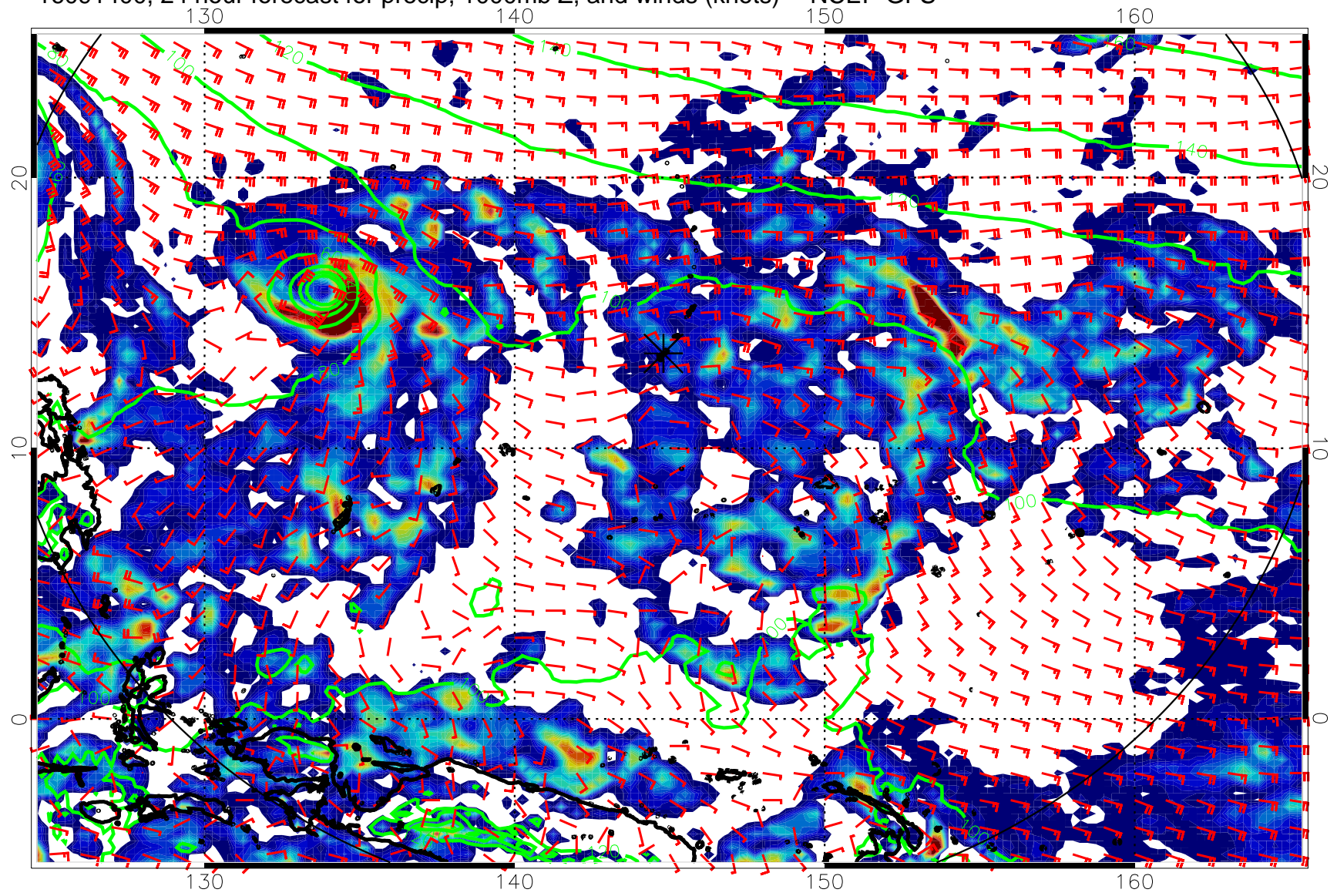
16091400, 24 hour forecast for precip, 1000mb Z, and winds (knots) -- NCEP GFS
