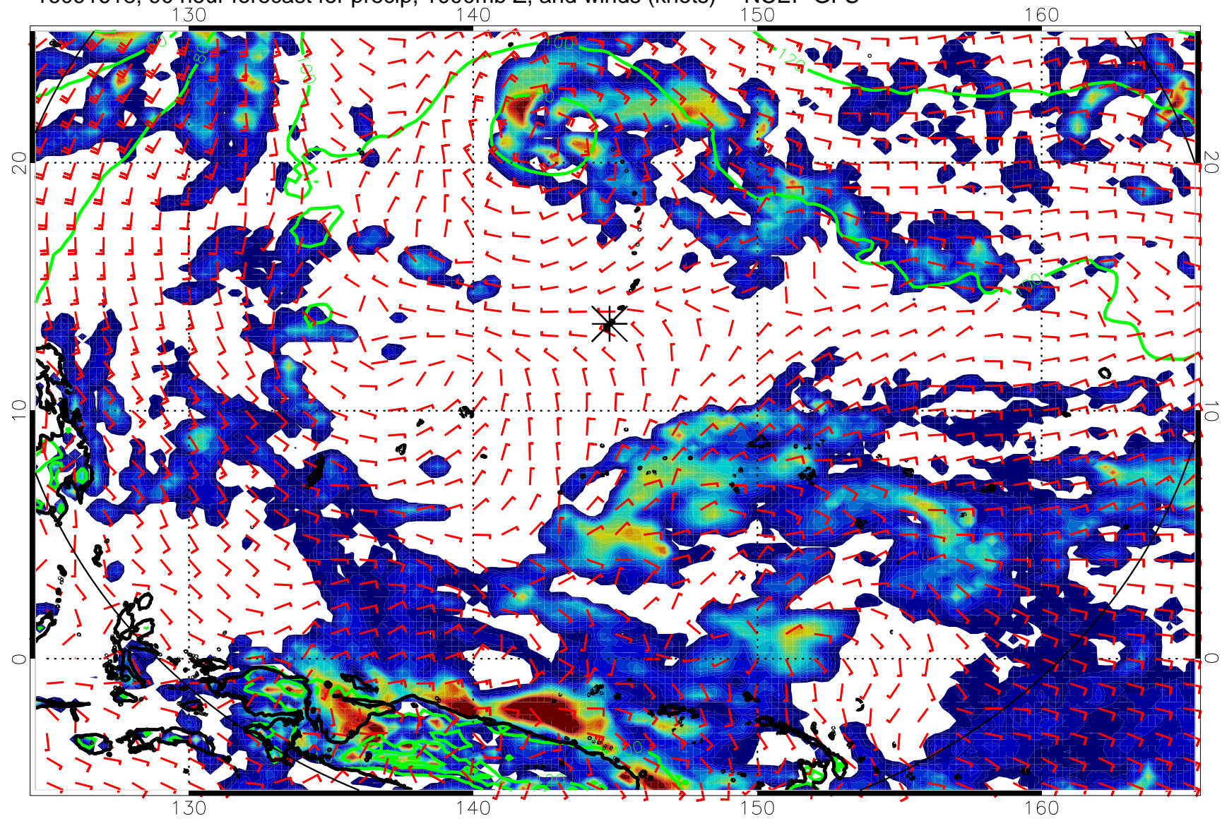
16091618, 90 hour forecast for precip, 1000mb Z, and winds (knots) -- NCEP GFS
