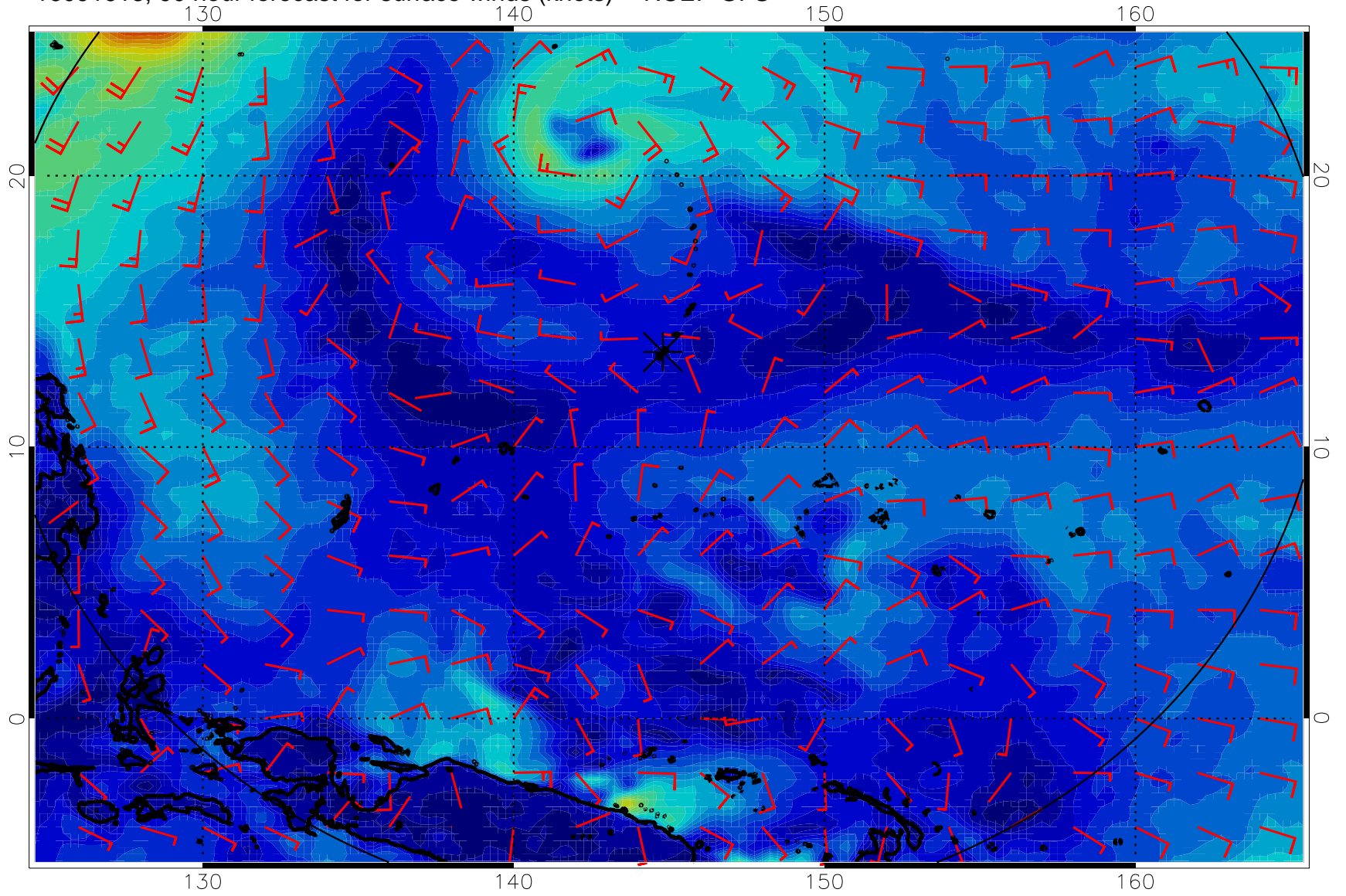
16091618, 90 hour forecast for surface winds (knots) -- NCEP GFS
