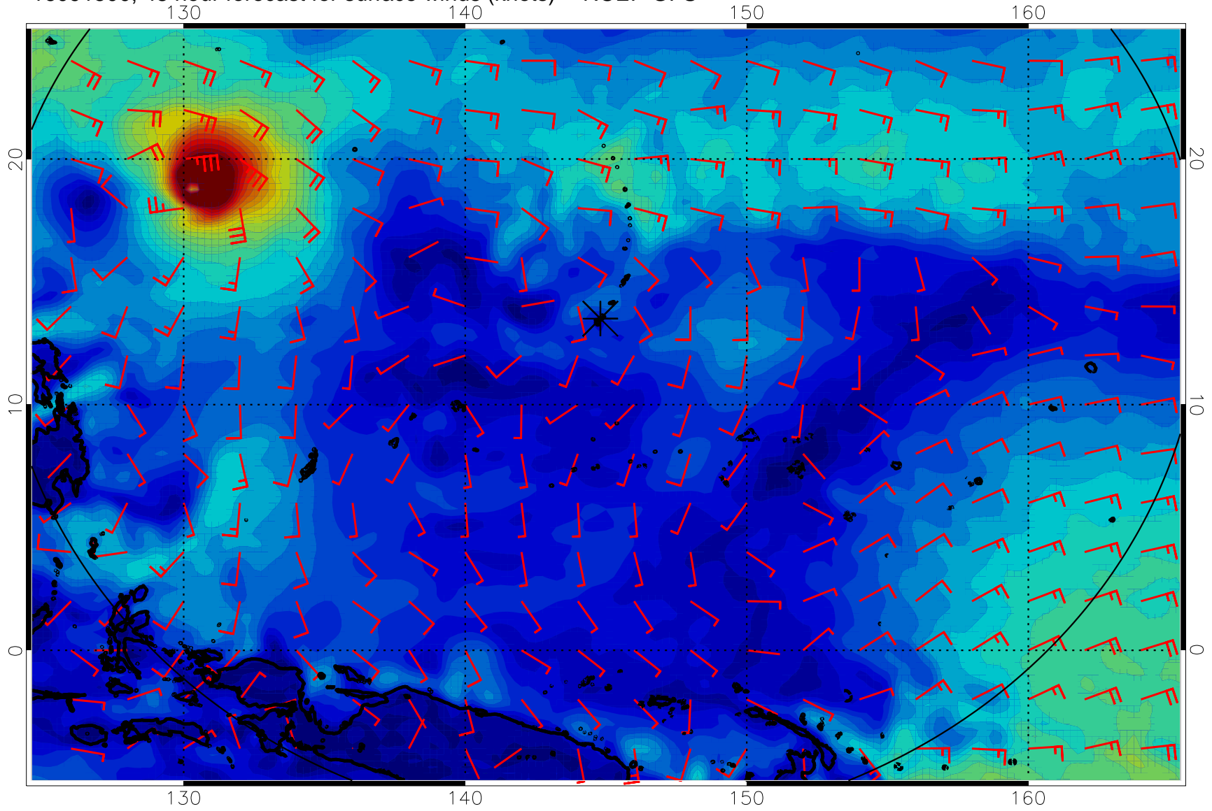
16091500, 48 hour forecast for surface winds (knots) -- NCEP GFS
