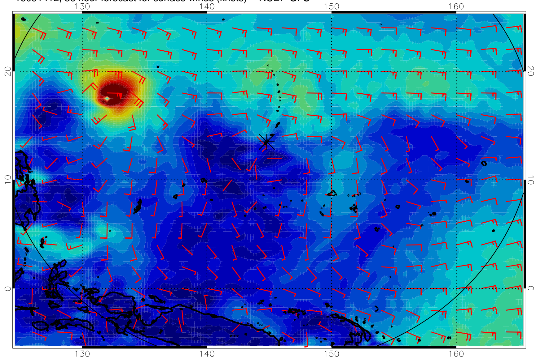
16091412, 36 hour forecast for surface winds (knots) -- NCEP GFS
