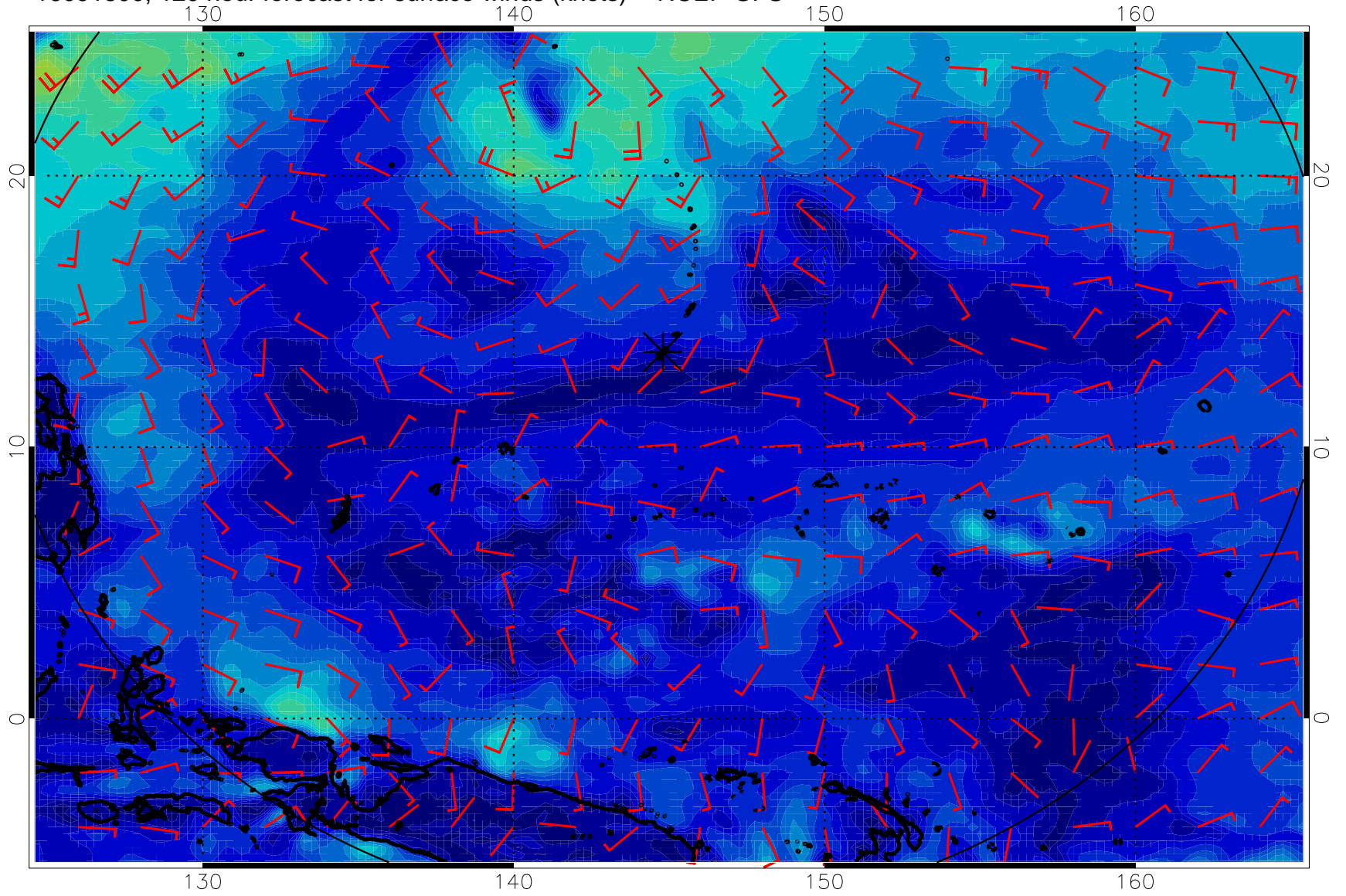
16091800, 120 hour forecast for surface winds (knots) -- NCEP GFS
