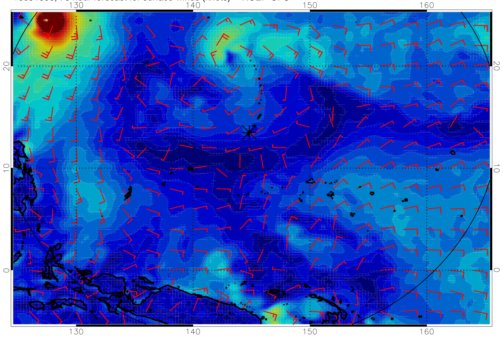
16091606, 78 hour forecast for surface winds (knots) -- NCEP GFS
