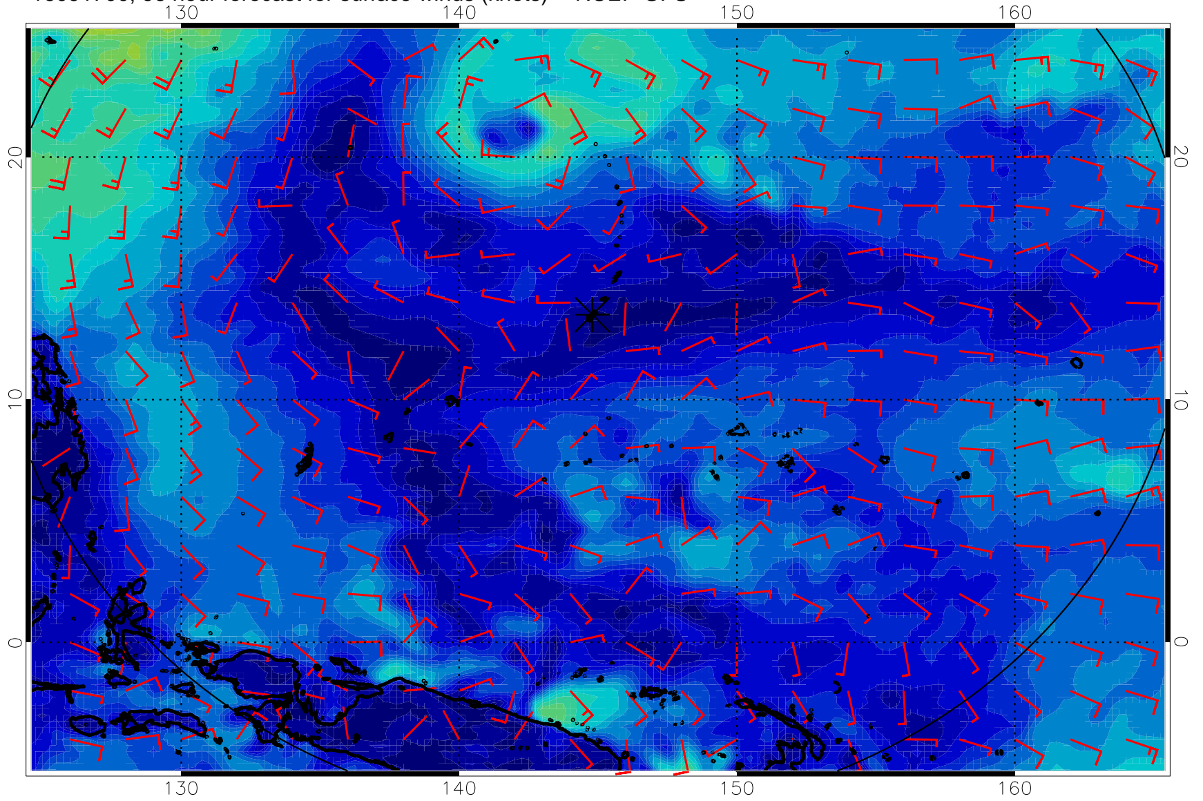
16091700, 96 hour forecast for surface winds (knots) -- NCEP GFS
