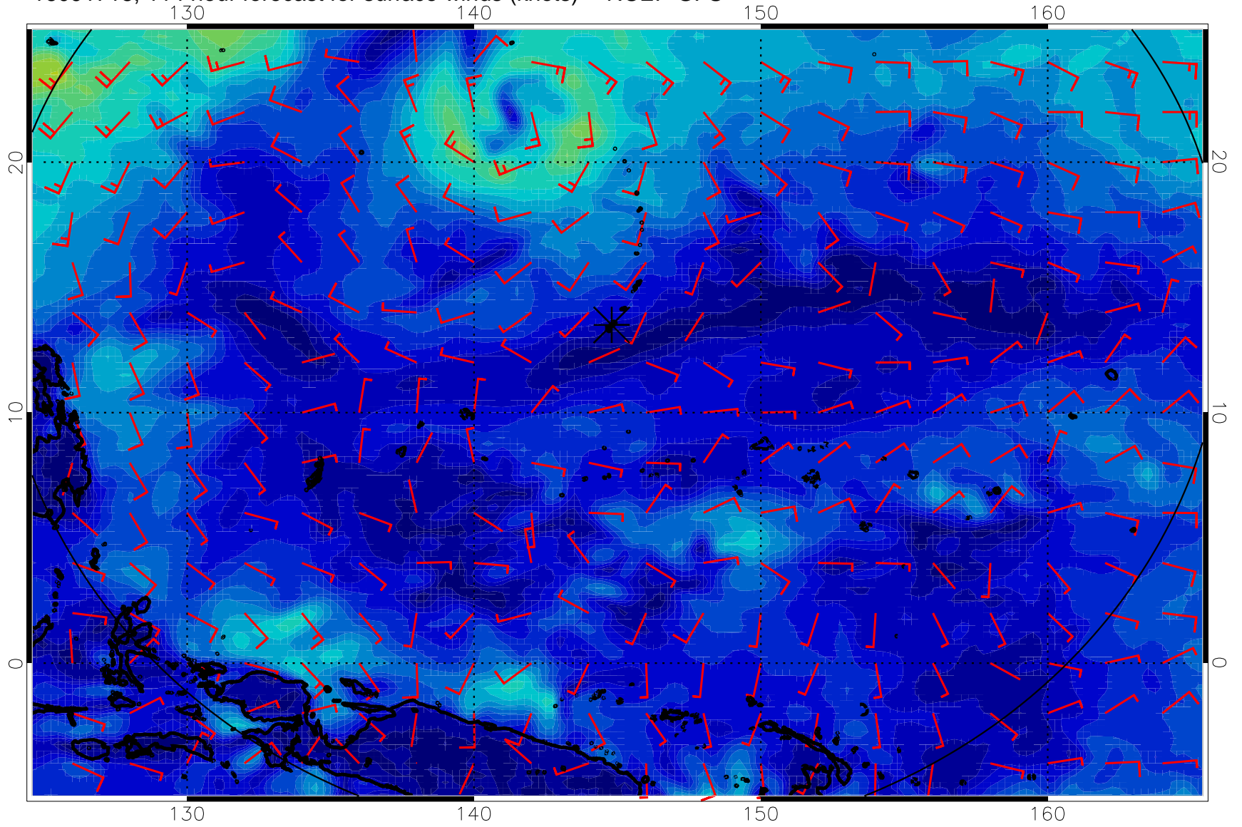
16091718, 114 hour forecast for surface winds (knots) -- NCEP GFS
