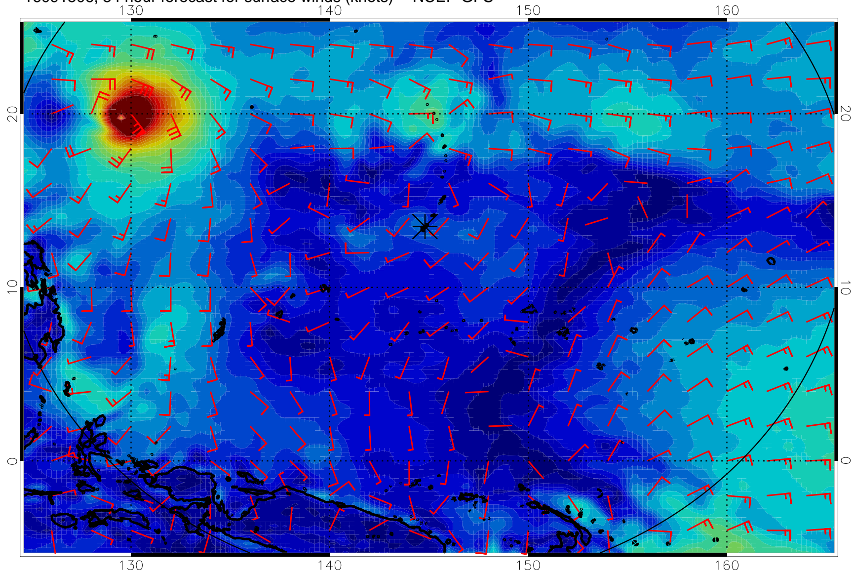
16091506, 54 hour forecast for surface winds (knots) -- NCEP GFS
