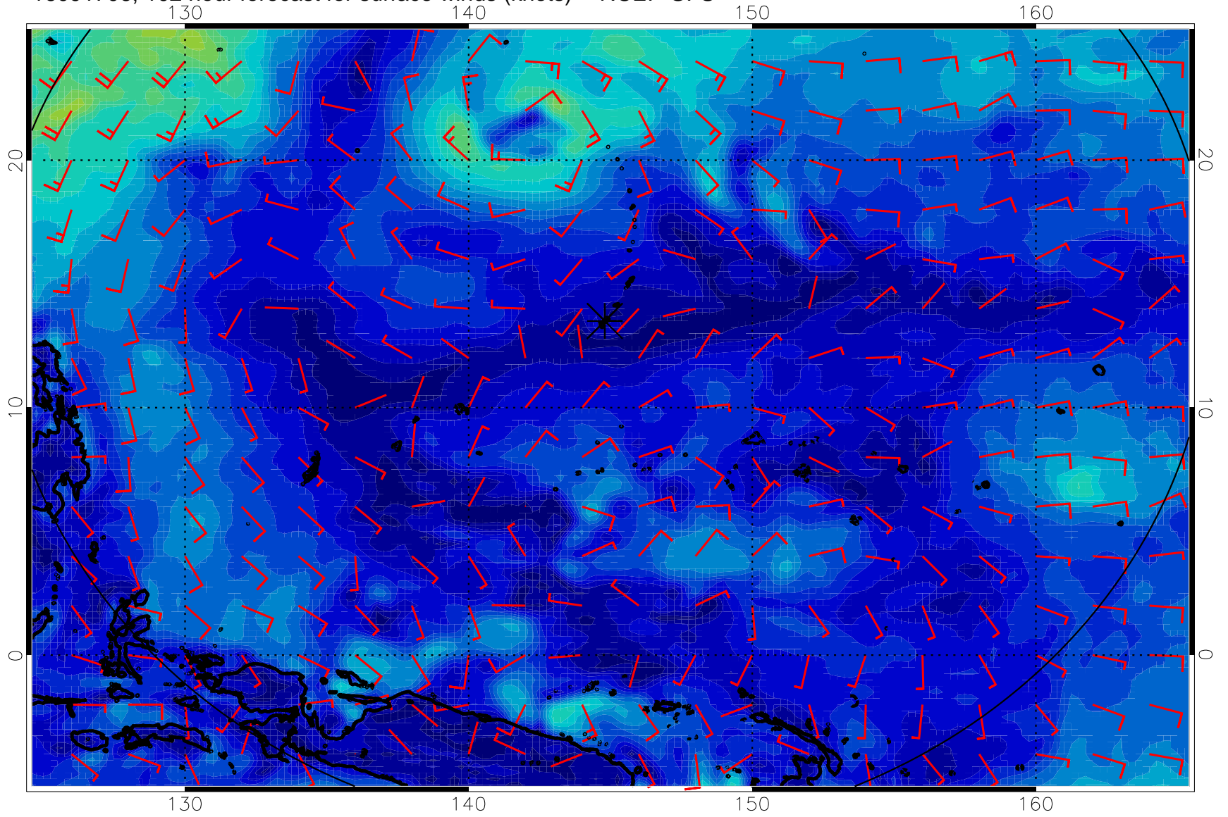
16091706, 102 hour forecast for surface winds (knots) -- NCEP GFS
