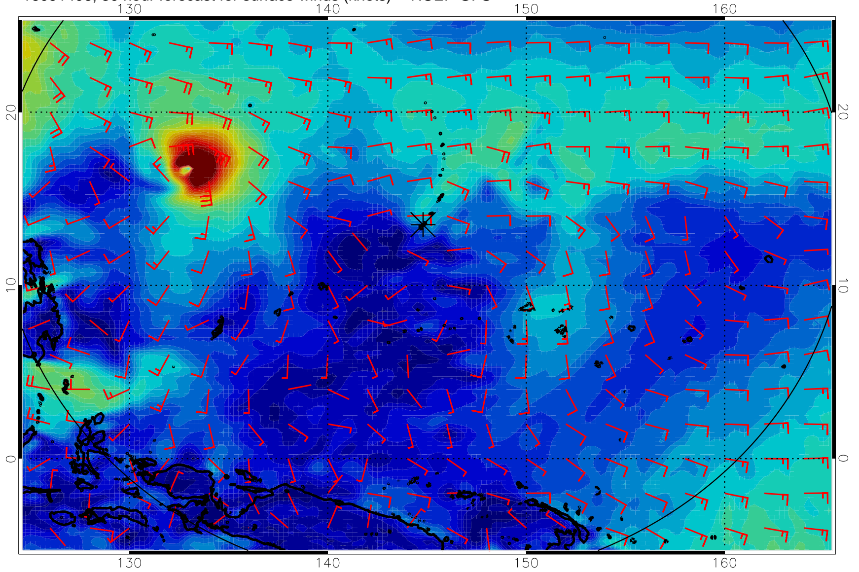
16091406, 30 hour forecast for surface winds (knots) -- NCEP GFS
