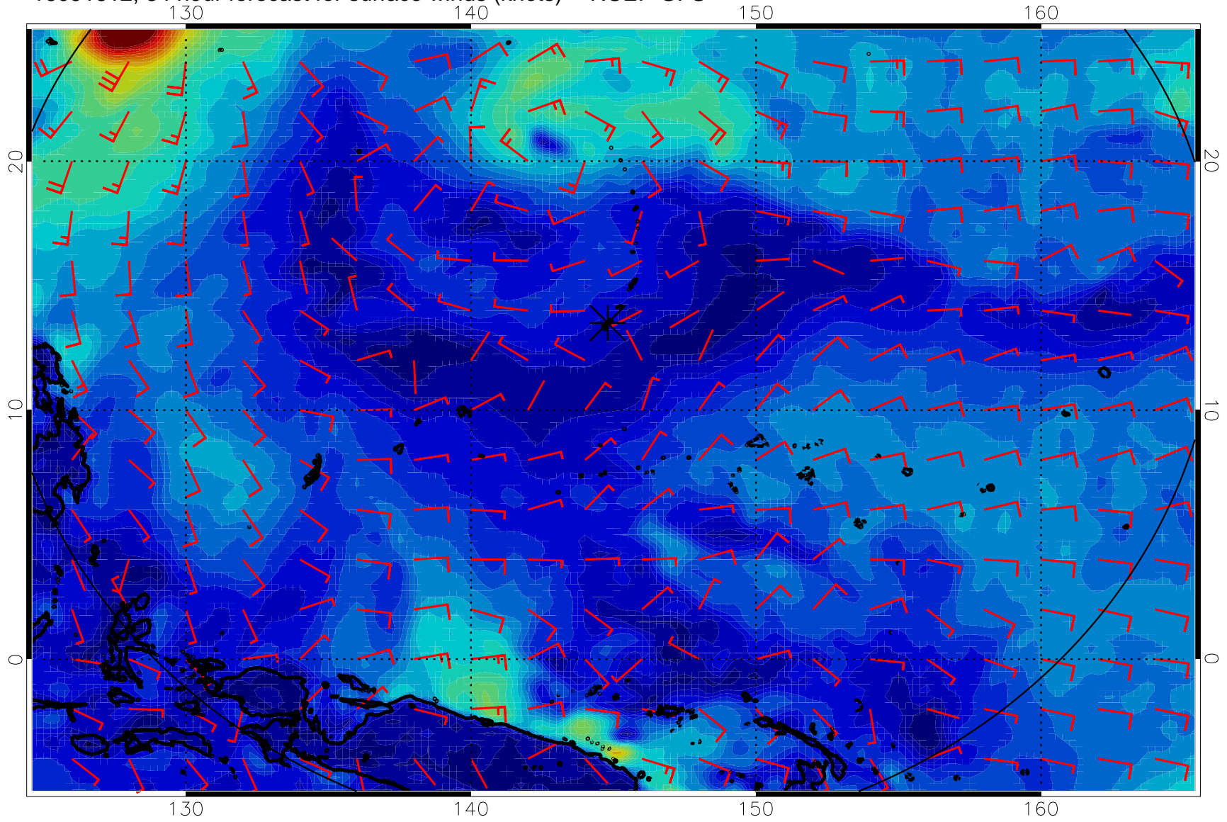
16091612, 84 hour forecast for surface winds (knots) -- NCEP GFS
