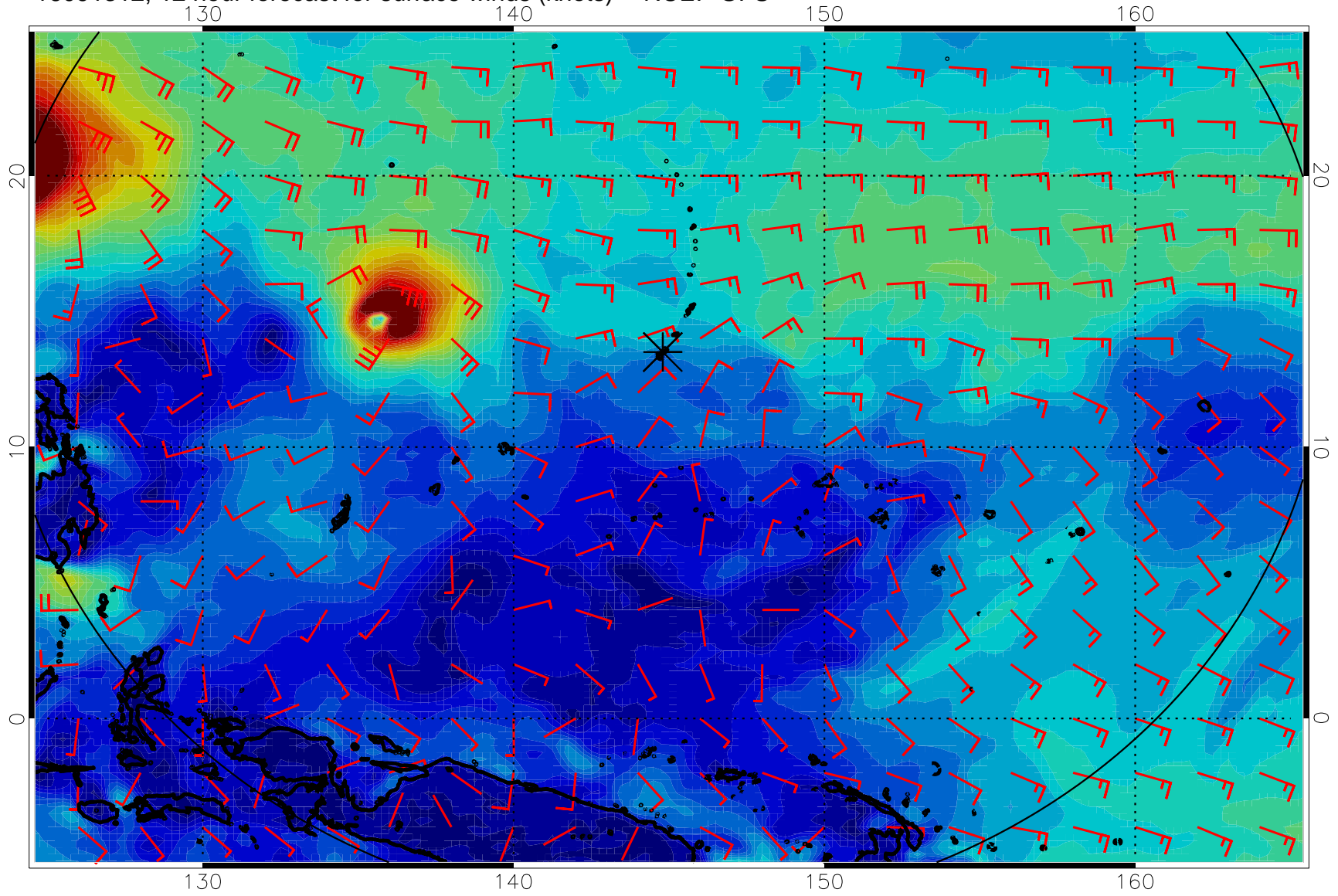
16091312, 12 hour forecast for surface winds (knots) -- NCEP GFS
