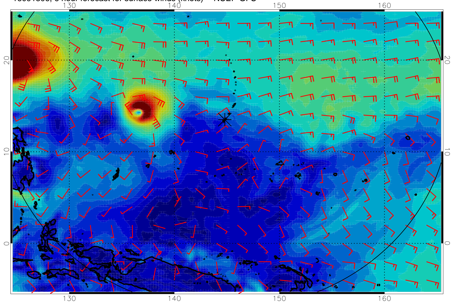
16091306, 6 hour forecast for surface winds (knots) -- NCEP GFS
