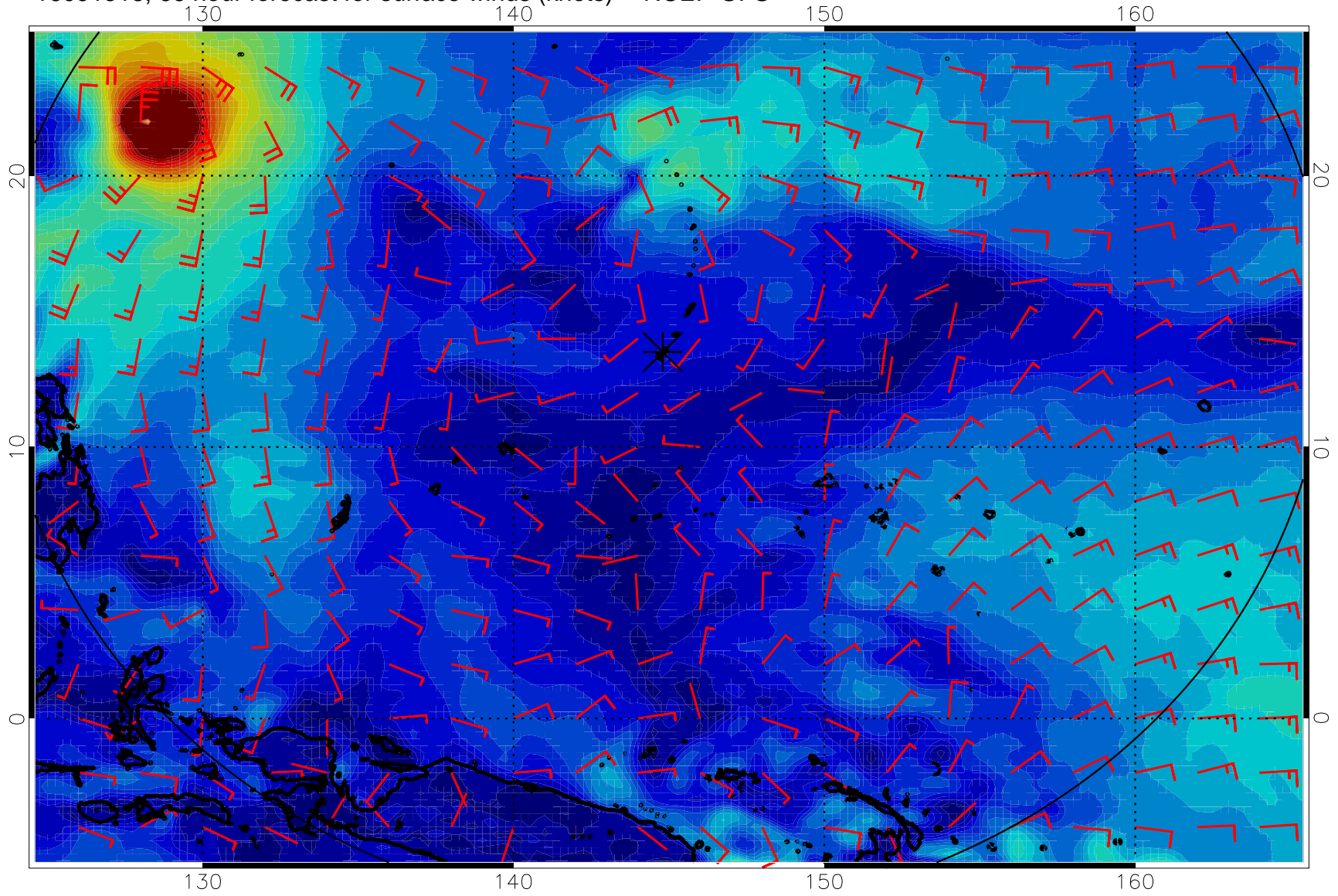
16091518, 66 hour forecast for surface winds (knots) -- NCEP GFS
