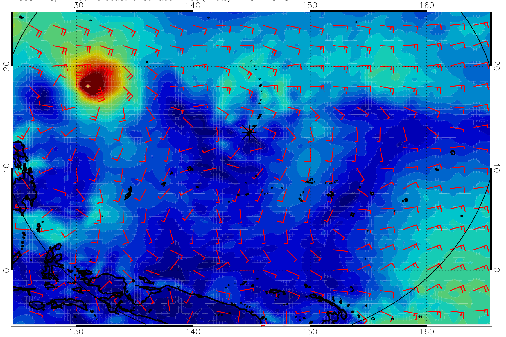
16091418, 42 hour forecast for surface winds (knots) -- NCEP GFS
