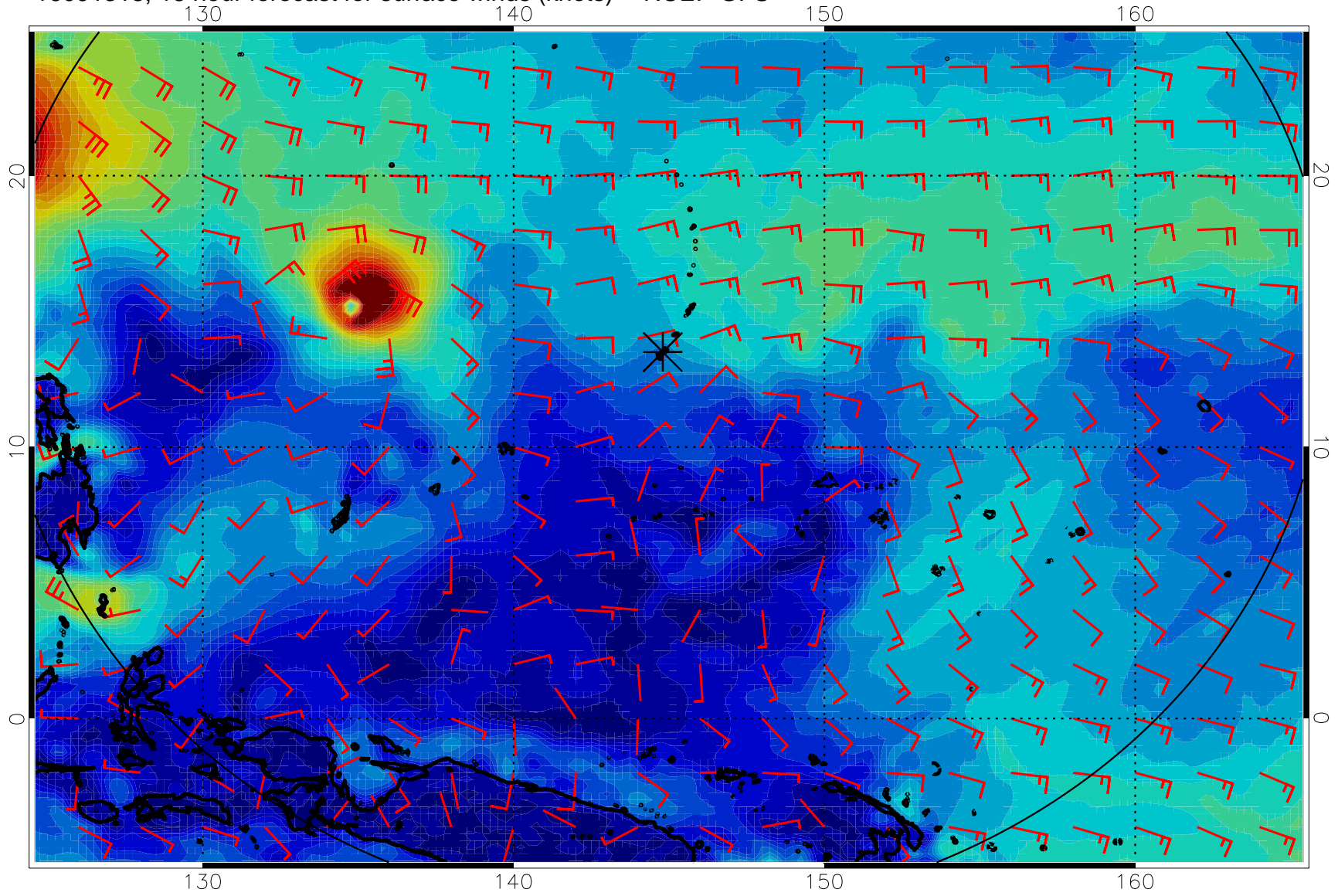
16091318, 18 hour forecast for surface winds (knots) -- NCEP GFS
