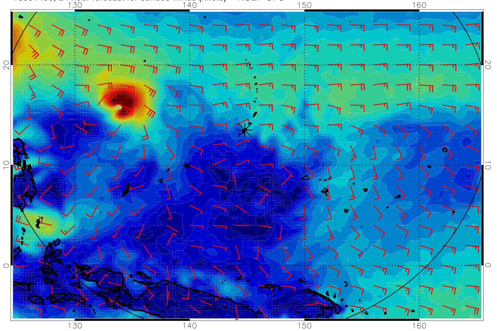
16091400, 24 hour forecast for surface winds (knots) -- NCEP GFS
