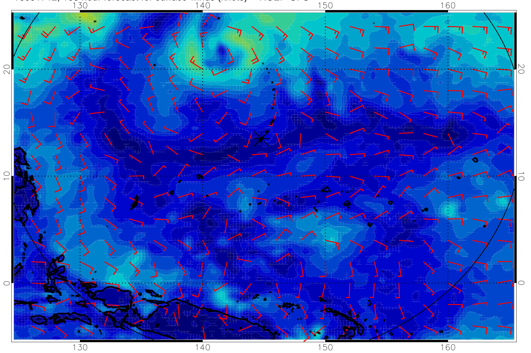
16091712, 108 hour forecast for surface winds (knots) -- NCEP GFS
