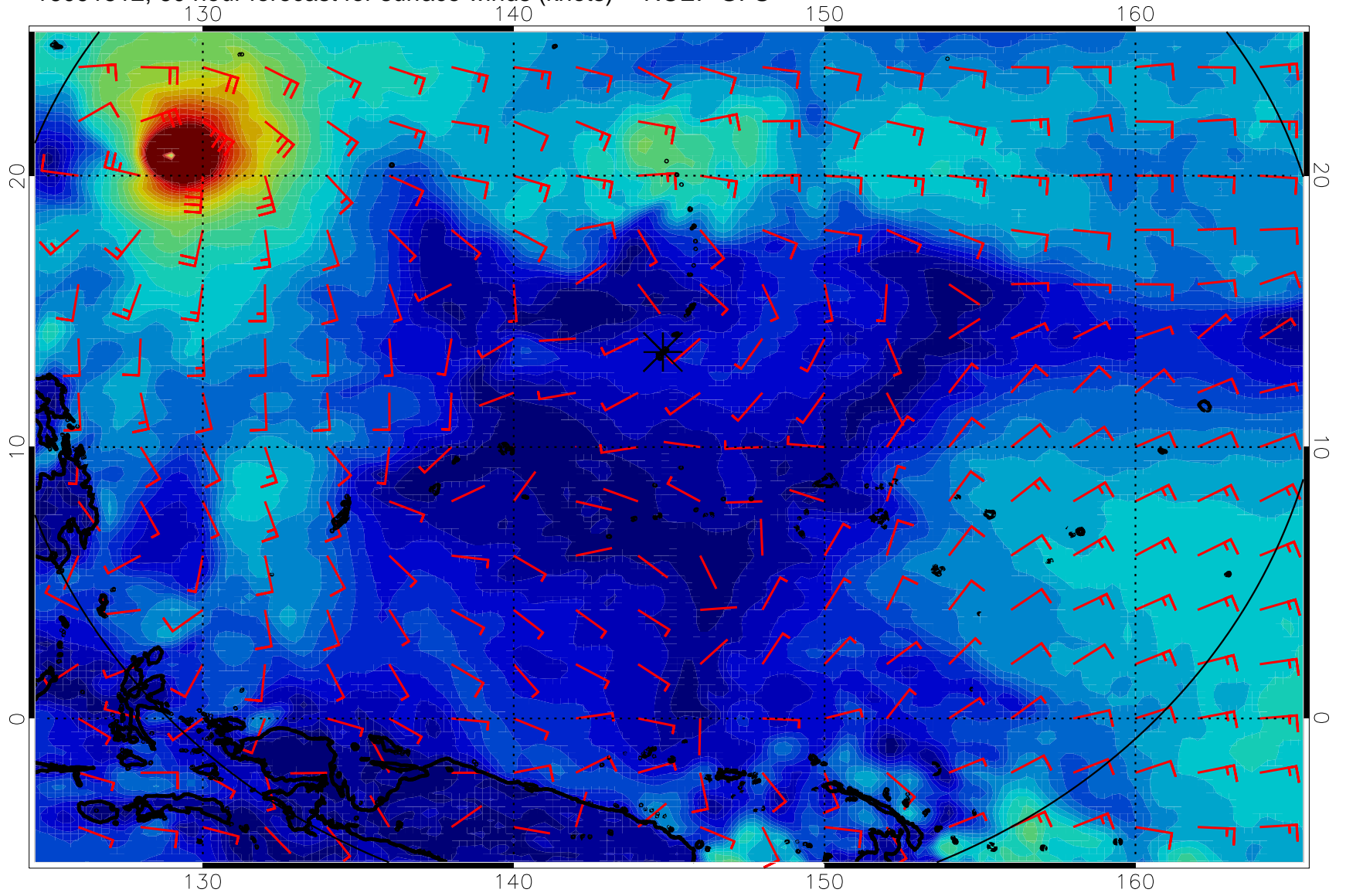
16091512, 60 hour forecast for surface winds (knots) -- NCEP GFS
