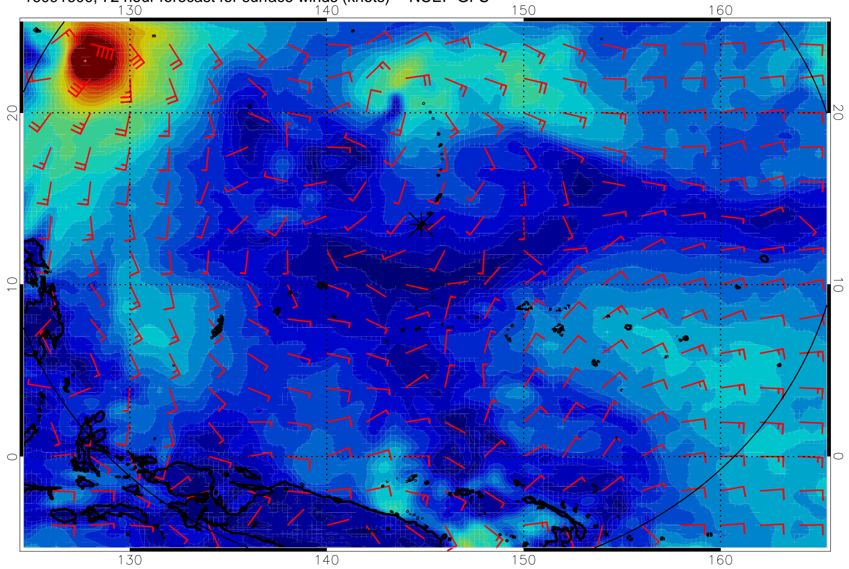
16091600, 72 hour forecast for surface winds (knots) -- NCEP GFS
